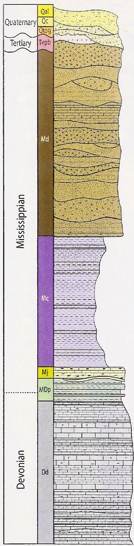
FIGURE 3.3-2 STRATIGRAPHIC COLUMN
