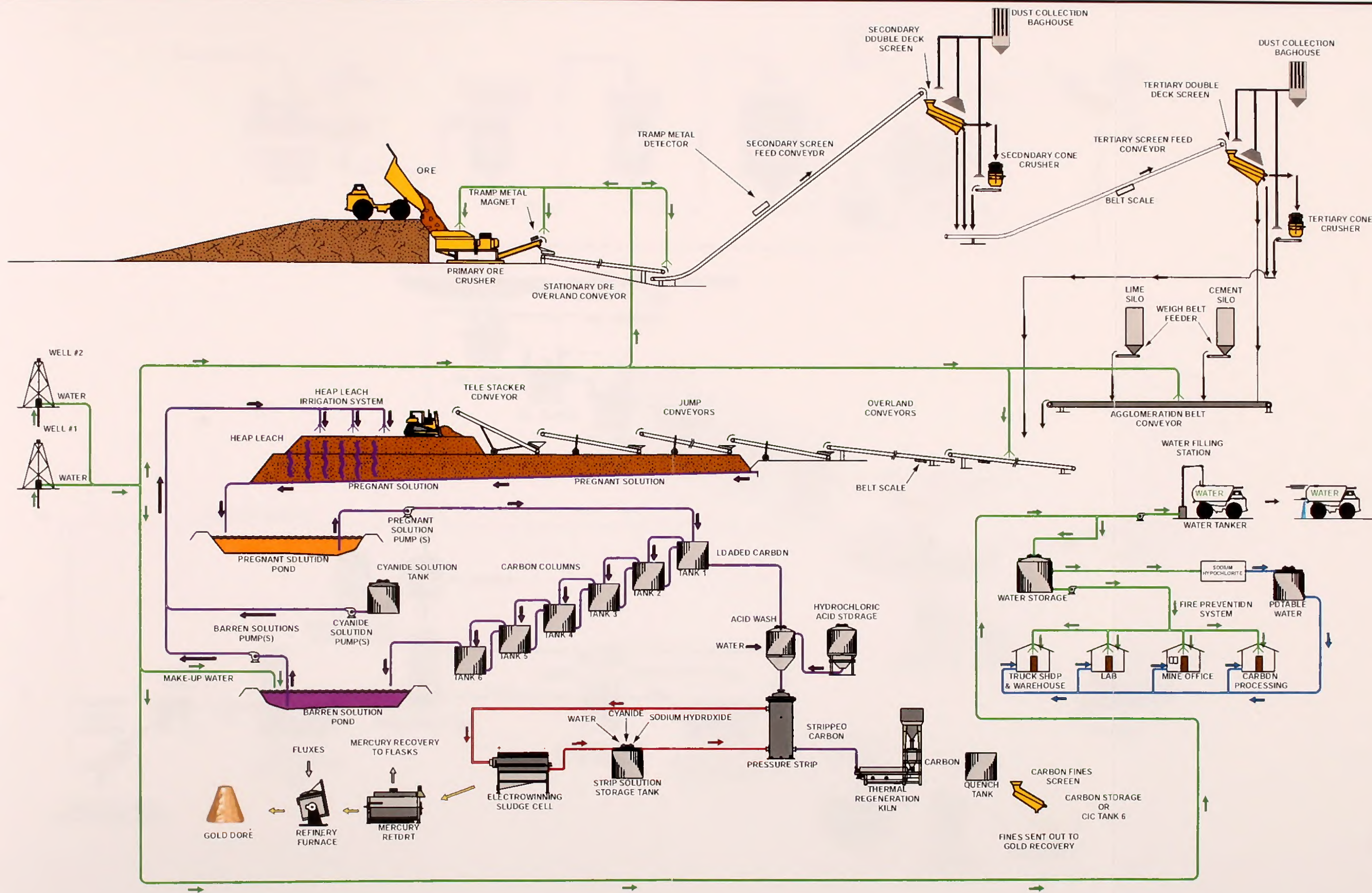
FIGURE 2.3-9 HEAP LEACH FLOWSHEET MIDWAY GOLD US INC. GOLD ROCK MINE PROJECT ADAPTED FROM FIGURE 11 IN MIDWAY 2013a. ADAPTED ON: NOV. 19, 2013
