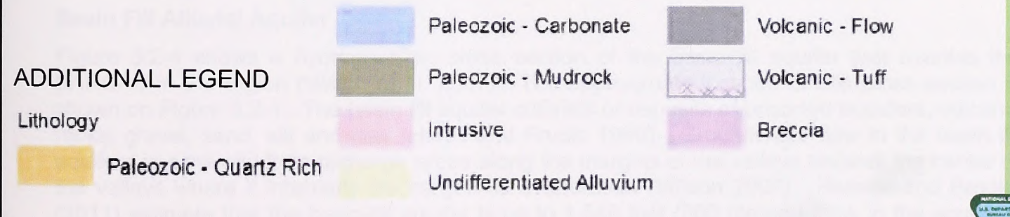
FIGURE 3.2-3 REGIONAL HYDROGEOLOGY
