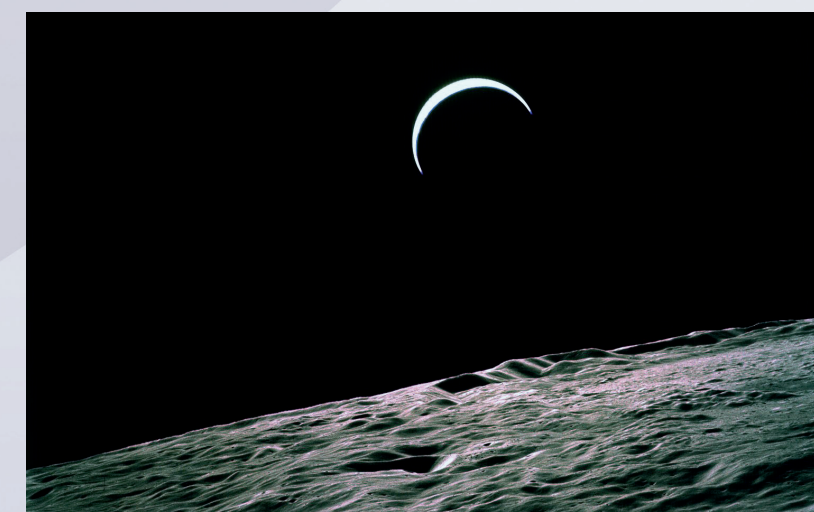
This view of the crescent Earth over the Moon's horizon was taken during the Apollo 15 lunar landing mission. Apollo 15 launched on July 26, 1971. Credits: NASA. https://go.nasa.gov/41490HC
