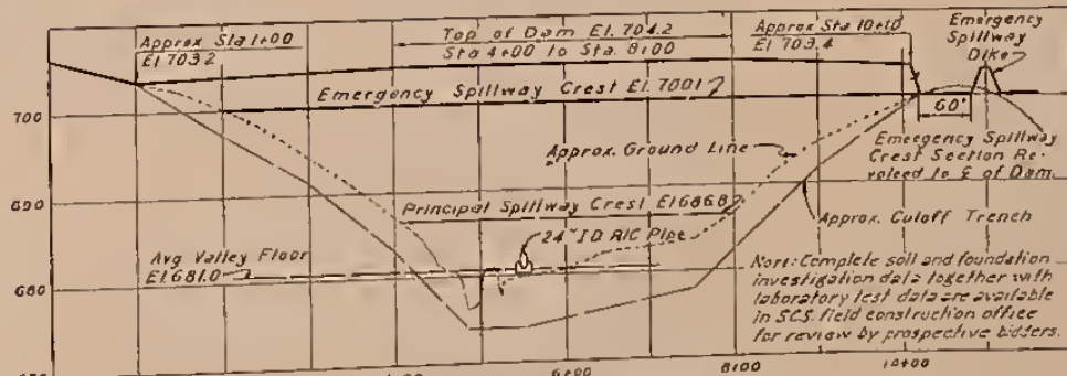
PROFILE ON C OF DAM
