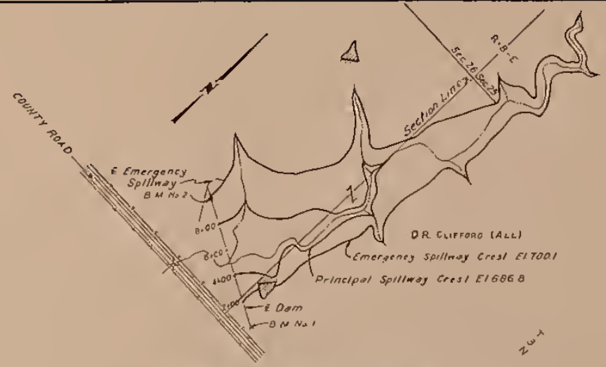
GENERAL PLAN OF RESERVOIR
