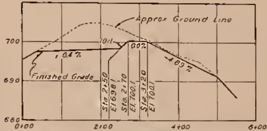
PROFILE ON C OF EMERGENCY SPILLWAY
