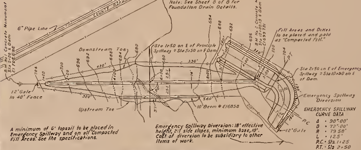
PLAN OF EMBANKMENT AND SPILLWAYS
