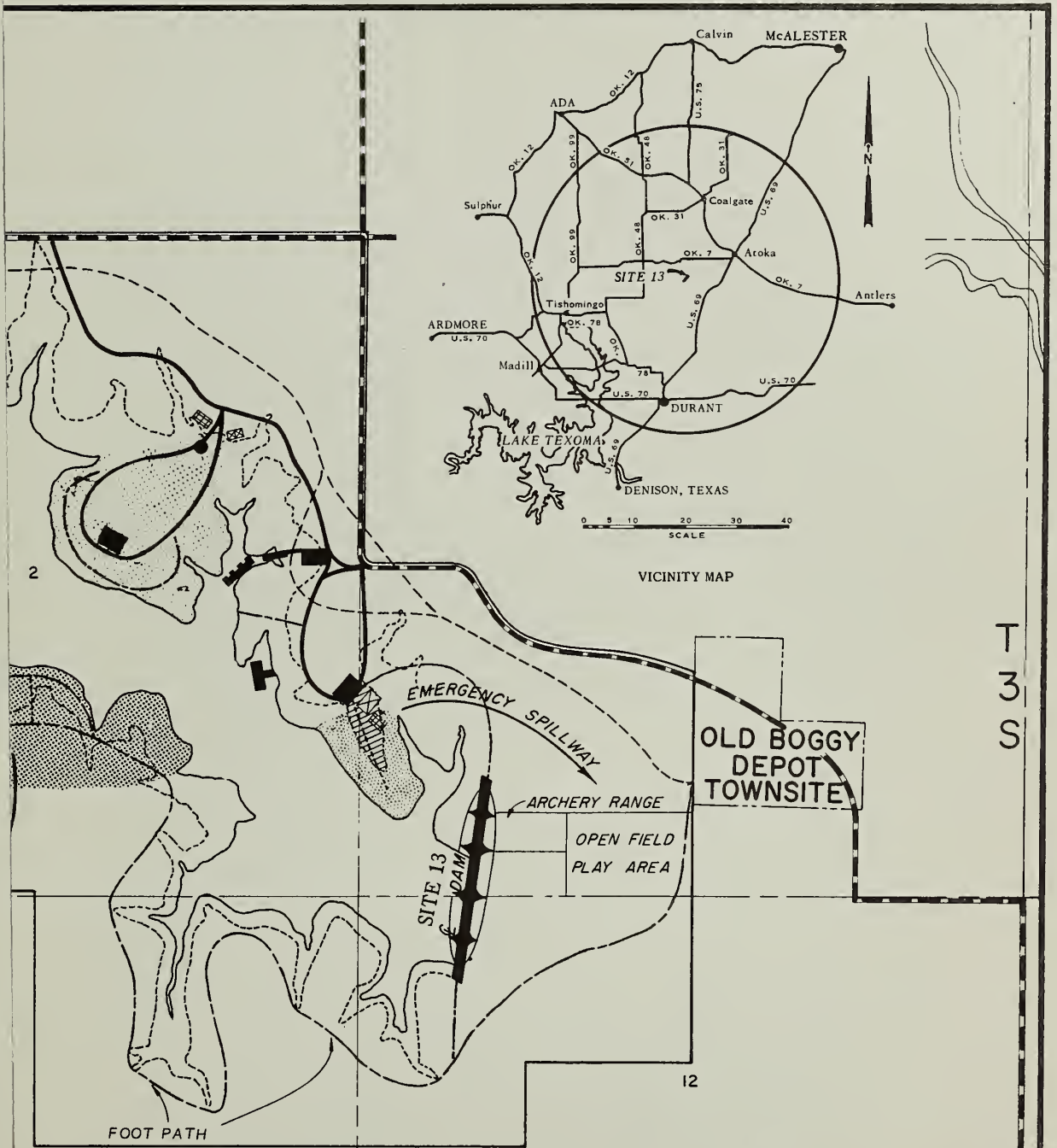
Figure 7 RECREATIONAL DEVELOPMENT LOWER CLEAR BOGGY CREEK WATERSHED SITE 13
