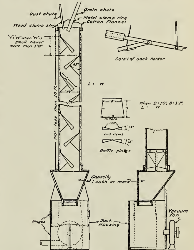
FIG. 3. DIAGRAM OF A MIXER OF THE PLAIN GRAVITY TYPE
