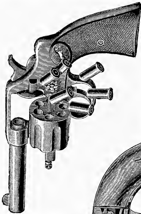
The Colt Self-ejecting Revolver.
