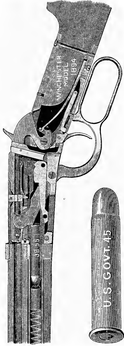
The Winchester (1894) Rifle and 1 Cartridge.
