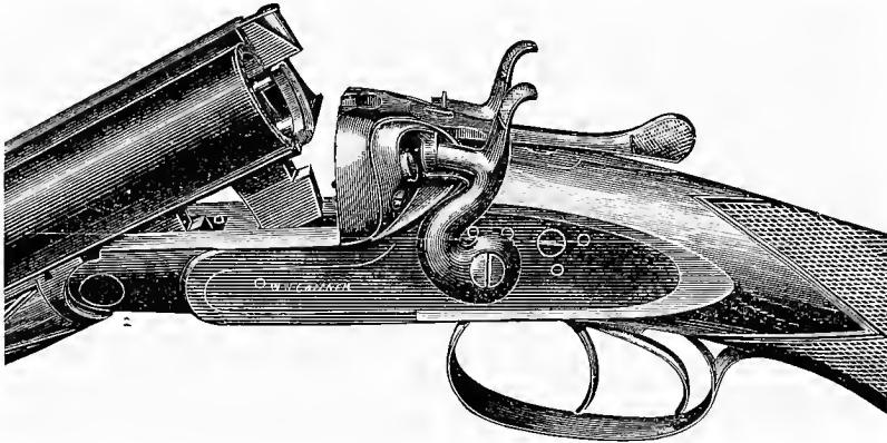
The Doll's-head Gun, with Bar Locks.
