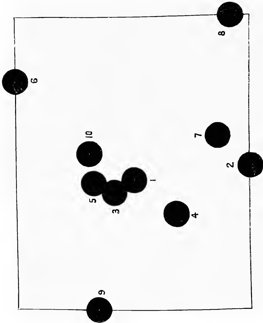
Diagram of .450-bore at 150 yards.
