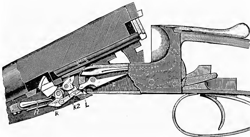
Maleham's Ejector Gun.
