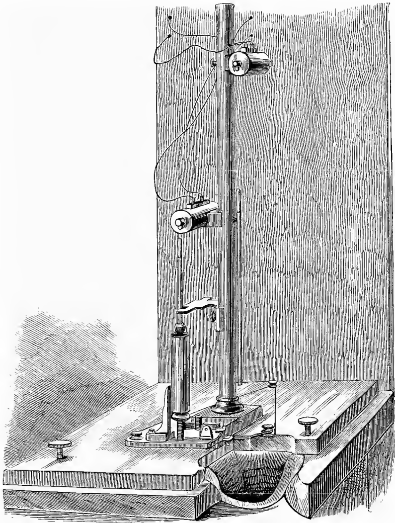
Boulengé's Chronograph.
