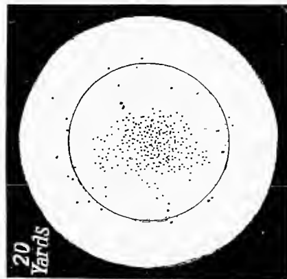
Facsimiles of patterns showing lateral deviation and stringing of the same pellets. Effects on stringing of heavy charge of powder.
