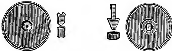
View of the Cap-chambers and Sections of Caps and Anvils of the "Eley" and "Life" Cases.
