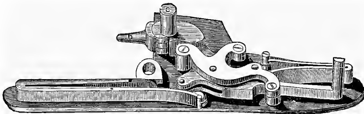
Lock of Murcott's Hammerless Gun.
