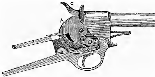
Mechanism of the Remington Rifle.
