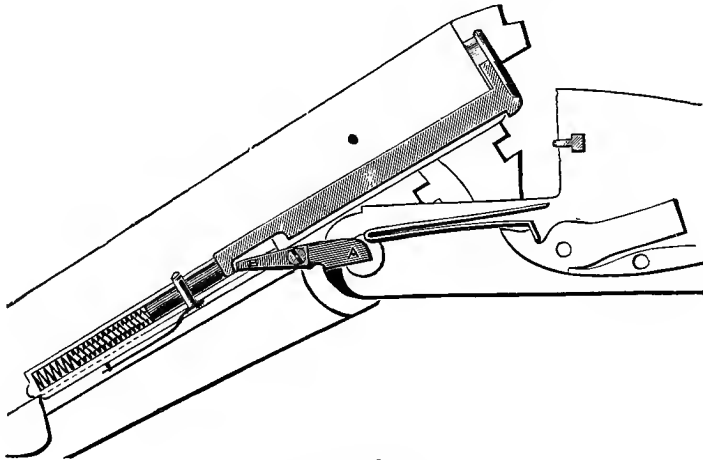
Harrison's Ejector.
