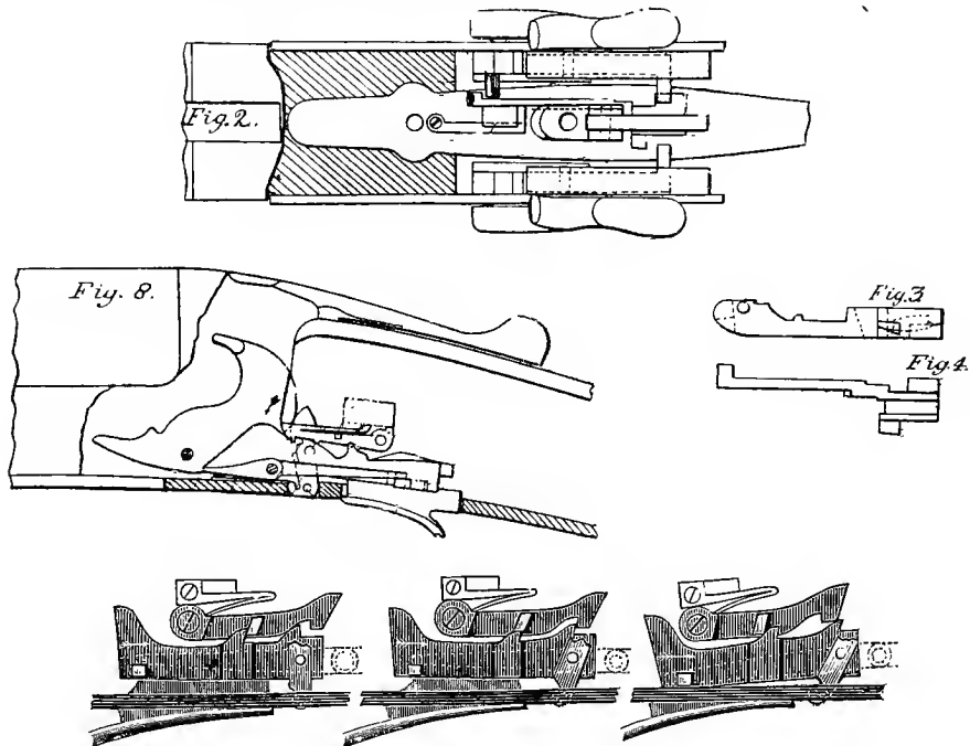
Jones' Single-trigger Mechanism.
