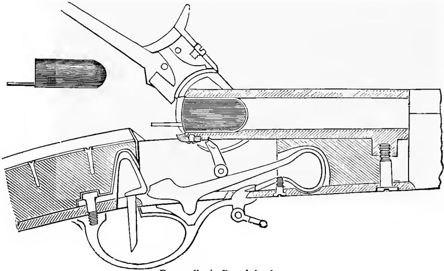
Demondion's Breech-loader.
