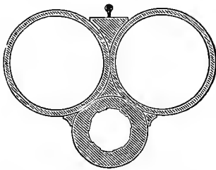
Muzzle of the Three-barrelled Gun.
