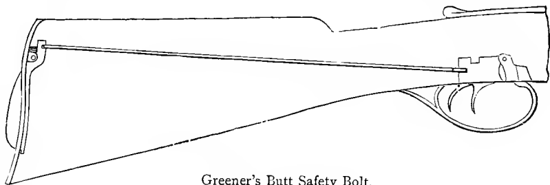
Greener's Butt Safety Bolt.
