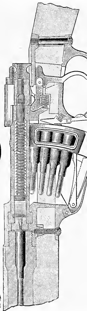
Roumanian Model Mannlicher, 1892
