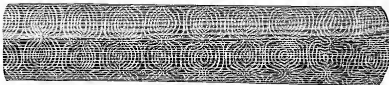
Two-Iron or "Boston" Damascus Barrel.
