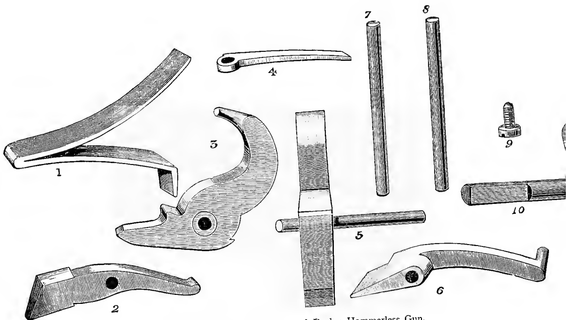
Lock-work of the Anson and Deeley Hammerless Gun.
