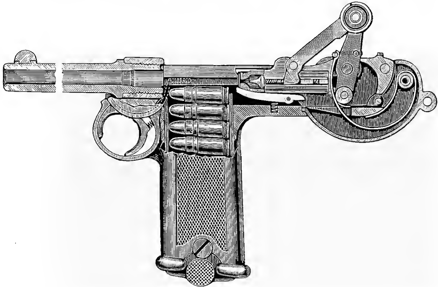
The Borchardt Automatic Magazine Pistol.
