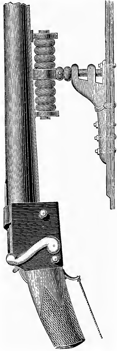
Greener-Field Punt Gun, with Indiarubber Recoil-breeching.
