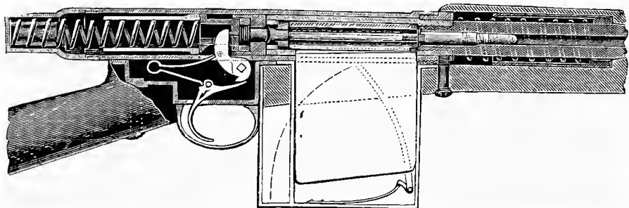
The Griffiths and Woodgate Automatic Rifle.
