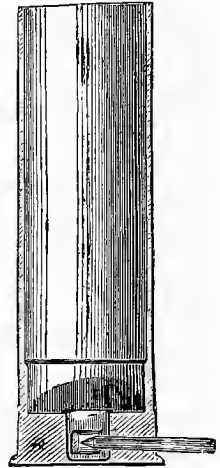
Section of the Lefauchaux Pin-fire Cartridge Case.
