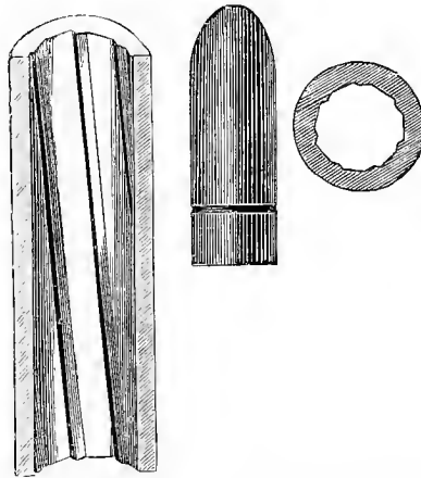
The Henry Rifling and Bullet, and Regulation Pattern Cartridge.
