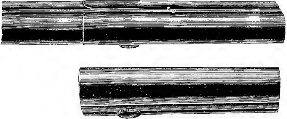
Dr. Maberley's Attachable Choke-muzzle.
