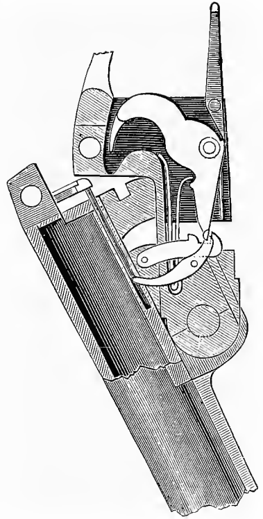
Greener's Self-acting Hammerless Gun.
