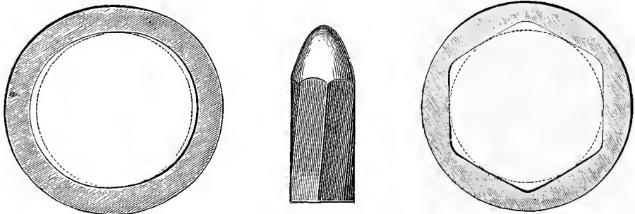
Lancaster Oval-bore Rifling, and Whitworth Rifling and Bullet.
