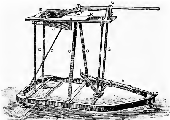
New Mechanical Gun-Rest and Recoil-Gauge.
