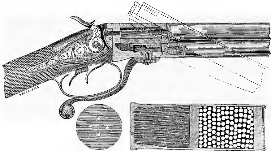
The Lancaster Central-fire Breech-loader and Cartridge.
