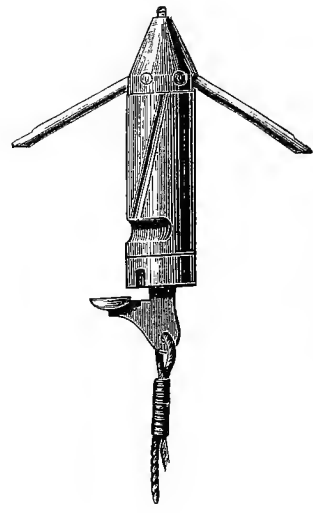
Explosive Bomb-lance.
