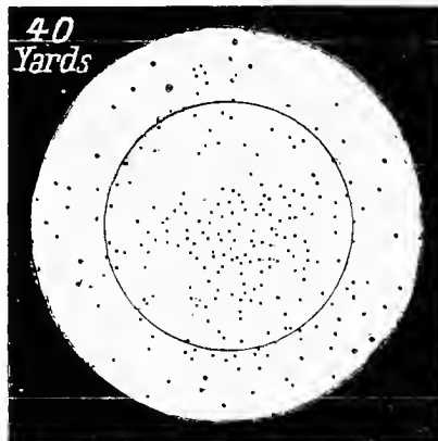
Pattern of the same CHOKE-BORED Gun at 40 Yards, with 49 grains of Schultze Powder and 1\frac{1}{4} oz. No. 6 Chilled Sht. (For stringing see page 349.)
