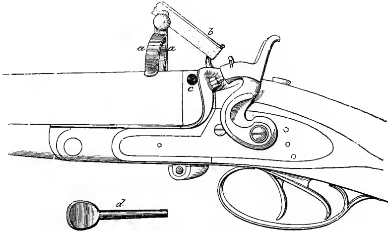
Experimental Breech-action.
