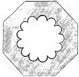
Polygroove Rifling, as used for Muzzle-loaders.
