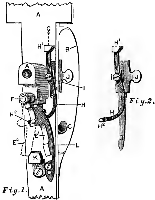
Charles Lancaster's Single-trigger Mechanism for Double-barrel Gun.
