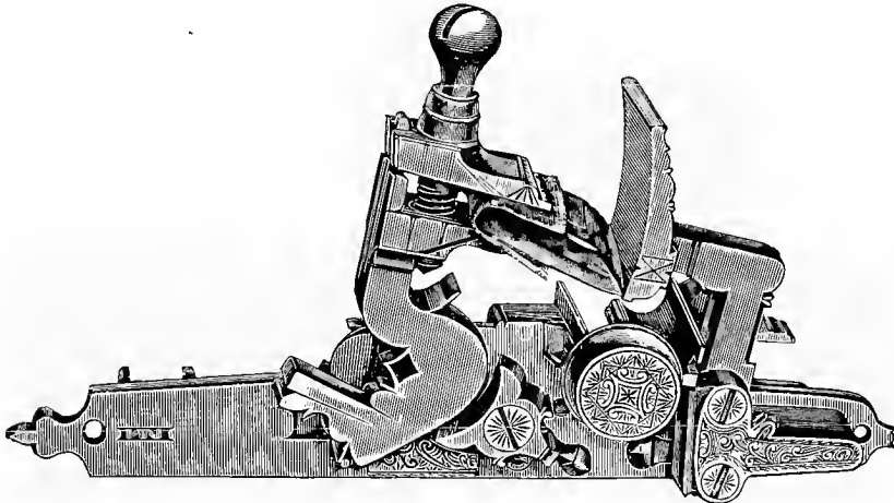
Flint-lock made by Moorish Gunsmiths at the Author's Factory in 1885.
