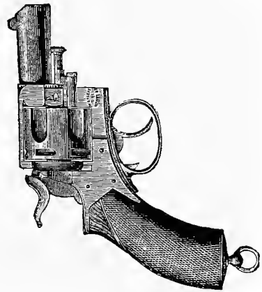
The R. I. C. Solid Frame Revolver.
