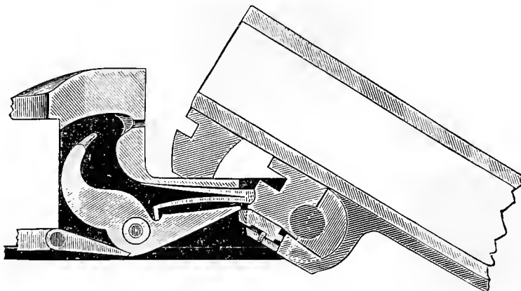
Mechanism of Greener's Patent Hammerless Lock.
