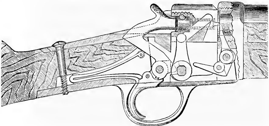
Section of the Field Rifle.—Sliding-block Pattern.
