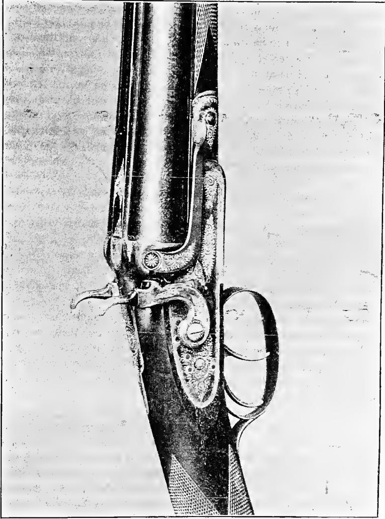
[Needham's Snap-action Mechanism.
