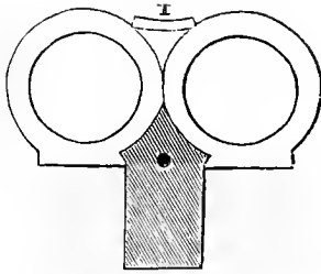
Dovetailed Barrel Lump.
