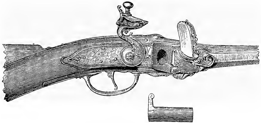
Italian Flint-lock Breech-loader.
