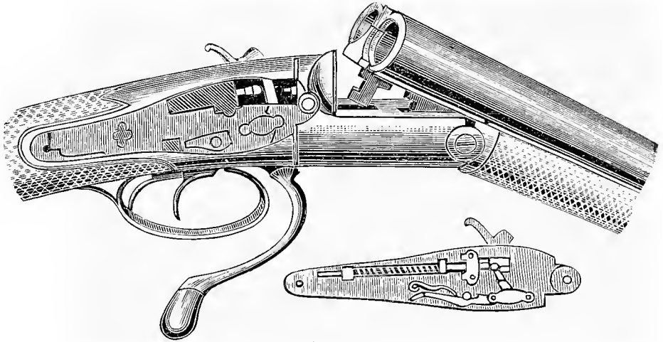
Langa's Self-cocking Gun, with Dummy Hammers.
