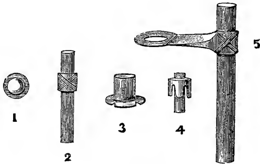
Detonators.
