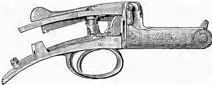
Mechanism of Hammerless Rook Rifle.
