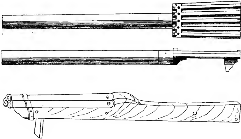
Multi-barrelled Hand-cannon.
