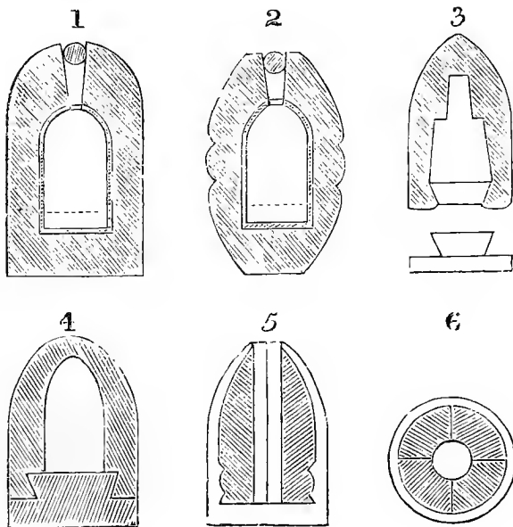
Explosive Shells.
