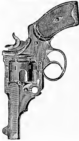
The Webley "Mark III."
