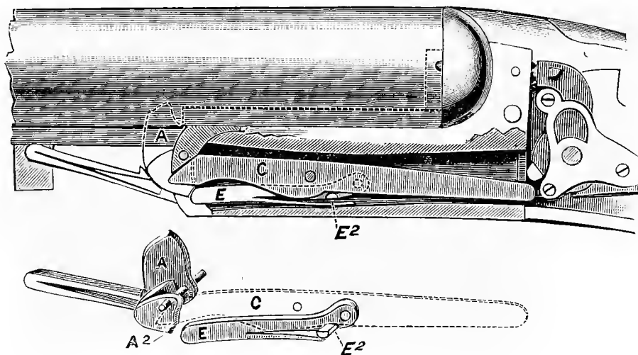
Southgate's Ejecting Mechanism and Separate Limbs.
