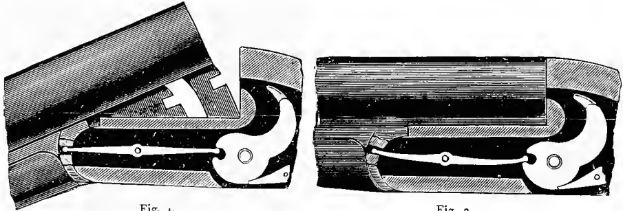
Greener's Emperor Hammerless Gun.
