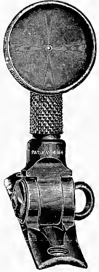
Lyman's Disc Peep Sight for Match Shooting.
