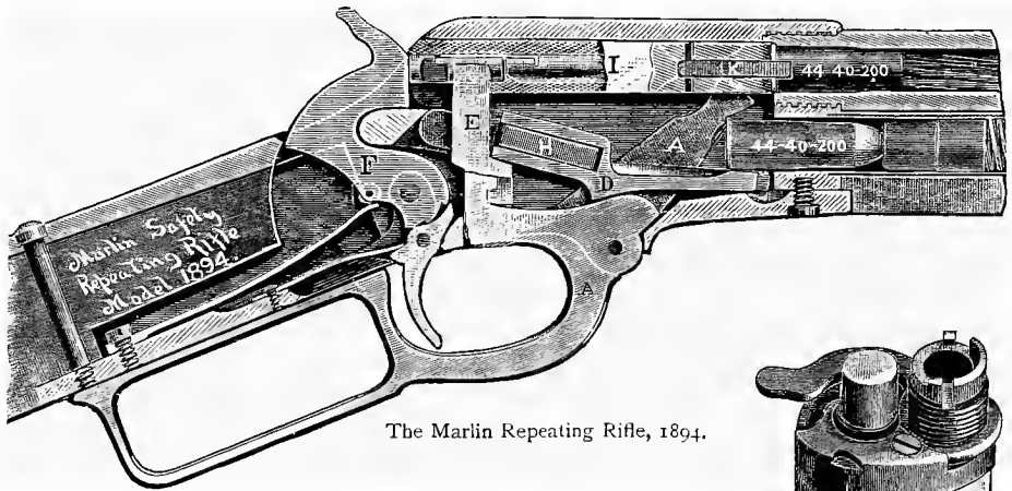
Marlin Rifle.
