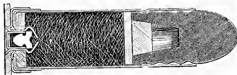
Boxer Cartridge, used in the Snider Rifle.
