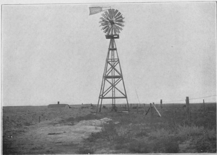
FIG. 1.—WINDMILL IN USE AT CHEYENNE, WYO., AT STATION FOR EXPERIMENTING WITH IRRIGATION AS A SUPPLEMENT TO DRY FARMING.
