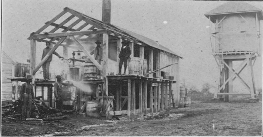
STEAM PLANTS FOR COOKING LIME-SULPHUR-SALT WASH.
