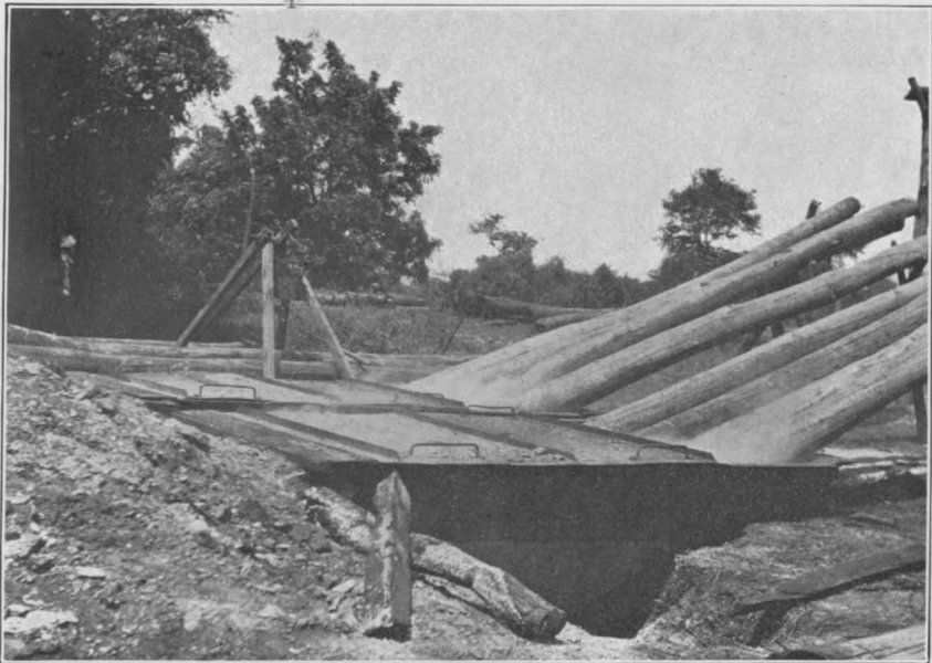
FIG. 2.—TREATING CHESTNUT POLES BY THIRD OR TANK METHOD, THORNDALE, PA., STATION.
