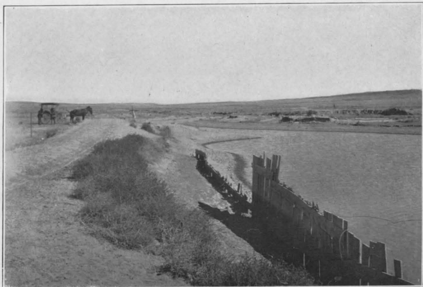
FIG. 2.—RESERVOIR IN USE NEAR CHEYENNE, WYO.
