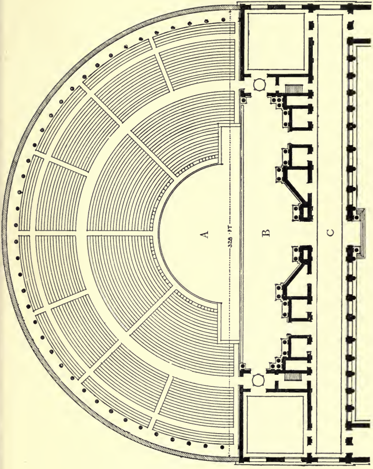
PLAN OF THE ROMAN THEATER AT ORANGE
