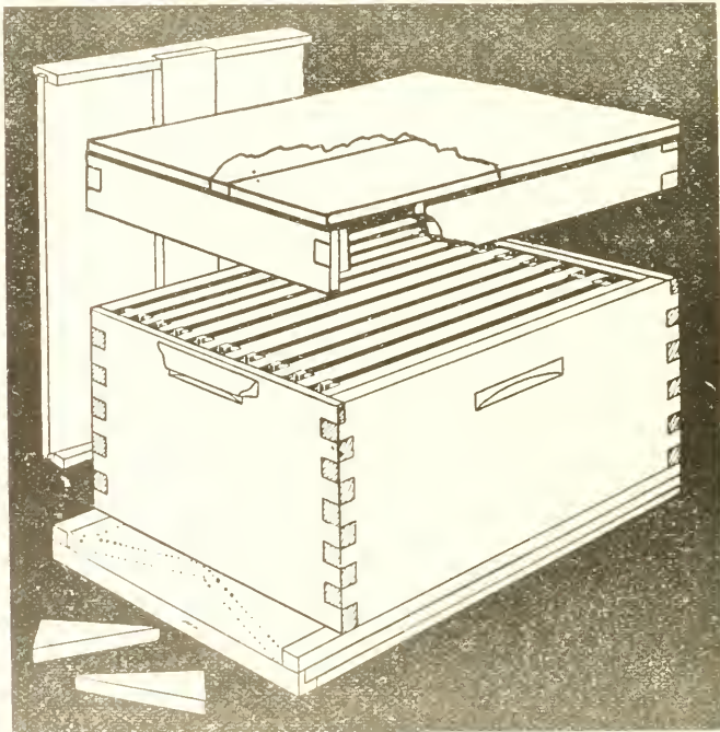
This is the hive used by nearly all Beekeepers, and is not tall enough to admit of honey sufficient to be stored above the bees for a winters supply; neither is it large enough to hold all the eggs a queen will deposit.
