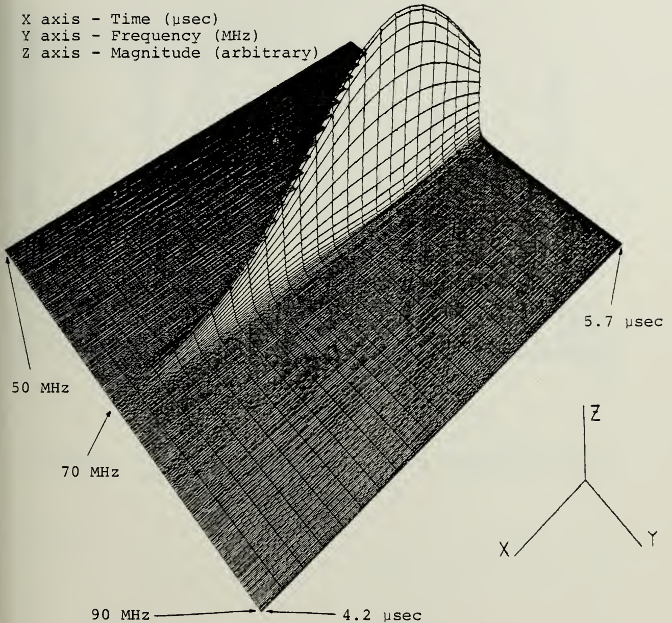
Figure 24. Image Plane Intensity Profile (Magnitude) Produced by a Monotonic 70 MHz Signal with an Incident Gaussian Beam and a Stepped Array Transducer (Dynamic Model)
