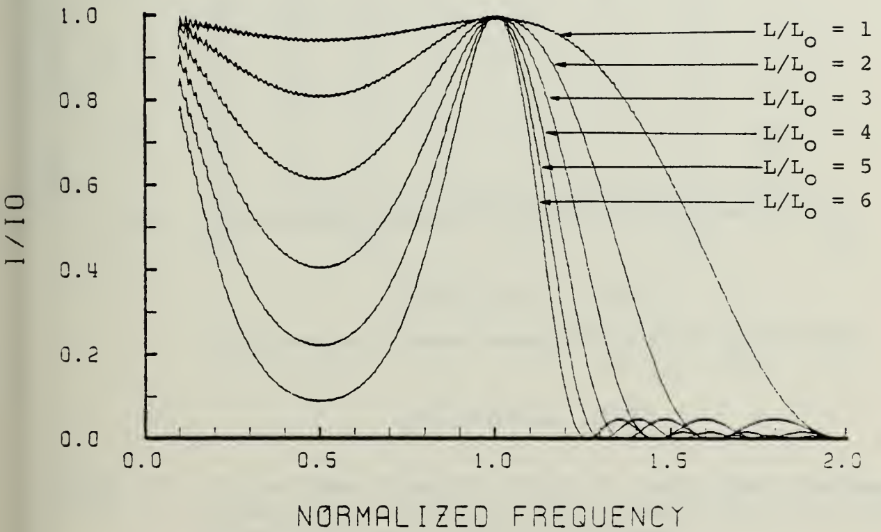
Figure 17. AOSA Implemented Diffraction Efficiency Bandshape
