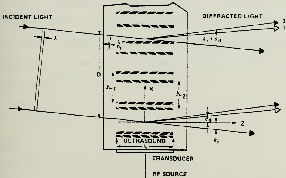
Figure 4. Bragg Cell Operation
