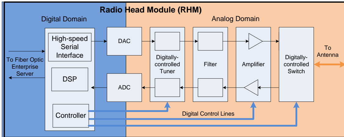
Figure 5. Architectural View of the RHM
