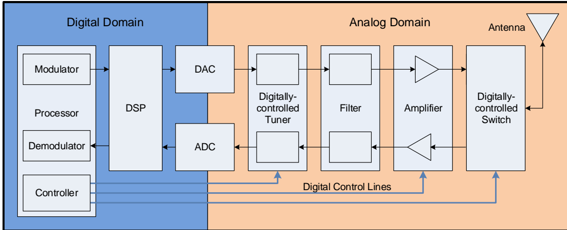
Figure 3. SDR Architecture. Adapted from Arnold et al. (2010), Baliga et al. (2011), and Thomas, McPherson, and Irvine (2016).
