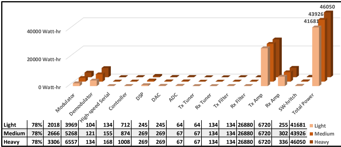
Figure 20. L-RTacAJ EWC Architecture Component Power Simulation
