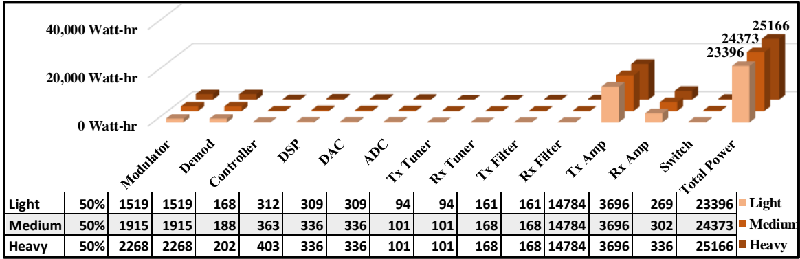
Figure 13. M-RTac Current Architecture Component Power Simulation
