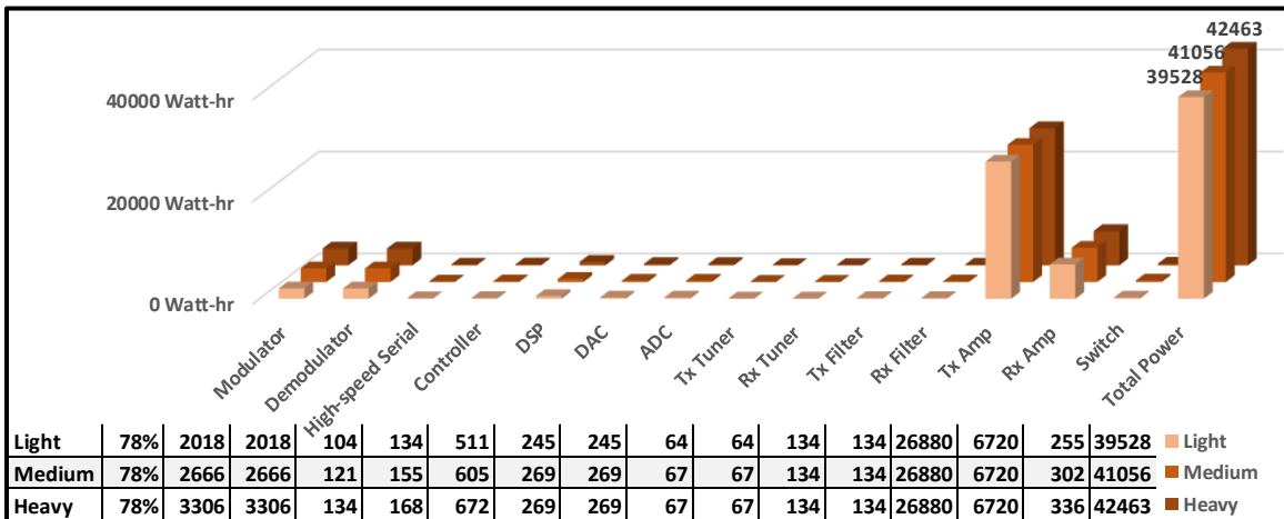
Figure 19. L-RTac EWC Architecture Component Power Simulation
