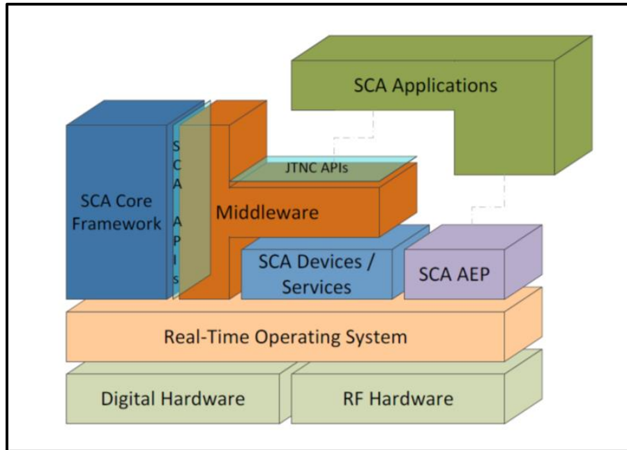
Figure 4. Layered View of SCA Adapted from DOD Waveform Standards Directorate (2016)
