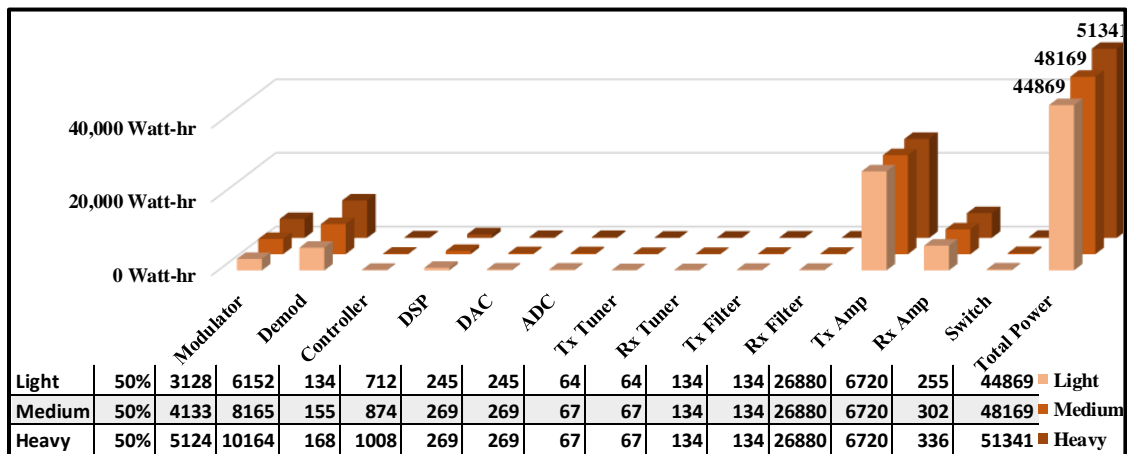
Figure 15. L-RTacAJ Current Architecture Component Power Simulation
