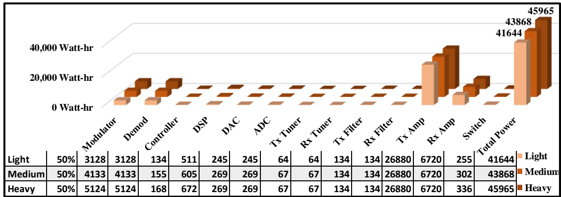
Figure 14. L-RTac Current Architecture Component Power Simulation
