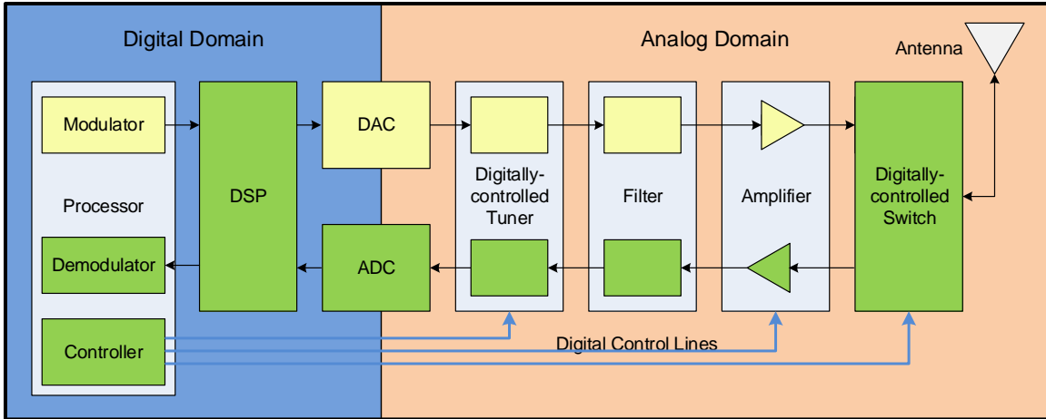
Figure 10. SDR Architecture in Receive Mode
