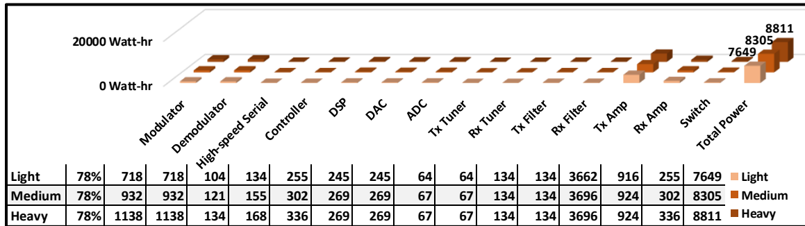
Figure 17. S-RTac EWC Architecture Component Power Simulation
