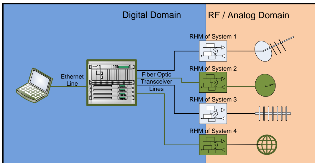
Figure 16. EWC Architecture of Multiple SDR Systems
