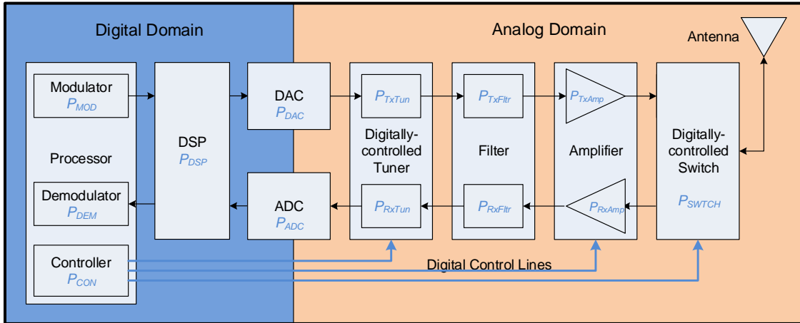
Figure 6. SDR Power Architecture
