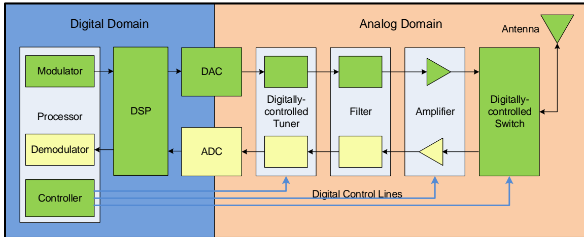
Figure 9. SDR Architecture in Transmit Mode
