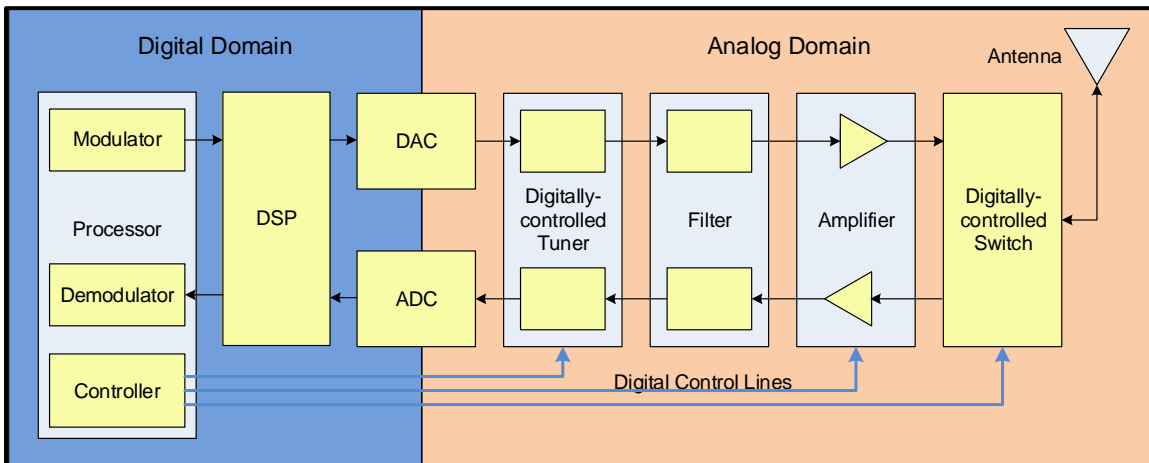
Figure 8. SDR Architecture in Stand-by Mode
