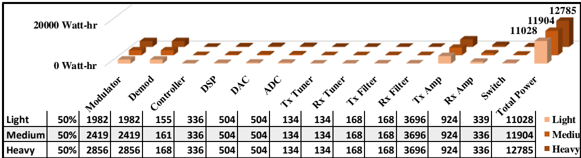
Figure 12. S-RTac Current Architecture Component Power Simulation
