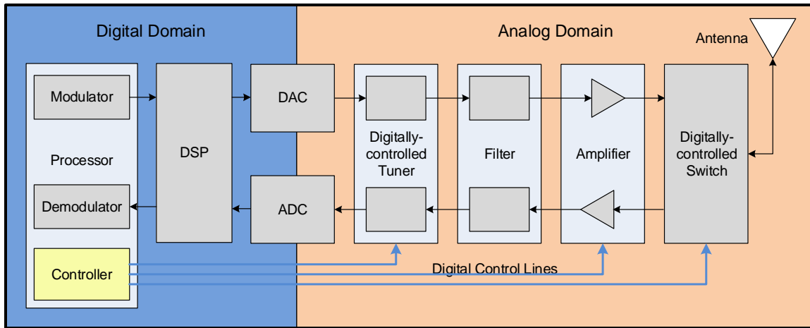
Figure 7. SDR Architecture in Sleep Mode
