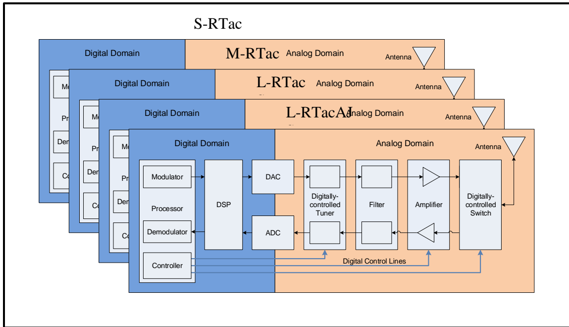
Figure 11. Current Architecture of Multiple SDR Systems
