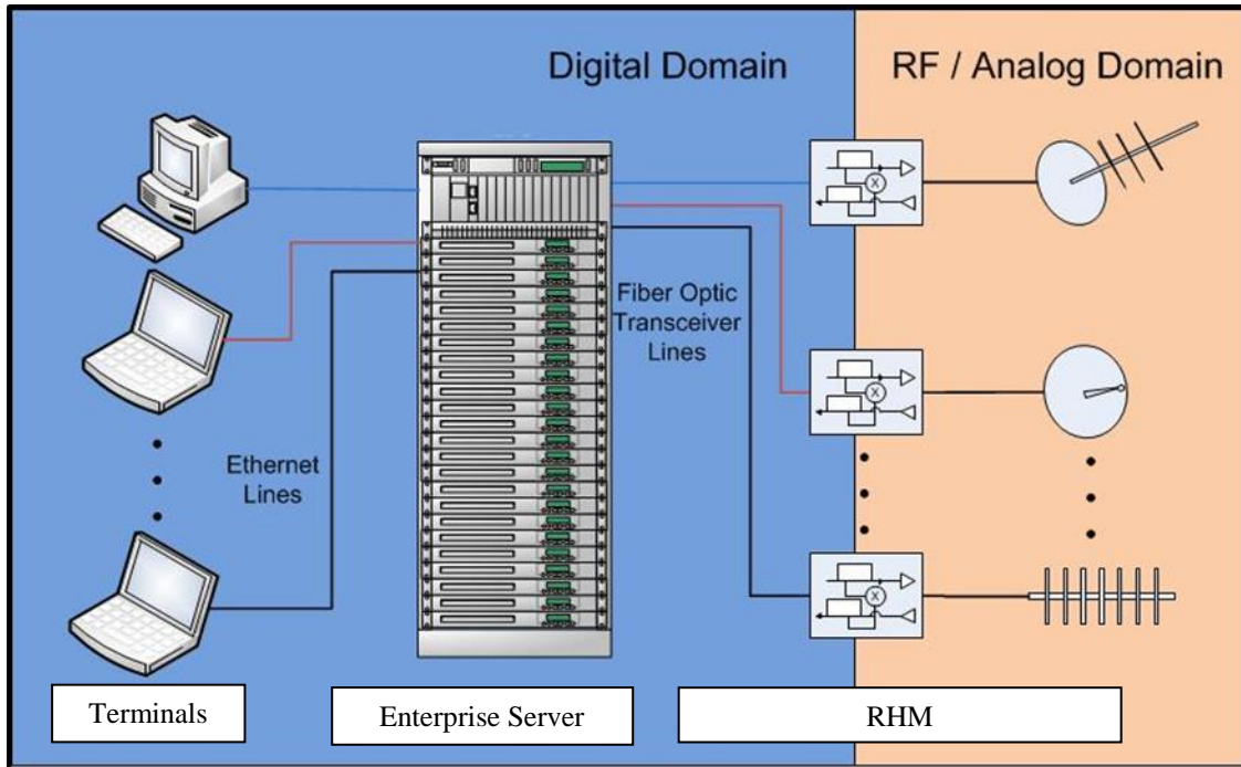
Figure 2. EWC Architecture
