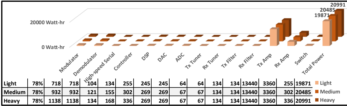
Figure 18. M-RTac EWC Architecture Component Power Simulation
