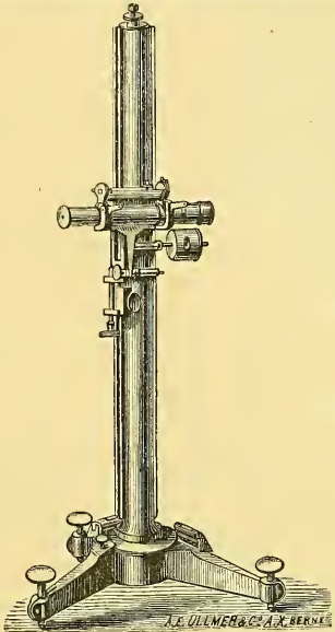
Cathetometer.
