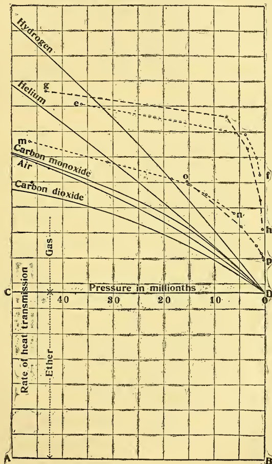
Chart Showing Relative Heat Conductivity of Gases.
