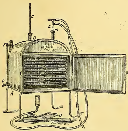
Laboratory Drying Ovens. (Devised by Prof. W. M. L. Coplin, M.D.)
