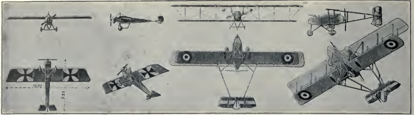
Fokker monoplane (German). Follows closely the French Morane, especially as to its balanced elevators. Equipped with a rotary Oberursel 80 or 100 h.p. engine. One of the first German machines to successfully employ a mechanically operated machine-gun firing through the sweep of the propeller.
