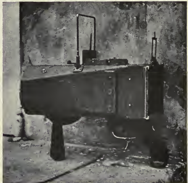
The pistol-camera for German airmen—the left side.
