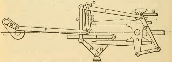
FIG. 174.—The Walschaerts Valve-gear.
