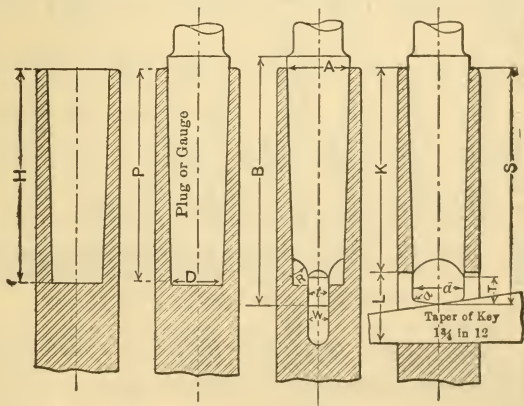
FIG. 216.—Morse Tapers. See table above.
