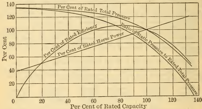
FIG. 147. CHARACTERISTICS OF A RADIAL BLADE FAN.
