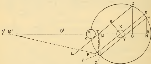
FIG. 171. — Sweet's Valve Diagram.
