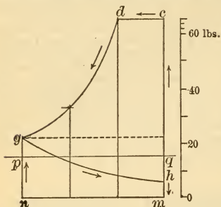
FIG. 166. — WOOLF ENGINE, IDEAL INDICATOR-DIAGRAMS.
