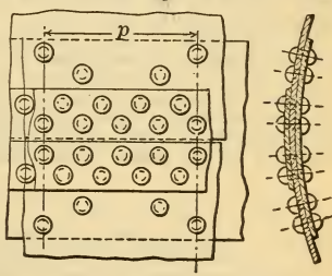
FIG. 97. QUADRUPLE RIVETING.
