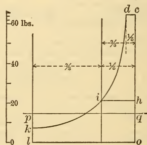
FIG. 168. — RECEIVER ENGINE, IDEAL DIAGRAMS REDUCED AND COMBINED.
