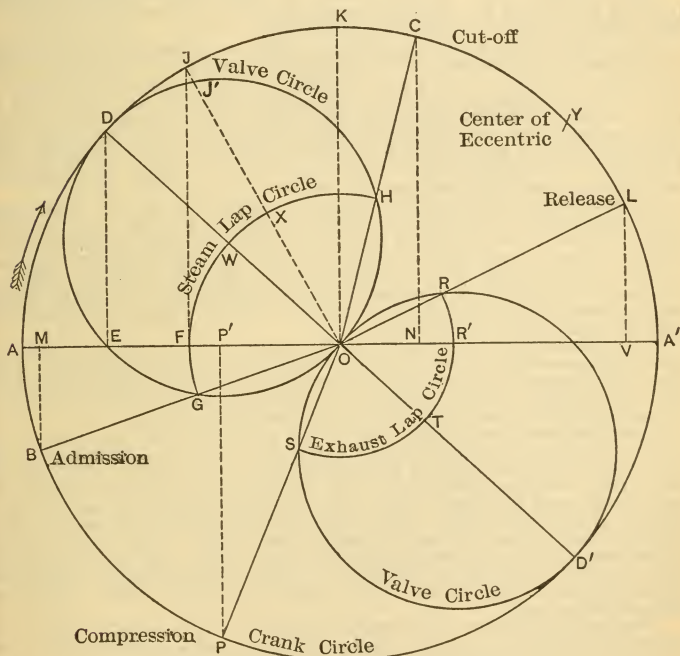
FIG. 172.—Zeuner's Valve Diagram.
