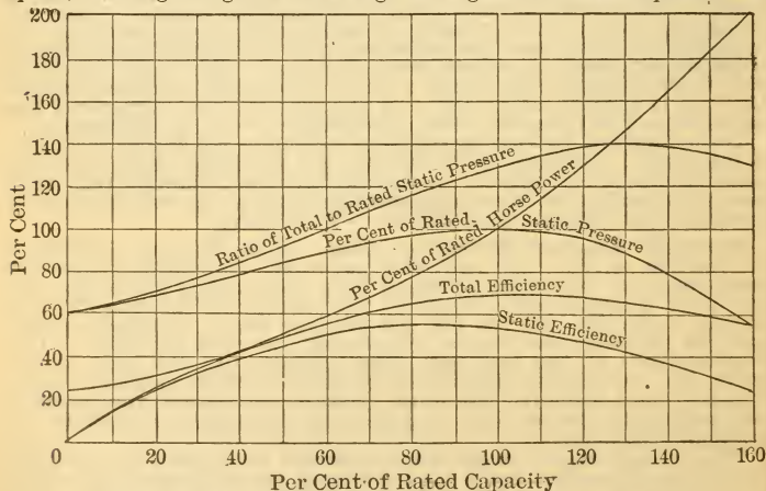
FIG. 148. CHARACTERISTICS OF A MULTI-BLADE FAN.
