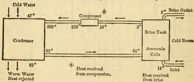
DIAGRAM OF AMMONIA COMPRESSION MACHINE.
