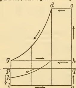
FIG. 167. — RECEIVER-ENGINE, IDEAL INDICATOR-DIAGRAM.
