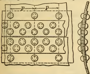
FIG. 96. TRIPLE RIVETING.
