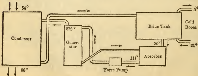
DIAGRAM OF AMMONIA ABSORPTION MACHINE.
