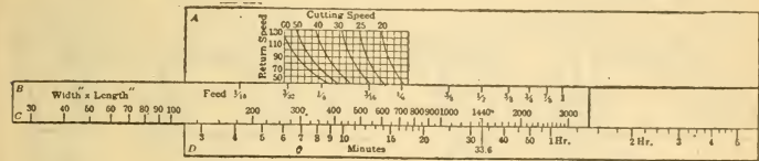
FIG. 197. PLANER TIME SLIDE RULE.
