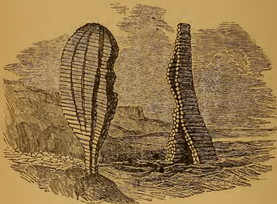
REMAINS OF BASALTIC DYKES.
