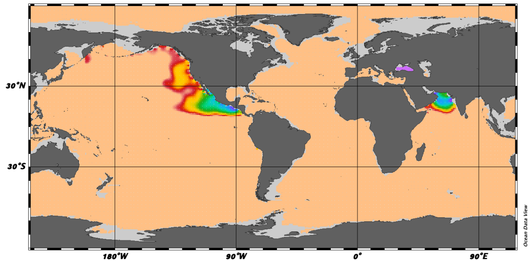
Oxygen [ml/l] @ Depth [m]=800
