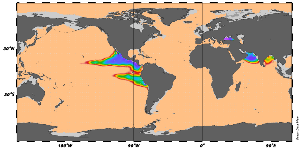
Oxygen [ml/l] @ Depth [m]=400
