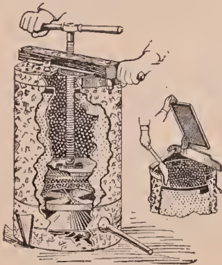
German Press.
