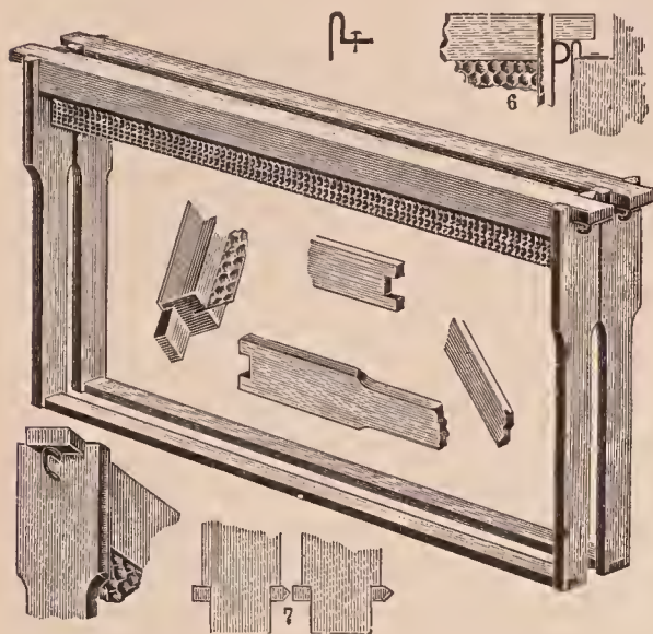
Fig. 5. Hoffman frames, regular.
