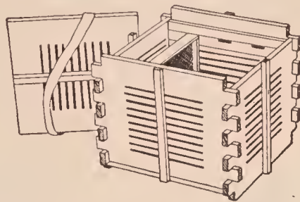
Parcel post mailing cage for bees without combs.
