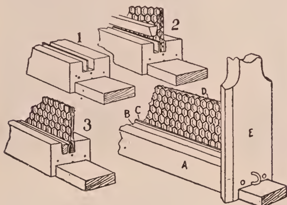
Wedge top-bar method of fastening foundation.
