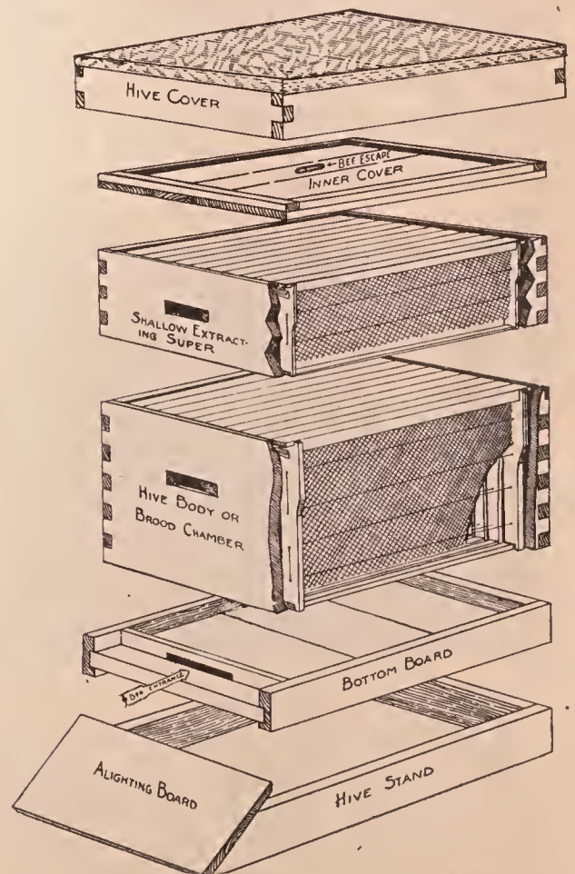
Modern Hive with Hoffman frames for production of extracted honey. Between super and hive body should be a queen-excluder. (Deep extracting super identical with hive body may be substituted for shallow extracting super.)
