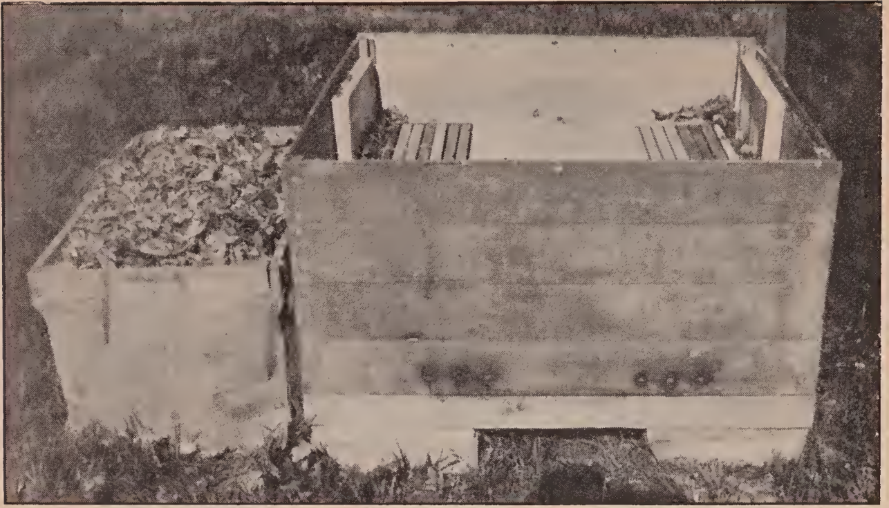
Fig. 8.—The Holtermann four-hive packing-case. Notice the three \frac{3}{4} -inch entrance holes. Notice also that there is no projecting ledge or doorstep to catch snow and ice, thus closing the holes, causing the death of the bees.
