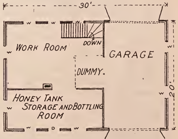
Garage and honey-house combined. The load may be taken off the auto and set directly on to the platform in the work room thru an opening in the wall.
