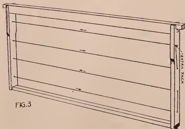
Fig. 3.—The old-style horizontal wiring that was used for a good many years. It made nice beautiful combs, but did not prevent the distortion of the cells within two inches of the top-bar.
