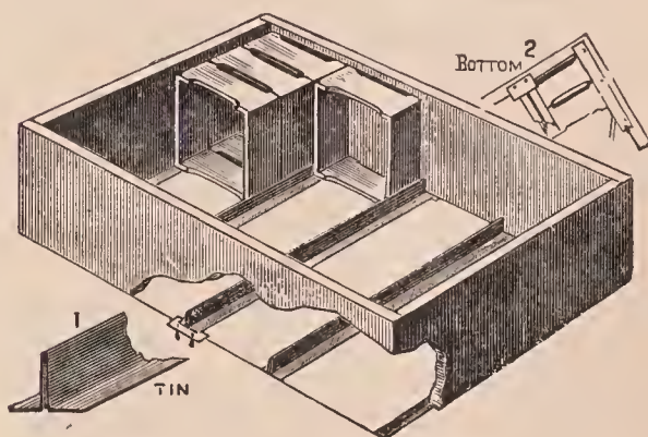
Regular T super.
