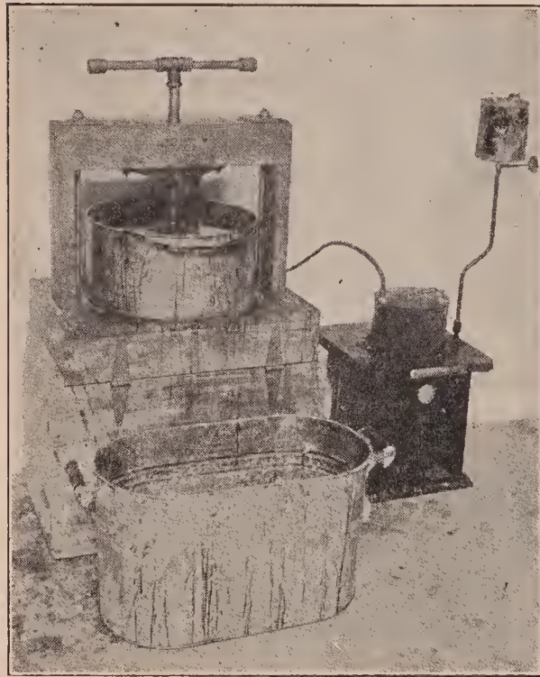
Fig. 13.—Apply the pressure. The wax rises to the top of the water. As much time may be given to the pressing as desired—no danger of chilling, because of the jet of steam.
