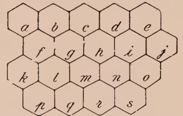
American foul brood: a, b, f, normal sealed cells; c, j, sunken cappings, showing perforations; g, sunken cappings not perforated; h, l, m, n, q, r, larvæ affected by disease; e, i, p, s, scales formed from dried-down larvæ; d, o, pupæ affected by disease. Three times natural size. (Original.)
