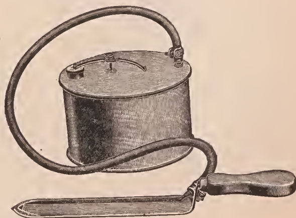
Steam honey-knife and boiler, showing construction of the safety valve, made of super spring at filter hole.
