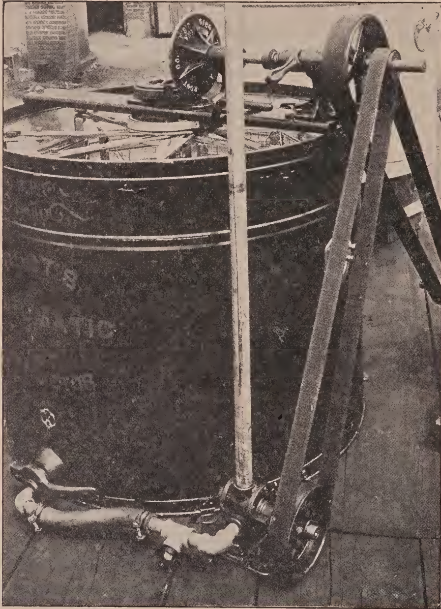
A closer view of the pump, showing the construction, method of belting, arrangement of pipe and hose connections and manner of tapping into honey-gate.
