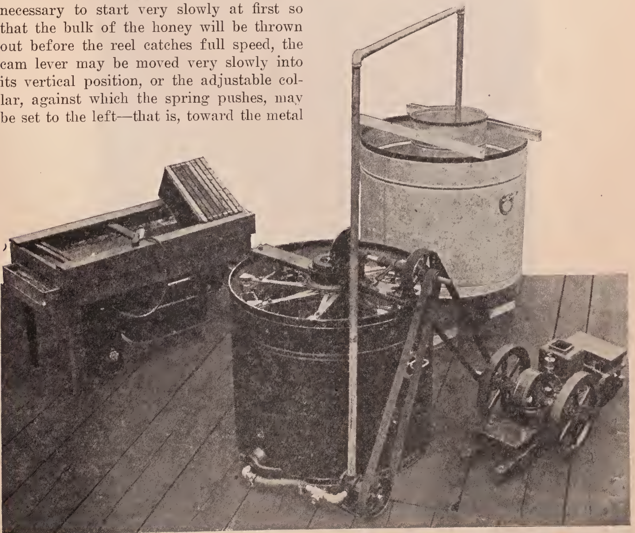
Ideal arrangement of extractor, pump, engine, tanks, etc.
