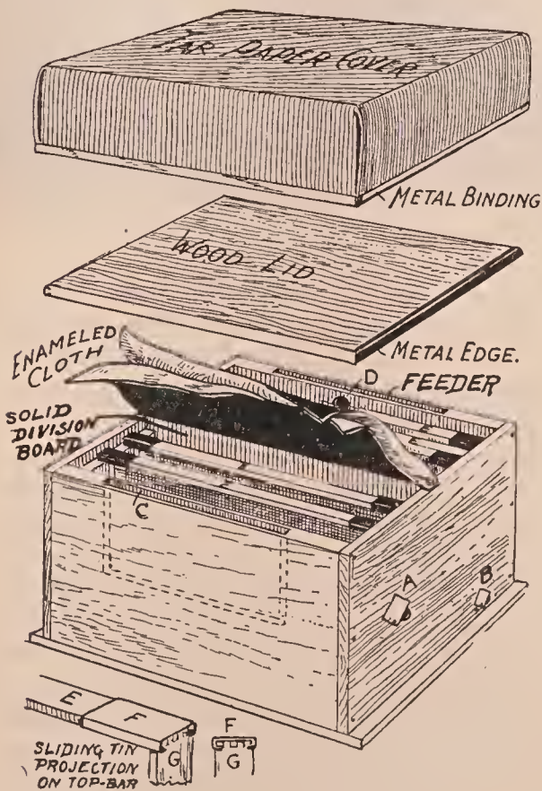
Fig. 1.—Twin mating-box.
