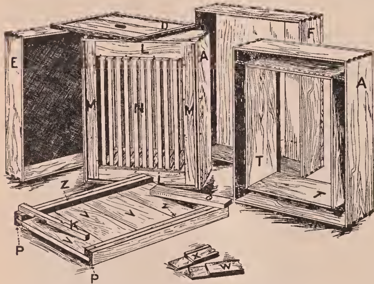
Buckeye hive dissected, showing separate parts, and how the brood-chamber packing is shut in by cleats M and L. A, outer wall brood-chamber; T, inner wall brood-chamber; X, W, packing space cover; L, M, packing space bottom; F, telescope cover; E, chaff-tray; D, super-cover.
