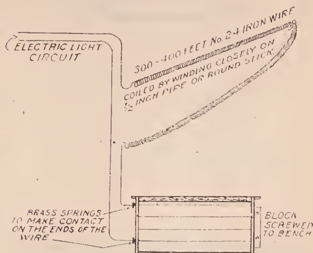
Electrical imbedding device.
