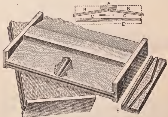
Gable cover.
