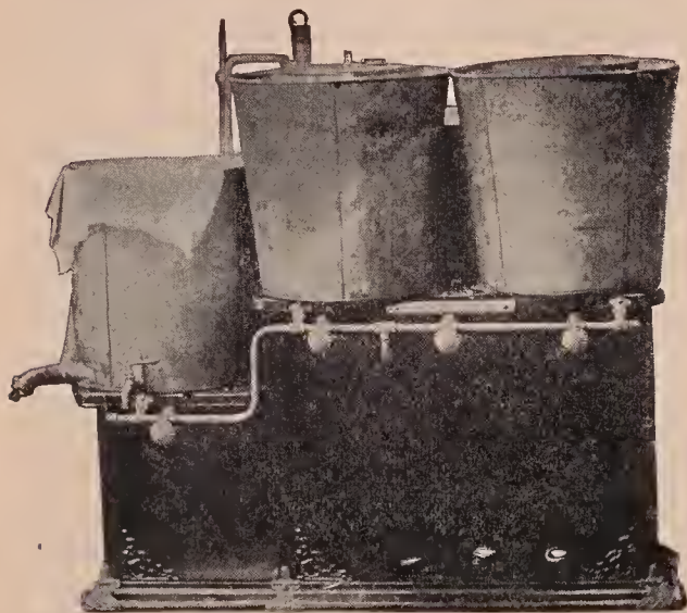
Mr. Fowls' melting-tanks, siphon, and gasoline stove.
