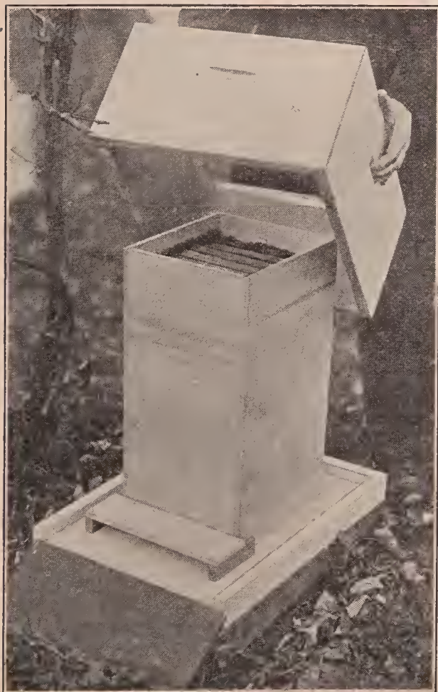
Figs. 11 and 12.—The Demuth plan of wintering bees outdoors in common hives or supers. An inner case is made so as to hold eight Langstroth frames stood on end. This makes a winter brood-nest relatively deep. During the coldest of the winter the bees will cluster in the top where it is warm.
