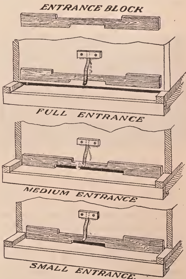
Contracted cleats for summer use.
