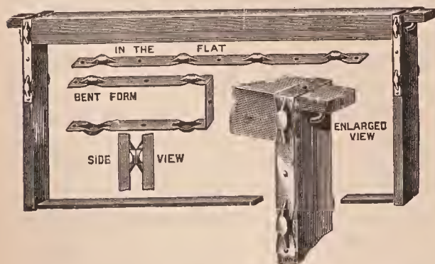
Fig. 6. Hoffman frames, metal-spaced pattern.
