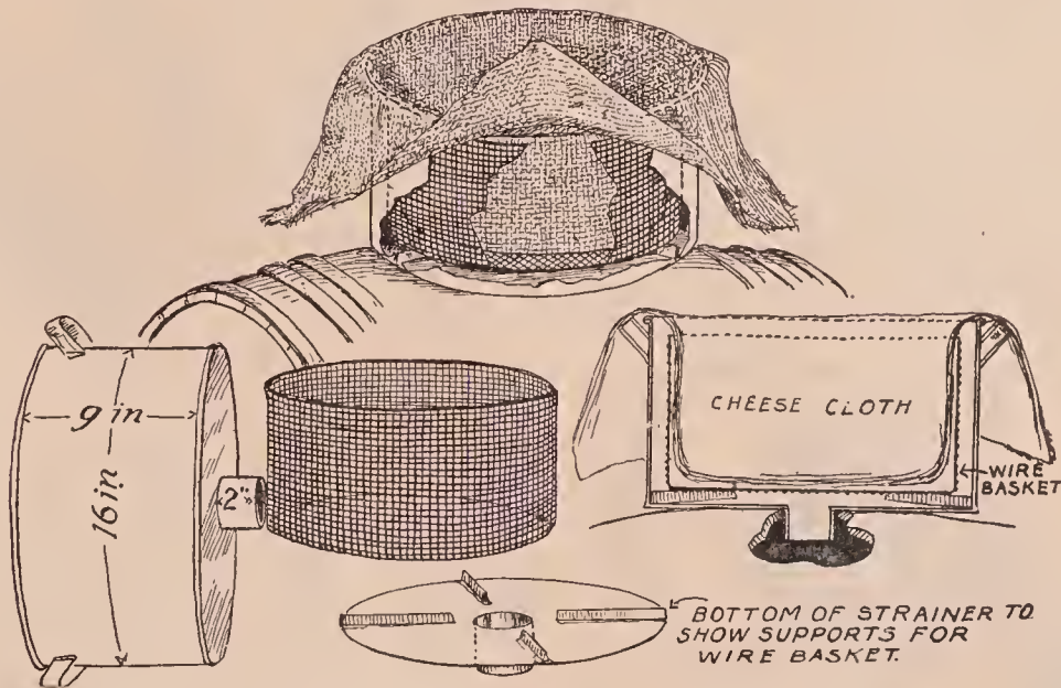
Pettit honey-strainer. (See page 337.)
