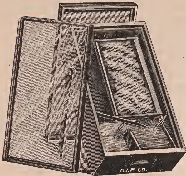
Doolittle solar wax-extractor.
