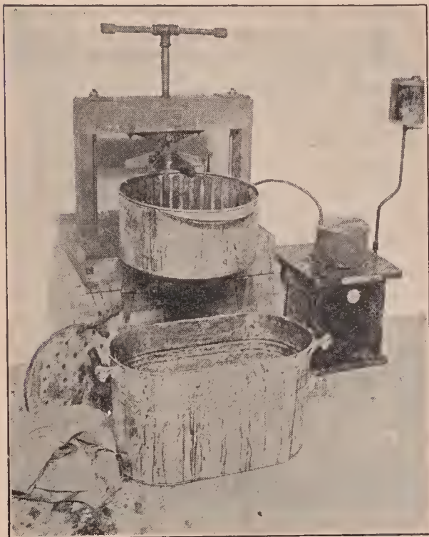
Fig. 11.—The press can be pulled forward ready for filling.
