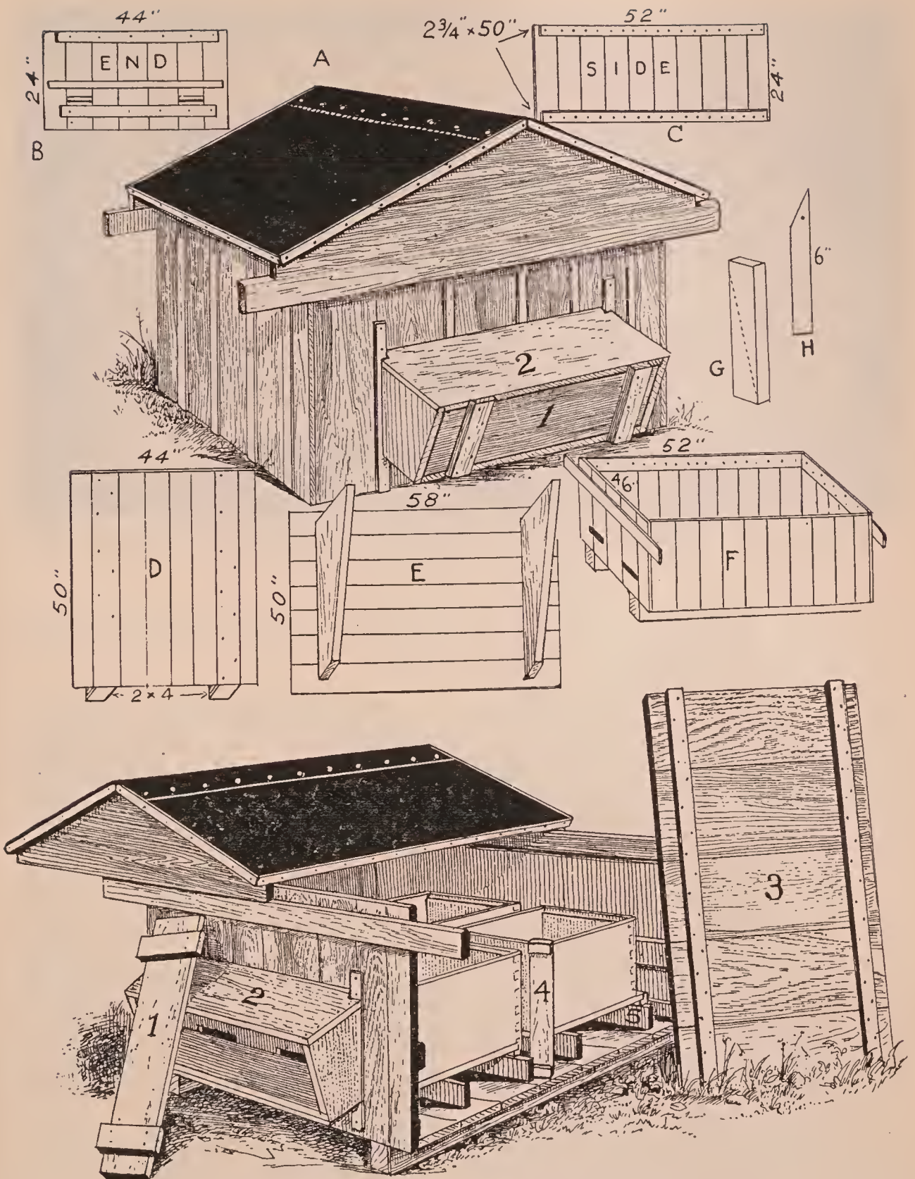
Fig. 7.—The original four-colony winter case as used by Ira Bartlett of Michigan 30 years ago. He was probably the original user of the principle.
