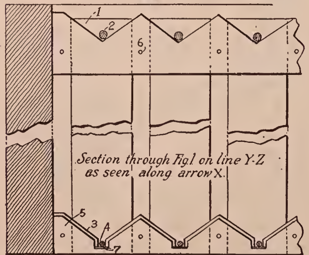
Hive-rabbit spacers.
