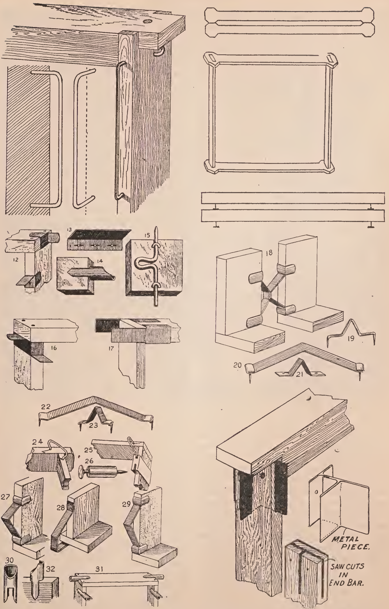
Various forms of frame-spacers.
