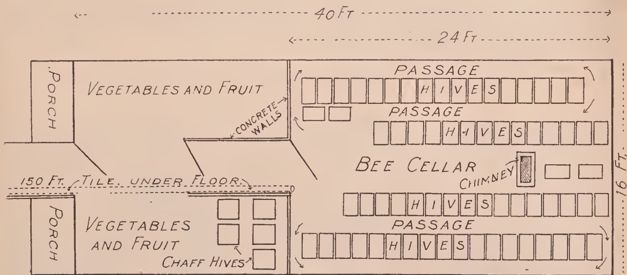
Fig. 1.—This is a diagram of the ground plan of the David Running bee-cellar which has wintered bees for the last 12 years with a loss of less than one per cent. The cellar proper is built in a sidehill. The bottom of the cellar is on a level with the ground in front. The walls are 6 inches thick, of concrete, with a concrete ceiling on top. Directly above the cellar is a concrete workshop and extracting-house. Between the ceiling of the cellar and the floor of this building above there is packing material of one foot of dry sawdust and one foot of air space; and then another set of joists covered with matched flooring. Between the ceiling and cellar roof is 6 feet, and the cellar is capable of holding between 300 and 400 colonies. It will be noticed that there are three doors to shut out the outside cold. The hives are piled as shown in the diagram. The ventilator, or chimney, has a 9 x 13 flue which extends clear up thru the building above. The outer cellar is sometimes used for wintering bees in double-walled hives.
