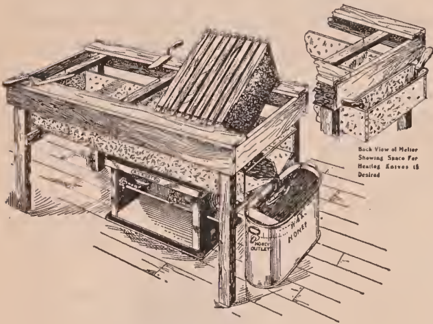
Peterson capping-melter.
