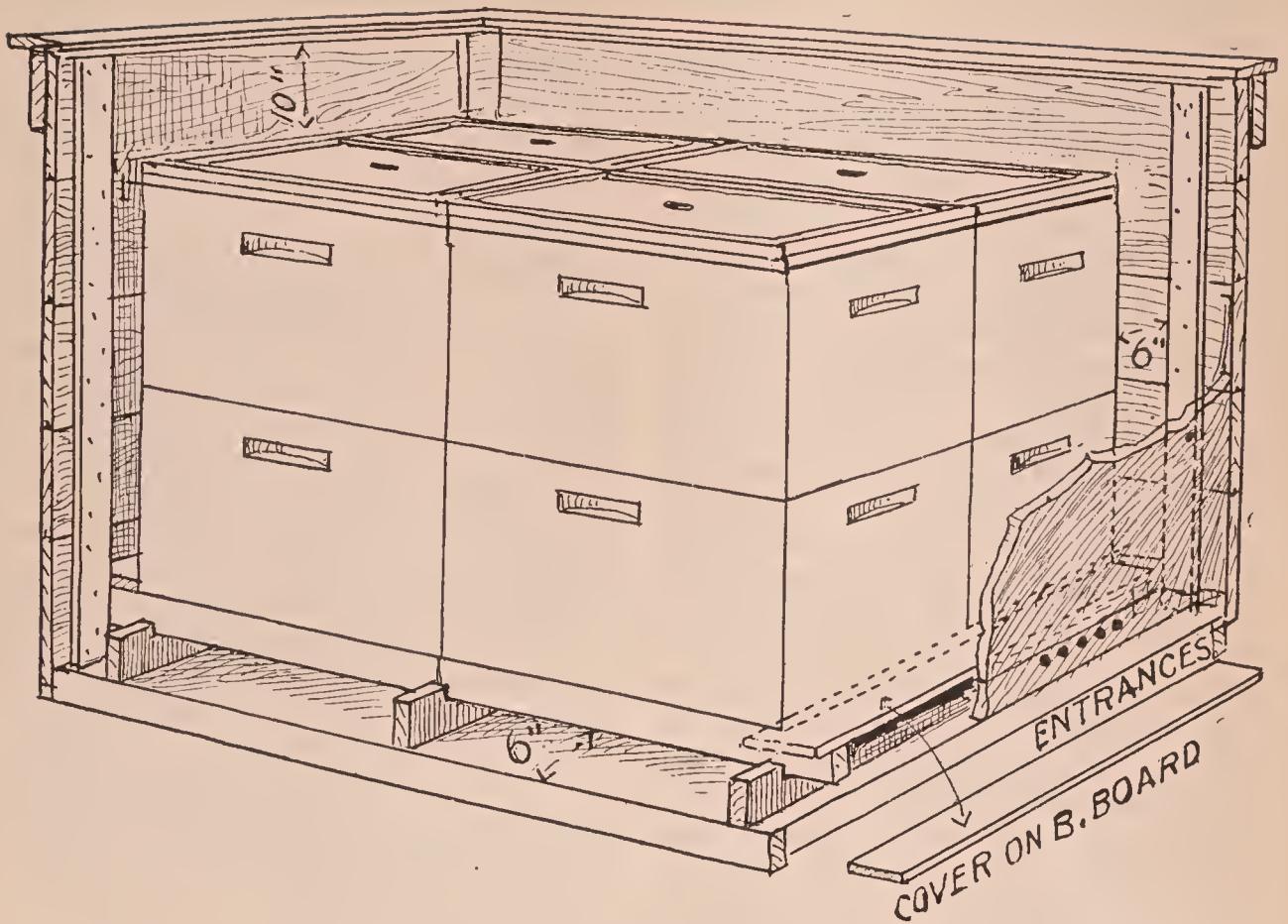
Fig. 9.—This is the plan recommended by Dr. E. F. Phillips and by a good many other beekeepers for wintering bees outdoors in single-walled hives. It contemplates a winter case made up of panels which are held together by means of screws or nails at the corners. This case should provide six inches of packing around the sides and ends, at least four inches under the bottoms of the hives, and at least ten inches on top. Phillips particularly recommends wintering in two-story hives. First, a double brood-nest makes a relatively deep wintering space. Second, it provides ample room for breeding in the spring. Third, it provide ample stores. Fourth, no attention is needed during spring. Spring management is practically eliminated. Attention is drawn to the five-hole entrance. All the holes except one in the center, according to Phillips, should be closed during cold weather. As spring approaches, one or more holes are opened up. The only objection to the plan here shown is the expense.
