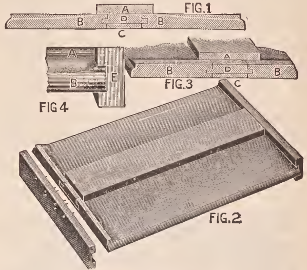
Excelsior flat cover.
