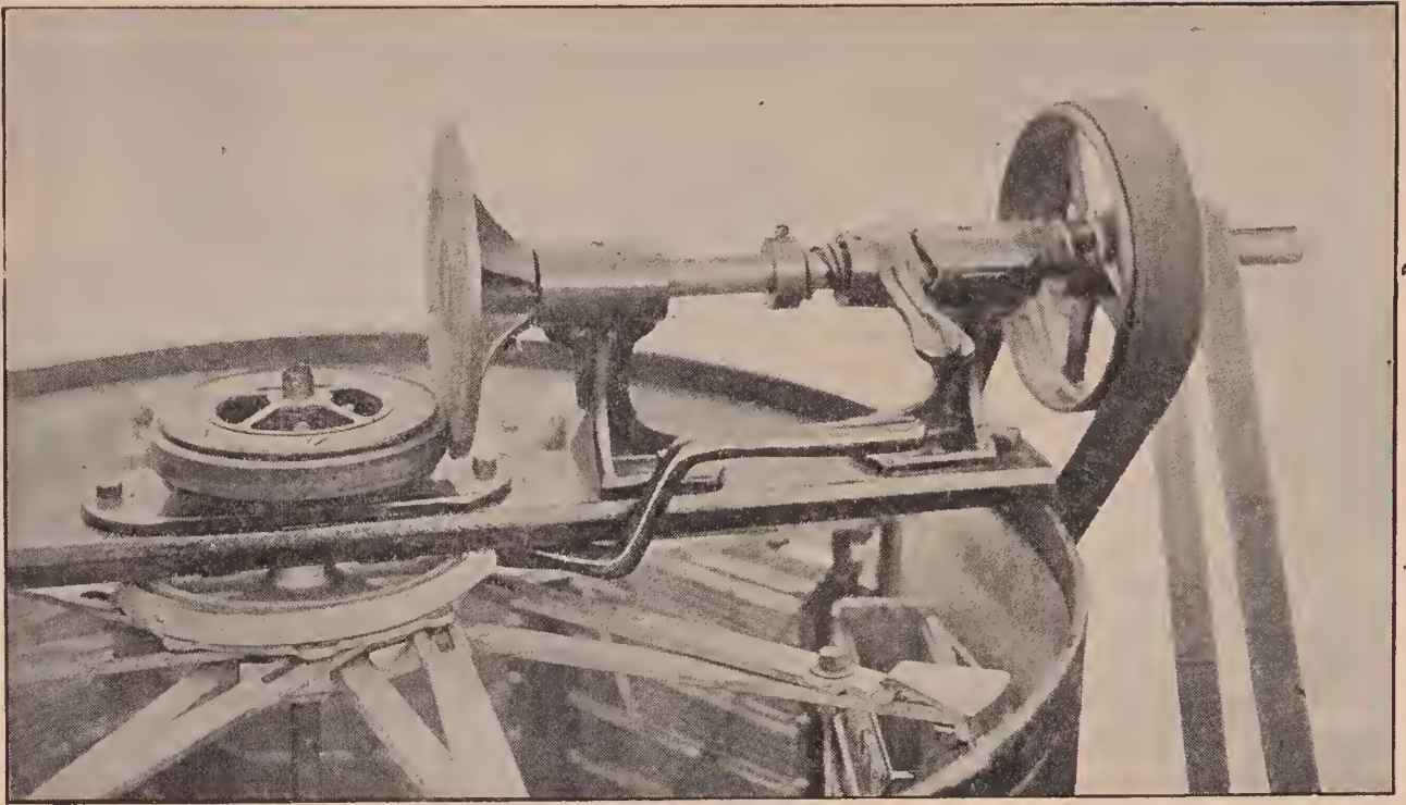
DETAIL OF FRICTION-DRIVE POWER EXTRACTING GEAR-BAR.
