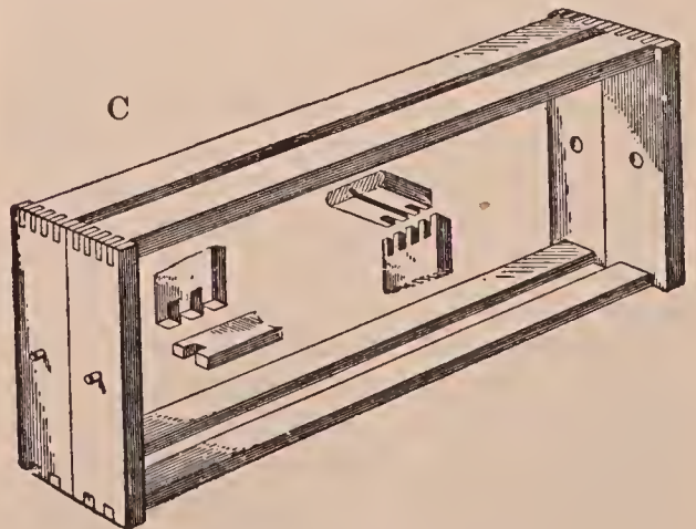
Danzenbaker closed-end frames.
