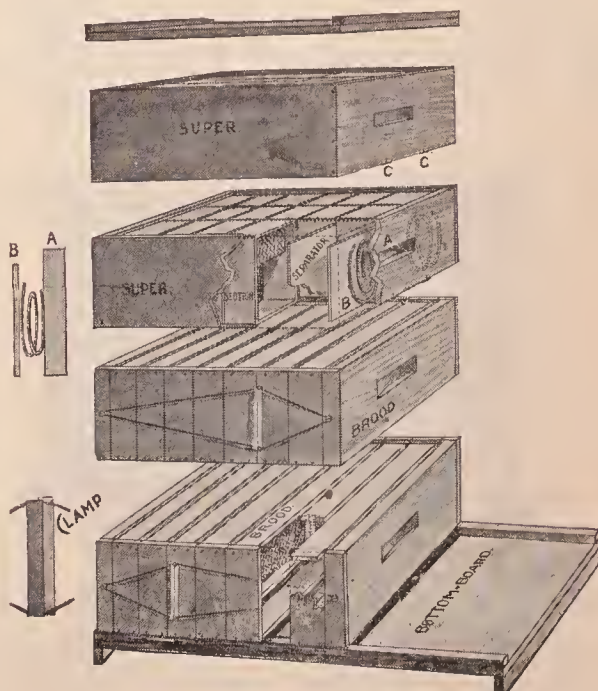
The Bingham Hive.
