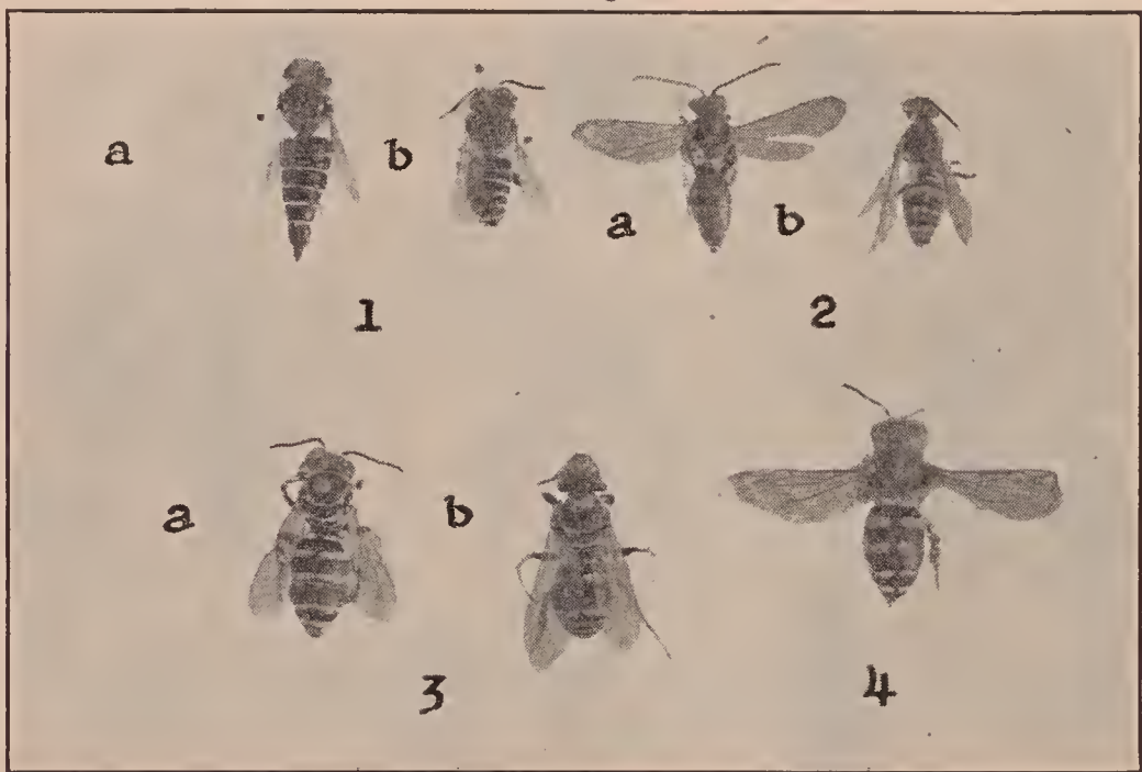
Fig. 5.—Parasitic bees: 1. Coelioxys rufitarsus ; a, female; b, male; 2. Nomada bella a, female; b, male; 3. Triepeolus donatus ; a, female; b, male; 4. Melecta miranda , female.
