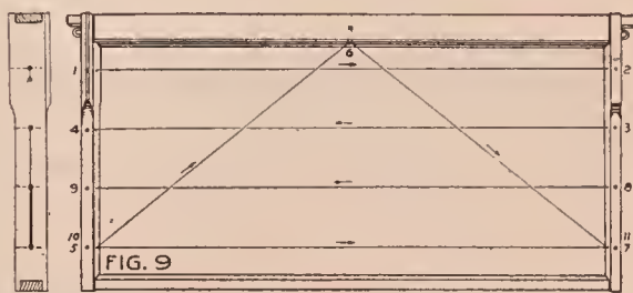
Fig. 9.—This is one of the best of any of the plans shown. The sheet of foundation should be placed between the diagonal and the four horizontal wires, when imbedding with electricity can be accomplished. It effectually prevents sagging of the foundation, but is not quite equal to the plans shown in Figs. 14 and 15.
