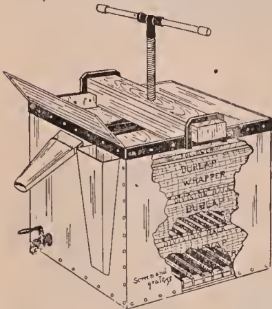
Fig. 5.—Hershiser hot-water wax-press.
