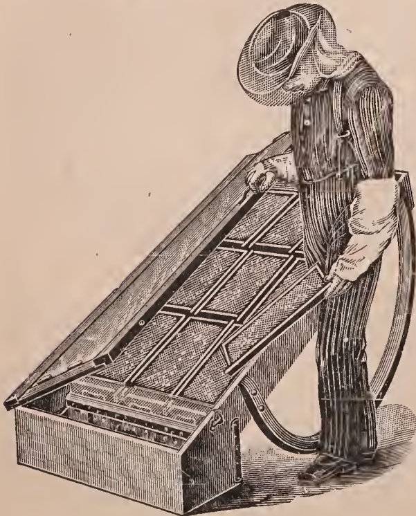
Fig. 1.—Boardman solar wax-extractor.
