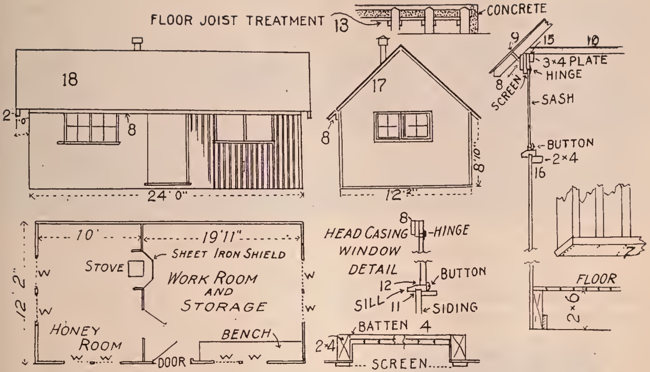
Neat design for both workshop and honey-room.
