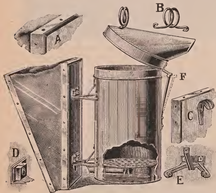
Fig. 1.—Details of the Root smoker—A.—Metal projection to aid the fingers in holding bellows; B.—Coiled wire handle; C.—Hook; D.—Lock nuts for legs; E.—Stamped metal legs; F.—Flexible hinge.
