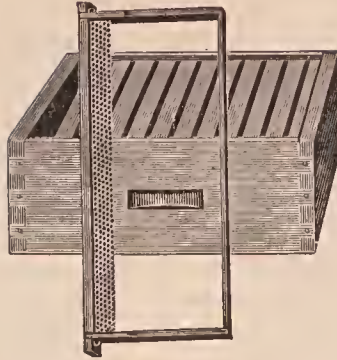
Fig. 2. Ten-frame shallow extracting super.
