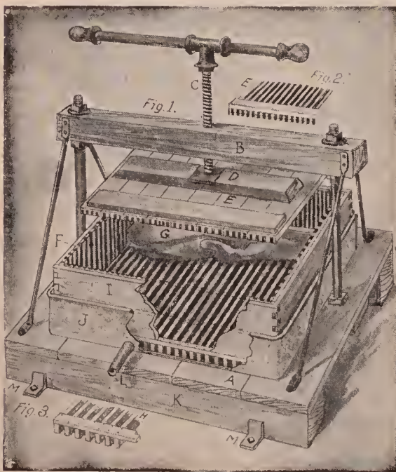
Fig. 8.—The original Hatch-Gemmell wax-press.
