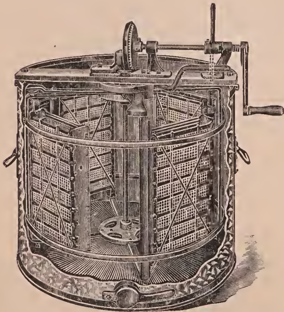
Root automatic four-frame extractor.
