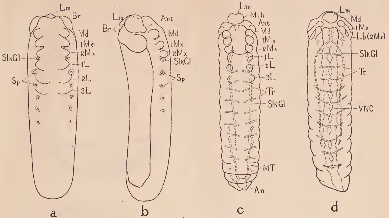
FIG. 2.—Three stages to the development of the egg (greatly magnified). The earliest stage at which the rudiments of the appendages are seen is represented by a and b; a, egg seen from the ventral (lower) side; b, from the right side; c, later stage, showing the development of the mouth parts, silk glands, etc.; d, embryo just prior to hatching, the development within the egg being completed; An, anus; Ant, antenna; Br, brain; 1L, 2L, 3L, thoracic legs; Lb, labium (lower lip); Lm, labrum (upper lip); Md, mandible; MT, malpighian tubules; 1 Mx, 2Mx, first and second maxillæ; SlkGl, silk gland; Sp, rudiment of spiracle; Tr, trachea; VNC, ventral nerve cord.
