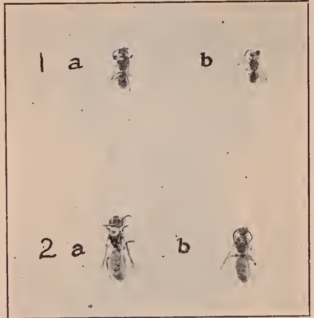
Fig. 1.—Primitive bees: 1, Prosopis modesta ; a, female; b, male. 2, Sphecodes ranunculi ; a, female; b, male. Tongues short, bodies smooth and nearly hairless, without pollen-brushes. The pollen and nectar are masticated as collected, and the regurgitated liquid is stored in the cells as food for the larvae.
