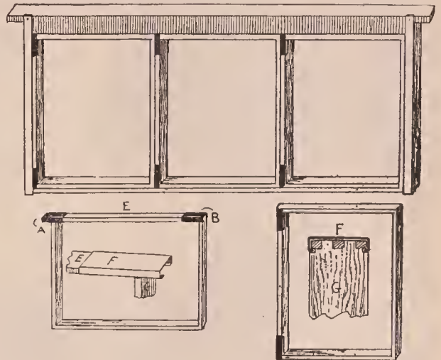
Twin-nuclei frame.
