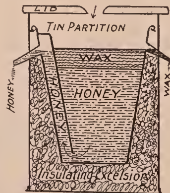
Sechrist's honey and wax separator.
