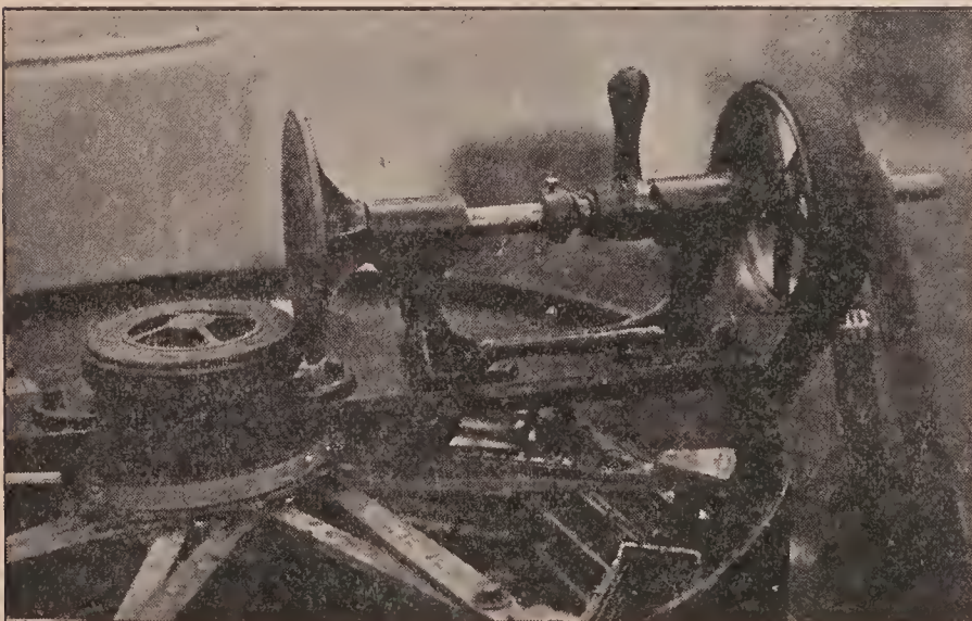
The cam lever in a vertical position. The disc is thus crowded over against the paper wheel on the vertical shaft so that the reel turns.
