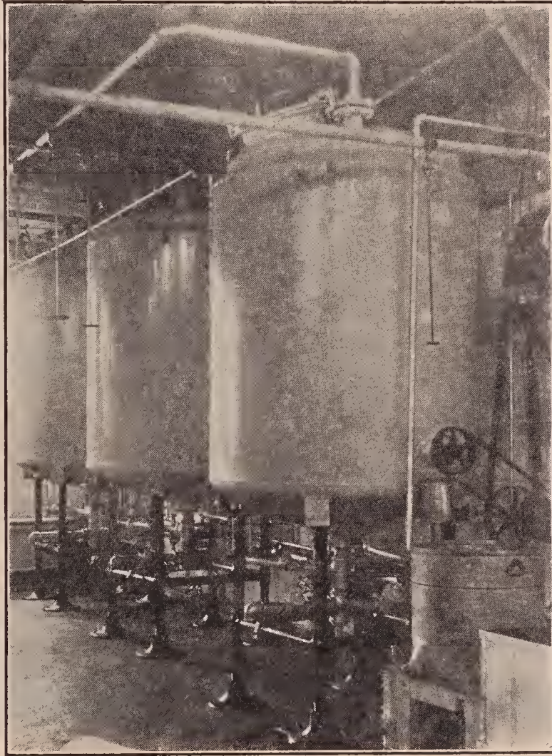
Bottling and packing of honey has kept pace with the advanced methods and improvement in equipment of the beekeeping industry in general. These jacketed steel tanks, glass enameled on the inside, in contrast with the old, unsanitary, open tanks, are convincing proof that honey packed by this method reaches the consumer in the most sanitary condition possible.
