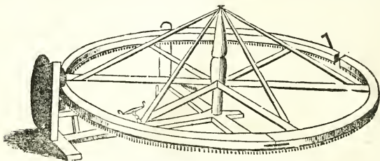
RIM-HORSE POWER.
