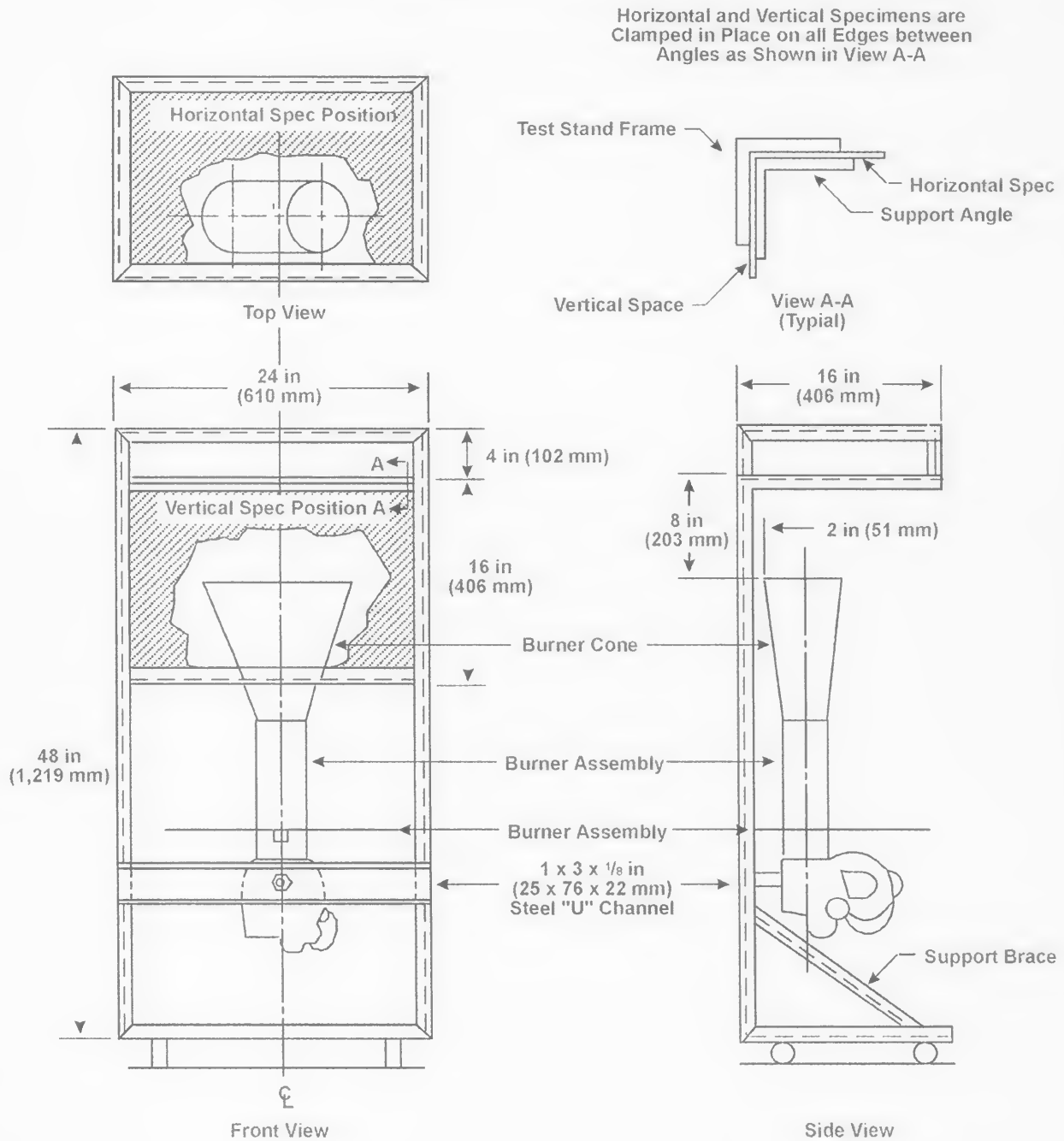
Figure 1: Test Apparatus for Horizontal and Vertical Mounting
