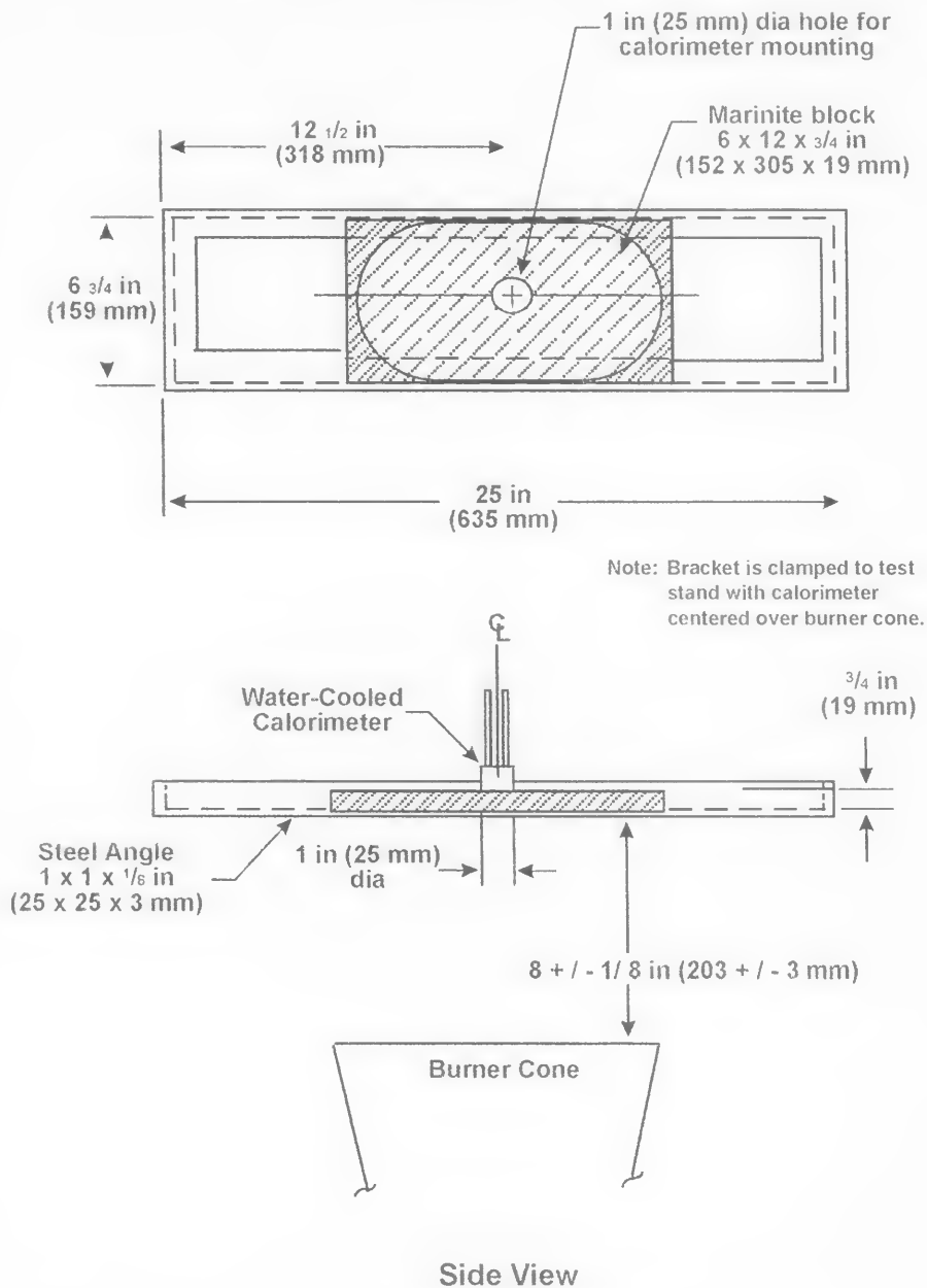
Figure 2: Calorimeter Bracket
