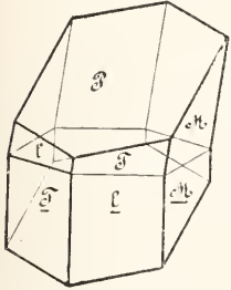
Fig. 6. Albit (Periklinzwilling). M = \{010\} \infty P \infty; P = \{001\} \infty P; T = \{1\bar{1}0\} \infty P; l = \{110\}, \infty P/.
