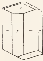
Fig. 15a. Turmalin. Trigonales Prisma I. Art. p = \{10\bar{1}0\} + \frac{\infty R}{2} ; hexagonales Prisma II. Art. m = \{11\bar{2}0\}, \infty P_2 ; am oberen Pol: Positive trigonale Pyramide: r = \{10\bar{1}1\}, \frac{R}{2} ; negative trigonale Pyramide: n = \{01\bar{1}2\}, -\frac{1}{2} \frac{R}{2} ; am unteren Pol: positive trigonale Pyramide. r = \{01\bar{1}1\}, +\frac{R}{2} .
