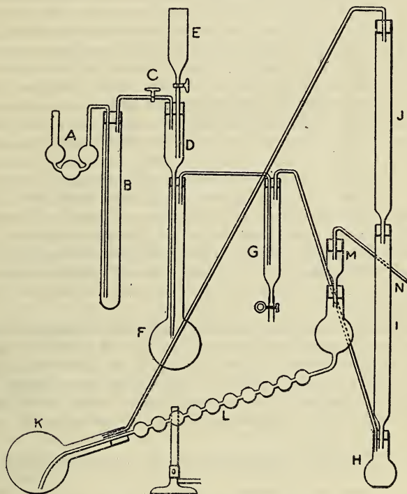
FIG. 1.—Apparatus for carbon determination.
