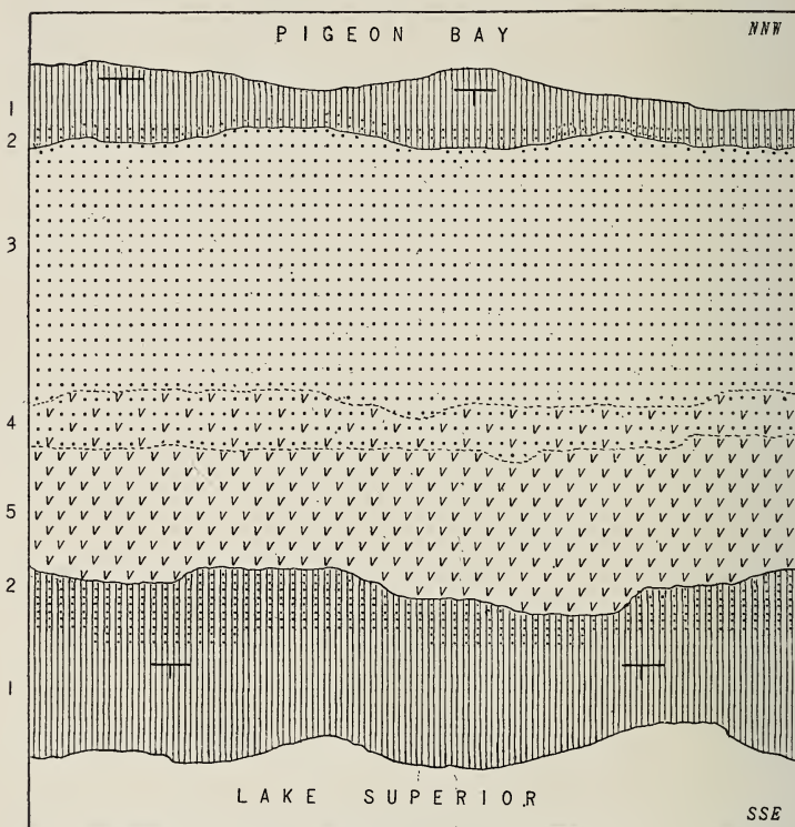
FIG. 4. Diagrammatic map of part of Pigeon Point, Minnesota, showing general relations among the different rock formations; after Bayley.
