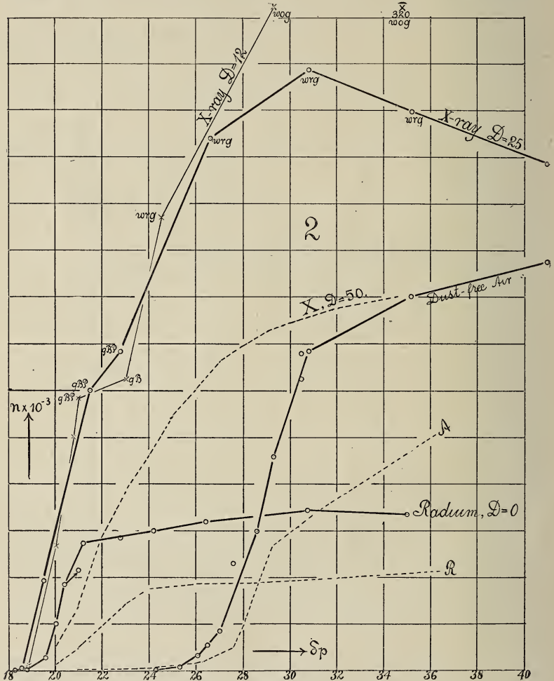
FIG. 2.—Charts for Table III showing the nucleation n in terms of the supersaturation (pressure drop \delta p ), for dust-free non-energized air, and for dust-free air energized by radium (10,000 \times , 10 mg.) from different distances D . The dotted curves show the corresponding cases (Dust-free air, A ; Radium, R ; X-rays, X ) for less rapid exhaustion (Table I). The vertical spaces represent 20,000 nuclei each.
