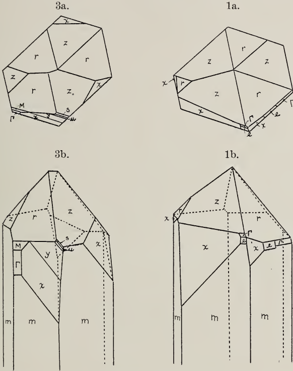
Orthographic and clinographic projections of quartz crystals from Rincon, California, from figs. 3 and 1, p. 126.
