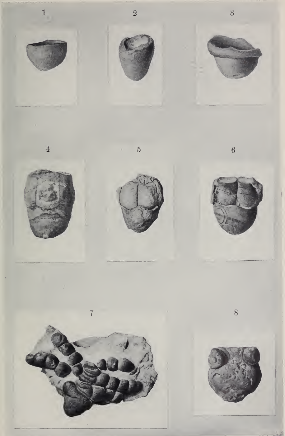
FIGURES 1-6.— Edriocrinus pocilliformis . FIGURES 7 and 8.— Brachioocrinus nodosarius .
