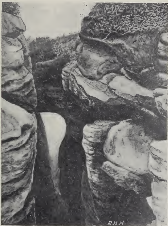
FIG. 2.—The North Adams Natural Bridge as seen from the south. 1893 Formerly the bridge probably extended nearly to the foreground of the picture.
