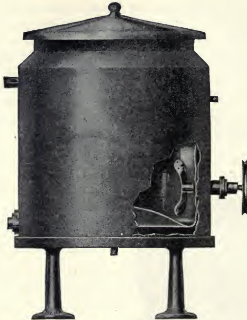
Fig. 38. Glass-enameled starter tank Courtesy Elyria Enameled Products Co.
