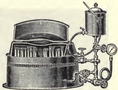
Fig. 98. Facile Steam Turbine Tester Courtesy D. H. Burrell & Co.
