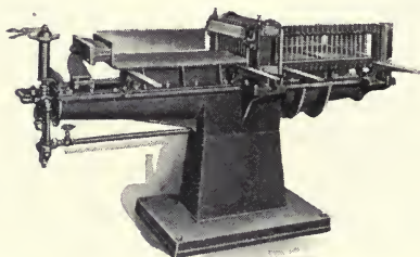
Fig. 75. C. F. Miller Hydraulic Cutter for Frozen or Otherwise Very Firm Butter
