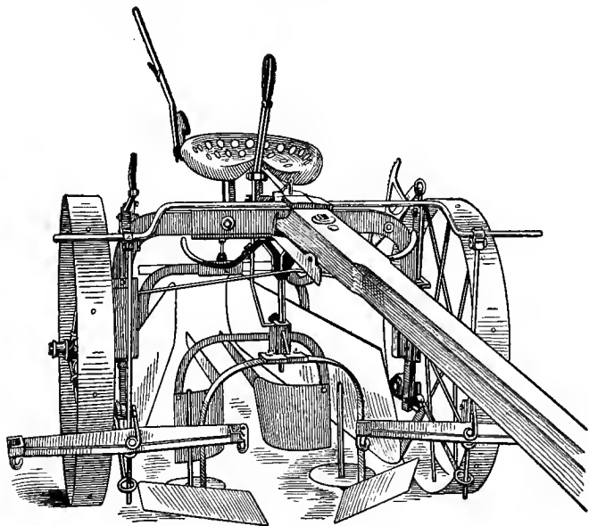
FIG. 77. CELERY HILLER
