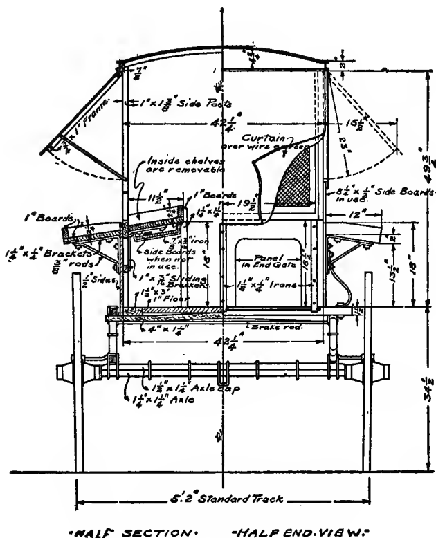
FIG. 55. RETAIL WAGON
