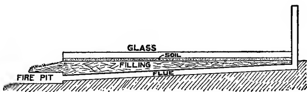
FIG. 20. FLUE-HEATED FRAME
