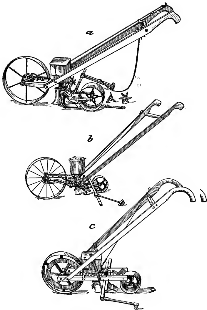
FIG. 29. DIFFERENT FORMS OF HAND SEED DRILLS
