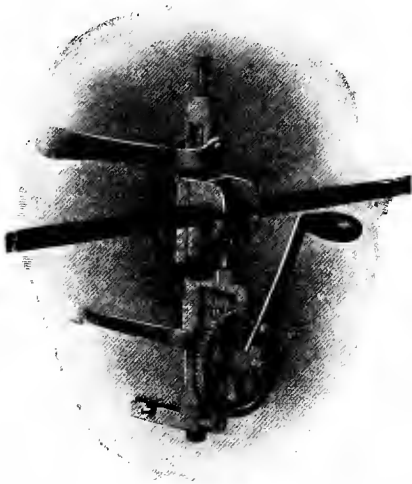
FIG. 15. DRILLING MACHINE FOR THE INSTALLATION OF THE SKINNER SYSTEM OF IRRIGATION
