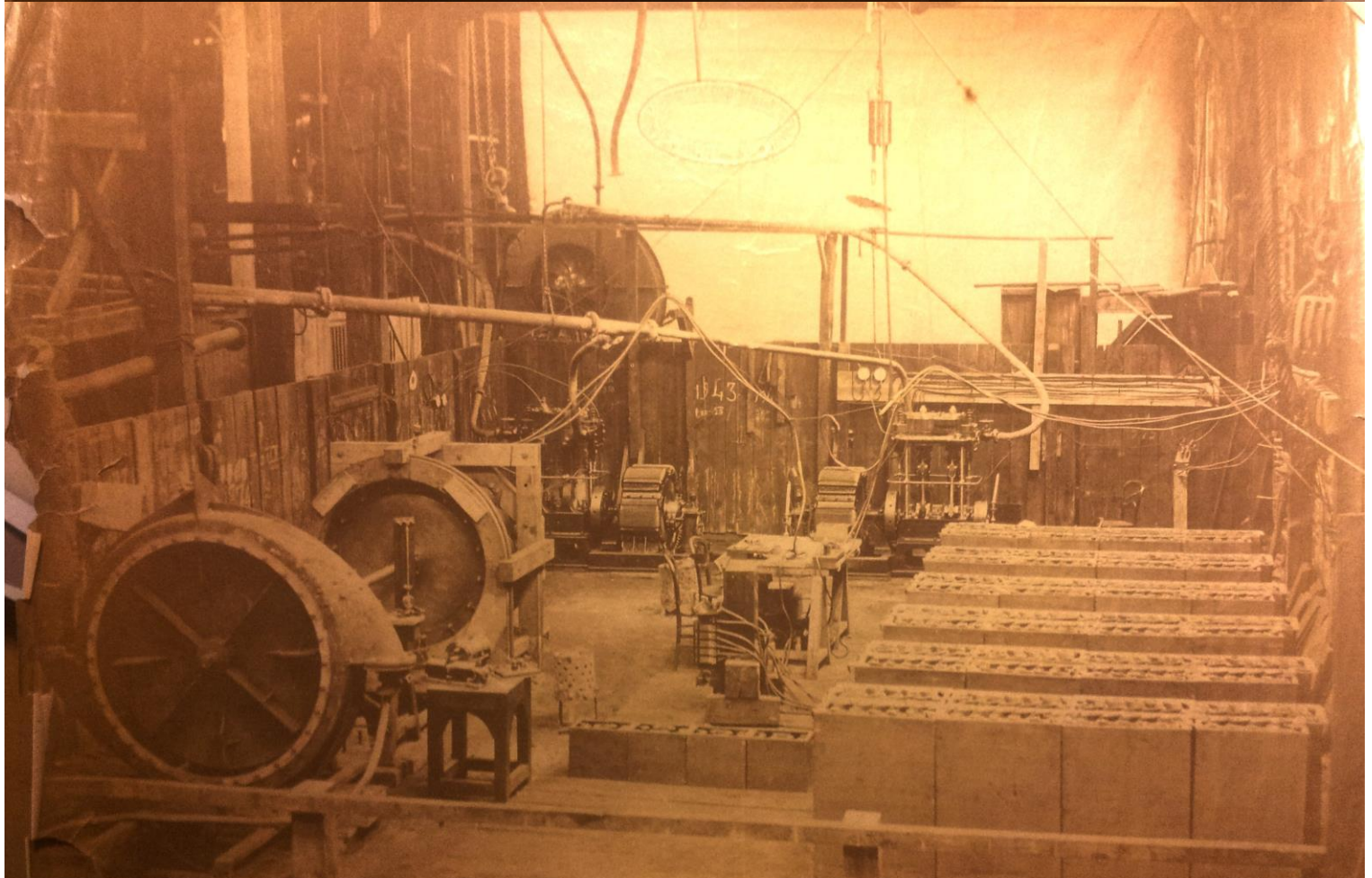
1888-04 – Tests of the A. C. KREBS multipolar electric motor for the GYMNOTE submarine in Le Havre (France) Academy of Sciences: " Test of an electric motor powered by accumulators intended for an underwater boat ".
