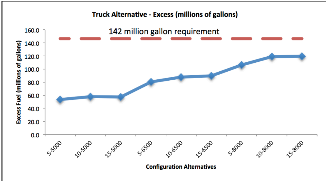
Figure 27. Excess Fuel (millions of gallons) versus 100% of consumed fuel
