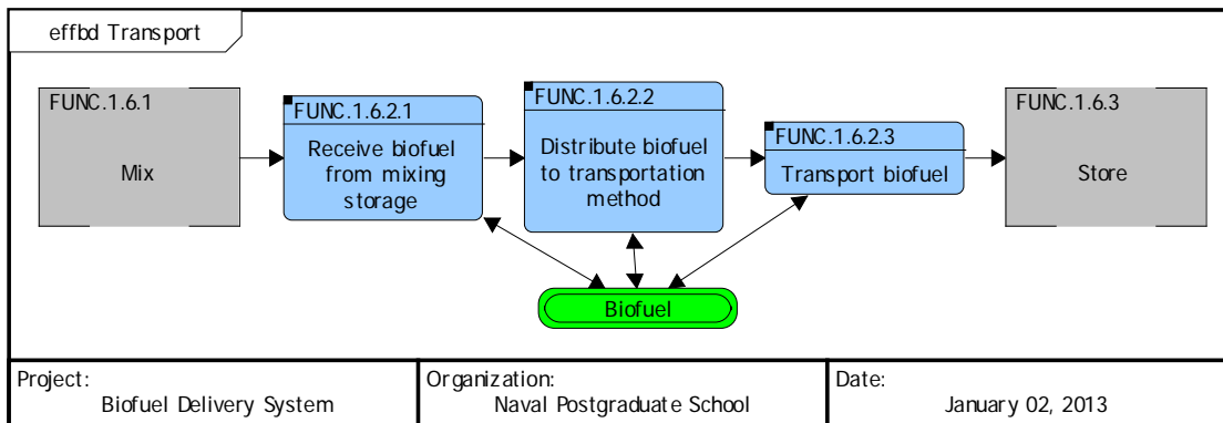
Figure 63. Transport (EFFBD)
