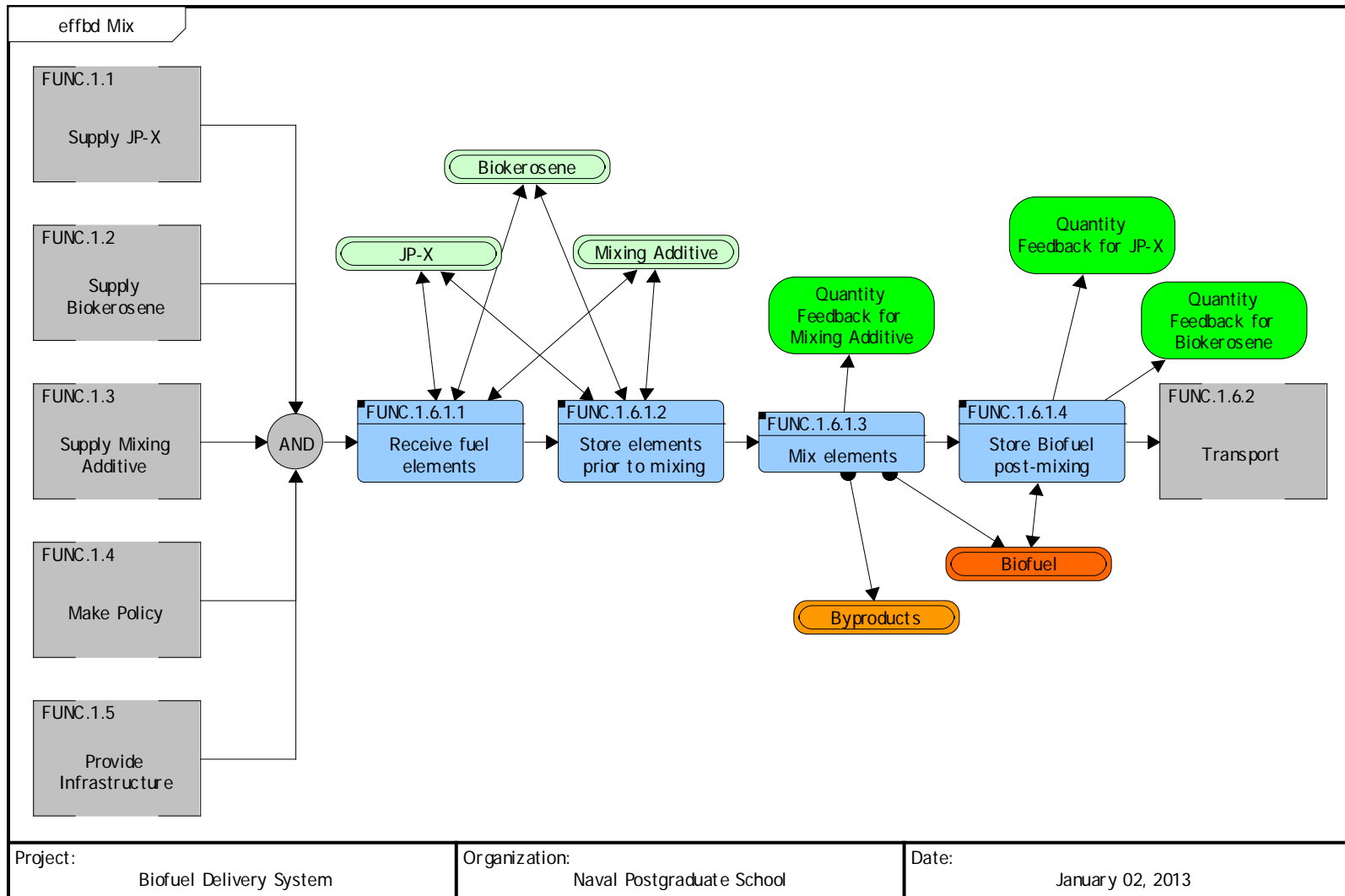
Figure 57. Mix (EFFBD)
