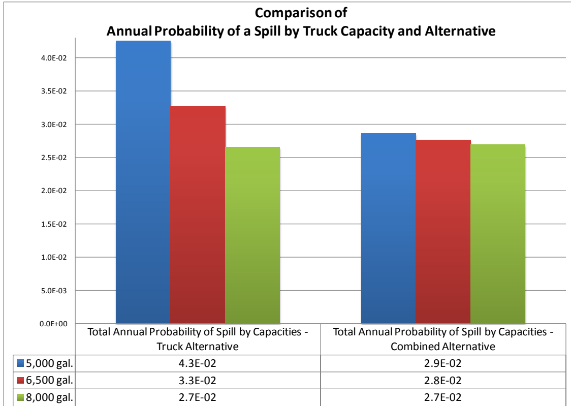
Figure 51. Annual Probability of a Spill – Alternative Comparison
