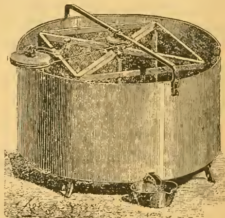
Fig. 3—Hruschka's Honey-Extractor.
