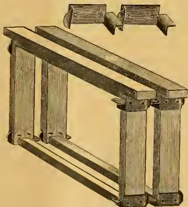
The Stephens' Frame-Spacer.
