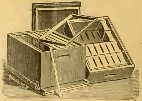
The "St. Joe" Hive.
