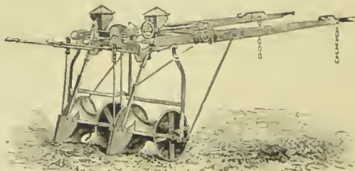
FIG. 70.—TWO-ROW TURNIP SOWER.
