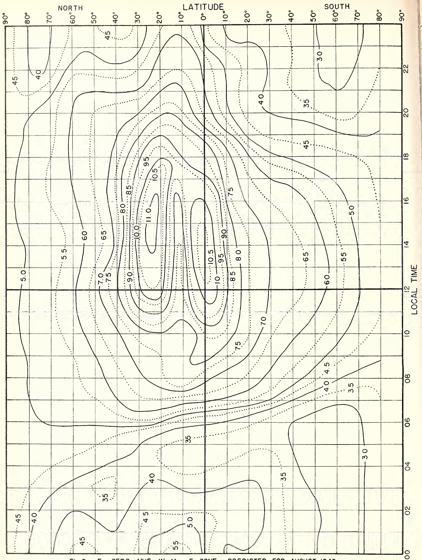
Fig.9. F 2 ZERO-MUF, IN Mc, E ZONE, PREDICTED FOR AUGUST, 1945.
