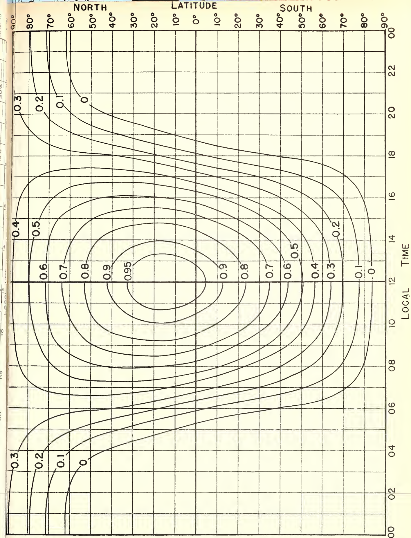
Fig. 16. ABSORPTION INDEX CHART (EXCLUDING AURORAL ABSORPTION) FOR AUGUST.
