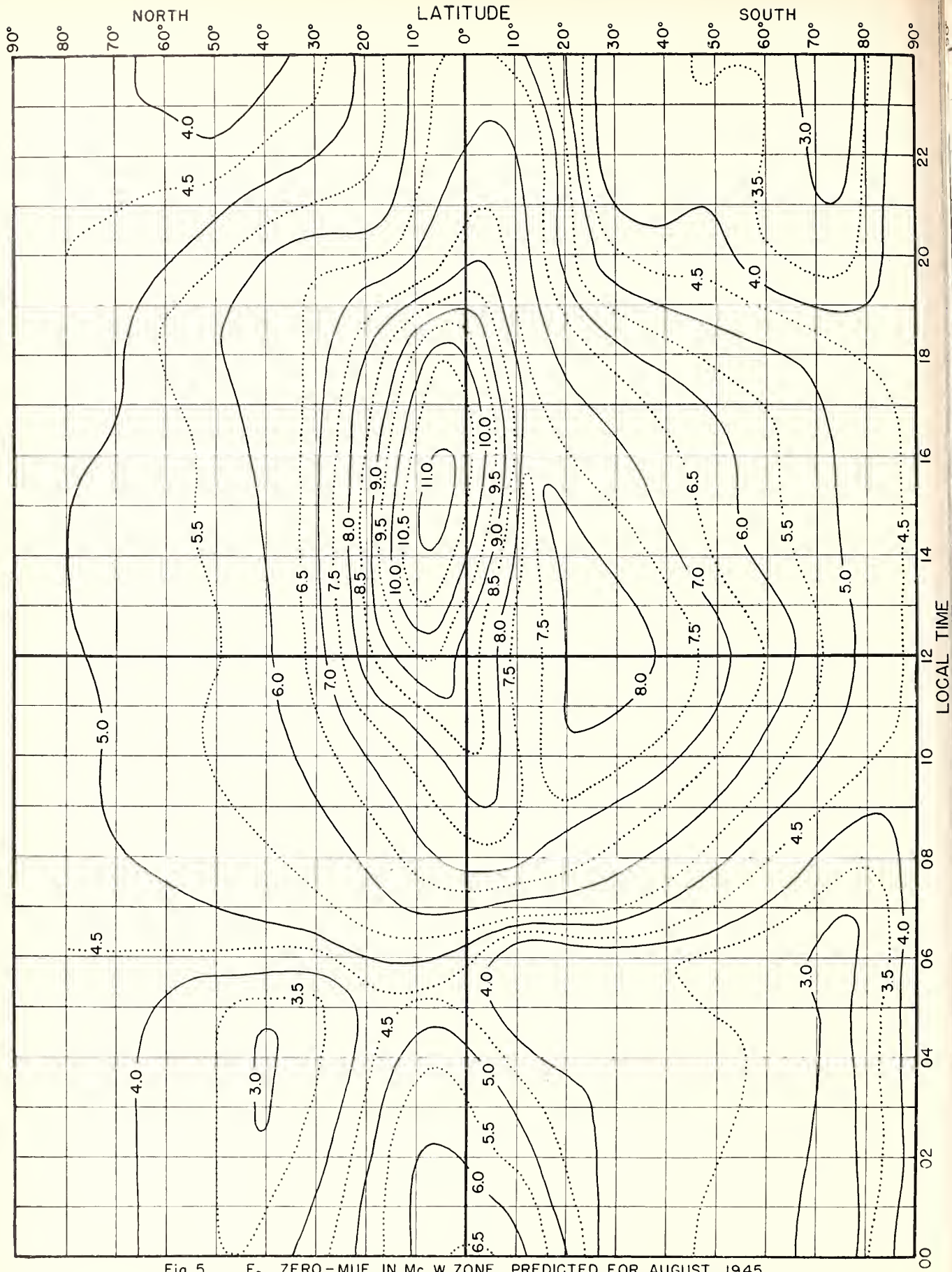
Fig. 5. F_2 ZERO-MUF, IN Mc, W ZONE, PREDICTED FOR AUGUST, 1945.
