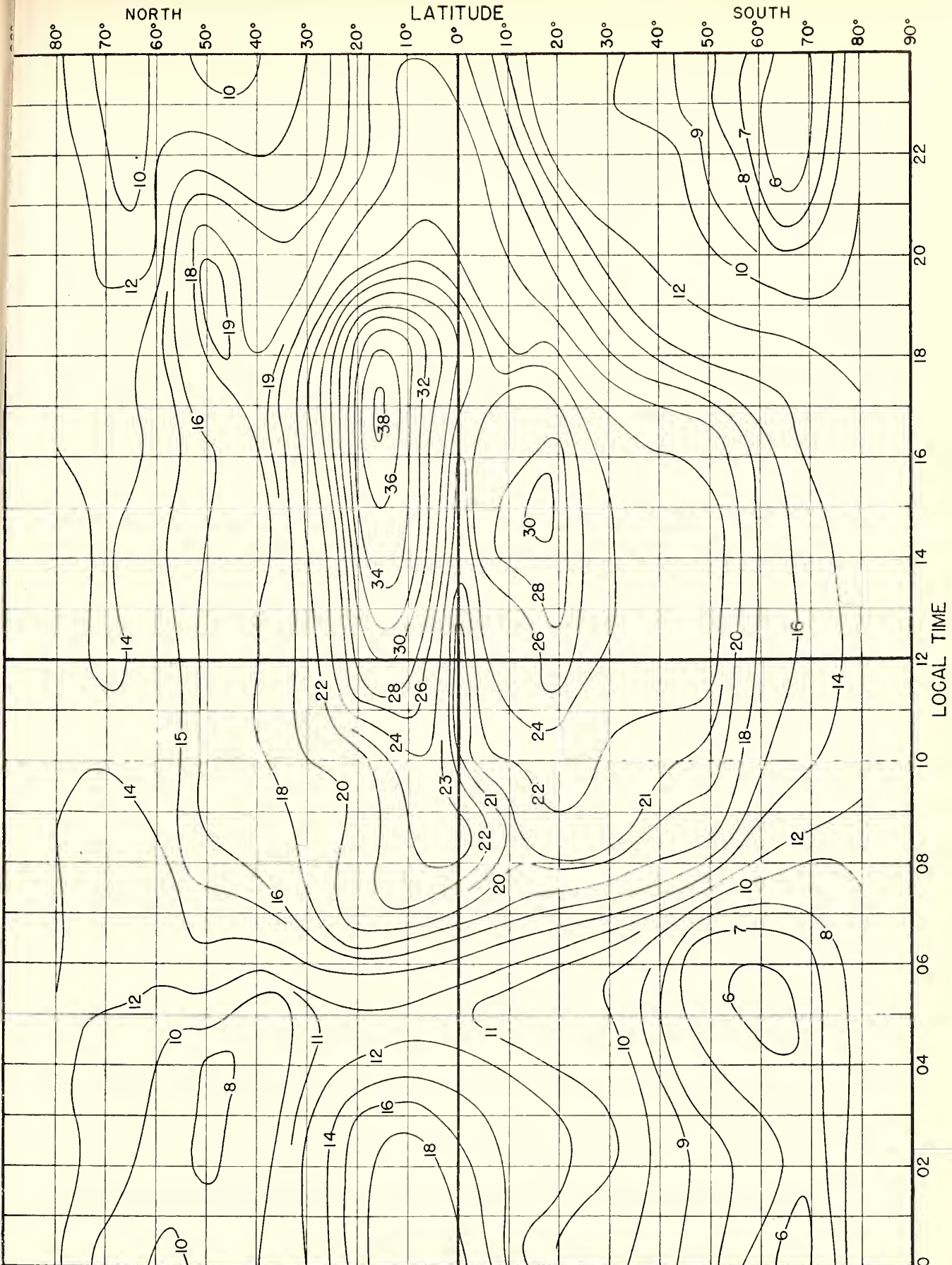
Fig. 8. F 2 4000-MUF, IN Mc, I ZONE, PREDICTED FOR AUGUST, 1945.
