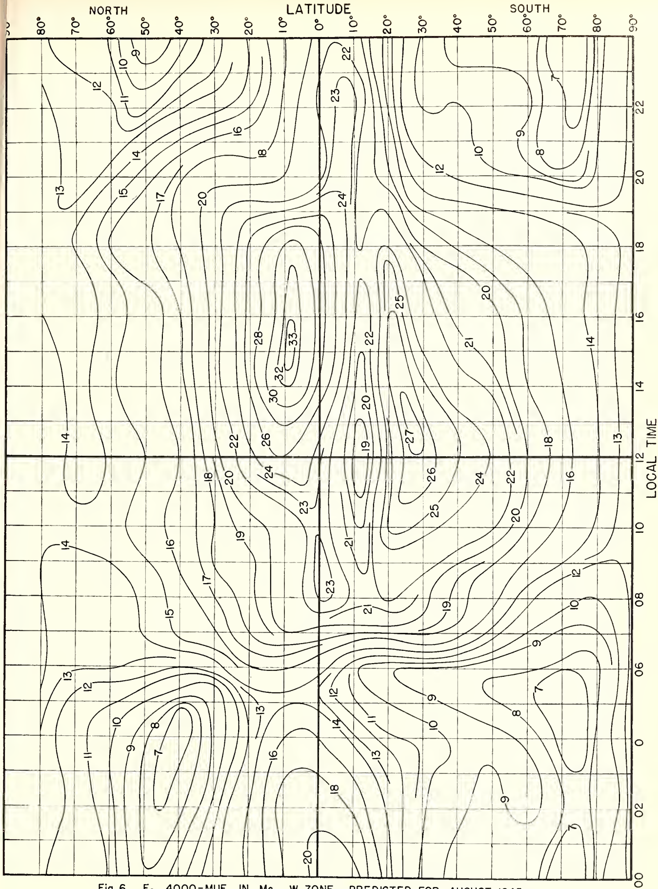
Fig. 6. F_2 4000-MUF, IN Mc, W ZONE, PREDICTED FOR AUGUST, 1945.
