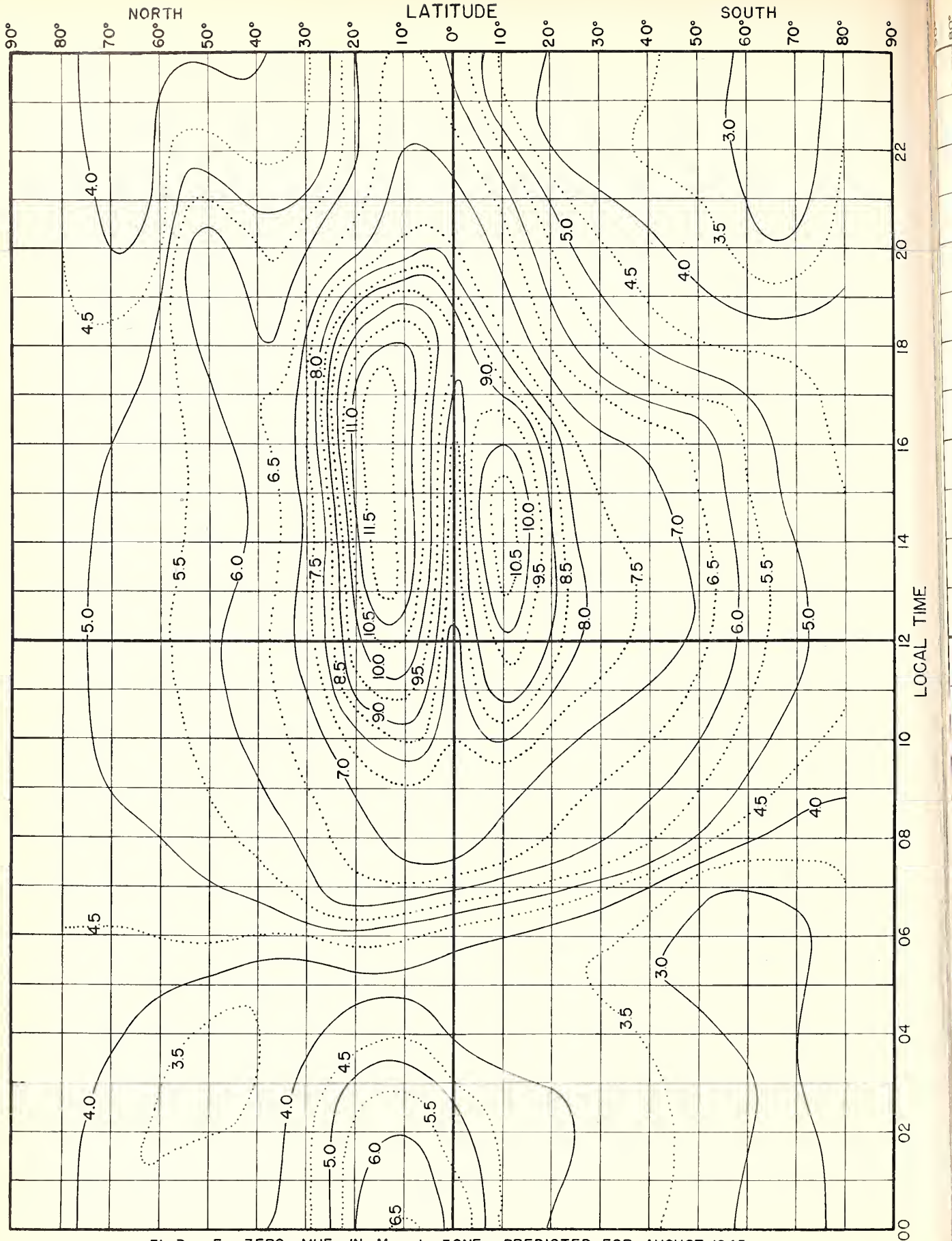
Fig.7. F 2 ZERO-MUF, IN Mc, I ZONE, PREDICTED FOR AUGUST, 1945.
