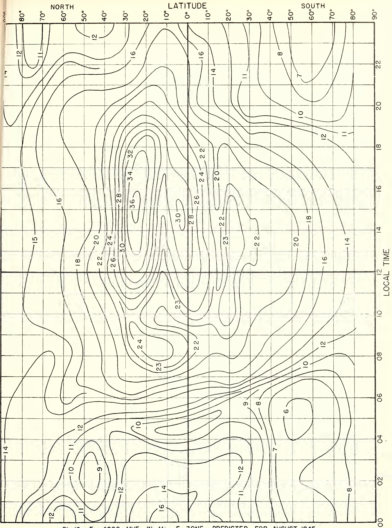
Fig.10. F_2 4000-MUF, IN Mc, E ZONE, PREDICTED FOR AUGUST, 1945.
