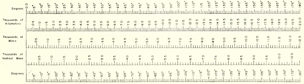
Fig. 4. NOMOGRAM (AFTER D'OCAGNE) FOR OBTAINING GREAT-CIRCLE DISTANCES, BEARINGS, LATITUDE AND LONGITUDE OF TRANSMISSION CONTROL POINTS, SOLAR ZENITH ANGLES. CONVERSION SCALE FOR VARIOUS DISTANCE UNITS.
