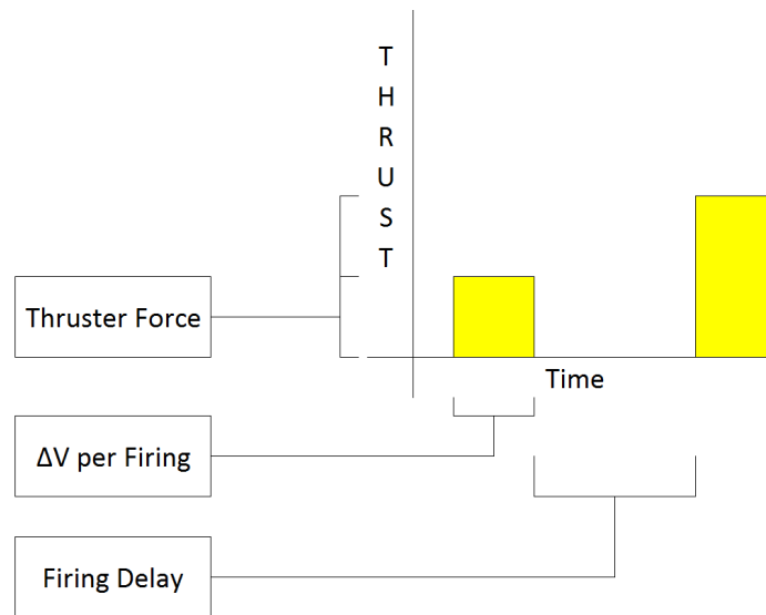
Figure 3.4. Visual depiction of spacecraft thrust parameters.
