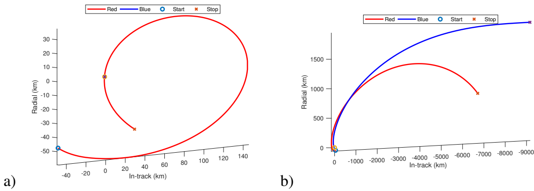
Figure 5.6. Relative position of spacecraft without Blue maneuver (a), and with continuous in-track Blue maneuver (b). NOTE: different axis.
