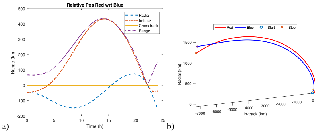
Figure 5.15. Position vs time for single direction pulse toward host (a), and relative position of the two spacecraft (b).
