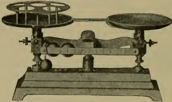
FIG. 32—CREAM-TESTING SCALES
