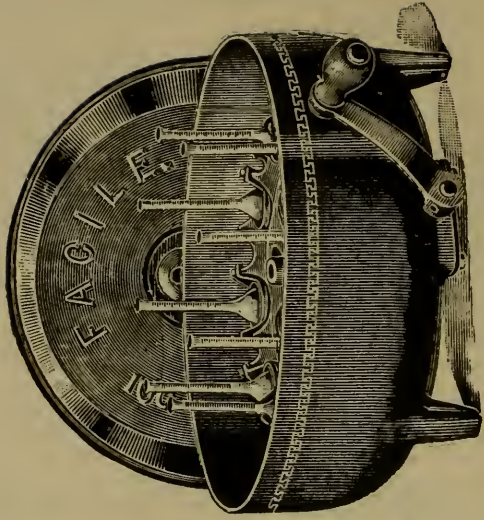
FIG. 15—HAND-TESTER
