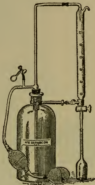
FIG. 13 AUTOMATIC BURETTE
