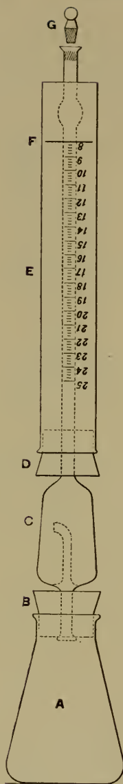
FIG. 36a GRAY'S APPARATUS READY FOR USE IN TESTING WATER IN BUTTER
