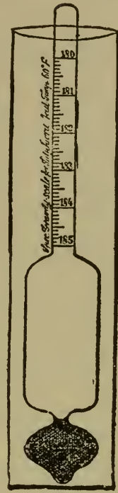
FIG. 18 HYDROMETER FOR TESTING STRENGTH OF SULPHURIC ACID
