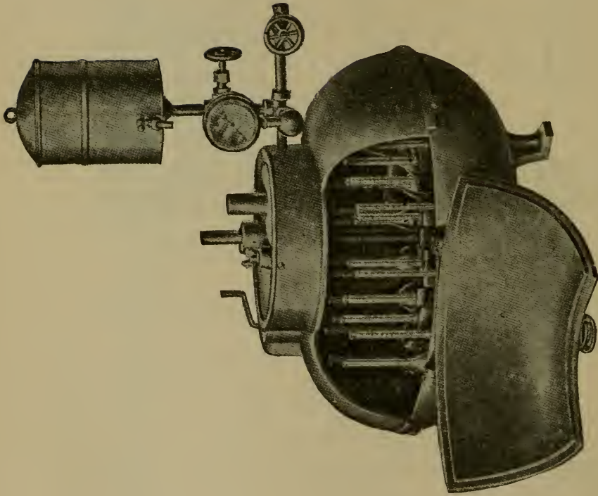
FIG. 14—STEAM-TURBINE TESTER
