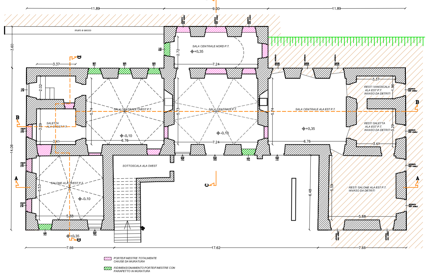
PIANO TERRA
