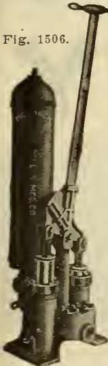
Fig. 1506. Outfit C, for One Lead of ½-in. Discharge Hose.
