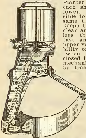
Valves Adjusted to Hill Drop.
