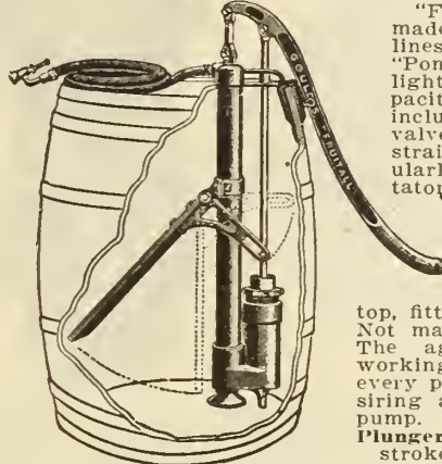
Fig. 1188. PUMP, EQUIPMENT, ETC.
