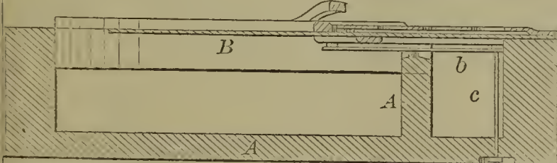
59069—F. E. Ramm— Piano Sounding Board.
