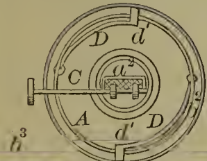
53031—J. Naylor—Steam Trap.
