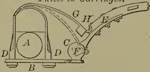
60296—S. H. Ward—Attaching Thills to Carriages.
