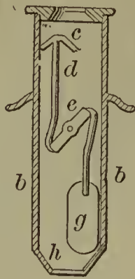
57948 W. P. Miller—Bottle Valve.
