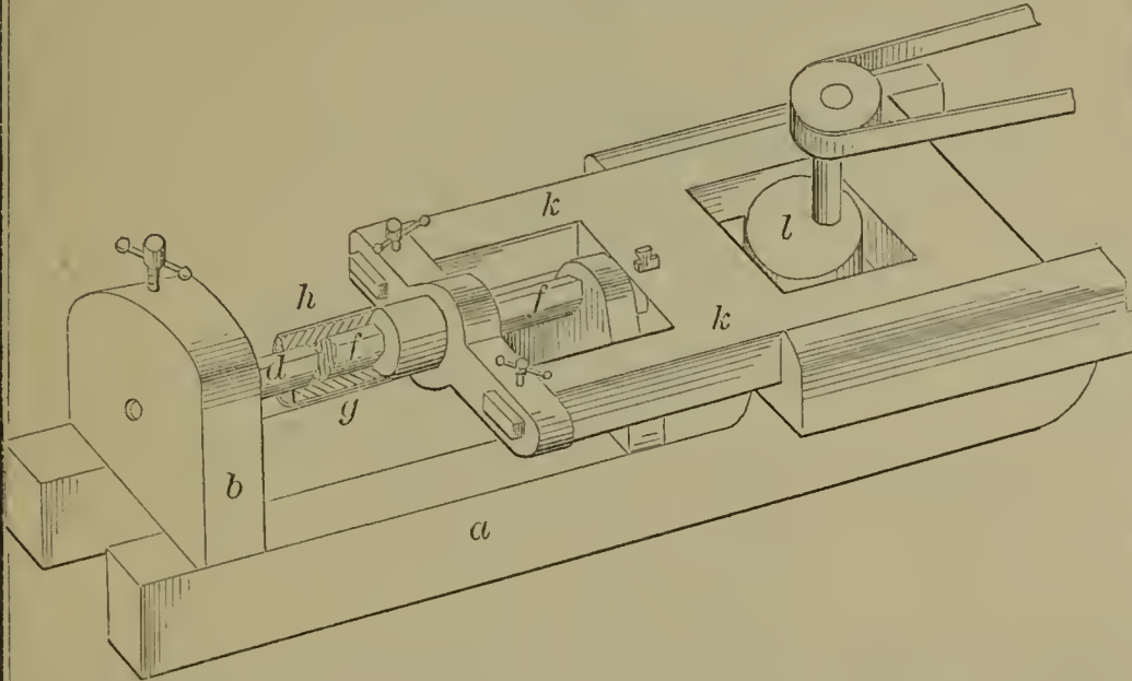
57045—R. Lyon— Riveting Machine.
