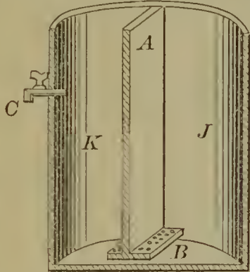
54414—W. H. Sangster— For Refining Petroleum.
