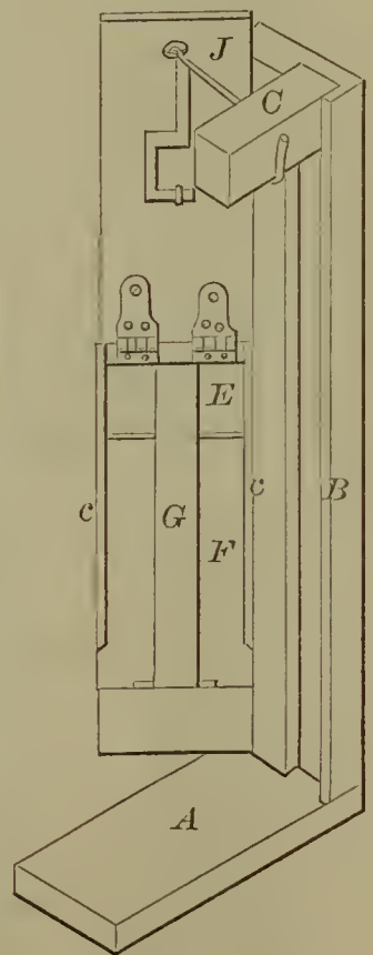
54436—J. C. Stoddard—Deflector for Car Windows.
