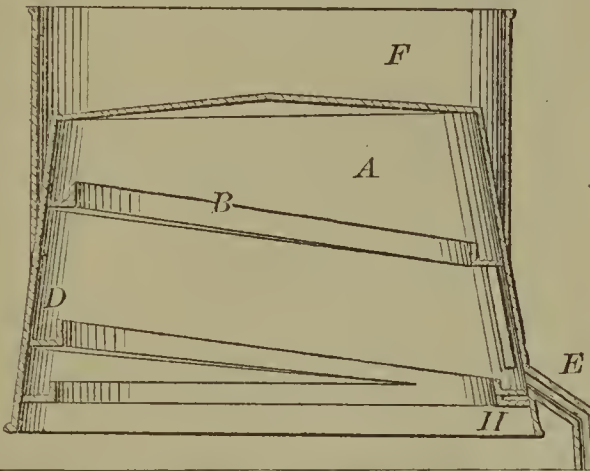
57934—E. Lyman—Gauge for Screw Cutting Tools.
