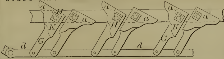
57404—E. Stiles—Safety Car Truck.
