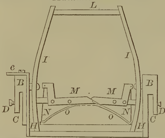
54460—Barker & Martin— Brick Press.
