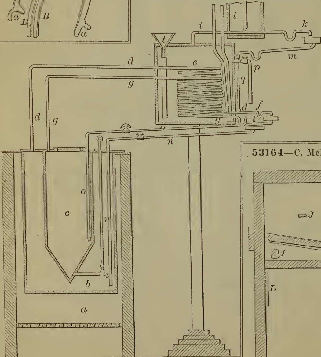
53167—A. Millochau—Distillation of Petroleum.
