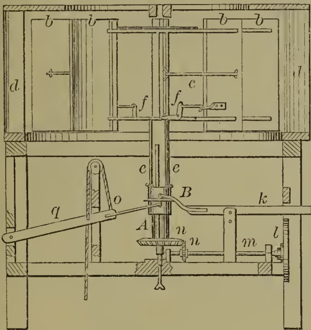
59729—D. Strunk— Wind Mill.
