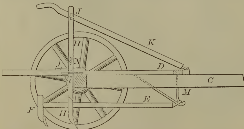
52222—L. Strickland—Cultivator Plow.
