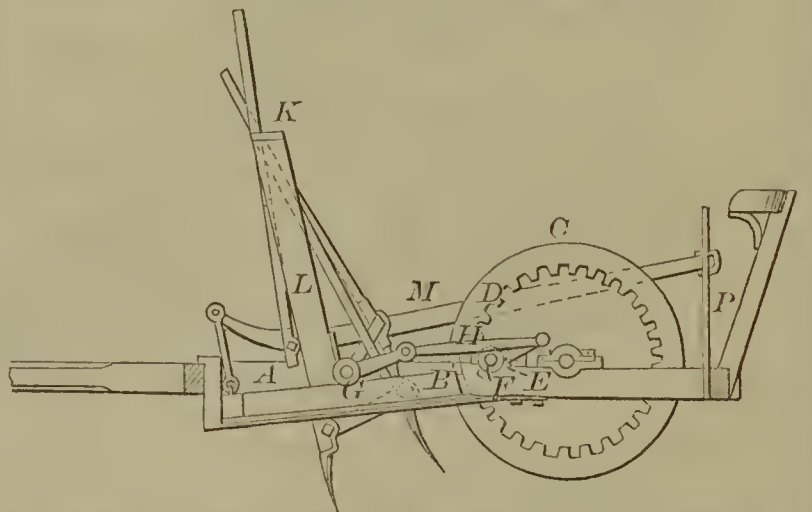
57242—S. Woodbridge—Soil Tilling Machine.
