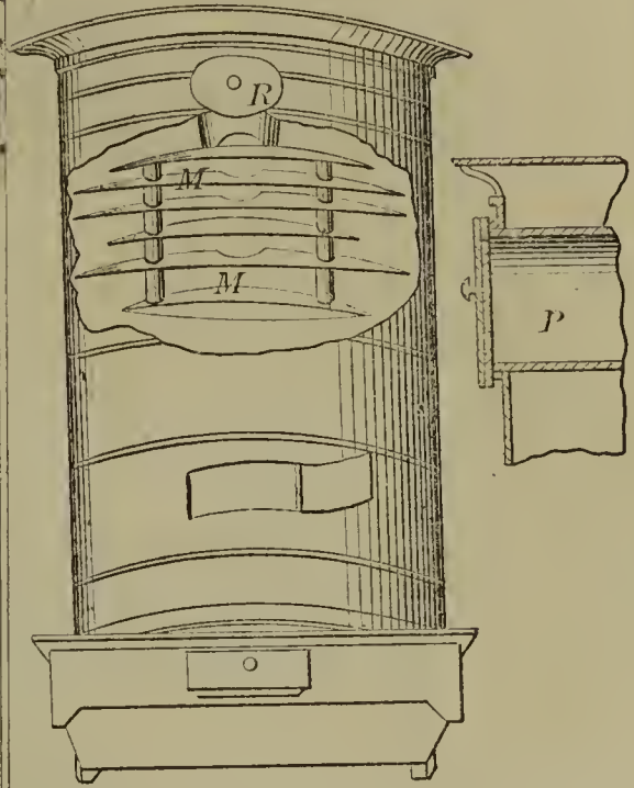
57481—Conver & Bothwick—Heat Radiator.
