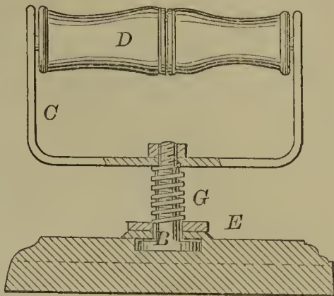
52514—J. Barton— Store Pipe Damper.
