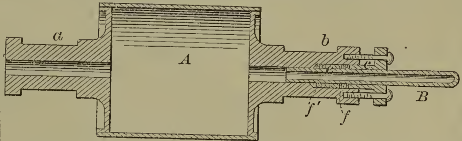
60369—J. Hatch— Packing Revolving Joints.
