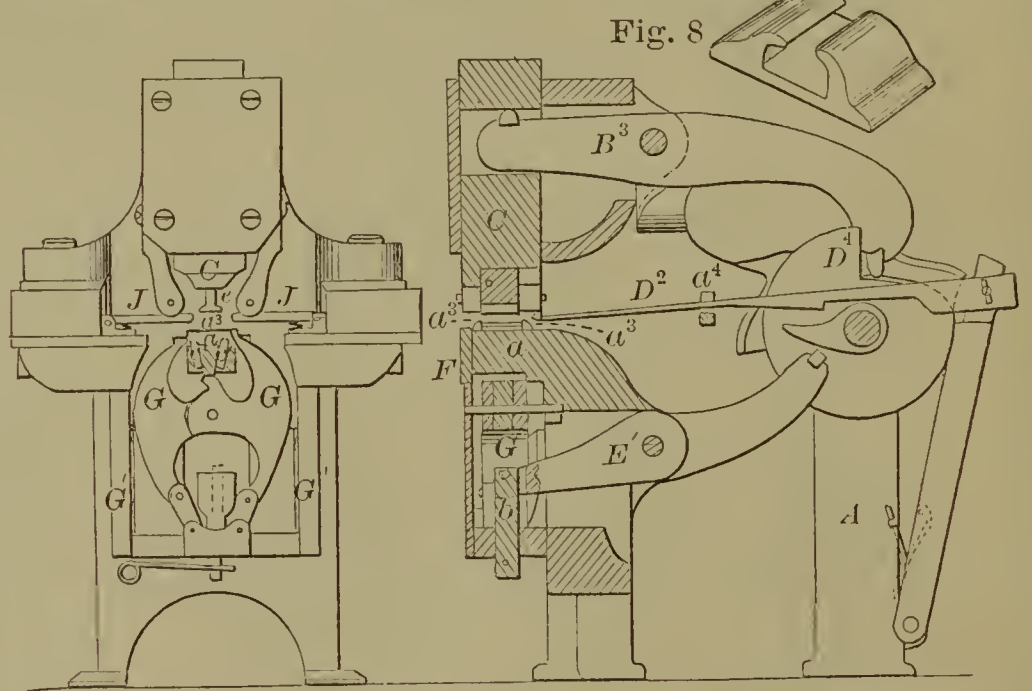
58155—W. V. Anden—Making Railroad Chairs.
