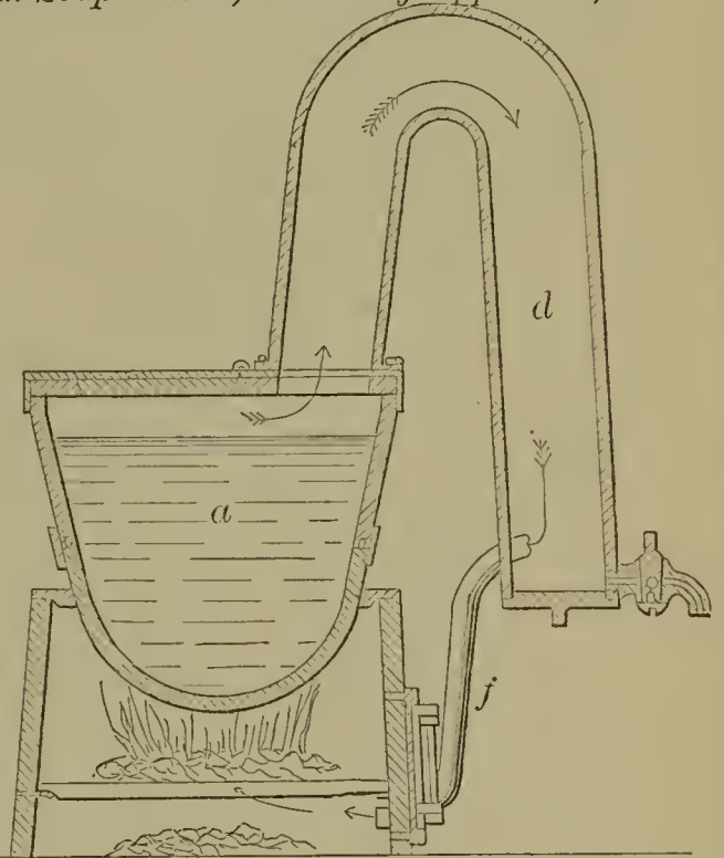
59260—W. H. Pinner—For Preventing the Escape of Gas from Soap Kettles, Rendering Apparatus, &c.
