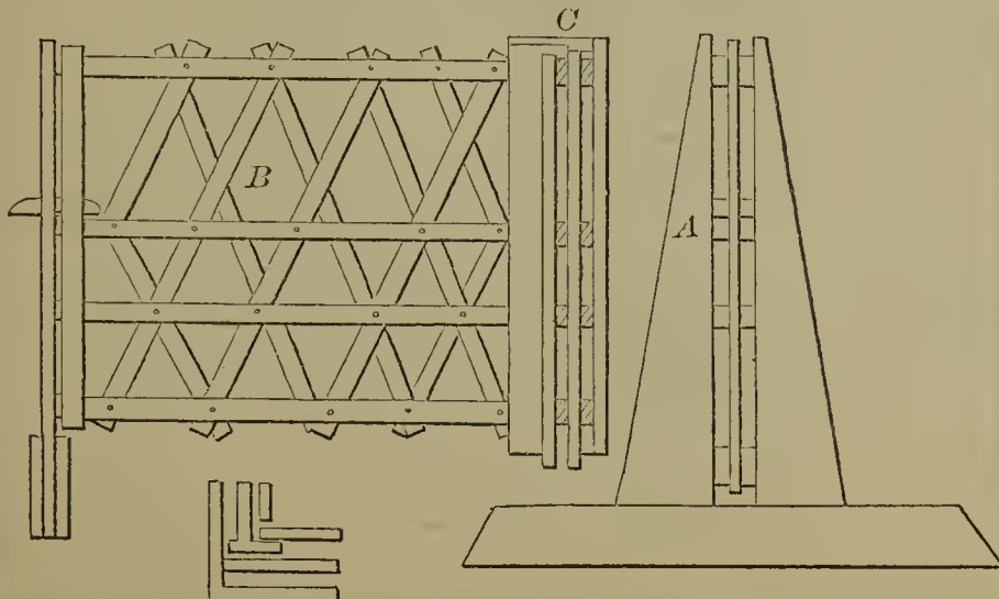
59185—F. C. Class— Portable Fence.
