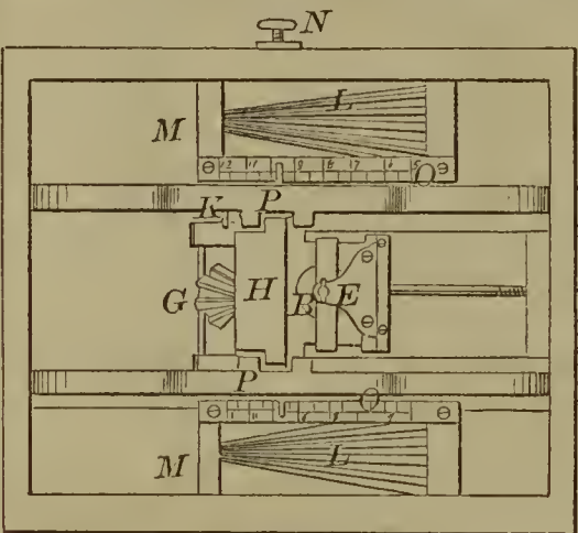
60619—J. Clarridge— Saw Set.
