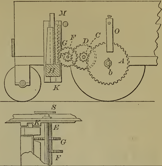
52916—E. Ward—Attaching Runners to Wheels of Wagons.
