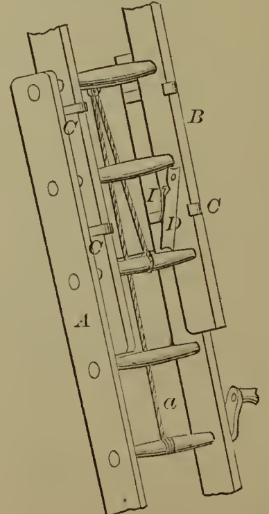
54778—A. Rogers— Extension Fruit Ladder.
