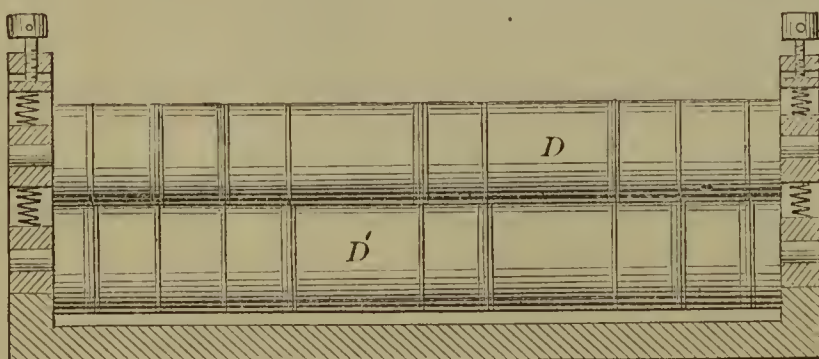
52817—H. Beebe—Apparatus for Folding Linen Bosoms.
