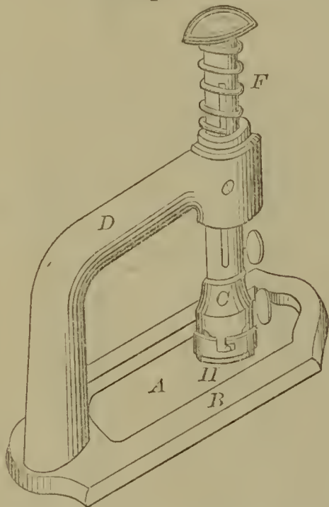
52666—S. B. Brague— Hand Stamp.
