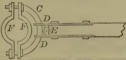
55515—B. McGrath— Boom Connection for Masts.
