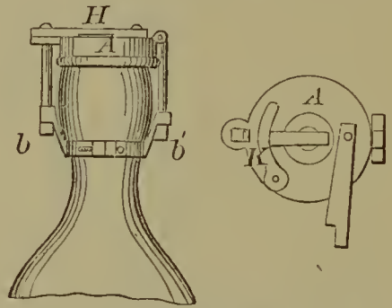
58175—R. Nutty—Drilling Machine.
