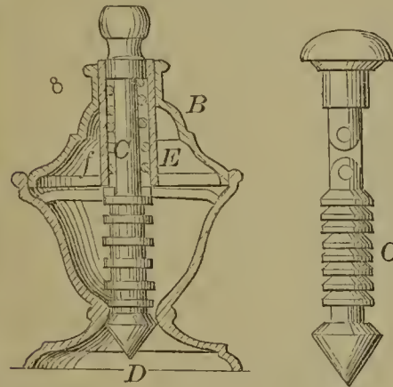
59406—J. M. Keepe— Sprinkler for Powdered Substances.
