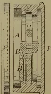
58271—D. Masten— Level.
