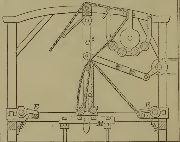
56048—W. F. Heywood—For Folding Cloth.
