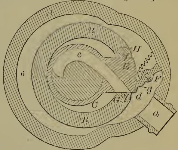
54565—H. B. Leach—Rotary Pump.
