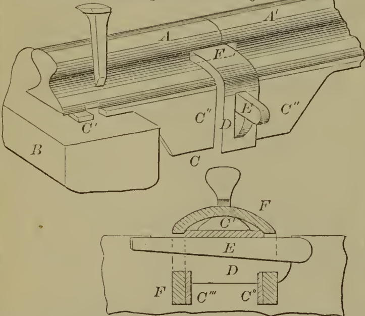
59219—C. Heisterman—For Wrinkling the Insteps of Boots and Shoes.
