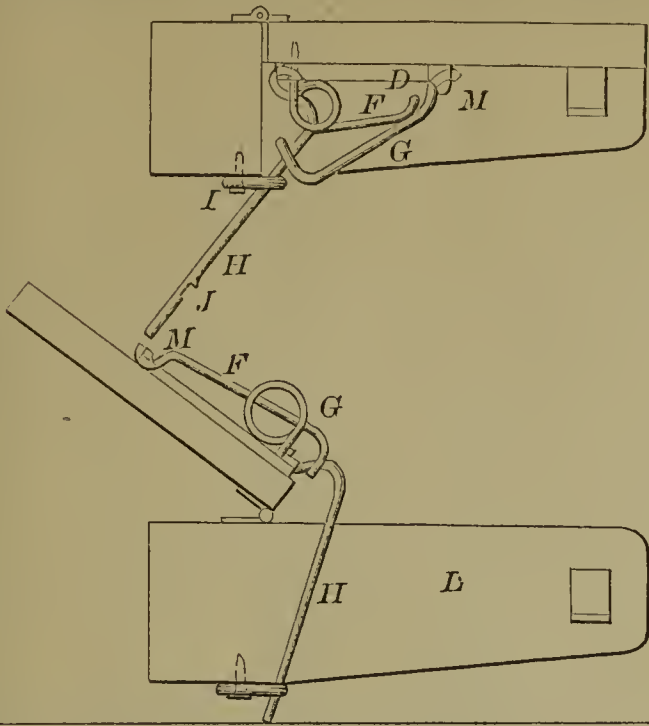
58405—J. C. Gould—Door and Gate Spring.
