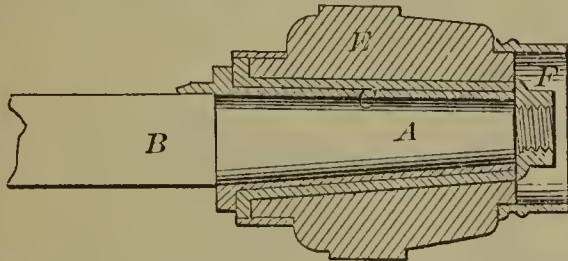
59162—S. Barker—Carriage Axle.
