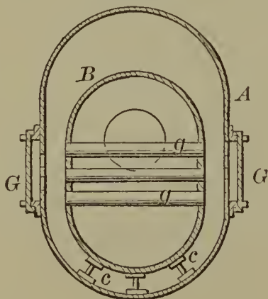
59952—W. Branagan—Steam Generator.
