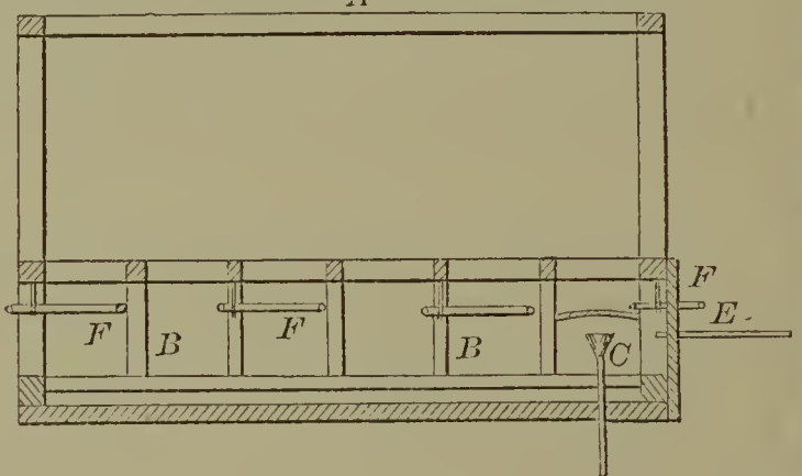
59998—J. W. Hanna—For Drying Lumber.
