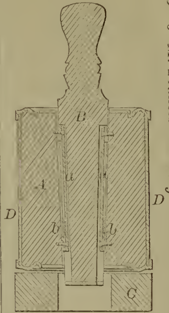
55845—J. M. Francis—Making Tin Fruit Cans.
