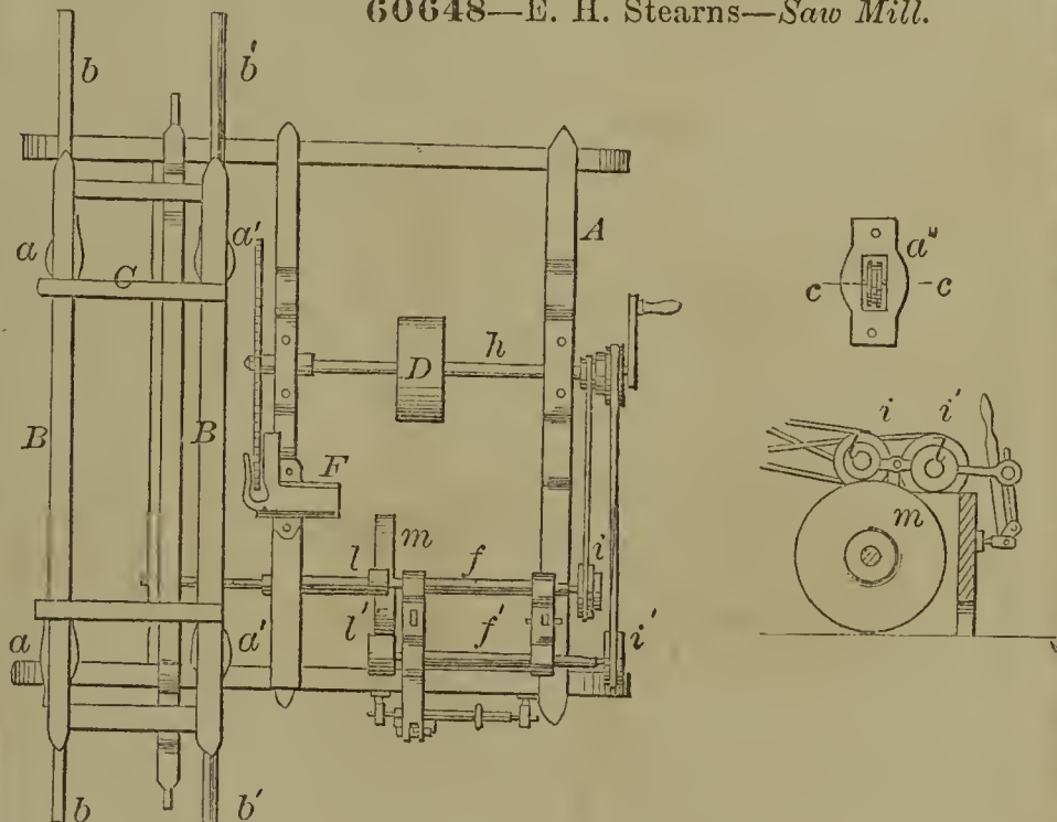
60648—E. H. Stearns—Saw Mill.
