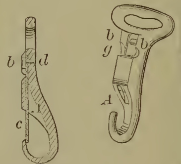
59506—Forbush & Letchworth— Snap Hook.
