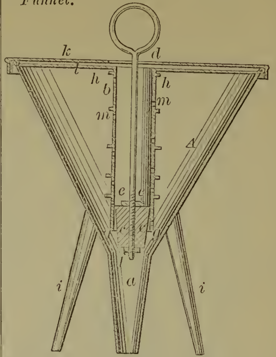
59034—W. E. Keene—Measuring Funnel.
