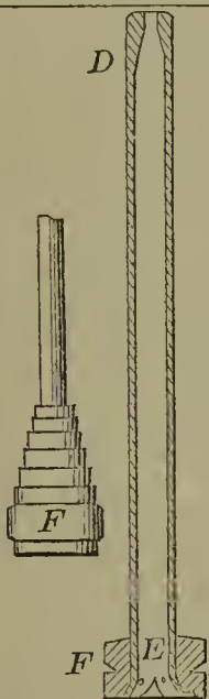
58910—T. Stead— Railroad Signal.
