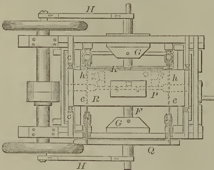
52044—F. Hoffman—For Polishing Wood.
