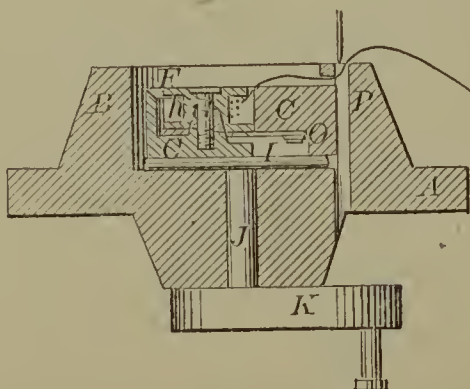
60021—G. H. Lenher—Sewing Machine Shuttle.
