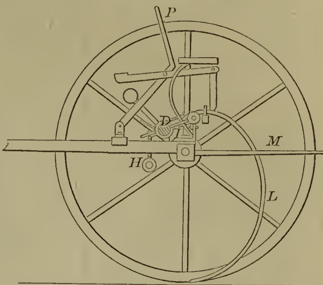
56189—G. Deal—Horse Rake.
