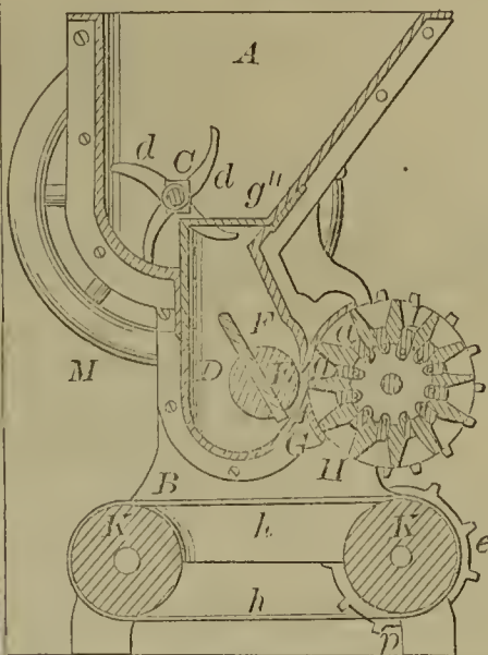
56205—P. M. Gilbert—Sugar Press.
