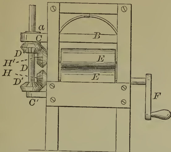
55487—W. F. Goodwin—Harvester Rake.
