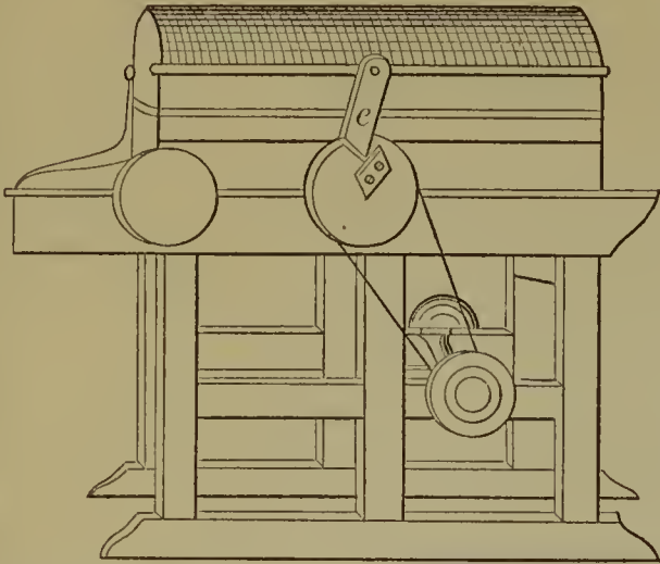
53072—W. W. Wiley— Combined Seeding Machine, &c.
