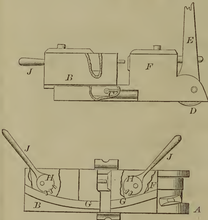
57410—T. Tully— Tire Shrinking Machine.
