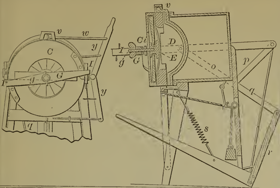
57639—Rowley, Sloane & Woodruff—For Carburetting Air.
