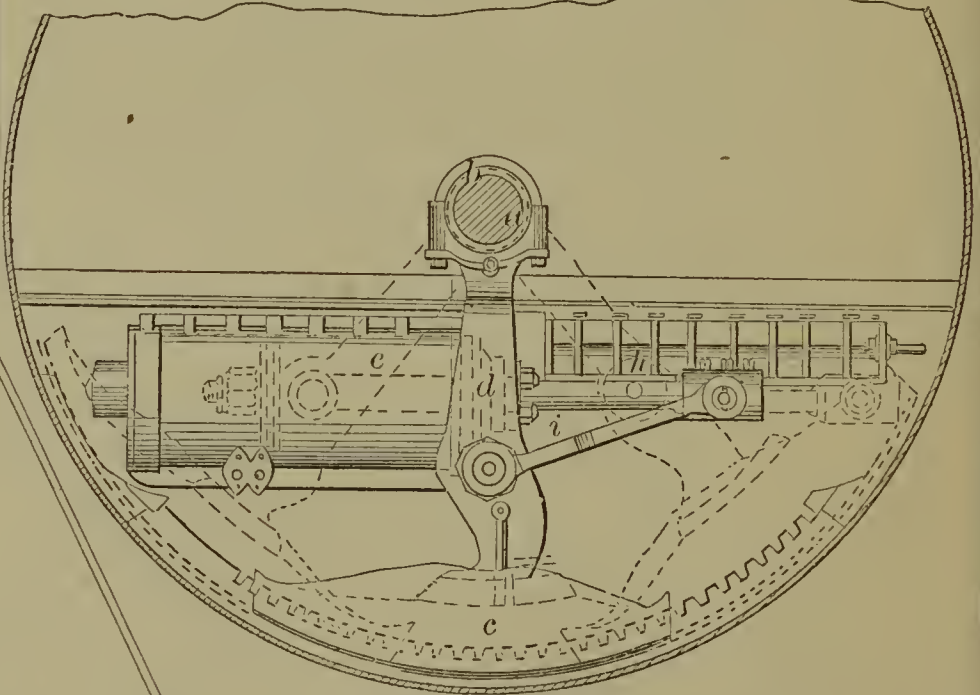
57834—W. L. & T. Winans—For Trimming Ships.
