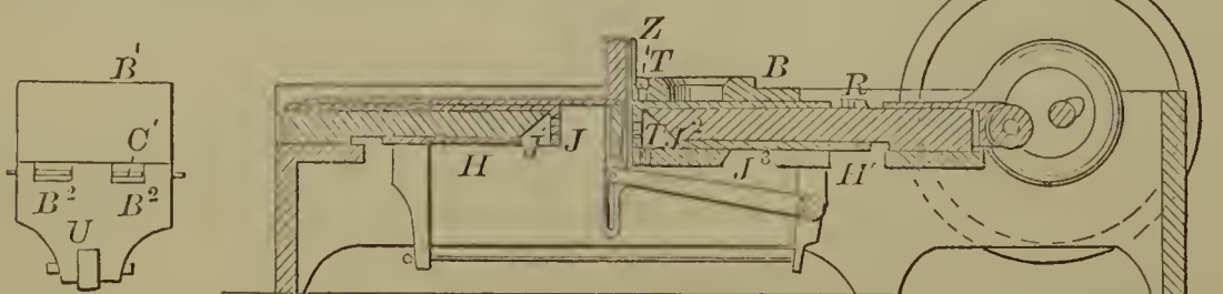
59080—J. Sangster— Brick Machine.
