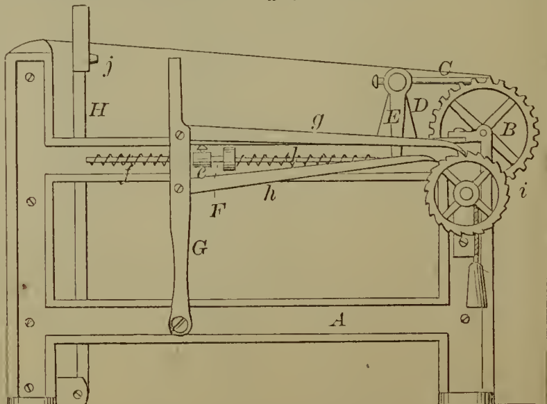
54066—S. Estes— Let-off for Looms.
