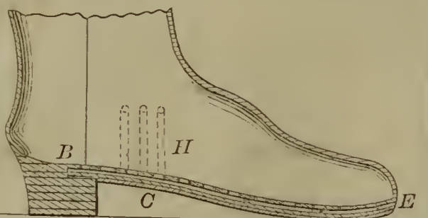
57371—S. Perry— Ventilating Boot.
