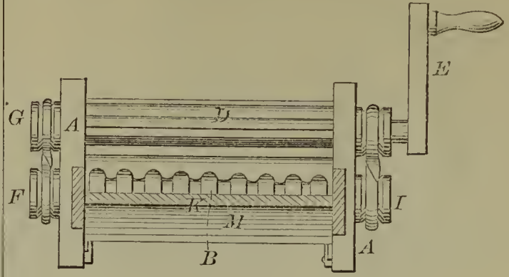
52062—J. C. Loveland— Dough Kneader.
