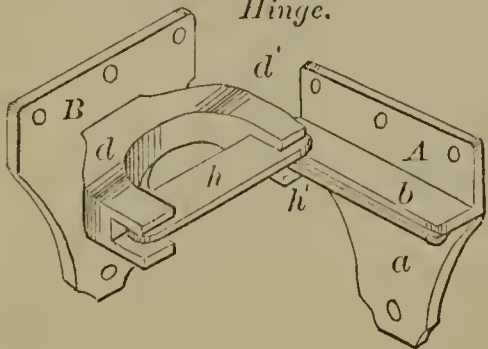
59202—Field & Carruthers—Gate Hinge.
