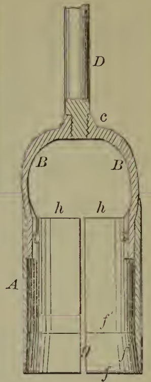
52180— Leeds & Hollowell— Post Hole Auger.
