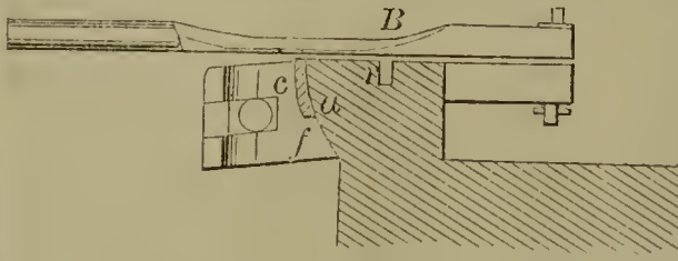
57392—E. Shaw—For Clamping and Stretching Leather.
