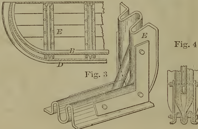
57359—R. Montgomery—Construction of Ships.
