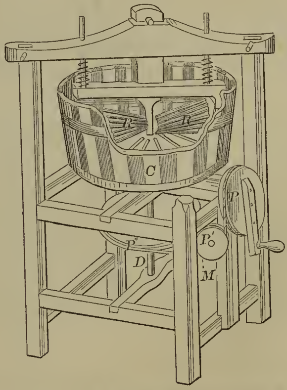
56001—W. Burnham—Washing Machine.
