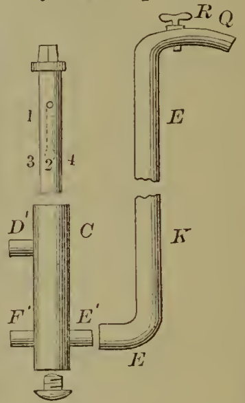
53736—H. L. Frailey—Hydrant Stop Cock.
