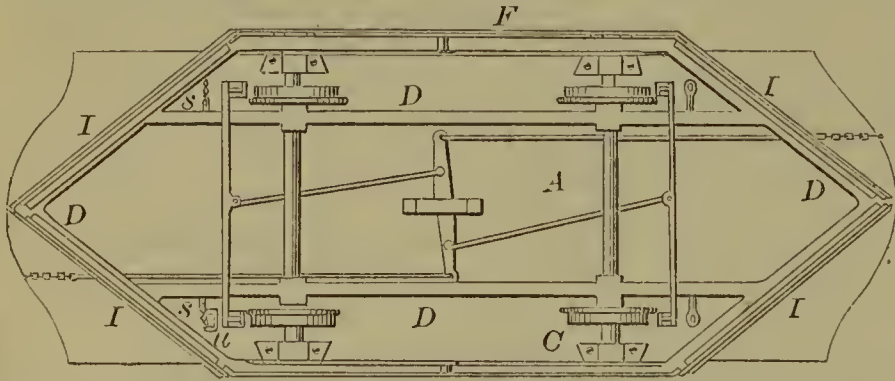
59652—J. R. Reader— Railroad Car.
