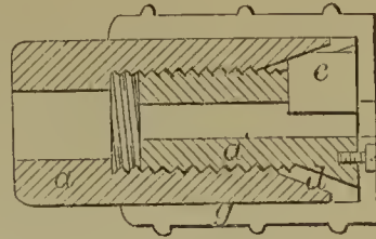
56981—R. W. Morse— Chuck.
