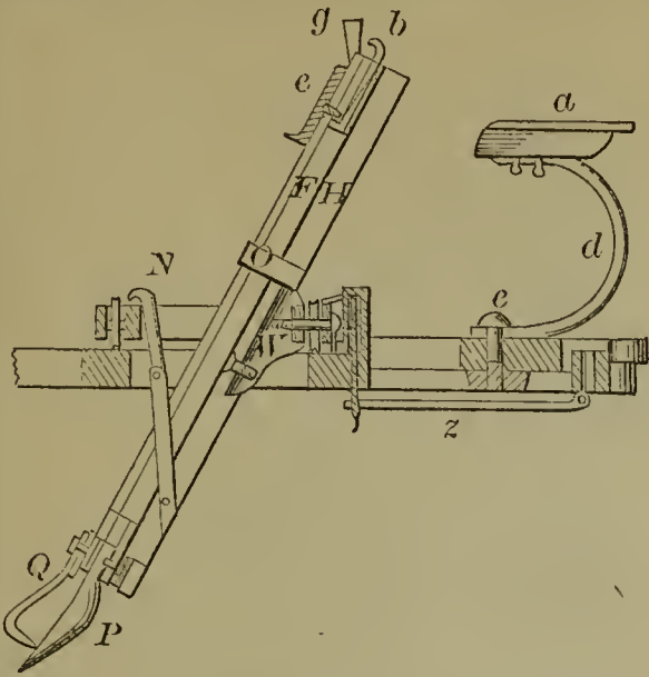
53446—C. Holman—Cultivator.
