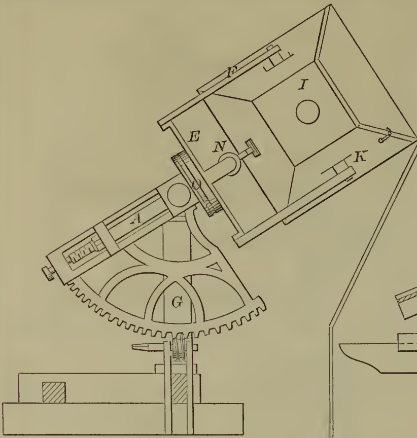
55523—Morawetz & Volkmar—Automatic Heliotrope.
