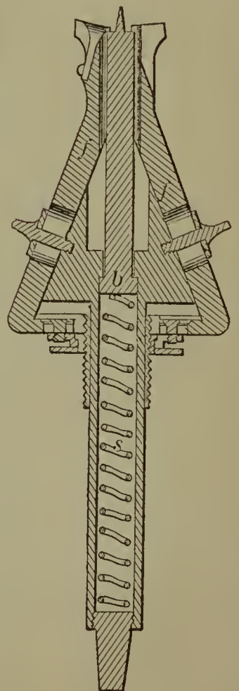
58658—J. McClure—Hollow Auger.
