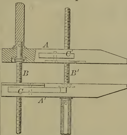
57195—H. Schmidt—Hand Screw Clamp.
