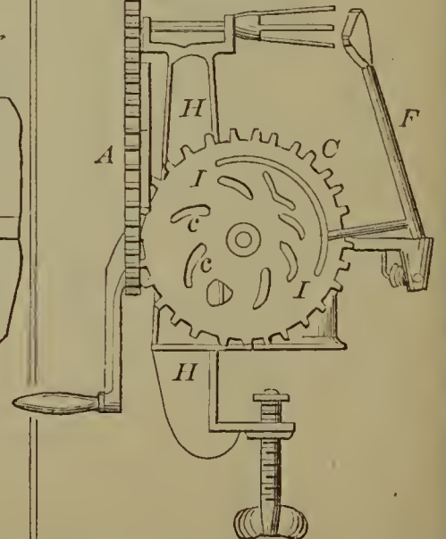
59884—D. H. Whittemore—Apple Parer.
