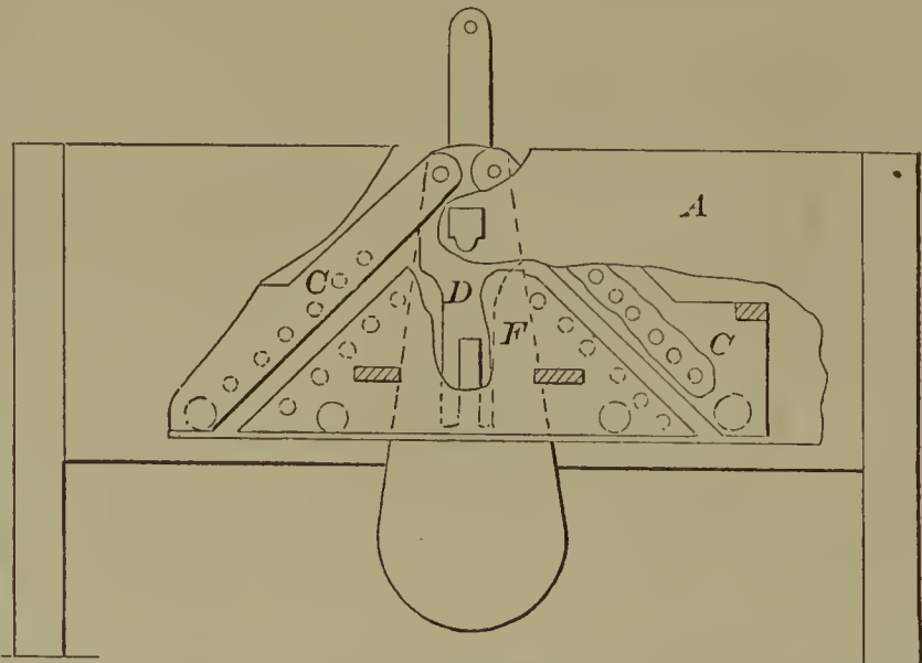
60414—V. Palmer—Churn.
