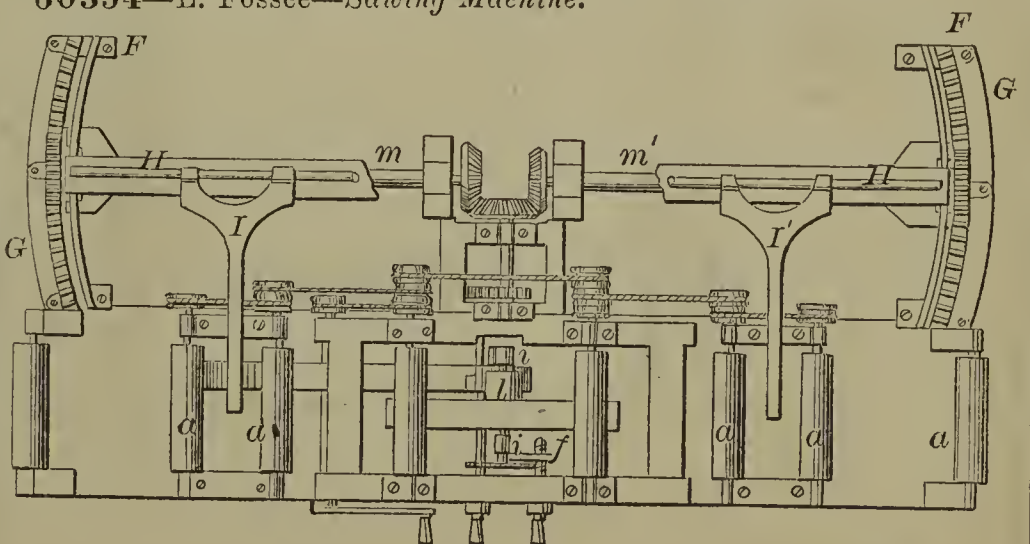
60354—L. Fossee—Sawing Machine.
