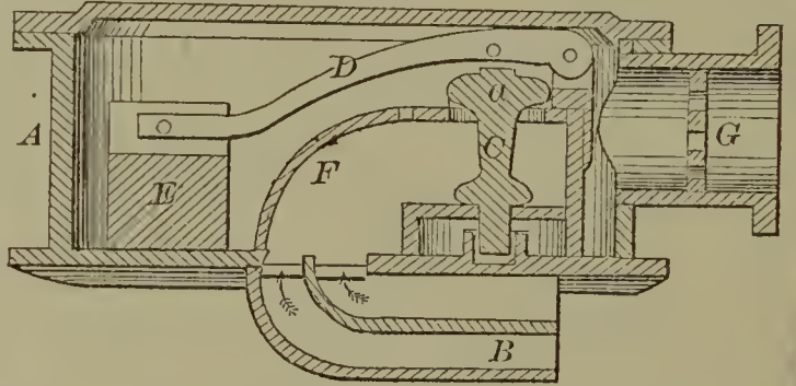
57993---S. Stucky--- Steam Generator Safety Valve.
