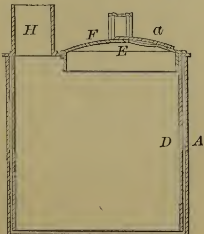
54814—A. N. Beach—Heating Stove.
