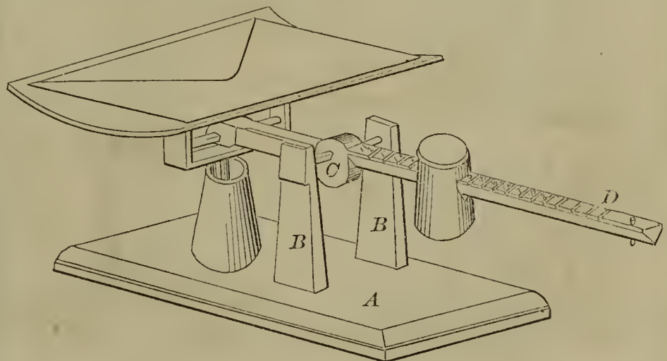
57364—R. Murdoch— Letter Scale Beam.
