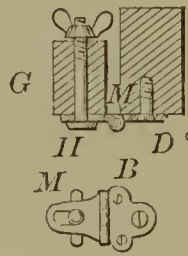
59107—W. T. Wells—Hinge.
