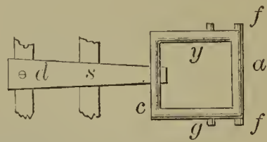
56745—J. Gribben—Die for Making Bolt Heads.
