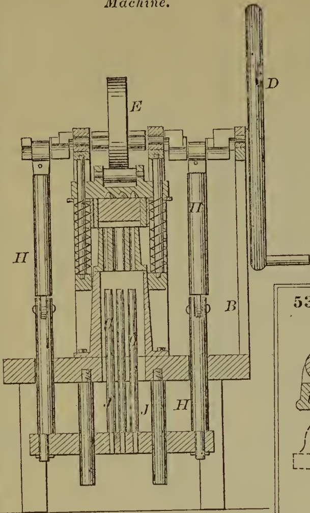
53402—N. W. Brewer—Wooden Pin Machine.
