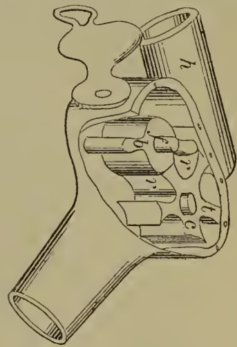
59792—D. Drawbaugh—Faucet.
