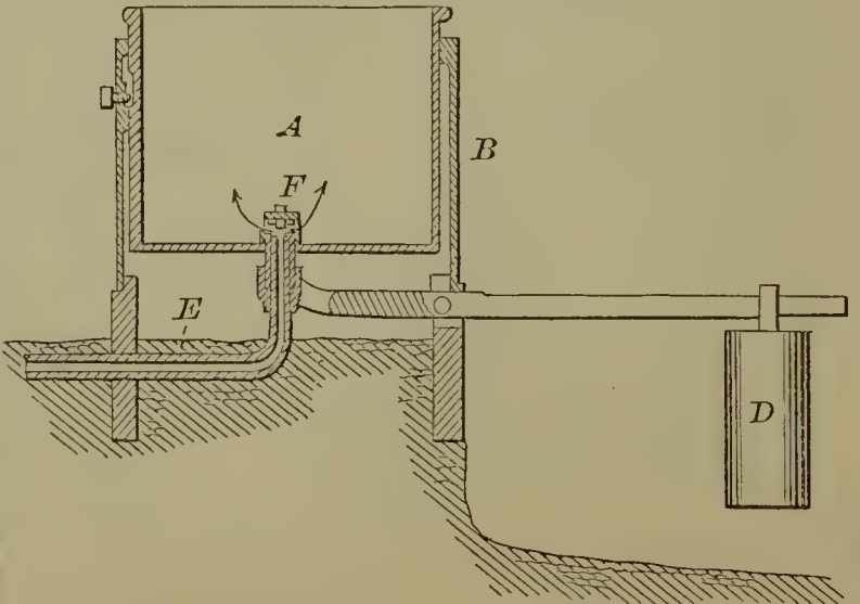
54009—R. S. Pickett— Self-feeding Water Tank.
