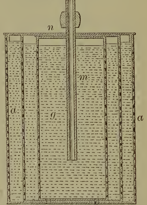
53584—Dewey & Tillotson— Reservoir for Wells.
