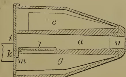
58145—Sinnott & McIntyre— Tuyere.
