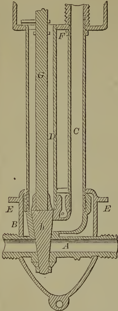
58862—E. McKinney— Coal Oil Stove.
