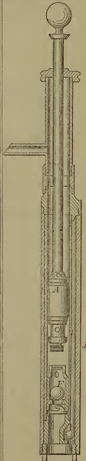
57086—A. Carver—Deep Well Pump.
