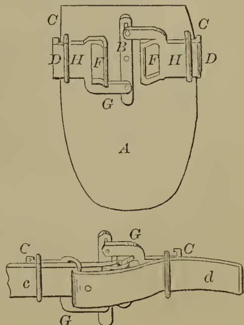
59575—M. Fleisher—Skate Fastening.
