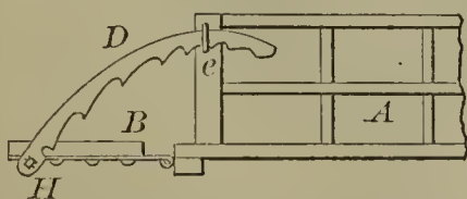
52230—S. Walker— Self-Locking Tail Board.
