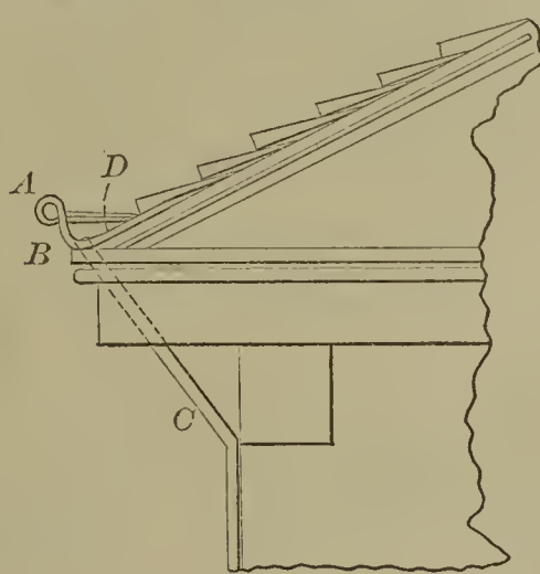
52438—T. C. Moore—Eaves Trough.
