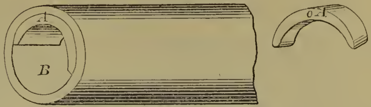
56905—C. W. Copeland—Tube Thimble.
