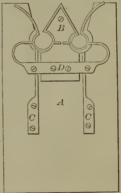
52237—H. B. Wolf—Sorghum Cane Stripper.
