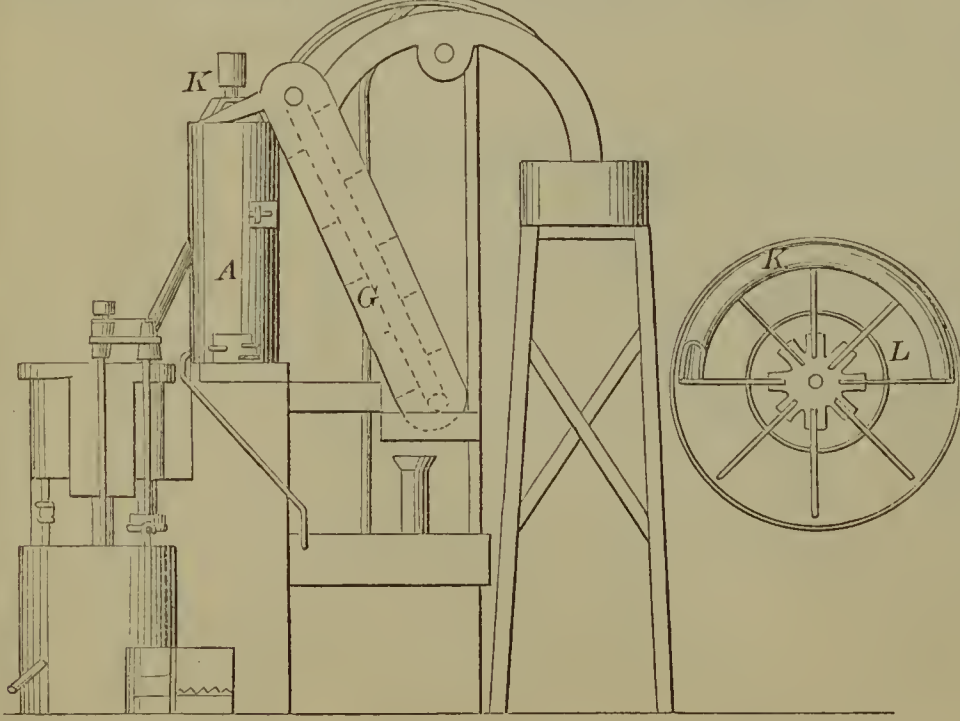
55261—J. H. Elward— For Separating Metals from Ores.
