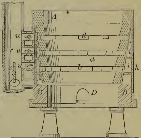
55204—Mackenzie & Isbell—Cupola and other Furnaces.
