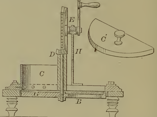
57070—D. Bearly— Vegetable Cutter.
