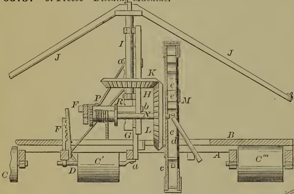
53737—C. Freese—Ditching Machine.
