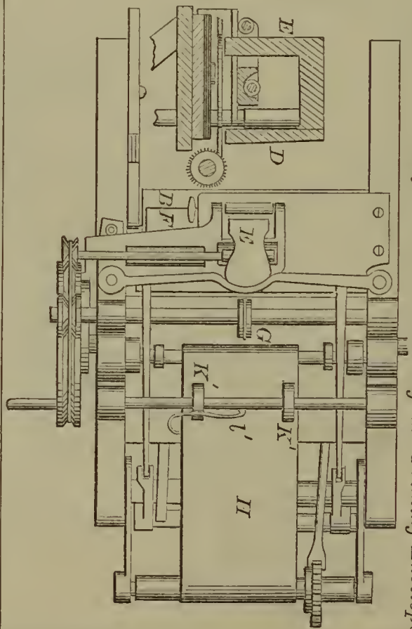
55562—T. V. Waymoth— For Gunning and Printing Envelopes.
