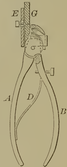
57044—J. Lyle— Saw Set.
