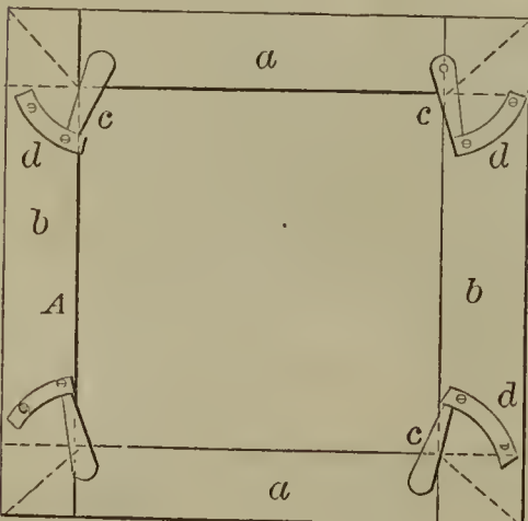
55579—C. Dowd—Canvas Stretcher.
