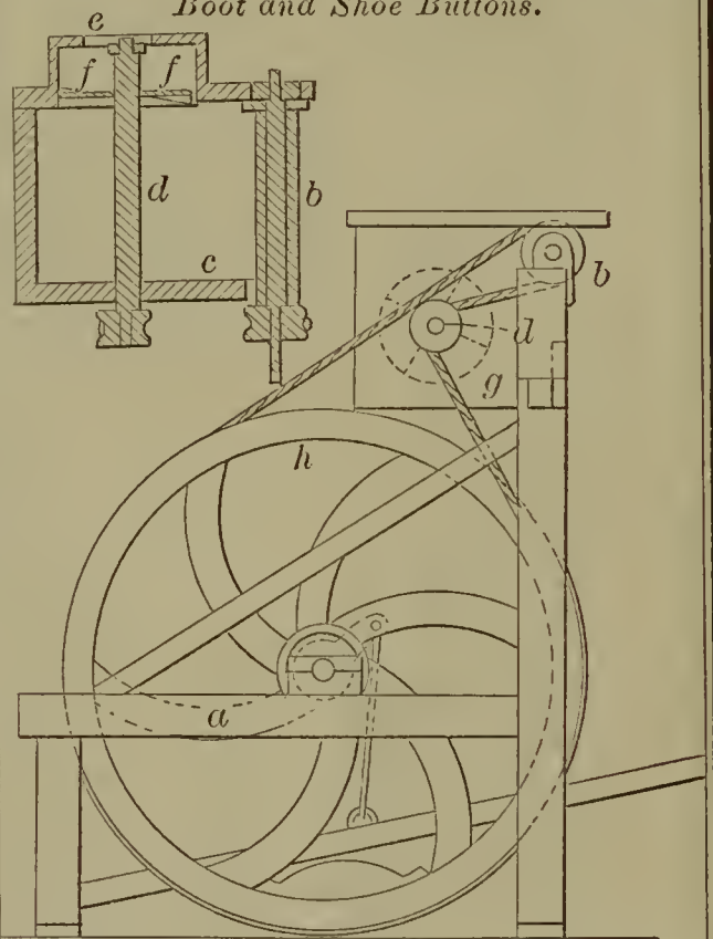
55664—Jewett & Everson—For Facing Boot and Shoe Buttons.
