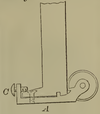
55567—J. N. Wilkins— Sewing Machine Caster.
