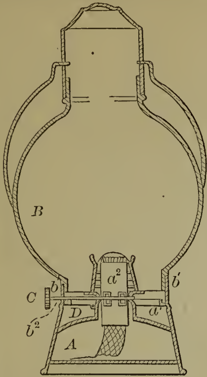
53027—J. C. Moore—Lantern.
