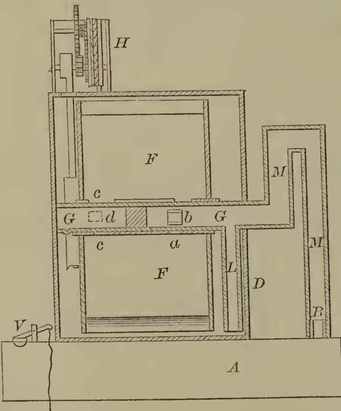
55949—F. H. Brown—For Carbureting Air.
