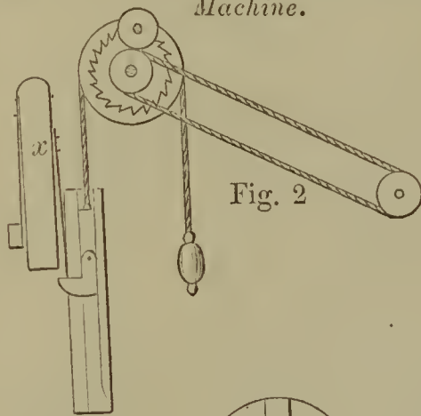
54493—J. Blayne—Hand Spinning Machine.
