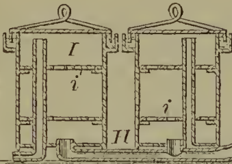
58005—P. H. V. Weyde— Distilling Petroleum and other Liquids.
