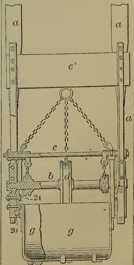
54649—A. T. Morris— Scoop for Excavating.
