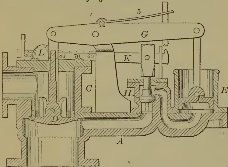
55127—A. Low— Safety Valve.
