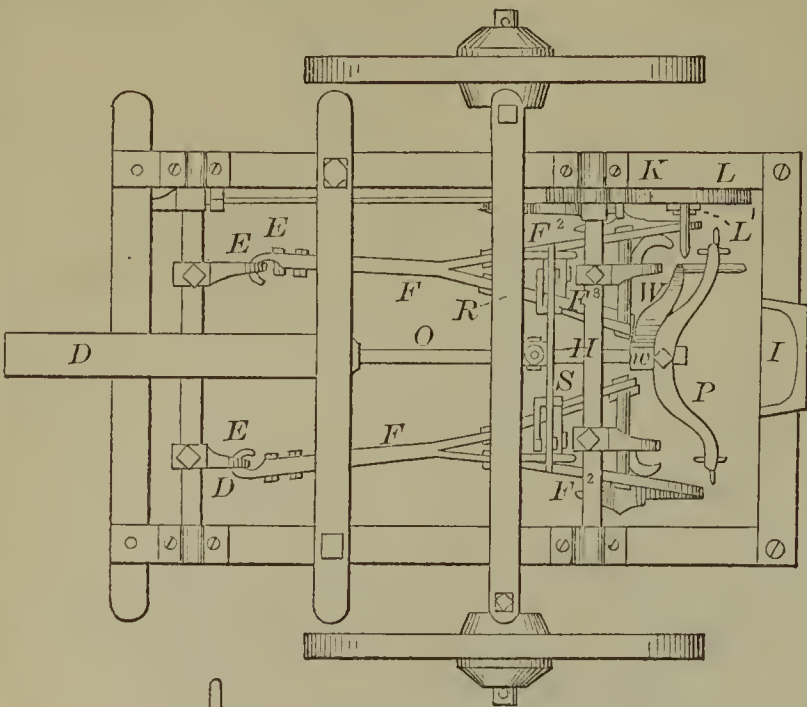
52165—H. Hammond—Cartridge Retractor.
