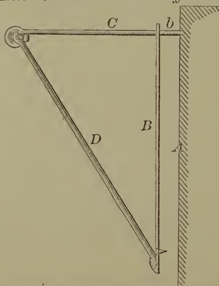
60122—H. Beckwith—Scaffold Bracket.
