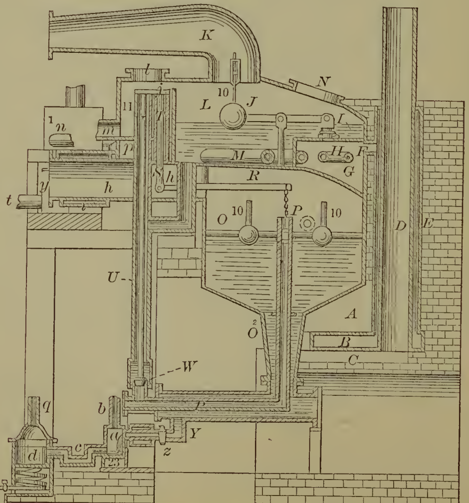
54355—D. Hull—For Washing Kaolin, &c.
