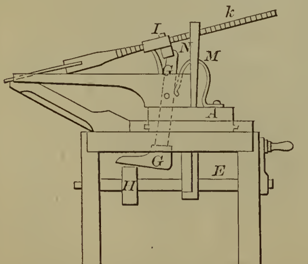
53924—C. D. Hunt—Nail Plate Feeder.
