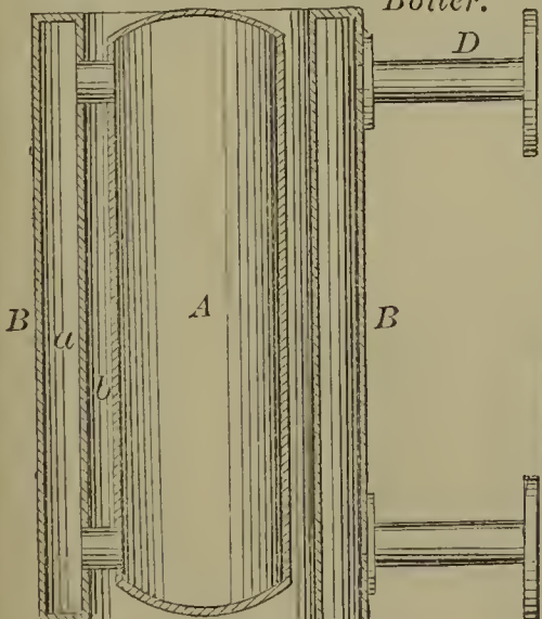
58807—C. Geisse—Gas Heater Boiler.
