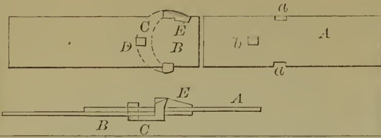
59445—I. Osgood—For Securing Wheel Hubs to Axles.
