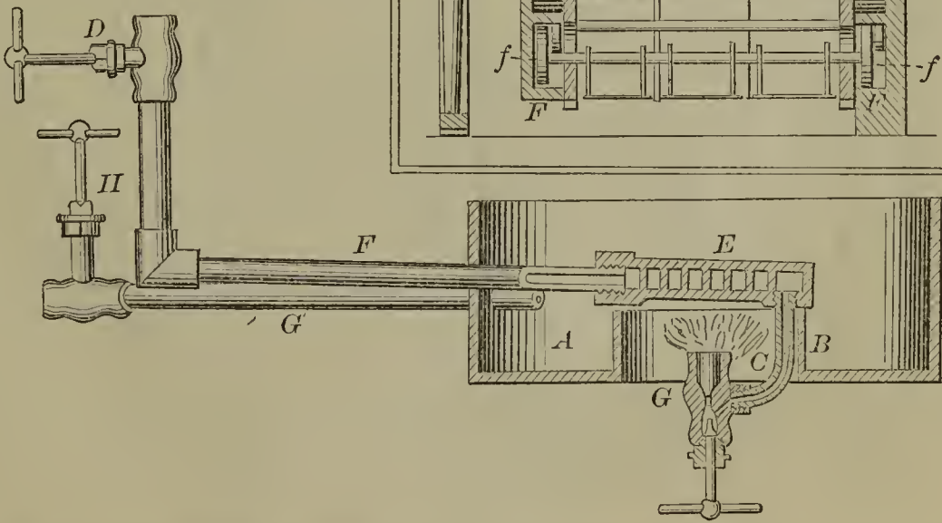
52246—A. J. Griffin—Hydro-Carbon Stove.
