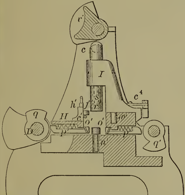
53352—J. C. Scribner—Churn.
