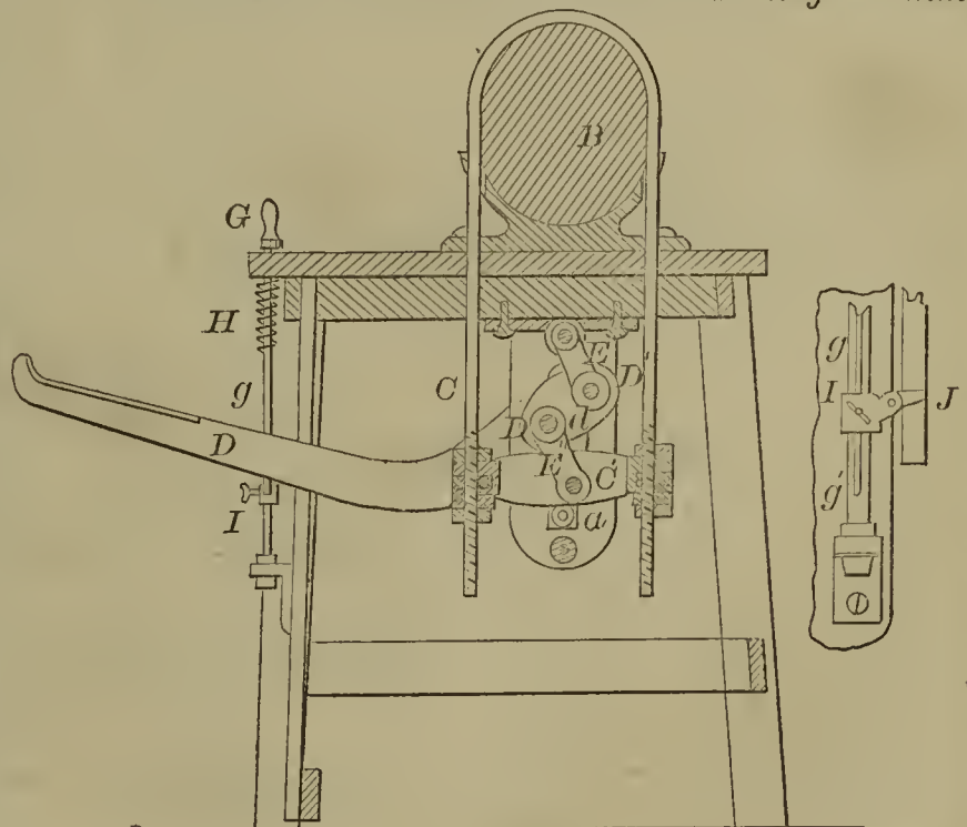
55282—D. A. Greene— Wood Bundling Machine.
