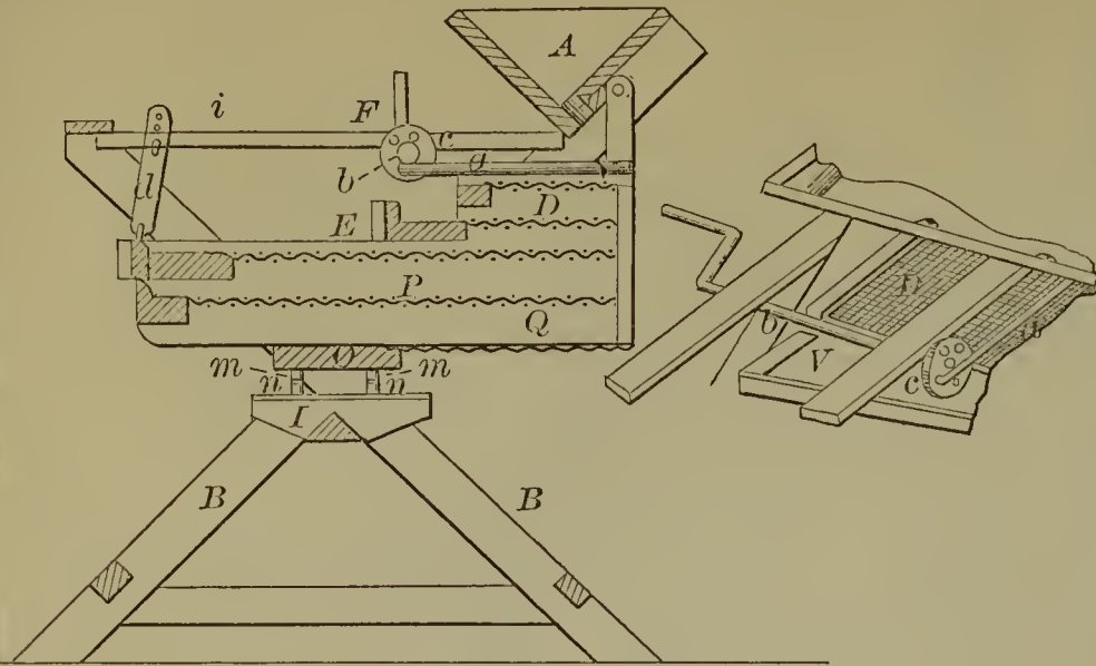
55156—Palmer & Gilliland—Stump Extractor.
