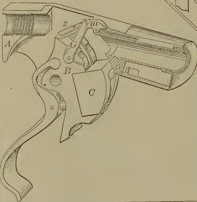
58737—C. M. Spencer— Magazine Fire Arm.
