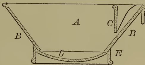
54741—J. C. Knoepke—Wash Basin.
