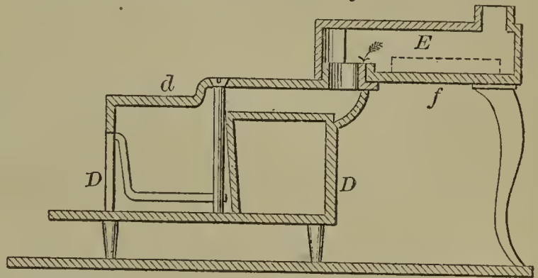
58061—J. Chambers—Cooking Stove.
