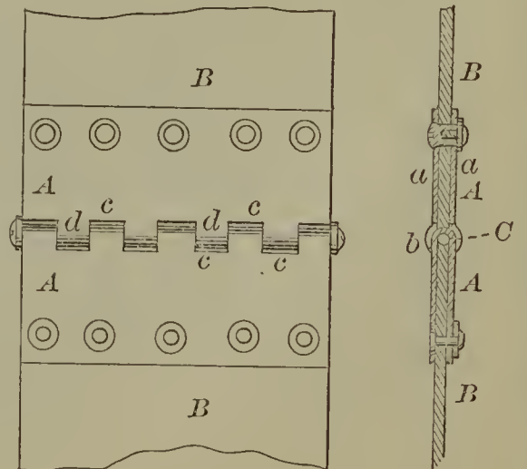
52178—W. Leas—Belt Coupling.
