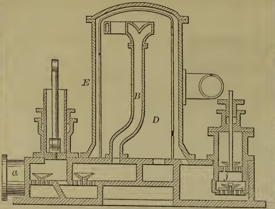
56131—L. C. White—Kerosene Burner.
