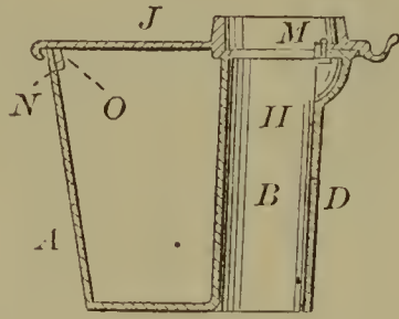
59897—D. Dishart—Washing Machine.
