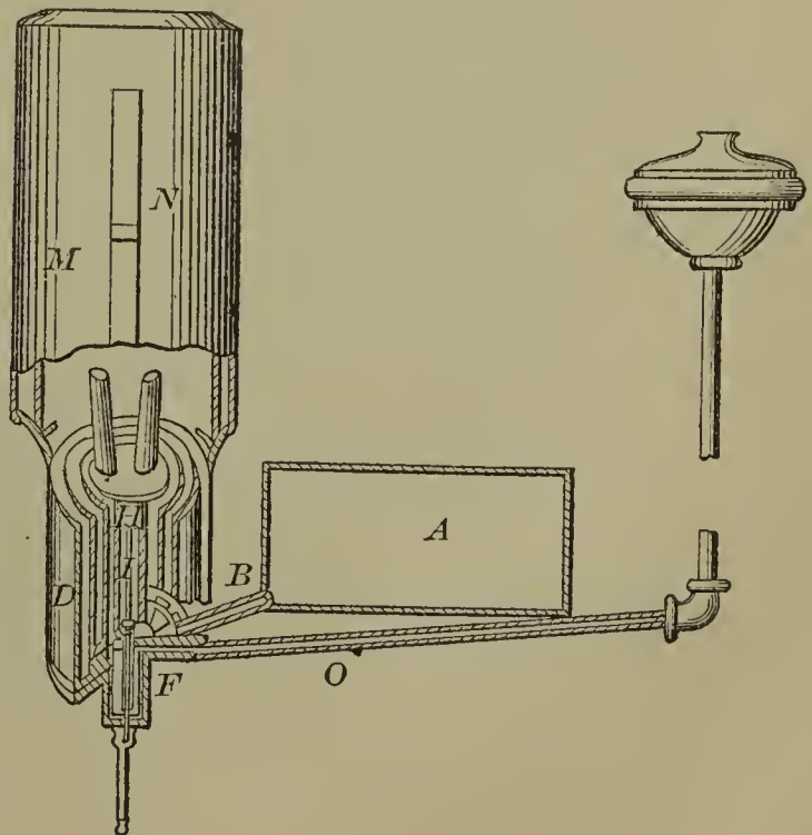
57880—H. W. Dopp—Wick Burner for Heating and Cooking.
