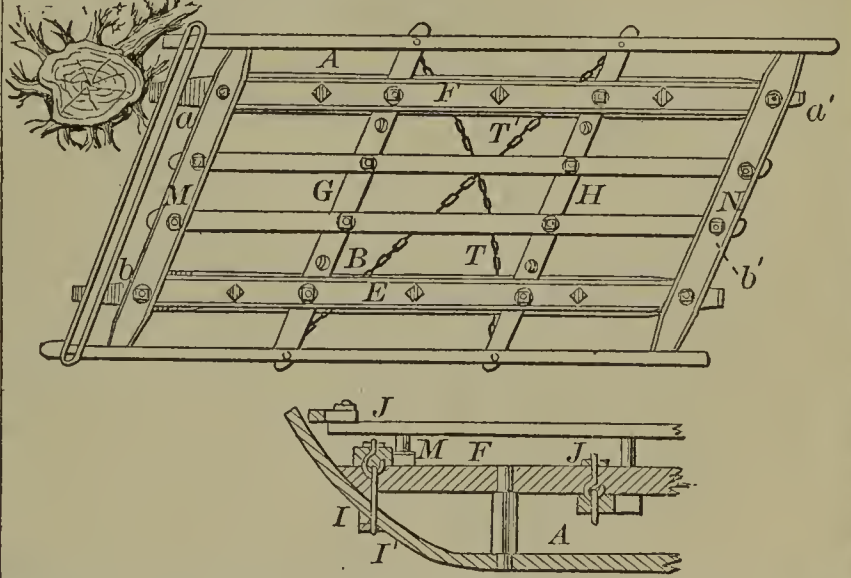
57964—B. F. Porter—Table Stand for Food.
