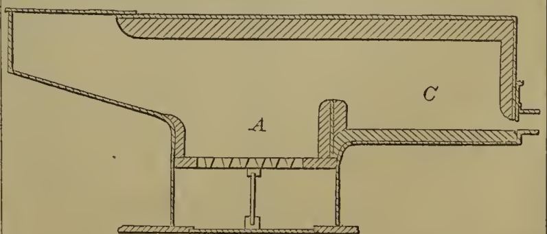
58346—Hotchkiss & Shattuck— Forge Furnace.
