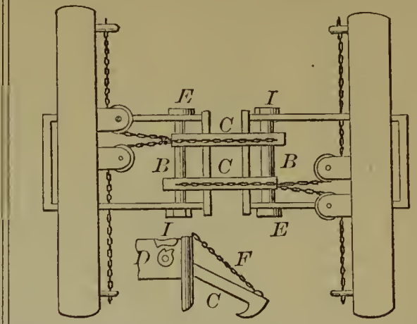
53037—Payne & Boxley—Car Coupling.
