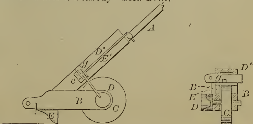
59123—Davis & Peabody—Seed Drill.
