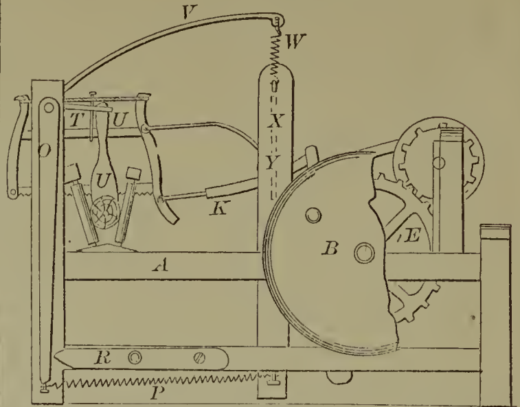
59998—J. W. Hanna—For Drying Lumber.
