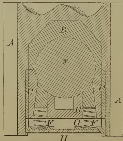
56977—M. V. Miller—Axle Box.
