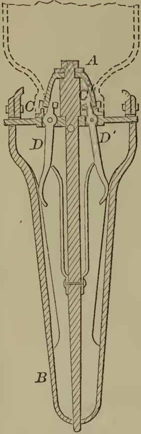
55989—W. Bergmann—Car Coupling.
