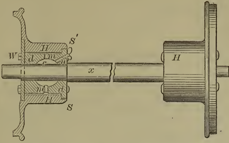
58791—Dupraz, Dumont & Dickason—Steering Apparatus.
