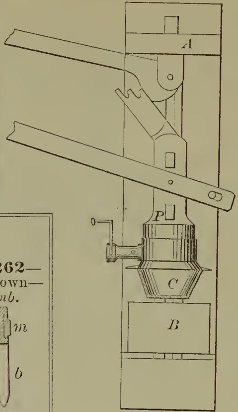
52266—G. G. Carver— Flour Sifter and Measure.
