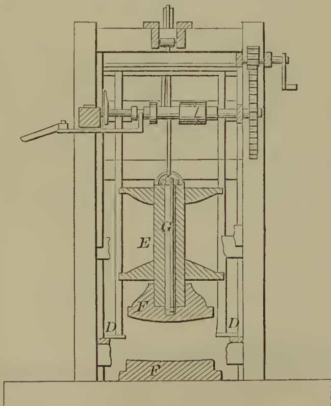
55976—J. Aughe—Drop Hammer.
