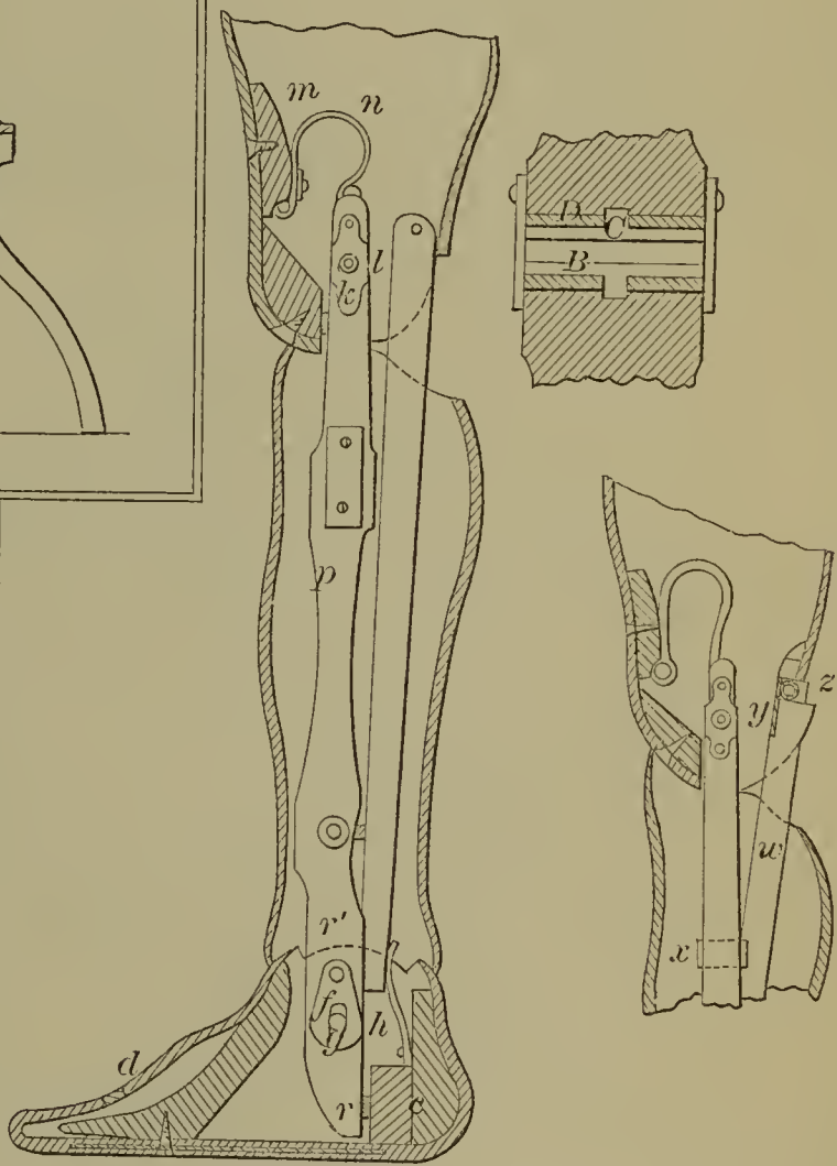
54364—Kimball & Lawrence—Artificial Leg.
