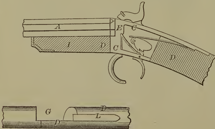
60188—G. Henry— Fitting Lock Plate to Fire Arm.
