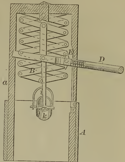
55980—J. C. Barrett—Water Elevator.
