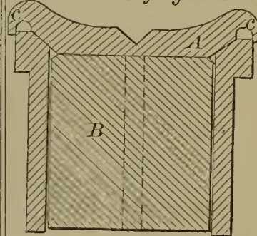
85294—G. W. Richardson— Steam Safety Valve.
