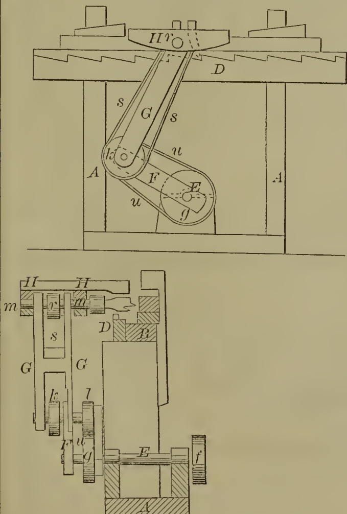
56195—S. E. Ellis—Wood Boring Machine.
