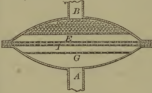
58055—J. F. Boynton—For Gas Machines and Carburetors.
