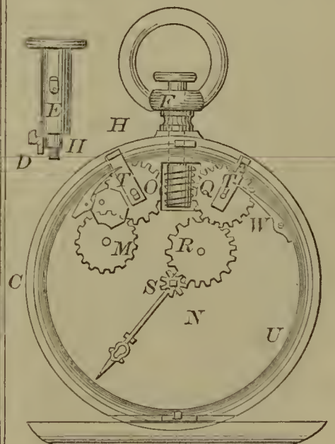
55750—A. Wadsworth—Watch.
