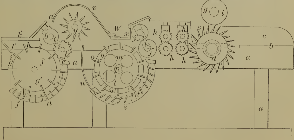
59501—S. A. Clemens—For Straightening, Breaking and Cleaning Flax Straw.
