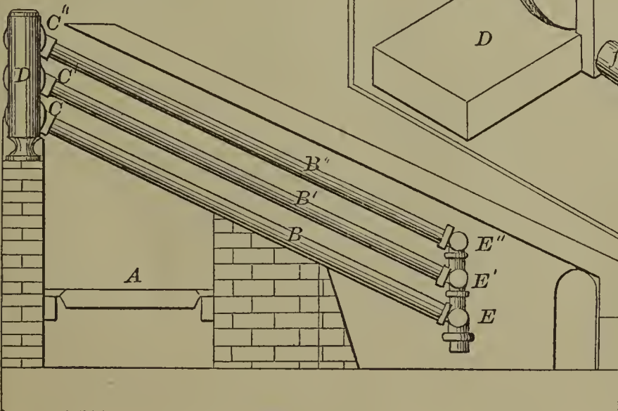
58017—C. S. Bell—Steam Generator.
