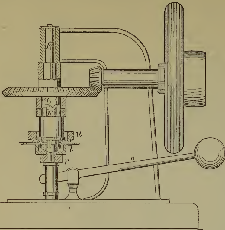
55209—E. Paye—For Turning Boiler Flanges.
