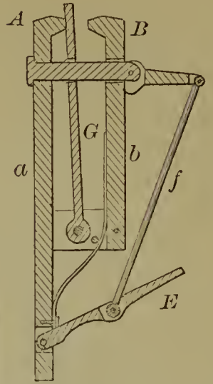
53736—H. L. Frailey—Hydrant Stop Cock.
