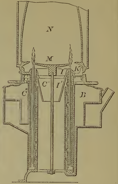
59898—H. W. Dopp—Tubular Wick Burner.
