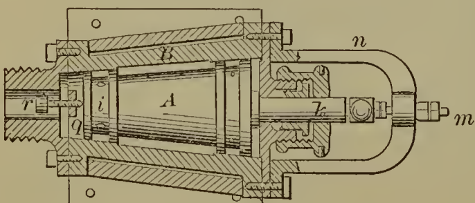
53410—J. W. Carhart—Balance Valve for Steam Engine.
