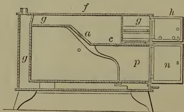
60446—G. W. Walker—Cooking Stove.
