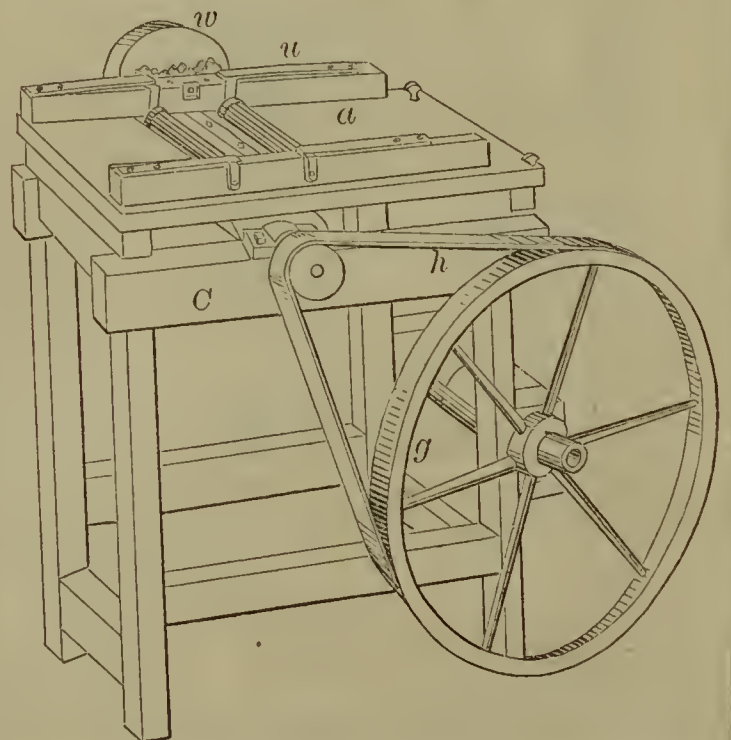
56254—D. Niles—Planing Machine.
