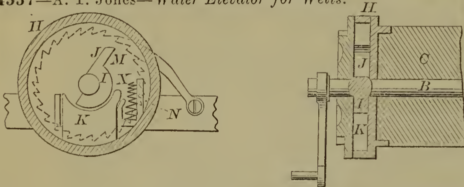
54557—A. T. Jones— Water Elevator for Wells.
