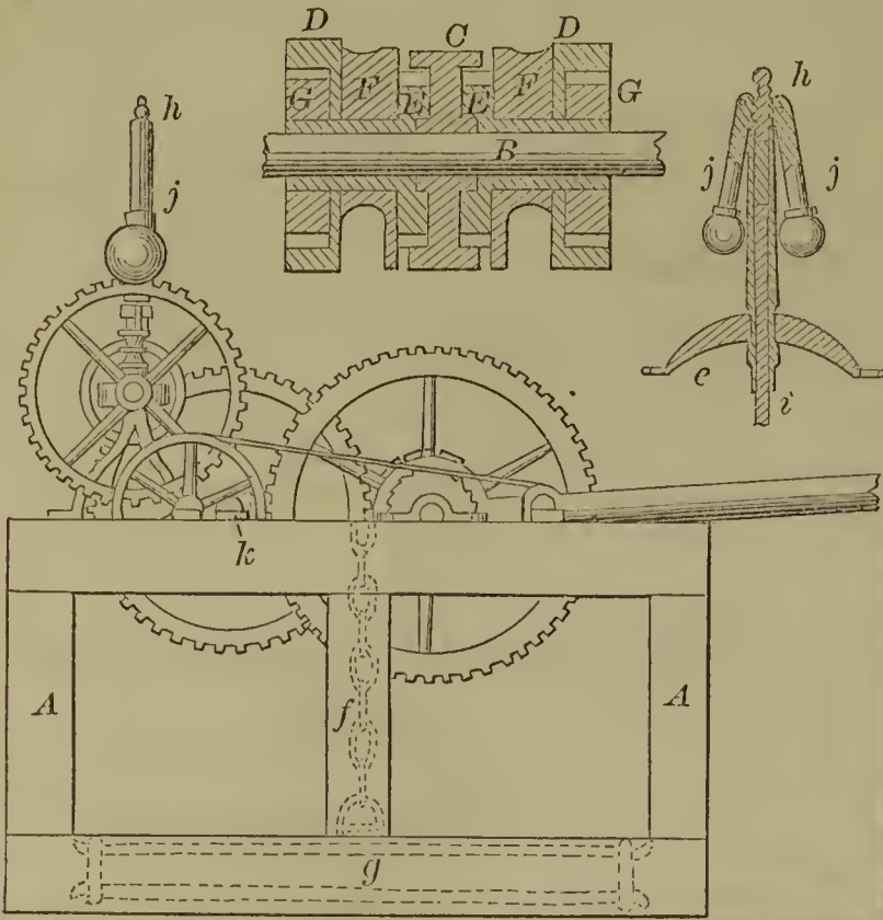
55328—J. McWilliams—Gas Generator.
