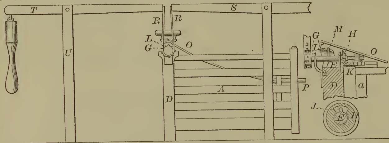
56019—Dixon & Close—Gate.
