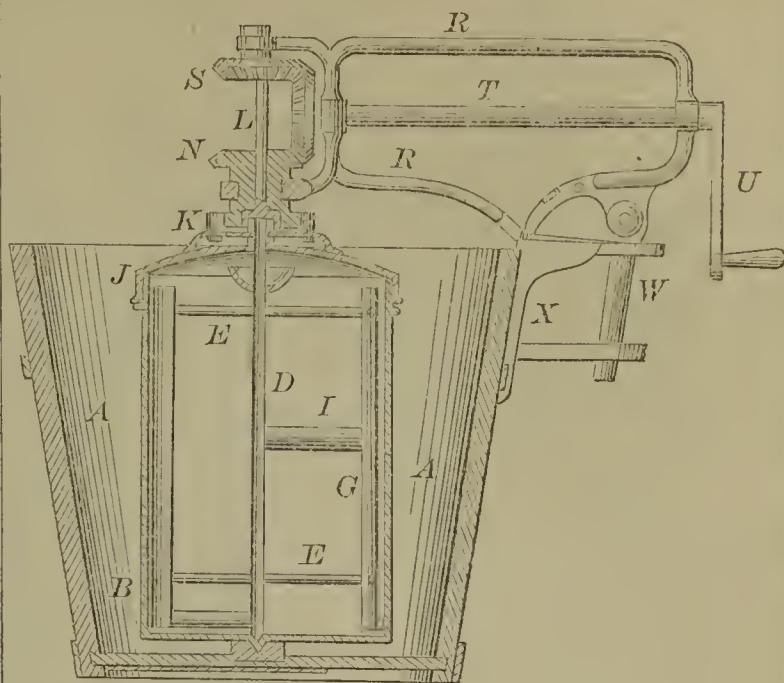
55820—J. R. Champlin—Cream Freezer.
