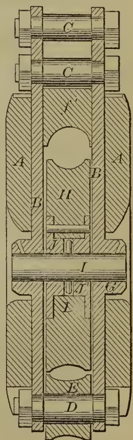
52874—G. Milsom—Tackle Block.
