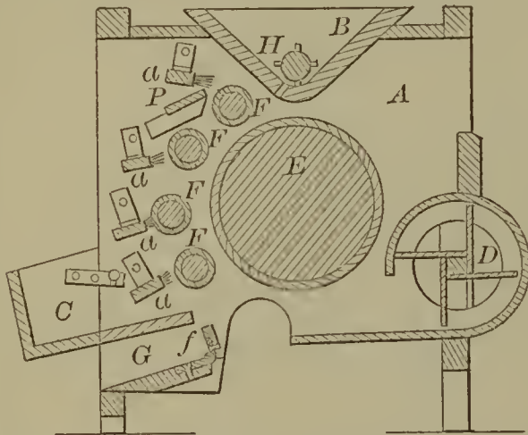
55800—W. M. Arnall—Grain Separator and Cleaner.
