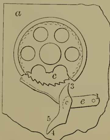
59273—L. D. Rundell— Car Brake.
