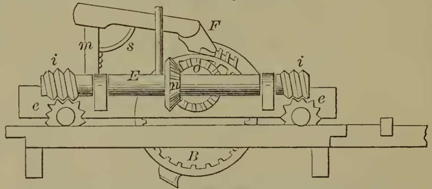
53951—Coult & Roach—For Separating Volatile Metals from Ores.
