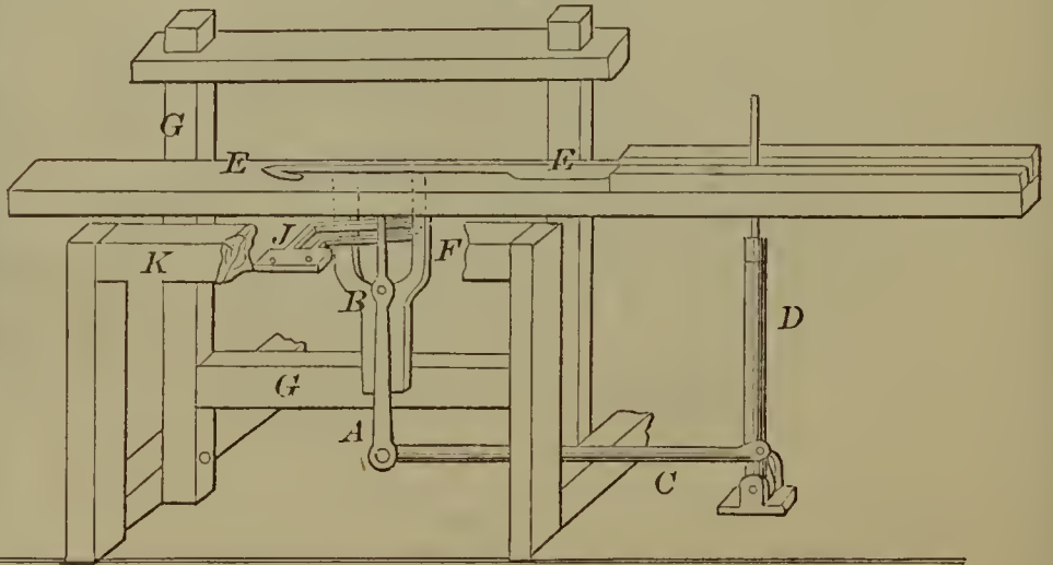
53892—Sherman & Baxter—Operating the Picker Staff for Looms.
