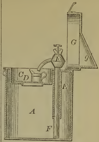
59067—T. Pratt— Tire Shrinking Machine.
