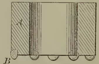
51814—L. Dow— Drill for Rock Boring.
