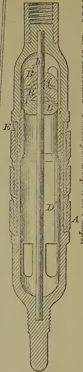
53630—E. Y. Kneeland— Piston for Deep Well Pumps.
