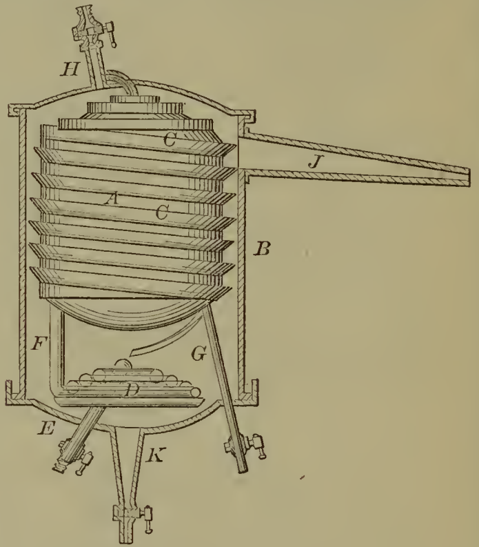
53964—L. V. Fiehet—Distilling Petroleum.
