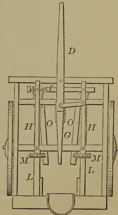
58380—E. Children—Cultivator.
