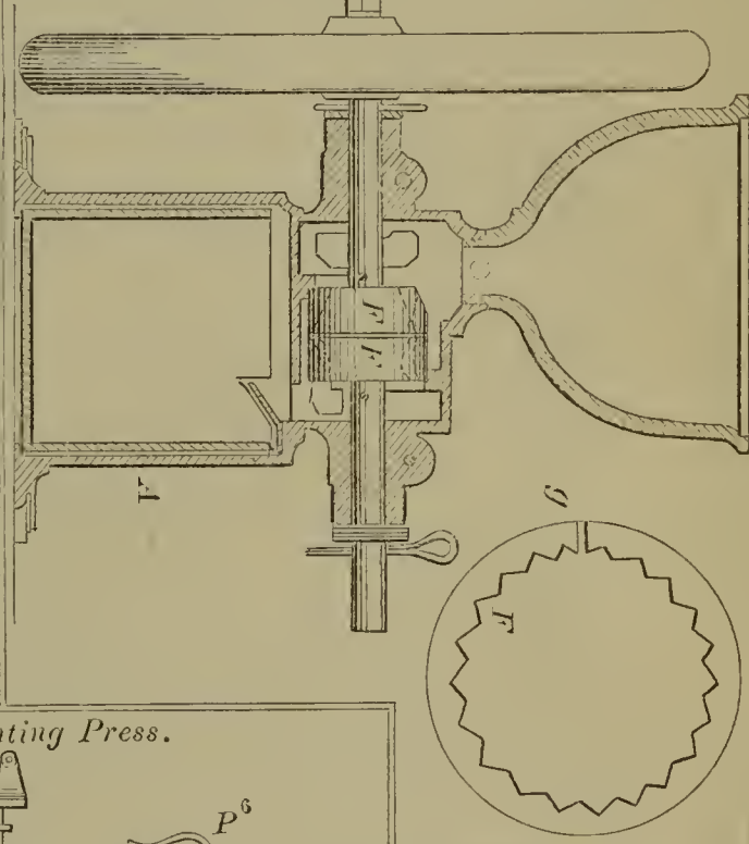
59528—Peugot & Laurent—Grinding Mill.
