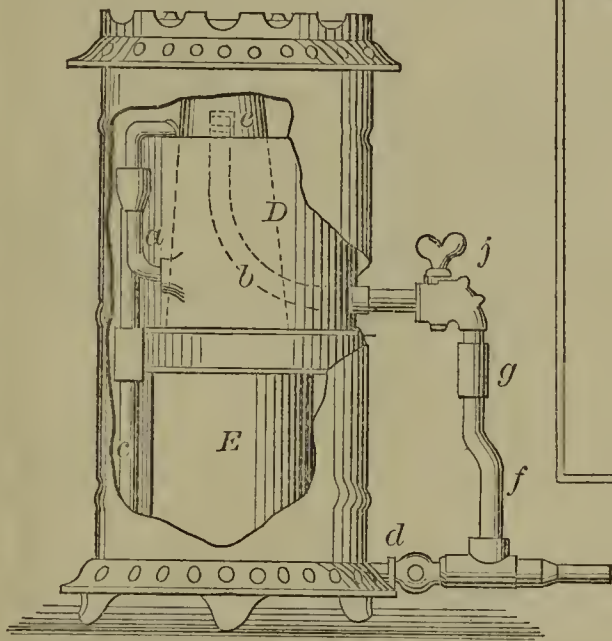
52300—Lesley & Craig— Gas Stove.
