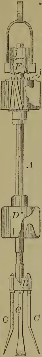
57828—C. Mather—Well Boring Drill.
