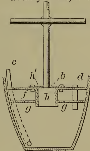
53451—J. F. Keeler—Portable Tank for Oil, &c.
