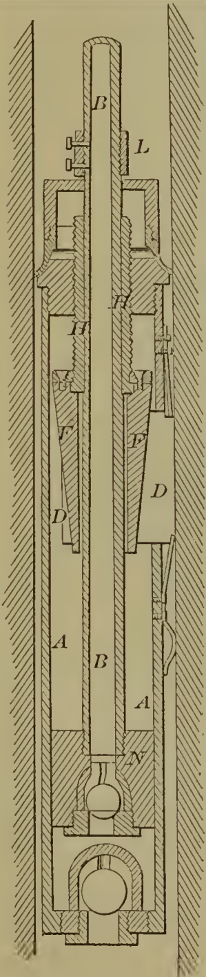
52947—W. S. Wilkinson— Pump for Oil Wells.
