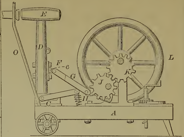
55009—W. Hyde—Rock Drilling Machine.
