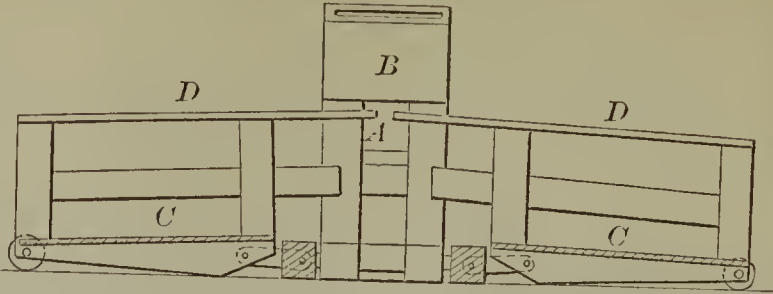
52009—H. J. Ruttan—For Ventilating Railroad Cars.
