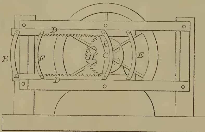
57178—J. B. Page—For Converting Motion.
