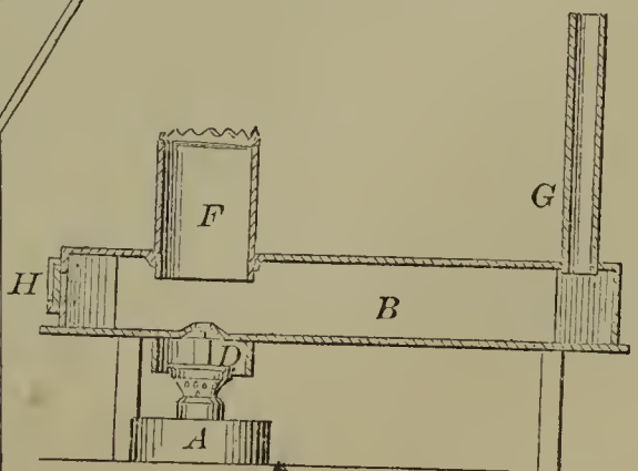
58822—S. P. Hildreth—Dentists' Lamp Stove.
