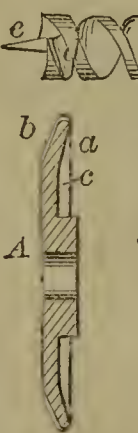
56058—R. Jennings—Tool for Finishing Augers.
