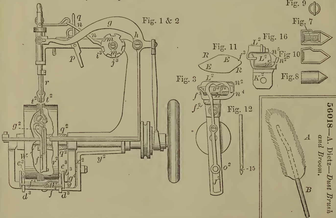
56020—G. L. Dulaney—Sewing Machine.
