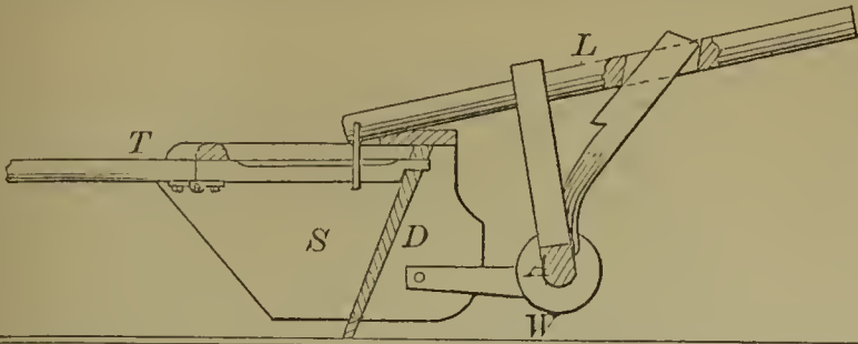
54374—H. R. Lavey—Reaping and Mowing Machine.
