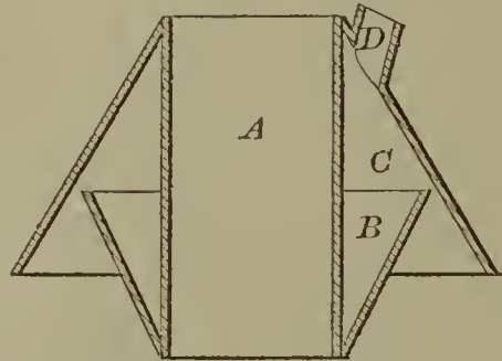
57939—McAfee & Wirt—Ground Drag.
