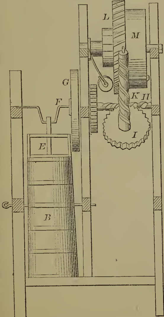
54634—N. E. Wilson— Churn.
