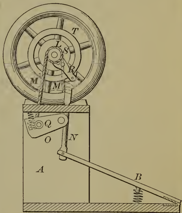
53046—E. P. Ryder— Treadle Motion.
