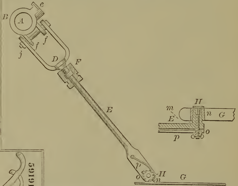
59192—J. W. Doty—Pitman for Harvesters, &c.
