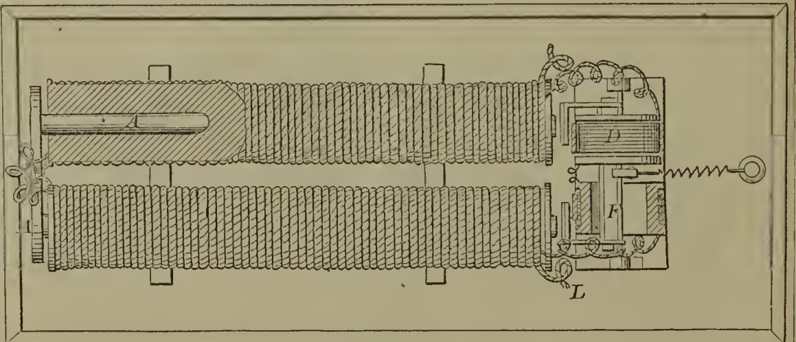
60432—T. P. Shaffner—Magnet for Telegraph.
