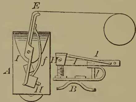
53783—Chandler & Goodrich—Thread Tension Device for Sewing Machines.
