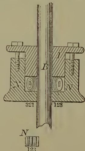
59918—McLean & Vanderear—Piston Rod Packing.
