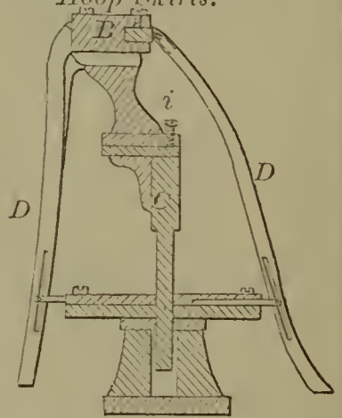
58949—H. S. Loper—Adjustable Frame for Hoop Skirts.
