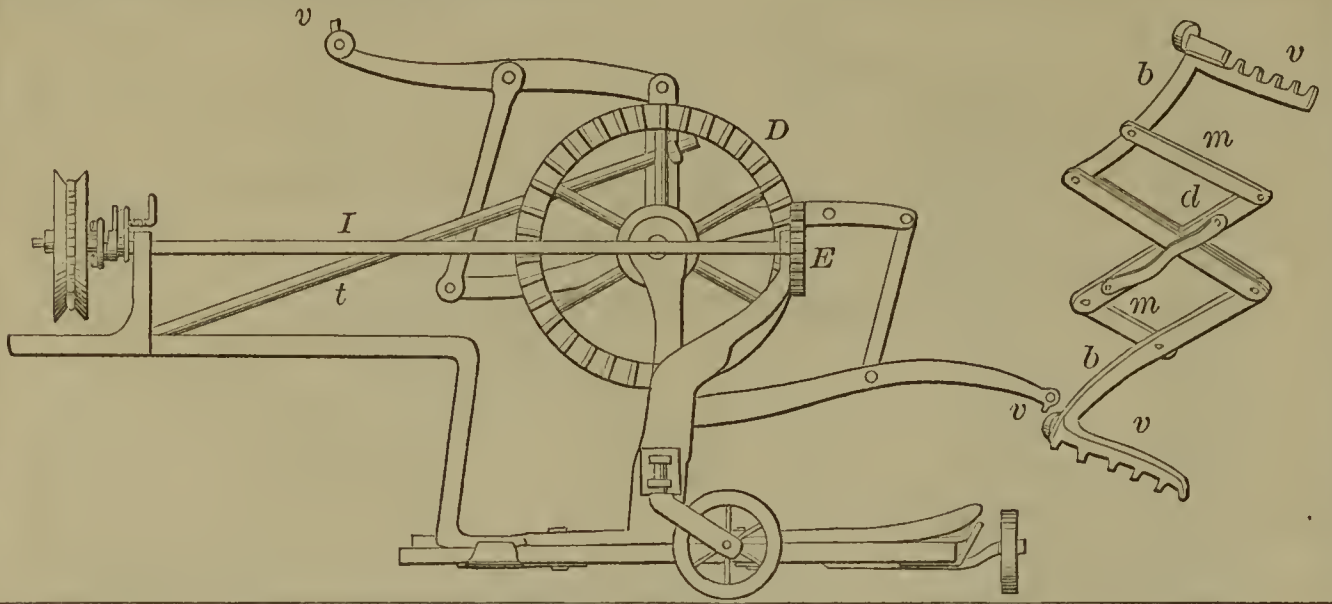
52701—E. T. Ford—Harvesting Machine.
