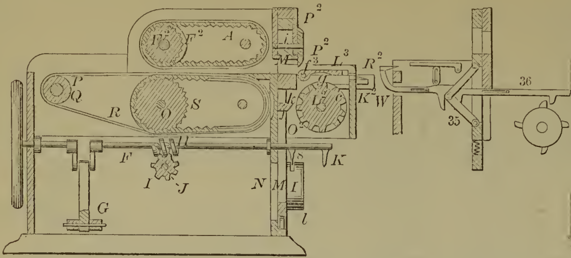
59490—M. D. Wells—Cotton Seed Planter.
