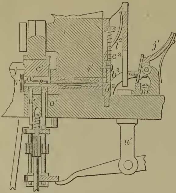
55799—J. Adams—Cutting Boots.
