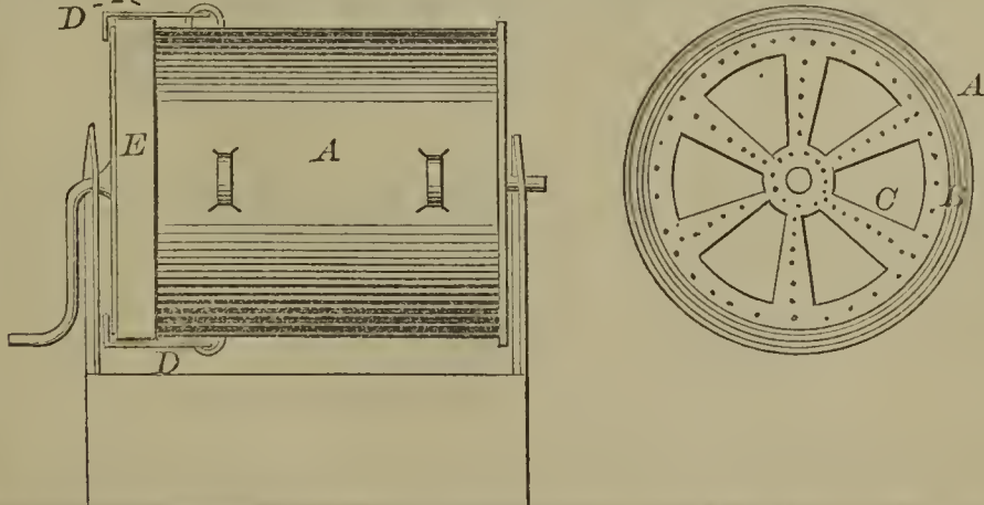
52456—G. B. Simpson—Amalgamating Gold and Silver.
