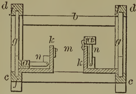
57986---T. Slight--- Baggage Car Door Lock.
