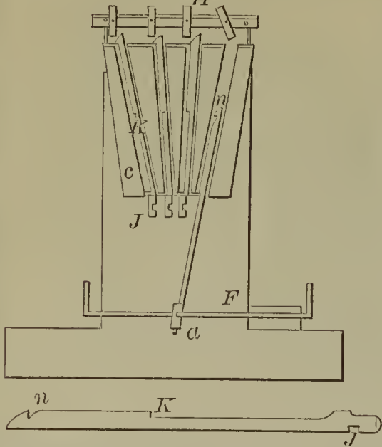
52075—J. Rankin— Churn.
