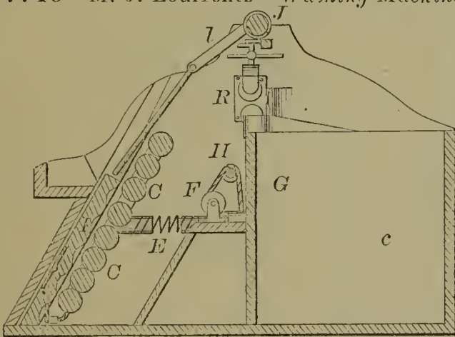
57740—M. J. Lourrentz— Washing Machine.
