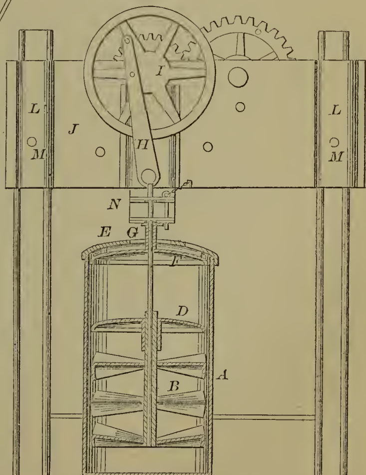
54769—G. H. Pool—Churn Dasher.
