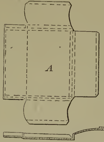
59942—A. Barnes— Manufacture of Sheet Metal Boxes.
