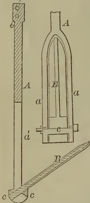
55594—E. D. Averell— Electro-Magnetic Attachment to Ruling Machines.
