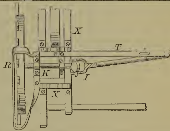
53035—A. B. Parsons—Washing Machine.
