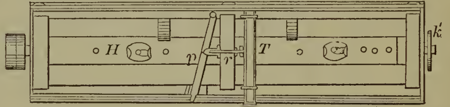
53177—J. Peacock—Barrel Washing Machine.
