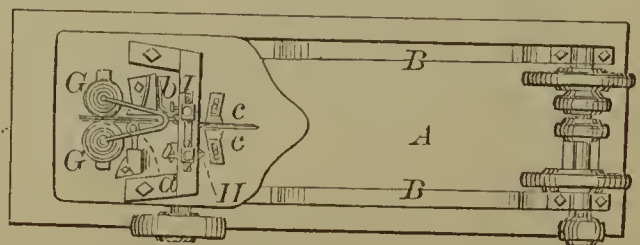
59821—J. C. Cook—Stave Machine.
