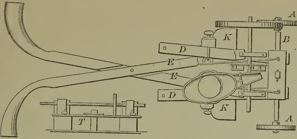
58818—A. Hartman—Railroad Switch.
