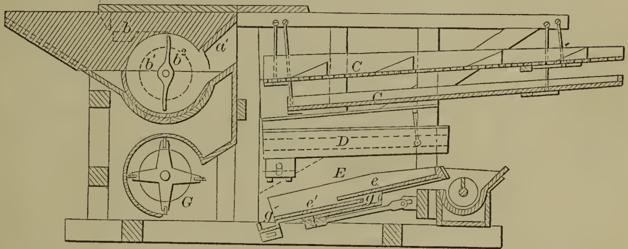
56583—M. H. Mansfield— Clover Threshing and Hulling Machine.
