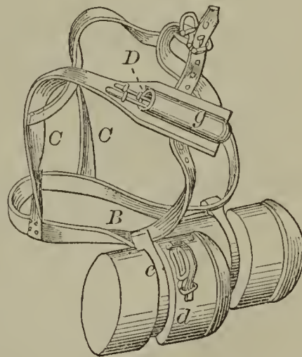
51971—E. Rousseil—Life Preserver.
