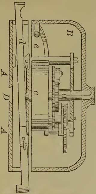
54353—E. Hoole—Burglar Alarm.
