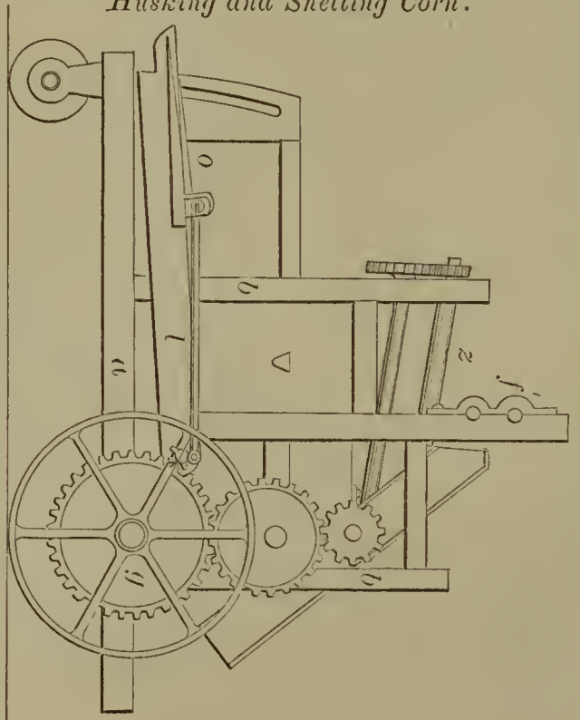
58785—D. A. Dickinson—For Harvesting, Husking and Shelling Corn.
