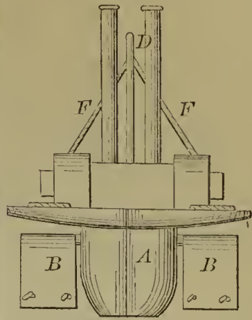
57859—T. Byrne—Dredging Machine.
