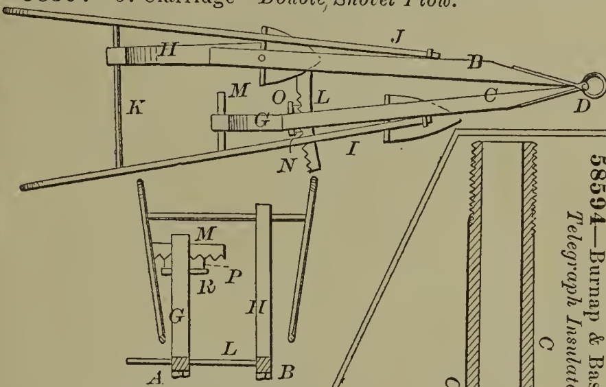
58597—J. Clarridge—Double Shovel Plow.
