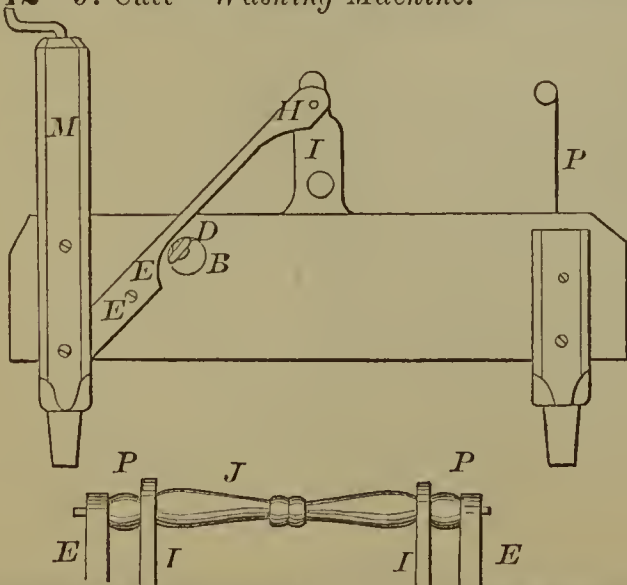
53112—J. Catt—Washing Machine.
