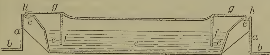
57285—Burket & Gray—For Treating Petroleum.
