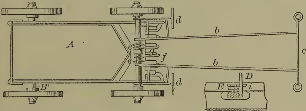
60323—W. C. Bartol—Brick Machine.
