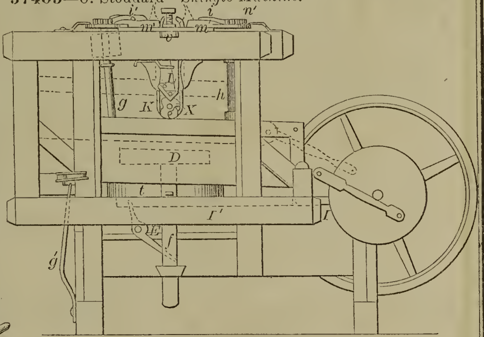
57405—O. Stoddard—Shingle Machine.
