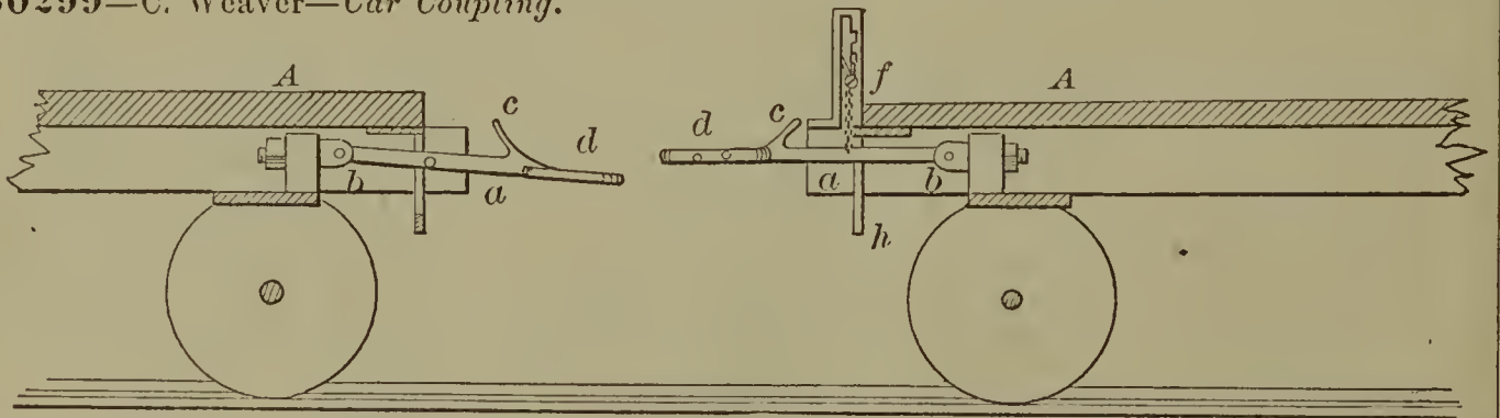
60299—C. Weaver—Car Coupling.
