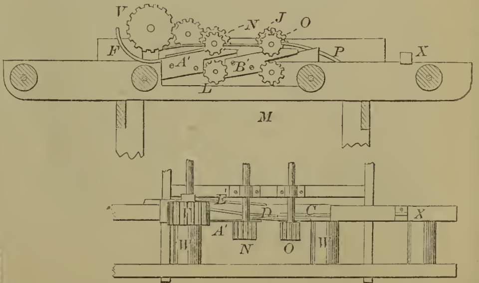
59369—J. Dobbins— For Bending Wooden Hoops.
