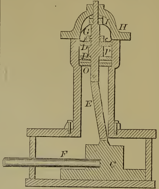
53708—Vanbebber, Sallee & Britton— Balanced Slide Valve.
