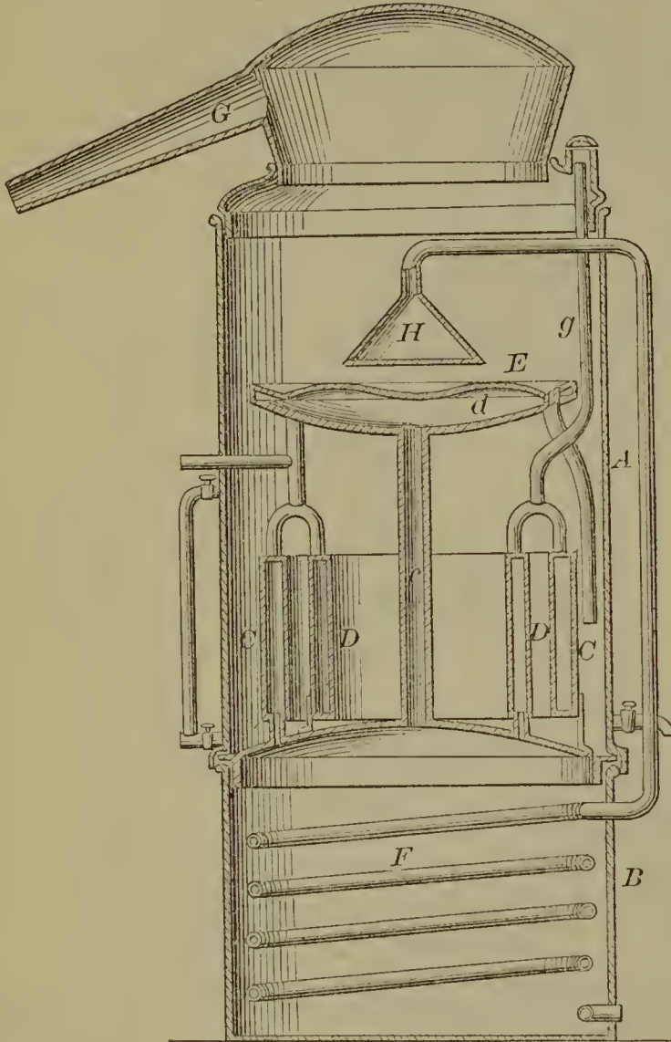
53581—H. G. Dayton— Distilling Spirits.
