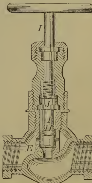
58496—T. S. Speakman— Safety Valve in Water Backs for Ranges.
