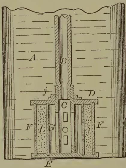
60311—W. H. Wiley—Well and Cistern Filter.
