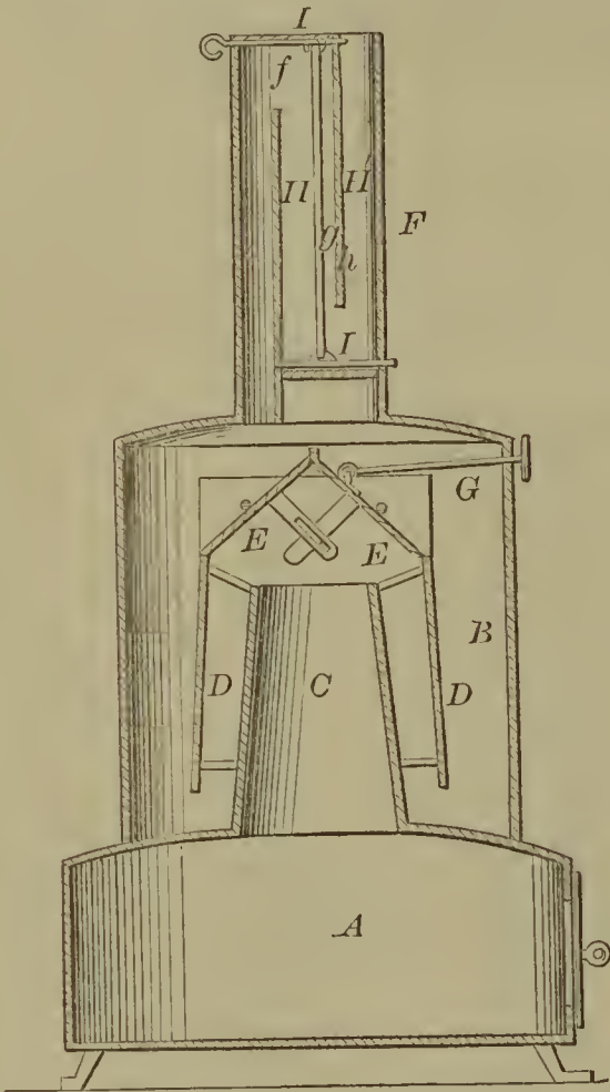
58811—G. D. Greenleaf— Stove and Drum.
