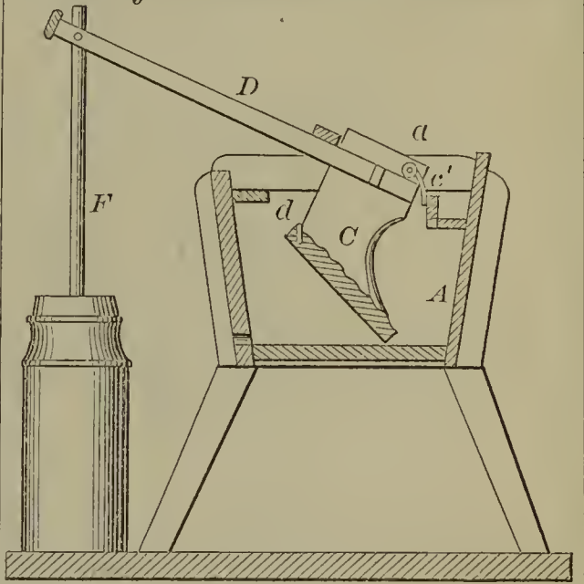
52275—S. R. Drummer—Beater Press.
