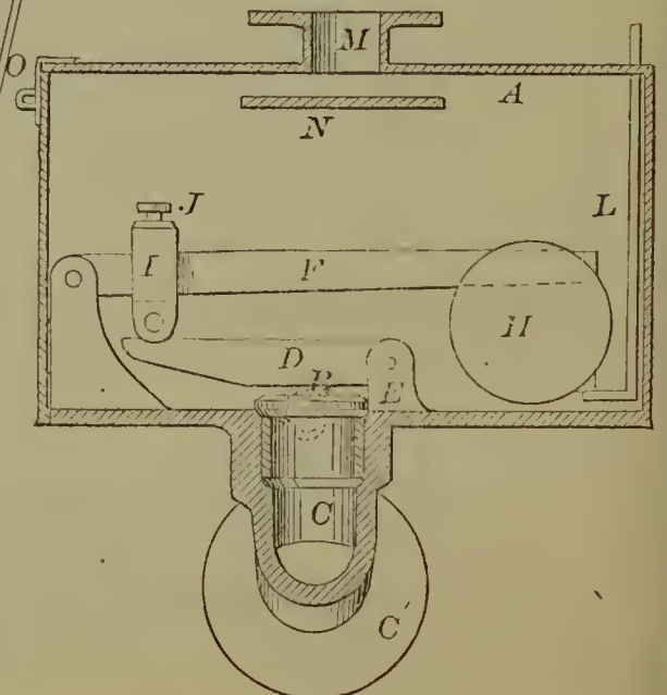
59764—C. M. Farrar—Lock-up Safety Valve.
