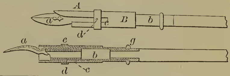
53624—J. E. Hunter— Broom Head.
