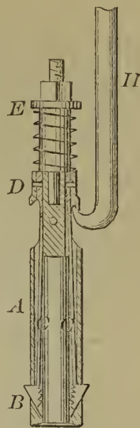
56961—J. H. Luther—Grab for Oil Wells.
