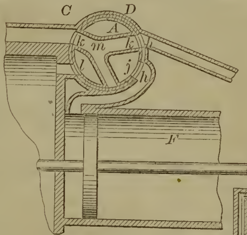
60638 —J. L. Mackey— Rotary Steam Valve.
