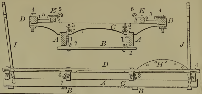
60270—Smith & Brumfield—Horse Rake.
