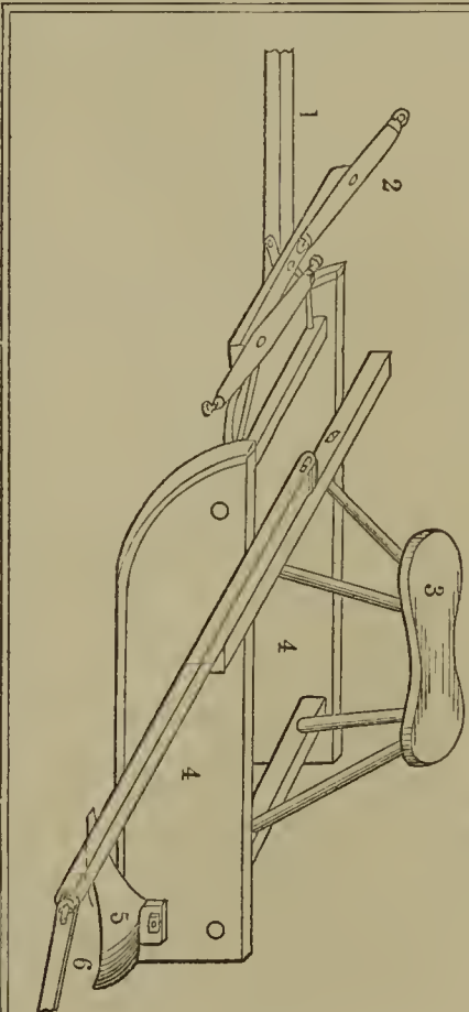
52598—J. Plumb—Furrower for Corn Planting.
