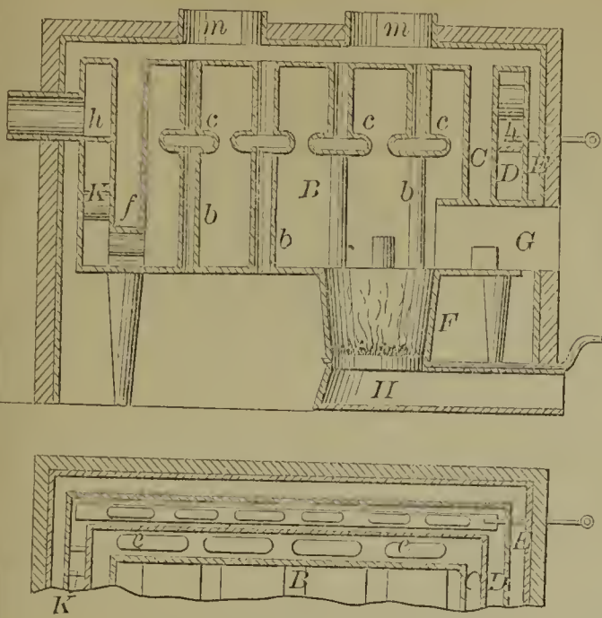
57026—H. Whittingham—Hot Air Furnace.
