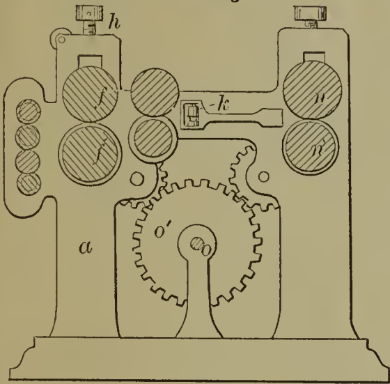
56393—C. A. Ensign— For Making Corded Binding.
