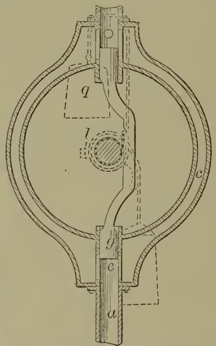
60084—F. Taggart—Steam Engine Governor.
