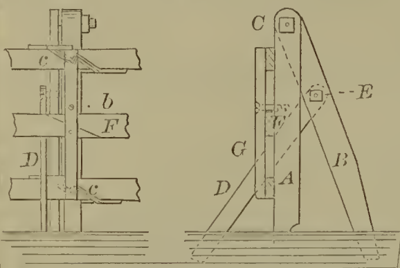
55881—J. McDonald—Carding Machine.
