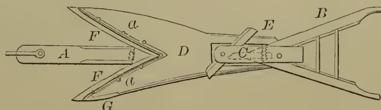
59557—J. Coffey— Bog Cutting Plow.
