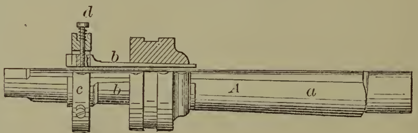
59948—I. Beetison—Expanding Mandrel.
