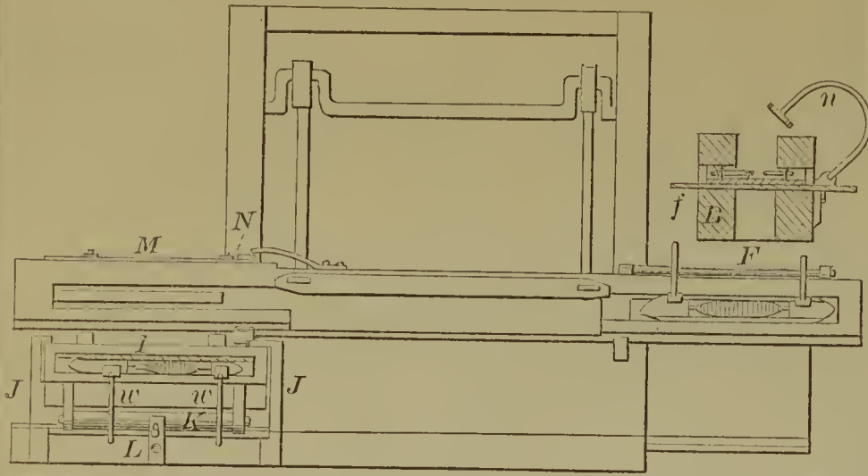
57712—P. W. Hart—Power Loom.
