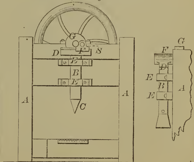
59423—Love & Thornly— For Operating Wood Splitting Machines.
