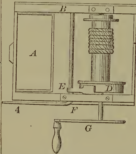
54231—T. Thomasson— Evaporator.
