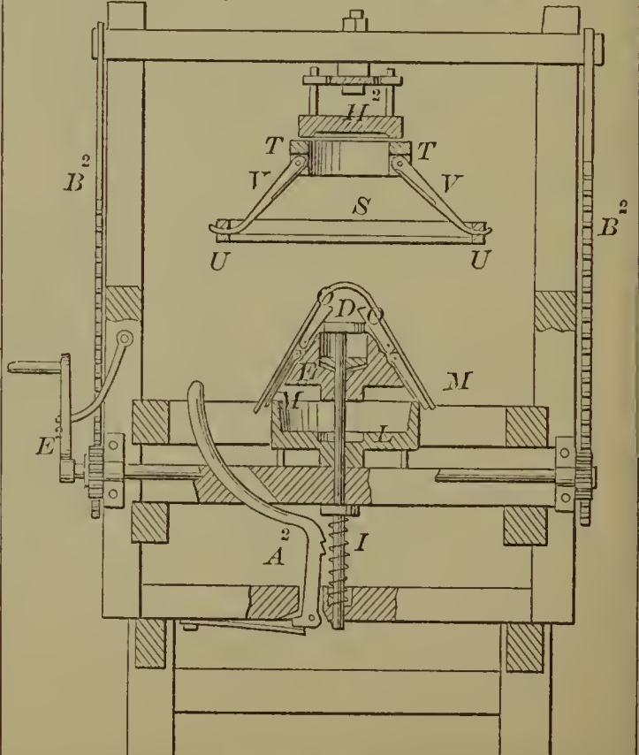
59707—S. Boyden—Hat Blocking Machine.
