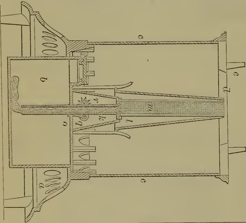
55032—O. F. Morrill—Petroleum Stove.
