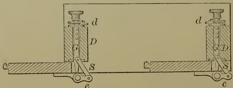
54996—J. Aborn— Blind Fastener.
