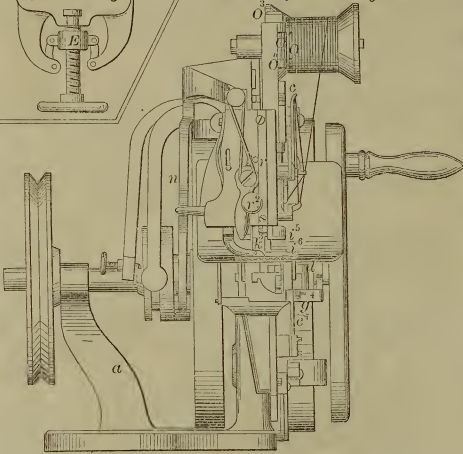
57451—J. M. Clements— Sewing Machine for Stitching Button Holes.
