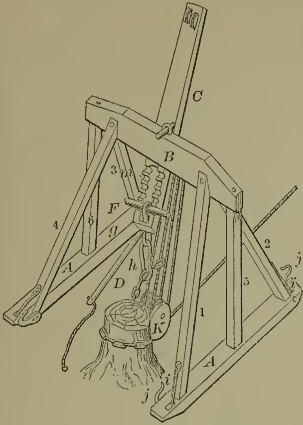
59904—I. Flanders— Stump Extractor.
