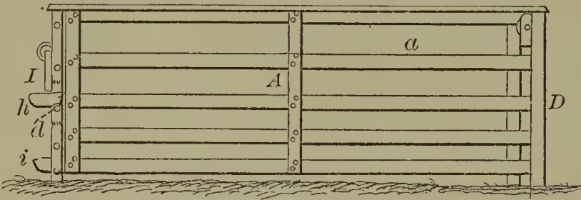
59930—S. Spoor—Gate.
