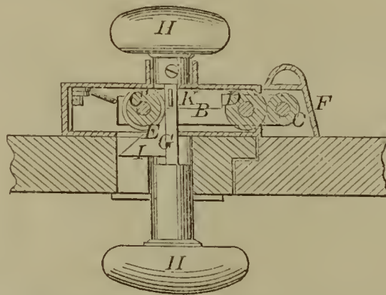
57428—J. E. Wootten— Winding Apparatus for Inclined Planes.
