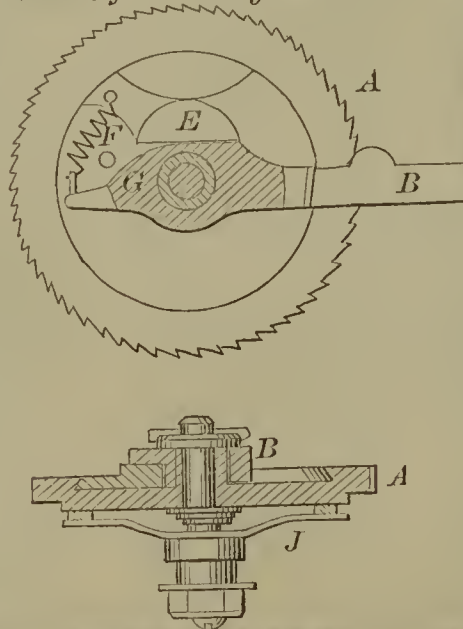
55847—A. Galleth—Feeding Wheel for Sewing Machines.
