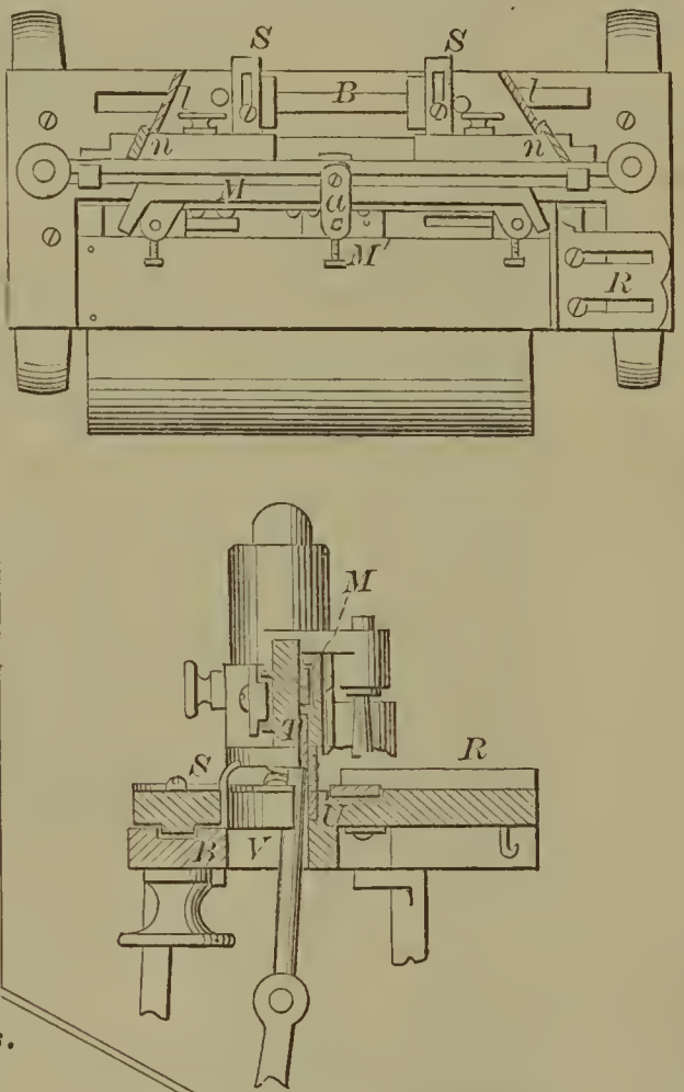
58812—Grissold & Sigwalt— For Making Paper Collars.
