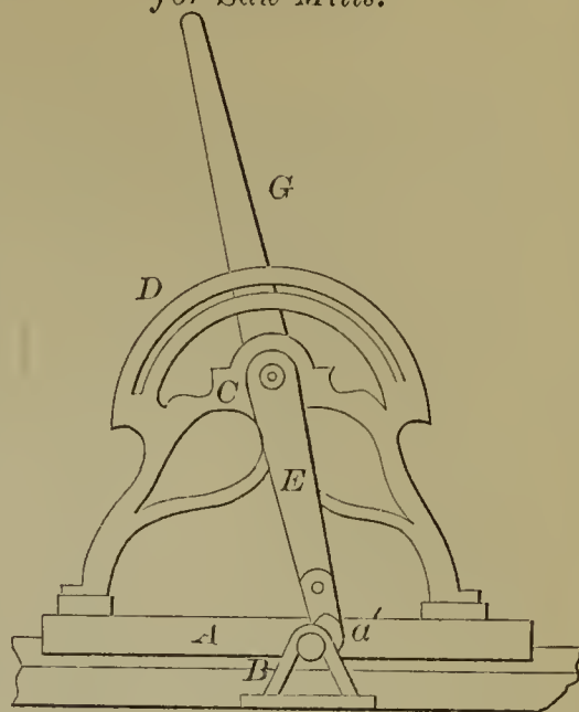
54330—H. H. Gridley—Head Block for Saw Mills.
