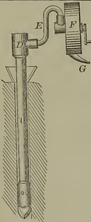
51984—O. G. Warren—Suction Drill.
