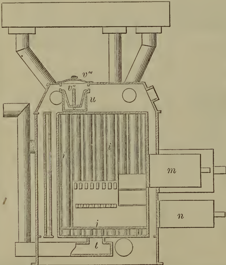
55564—E. Webster— Hot Air Furnace.
