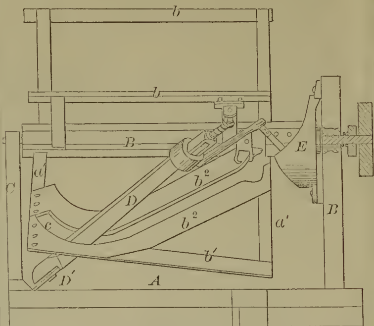
55884—D. Morris—Well Boring Apparatus.
