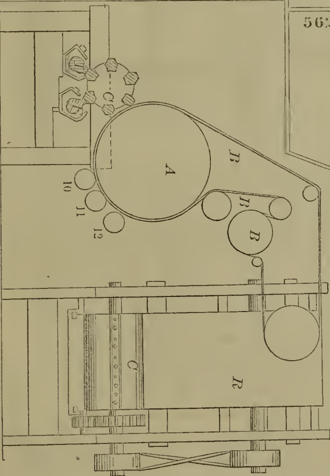
56208—J. Green—Printing Textile Fabrics.
