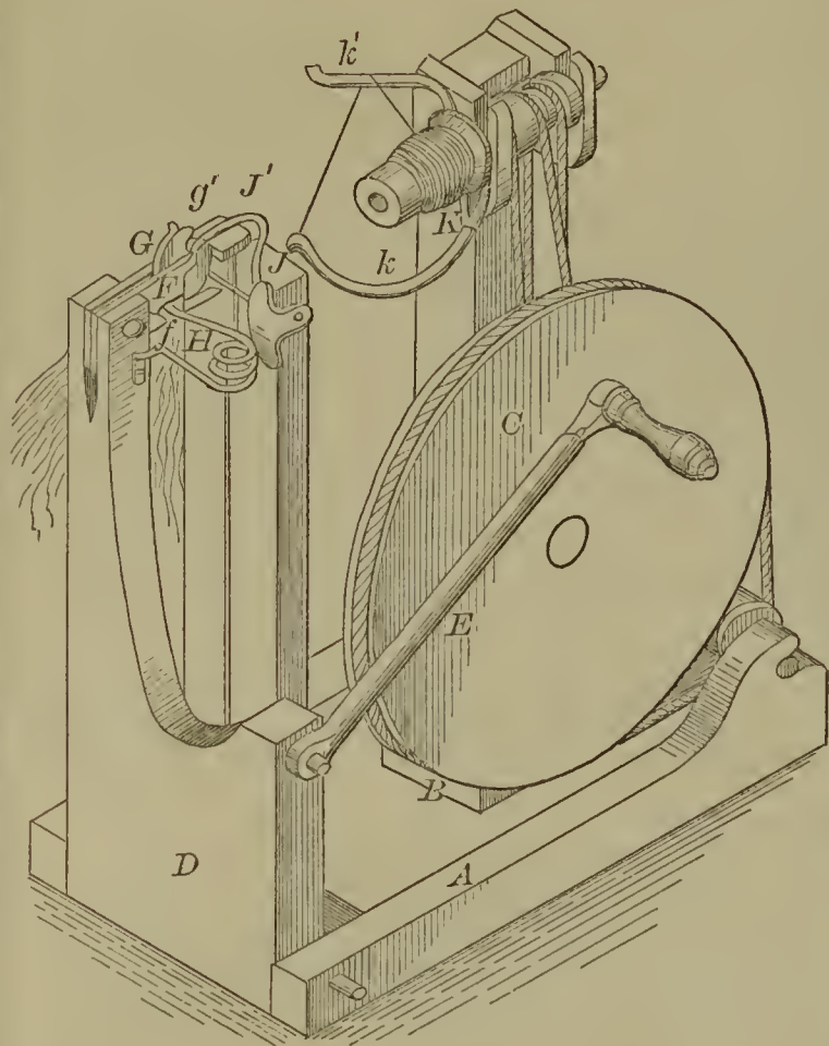
52506—L. Skeels— Flax Spinning Machine.
