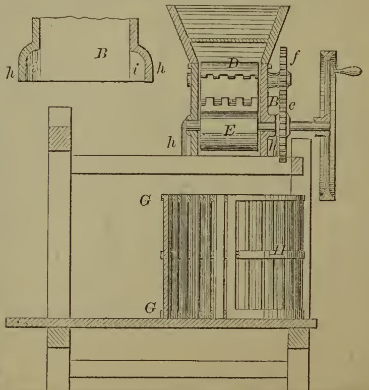
57833—H. Sells—Cider Mill.
