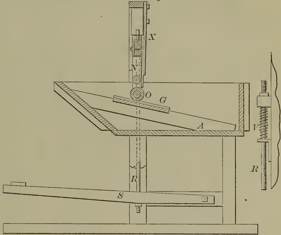
52185—A. Mitchell— Washing Machine.
