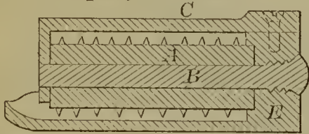
53423—W. W. Dutcher—Roller Temple for Looms.
