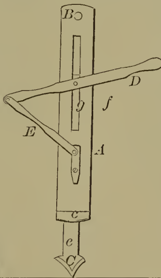
58237—D. Fasig— Straw and Hay Knife.
