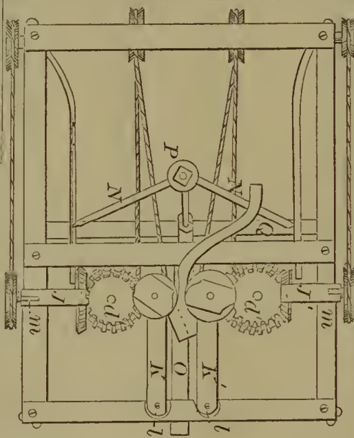
56548—J. Garfield—Planing Machine.
