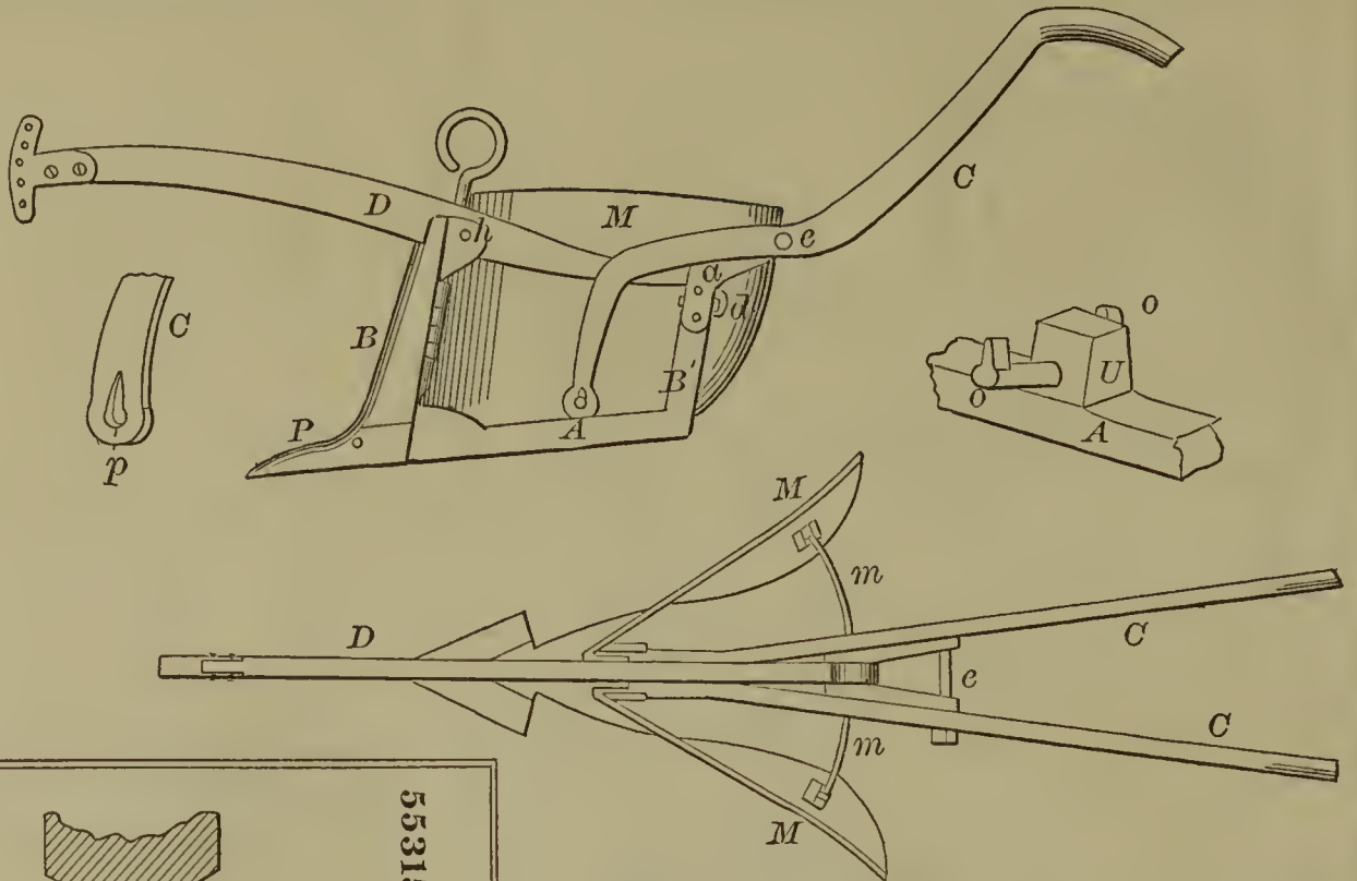
55312—M. Kennedy— Plow.
