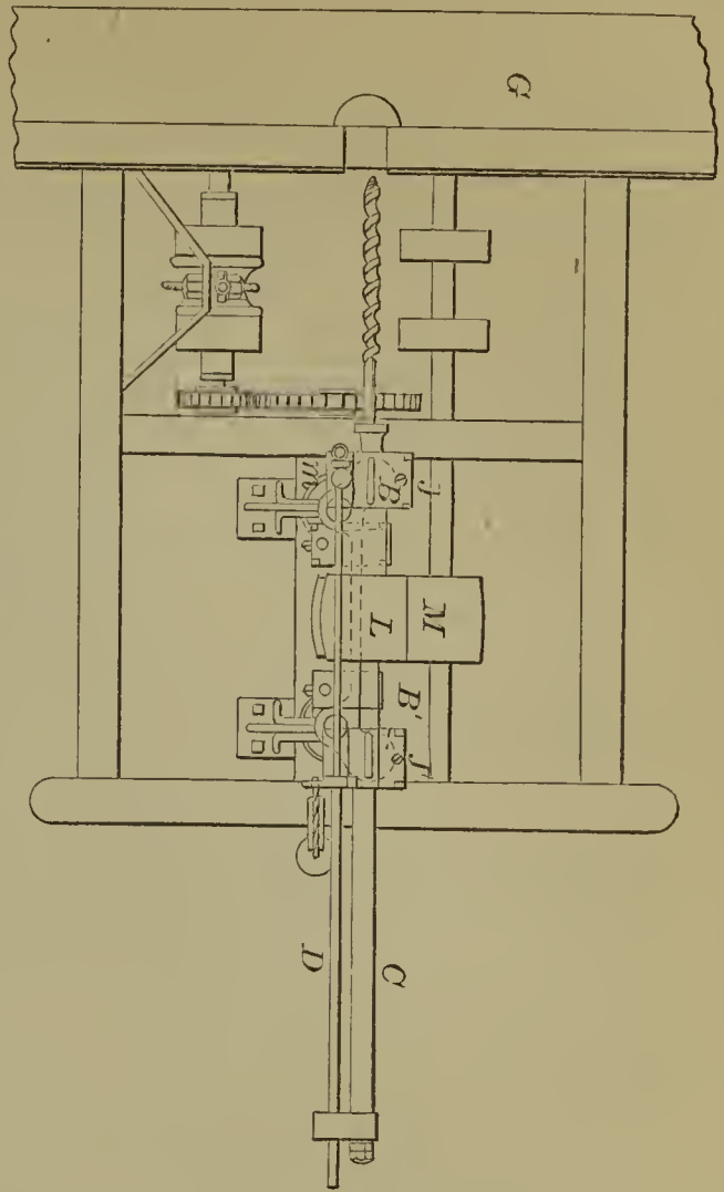
57718—D. Hoit—Wood Boring Machine.
