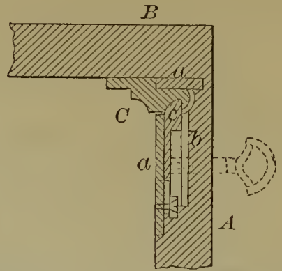
55048—Bohannon & Johnson— Lock.
