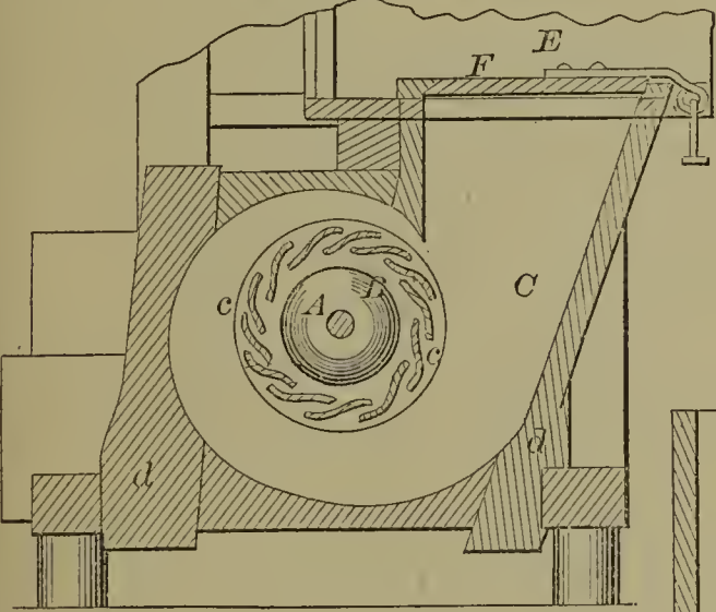
54660—I. J. W. Adams— Water Wheel.
