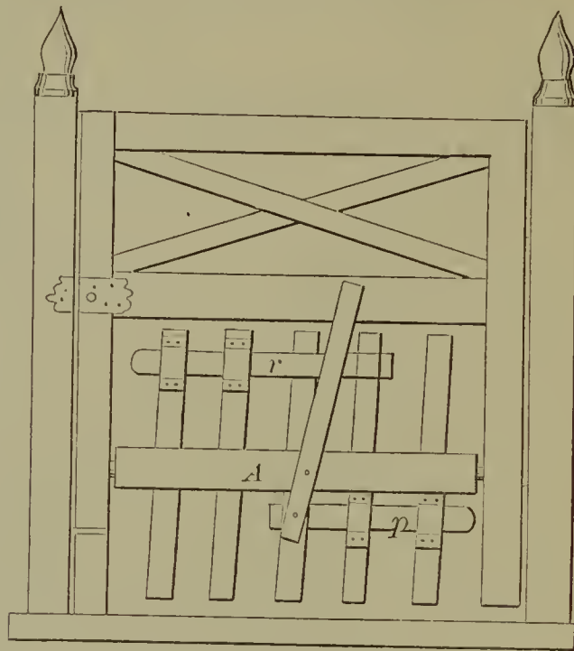
55481—P. Freeman—Gate.
