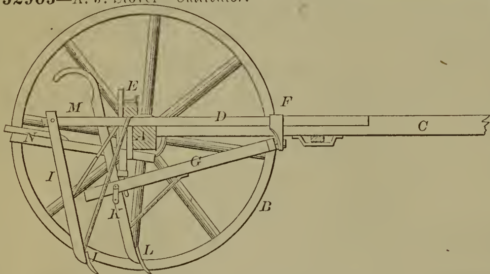
52905—A. J. Stover—Cultivator.
