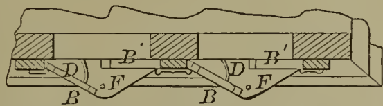
60470—R. C. Bristol— Water and Steam Separator for Steam Generators.
