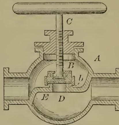
54025—T. A. Searle— Globe Valve.
