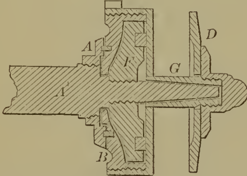
58247—C. H. Guard—Attaching Hubs to Acles.
