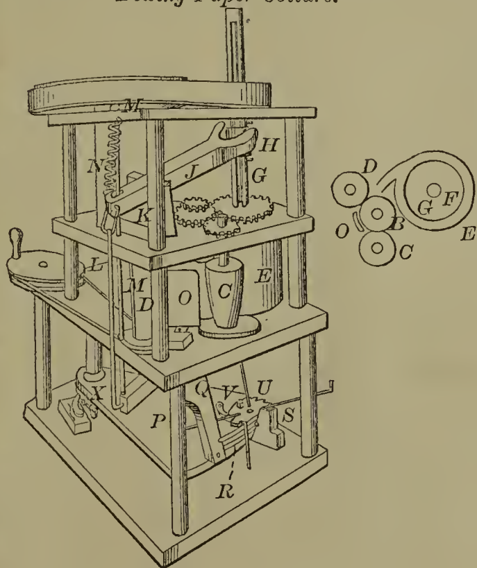
60484—Currier & Wells—For Finishing and Boxing Paper Collars.
