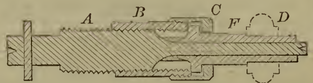
55681—C. W. Le Count— Adjustable Mandrel.
