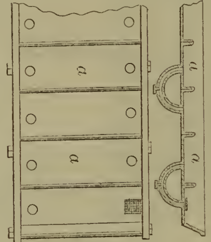
57224—P. O. V. Slyke—Sorghum Evaporator.
