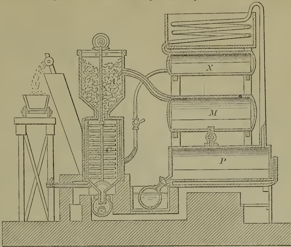
52283—H. P. Gengembre—For Extracting Oil, &c., from Minerals.
