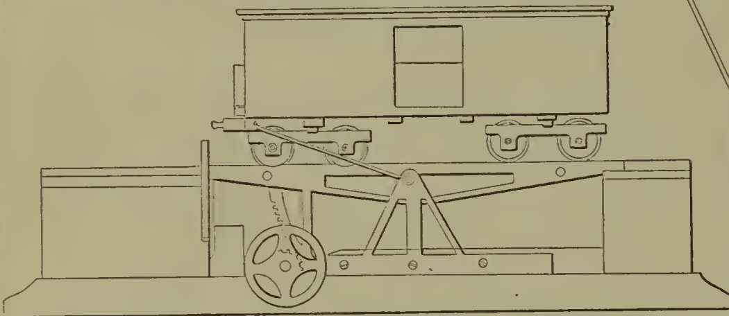
58928—D. J. Whittemore—For Unloading Grain Cars.
