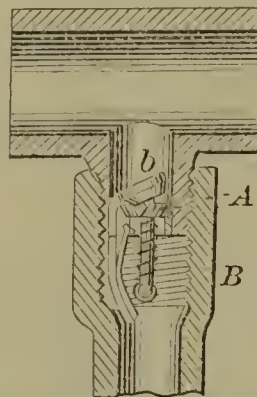
54915—B. Jacobs— Attachment to Gas Fixtures.
