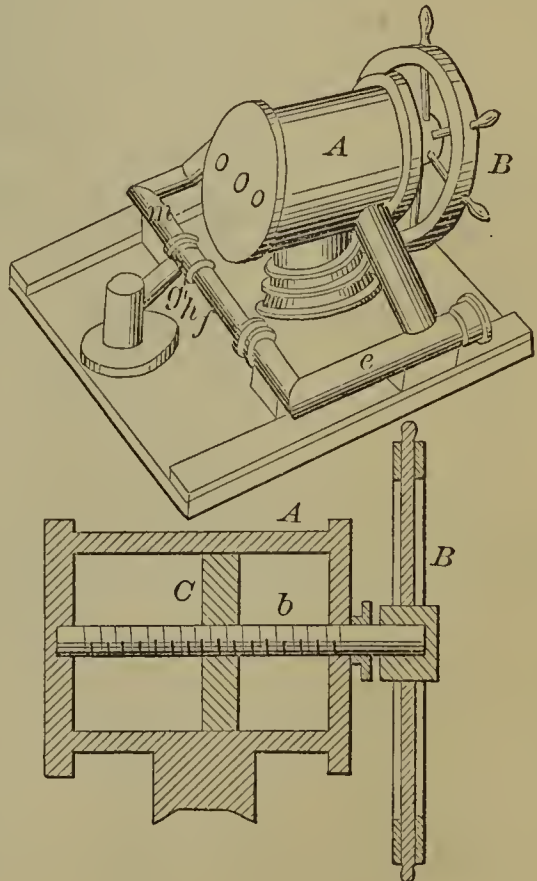
52970—H. O. Cook— Hydraulic Steering Apparatus.
