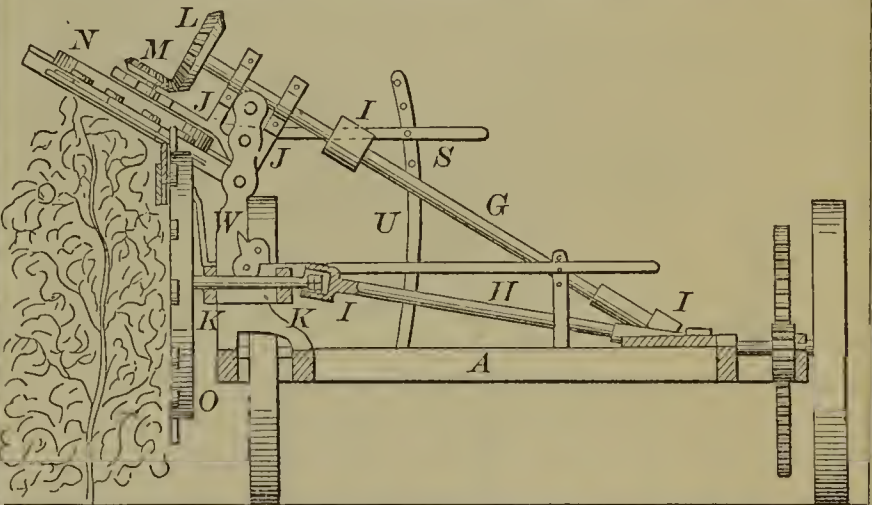
53033—D. Oliver—Hedge Cutting Machine.
