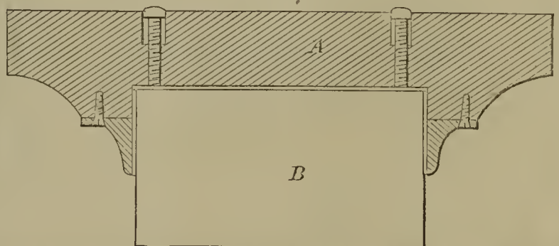
52491—J. Hankey— Carrier's Scourer.
