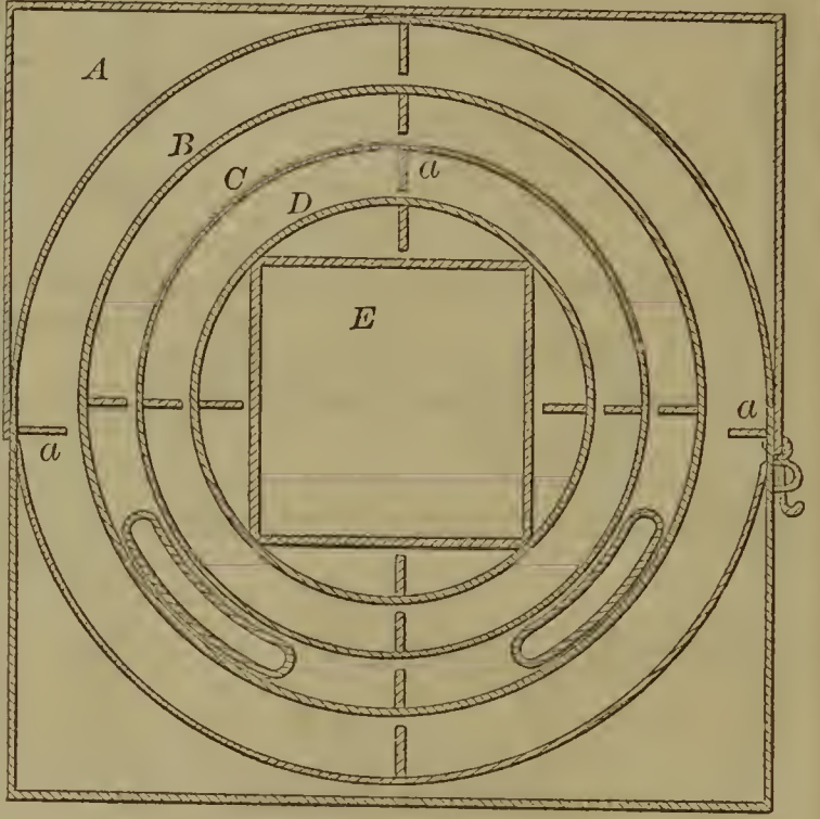
56451—Saladee & Armstrong—Padlock.
