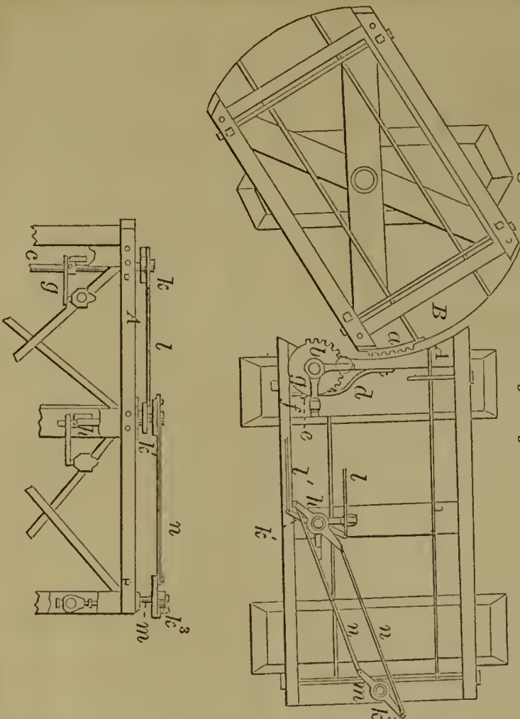
56492—Fowler & French— Percussion Cap Trimming Machine.
