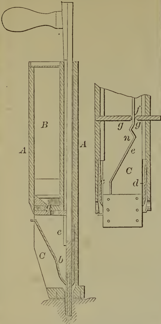
55399—C. A. Wakefield— Hand Corn Planter.
