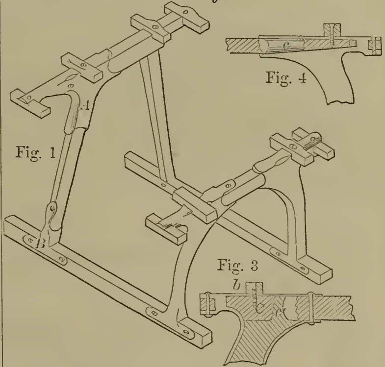
55705—T. W. Porter— Sleigh.
