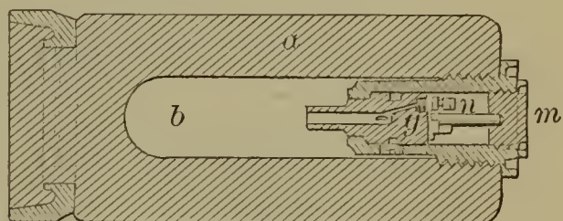
54027—J. F. Sherman— Percussion Fuse for Explosive Shells.
