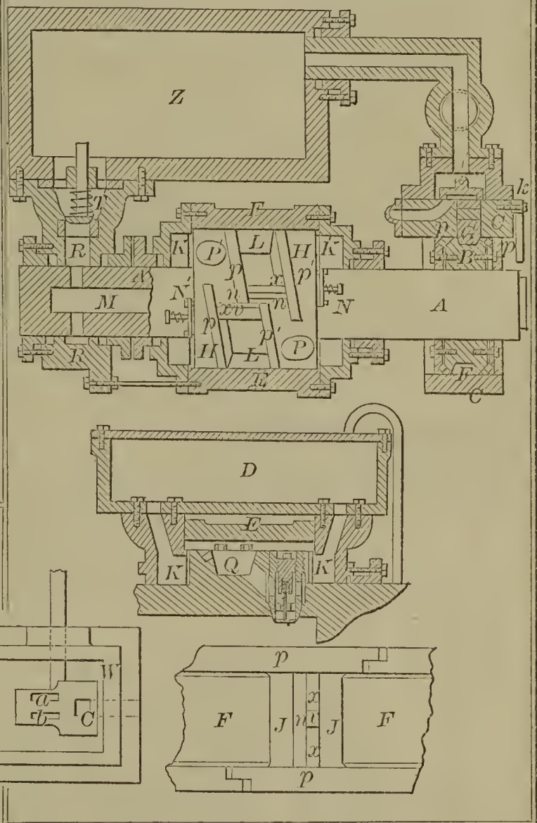
57298—J. Dreisörner—Hydraulic Engine.
