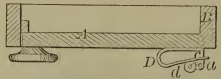
57239—J. D. Winslow—Shutter Fastening.
