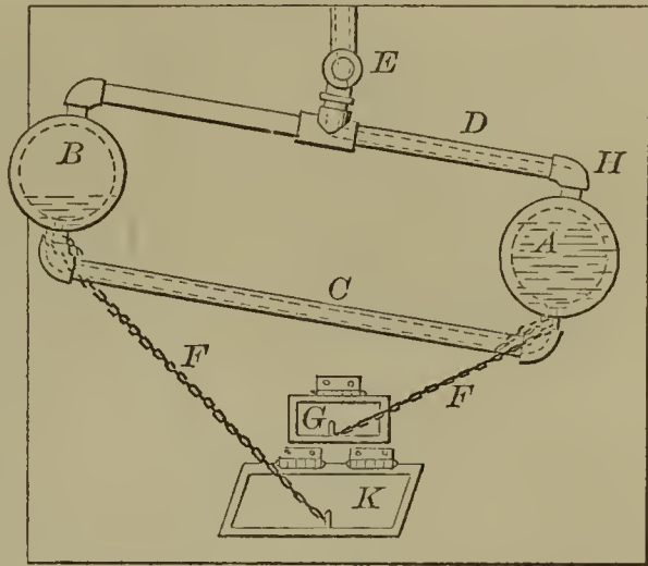
52694—J. W. Dixon—For Manufacture of Paper Pulp
