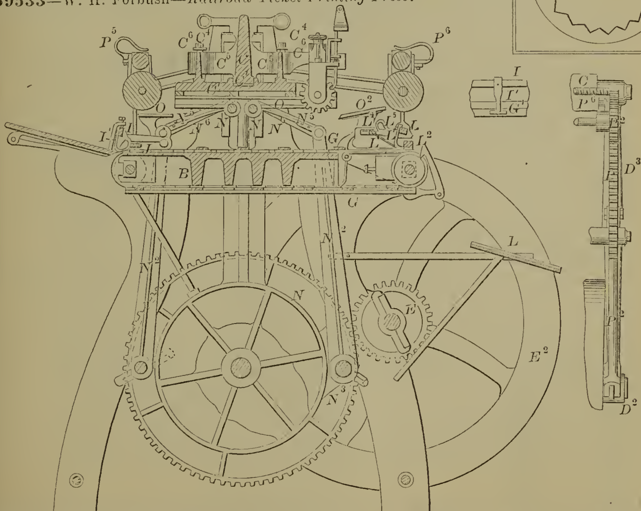
59533—W. H. Forbush—Railroad Ticket Printing Press.
