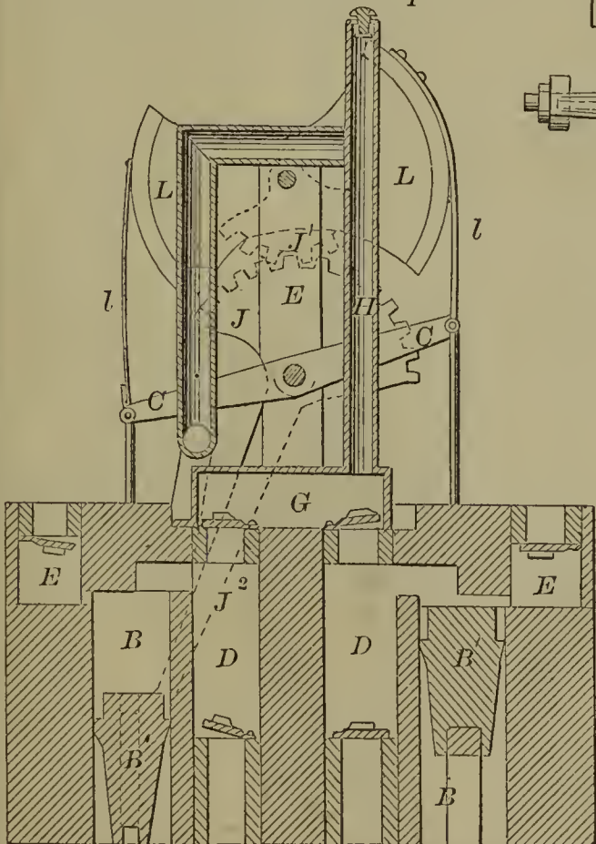
56637—D. M. Thomas—Pump.
