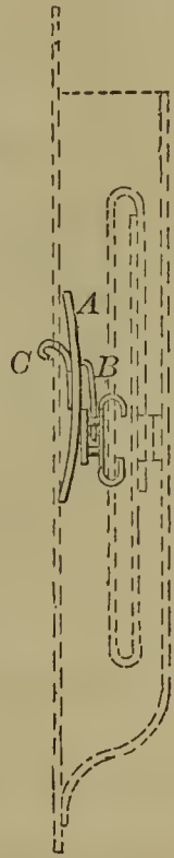
56145—C. Leffingwell—Head Block for Saw Mills.
