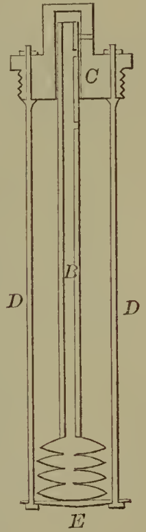
55801—A. Arnold—To Prevent Boiler Explosions.
