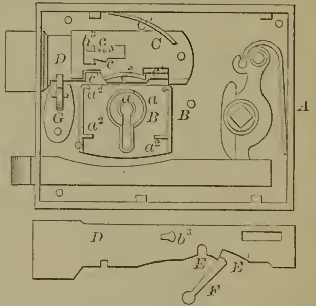
55244—Corbett & Burns— Lock.
