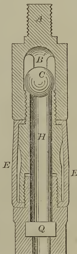
51990—Allen, Rouse & Melcher—Packing Pump Pistons.
