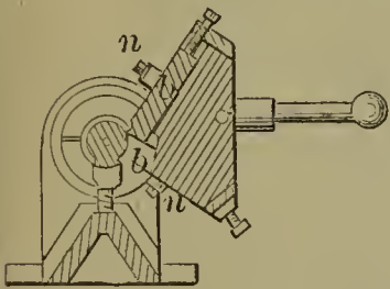
59871—D. H. Stephens— For Making Rule Joints.
