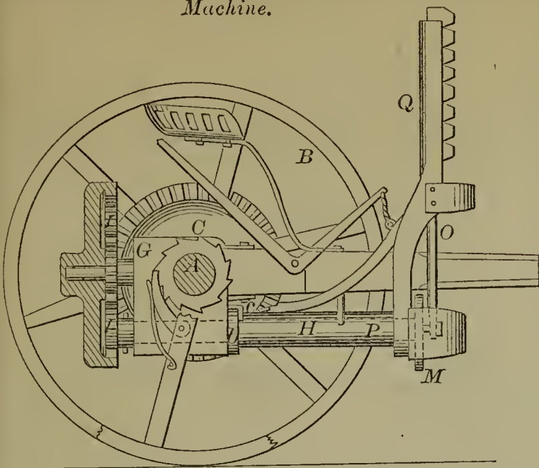
53198—D. H. Thayer— Reaping and Mowing Machine.
