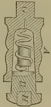
52497—Perry & Gladding—Door Guard.
