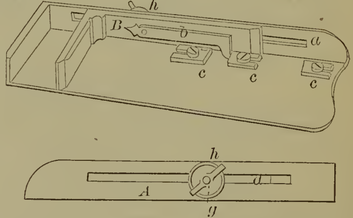
54979—W. T. Tillinghast— Composing Stick.
