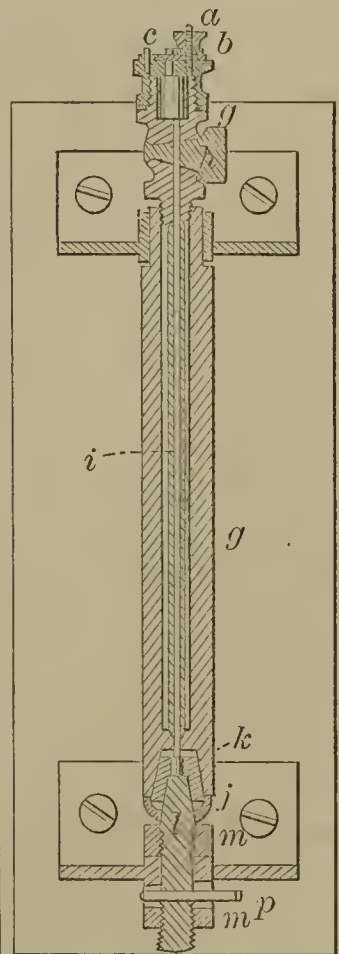
52454—J. F. Schuffenker—Lubricating Vertical Shafts.
