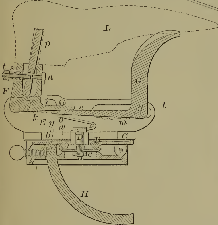
54958—U. Reynolds— Fifth Wheel for Vehicles.
