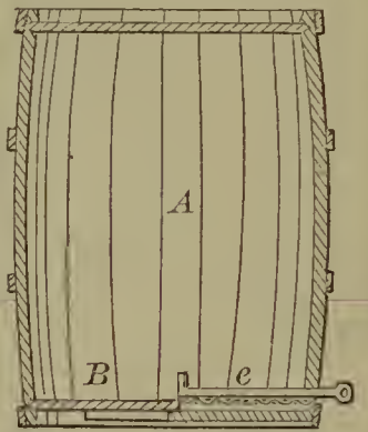
54444—W. H. Towers— Flour Barrel.
