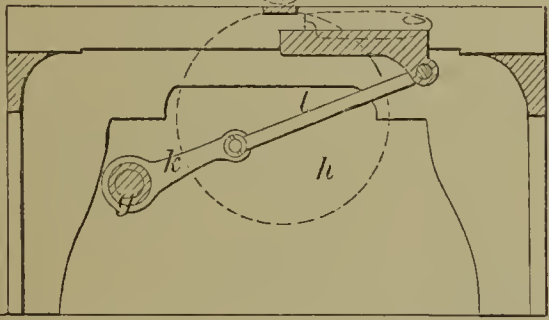
58187—Ackland, Mitchell & Mustapha— Cotton Gin.
