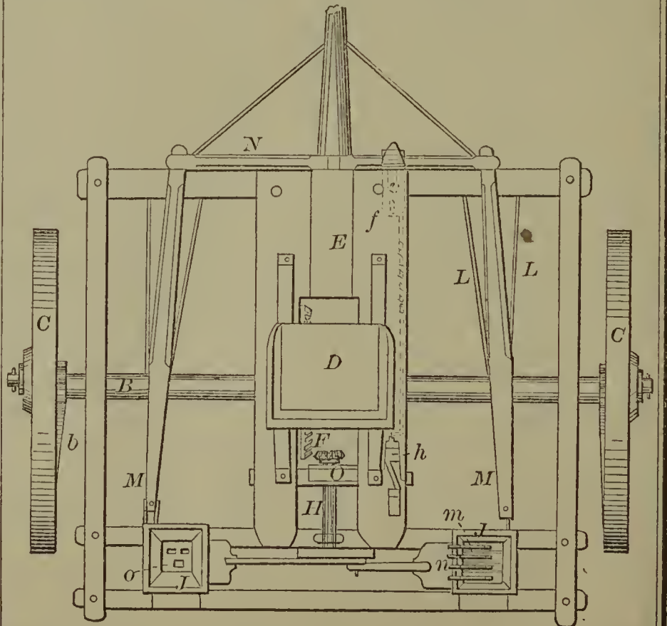
57994---S. M. Swartz--- Combined Corn Planter and Plow.
