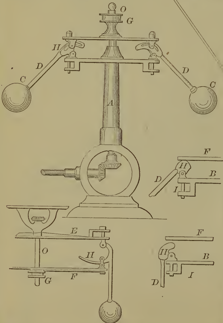
59411—E. H. Knight—Governor.
