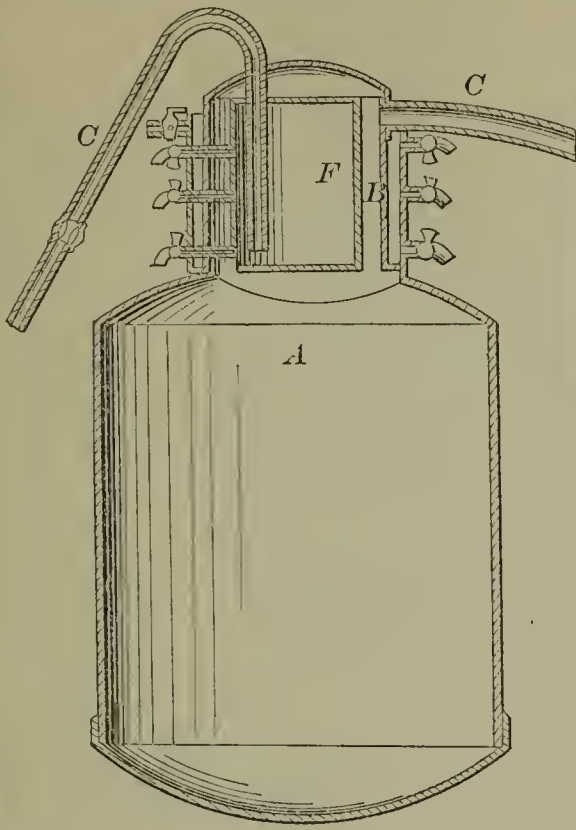
52151—L. S. Fales—For the Distillation of Tar, &c.
