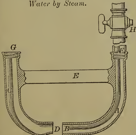
58317—J. W. Stiles— Raising Water by Steam.
