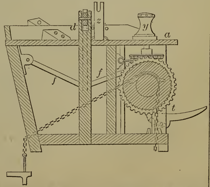
54688—G. Coffin— Operating Ship's Windlass.
