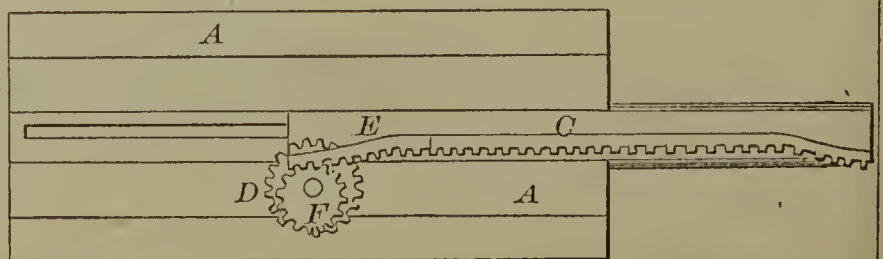
60301—C. Wells—Rack Motion for Hand Presses.
