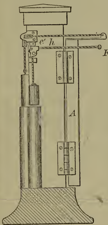
55906—Raymond & Miller—Fence Gate.
