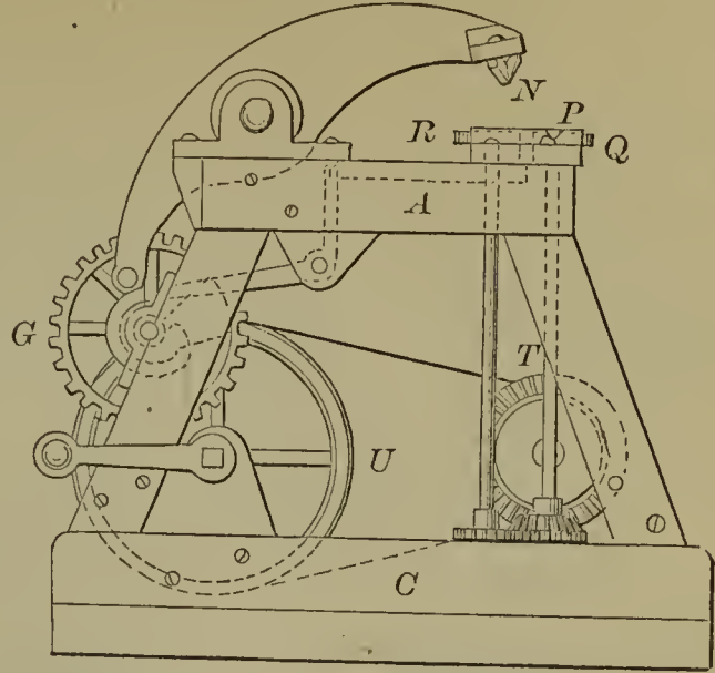
59134—C. E. Moore—For Folding Paper Collars.
