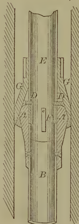
52448—Robinson & Strong—Packing for Deep Wells.
