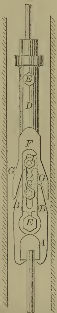
52437—D. F. Mellen—Grab for Oil Wells.
