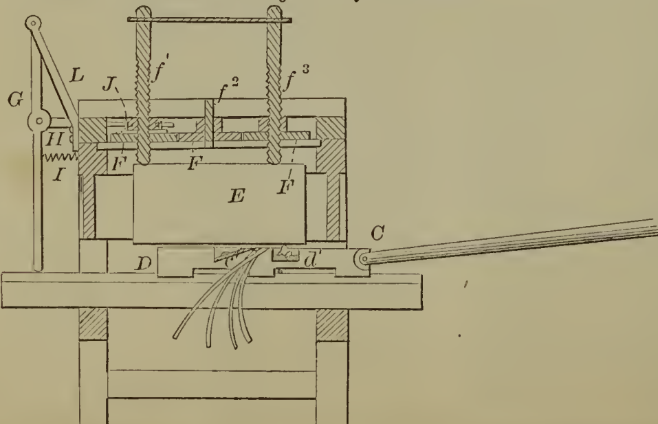
55415—M. Free—For Cutting Slats for Blinds.
