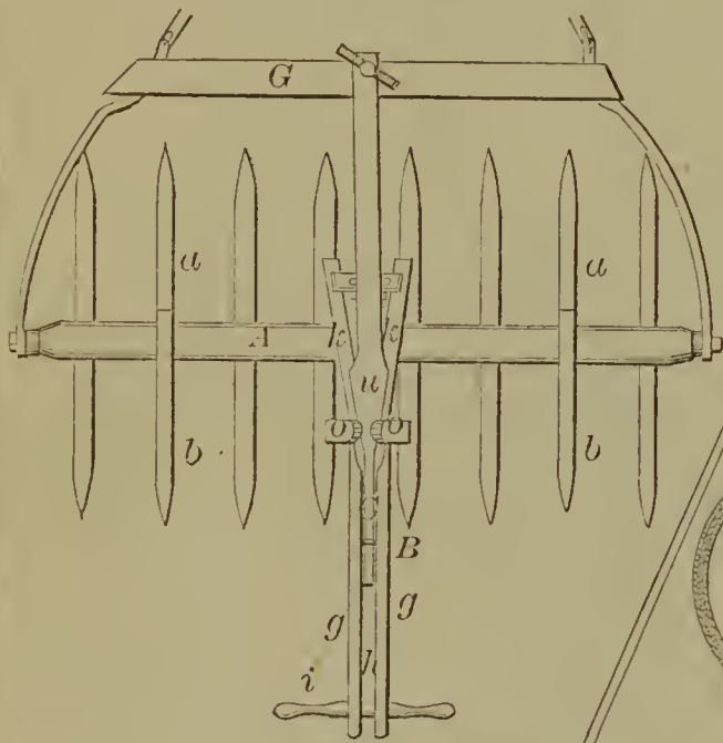
59113—J. Wood—Horse Rake.
