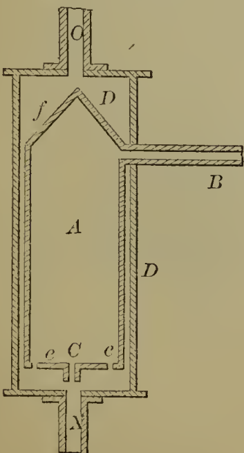
54940—J. Nicholson— Feed Water Heater.
