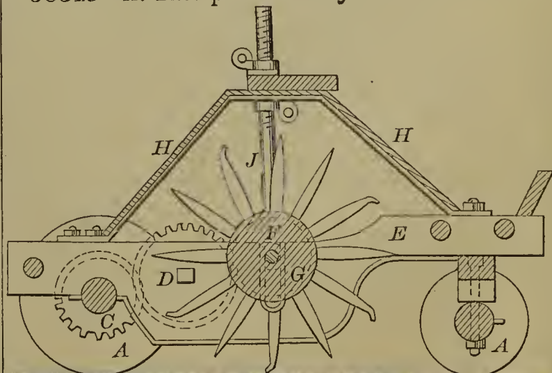
58319—A. Thompson— Rotary Cultivator.
