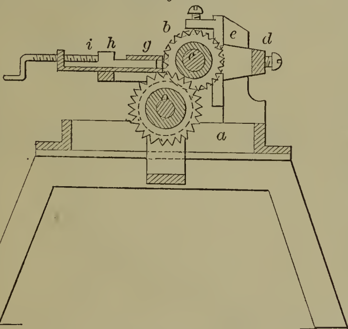
54262—T. J. Sloan—Grinding Mill.
