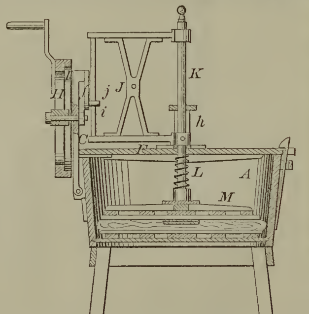
51977—Stafford & Crossman—Washing Machine.
