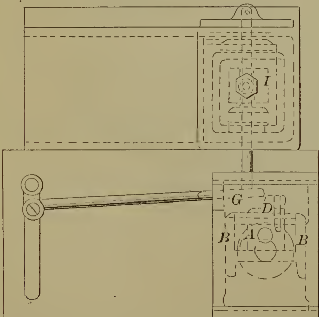
54153—J. L. Hewes—Cut-off Valve.
