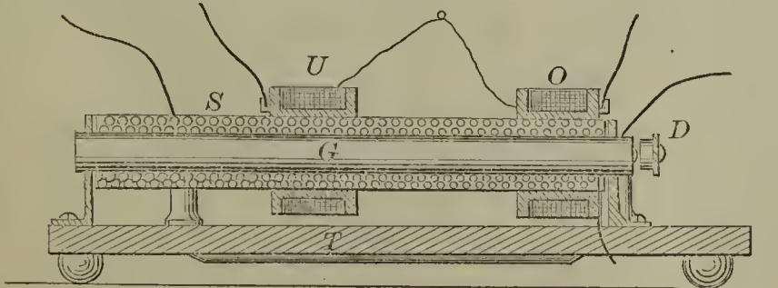
52054—Dr. J. Kidder— Induction Coil.
