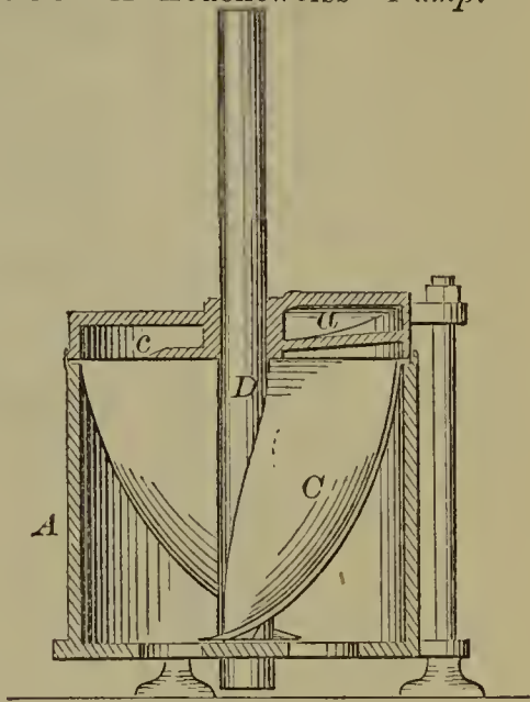
53939—A. Leuchtweiss— Pump.
