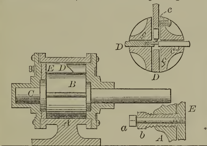
51936—W. & R. Foster—Rotary Pump.
