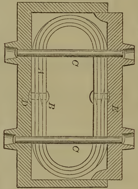
56084—W. R. Nichols— Car Spring .
