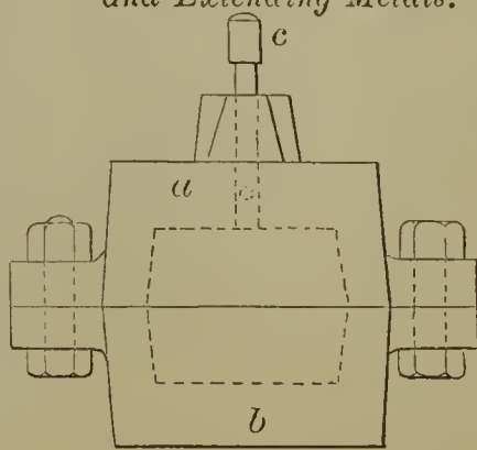
56807—J. F. Shearman—Compressing, Condensing and Extending Metals.
