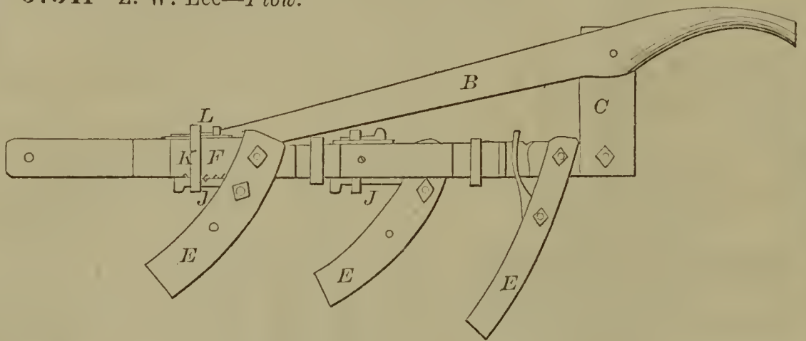
57341—Z. W. Lee— Plow.
