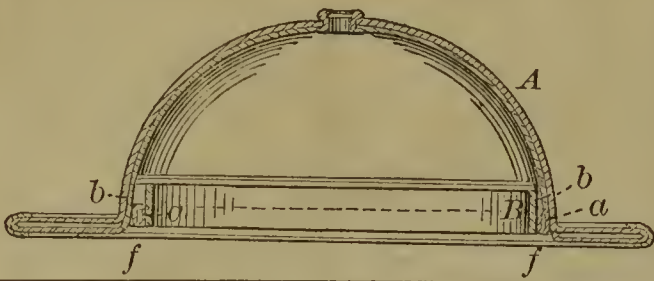
56448—T. L. Reed—Coupling for Gas Fixtures.
