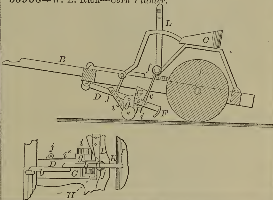
55908—W. E. Rich—Corn Planter.
