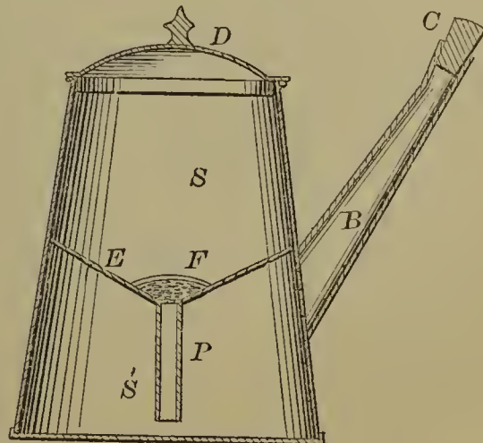
58396—W. Edson—Coffee Pot.
