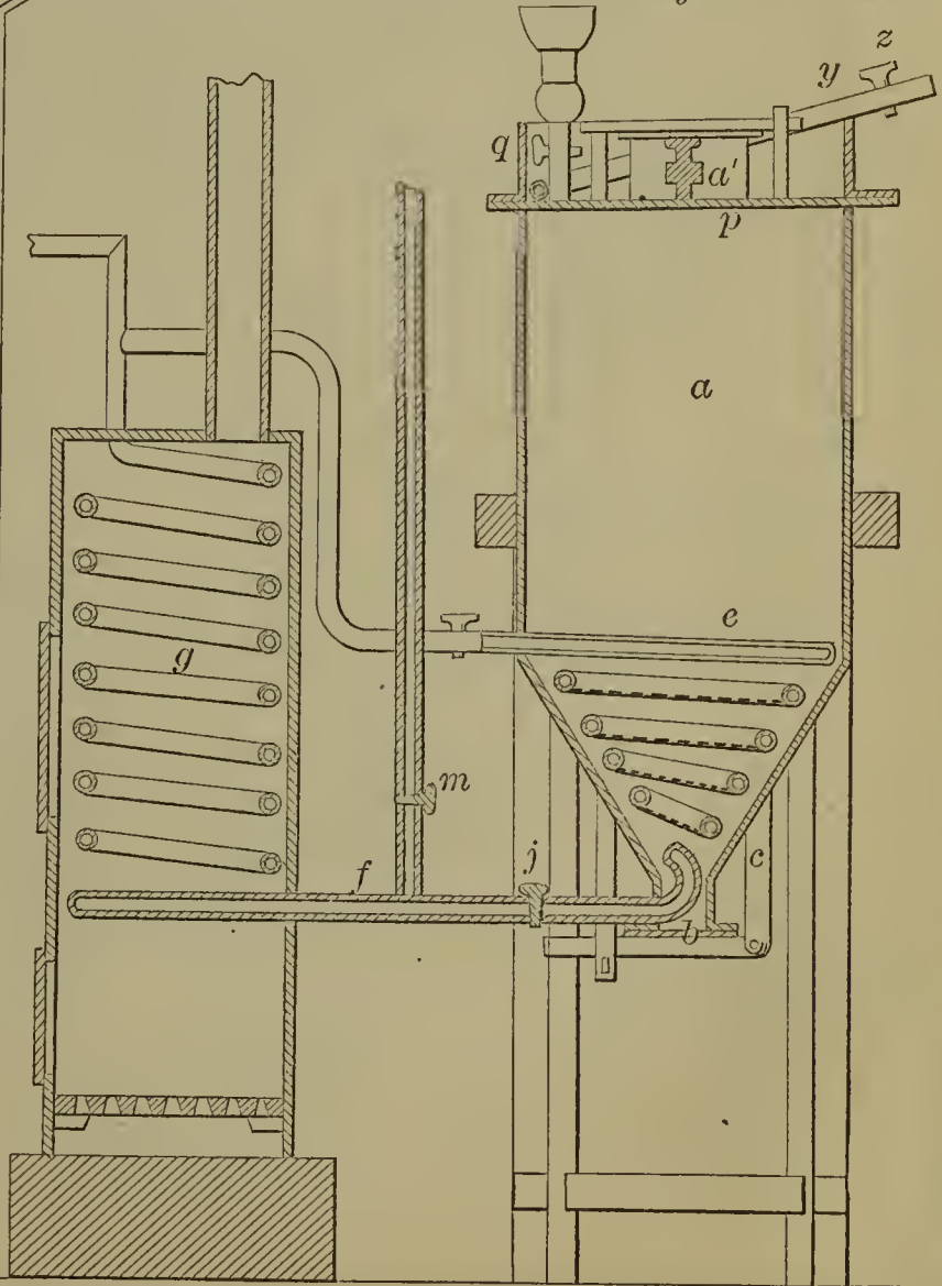
54412—V. B. Ryerson—Extracting Precious Metals.
