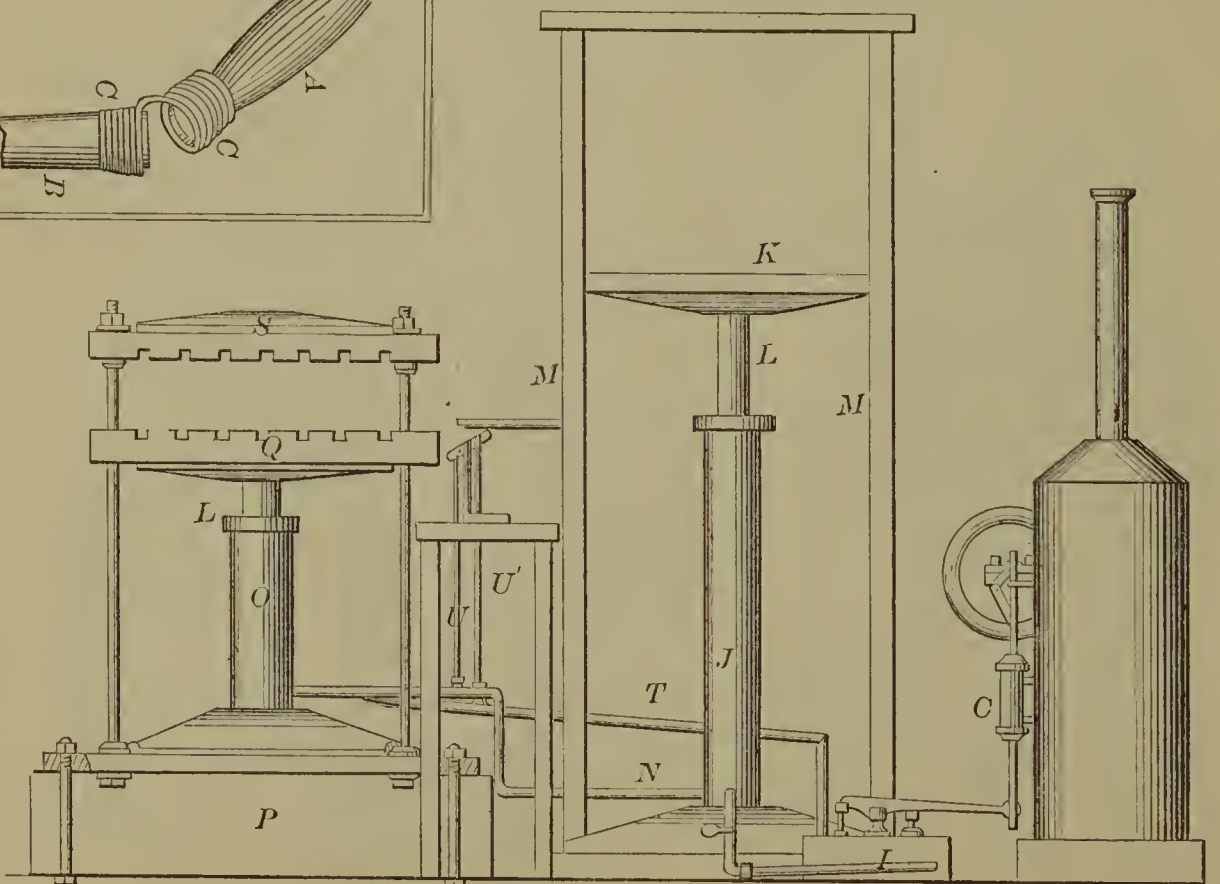
59853—T. E. McNeill—Cotton Press.
