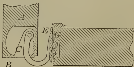
55987—G. W. Beers—Carriage Hinge.
