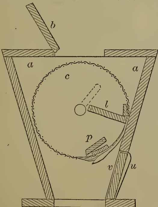
54149—P. Harlow— Ash Sifter.
