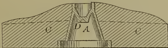
57752—L. B. Moore—Corn Cultivator.
