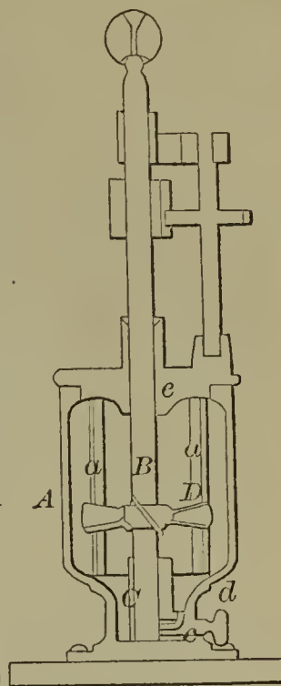
60192—R. K. Hamton— Steam Engine Governor.
