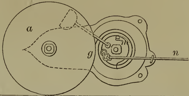
58576—H. Barton— House Bell.
