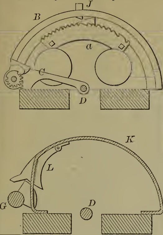
53988—W. O. Jones—Steering Apparatus.
