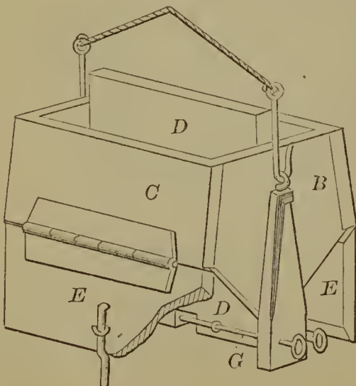
58248—J. Haines—Fuel Damper.
