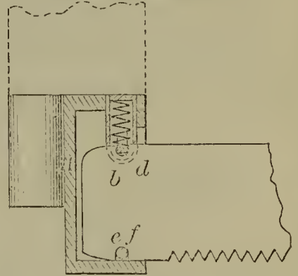
52285—W. H. Gilliam—Attaching Saws to Handles.
