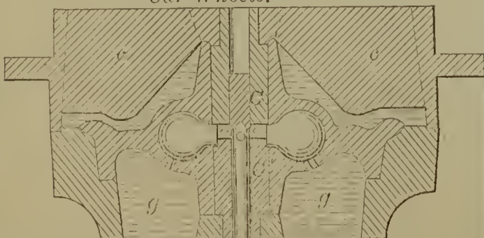
56958—J. W. Latcher— Centre Chill for Car Wheels.
