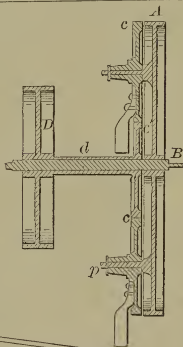
60126—W. Bicknell—Communicating Motion.
