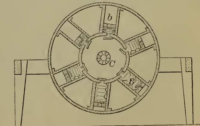
53609—F. Hainsworth—Rotary Blower.
