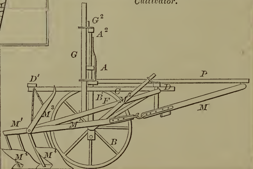
60589—W. W. St. John—Gang Plow and Cultivator.
