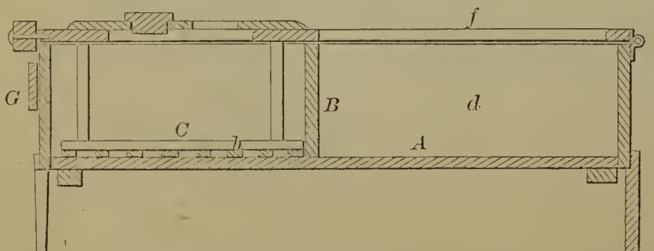
54965—E. Sawyer—Washing Machine.
