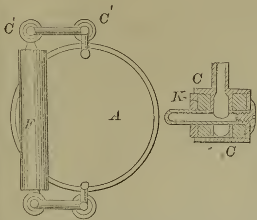
55821—R. Cochran—Pump.
