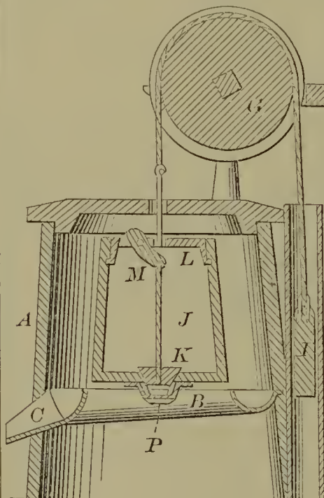
55025—J. W. Wheeler— Water Drawer.
