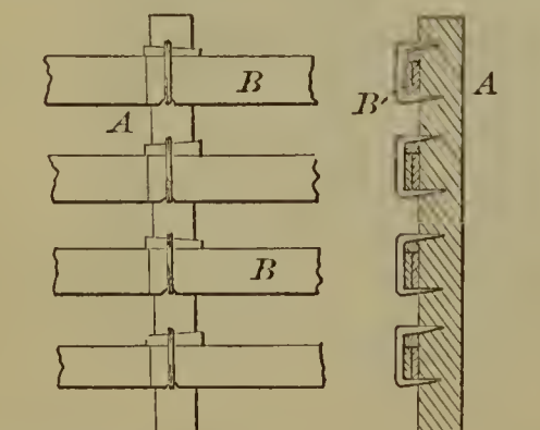
52981—J. Edmunds—Fence.
