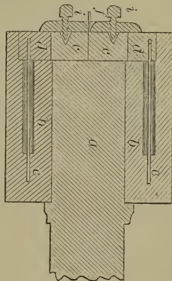
58730—E. J. Manville—Wire Pointing Machine.
