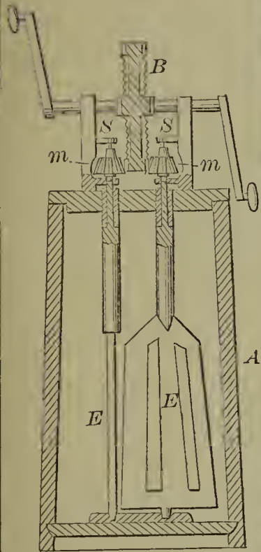
55407—H. Whisler—Churn.
