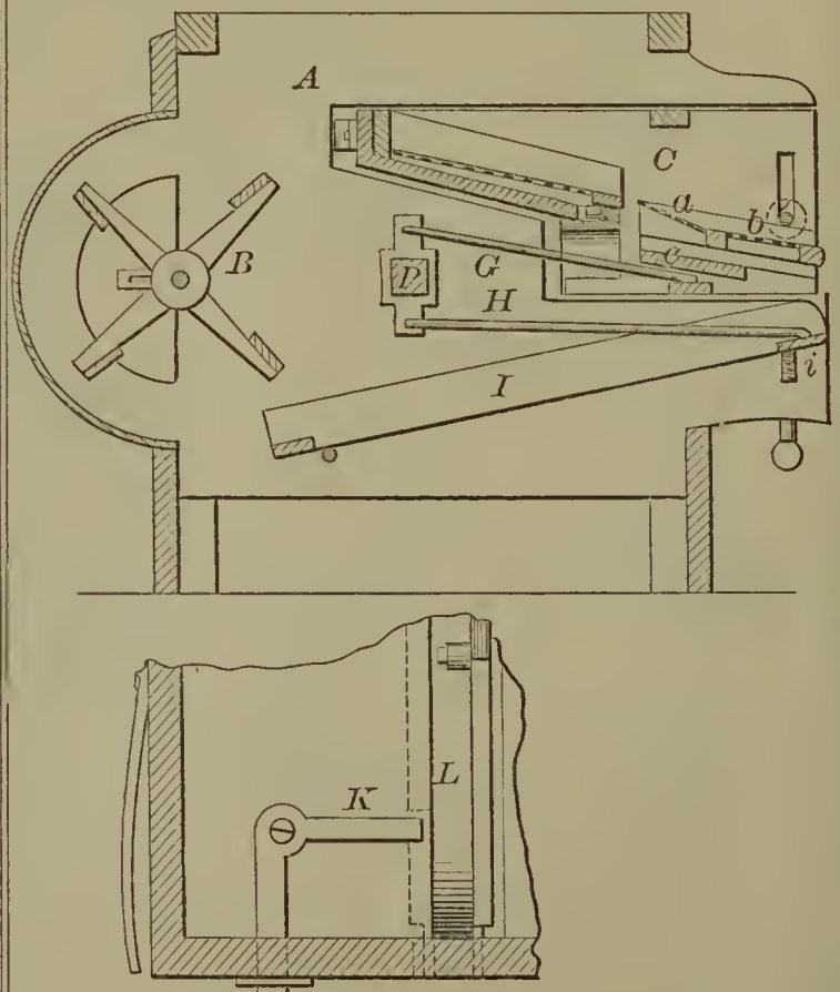
58707—Wirts & Swift— Grain Separator.
