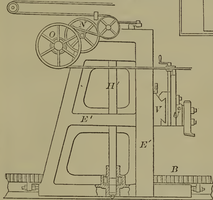
55723—W. Sellers— Planing Machine.
