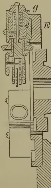
60067—D. T. Sanford— For Embossing Brass Tubes.
