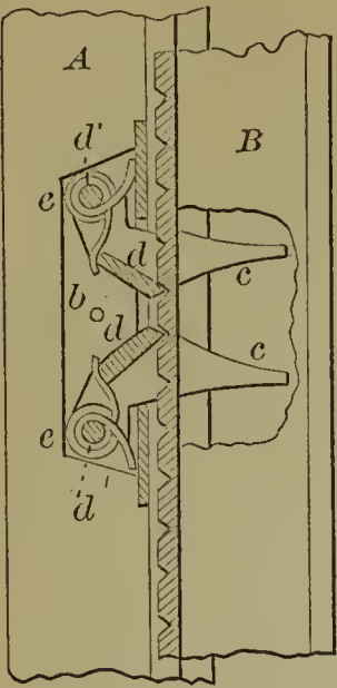
54953—D. A. Pratt— Sash Fastening.
