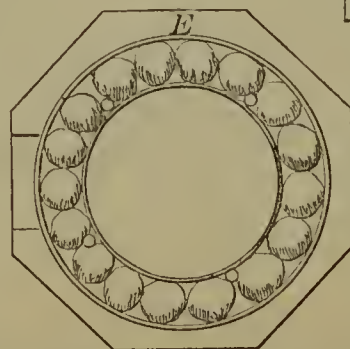
53475—T. W. Peirce— Beehive.
