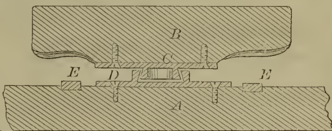
56207—X. W. Gordon—Coupling for Vehicles.
