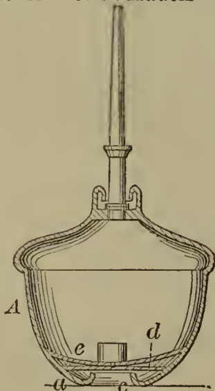
54540—C. J. Hauck— Oiler .
