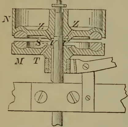
Friction Coupling.
