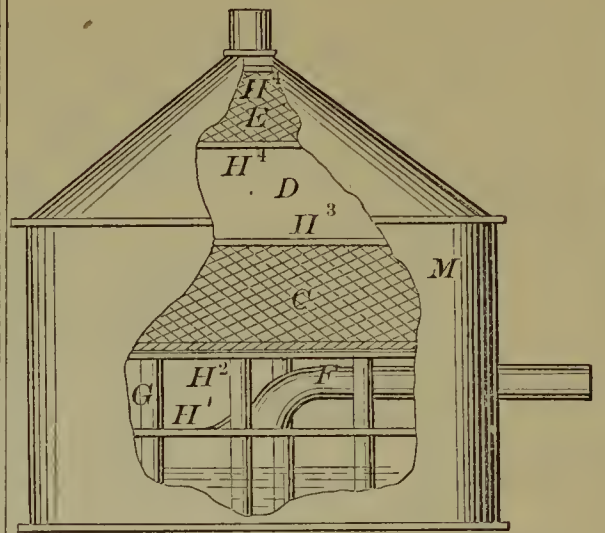
53980—Hotchkiss & Buss—Brick Machine.
