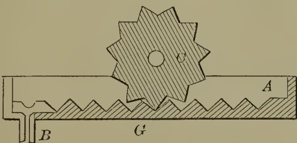
59985—R. R. Eastman—Butter Worker.
