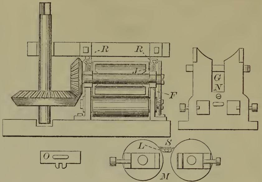
52207—T. L. Roberts—Mill for Grinding Sugar Cane.
