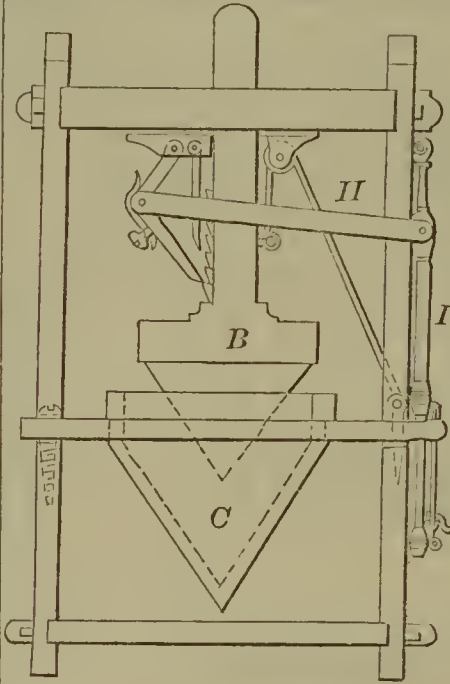
57277—C. Beach—Cider and Wine Press.
