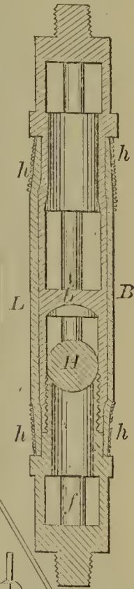
57840—R. N. Allen—Piston for Deep Well Pumps.
