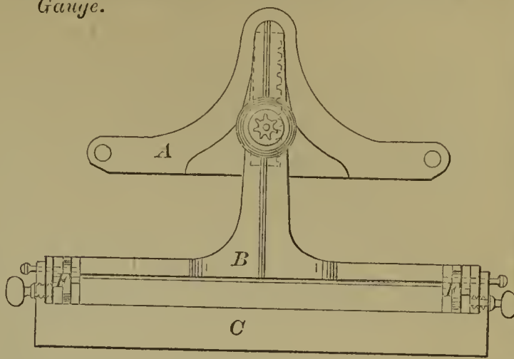
58498—Stanley & Goodrich— Angular Saw Gauge.
