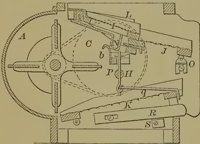
54895—P. Griswold— Grain Separator.
