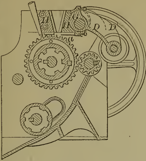
59676—C. W. Stafford—Ore Crusher.
