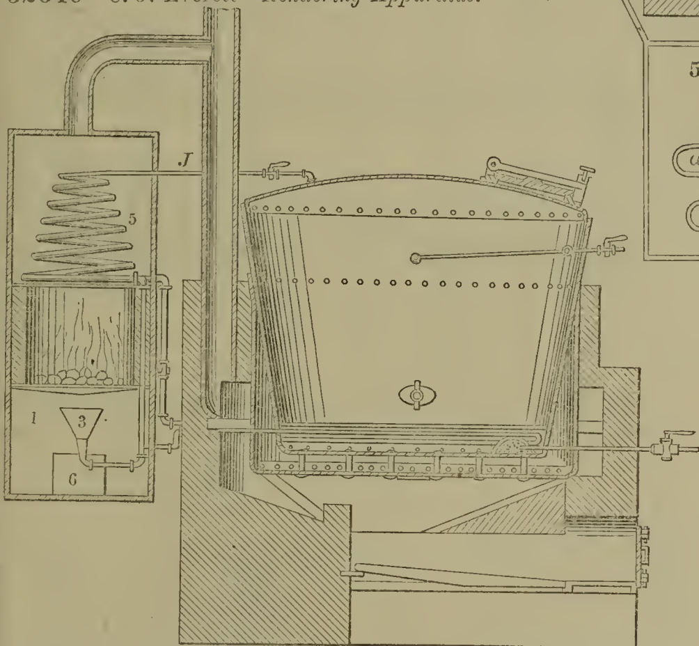
52640—C. J. Everett—Rendering Apparatus.
