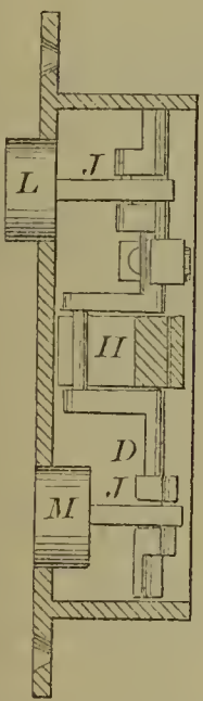
54348—J. M. Hopkins—Bolt Fastening.
