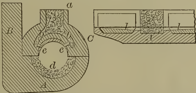
52723—H. Logan—Sluice for Quartz Mills.
