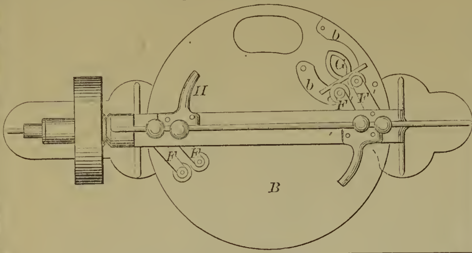
57634—Hill & Greene— Printing Press.
