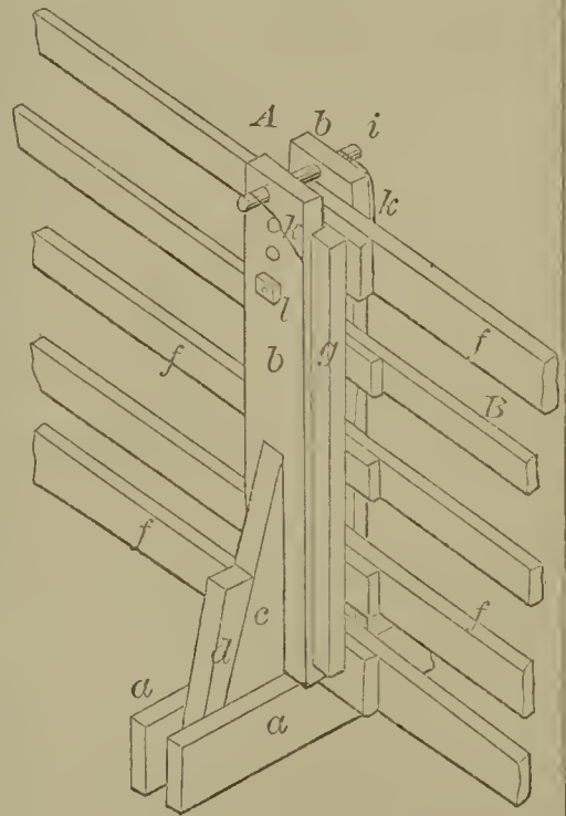
52611—S. Saunders—Fence.
