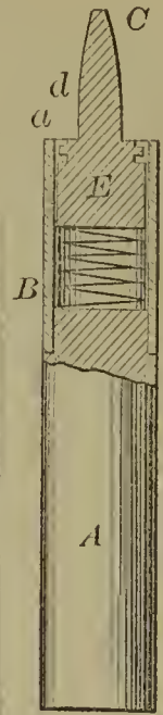
59483—D. Tuttle— Trace Lock.
