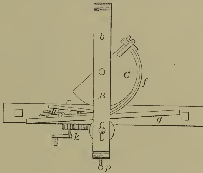
56788—J. Newman—Wood Bending Machine.
