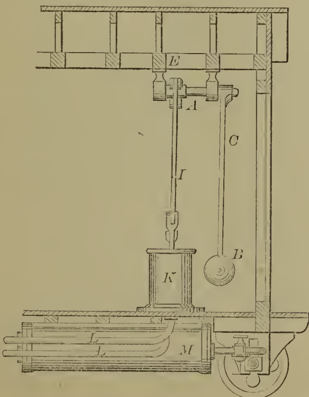
59226—E. S. Hutchinson—Automatic Blast for Carburettors in Railroad Cars, &c.
