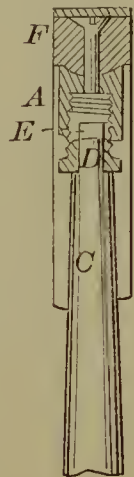
54155—G. G. Hickman—Carriage Wheel.
