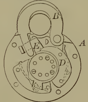
57539—W. McLean—Seal Lock.
