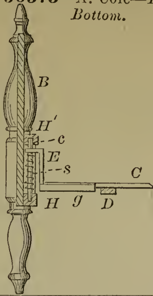
56374—E. G. Connelly—Churn Dasher.
