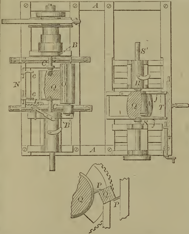
57145—H. Inman— Lathe for Turning Wagon Hubs.
