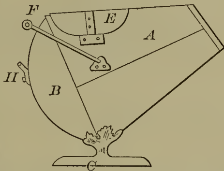
52861—H. B. Lansing— Corn Planter.
