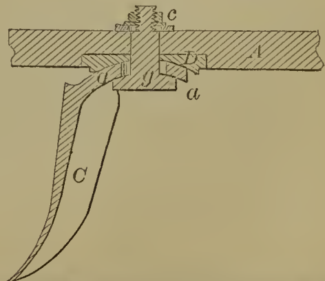
58533—G. W. Zeigler—Attaching Cultivator Teeth to Frames.
