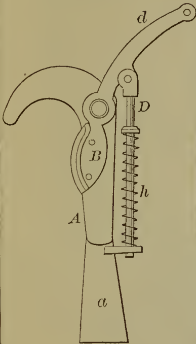
55043—A. Baumann— Pruning Shears.
