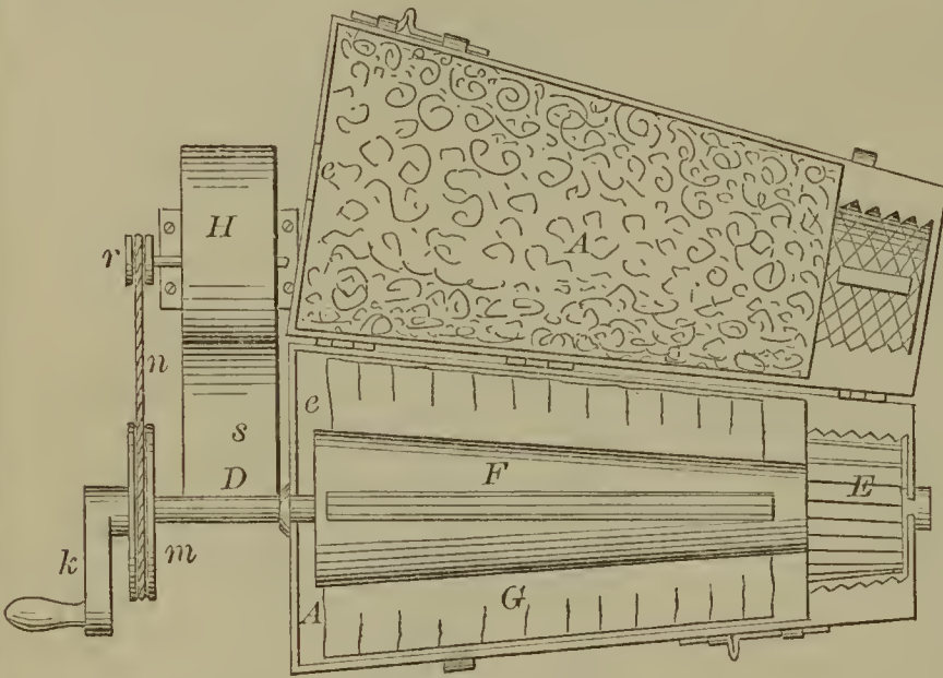
55947—R. Anderson—Coffee Hulling Machine.
