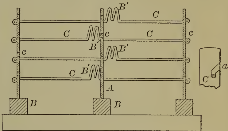
53418—E. Cozad—Fence.
