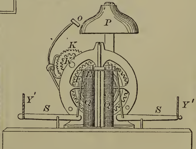
58662—E. Middleton—Fire and Burglar Alarm.
