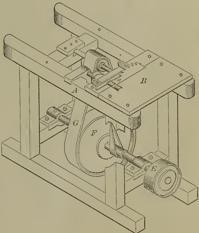
52188—J. Mutt— Feed Rollers to Circular Saws.
