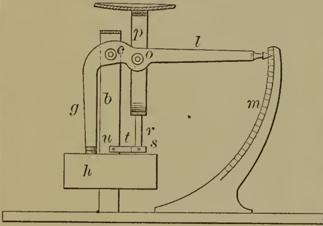
53050—L. Shepard—Scale for Weighing.
