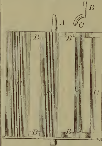
59493—W. G. Wilcox—Smut Machine.
