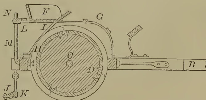
55826—J. Custer—Cultivator.
