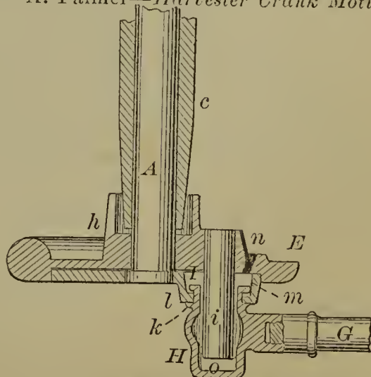
54397—A. Palmer— Harvester Crank Motion.
