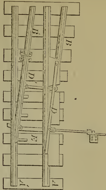
53674—P. Quinn—Railway Switch.
