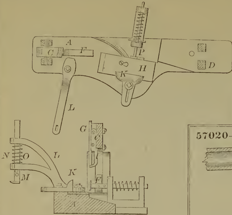
57018—O. Vanorman—For Tenoning Spokes.
