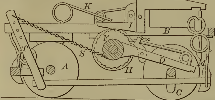
56030—N. B. Forrest— Car Brake.
