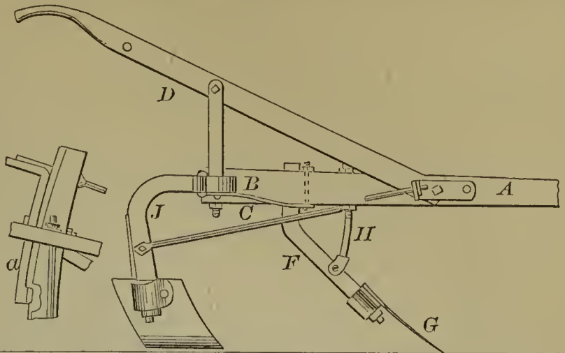
56289—D. C. Stover—Cultivator.
