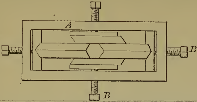
53781—O. C. Burdick—Die for Punching.
