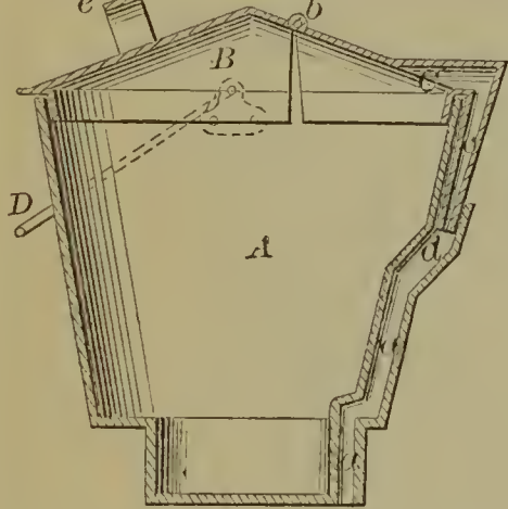
54964—S. E. Saul—Boiler for Culinary Purposes.
