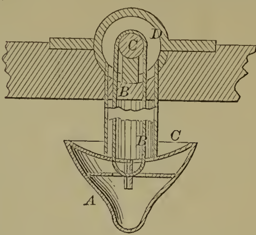
58408—D. Hagerty—Melting and Moulding Tinners' Solder.
