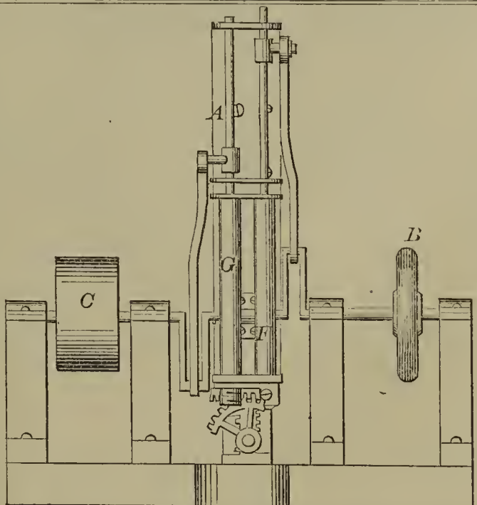
57512—H. Hubbell— Hydraulic Engine.
