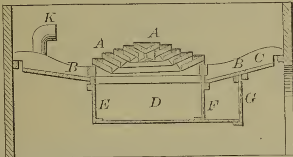
59334—J. F. Collins—For Distilling Petroleum, &c.
