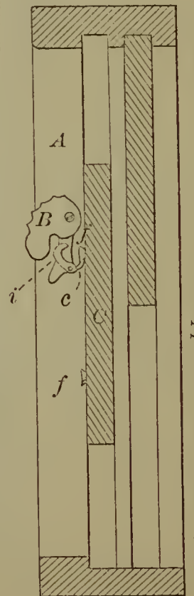
53907—I. H. Wait—Sash Supporter and Fastener.
