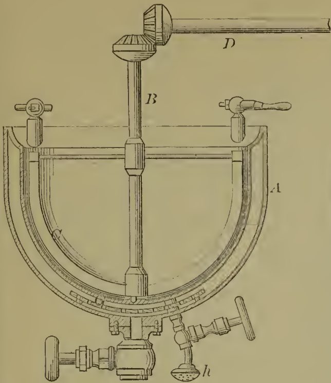
59350—W. Branagan—Lard Boiler.
