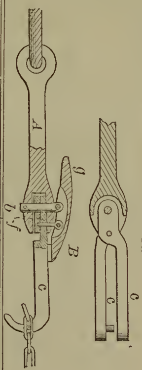
52392—E. Davidson— Cable Stopper.
