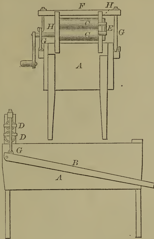
52423—J. Lee—Clothes Wringer.
