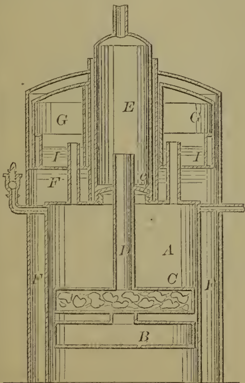
59473—L. Stevens—For Carburetting Air.
