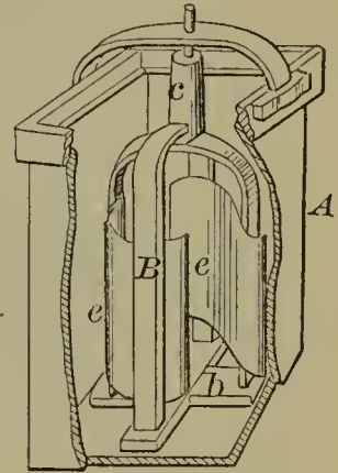
53591—D. Dunton—Churn.
