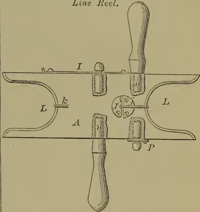
58378—H. W. Chamberlain—Cord and Line Reel.
