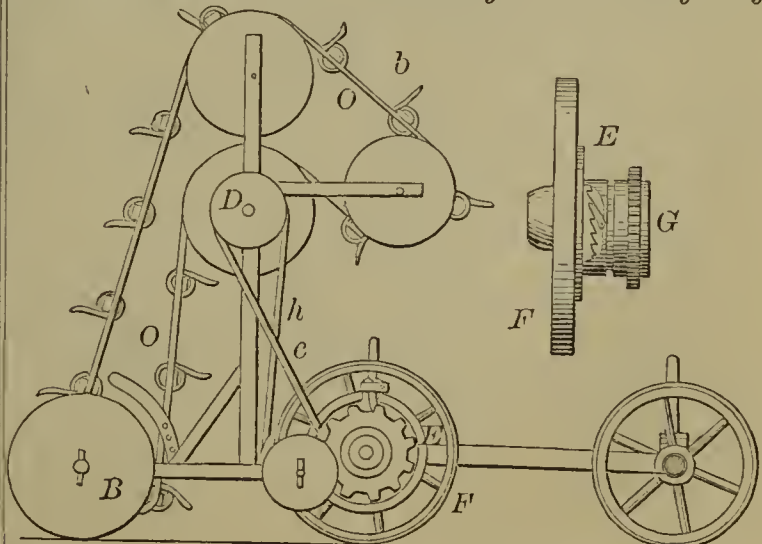
59105—M. Webb— For Raking and Loading Hay.
