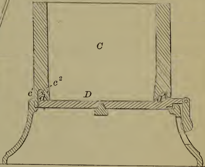
54725—C. Hires—Grate.
