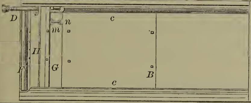
58837—H. Kewley—Stopwater for Oil Well Tubing.
