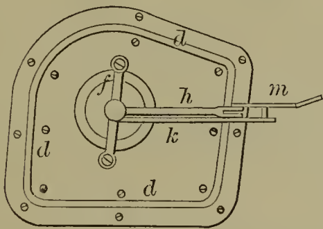
53954—J. Crimmmins— Stove Pipe Drum.
