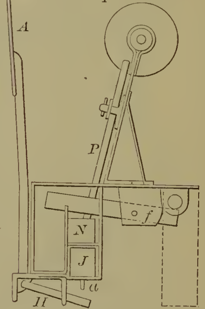
58226—L. Cutting—Spinning Machine Stop Motion.
