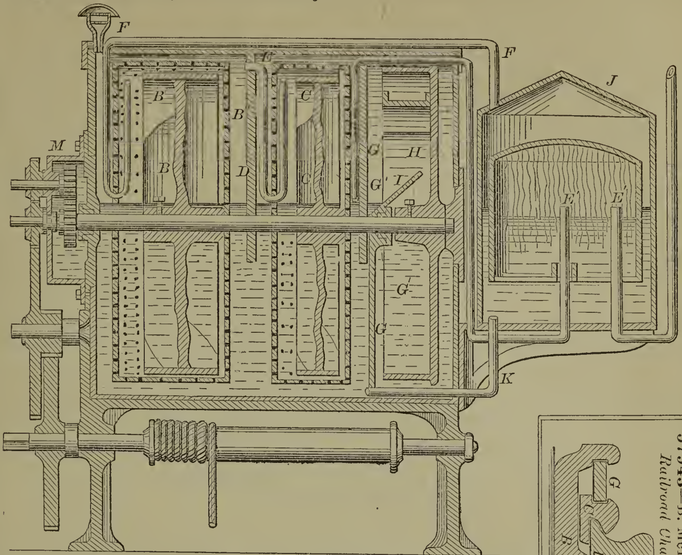
57942—W. R. McCutcheon— Churn.
