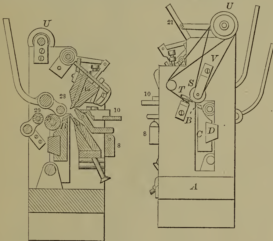
54043—A. H. Van Gieson—Leather Splitting Machine.
