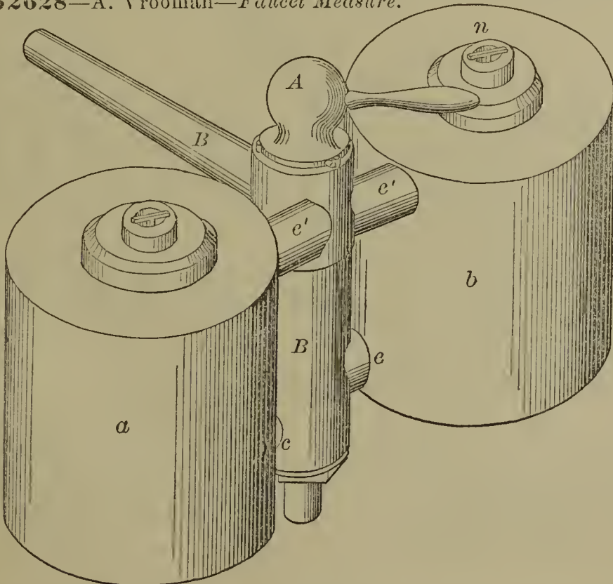
52628—A. Vrooman— Faucet Measure.
