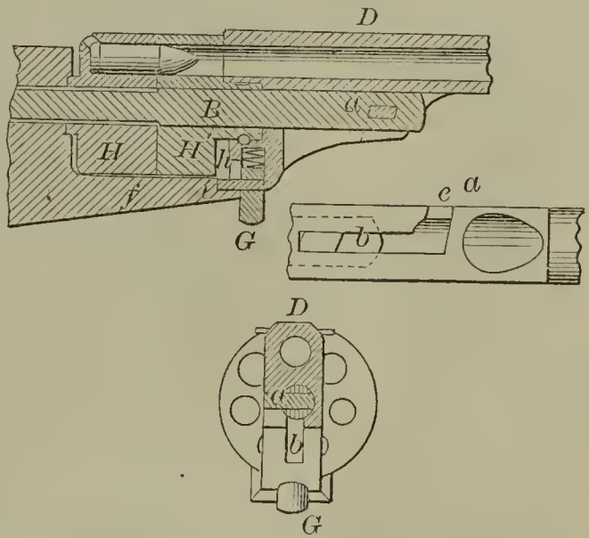
51836—B. F. Joslyn—Revolving Fire Arm.
