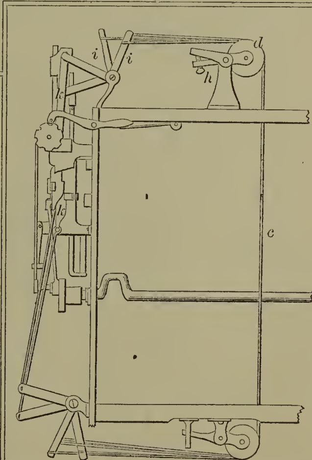
59972—G. Crompton—Harness Motion for Looms.
