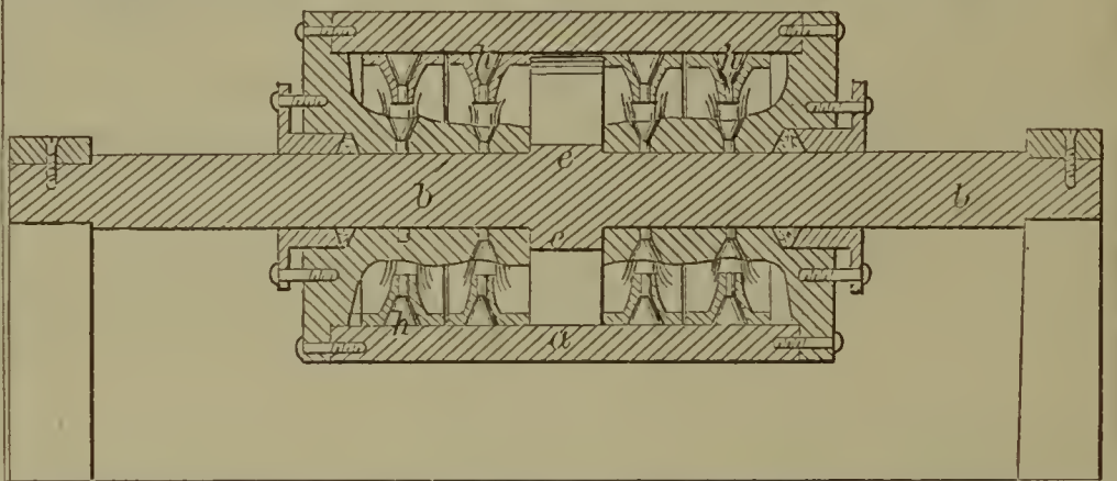
60444—O. Tufts—For Oiling Bodies Rotating around Shafts.
