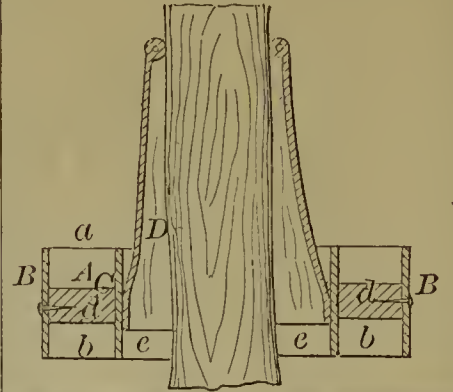
54144—A. Hamar— Boring Artesian Wells.
