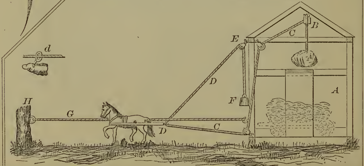
52808—H. Maycock—Operating Horse Hay Forks.
