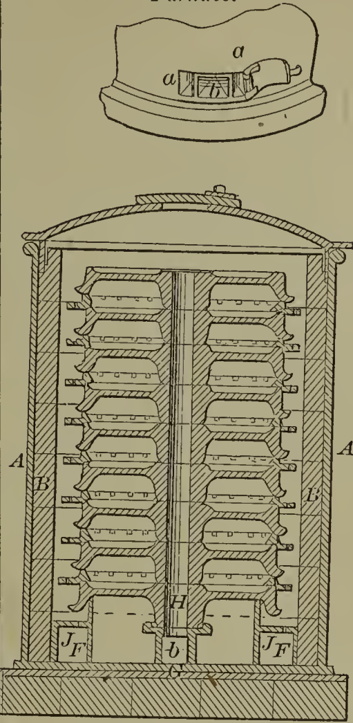
58666—H. W. Moore—Annealing Furnace.
