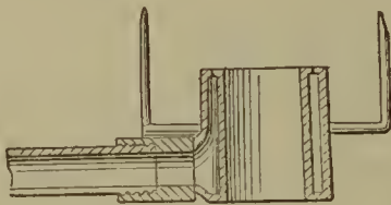
58769—J. H. Bruen— For Sinking and Tubing Wells.
