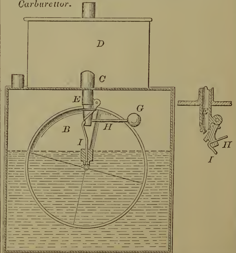
58422—E. S. Hutchinson—Automatic Feed for Carburettor.
