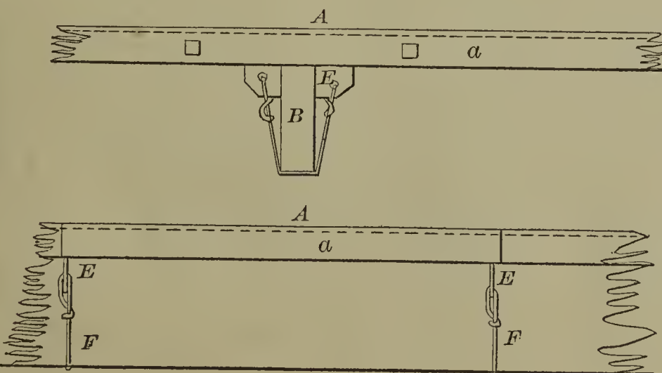
57997—G. Taylor—Malt Kiln Floor
