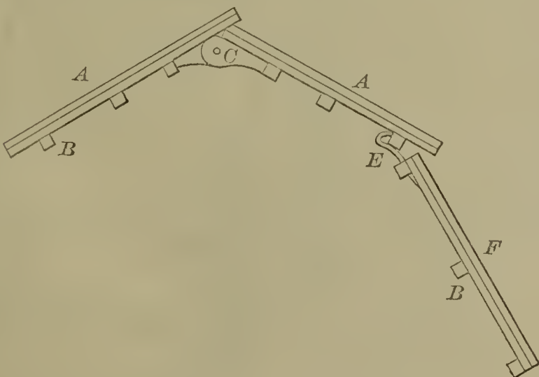
52613—M. Simmons—Roof.
