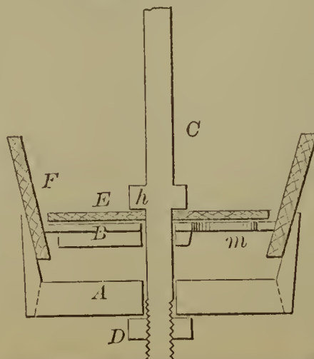
57760—B., E. & B. Pickering— Pump Piston.
