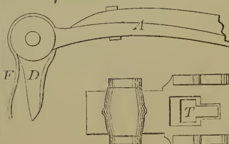
59455—Rood & Hackett—Thill Coupling.
