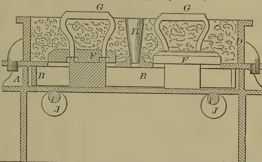
55504—P. W. Lamb— For Moulding Castings.
