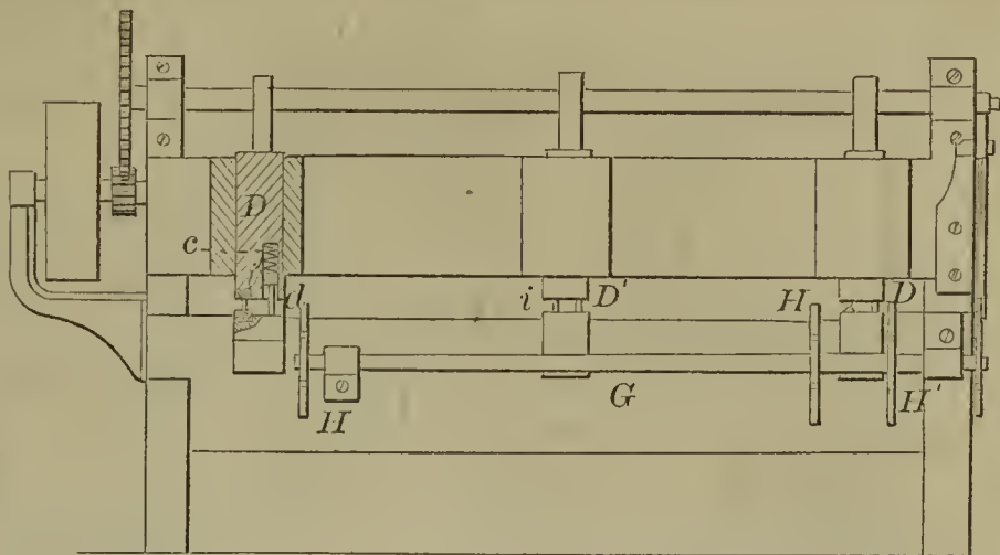
57251—J. Fox— For Flattening and Punching Umbrella Ribs.
