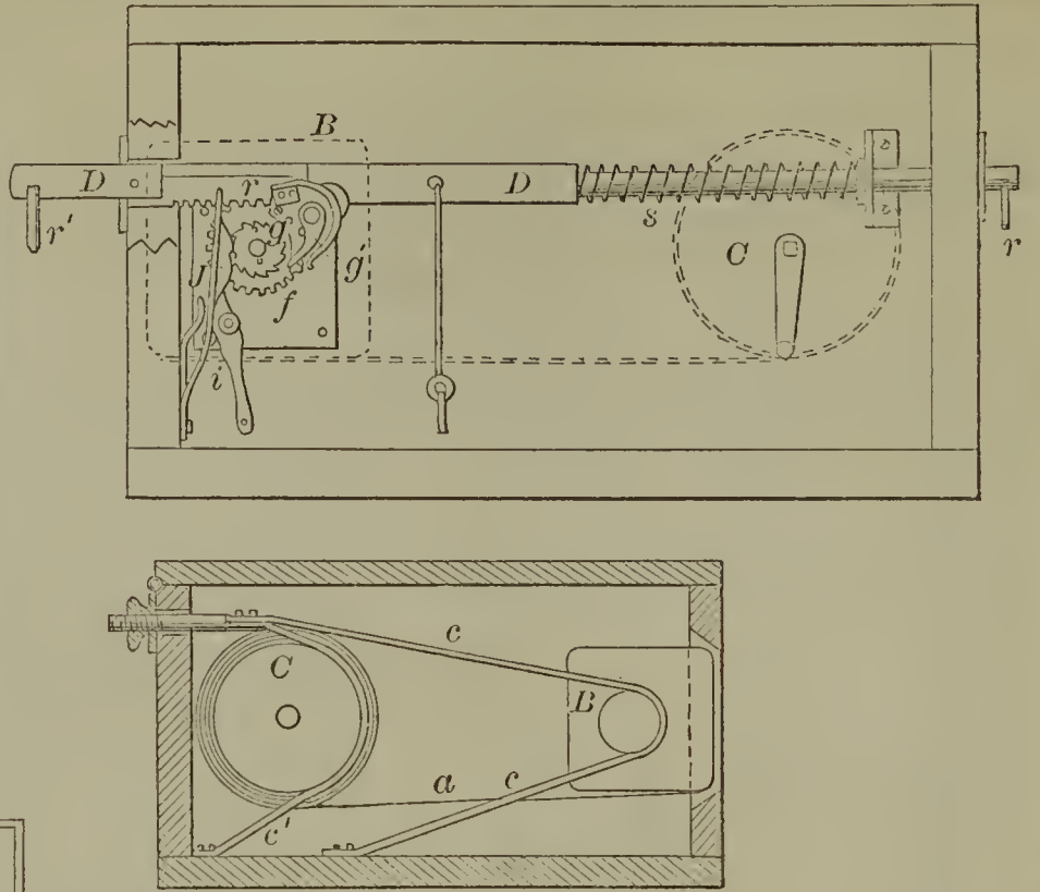
51927—A. S. Cox— Railroad Station Indicator.
