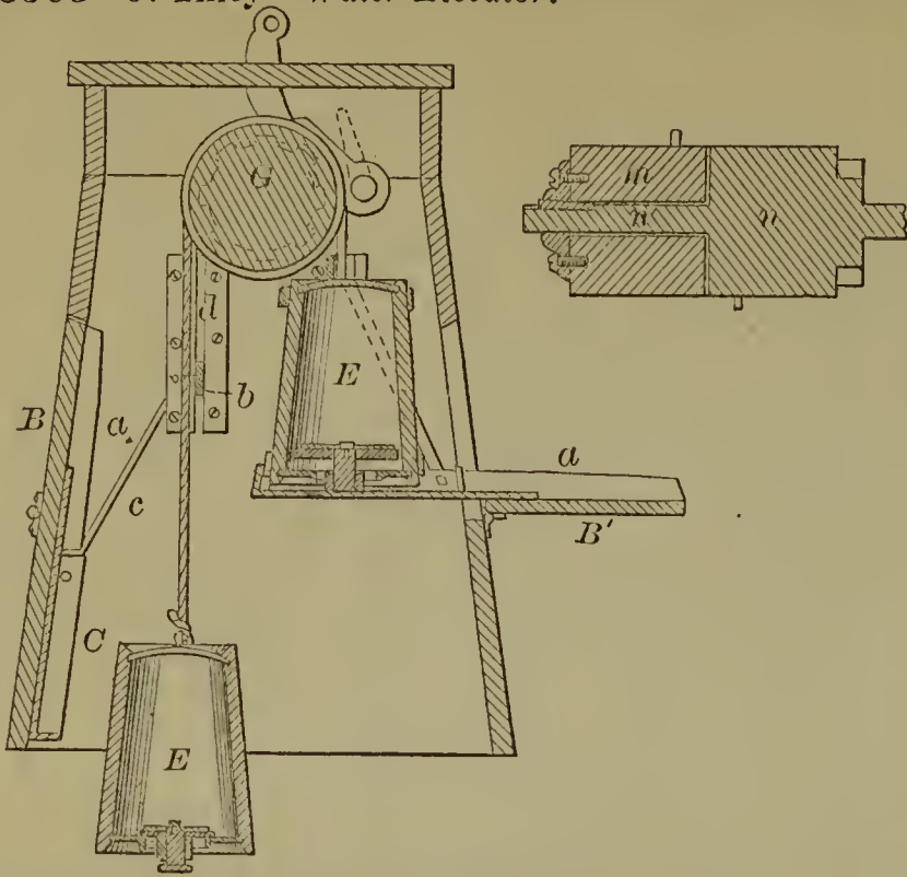
53505—J. Tilley—Water Elevator.
