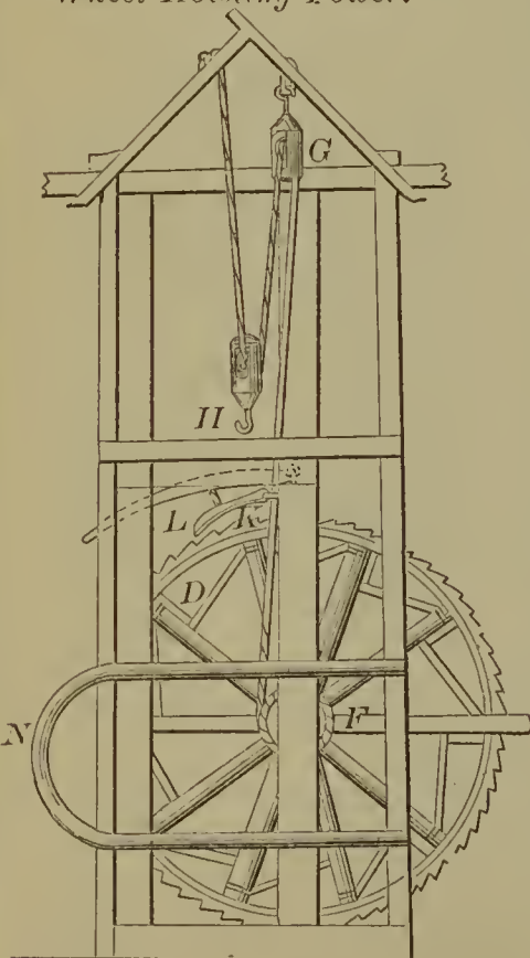
59818—J. B. Cassel—Tread Wheel Hoisting Power.
