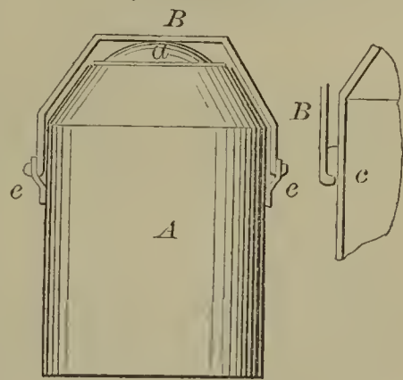
55953—G. H. Hammer— Fastening for Fruit Cans.
