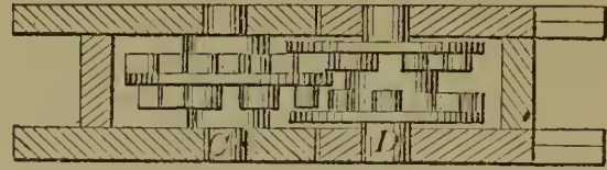
54590—C. C. Parsons—Cast Iron Apparatus for Superheating Steam.
