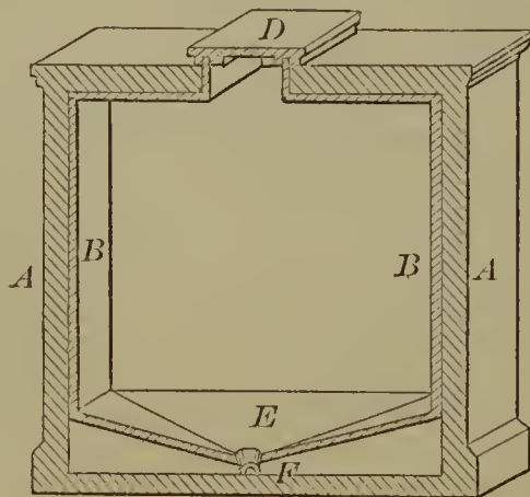
54657—E. L. Allen—Vessel for Petroleum, &c.
