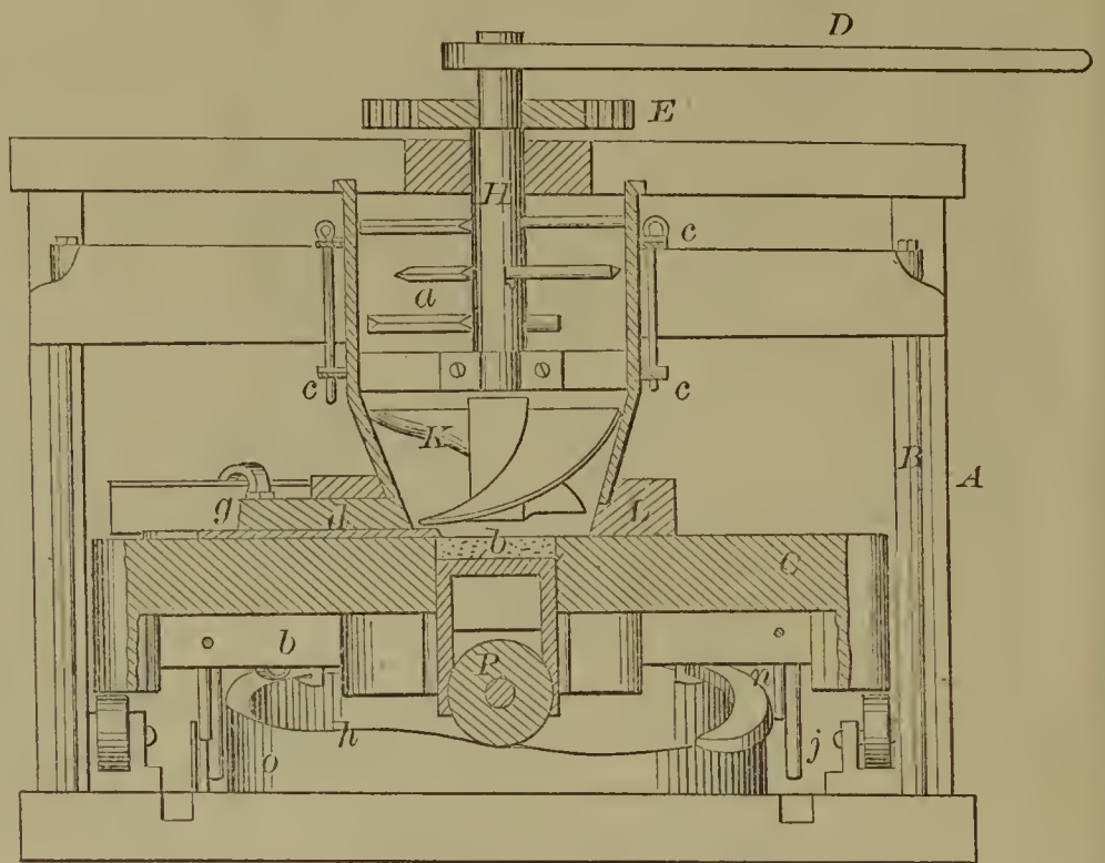
55276—W. M. Garrison— Cracker Machine.
