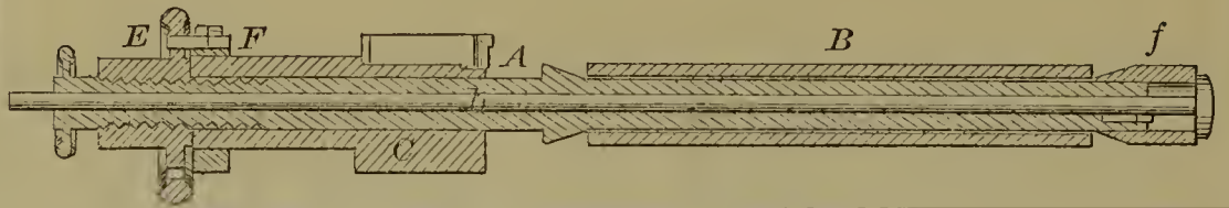
53328—L. M. Patterson—Gang Plow.
