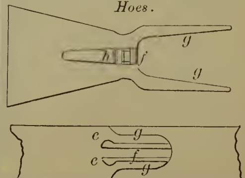
59744—R. Harper—Manufacture of Hoes.
