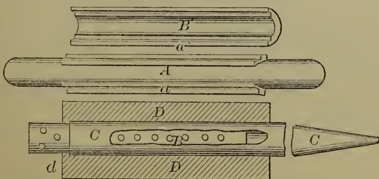
54651—H. Robbins— Roll for Wringers.
