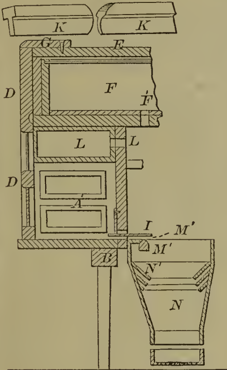
56551—G. Graffham— Beehive.
