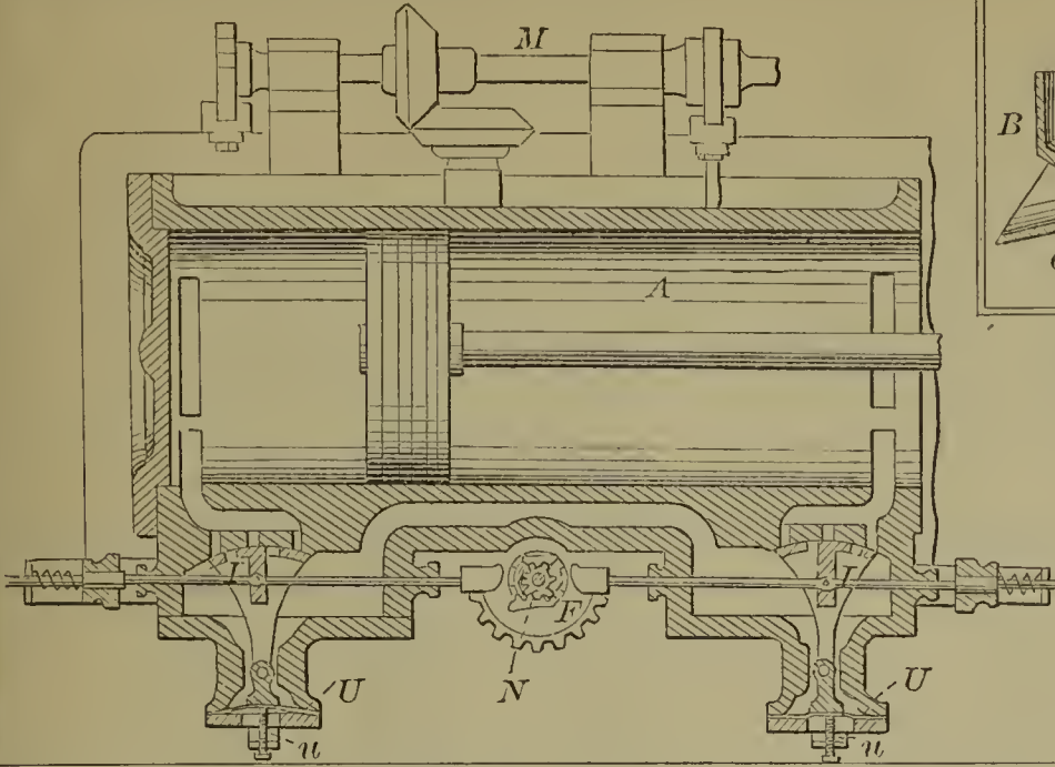
59887—W. Wright—Variable Cut-off Valve Gear.
