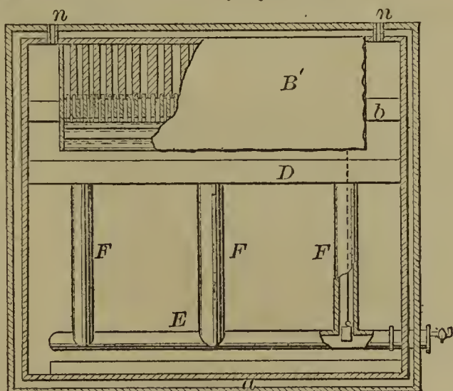
56094—Rees & Tevis—Refrigerator.
