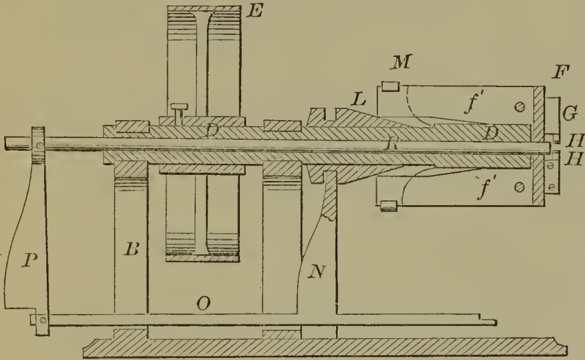
55171—A. B. Simonds—Screw Cutting Machine.
