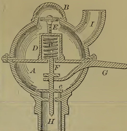
56409—E. Hamilton—Safety Valve.
