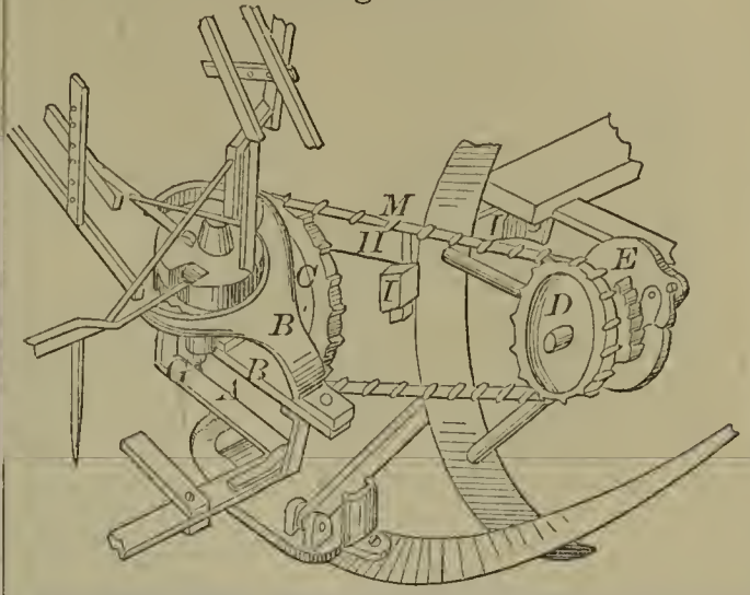
55837—J. A. Dodge— Harvester.
