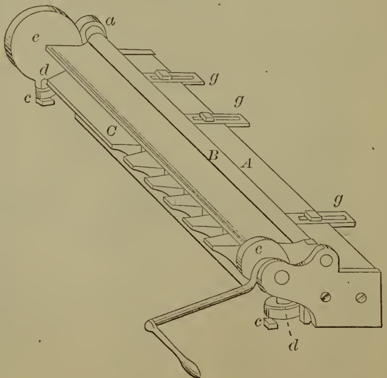
54342—W. H. Henderson— Tinman's Edging Tool.
