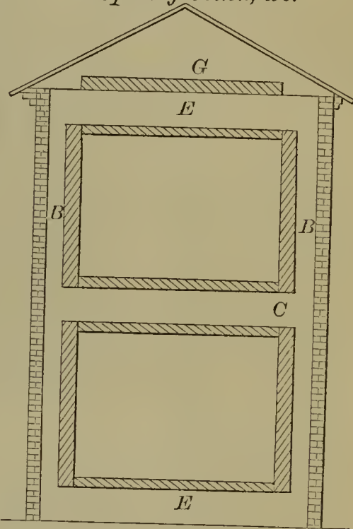
55118—R. Kitson—Picker House for Opening Cotton, &c.
