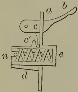
51983—G. W. Wareham—Sash Fastener.
