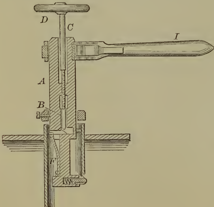
55391—N. Thomas— For Cutting Off Boiler Tubes.
