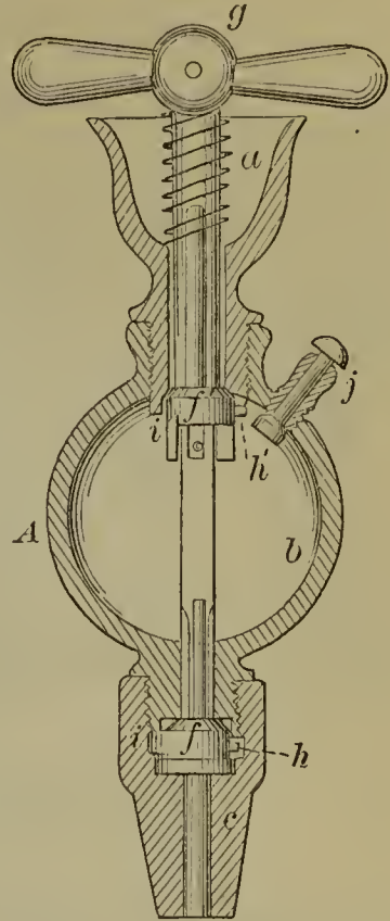
53973—G. Hagenmeyer—Grease Cup.
