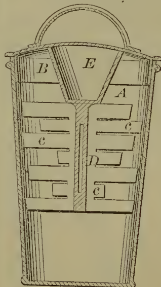
53429—H. D. & J. H. Felthouse—Egg Beater.
