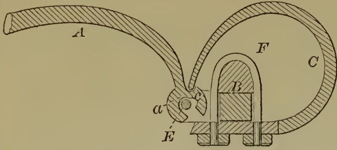
53828—W. R. S. Hunter—Attaching Thills to Carriages.
