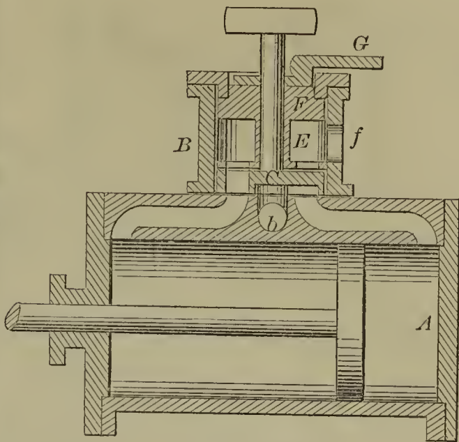
55518—B. F. McKinley— Balanced Cut-off Valve.
