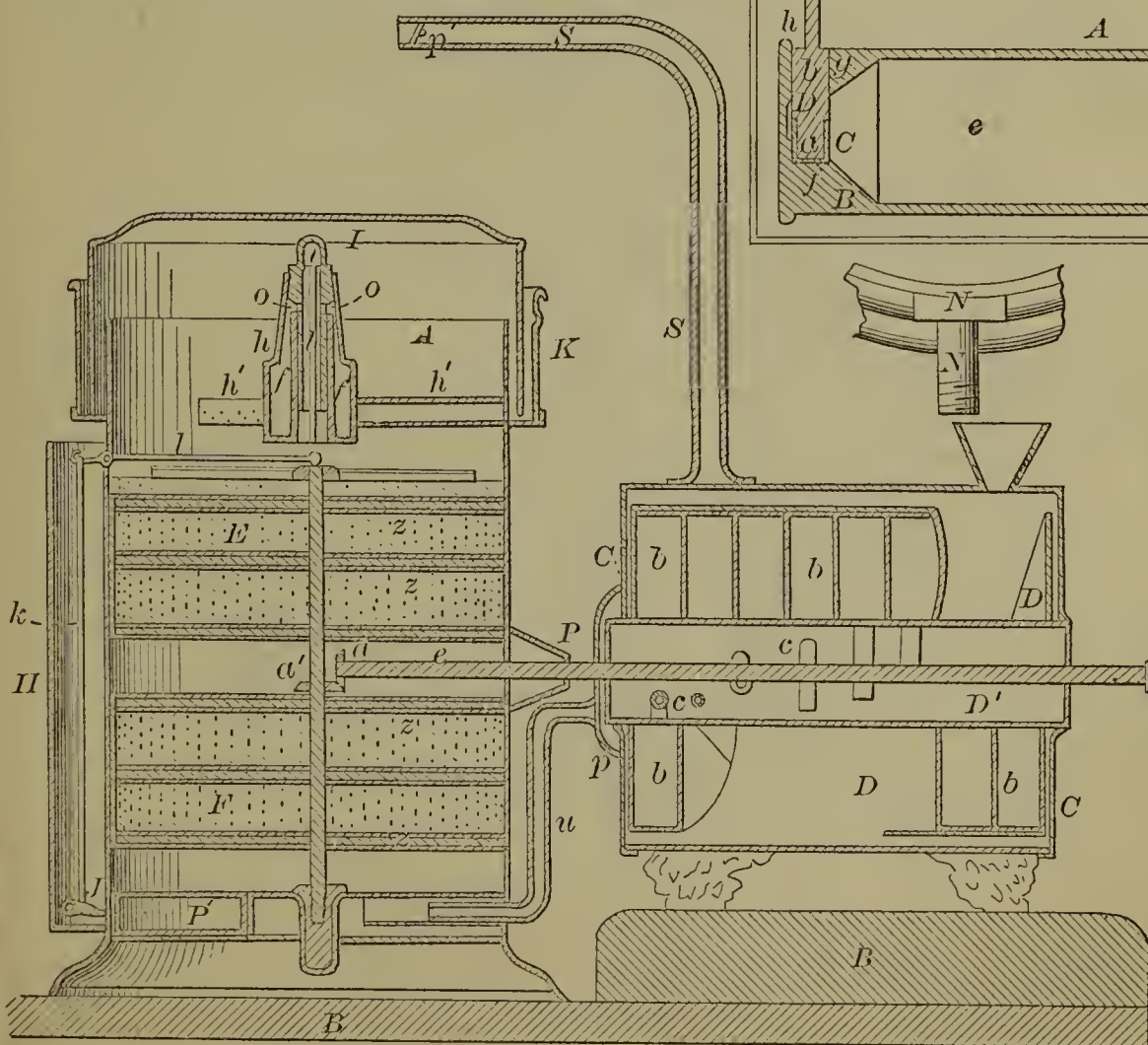
53504—W. Thompson— For Carburetting Air.
