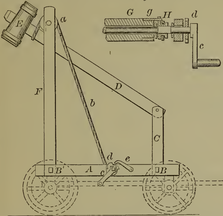
52814—W. W. Barnes—Machine for Raking and Loading Hay.
