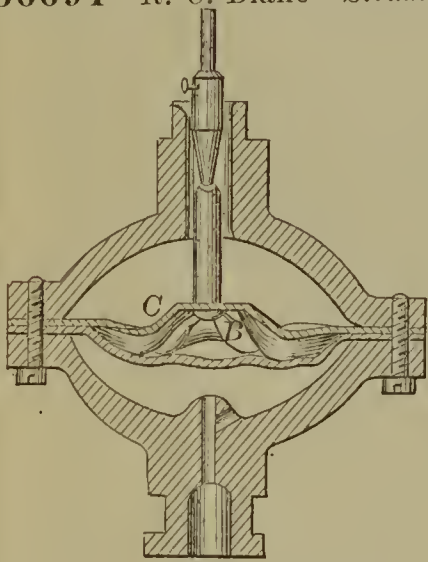
56694—R. C. Blake—Steam Gauge.
