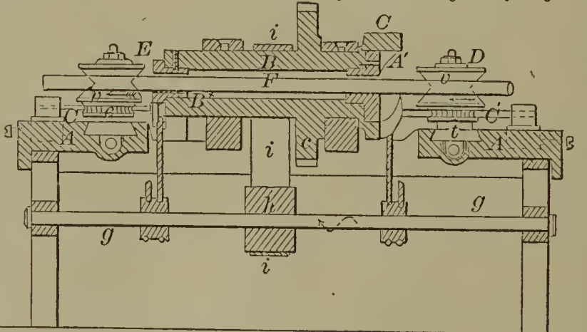
58605—J. J. Conley—Lathe for Turning Shafting.
