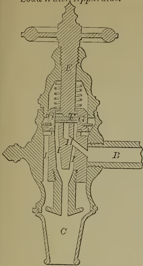
56709—W. P. Clark—Cock for Soda Water Apparatus.
