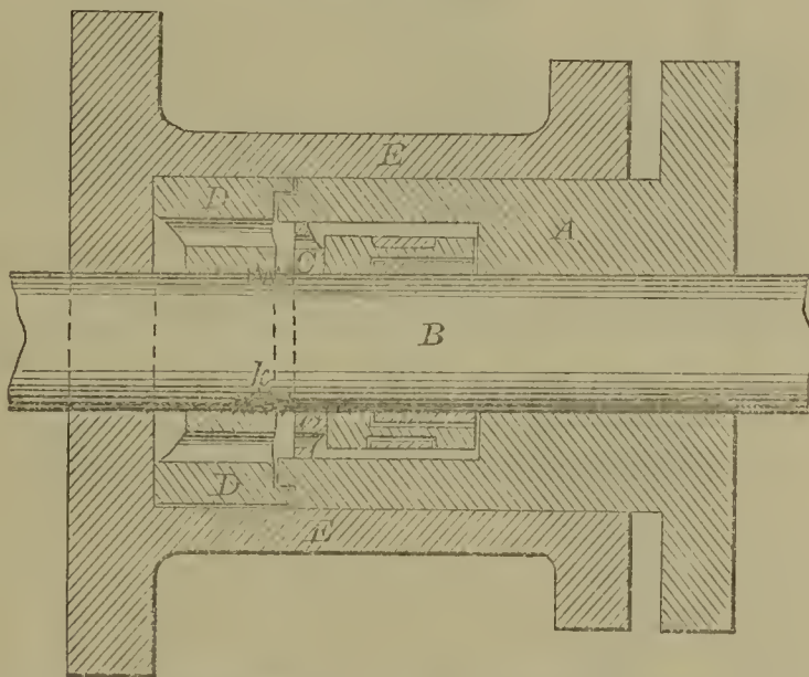
52575—C. F. Jauriet— Metallic Packing for Stuffing Boxes.
