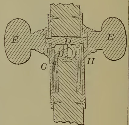
56808—G. A. Sherlock—Lock.
