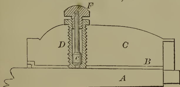
60049—G. W. Parsons—For Lubricating Axle Journals, &c.
