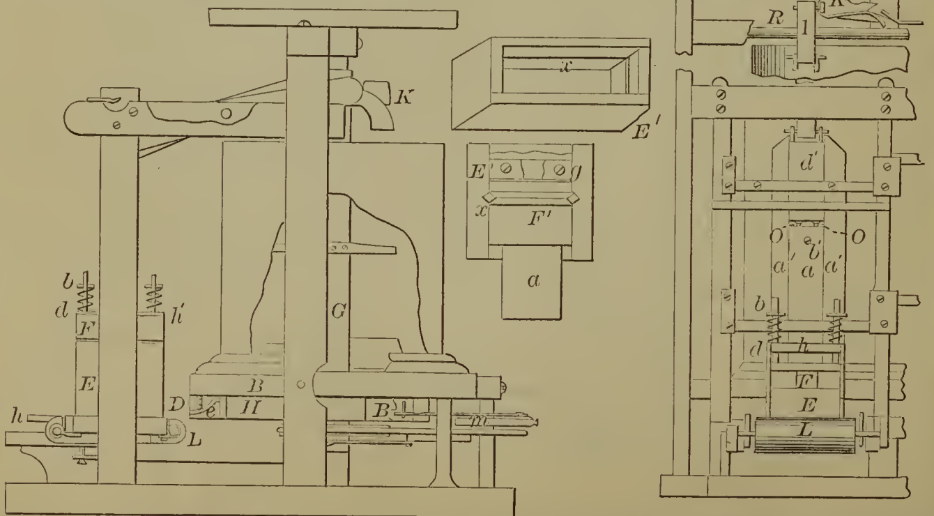
56847—Capron & Winchell—Brick Machine.
