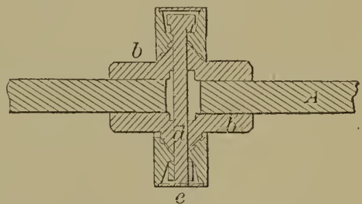
58330--J. L. Winslow--Shaft Coupling.
