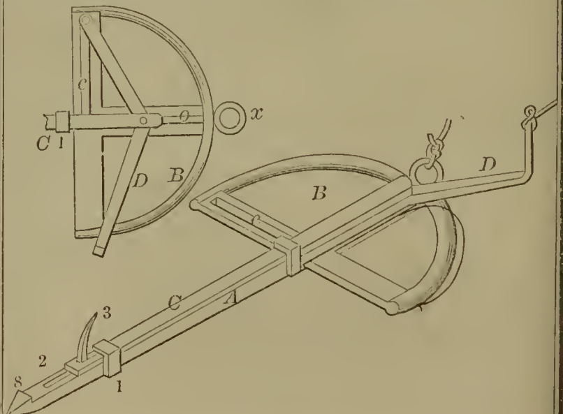
55278—E. Gilliam— Horse Hay Fork.
