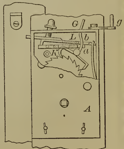
53239—W. H. Winans— Burglar Alarm for Windows.
