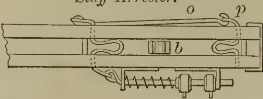
52367—E. & H. C. Phillips—Picker Staff Arrester.
