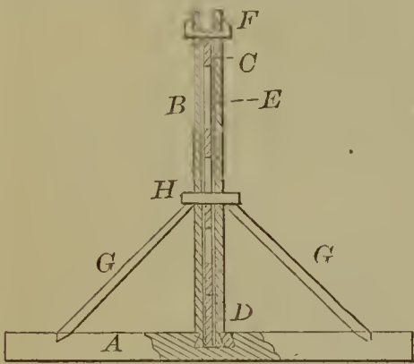
56826—Stone & Blocker—Fence.
