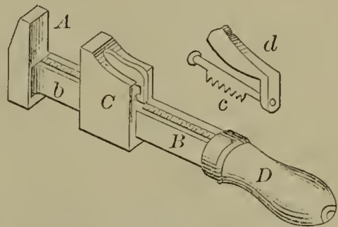
57547—I. & C. M. Morris— Wrench.
