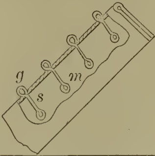
55853—C. Goodyear, Jr.— Lacing for Boots and Shoes.
