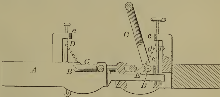
59860—H. L. Ogden—Car Coupling.
