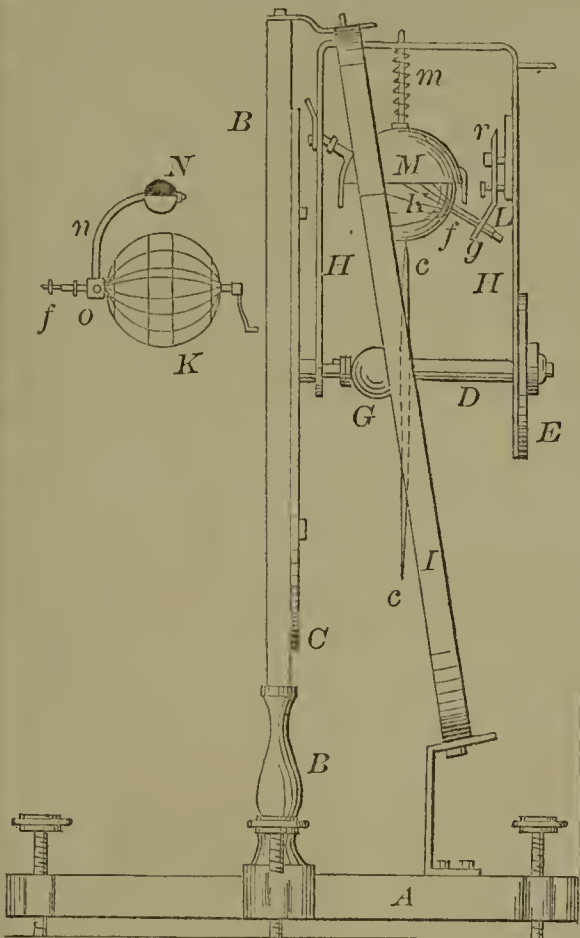
60642—E. Root—Terrasphere.
