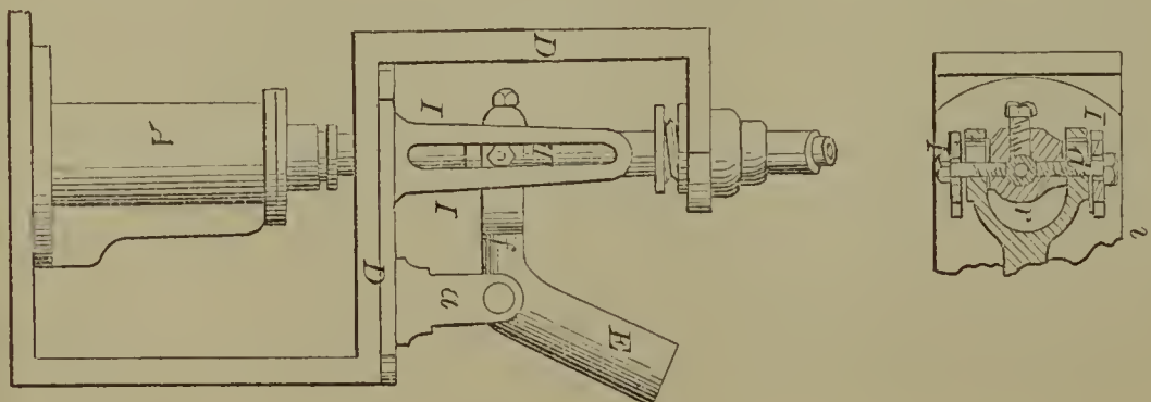
58918—I. Van Olinda—Communicating Reciprocating Motion to Pumps, &c.
