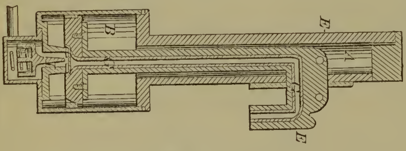
59673—A. J. Smith—Bolt Cutter.
