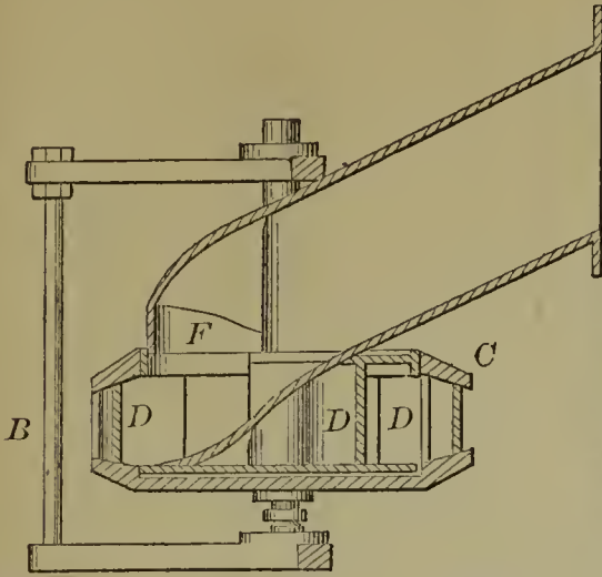
54942—A. Peckham— Cotton Seed Planter.
