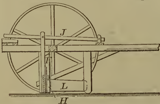
56285—M. Smith— Street Scraper.
