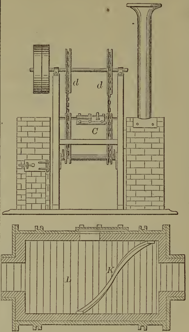
60134—W. Brückner—Furnace for Desulfurizing Ores.
