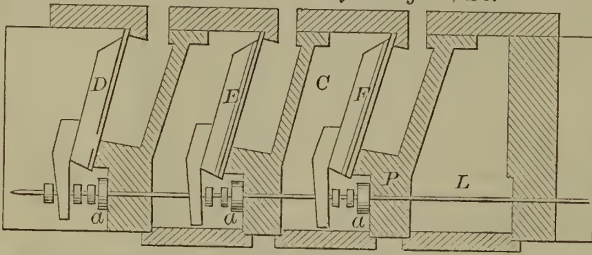
55575—F. Brown—Oscillating Engine.
