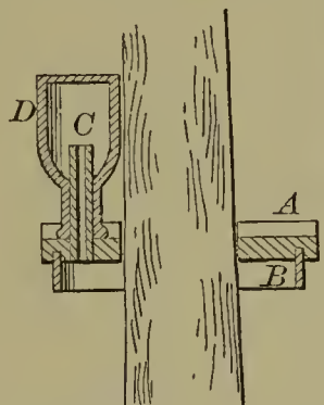
53776—T. F. Boyer— Clamp for Brooms.
