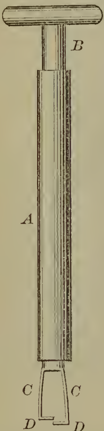
52267—M. C. Chamberlin— Earth Borer.
