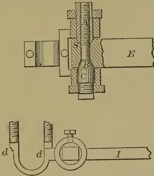
54840—C. H. Bassett—Coupling for Carriage Thills.
