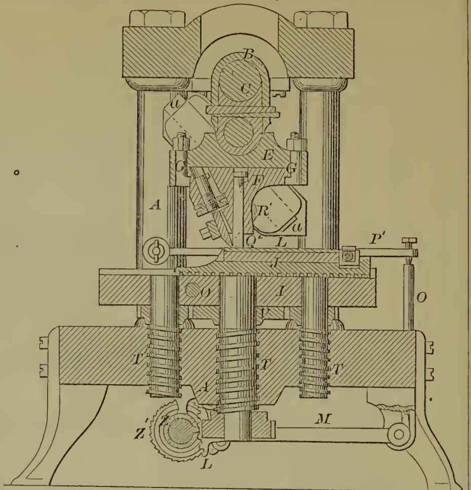
52804—J. C. Cooke—File Cutting Machine.
