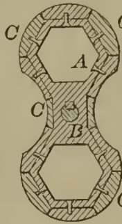
Crosshead for Blowers.
