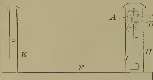
55878—O. J. Livermore—Can Opener.
