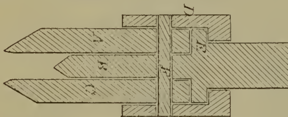
53586—J. C. Dickey— Rock Drill.
