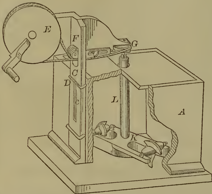
56117—I. H. Stoddard— Ship's Table.
