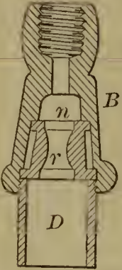
56448—T. L. Reed—Coupling for Gas Fixtures.
