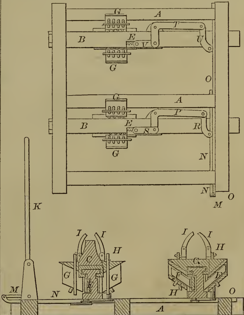
56145—C. Leffingwell—Head Block for Saw Mills.
