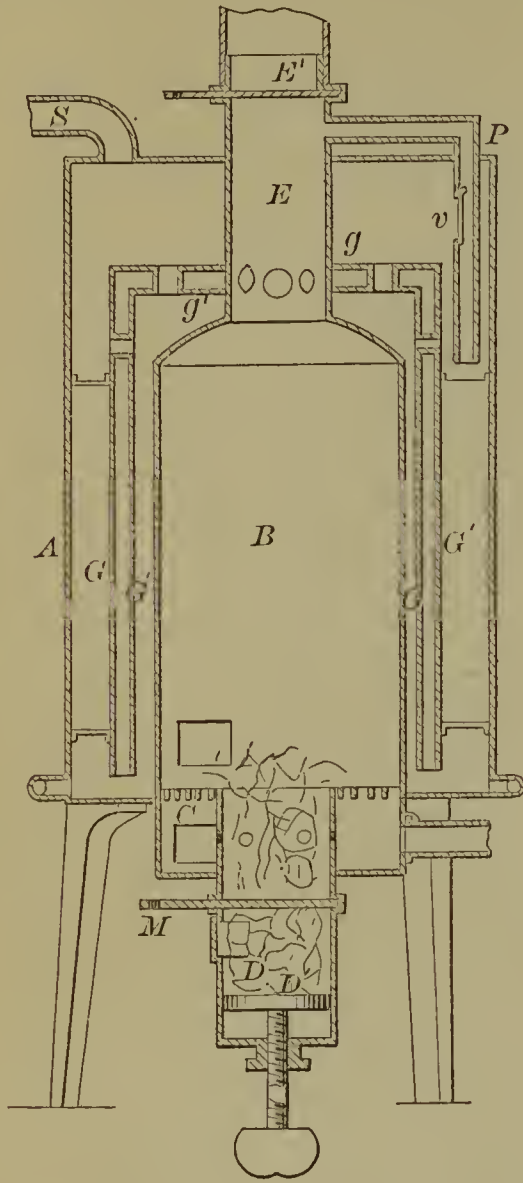
54730—D. C. Howell—Steam Generator.
