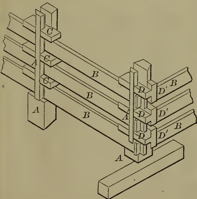
60576—W. B. Shelton— Fence.
