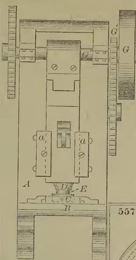
55790—J. H. Tobey—Swaging Machine.
