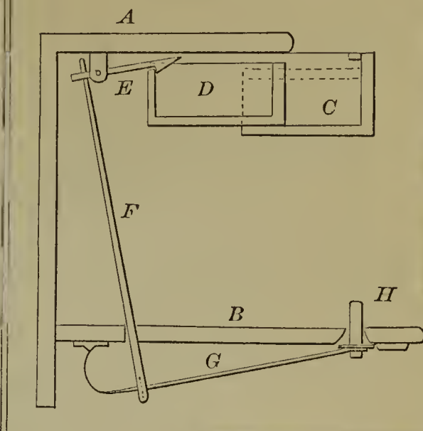
53827—S. Hubbell, Jr.— Catch for Money Drawers.
