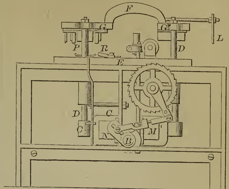
56325—R. Parks—Envelope Machine.
