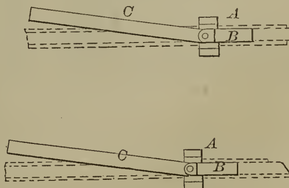
55943—J. A. Williamson—Railroad Switch.
