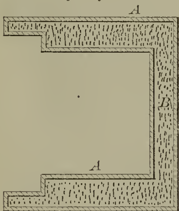
51937—S. T. Fowler—Fire Proof Safe.
