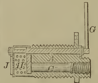
57216—T. Ferrel— Plow Cleaning Attachment.
