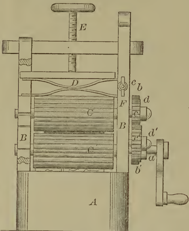
52441—W. H. Nichols—Washing Machine and Wringer.
