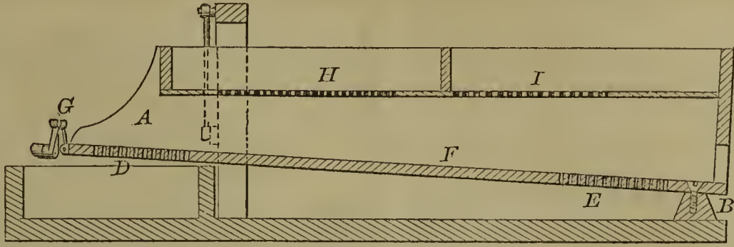
56140—W. Blessing—Preparing Cotton Seed for Planting.
