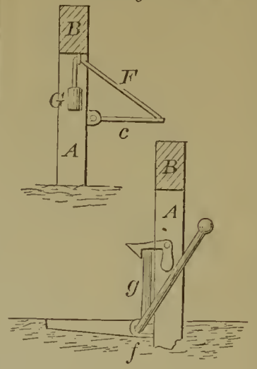
57715—A Hill—Railway Crossing Guard.
