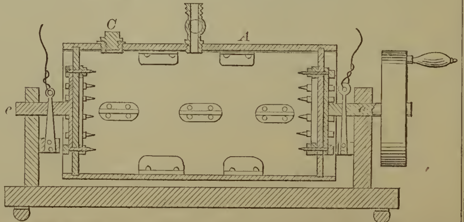
57009—W. M. Storm—For Ripening Liquors.
