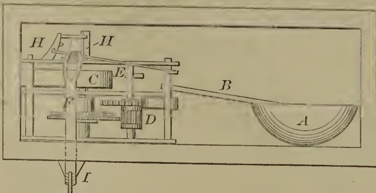
55754—H. Wickham, Jr.—Burglar Alarm.
