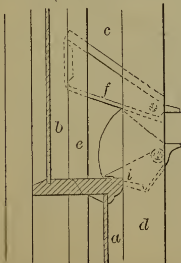
55057—E. A. Campbell— Sash Supporter.
