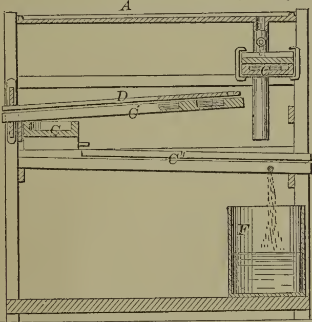
57898—G. Hasecoeter—Loom for Weaving Slatted Window Shades.
