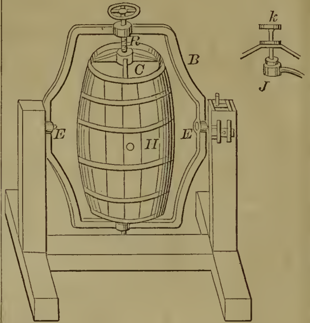
56483—J. O. Woodruff—Applying Liquids to Casks.
