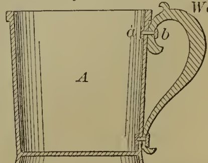
54620—Smith & Pomeroy— Fastening Handles to Plated Ware.
