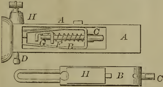
57385—J. B. Rumsey—Car Coupling.
