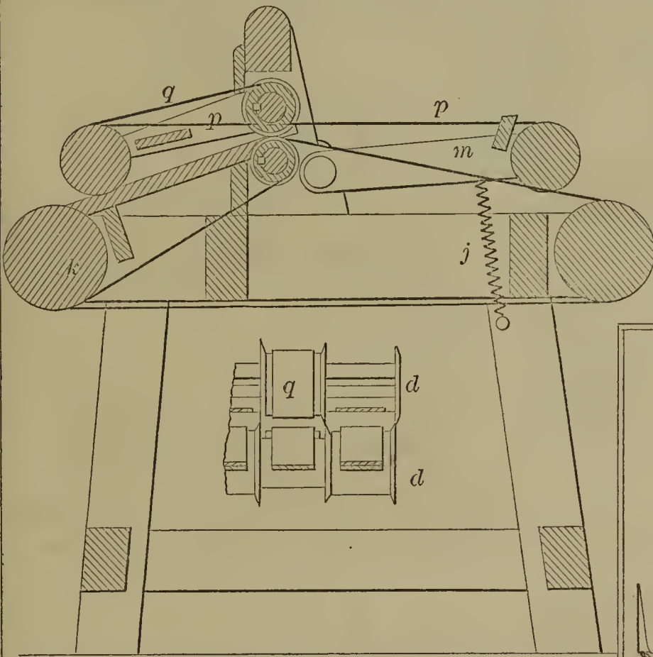
55335—Merriam & Norton—Glueing and Cementing Machine.
