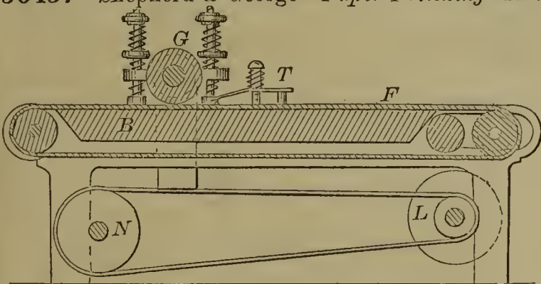
56457—Shepherd & George—Paper Polishing Machine.
