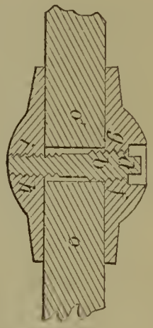
54212—S. P. Ruggles— Shaft Coupling.
