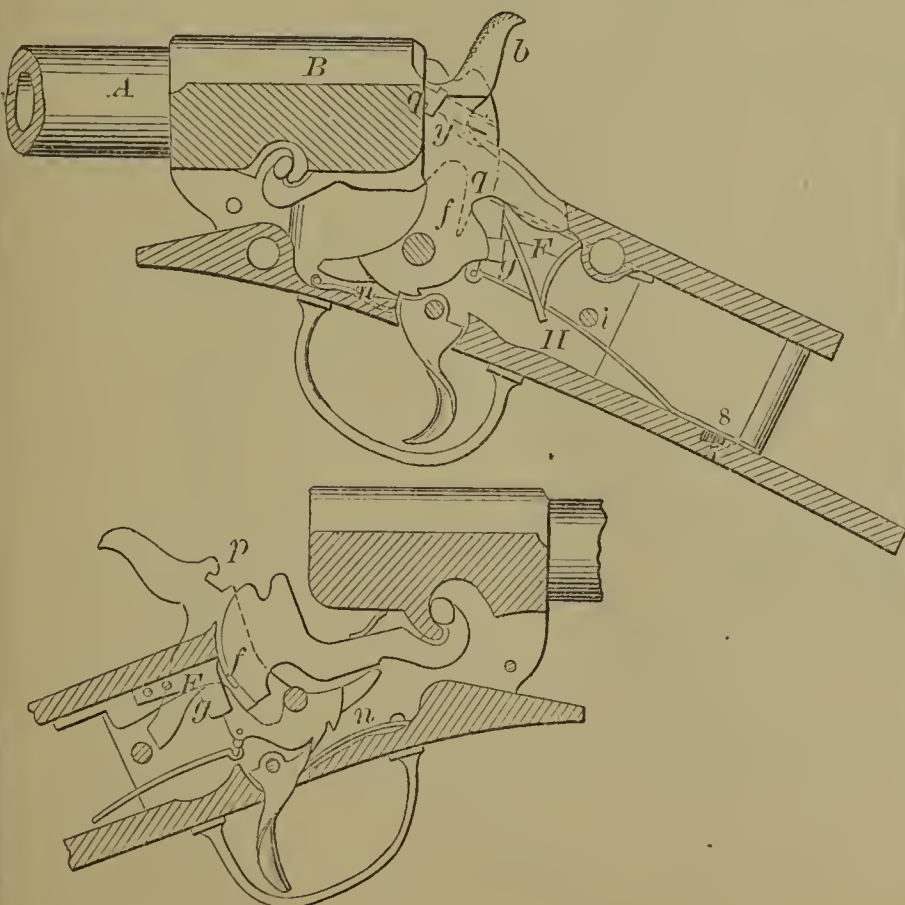
58444—R. McChesney— Breech-Loading Fire Arm.
