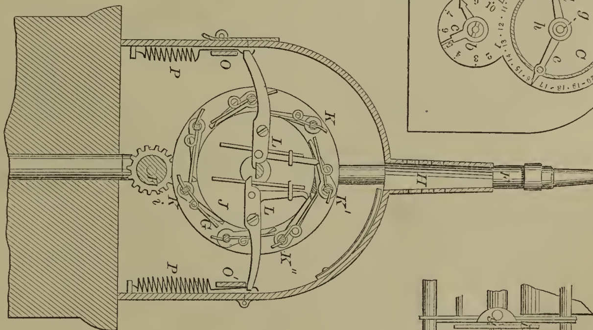
55909—H. S. Richardson—Gas Lighting Machine.
