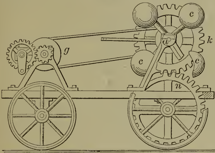
54220—J. A. Schule— Motive Power.
