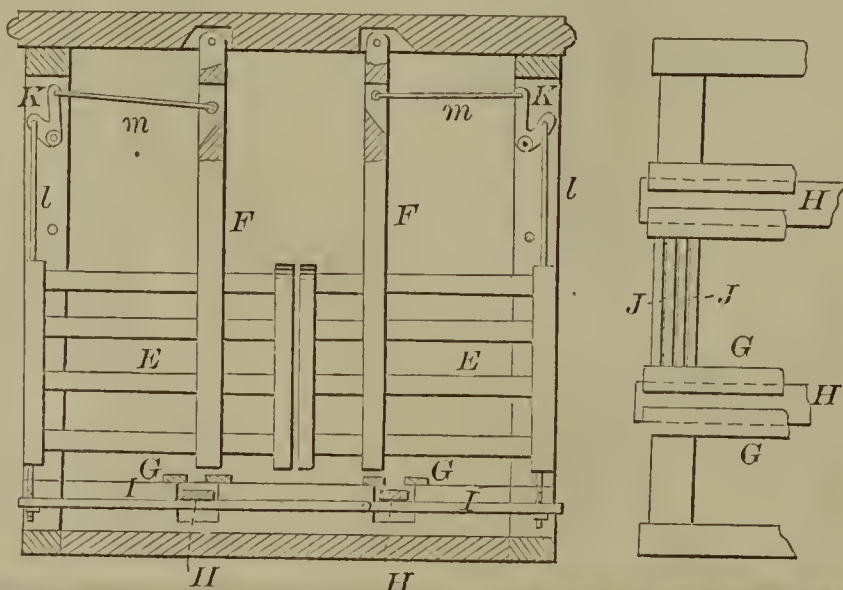
55633—Elkins & Green— Automatic Gate.
