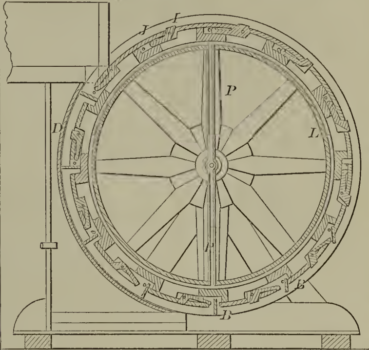
52021—N. Bowker— Water Wheel.
