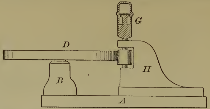
54254—T. J. Powers— Priming Metallic Cartridges.
