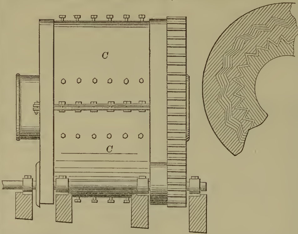
52532—T. J. Chubb—Quartz Mill.
