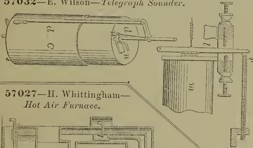
57032—E. Wilson—Telegraph Sounder.
