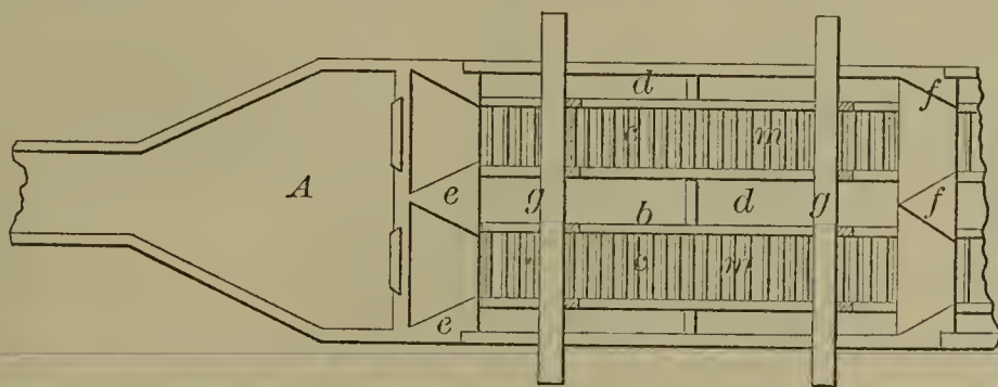
52723—H. Logan—Sluice for Quartz Mills.
