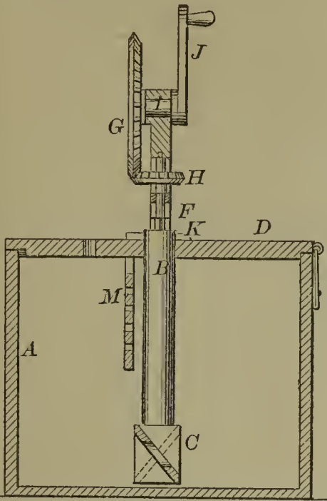
58063—D. P. Chesbrough—Waste Water Receptacle.
