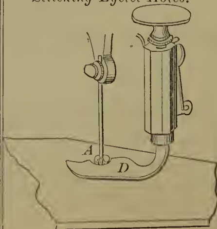
54671—W. B. Bartram— Sewing Machine for Stitching Eyelet Holes.
