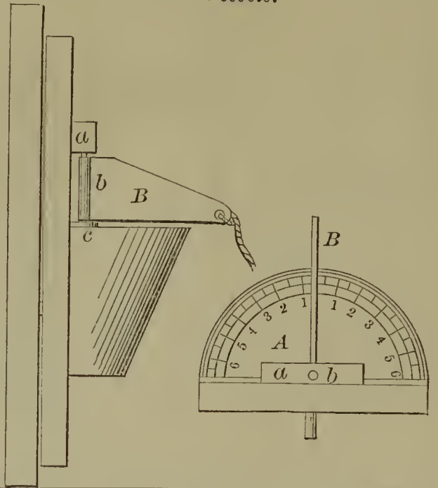
56003—T. Byrne— Leeway Indicator for Vessels.
