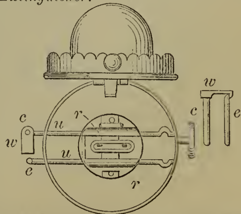
53679—Richardson & Ward—Lamp Extinguisher.
