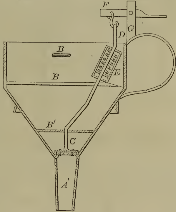
57494—C. W. Fuller— Funnel Measure.
