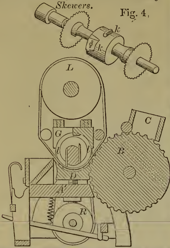
53113—A. Chambers—Machine for Cutting Files.
