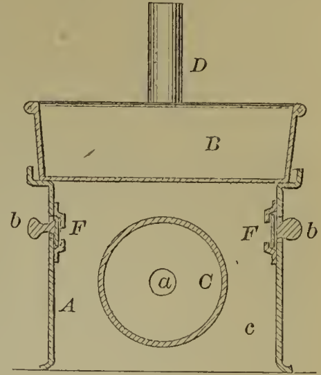
56783—J. Munn—For Heating and Melting Roofing Material.
