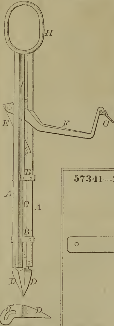
57342—W. Lieber— Button Hole Cutter.
