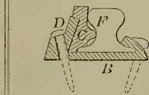
57530—W. M. Martin—Railroad Wedge Rail.
