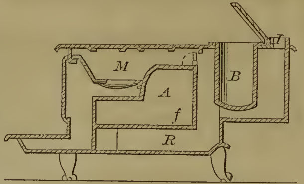
56525—E. Bussey— Cooking Stove.
