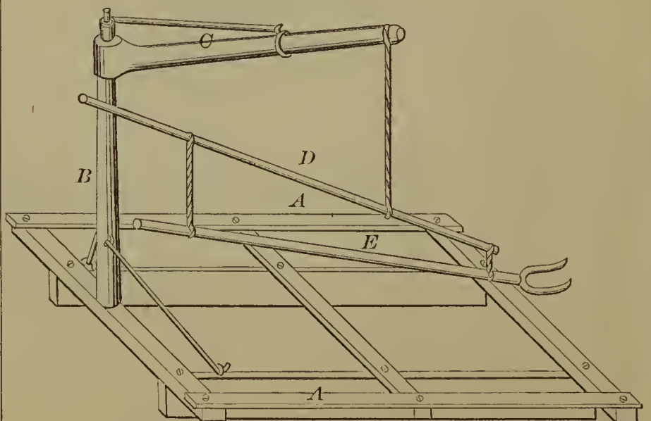
54084—G. Race—Hay Loader.
