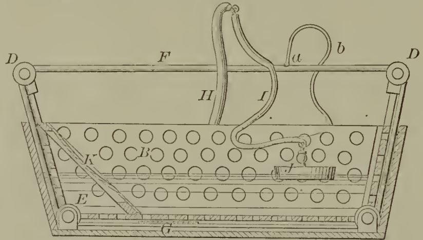
51948—J. Kidder— Electrical Bath Tub.
