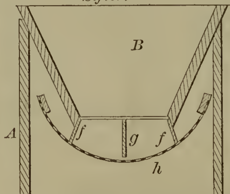
52746—H. F. Read—Flour Sifter.
