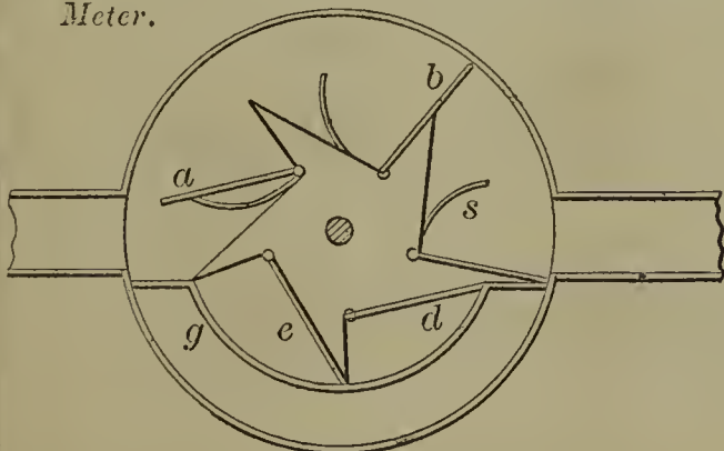
60437—H. H. Stuart—Gas and Liquid Meter.
