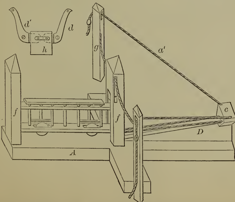
55476—W. Elliott— Farm Gate.
