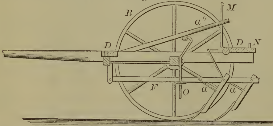
59022—R. C. Howard— Corn Plow.
