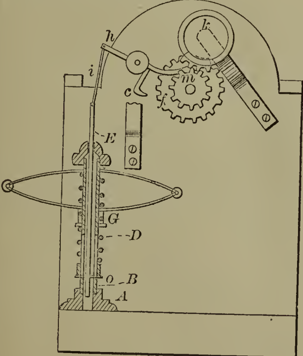
58563—G. Keeble— For Cutting Continuous Sheets of Paper.
