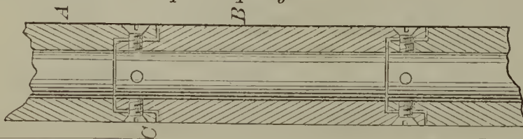
51910—E. Barbaroux—Pipe Coupling.
