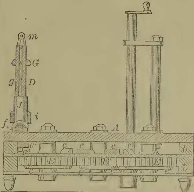
52575—C. F. Jauriet— Metallic Packing for Stuffing Boxes.
