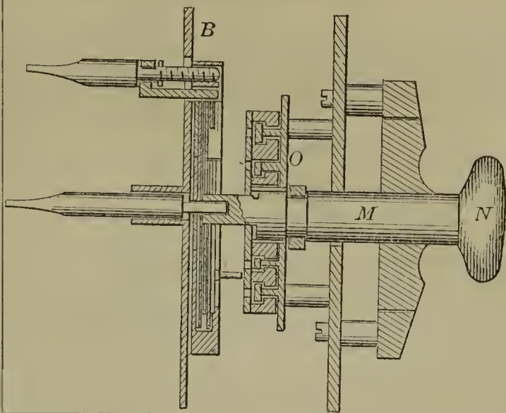
57509—G. W. & E. Hopkins— Automatic Steam Valve.
