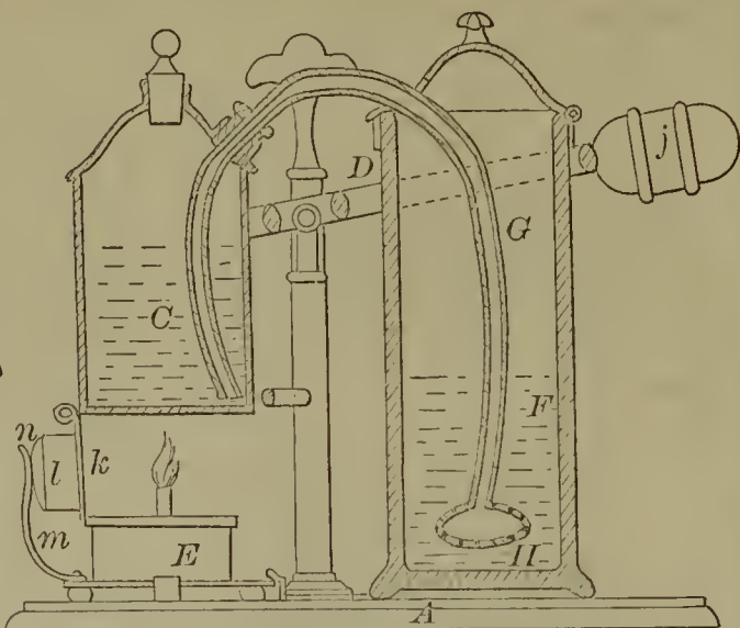
55509—F. Liesche—For Making Coffee.
