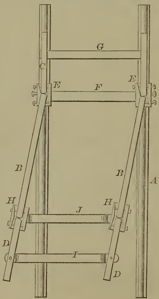
54478—N. Pullman—Switch for Replacing Cars.
