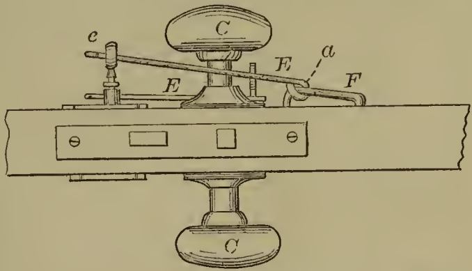
56071—S. Macferran—Door Key Fastener.
