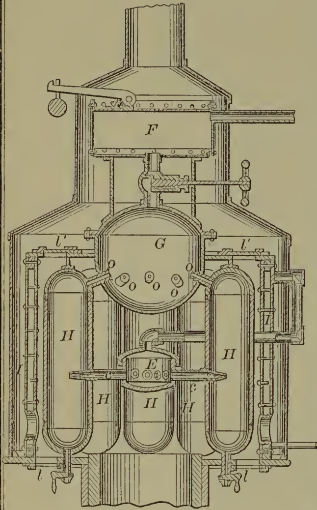
59947—F. Baumann—Steam Generator.
