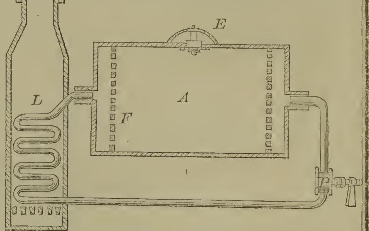
52543—J. W. Dixon— For Making Paper Pulp.
