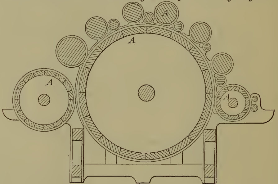
55111—B. H. Jenks— Treating Wood for Carding Engines.
