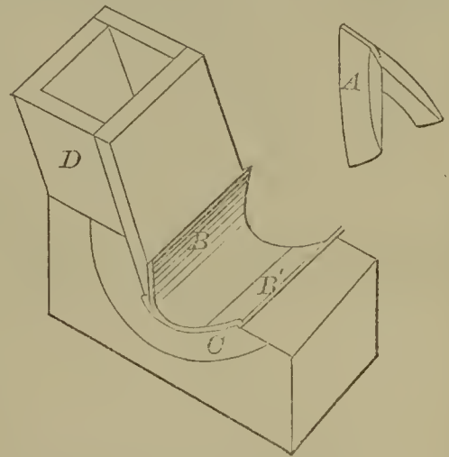
52578—L. M. Larsh— Water Wheel.
