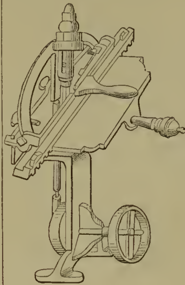
58151—A. Sweetland—Saw Filing Machine.
