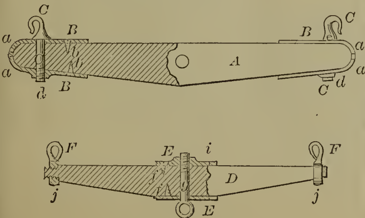
59164—L. Barnes—Whiffletree.
