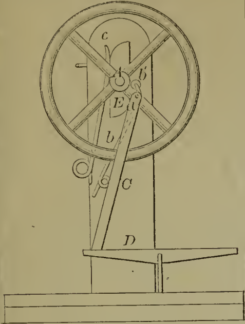
54630—A. Warth— Attachment to Treadles.
