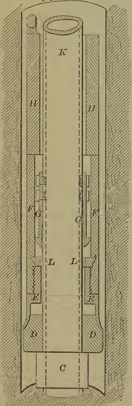
53073—W. S. Wilkinson— Packing for Oil Wells.
