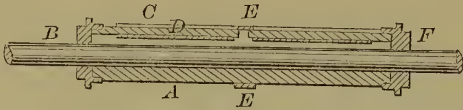
55077—S. F. Emerson— Roller for Wringing Machines.
