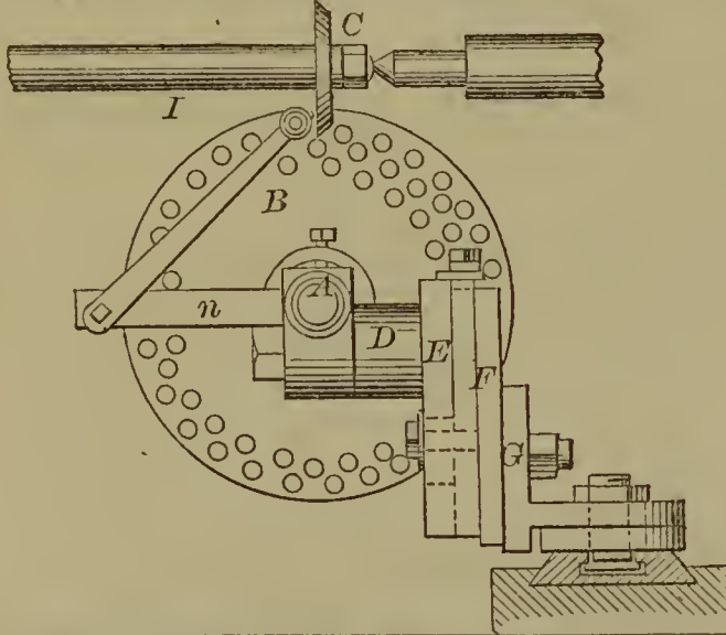
56152—P. L. Weimer—Metal Tube Machine.
