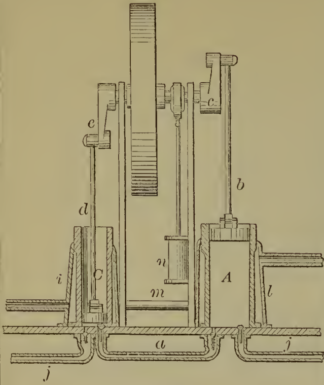
59124—J. N. Dennison—Air Compressing Pump.
