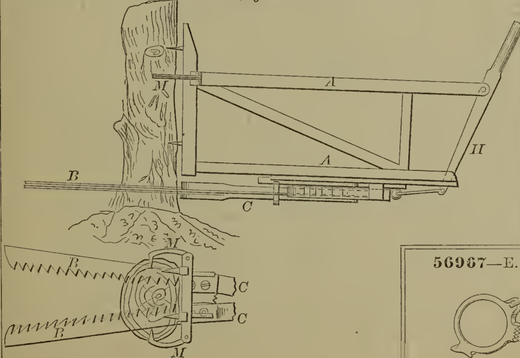
56965—J. D. Matthews—Sawing Machine.
