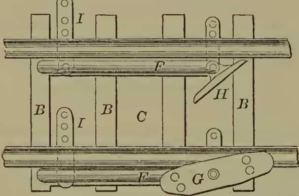
60487—S. T. Denise—Railroad Switch.
