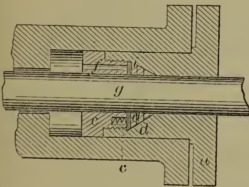
53542—E. T. Prindle— Piston Rod Packing.
