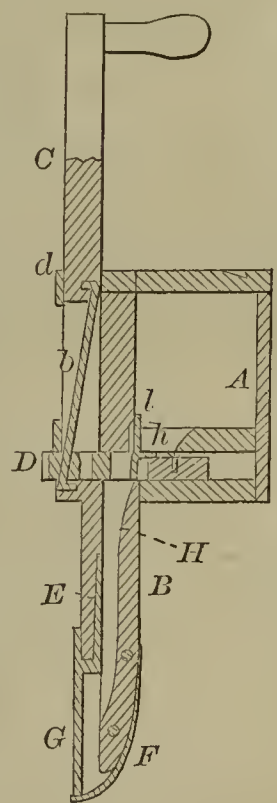
55517—D. McKanna— Hand Corn Planter.
