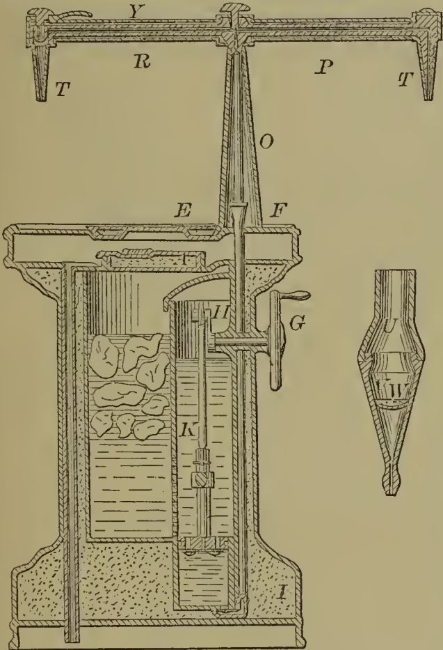
58375—J. W. Cahill—Soda Fountain.
