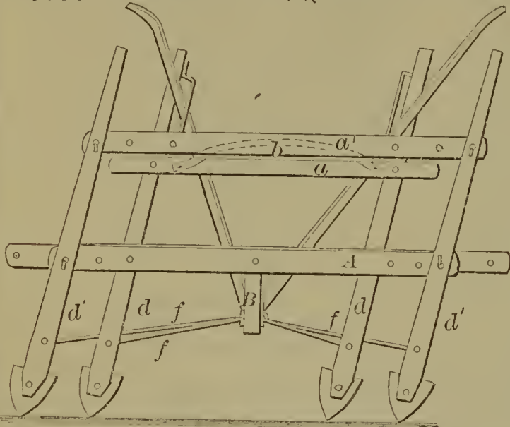
58384—T. J. Cornell—Gang Plow.
