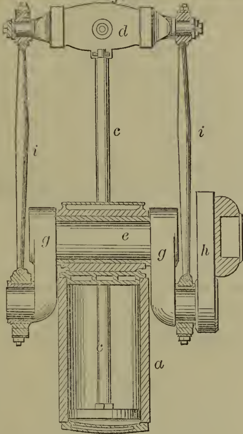
55516—W. L. & T. Winans— Steam Engine.
