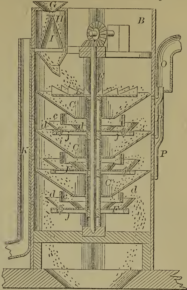
58254—R. Heneage— Grain Dryer.
