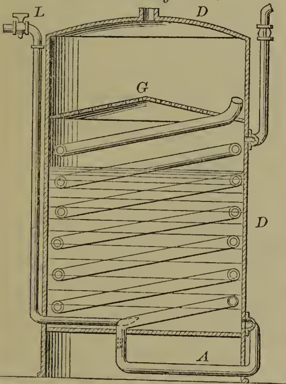
53481—Pond & Richardson— Apparatus For Carburetted Air.
