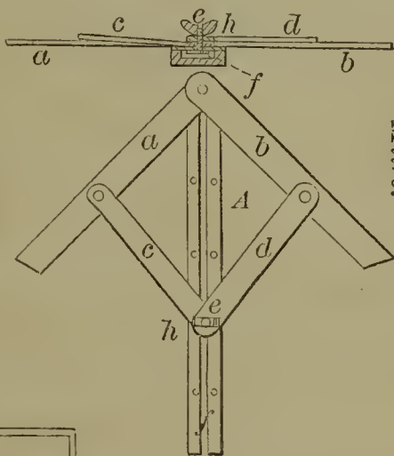
60649—W. H. Stewart—Sawing Machine.
