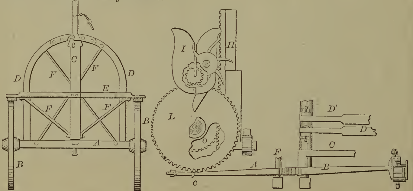
60209—J. J. Look—Wagon Brake.
