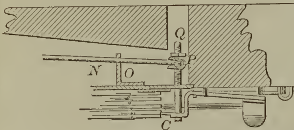
51999—G. M. Hopkins—For Turning Leaves of Music.
