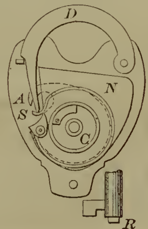
56617—C. W. Saladee—Padlock.
