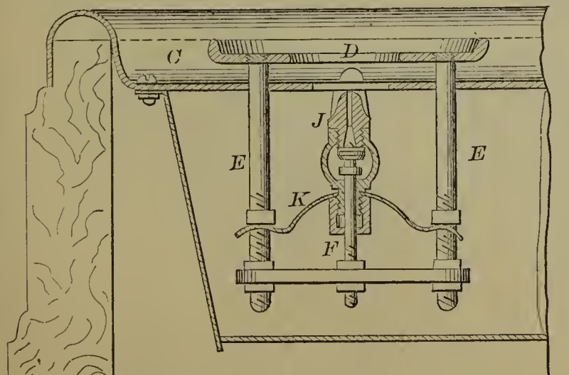
54973—D. M. Somers— Tumbler Washer and Cooler.
