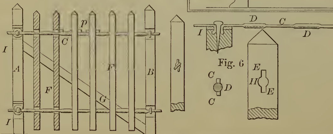
53616—W. D. Hillis—Fence.
