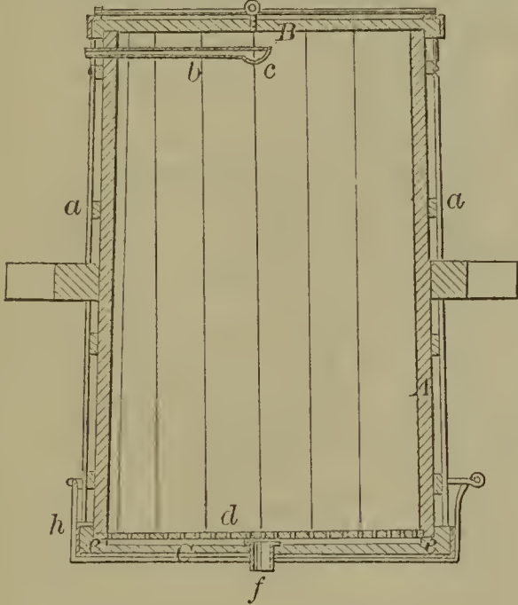
57218—N. S. Thomas— For Extracting Tanning Matter from Bark.
