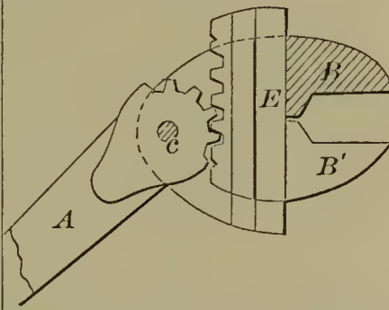
52930—W. Morehouse—Wrench.
