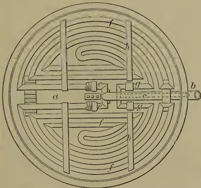
55747—Trageser & Schreiber—Coil for Brewers' Boilers.
