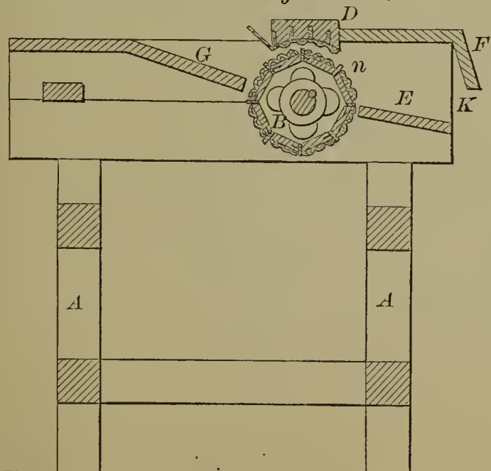
53694—J. P. Smith— Threshing Machine.
