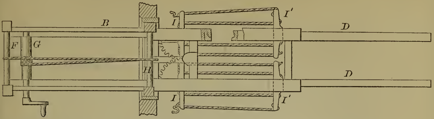
53544—D. T. Robinson— Car Brake.
