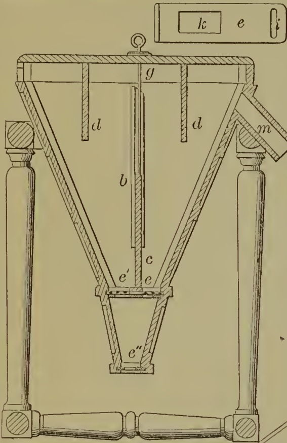
53718—Whelpley & Storer— Separating Ores.
