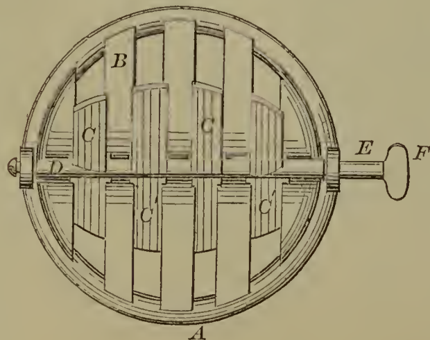
54197—S. R. Nye—Stove Pipe Damper.
