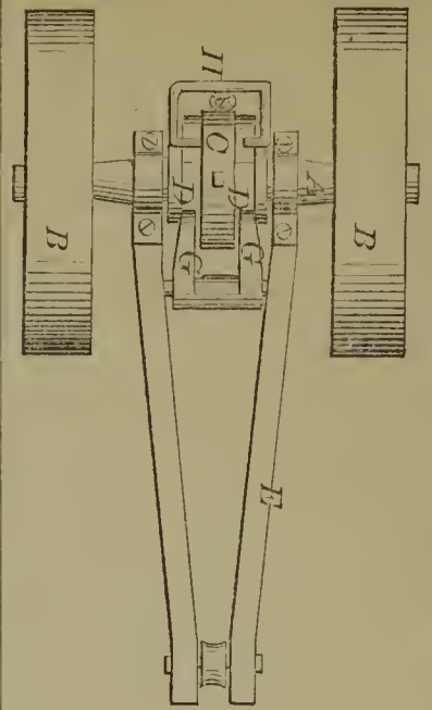
57067—Ball & Houghtelin— Grubbing Machine.
