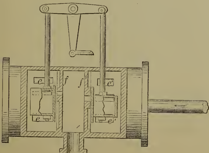
56841—A. H. Woodruff—Slide Valve.
