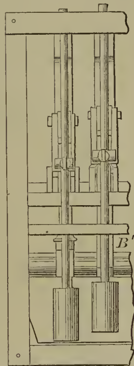
58775—W. Churchill—Steam Engine Governor Valve.
