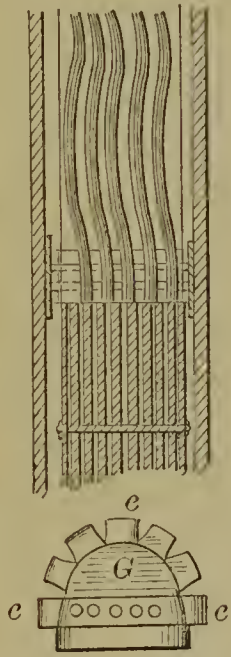
53700—J. Story— Telegraph Cable.
