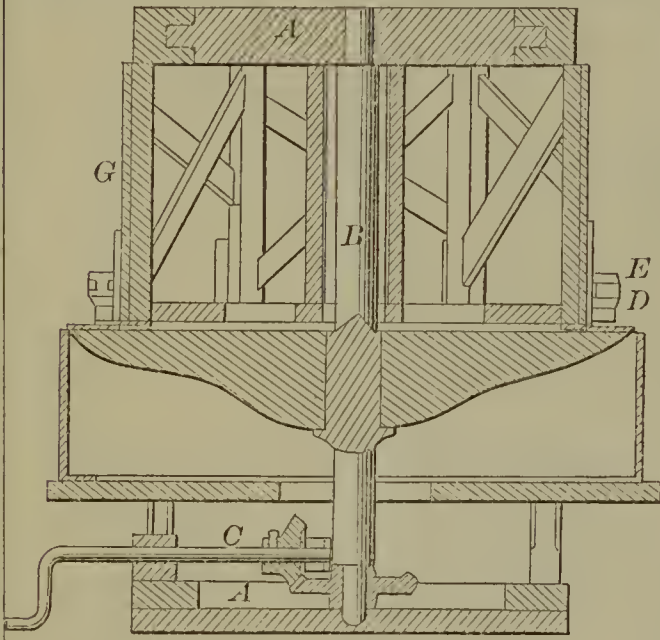
52251—J. Taggart—For Slivering Wood.
