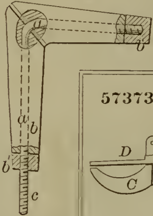
57368—Ogborn & Chapin— Stove Pipe Damper.
