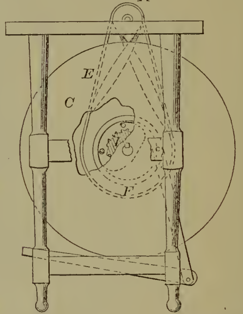
53312—C. B. Lewis— Mechanical Movement.
