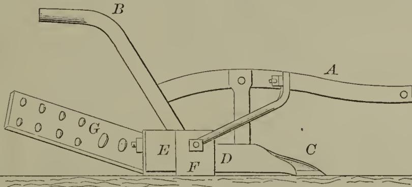
51817—R. Elliot— Plow and Scraper.
