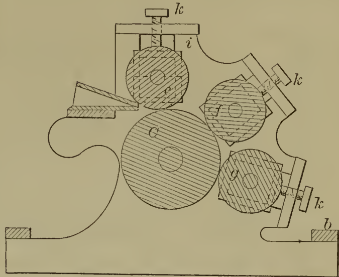
52785—J. H. Darlington—Pressing Paper Collars.
