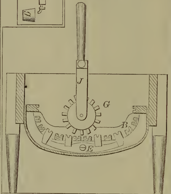
55634—J. C. Fellows— Washing Machine.
