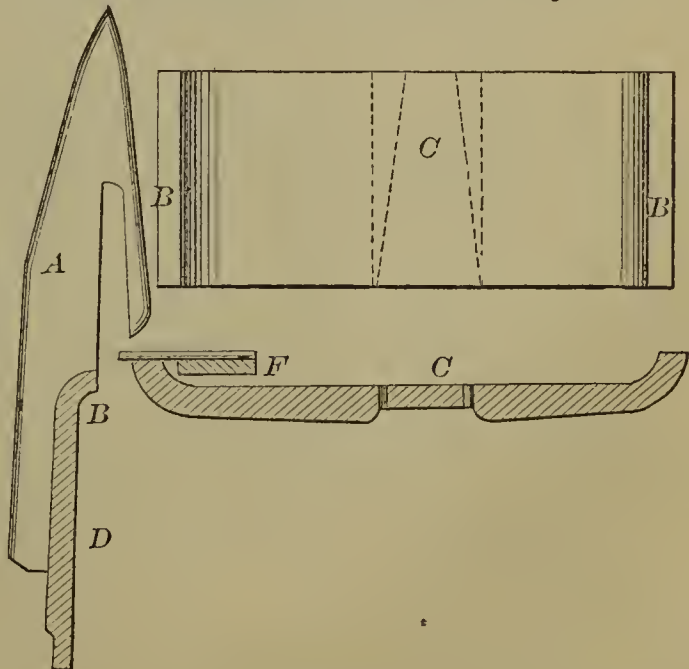
55074—R. Dutton—Harvester Finger Bar.
