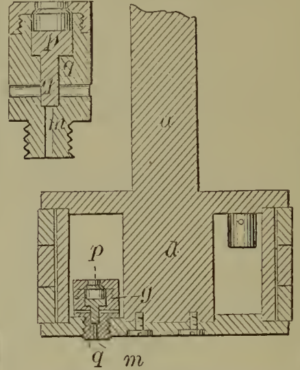
55387—E. Sullivan— Piston Head for Steam Engines.
