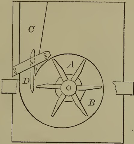
52358—W. R. Close—Water Wheel.
