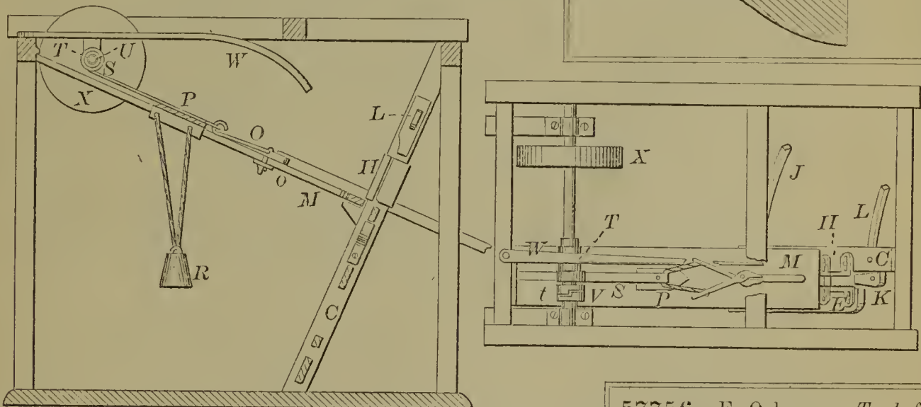
57756—E. Osborne—Tool for Making Wooden Legs.
