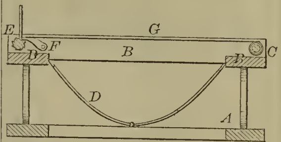
57183—S. Petre—Derrick for Raising Sunken Vessels.
