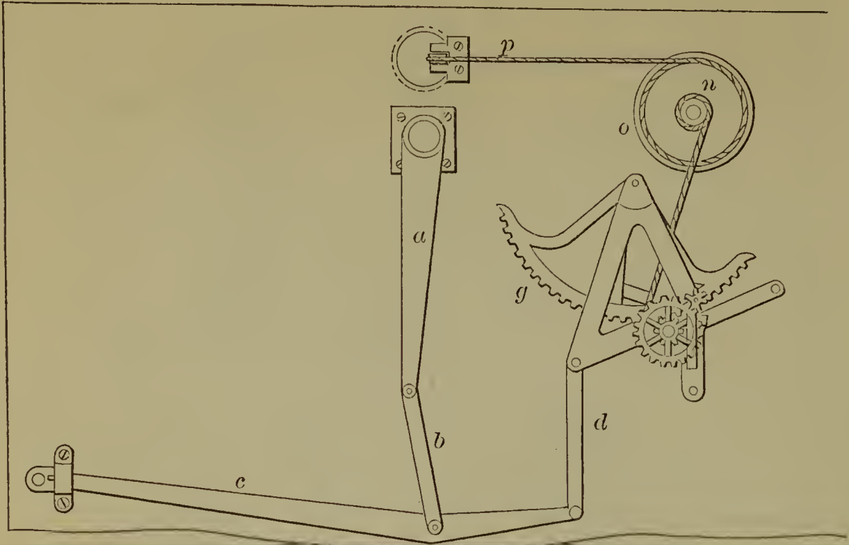
53934—M. W. Ruthven— Steering Apparatus.
