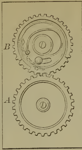
59064—L. B. Potter— Intermittent and Expansive Gearing.
