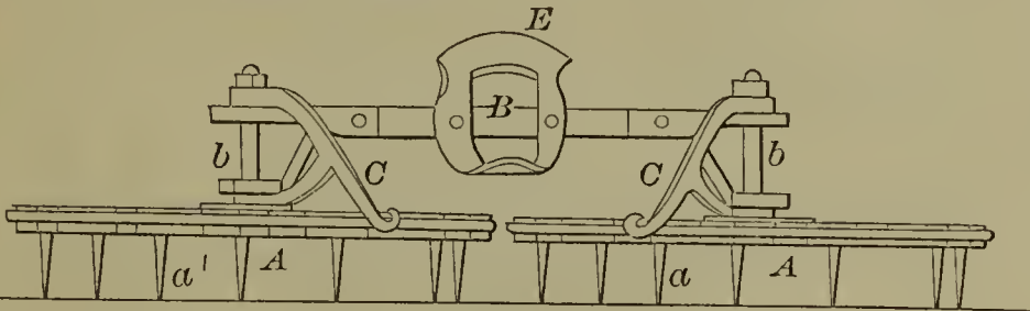
53850—A. Mero—Harrow.
