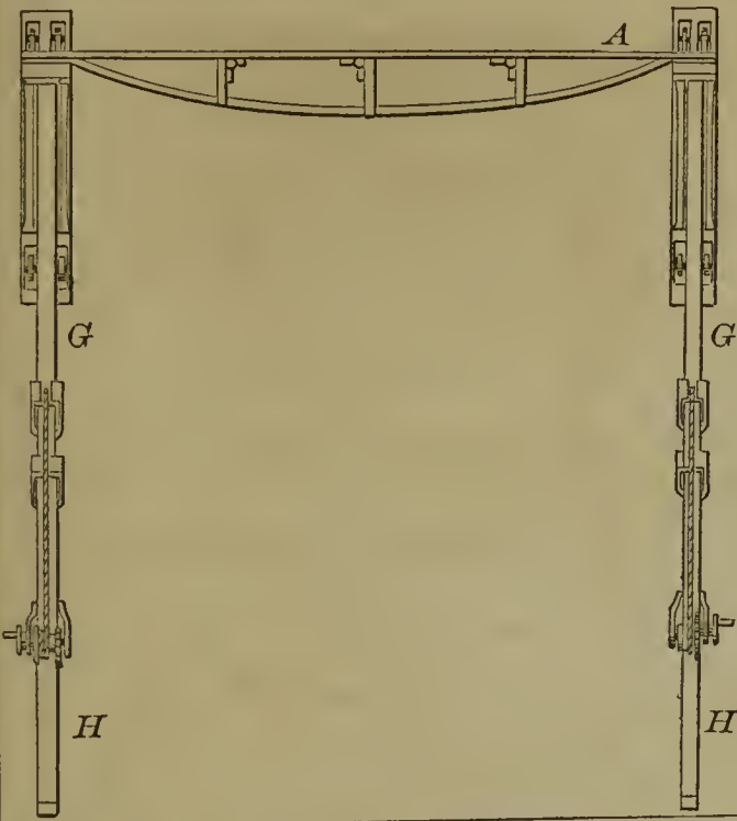
56437—Newbanks & Powel—Scaffold.
