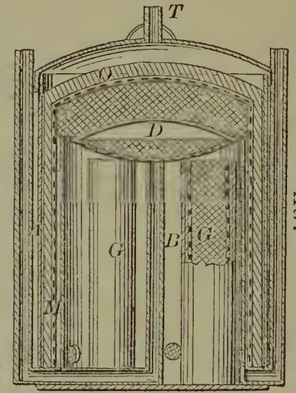
58859—M. J. McCormick— Vault Light.
