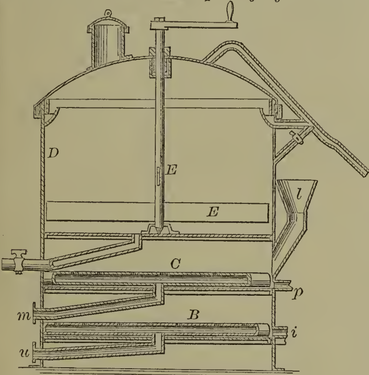
60179—F. Haack—For Imparting Age to Wines.
