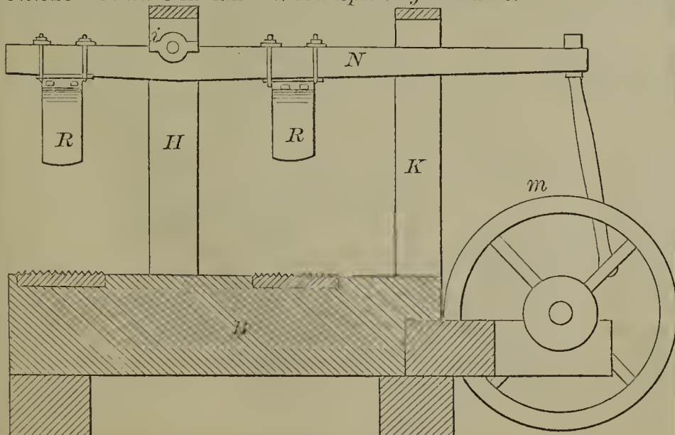
52215—J. H. Silkman—Wood Splitting Machine.
