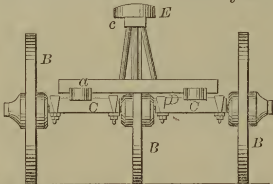
52482—J. I. Wilson—Furrowing Machine.
