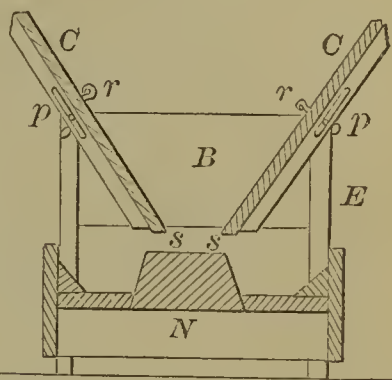
58531—C. E. Wright—Cherry Stoner.
