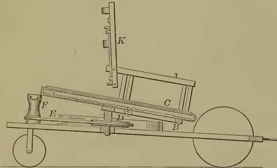
52819—T. Boyd—Corn Harvester.
