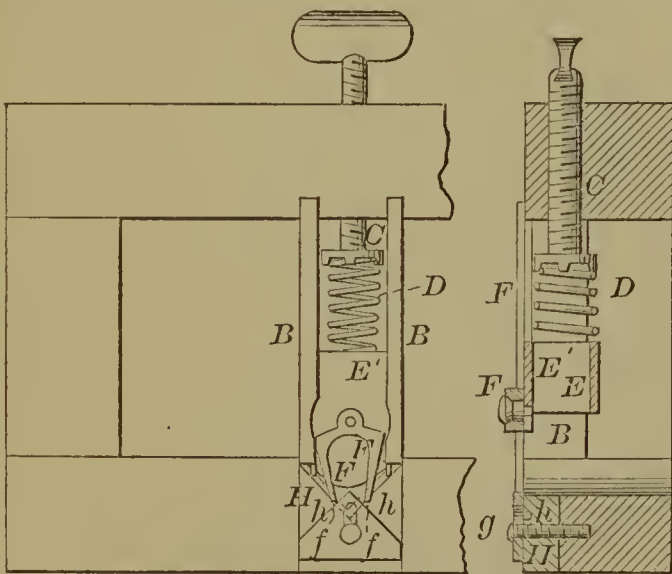
54882—G. F. Foote—Tool Holder for Dentists.
