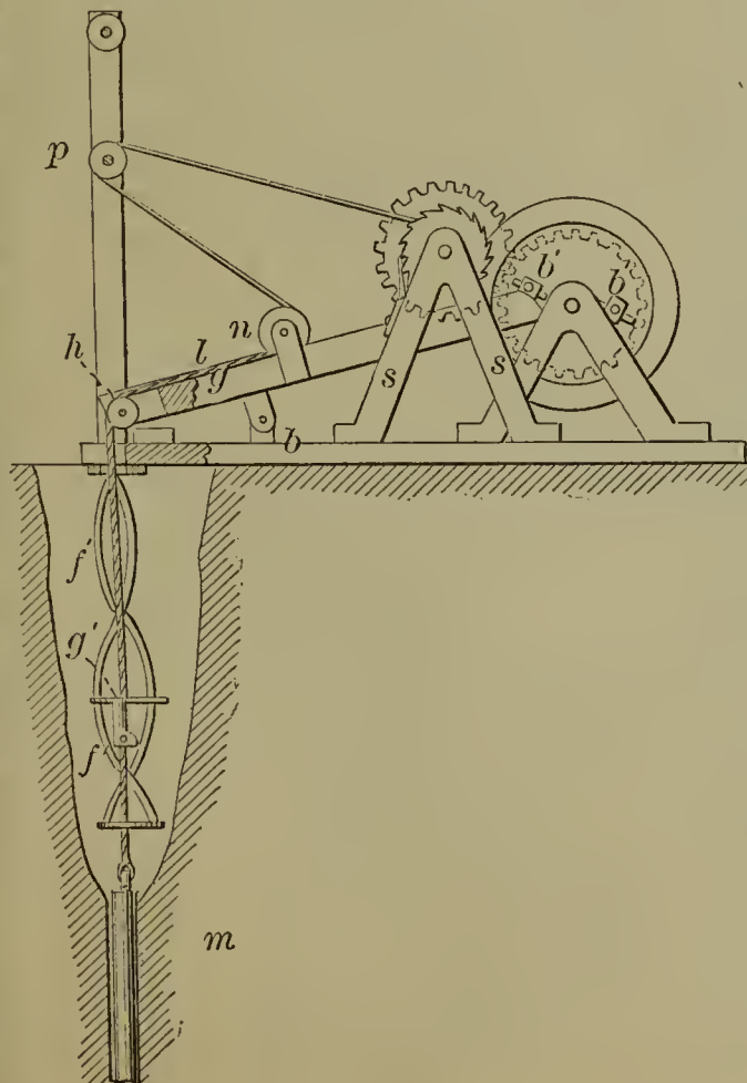
54011—G. R. Platt— Oil Well Drill.
