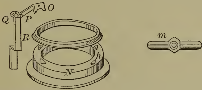
53343—E. Robinson—Portable Water Closet.
