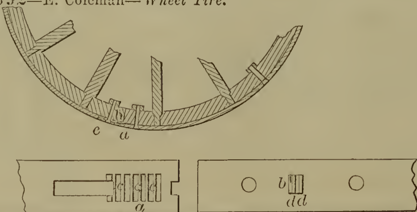
57092—E. Coleman—Wheel Tire.
