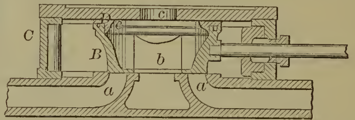
59848—J. Lochhead—Balanced Slide Valve.
