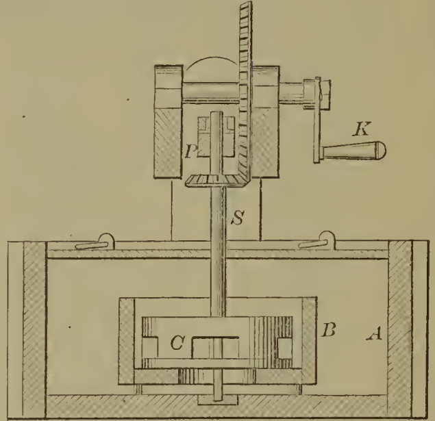
59282—Z. B. Shannon— Churn.
