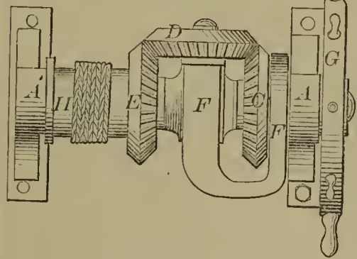
57695—S. H. Everett—Lubricating Brush.
