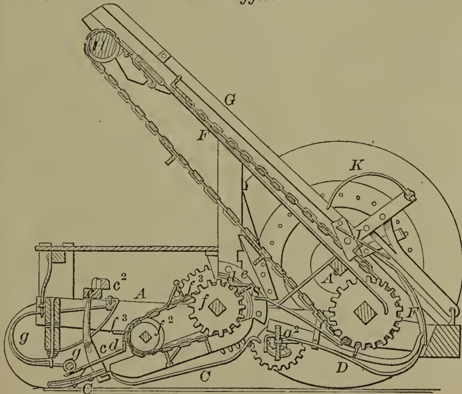
60501—A. Gilmore— Potato Digger.
