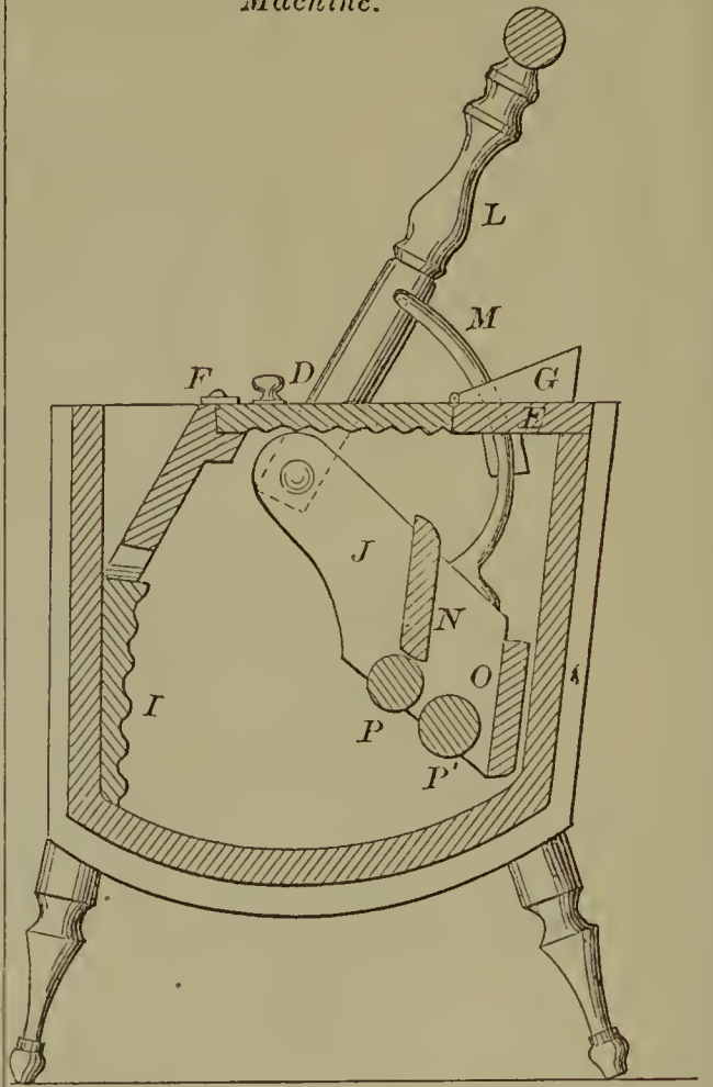
56644—F. W. Vosmer—Washing Machine.
