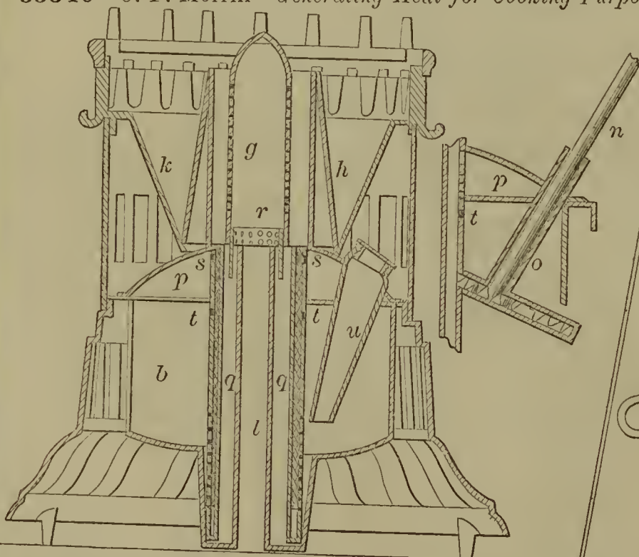
55340—O. F. Morrill—Generating Heat for Cooking Purposes.
