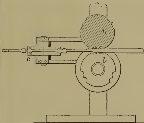
55270—T. Fowler—Horse Shoe Nail.
