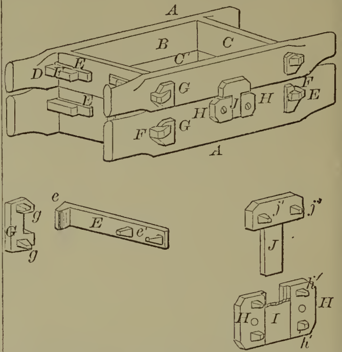
57903—J. G. Holliday—Moulders' Flask.
