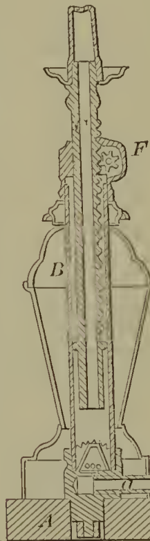
55447—Allen & Riddell— Portable Gas Stand.
