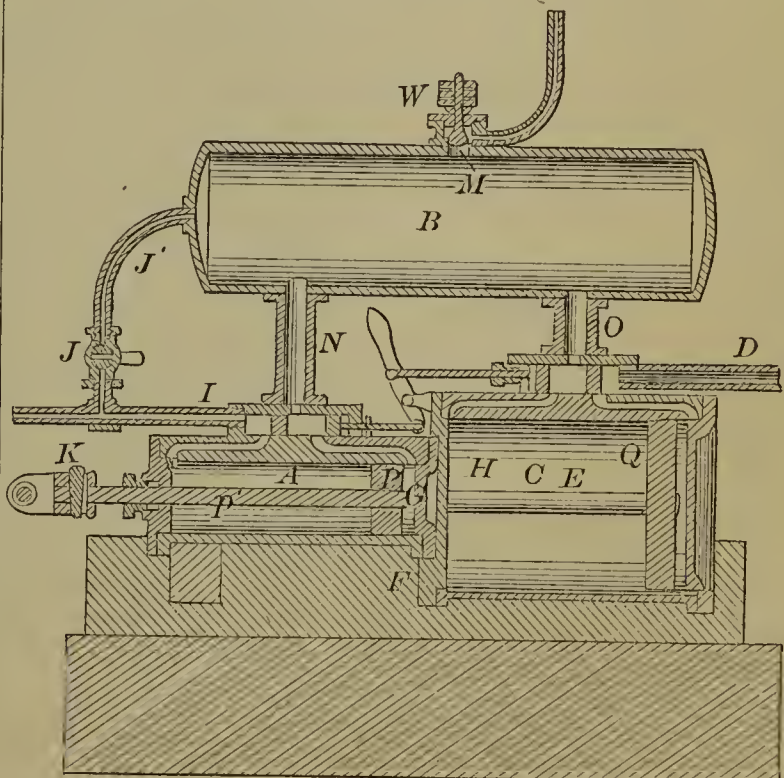
54150—A. Hartupce— Steam Engine.
