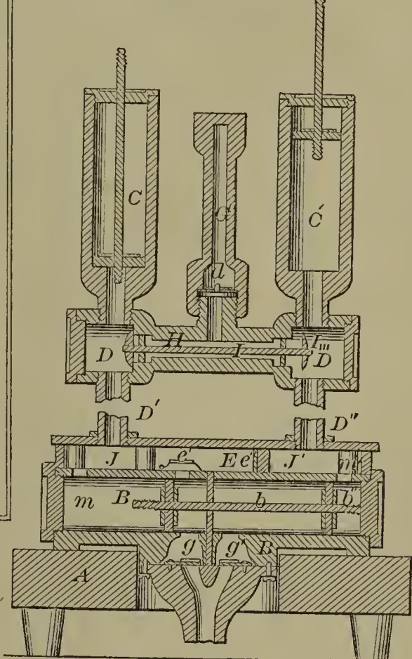
60535—O. Miller—Pump.
