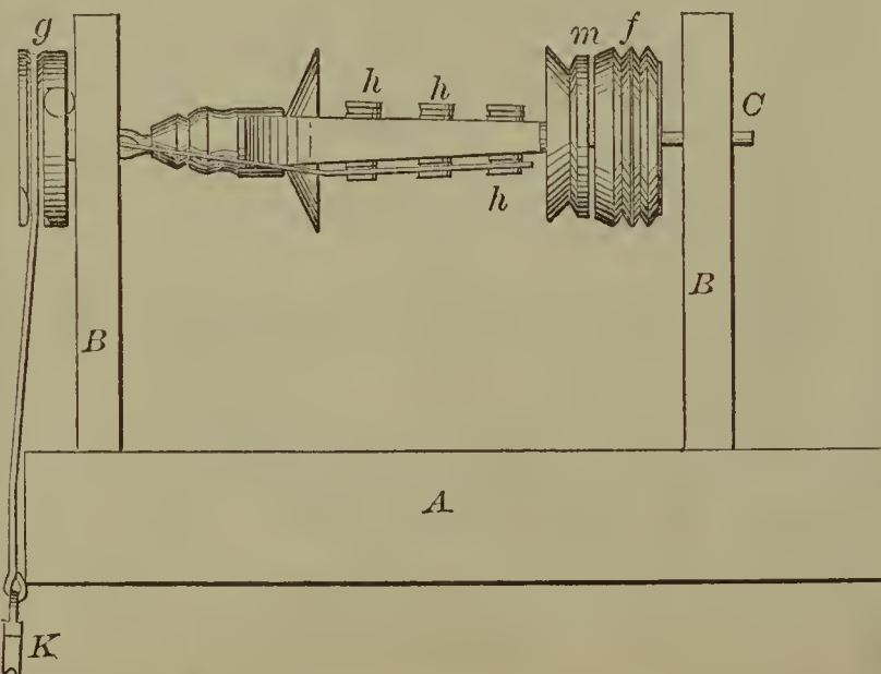
60314—T. Woods—Stone Drill.
