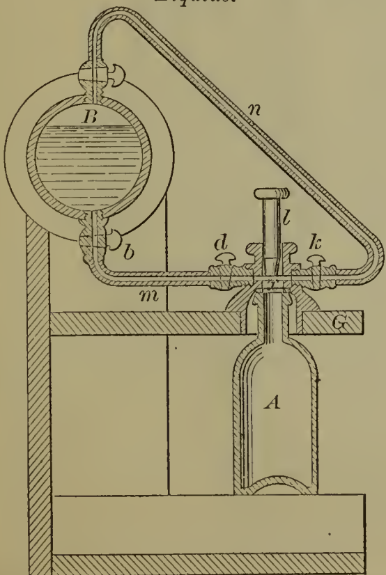
53019—J. Mathews, Jr.— For Bottling Liquids.
