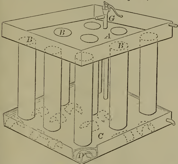
55532—C. F. Pike— For Cooling Oil, &c.
