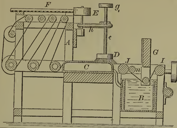
57958—J. E. Pattison—Treating Cane Juice.
