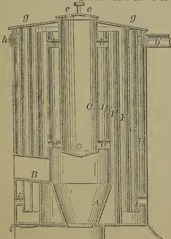
57028—H. Whittingham—Hot Air Furnace.
