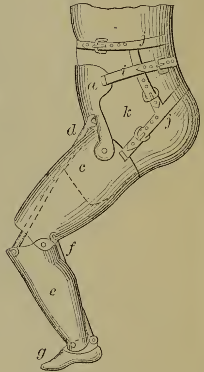
54972—P. J. Smith— Mechanical Movement.
