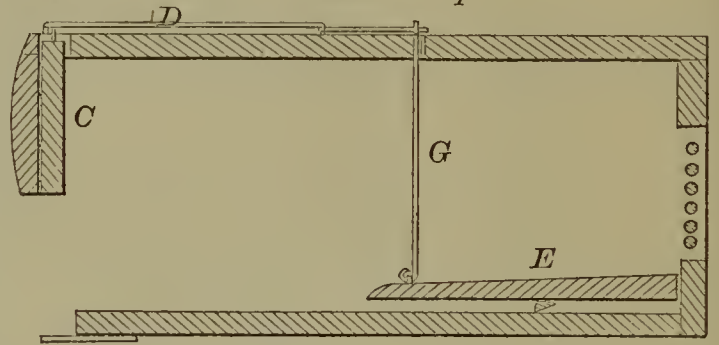
54241—G. Wolf—Animal Trap.
