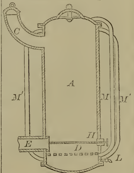
52544—J. W. Dixon— For Making Paper Pulp.
