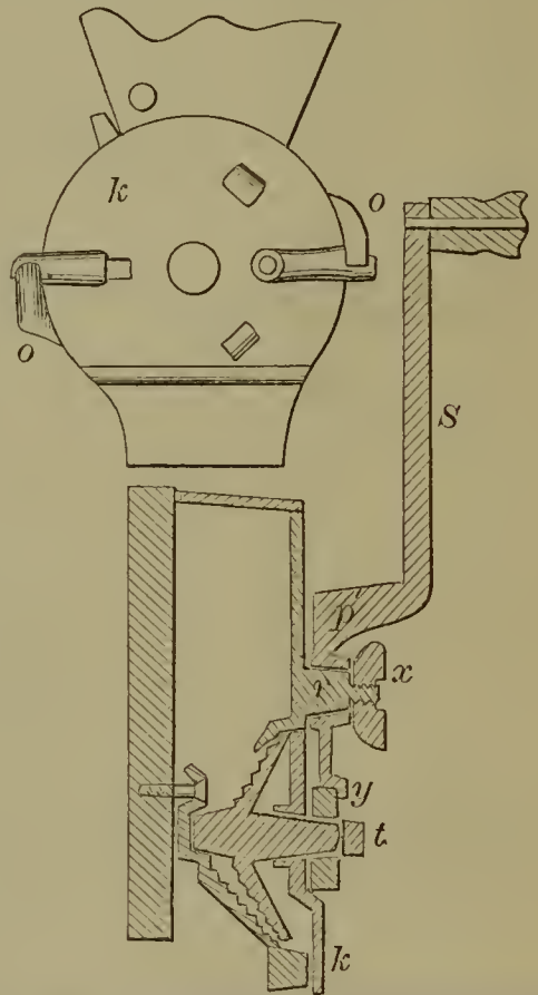
53129—C. R. Edwards—Coffee Mill.
