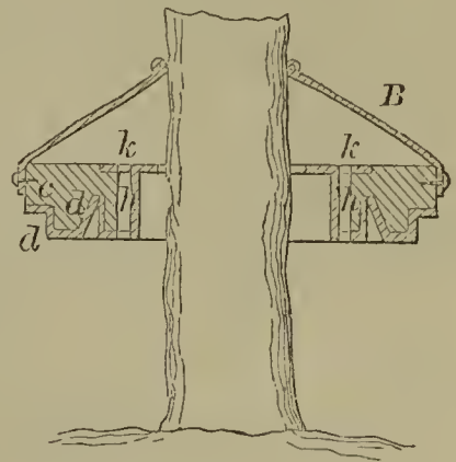
55776—W. & D. McCaine— Tree Protector.
