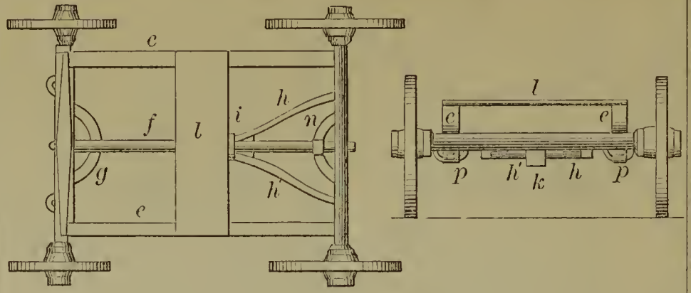
53568—C. T. Bush— Carriage.
