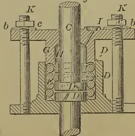
58204—C. P. Benoit—Piston Rod Packing.
