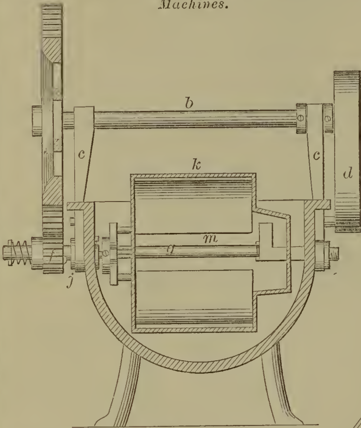
54493—J. Blayne—Hand Spinning Machine.
