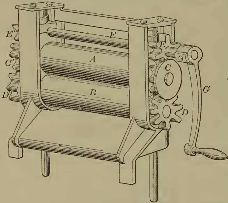
56595—Morris & Eynon— Granulating Furnace Slag.
