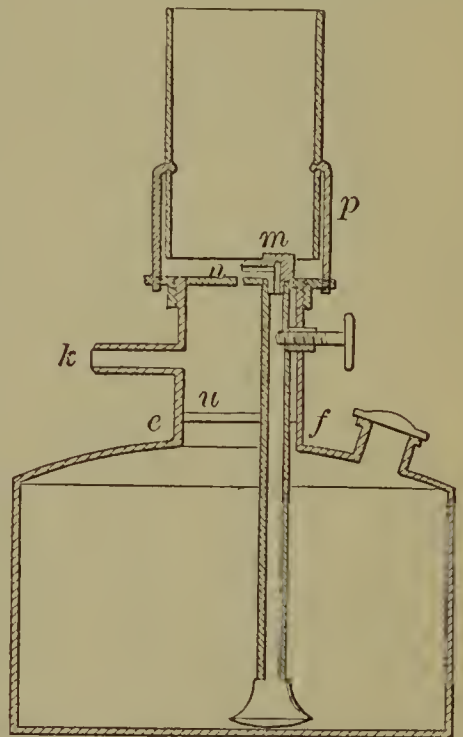
53769—E. H. Ashcroft—Cistern for Draining Peat.
