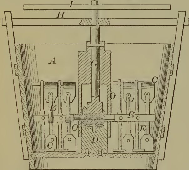
53600—George & Hague—Brick Machine.
