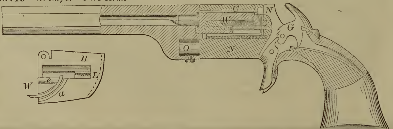
55719—A. Sayer—Fire Arm.
