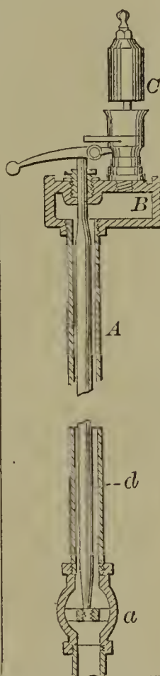
60470—R. C. Bristol— Water and Steam Separator for Steam Generators.
