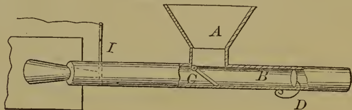
54783—S. Scotton— For Shooting Gravel at Cows on Rail Road Tracks.
