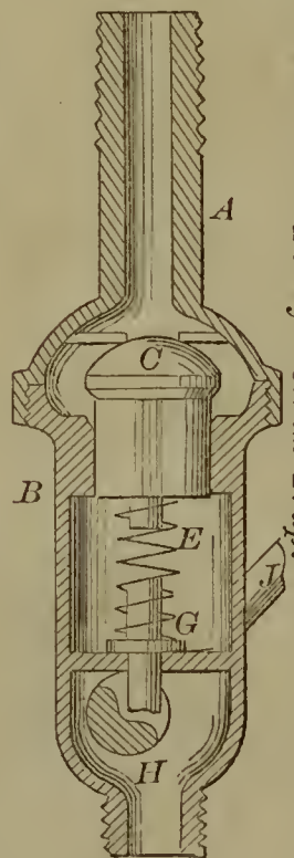
60622—T. N. Davey— Steam Trap.
