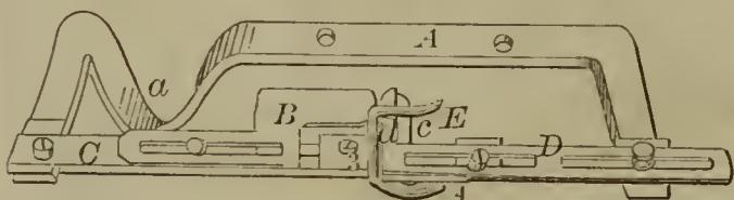
57374—W. Preiss— Folding and Plaiting Device for Sewing Machines.
