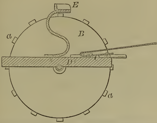
54472—N. G. Whitmore— Blacking Brush.
