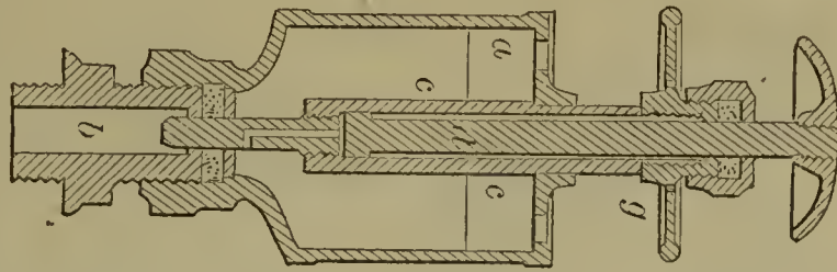
57079—G. B. Brayton— Oil Injector for Steam Engines.
