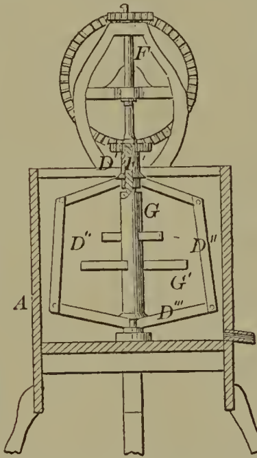
60493—S. S. Elder—Churn, Beer Cooler, &c.
