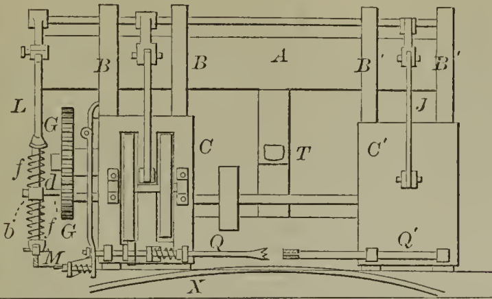
52001—Manderson & Favinger—For Removing Carries of Vessels.
