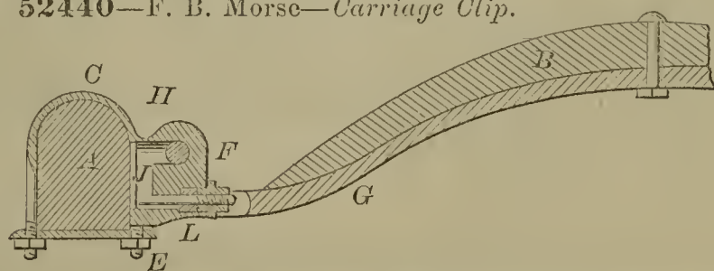
52440—F. B. Morse—Carriage Clip.
