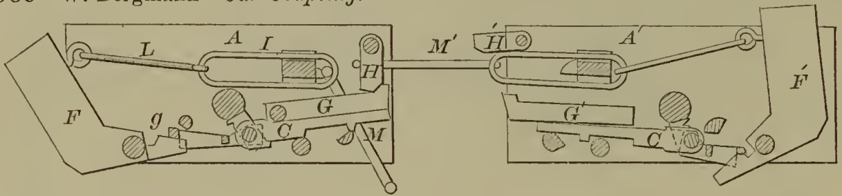
55989—W. Bergmann—Car Coupling.
