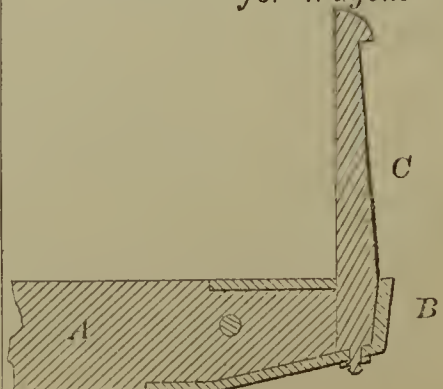
55453—D. L. Babcock— Bolster for Wagons
