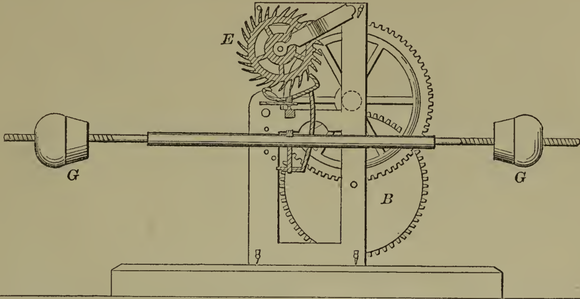
60305—J. Whitehead—Hand Loom.
