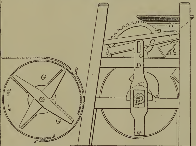
58630—F. Frye—Winnowing Machine.
