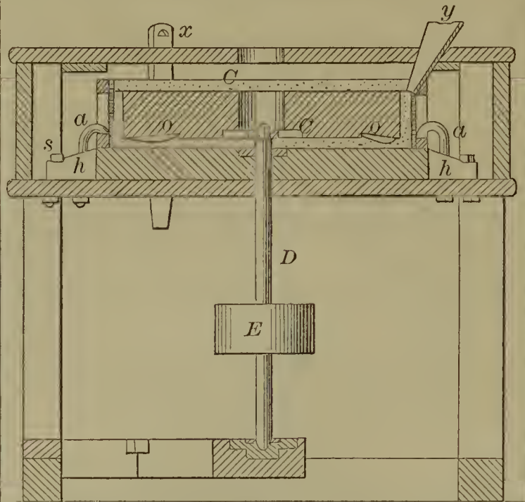
52780—E. Wright—Let-off for Looms.
