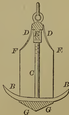
54847—C. F. Brown— Anchor.
