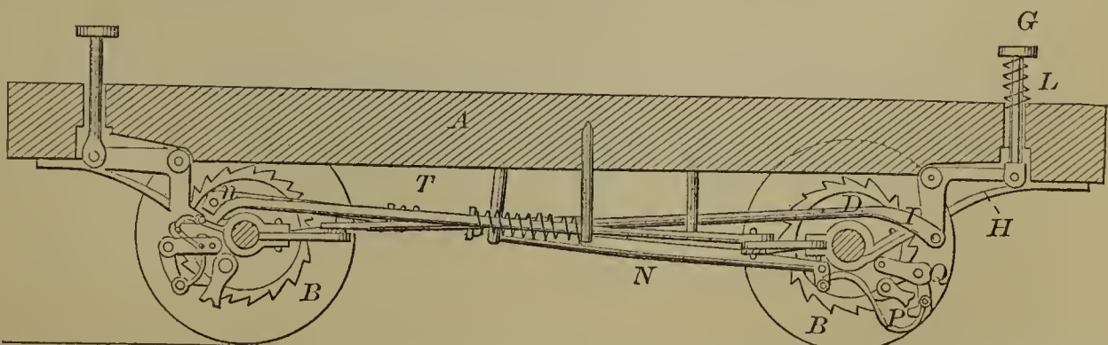
54363—J. E. Kelsey—Stopping and Starting Cars.
