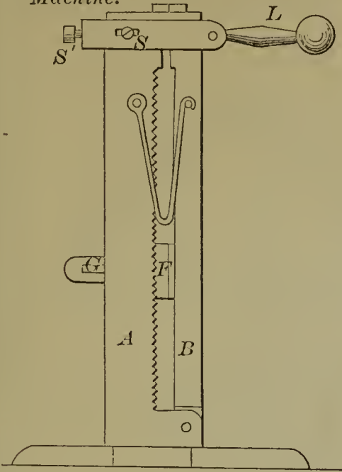
52912—A. Tucker—Bolt Heading Machine.
