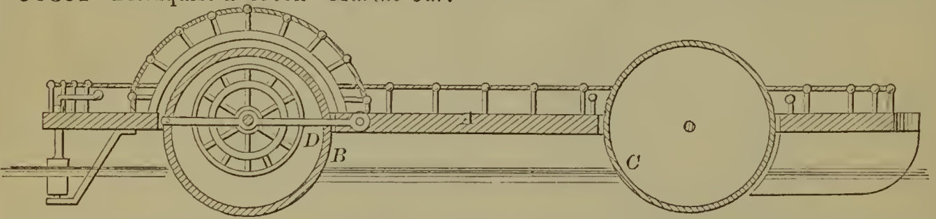
56351—Blomquist & Crook—Marine Car.
