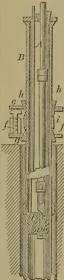
52866—J. H. Luther—Oil Well Tube Extractor.
