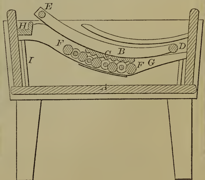
53035—A. B. Parsons—Washing Machine.
