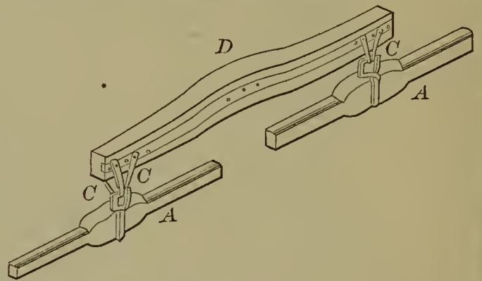
55112—N. Johnson— Whiffletree.
