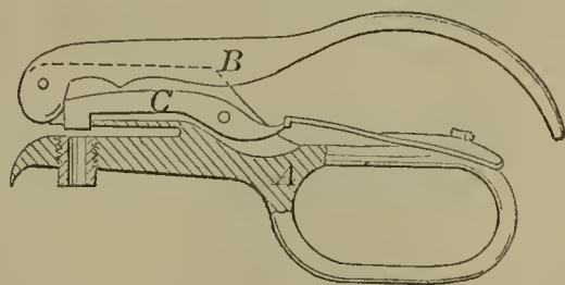
57136—C. B. Holden— Punch.
