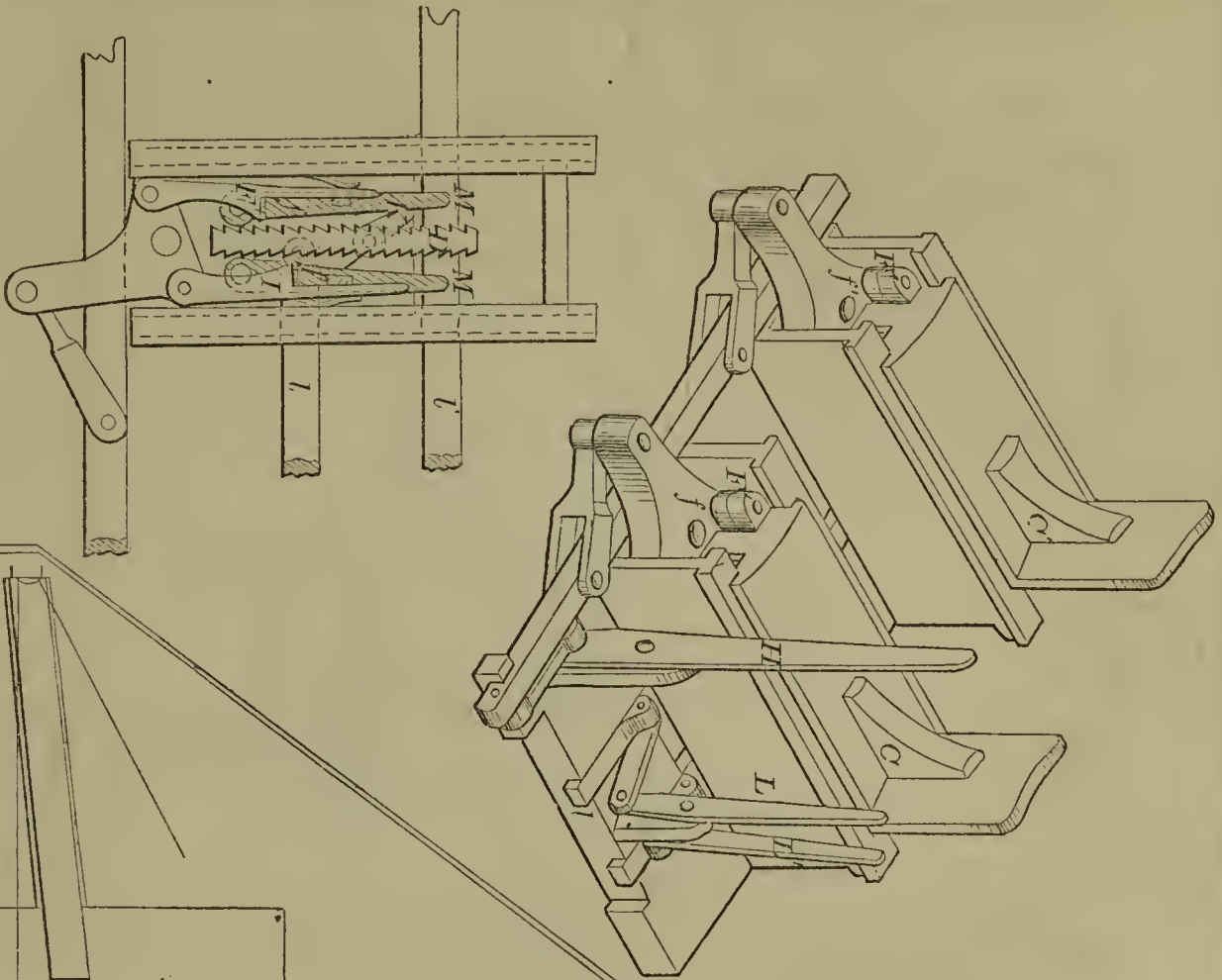
57180—J. W. Parsons—Head Block for Saw Mills.
