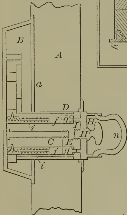
52230—S. Walker— Self-Locking Tail Board.
