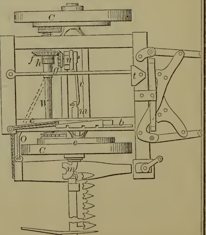
53040—J. G. Perry—Reaping and Mowing Machine.
