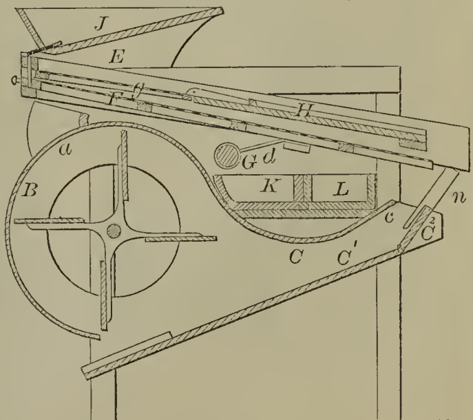
52071—E. C. Patterson— Grain Separator.
