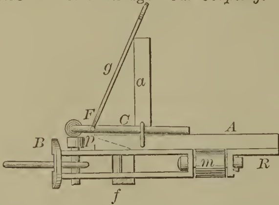
58723—D. C. Guttridge—Car Coupling.
