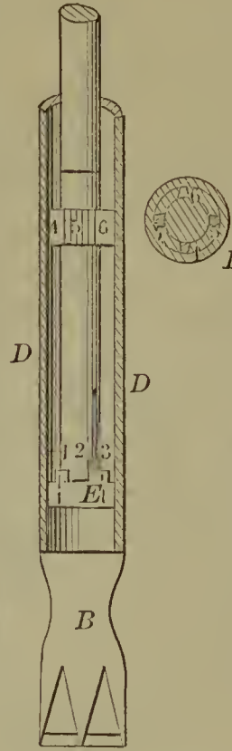
58809—J. & A. W. Gillmore— For Sinking Well Tubes.
