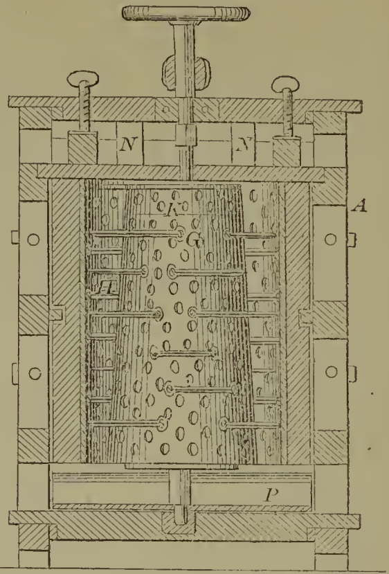
58912—S. Stukeley—For Grinding Cob and Corn.
