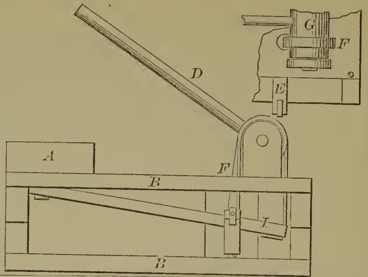
59294—A. H. Tingley— Heat Regulator for Hot Air Furnaces.
