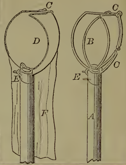
60564—H. F. Schroder— Pan for Evaporating Sugar.
