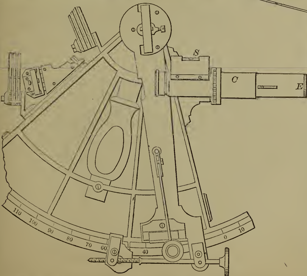
54698—G. Davidson—Sextant.
