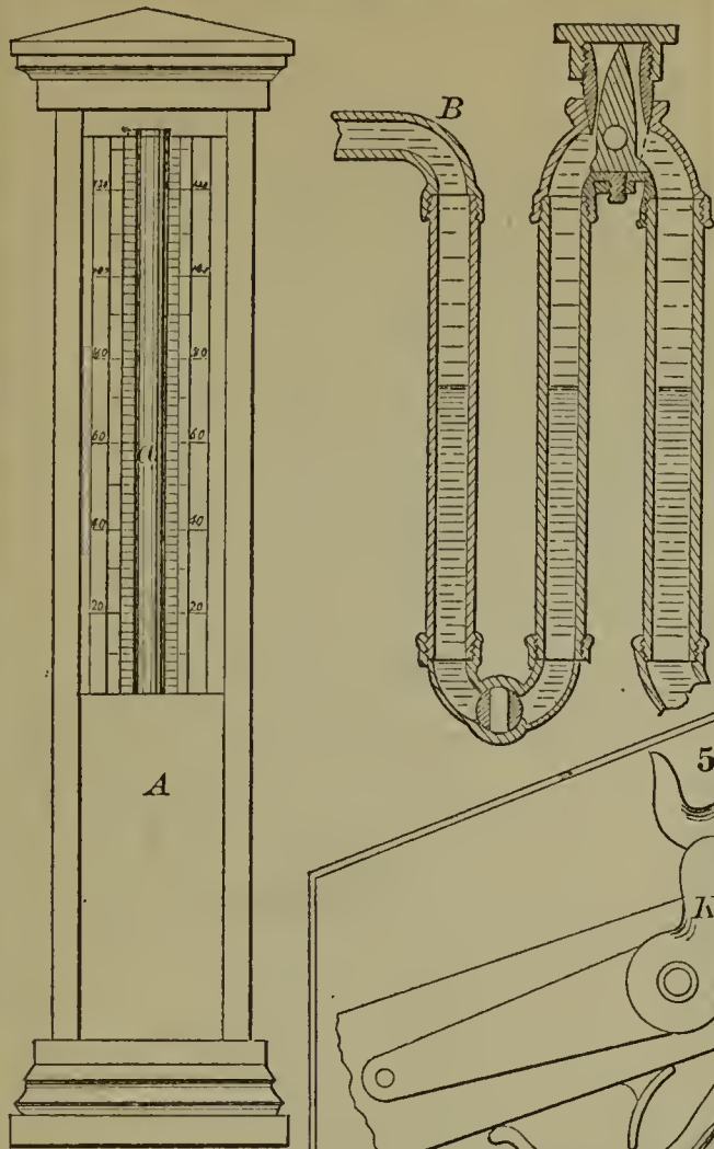
53183—E. Quinn— Steam Gauge.
