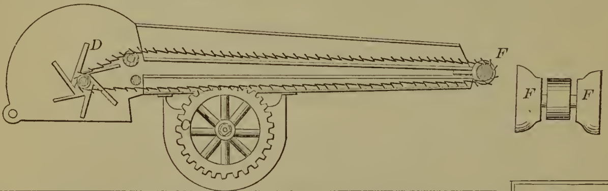
53148—F. Humphrey— Coffee Roaster.
