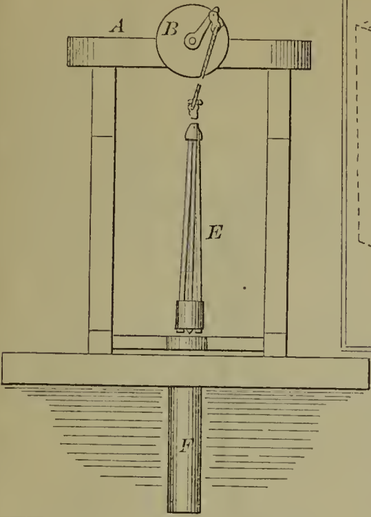
53603—S. Godfrey—Grinding Mill.
