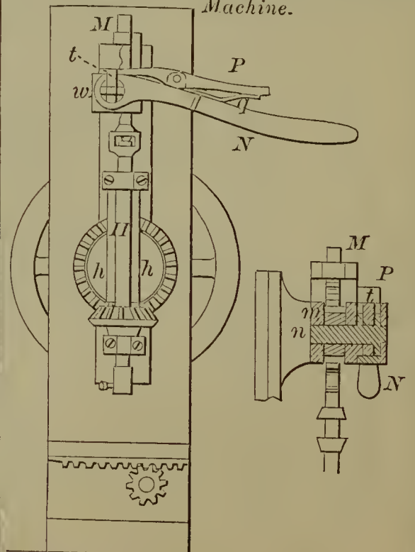
53981—T. M. Howard—Drilling Machine.
