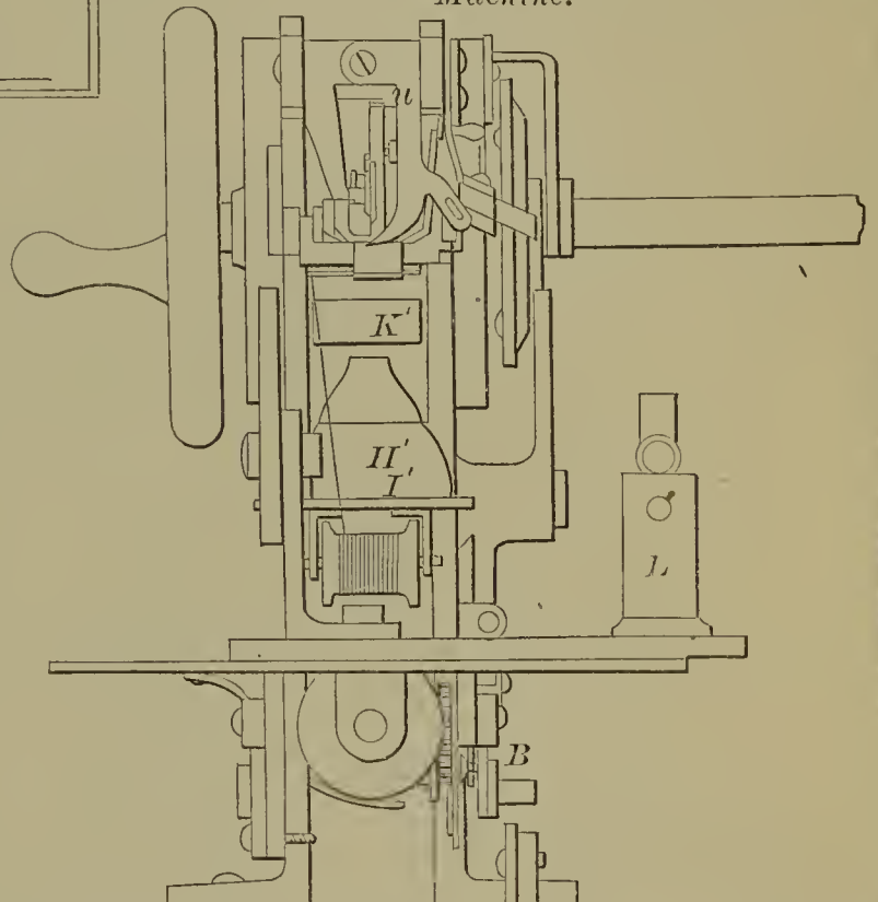
56729—A. Destony—Boot and Shoe Sewing Machine.
