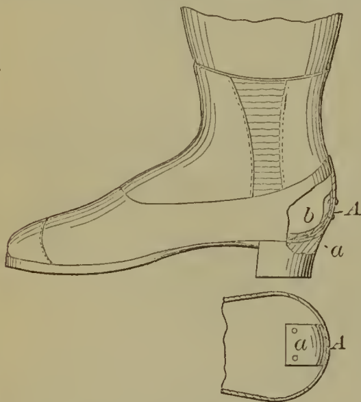
59075—J. Reising— Counter Supporter.
