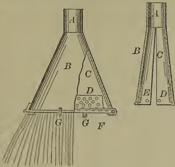
55936—J. Wasson—Broom Head.
