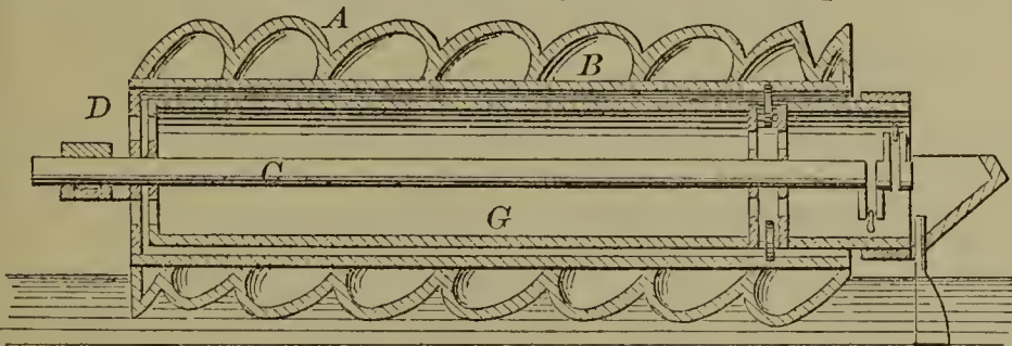
53316—D. E. Masnata— Revolving Screw Steamship.
