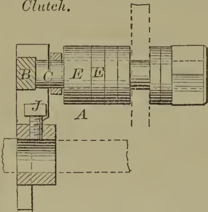
60113—R. Allen—Lathe Clutch.
