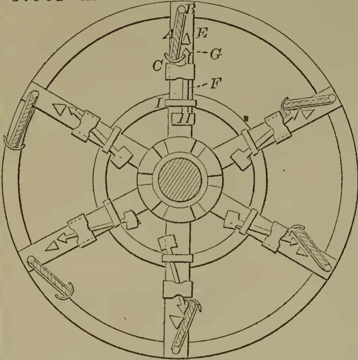
57901—A. Heuston—Paddle Wheel.
