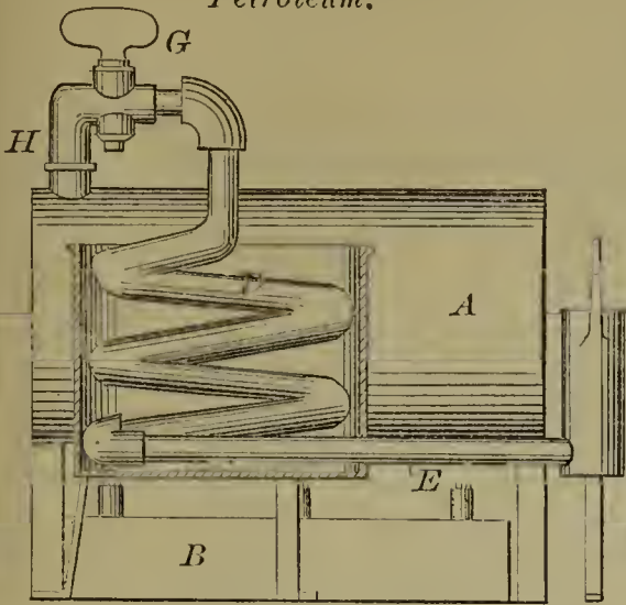
54157—A. D. Higham— Distilling Petroleum.
