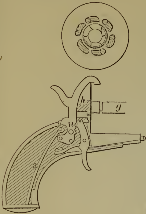
53548—P. Polain— Revolving Fire Arm.
