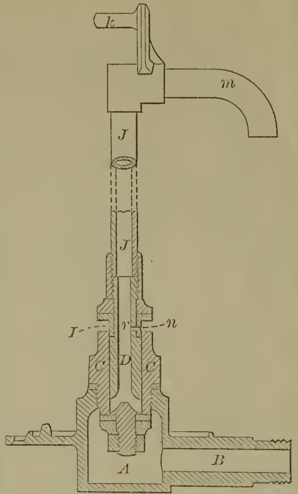
55782—Pixley & Robertson—Hydrant.
