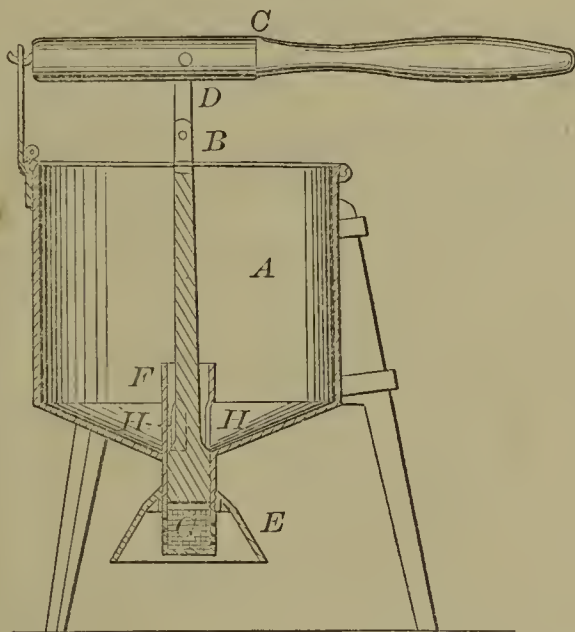
52661—L. Bishop—Press and Strainer for Cream Paste.
