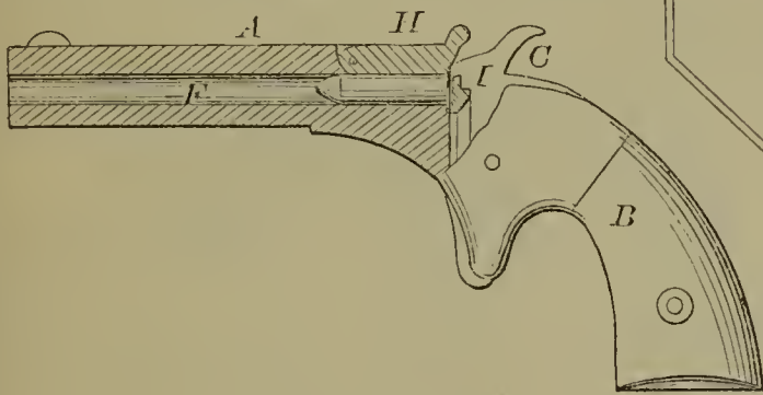
54500—H. Reynolds— Breech-Loading Fire Arm.
