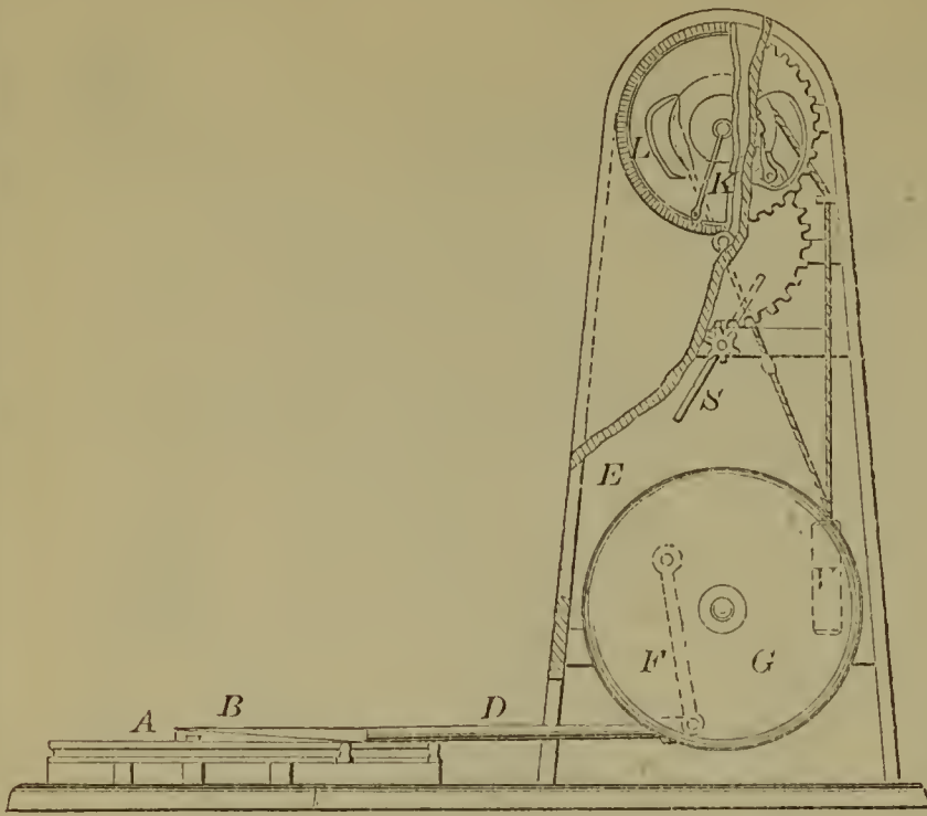
59688—W. J. Walker—Apparatus to be attached to Stills to prevent frauds on the Revenue.
