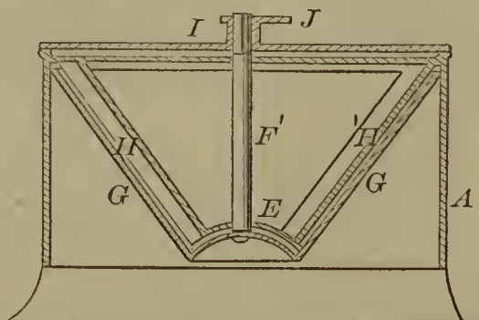
52729—W. C. McGill—Flour Sifter.
