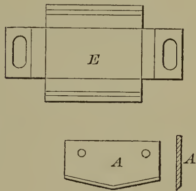
59944—R. T. Barton—For Making Paper Boxes.
