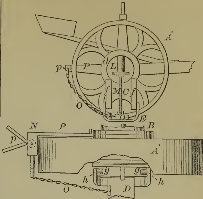
54392—Nevergold & Stackhouse— For Raking and Loading Hay.
