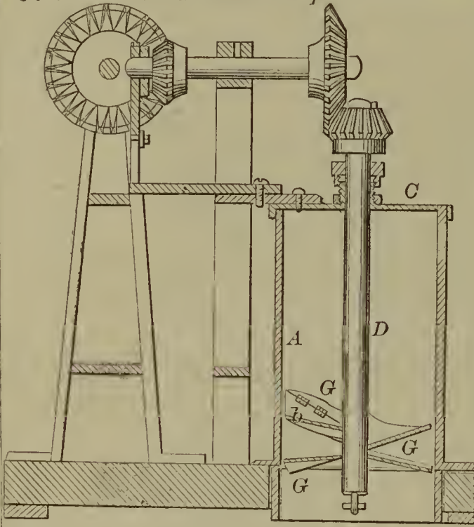
57499—J. P. Gruber—Pump.
