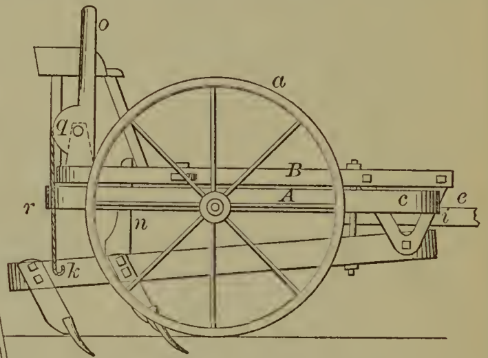
52998—I. Henton—Cultivator.
