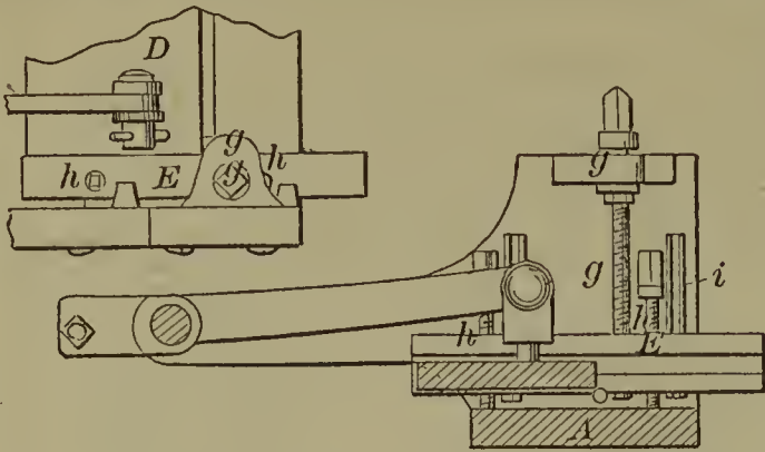
60260—R. Safely—For Straightening Shafting.
