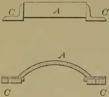
59371—J. E. Earle— Furniture Pad.
