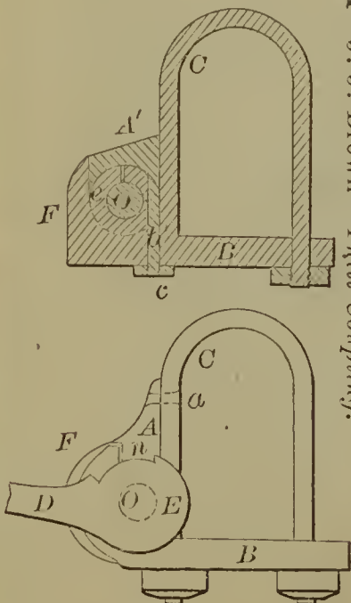
57848—W. M. Beeman—Register for Regulating Time Keepers.
