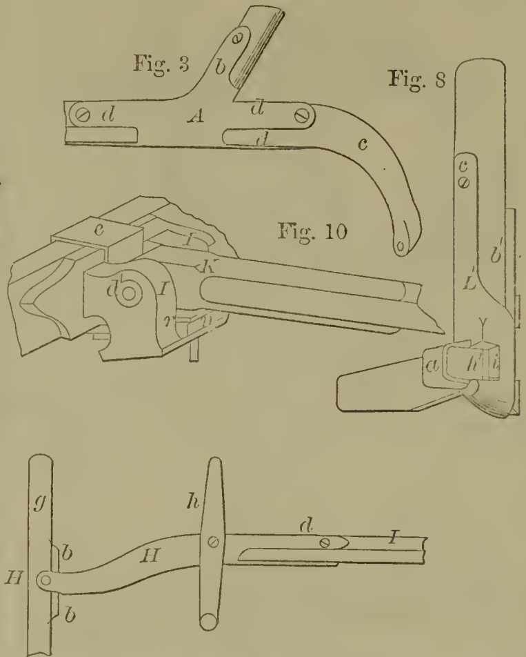
52601—J. S. Preston— For Raking and Loading Hay.
