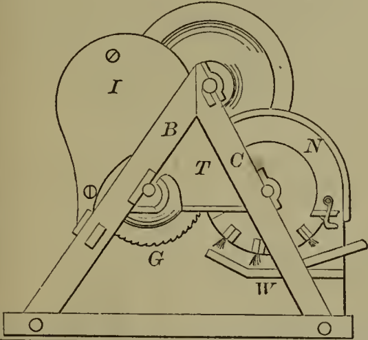
53912—E. P. Whitecomb—Churn.
