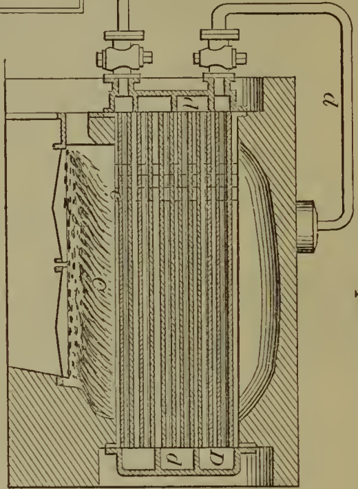
52982—L. V. Fichet—Steam Superheater.
