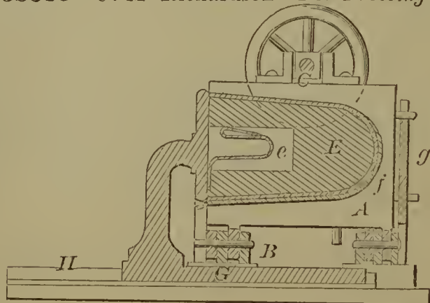
58555—G. M. Richardson—For Pressing Bonnets.
