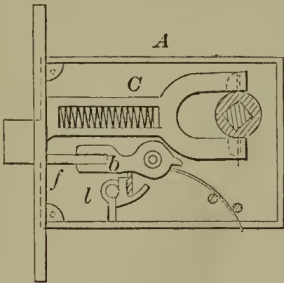
58688—A. W. Snow—Lock.
