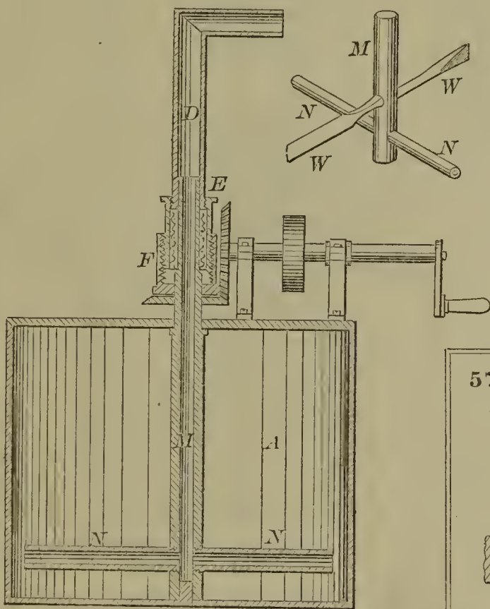
57285—Burket & Gray—For Treating Petroleum.
