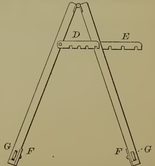
53705—S. I. Trask— Clothes Dryer.
