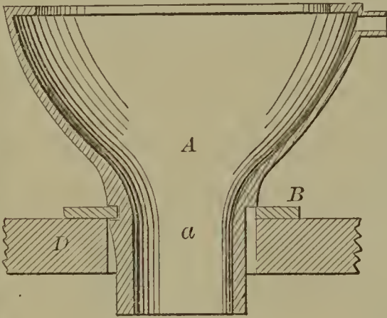
60153—R. Diven— Privy Bowl. Flange.
