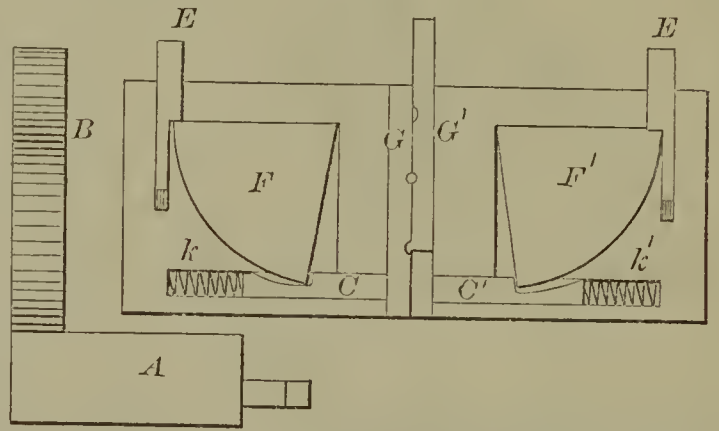
52218—E. Smith—Saw Set.
