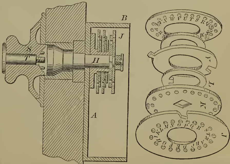
53959—W. B. Dodds— Lock.
