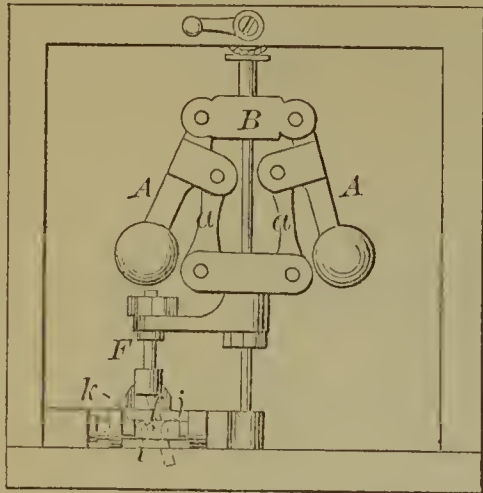
54336—W. J. Hallefas— Engine Governor.
