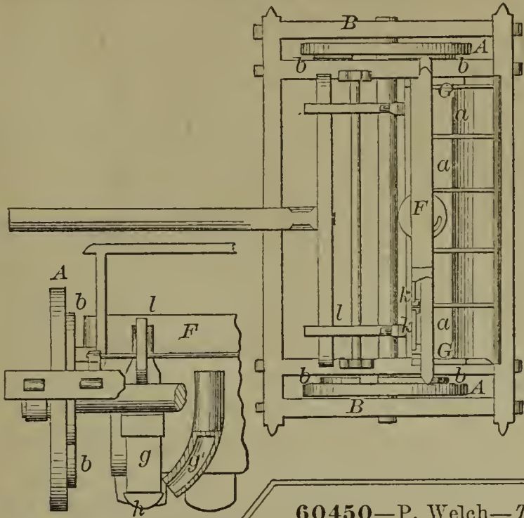
60447—J. C. Walkinshaw— Corn Planter.
