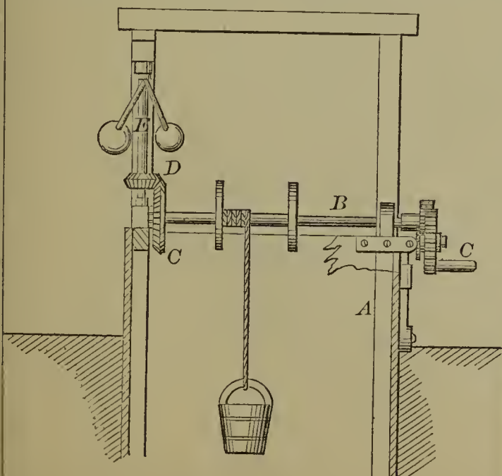
54334—C. Gullmann—Well Curb.
