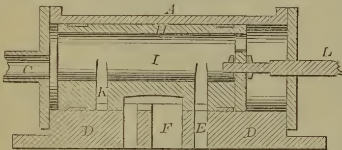
59096—J. Trent— Balanced Steam Valve.
