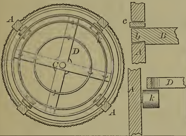
53504—W. Thompson— For Carburetting Air.
