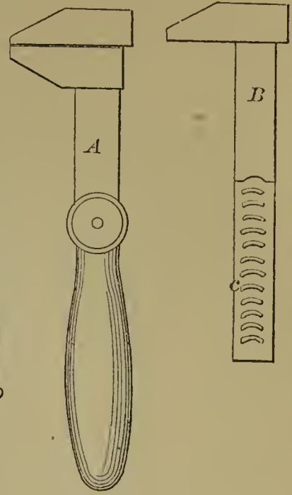
54888—G. P. Ganster—Wrench.
