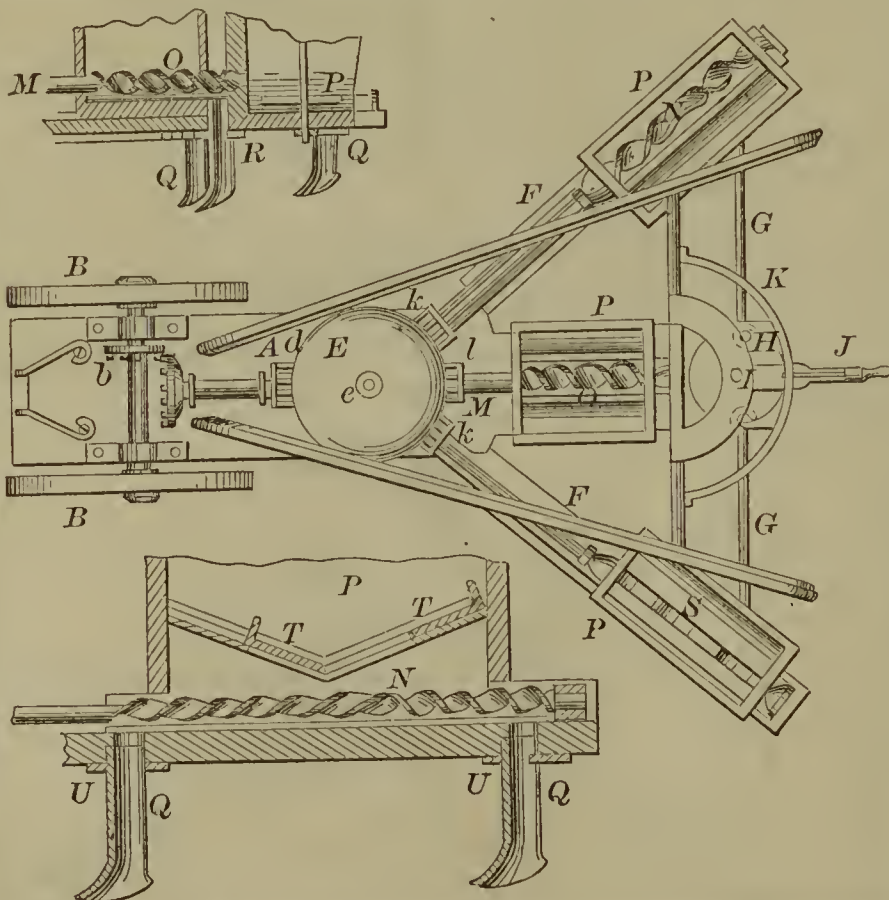
56664—G. Zorger—Wheat Drill.
