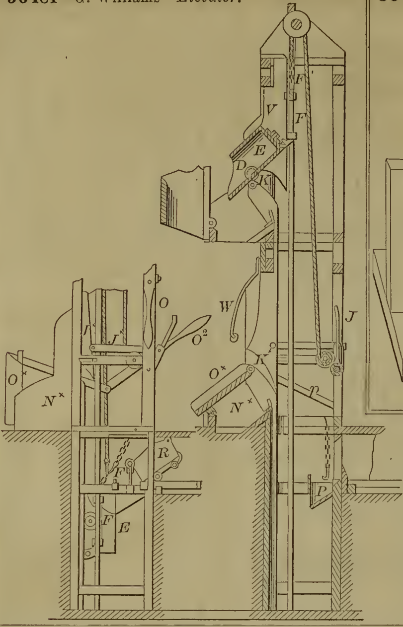
56481—G. Williams—Elevator.
