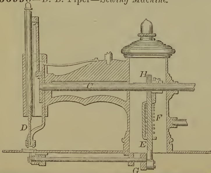
56990—D. B. Piper—Sewing Machine.
