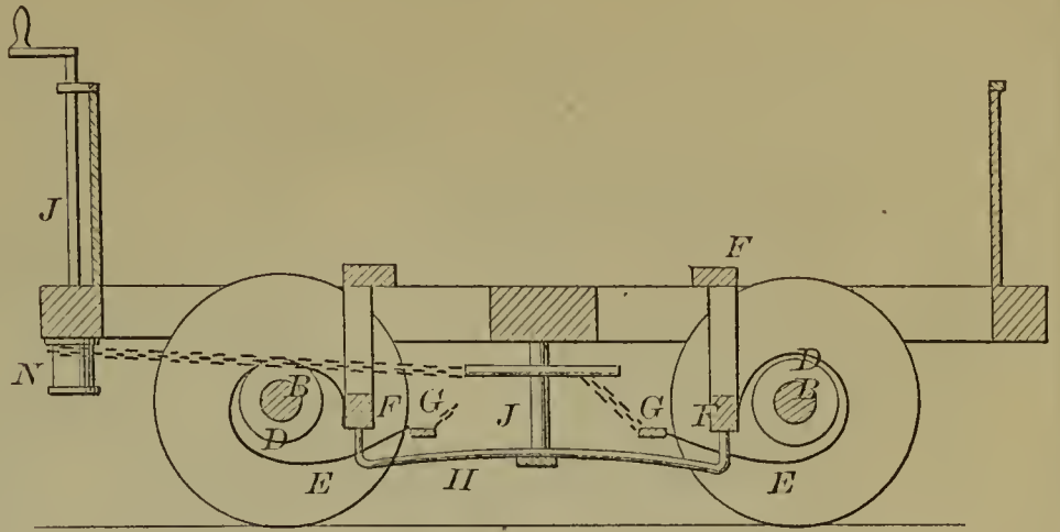
53365—W. Warner— Car Brake.
