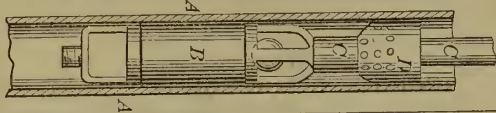
56430—I. W. McGaffey— Cotton Seed Planting Machine.
