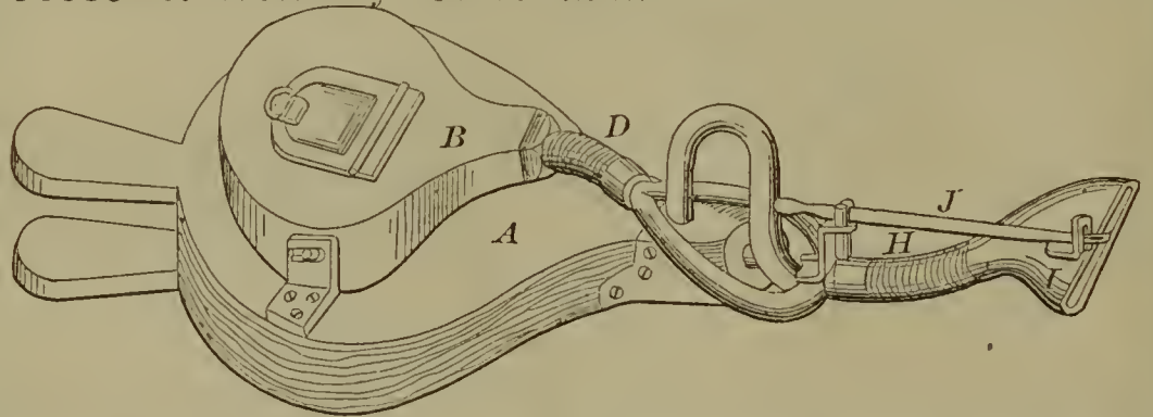
56558—J. W. Hendley—Sand Bellows.
