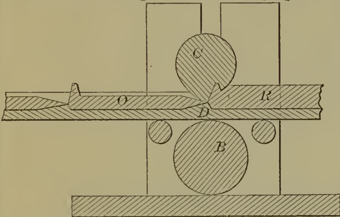
54610—Seeley & Jacobie— Brick Machine.
