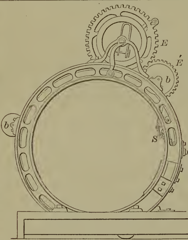
57904—S. T. Holly—Grain Binder.
