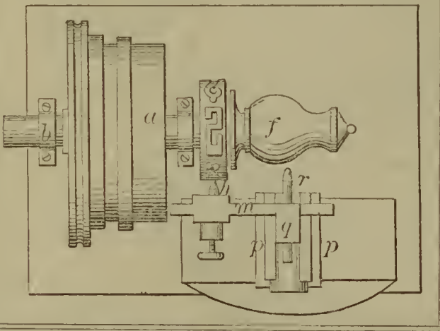
57158—T. Lippiatt—Rose Engine Lathe.
