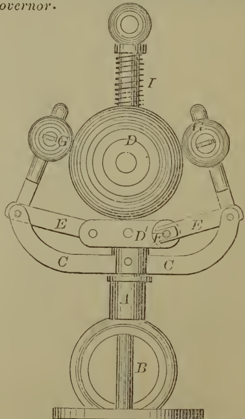
56956—T. S. La France— Steam Engine Governor.
