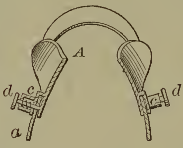
58121—J. Meyer—Saddle.
