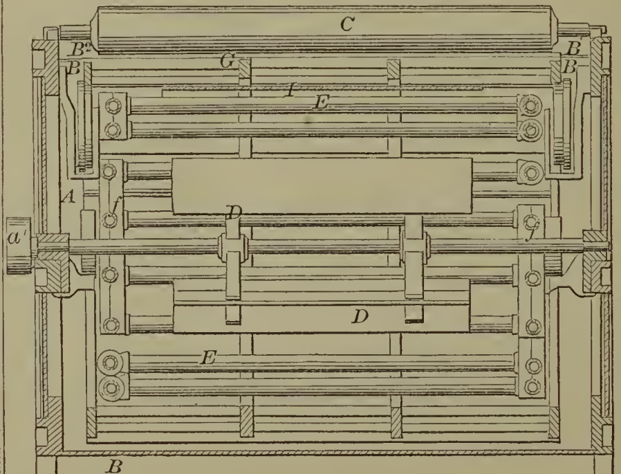
60103—H. Whitehill— For Drying Yarn.
