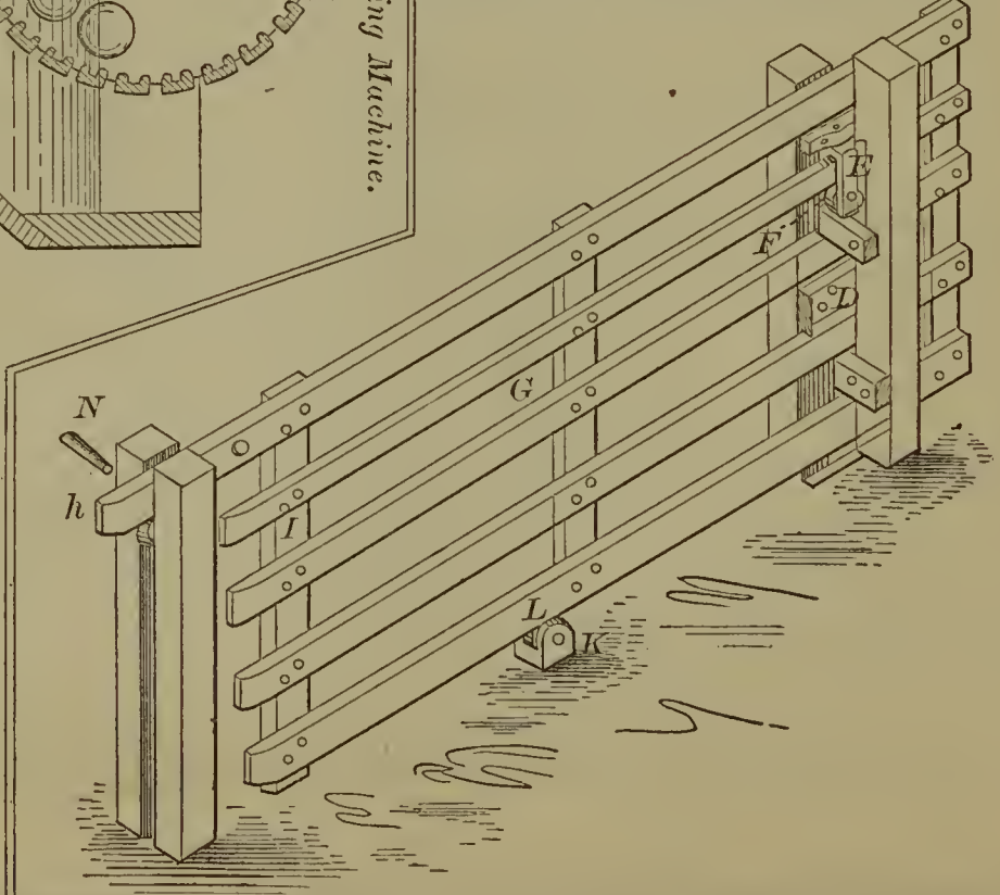
53053—W. Snyder—Farm Gate.
