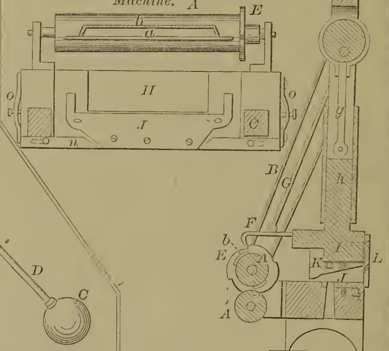
59410—H. F. Knapp—Paper Collar Machine. A
