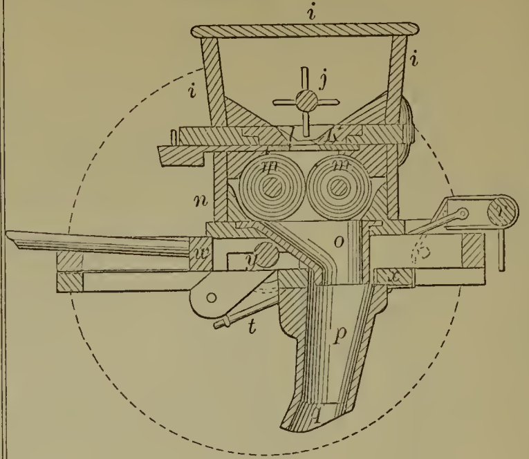
55184—L. N. Warren— Grain Drill.
