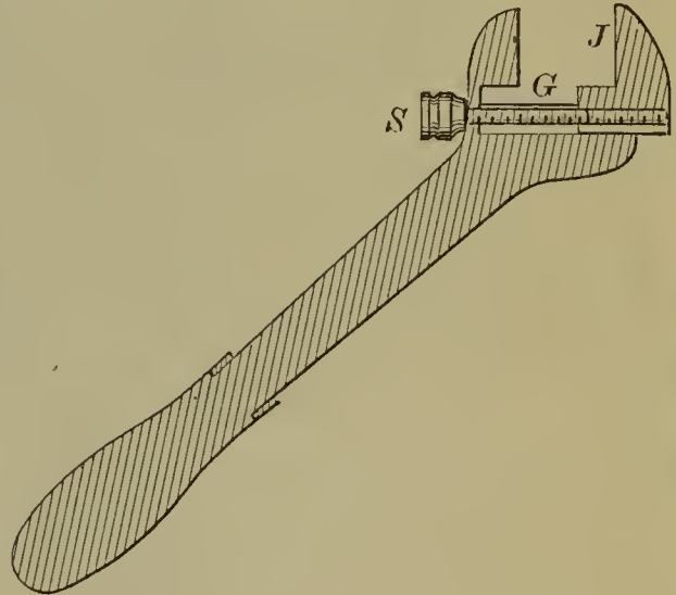
53016—H. W. Love— Screw Wrench.
