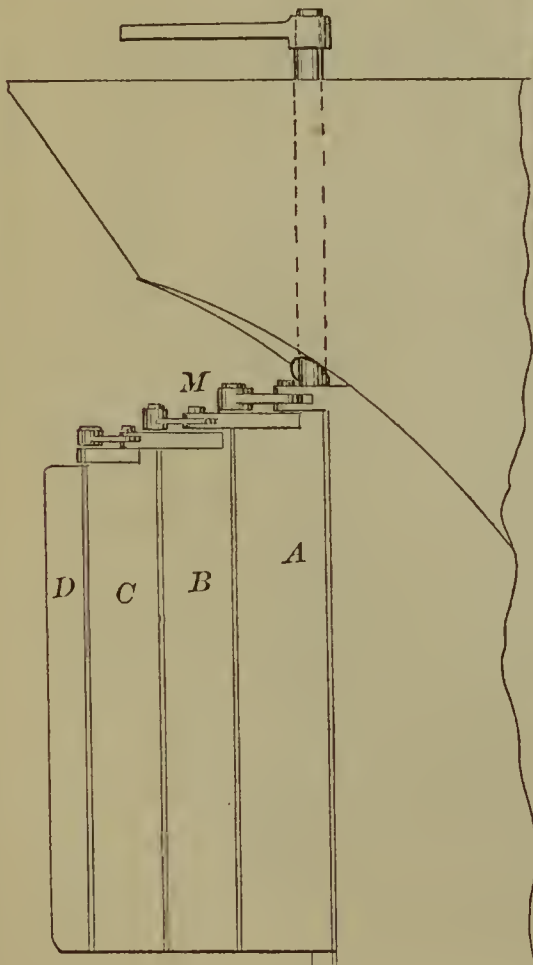
53936—M. W. Ruthven— Rudder.
