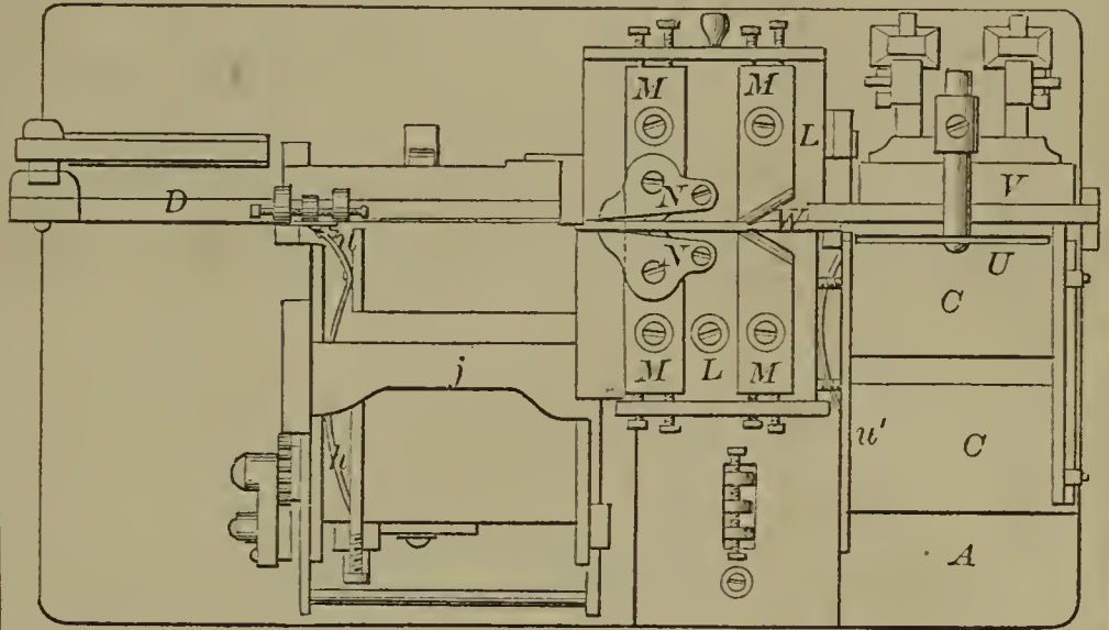
60450—P. Welch— Type Dressing Machine.
