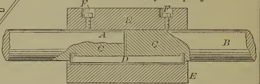
55200—P. Crowl— Vise.
