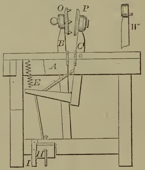
57522—J. D. Leach—For Holding the Heads of Casks.
