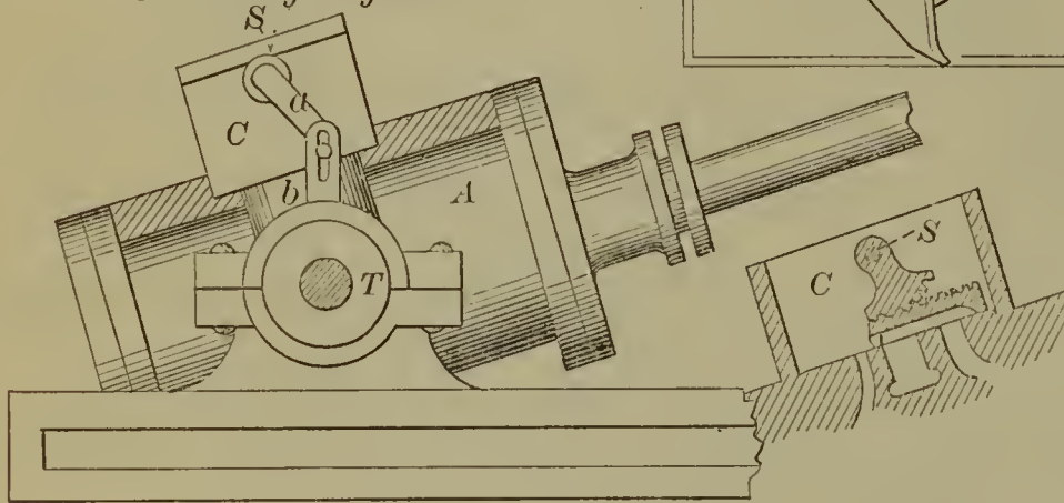
53570—H. T. Carter— Valve Gear for Oscillating Engines.
