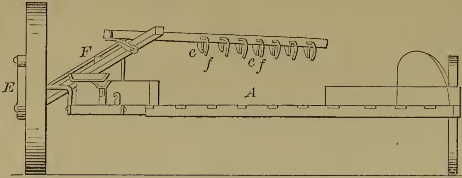
55060—P. C. Chipron—Harvester Rake.
