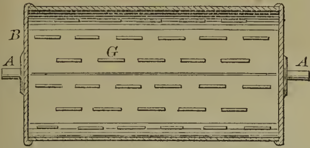
57907—S. D. Horton— Founders' Cleansing Mill.
