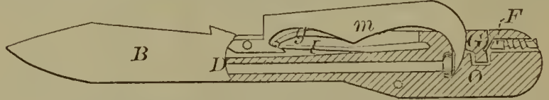
53473—A. J. Peavey— Combined Pistol and Pocket Knife.
