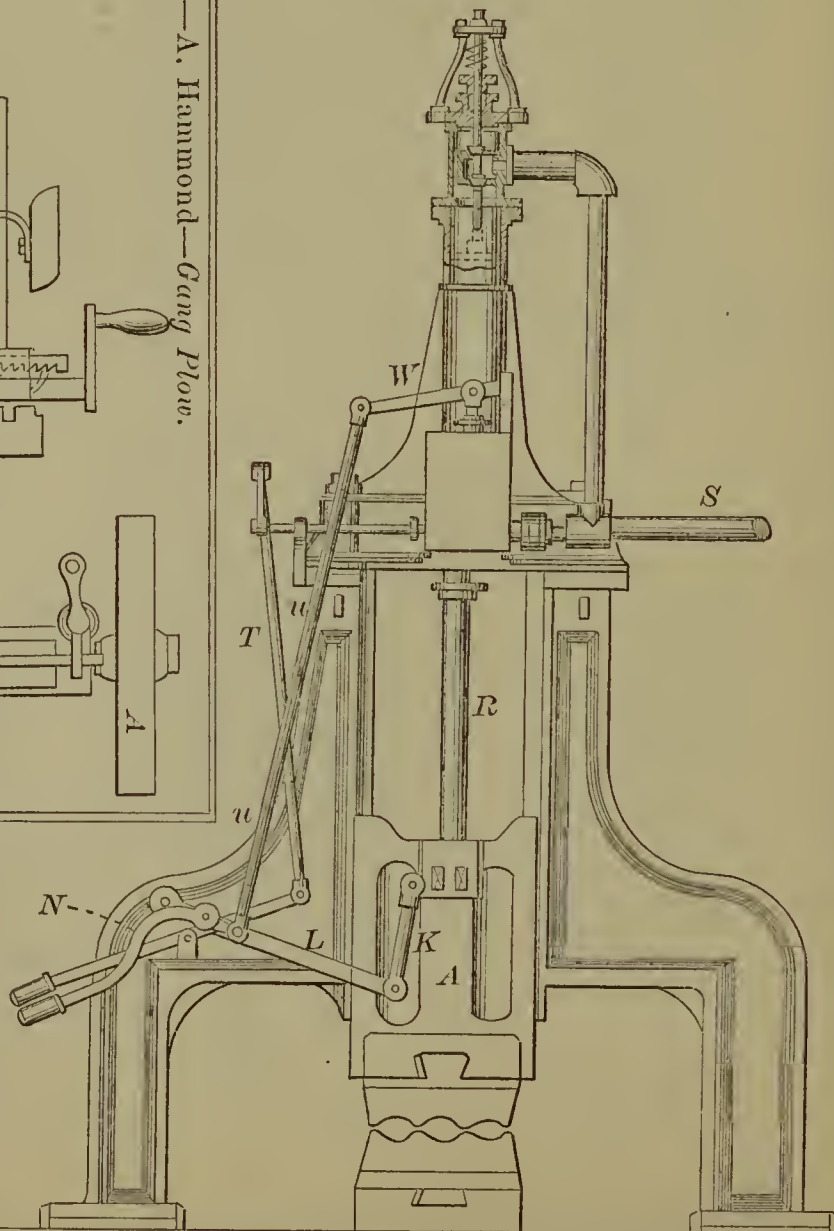
53442—H. Hamilton—Valve Gear for Steam Hammers.
