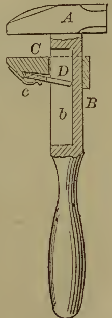
56147—A. M. Olds—Wrench.
