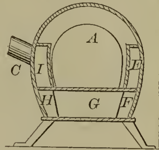
56649—T. White— Stove.
