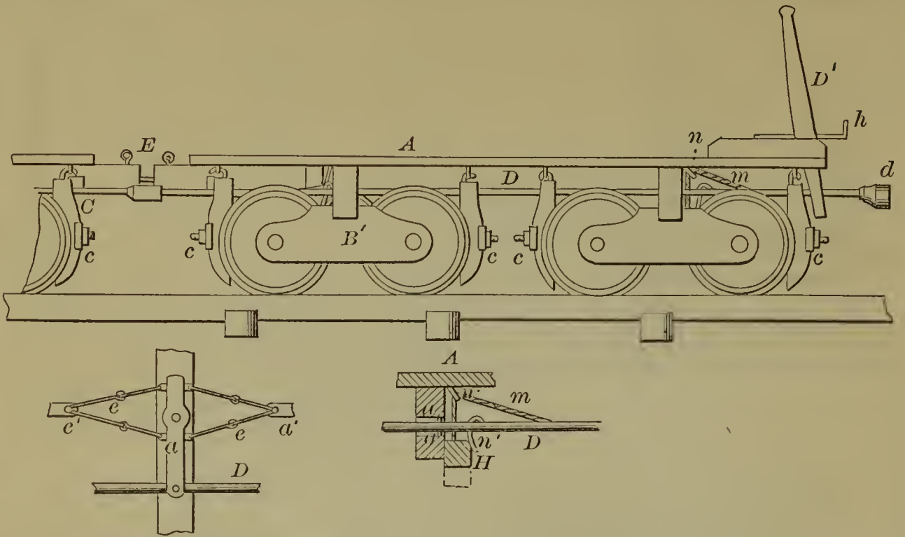
53006—M. Ingersoll— Railroad Car Brake.
