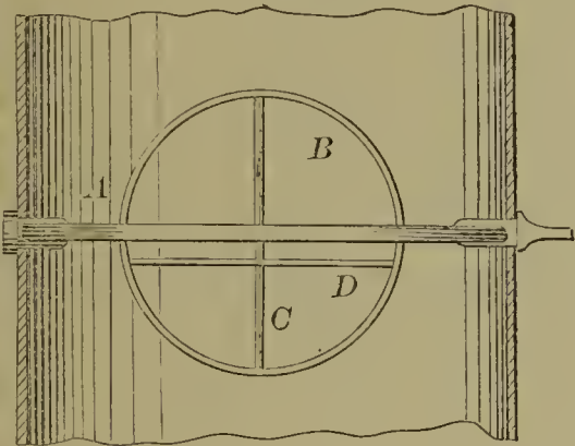
58233—N. J. Eldred— Stove Pipe Damper.
