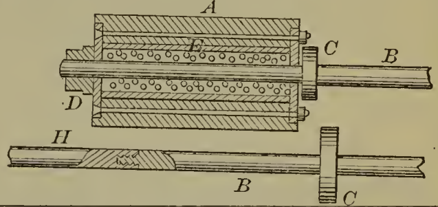
53189—I. M. Rose— Drilling and Driving Machine.
