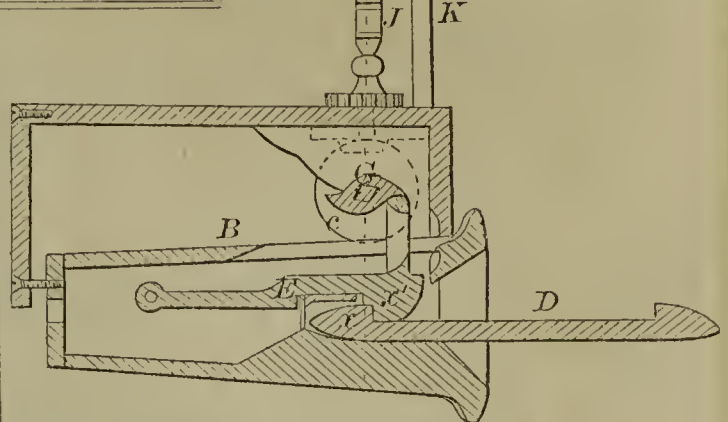
57401—T. H. Spencer—Blacking Box.
