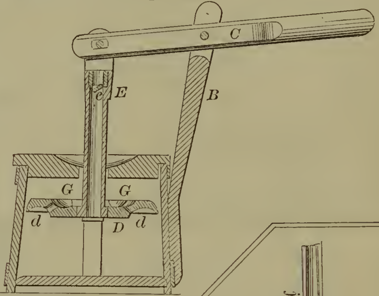
56661—J. Young—Churn.
