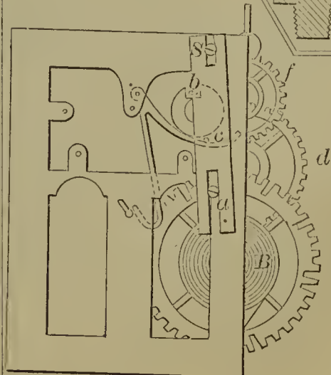
57843—B. Bacon—Striking Works for Clocks.
