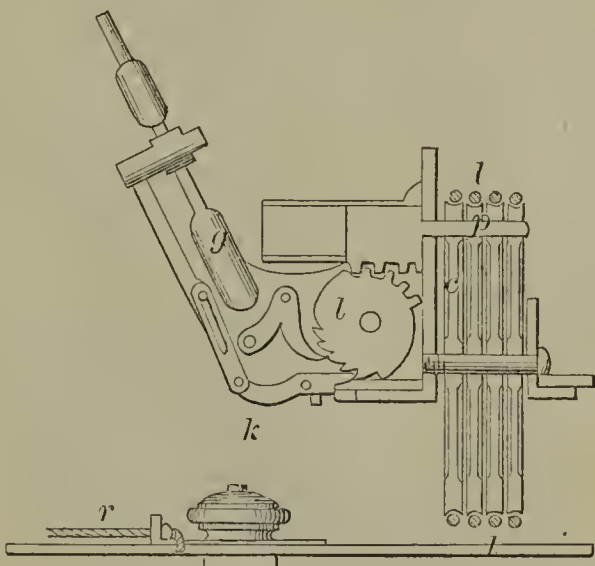
51804—C. C. Clapp— Book Leaf Turner.
