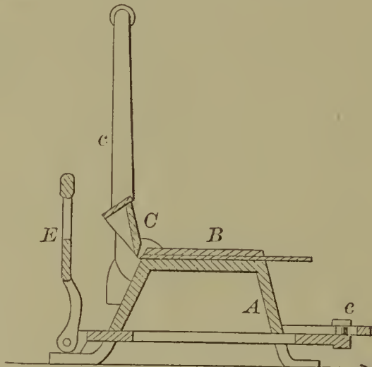
54341—W. H. Henderson— Tinman's Forming Tool.
