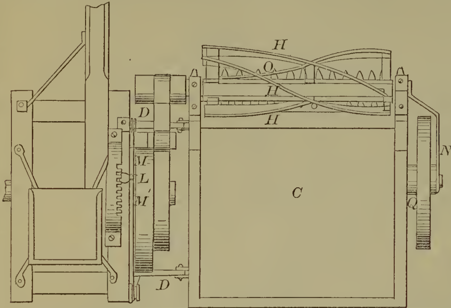
54370—E. Kramer—Clover Harvester.
