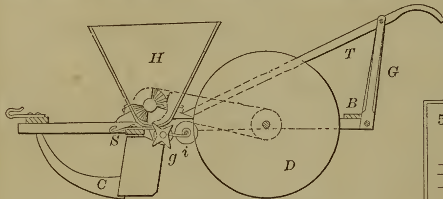
56430—I. W. McGaffey— Cotton Seed Planting Machine.
