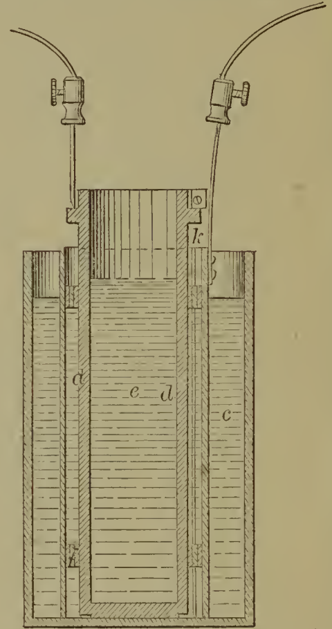
57687—J. Dixon—Galvanic Battery.
