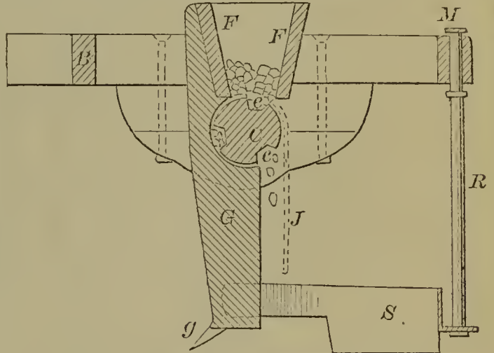
54633—M. Wilkinson— Corn Planter.
