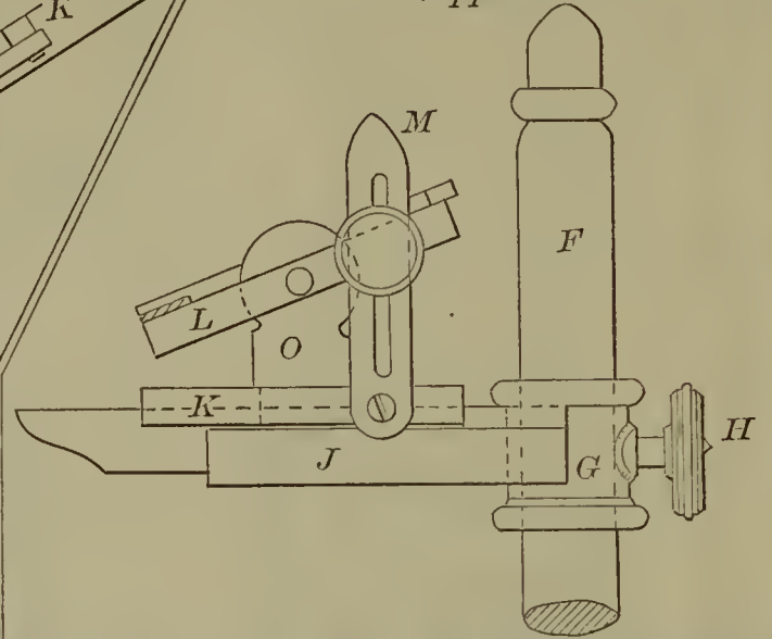
55525—E. Müller—Photographic Apparatus.
