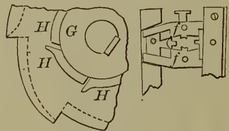
52998—I. Henton—Cultivator.
