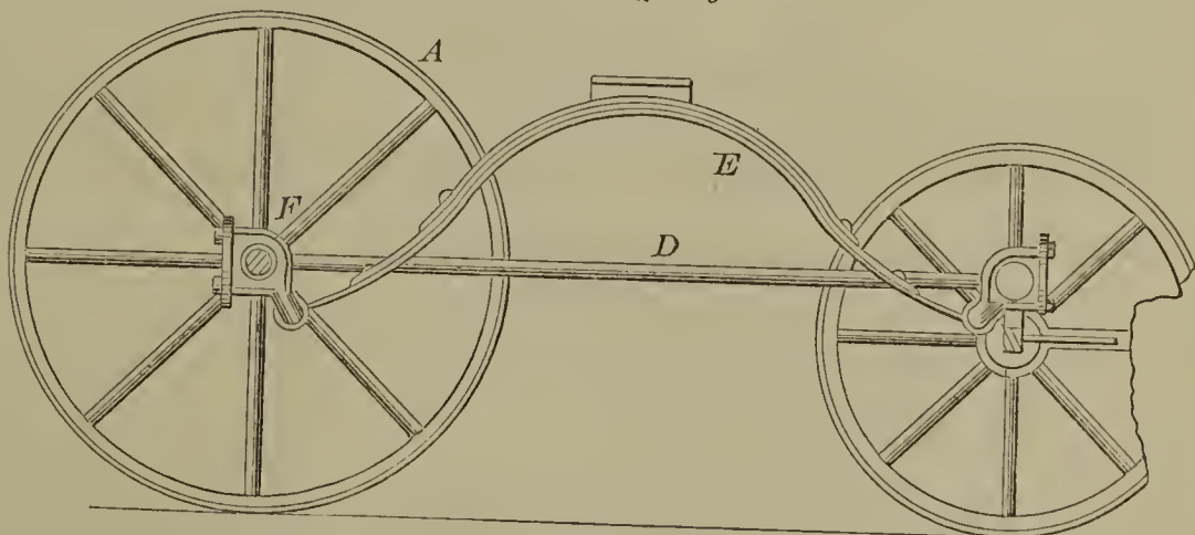
55985—B. M. Beckwith—Carriage Spring.
