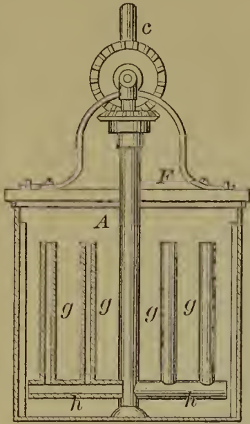
53126—K. W. Doudna—Broom Corn and Sorghum Stripper.
