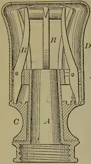
53175—C. Oyston— Nozzle for Fire Engines.
