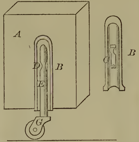
52420—Kane & Brown—Caster for Furniture.
