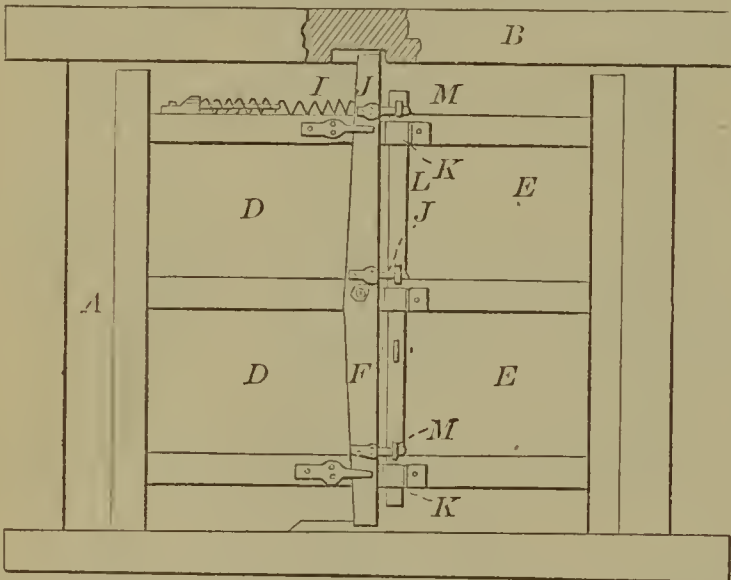
59248—D. N. Minor—Baru Door Fastening.
