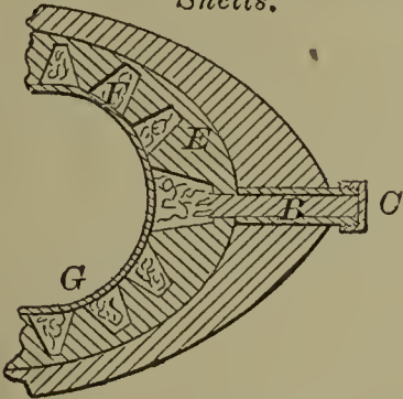
60567—T. P. Shaffner— For Charging Shells.
