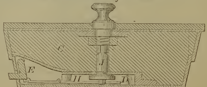
57040—W. B. Dodds—Safe Lock.
