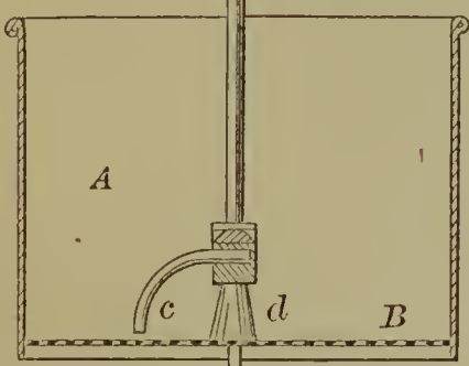
56318—R. M. Yorks—Washing Machine.
