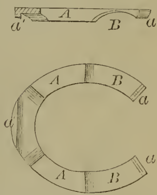
57033—D. Winer—Propelling Apparatus for Vessels.
