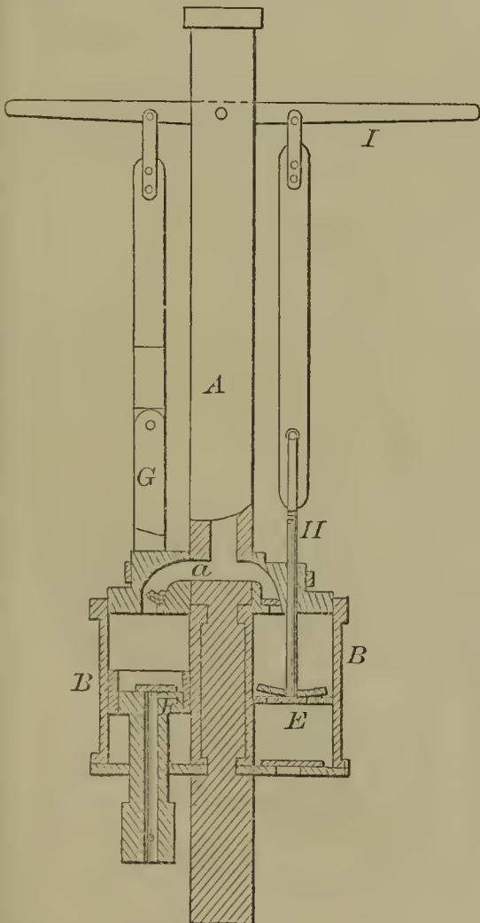
52485—L. Beemer— Pump.
