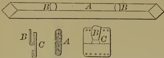
58173—E. C. Little—Moulders' Flask.
