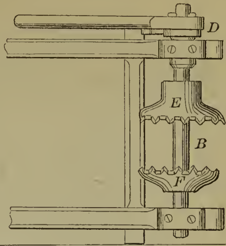
59641—S. Perry—Sawing Machine.
