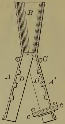
53964—L. V. Fiehet—Distilling Petroleum.
