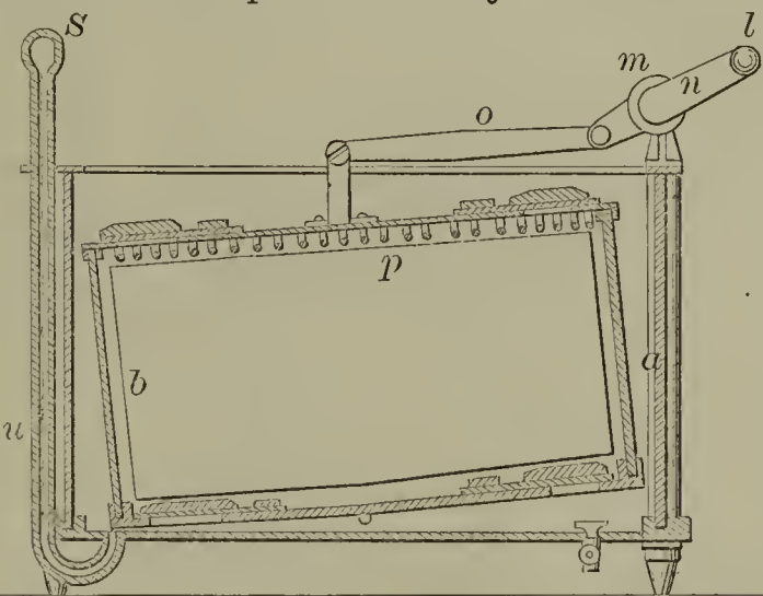
51872—E. Shopbell— Upsetting Wagon Tire.
