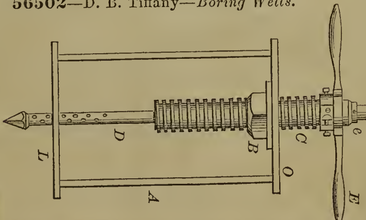
56502—D. B. Tiffany—Boring Wells.
