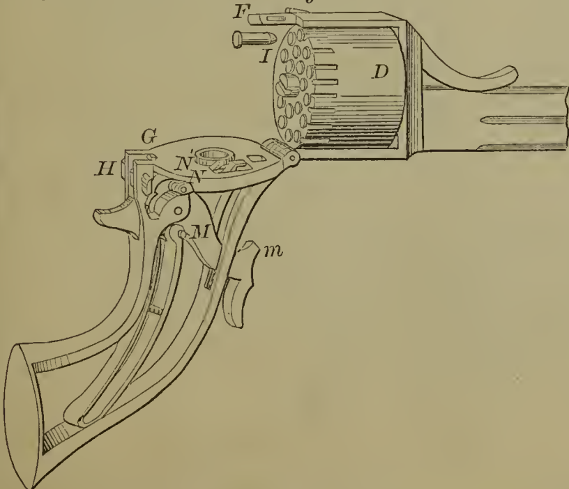
57864—A. Christ—Revolving Fire Arm.
