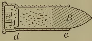
55676—T. T. S. Laidley— Priming Metallic Cartridges.
