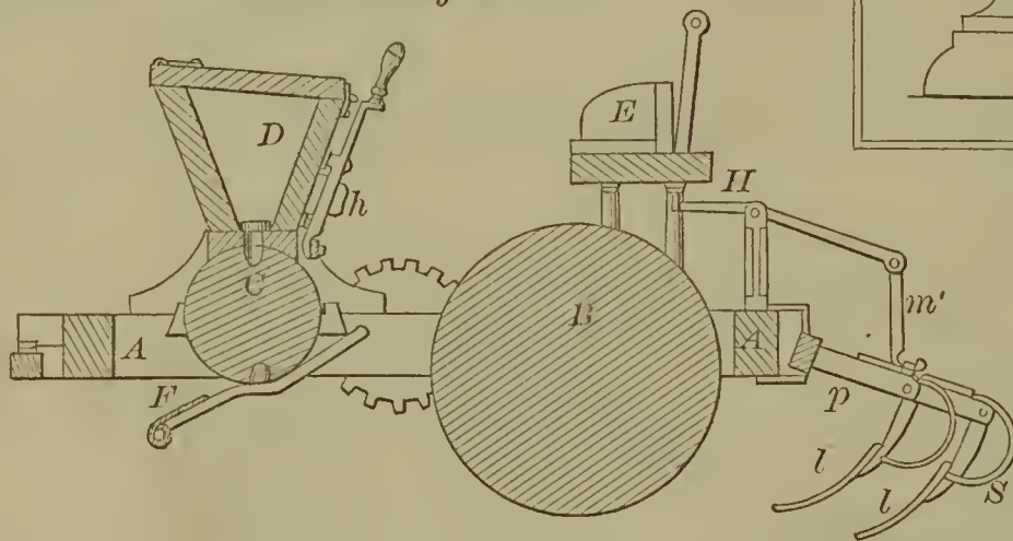
52445—J. B. Pitts—Seeding Machine.
