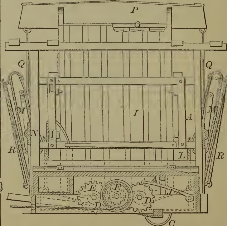
52911—C. H. Thatford—Baking Press.
