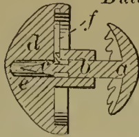
54071—C. Robitaille—Button.
