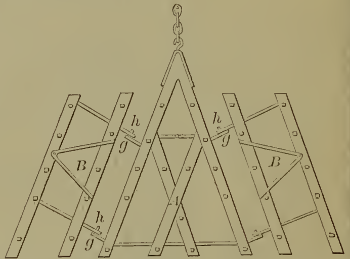
57851—E. Bradley—Harrow.
