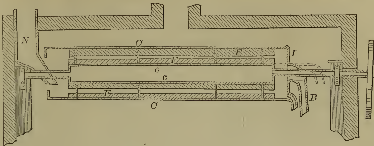
56255—J. Norton, 3d— Grain Dryer.
