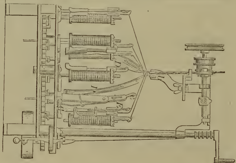
57326—Howe & Mackrell— Braiding Machine.
