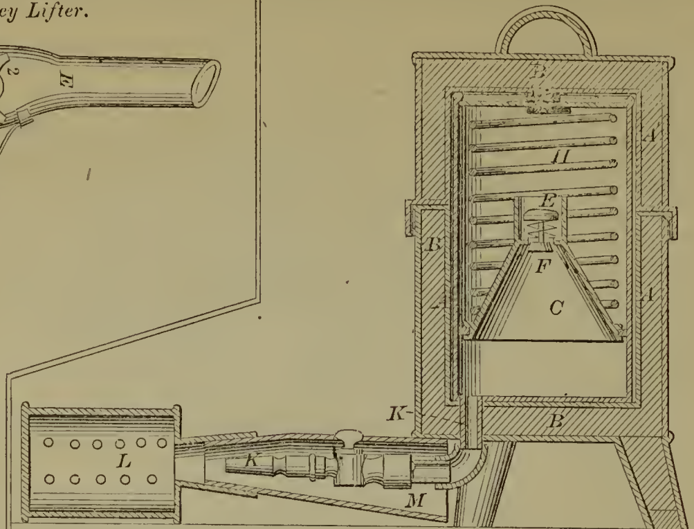
54243—R. Yoilding—For Burning Tar.
