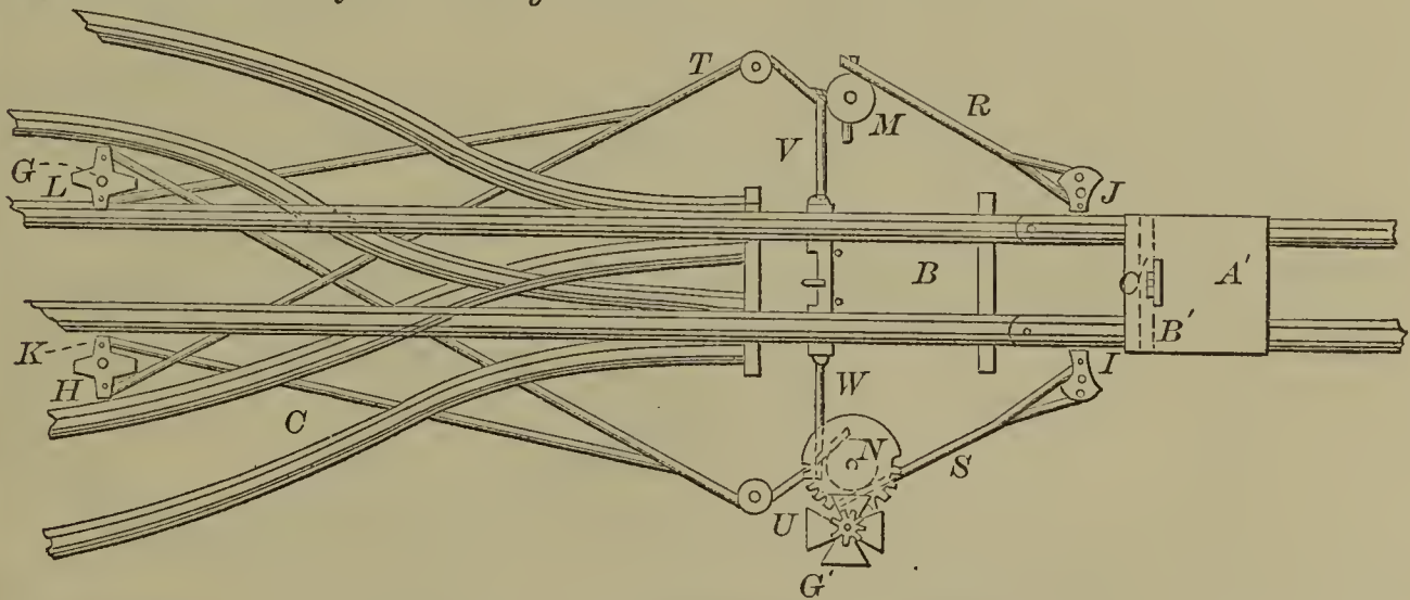
54513—J. E. P. Doyle—Railway Switch.
