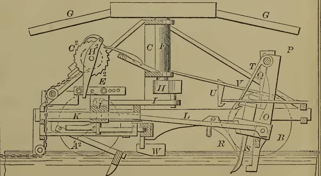
58413—E. Heath—Ditching Machine.
