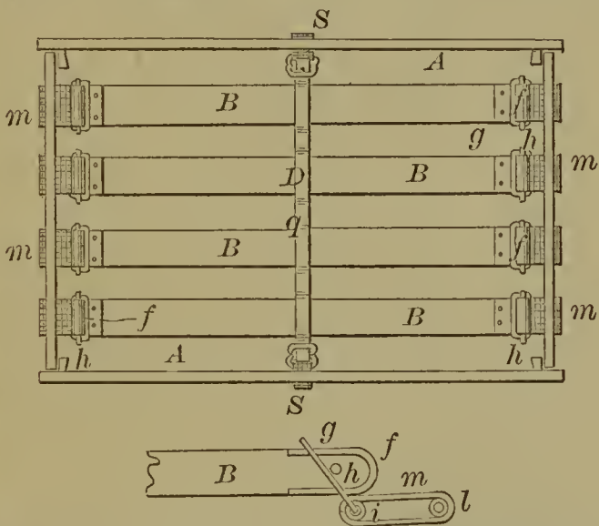
54880—D. C. Flint—For Stripping Cane.
