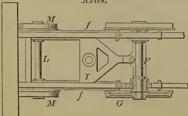
53009—J. P. Laird— Bearings of Locomotive Axles.
