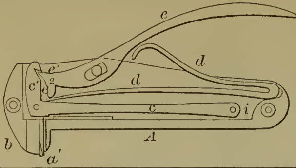
52921—A. Whittemore—Vaccinator.
