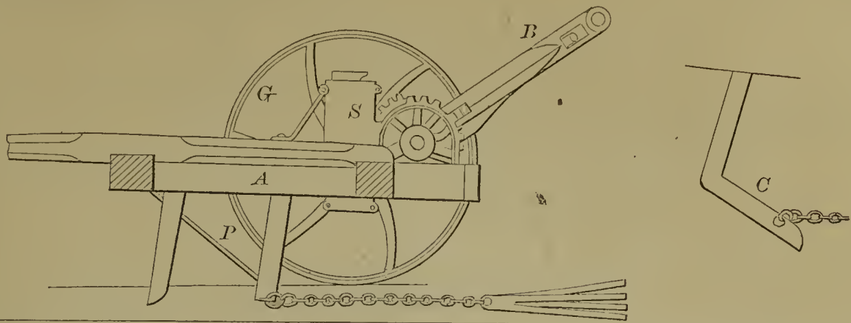
58143—S. Secrist— Corn Harvester.
