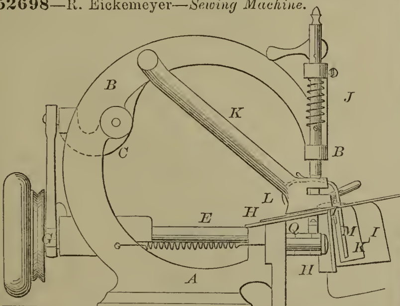
52698—R. Eickemeyer—Sewing Machine.
