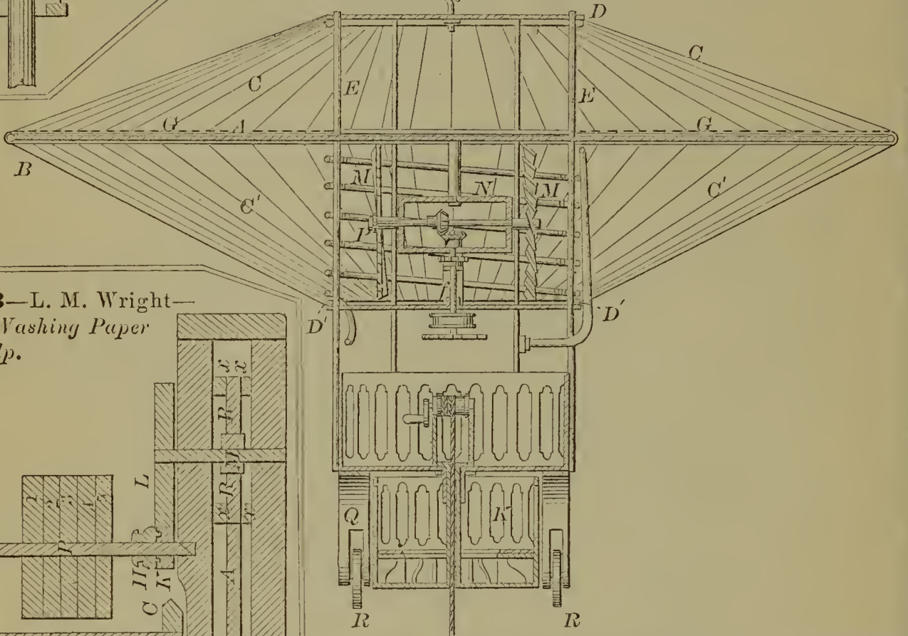
54994—C. E. Yager— Flour Sieve.
