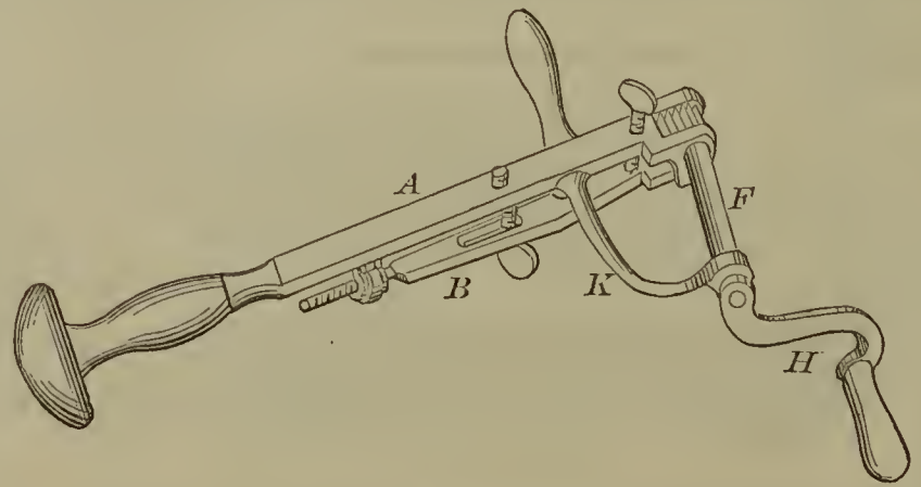
55617—E. A. Bushnell—For Sharpening Horse Shoe Culks.
