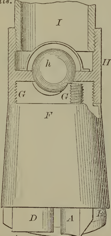
52164—J. Grieves—Drill for Wells.
