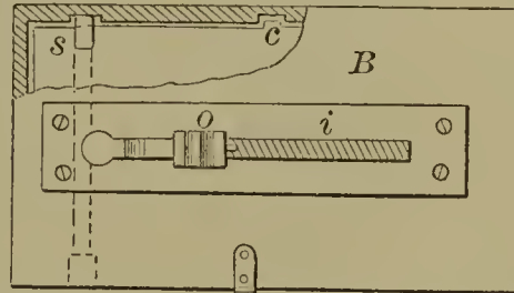
58359—Petrie & Teal— Wool Washing Machine Lifting Cylinder.
