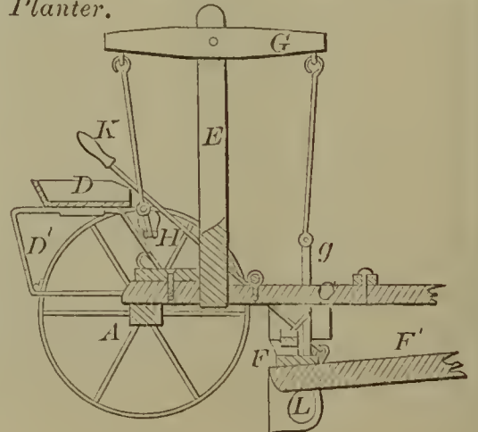
58798—J. M. Fate—Corn and Cane Planter.
