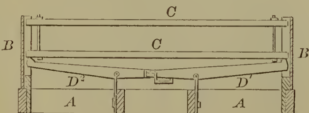
56976—C. Miller—Harness Motion for Looms.
