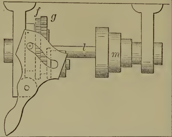
54522—J. L. Fountain— Attaching Cultivator Blades.
