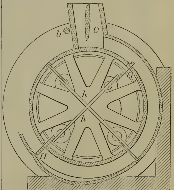
52259—M. Bell—Water Wheel.
