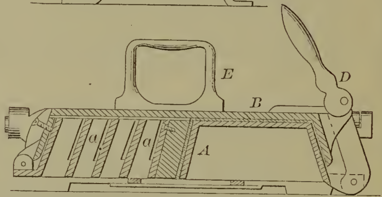
54342—W. H. Henderson— Tinman's Edging Tool.
