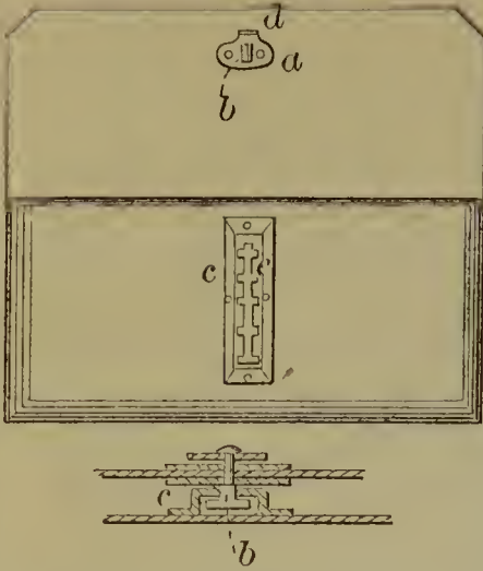
53524—C. Crow—Trammel for Ellipses.
