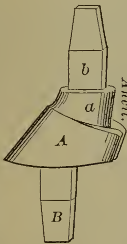
56313—S. R. Wilmot— Die for Forming Sheet Metal Vessels.
