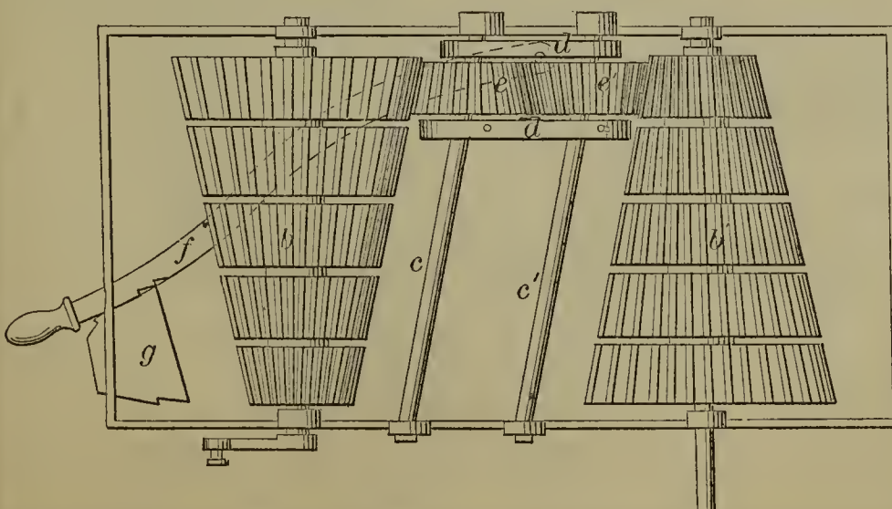
53202—J. H. Wait— Device for Changing Speed.
