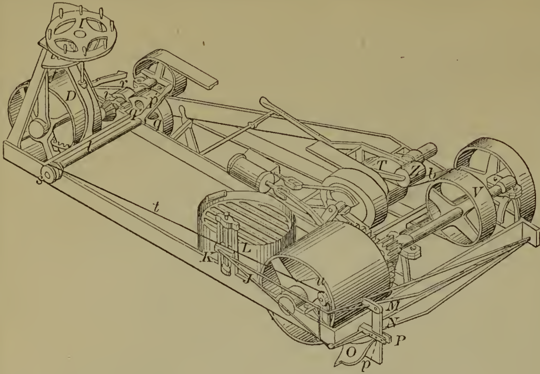
54224—G. Simonson— Steam Plow.
