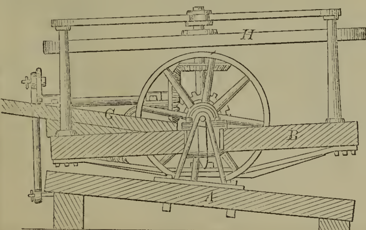
52287—J. H. Haven—Motive Power.
