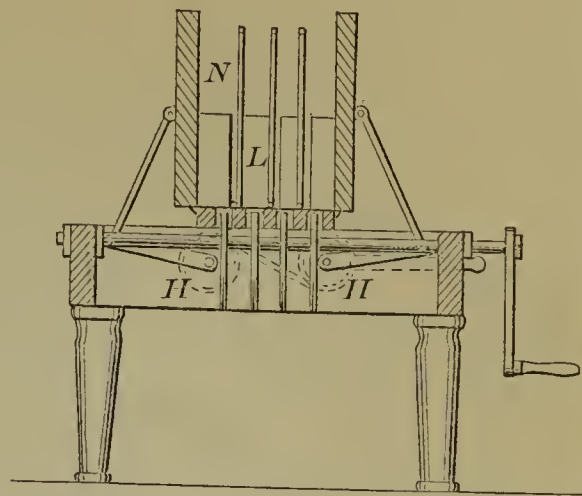
55118—R. Kitson—Picker House for Opening Cotton, &c.
