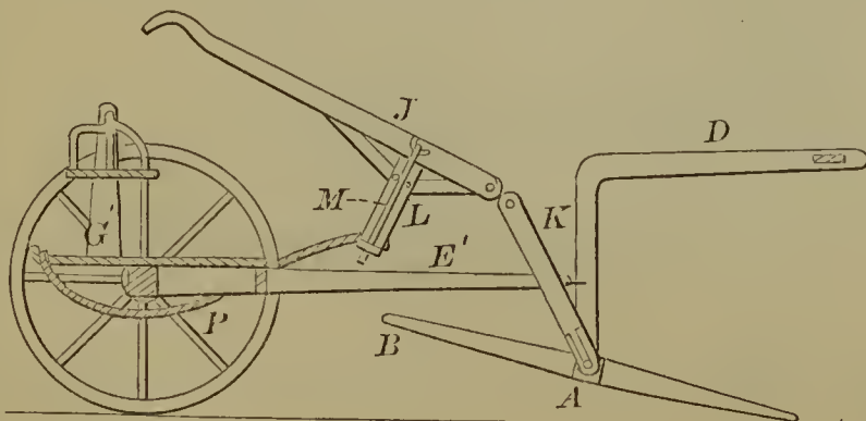
54947—W. M. Piatt—Horse Rake.
