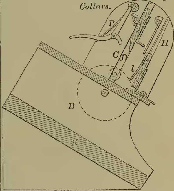
59684—H. Tucker—Venting Core for Foundry Purposes.
