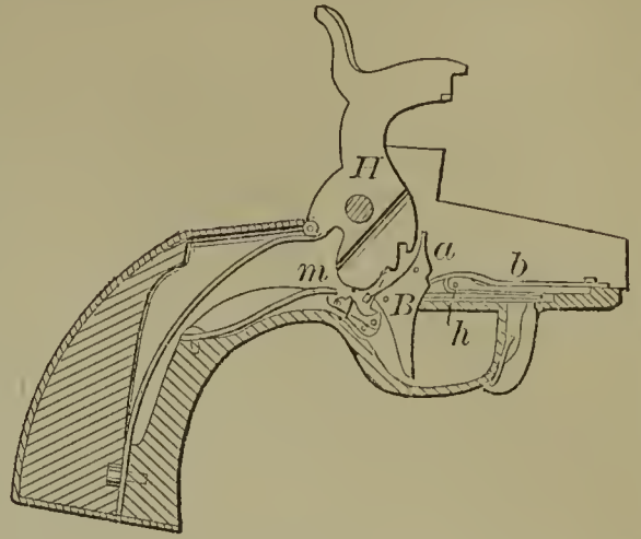
57978—F. Schenck—Gun Lock.
