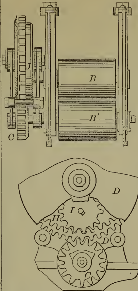
53235—J. B. Rumsey— Car Brake.
