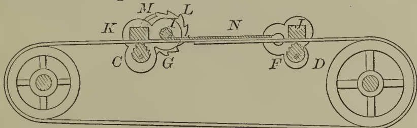
51970—S. Rogers—Belt Stretcher.
