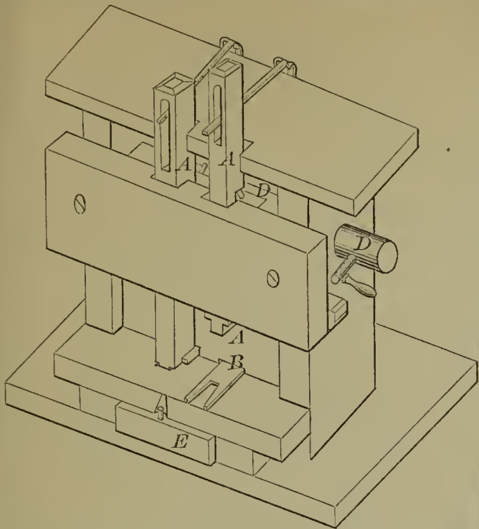
56744—W. Gowen—Washing Machine.
