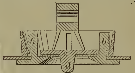
58087—H. R. Foote— Generating and Burning Vapor of Hydro Carbon Oil.
