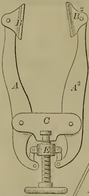
57447—A. C. Stockmar— Hand Vise or Clamp.
