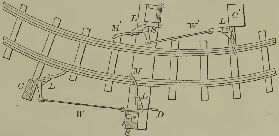
51952—A. W. Livingston—Railway Signal.
