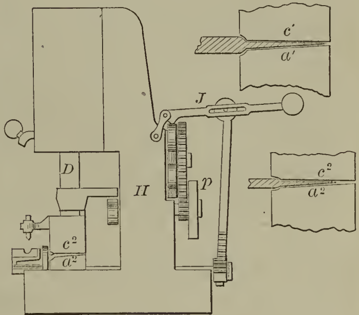
51986—J. A. Whitney—Horse Shoe Nail Machine.
