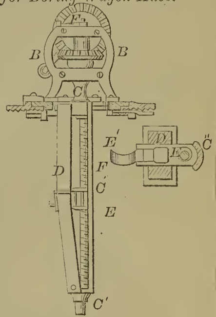
59417—S. Lavenue— Machine for Boring Wagon Hubs.
