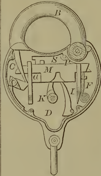
59615—E. Lawshe—Lock.
