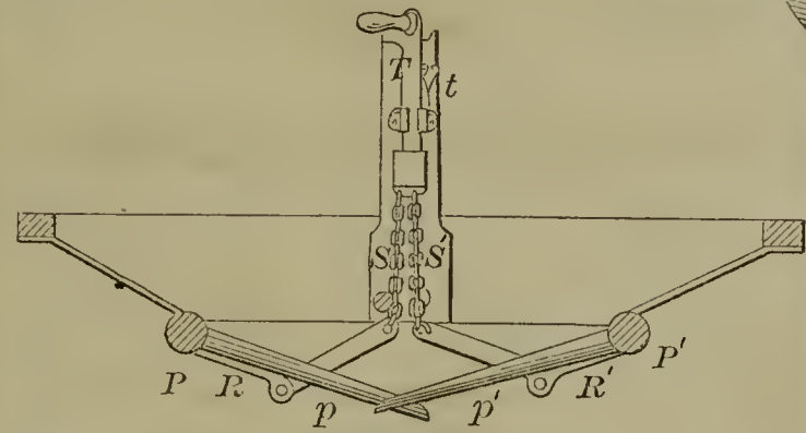
57361—T. A. Morley— For Cutting Corn from the Cob.
