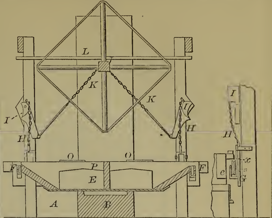
53033—D. Oliver—Hedge Cutting Machine.
