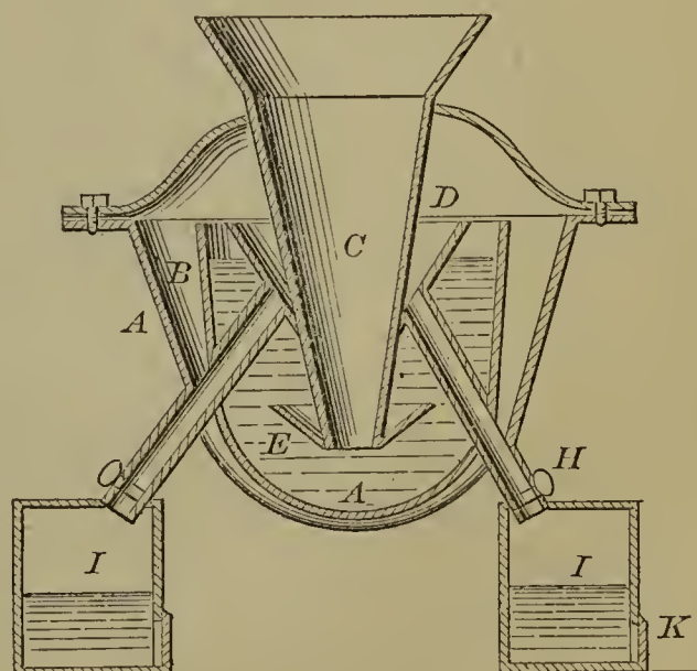
52846—E. Hamilton— Amalgamator.
