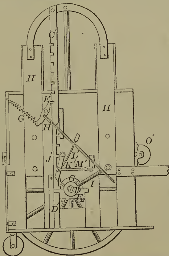
60323—W. C. Bartol—Brick Machine.
