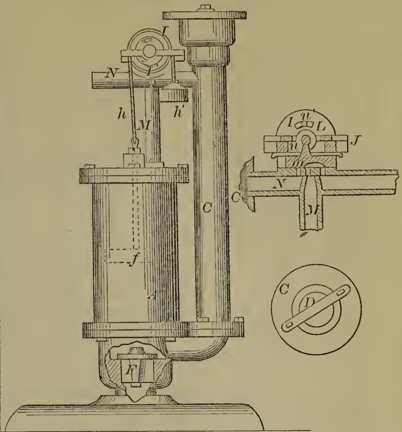
53170—J. C. Morgan— Steam Pump.
