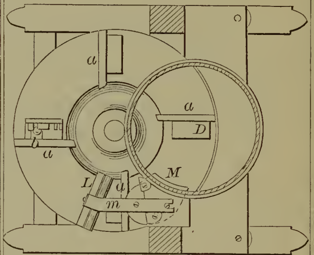
53980—Hotchkiss & Buss—Brick Machine.
