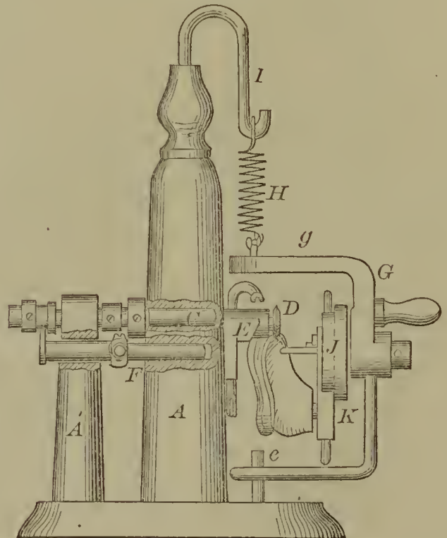
52498—Thompson & Tripp—Heel Polishing Machine.
