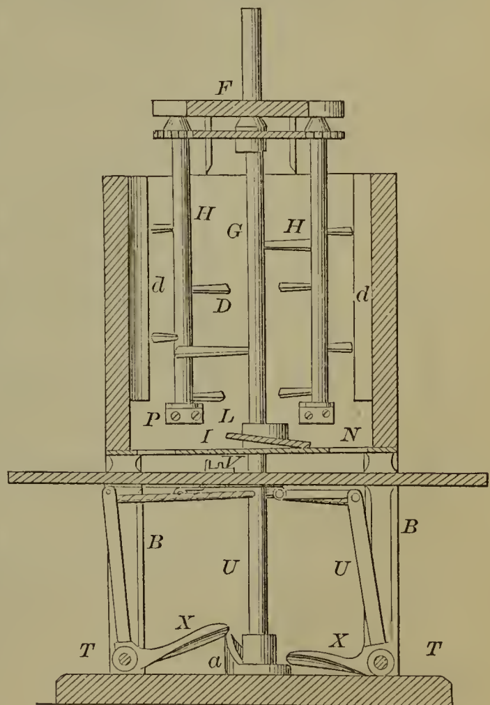
53868—B. Porter—For Grinding Clay.
