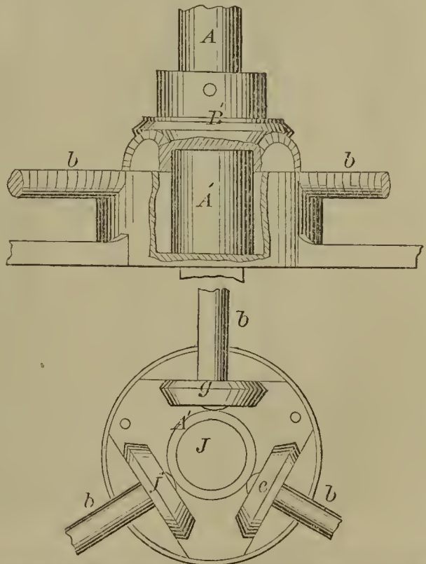
57319—T. Harper— For Boring Wagon Hubs.
