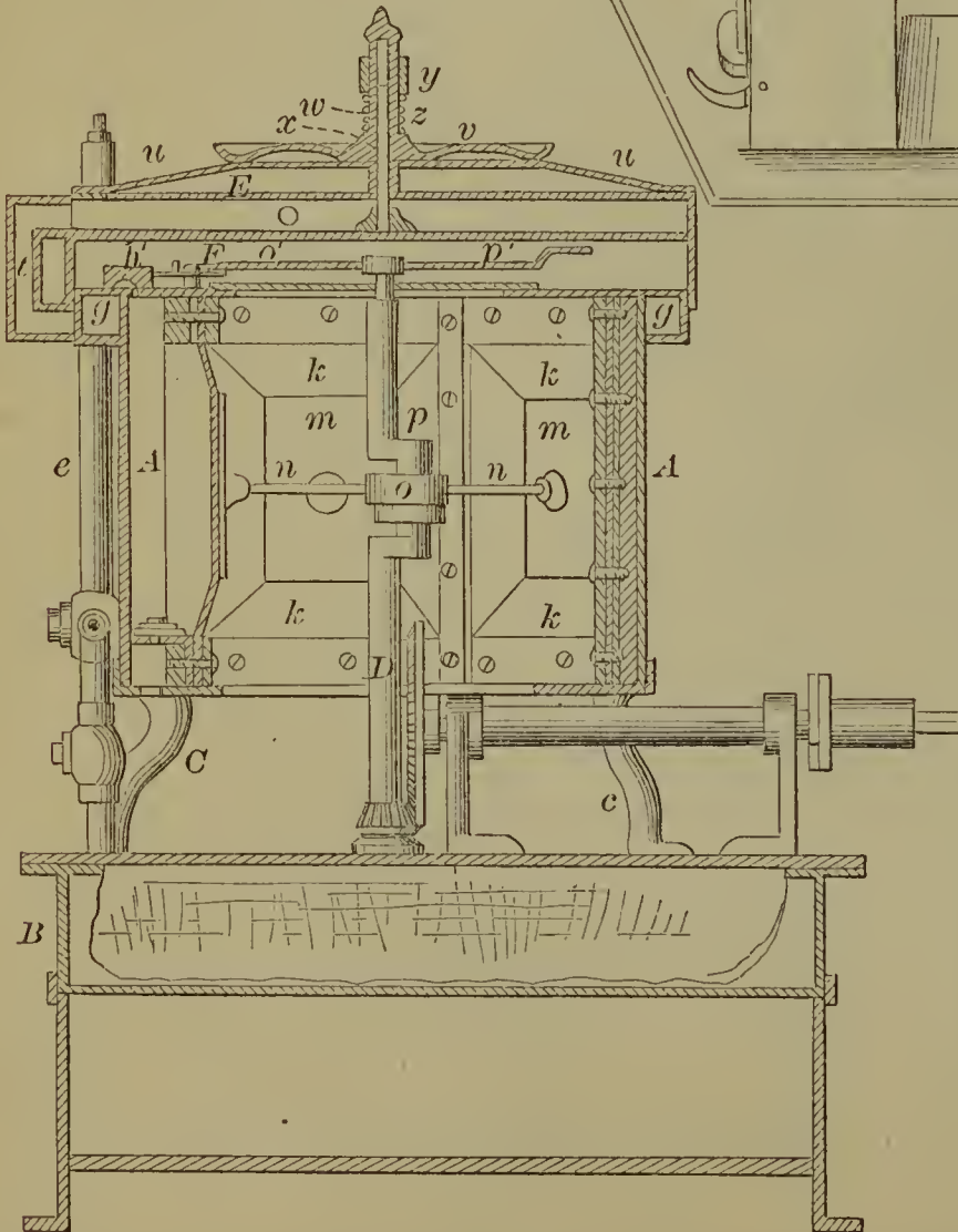
54132—O. P. Drake—For Carbureting Air.
