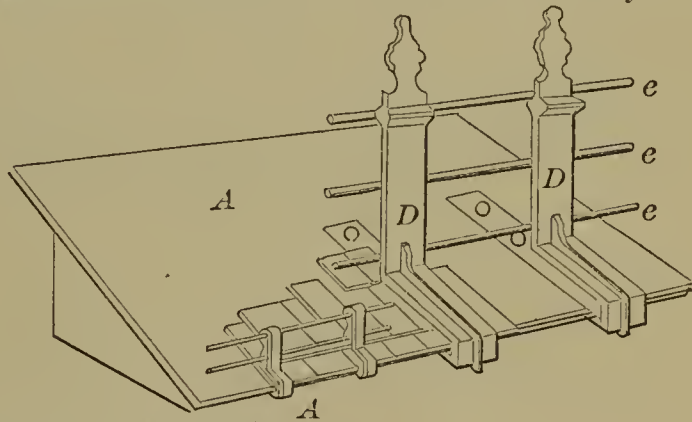
58413—E. Heath—Ditching Machine.
