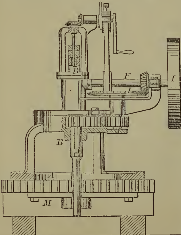
58568—R. Allison— Boring Machine.
