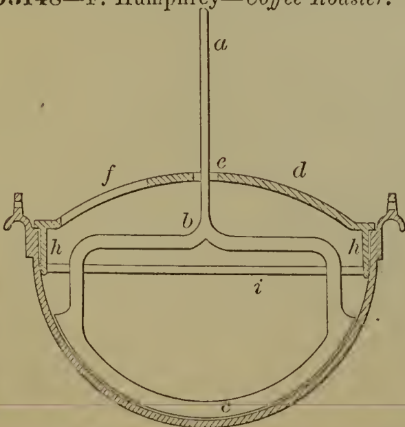
53148—F. Humphrey— Coffee Roaster.
