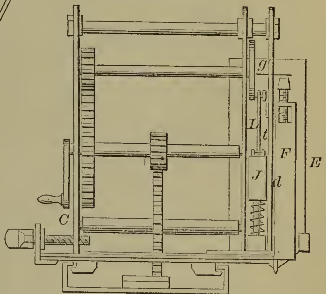
53940—J. Armstrong— Stone Dressing Machine.
