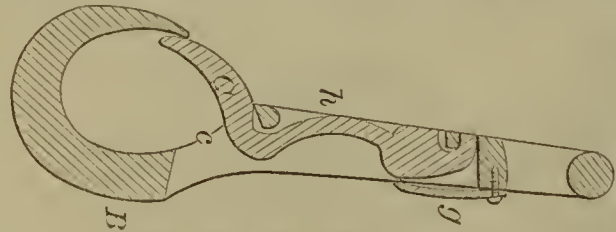
56265—Quinn & Summers— Snap Hook.
