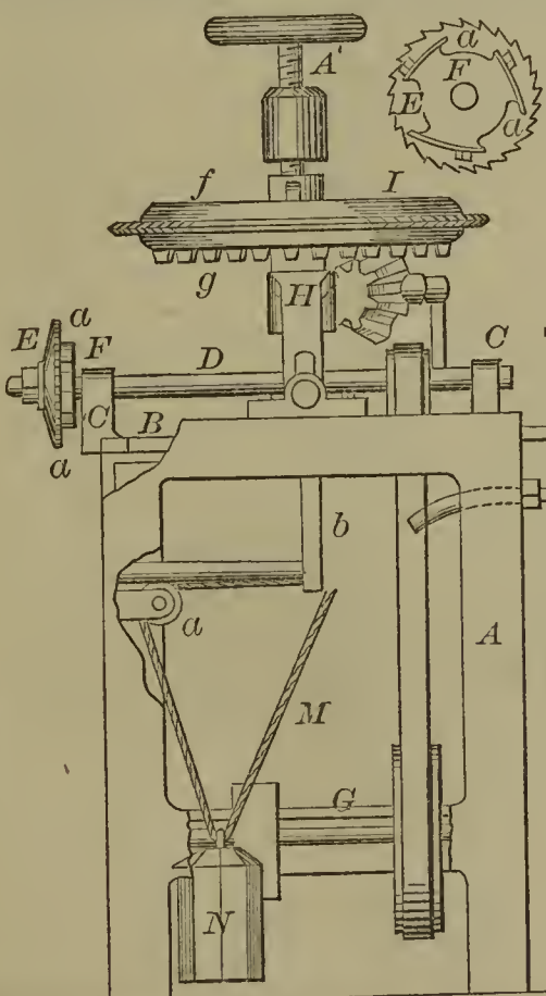
52772—J. S. Thompson—Barrel Head Machine.
