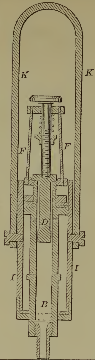
58588—C. P. Brown—Seed Planter.
