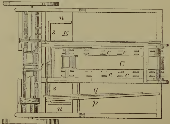
59205—T. Frame—For Raking and Loading Hay.
