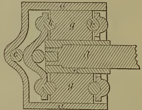
53024—J. C. Merritt— Stove Pipe Damper.
