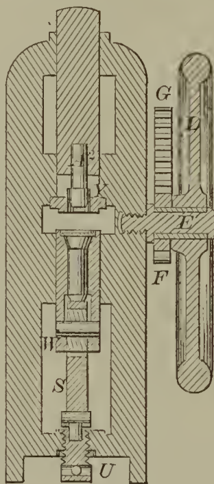
51960—J. North—Press for Striking up Metal.
