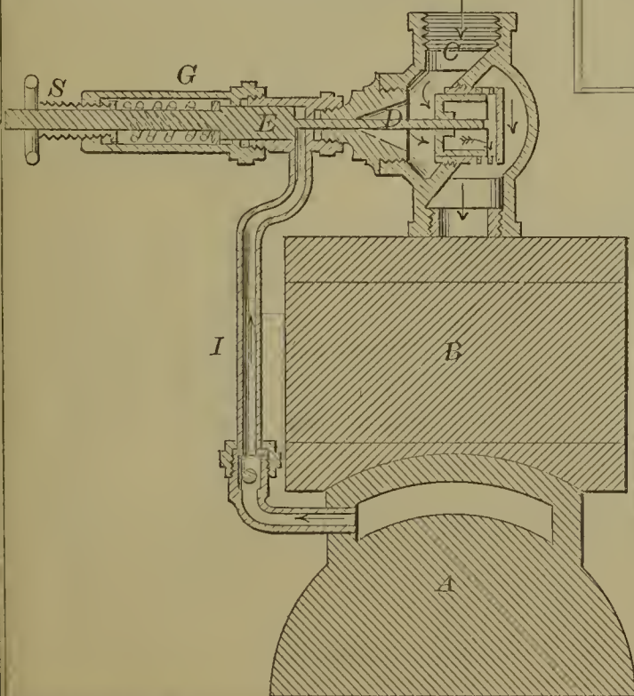
59442—G. E. Noyes— Steam Governor.
