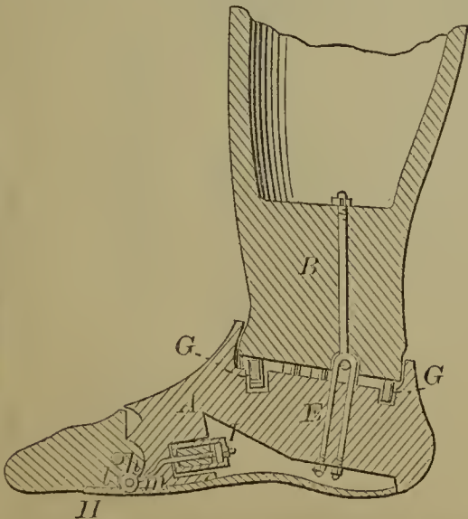
57666—D. Bly— Artificial Leg.
