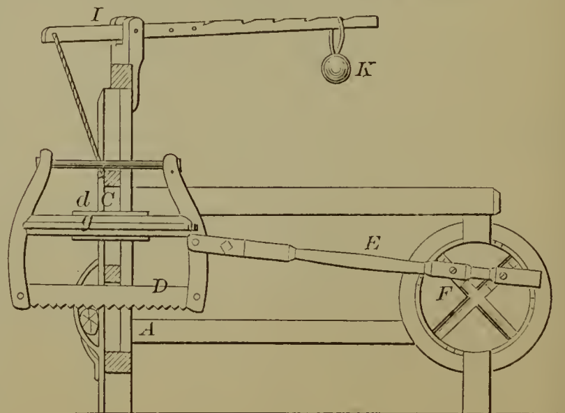
53804—Fryatt & Edmonds— Sawing Machine.
