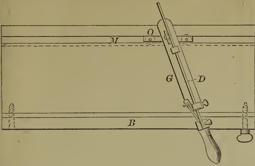
54709—Frazer & Hinchman—Saw Filing Machine.
