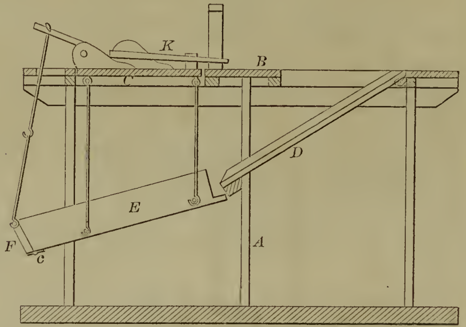
57407—W. H. Taylor— Weighing Device.
