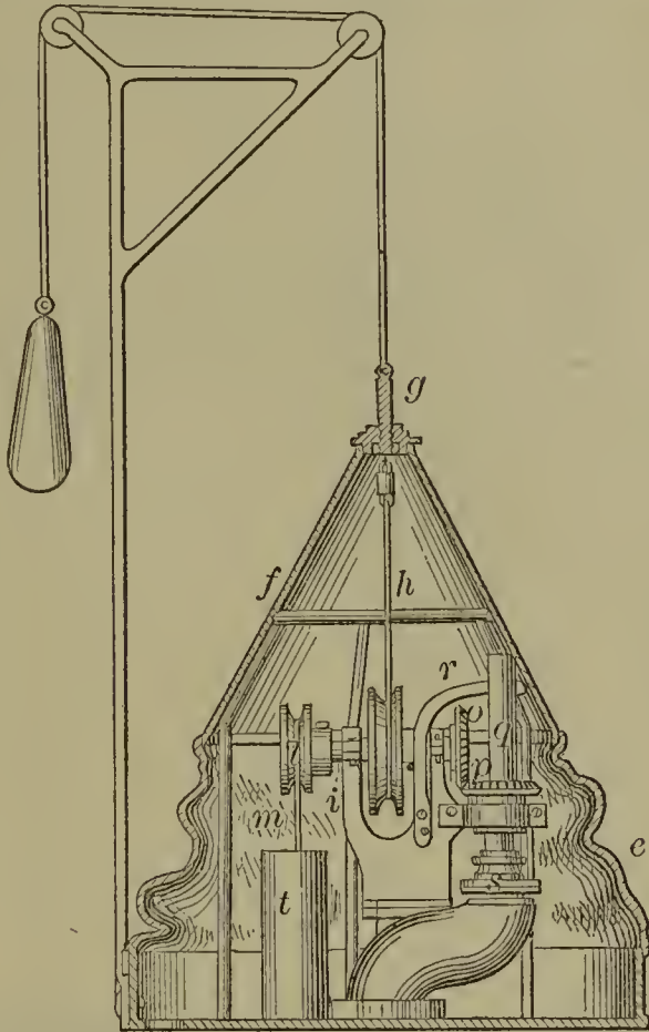
54423—D. Shive— Steam Engine Governor.
