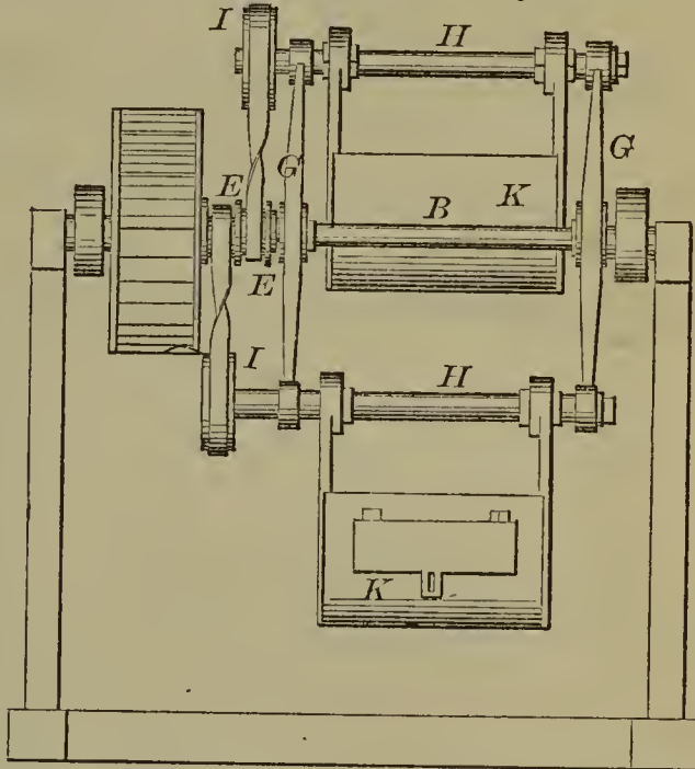
53914—J. Woolf—Transmitting Power.
