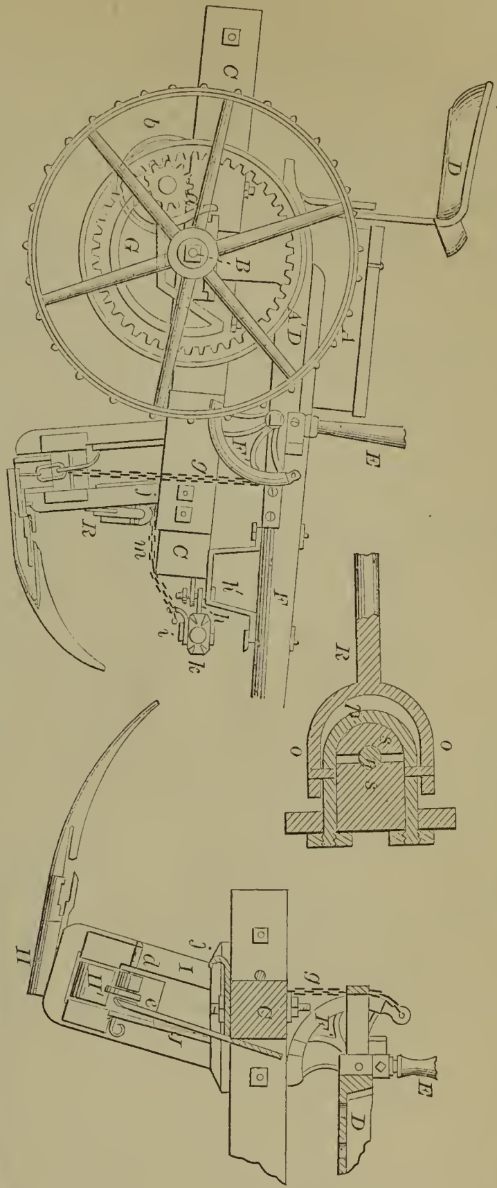
56698—R. Bryson— Harvester.
