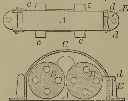
58771—F. H. Carney— Car Seat Indicator.
