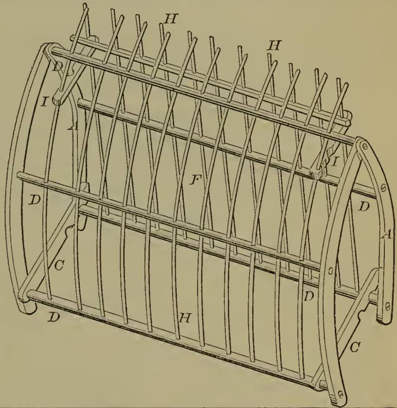
53057—C. Tompkins—Harvester.
