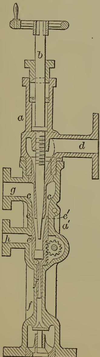
55218—Robinson & Gresham—Water Injector.
