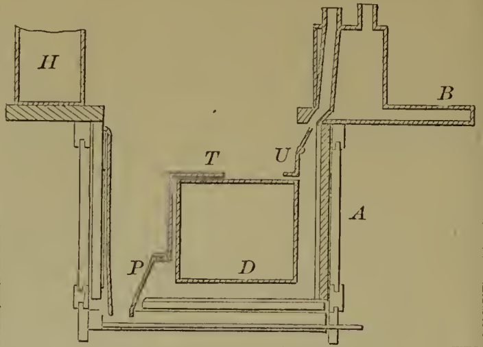
54721—D. Heilig— Cooking Stove.
