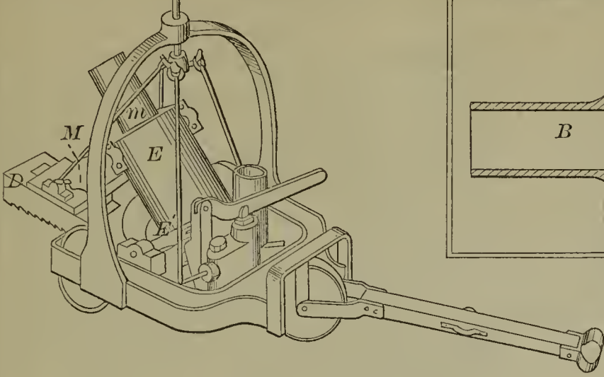
52210—J. Ryan—Hydraulic Jack.
