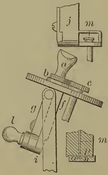
59901—W. Fitzgerald—Pegging Machine.
