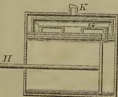
57386—Sangster & Ware—Steam Engine Valve.
