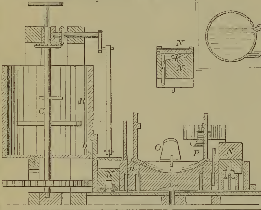
56705—S. Cary— Boring and Grinding Apparatus.
