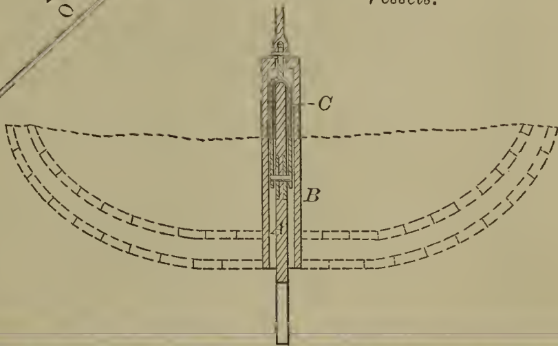
52708—J. F. Hall— Hanging Centre Boards of Vessels.
