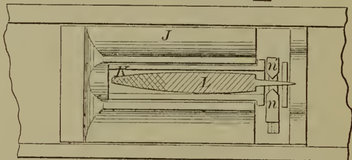
52806—A. O'Neill—Guard Plate for Boilers.
