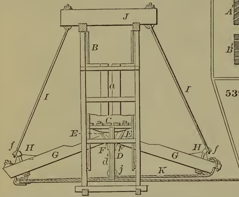
53919—A. Gilmore—Coffer Dam.
