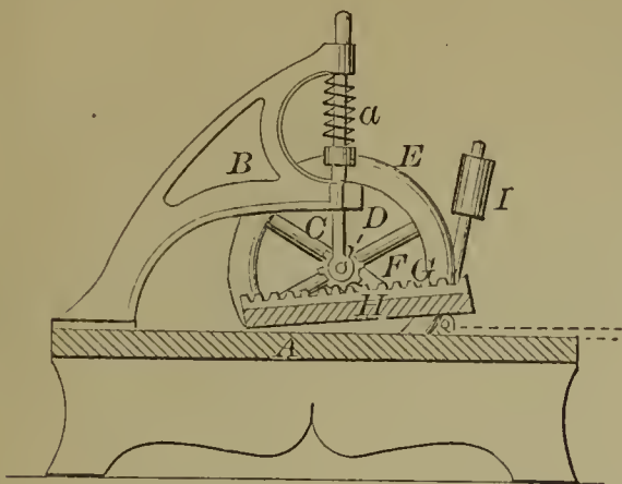
59854—C. V. Mead—For Rolling Rubber.
