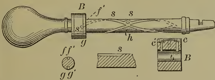
54070—J. H. Palmer—Lubricating Oil Cup.
