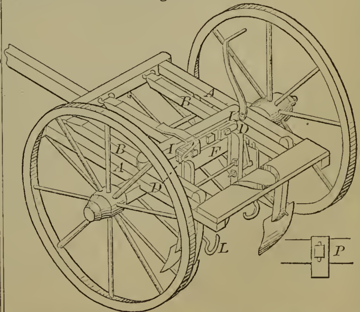
54637—B. F. Young— Cultivator.
