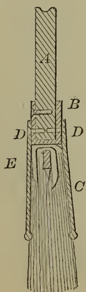
55409—J. Wisner—Broom.
