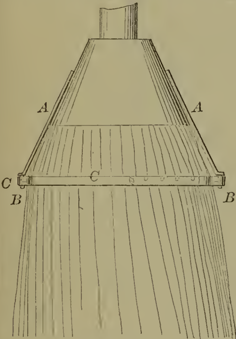
59011—J. Harris— Broom Head.
