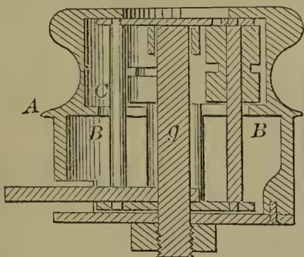
55500—F. G. Johnson— Knob Lock.
