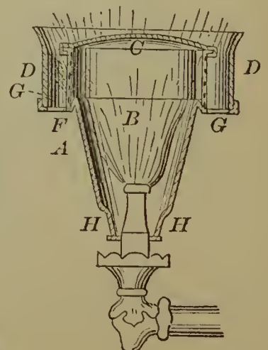
54114—Clark & Savage—Burner for Gas Stoves.
