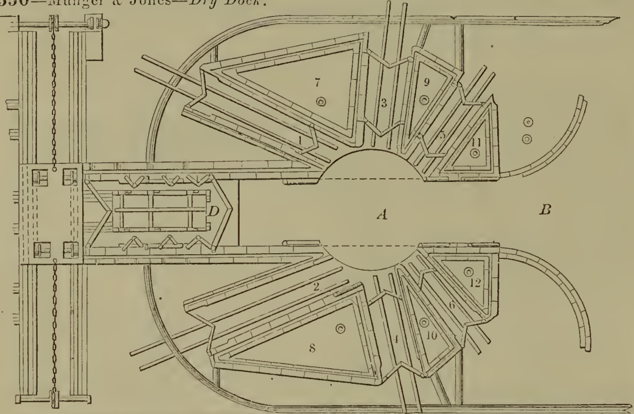
57550—Munger & Jones—Dry Dock.
