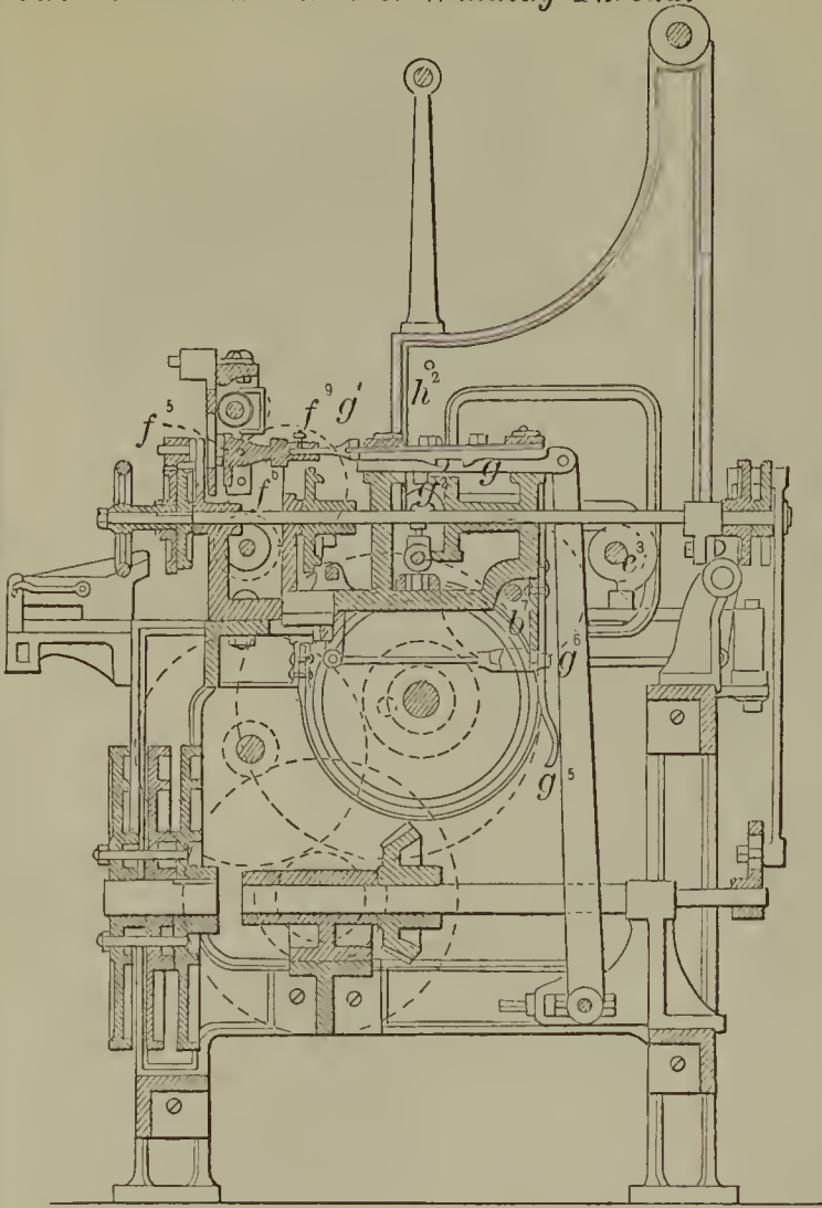
51907—W. Weild—For Winding Thread.
