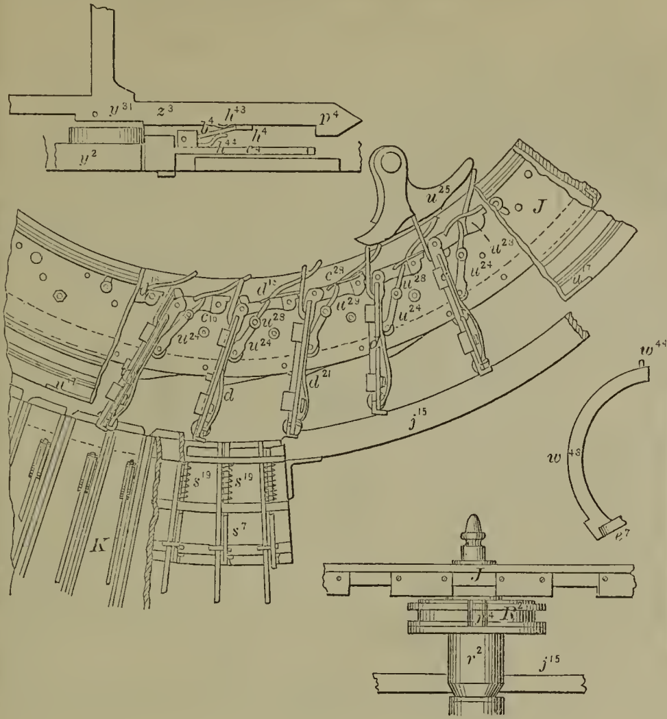
52254—Alden & Mackay—Setting and Distributing Types.
