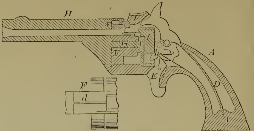
54065—J. B. Doolittle— Revolving Fire Arm.
