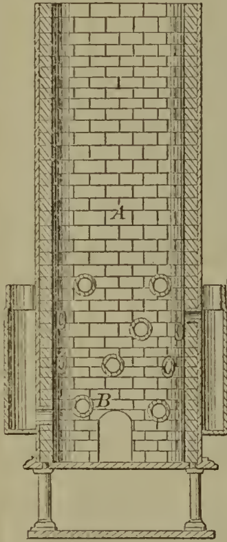
60440—C. Truesdale—Cupola Furnace.
