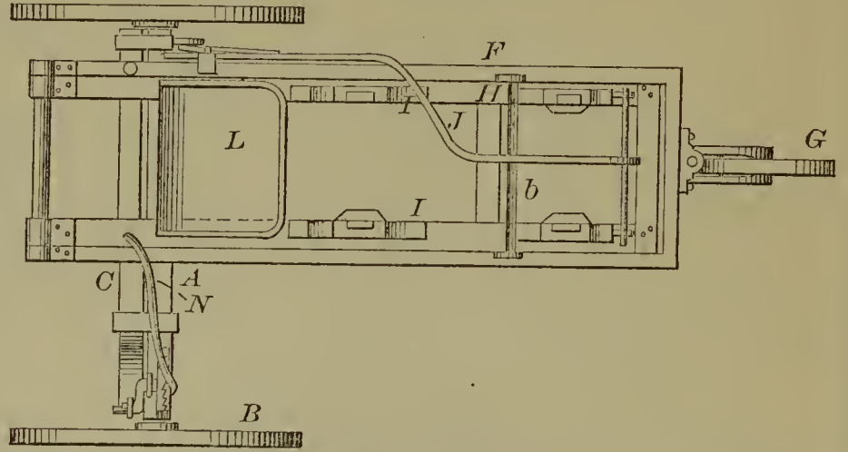
53326—D. J. Noble—Cultivator.
