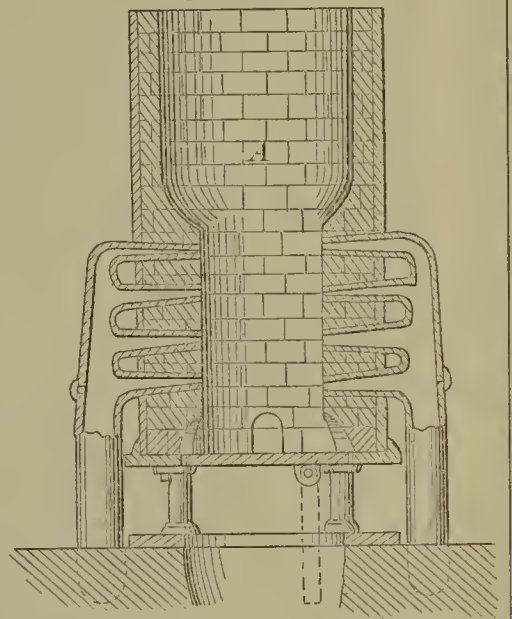
54470—C. Truesdale— Cupola Furnace.
