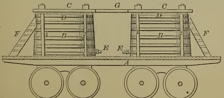
53794—J. & A. Densmore—Car for Transporting Petroleum.
