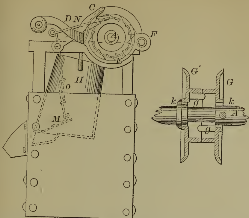
54282—E. Bigelow—Measuring Faucet.
