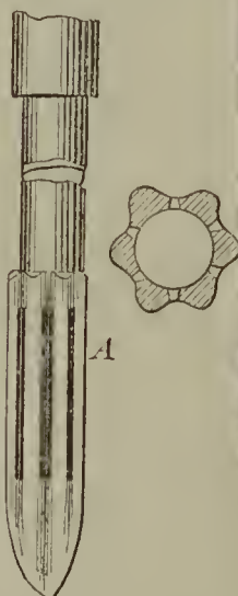
51980—W. W. St. John—Drill Head.
