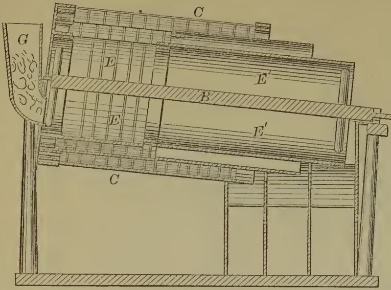
57002—J. B. Smith—Coal Screen.
