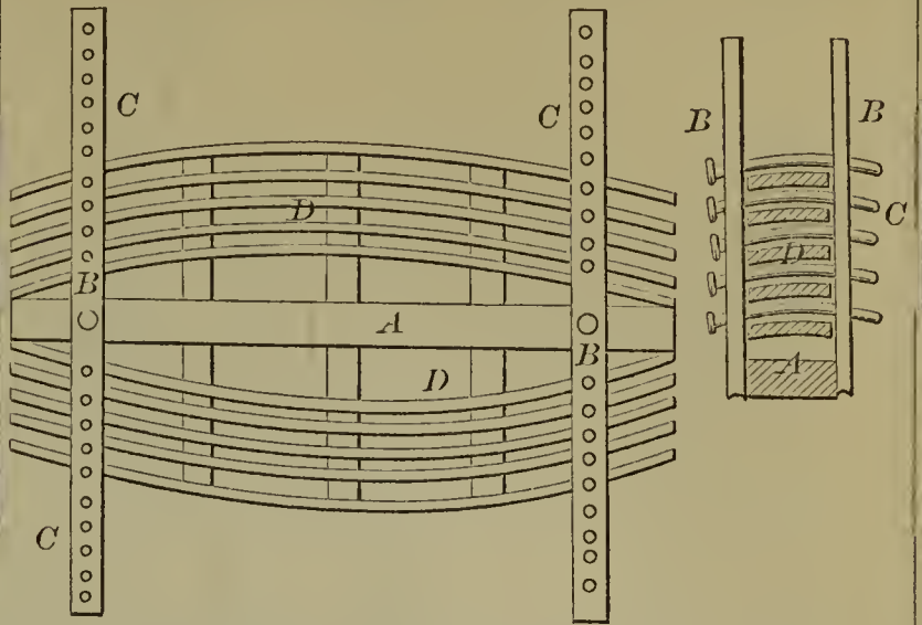
53983—C. B. Hutchinson—Machine for Bending Staves.
