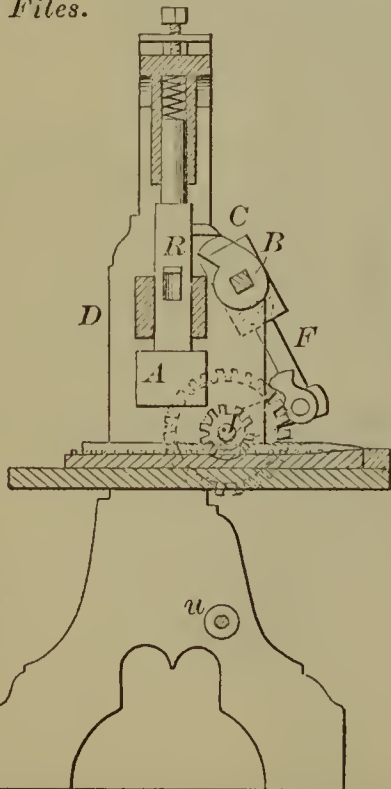
53650—G. Miller— For Cutting Files.
