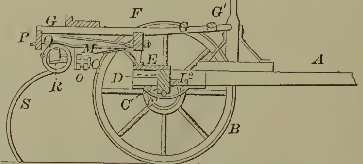
58691—J. M. Stanyan—Dough Mixer.
