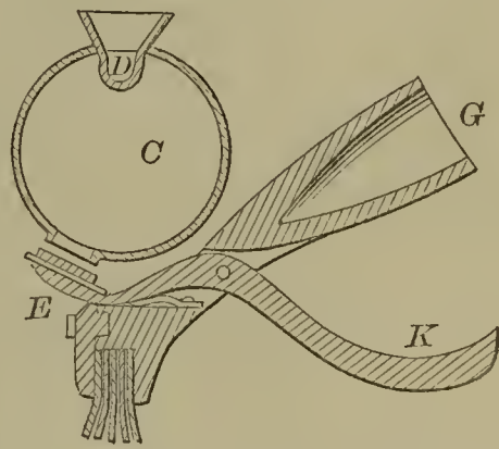
54485—H. Austin— Coupling for Carriage Felloes.
