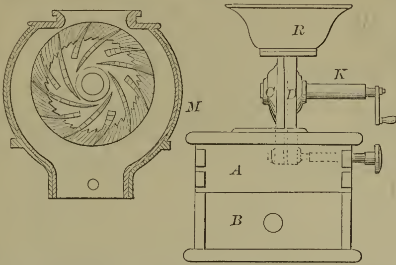
58777—C. P. Colby—Quartz Mill.
