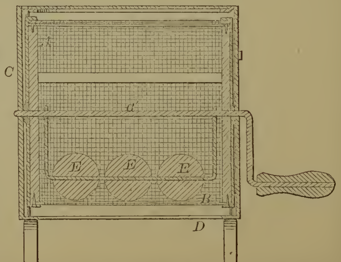
54788—E. Spencer—Flour Sifter.
