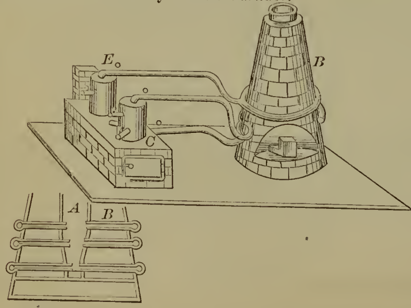
54215—S. C. Salisbury— Blast Furnace.
