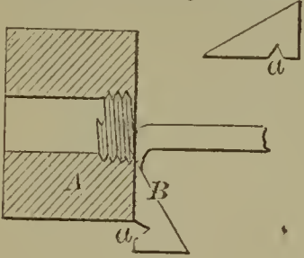
57934—E. Lyman—Gauge for Screw Cutting Tools.
