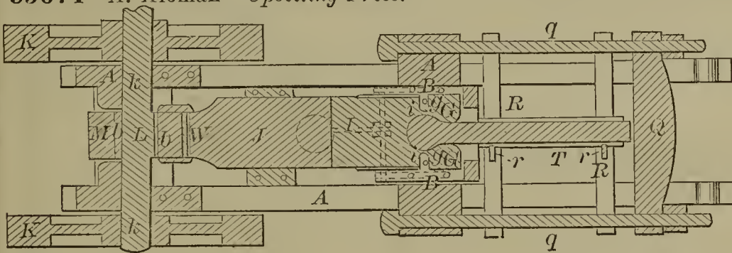
55674—A. Kloman—Upsetting Press.
