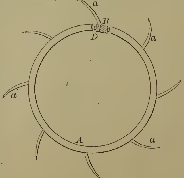
58289—Quinby & Lobdell—Rotary Digger.
