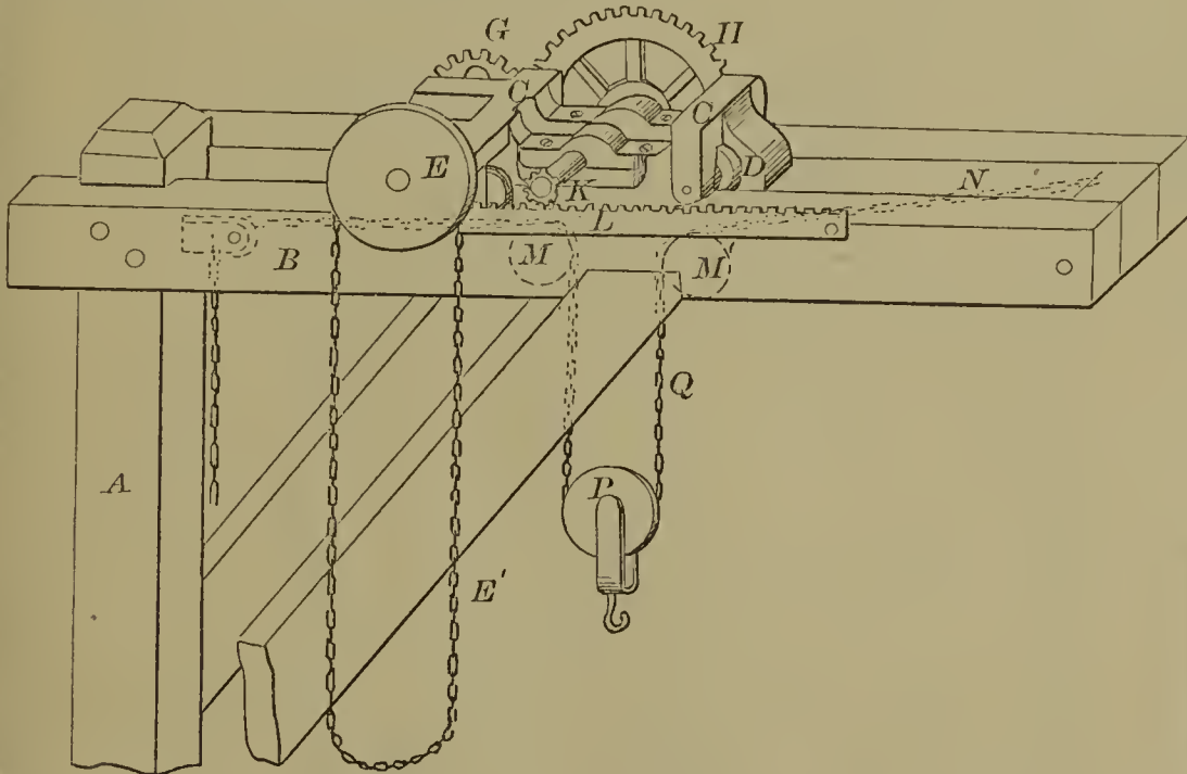
58340—D. Frisbie— Hoisting Apparatus.
