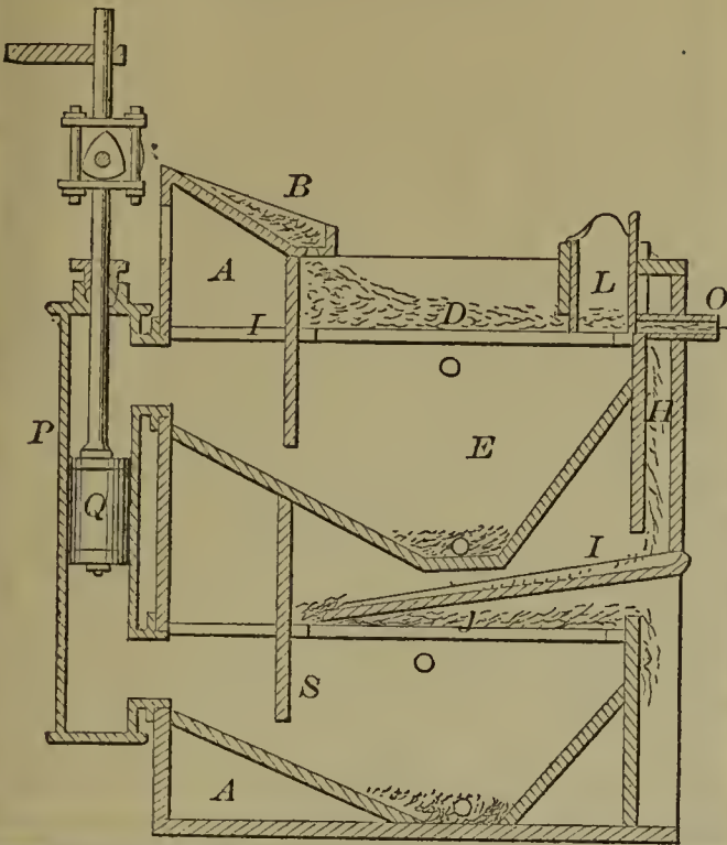
54697—T. Davey—Ore Separator.
