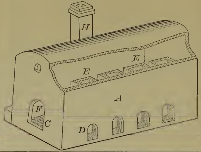
45308—J. W. Dixon— Manufacture of Paper Pulp.
