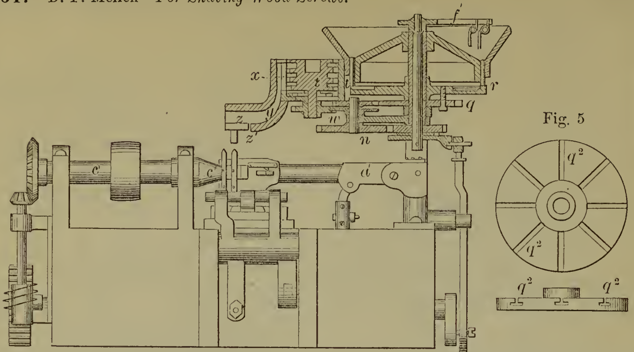
53648—D. F. Mellen— For Nicking Screws.
