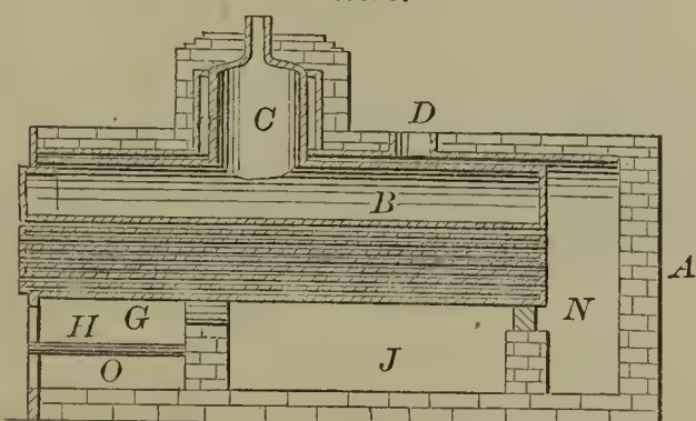
55958—C. S. Nelson— Setting Stationary Steam Boilers.
