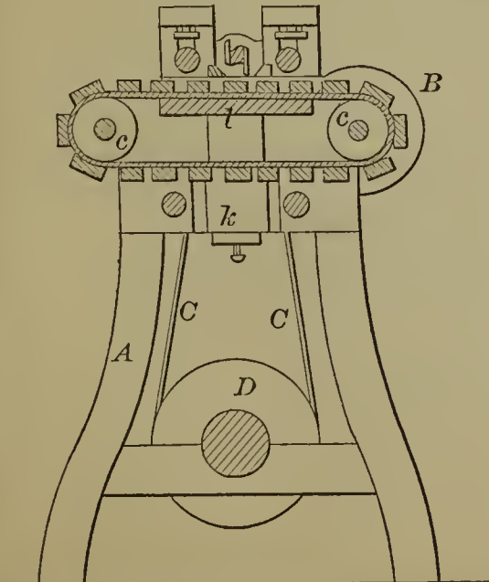
53107—L. W. Boynton—For Making Skewers.
