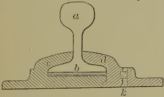
59180—H. Carpenter— Railway Chair.
