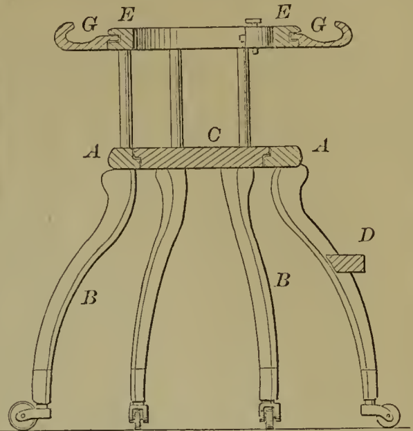
54546—C. Holtz— Chair and Walker for Children.
