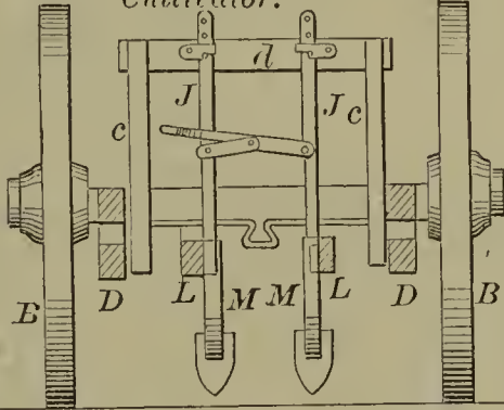
56289—D. C. Stover—Cultivator.
