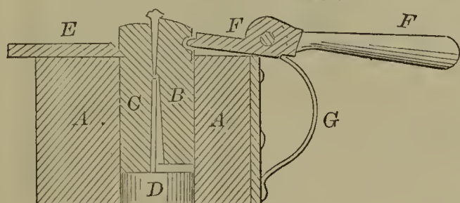
55536—Reynolds & Hilbright— For Forming Heads on Harness Nails.
