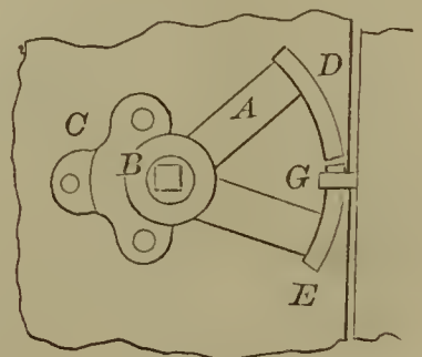
55326—J. W. McLean—Gate Latch.
