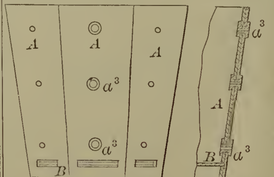
55851—I. C. Gleason—Fruit Basket.
