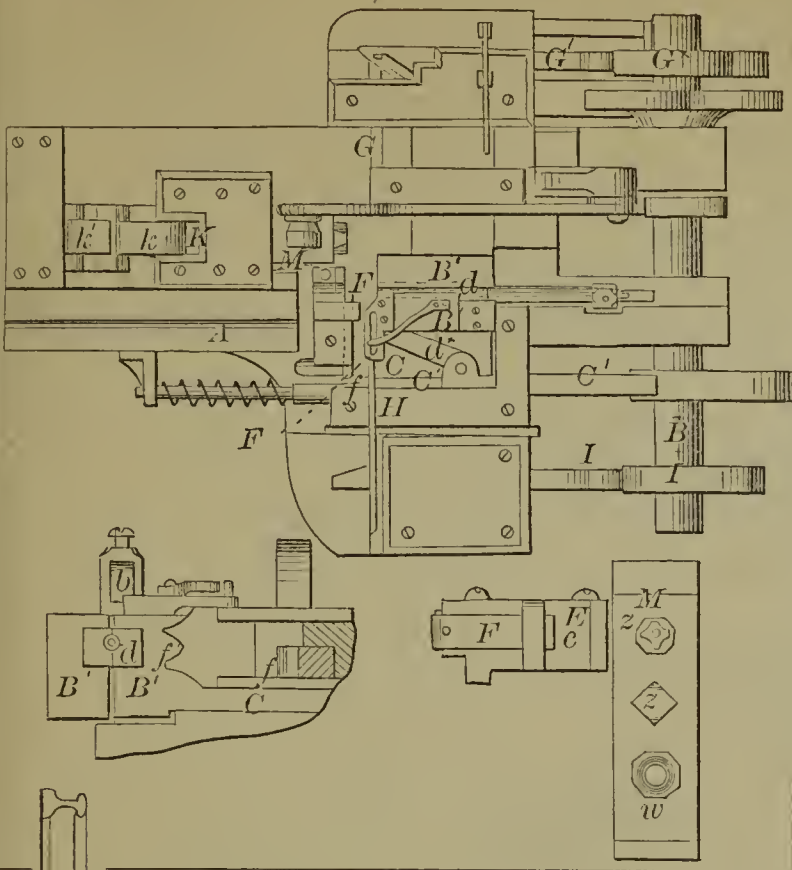
59100—B. Walker— Bolt Heading Machine.
