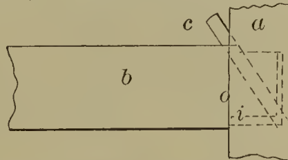
59795—W. H. Elliot—Bedstead Fastening.
