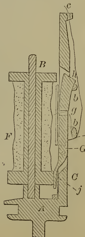
55239—Chambers & Robinson—Yarn Delivery for Braiding Machines.
