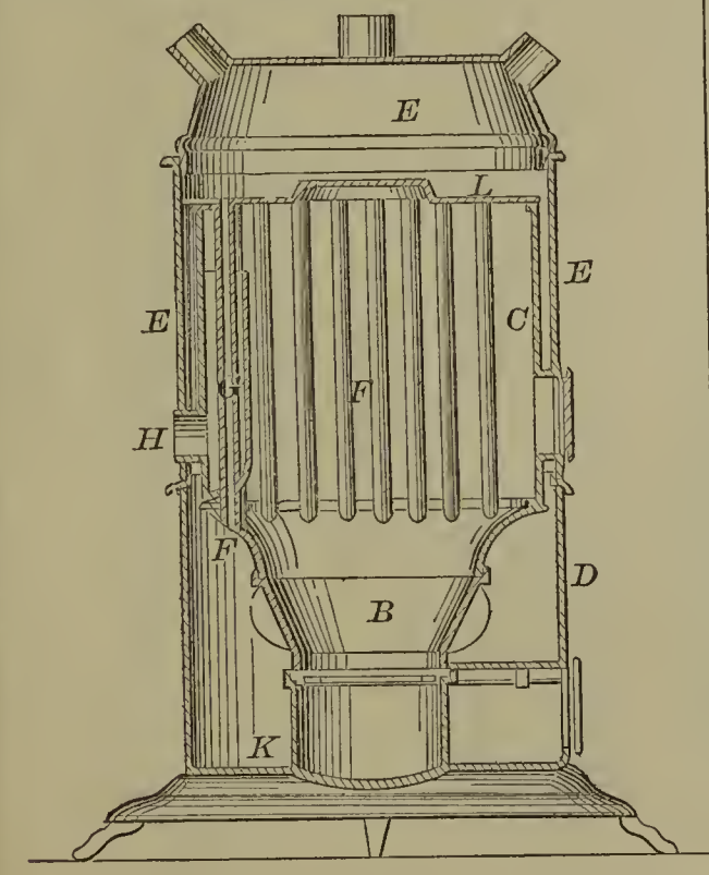
55997—N. A. Boynton—Coal Stove.
