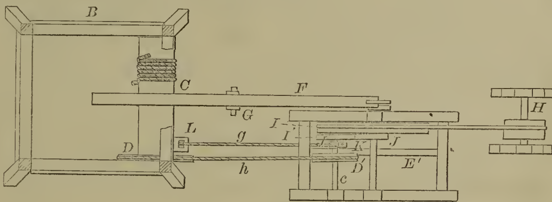
52642—S. J. Goucher—Well Boring Apparatus.
