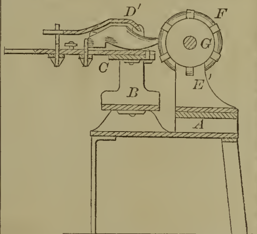
60647—M. Spenle—Lathe.
