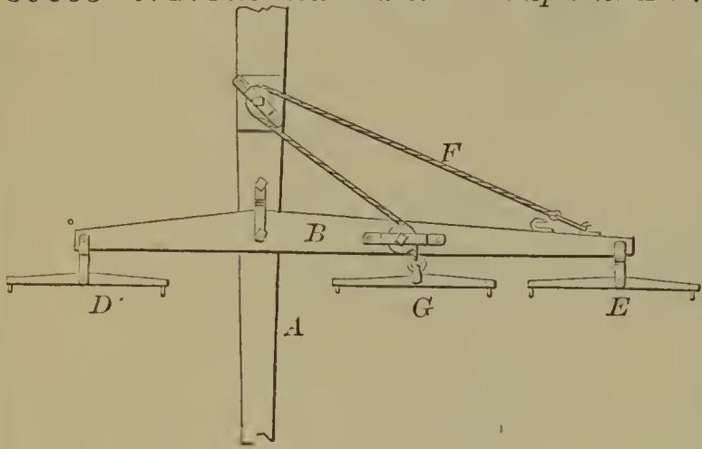
59053—J. B. Morrison—Three Horse Splinter Bar.
