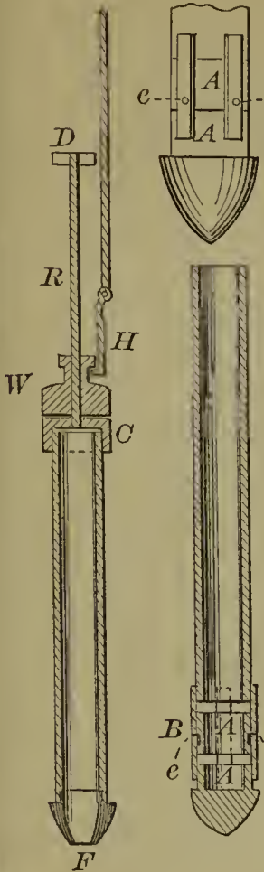
52853—B. J. C. Howe— Sinking Wells.
