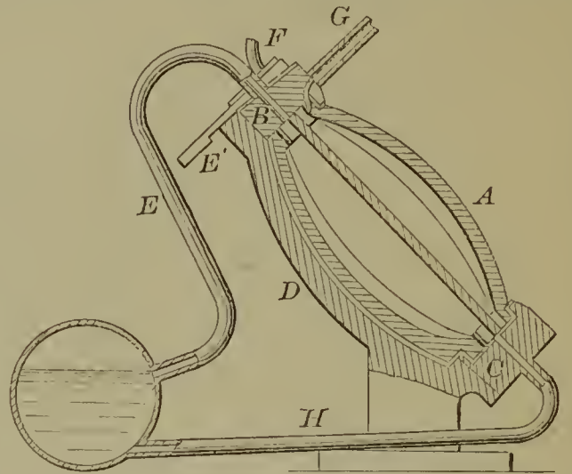
56706—B. Chalfant— Automatic Boiler Feeder.
