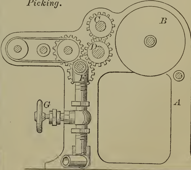
55490—P. S. Haines—Treating Wool for Picking.
