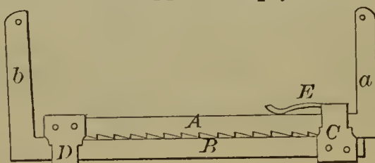
52958—A. P. Briggs— Clamp for Furnace Men's Use.
