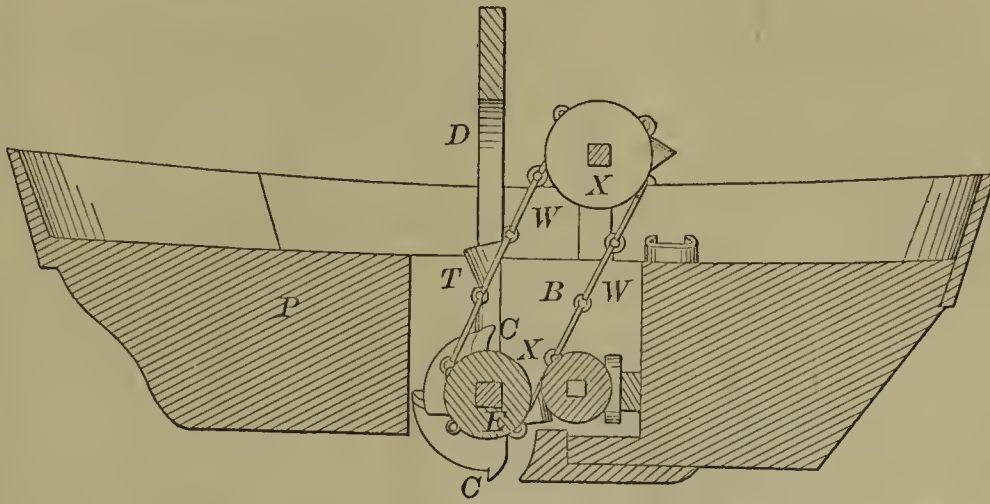
55347—W. H. Nobles—Steam Dredging Boat.
