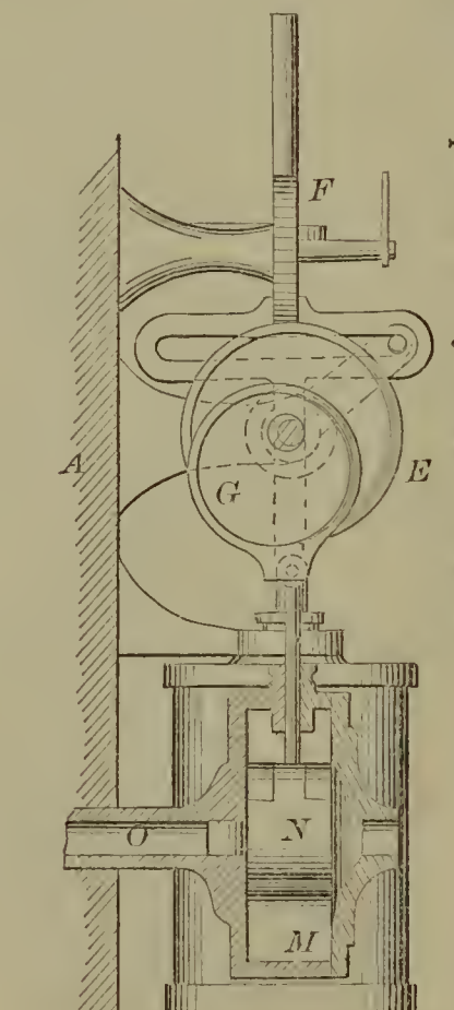
55547—Spencer & Meyer— Water Meter.
