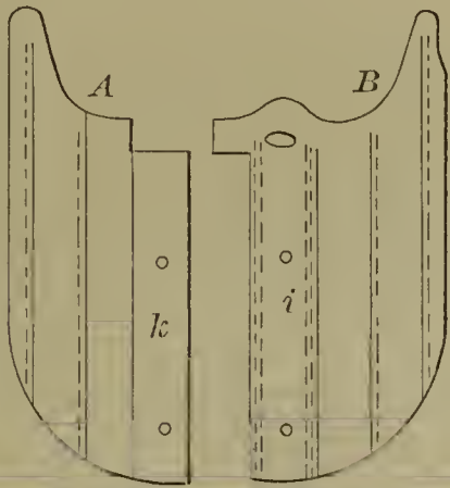
52789—A. Lawrence—Steam Engine Governor.
