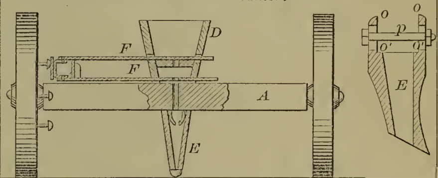
53304—R. Ketcham— Seed Planter.
