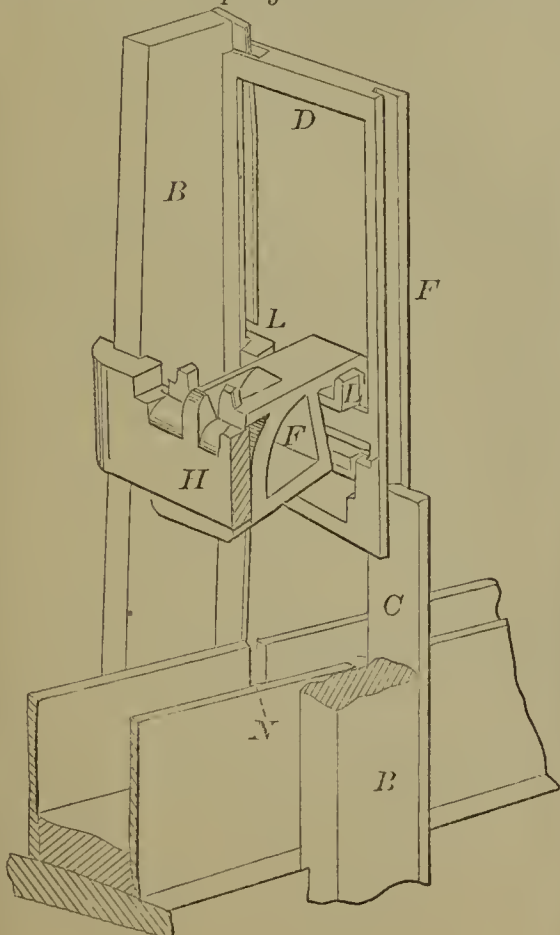
59243—G. Martz—For Hoisting and Dumping Coal.
