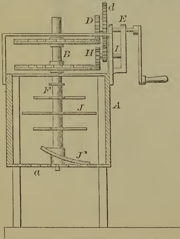
53600—George & Hague—Brick Machine.
