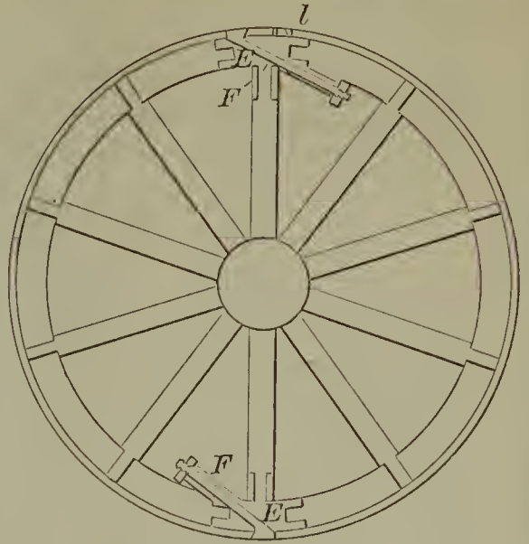
51808—A. J. Curtis— Carriage Wheel.
