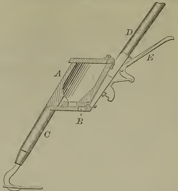
51825—C. L. Green—Hand Corn Planter.
