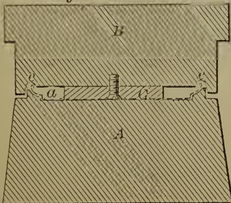
56313—S. R. Wilmot— Die for Forming Sheet Metal Vessels.
