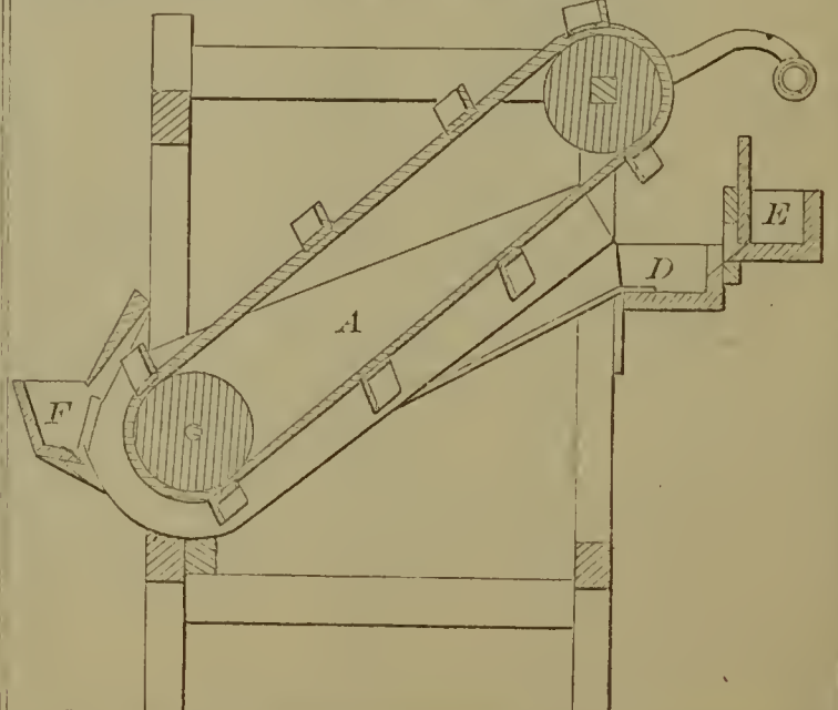
59481—Todd & Downer— Washing Sand.
