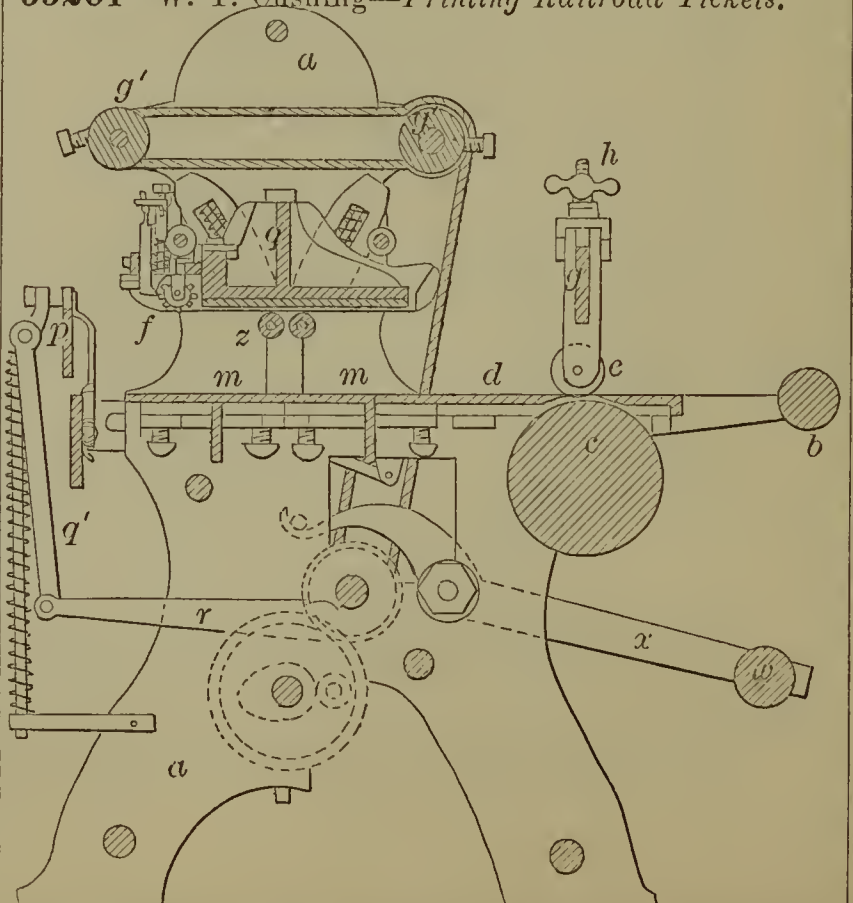
55201—W. T. Cushing— Printing Railroad Tickets.
