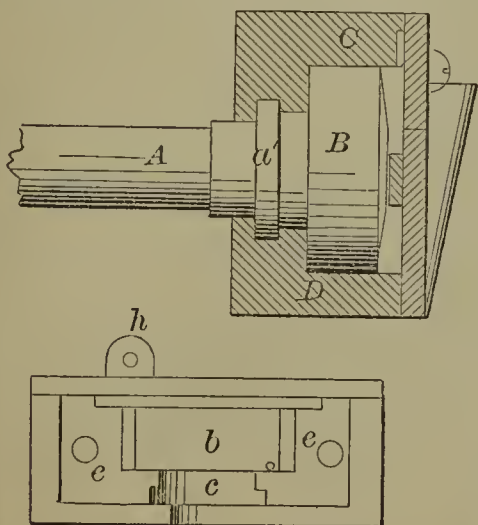
60064—H. B. Rowley—Axle Box.
