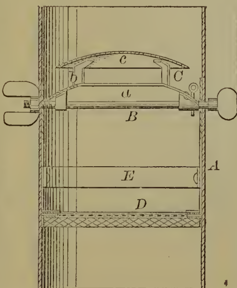
54976—D. & S. Sweeney— Store Pipe Damper.
