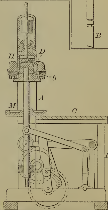
53661—Osterheld & Eickmeyer—Machine for Blocking and Shaping Hats.
