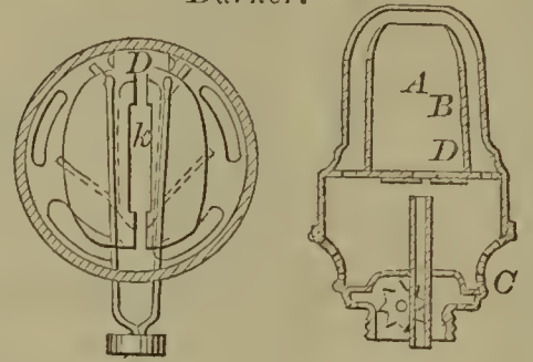
57276—W. W. Batchelder—Vapor Burner.
