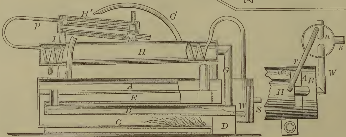
58813—Hall & Ellis— Distilling Apparatus.
