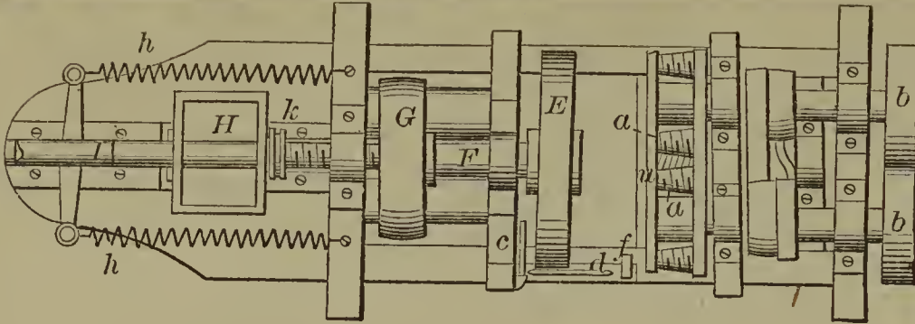
58134—T. T. Prosser—Making Screws.
