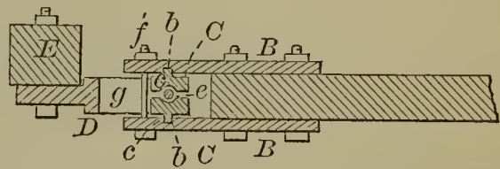
53206—J. W. Weston— Lining for Artificial Limbs.
