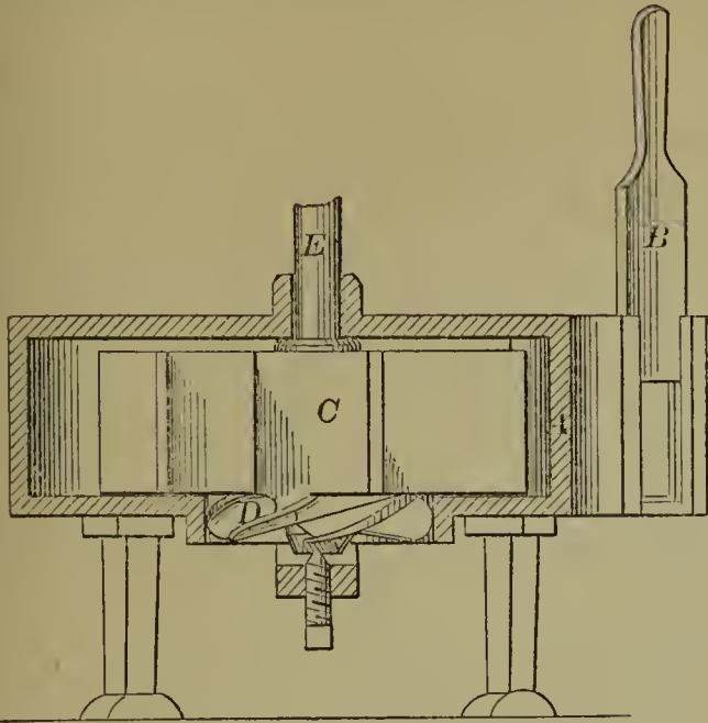
53788—A. P. Conant—Water Wheel.
