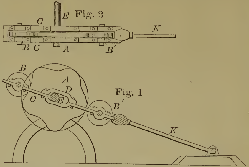
58304—Saladec & Veach—Mechanical Movement.
