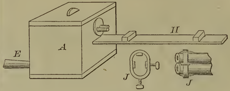
55596—E. Allen— Heating and Soldering Gun Barrels.
