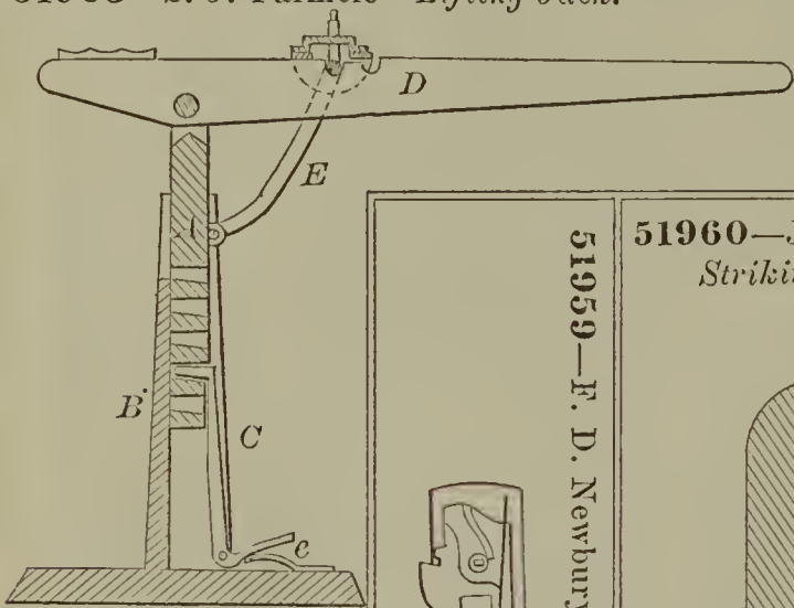
51963—S. J. Parmele—Lifting Jack.
