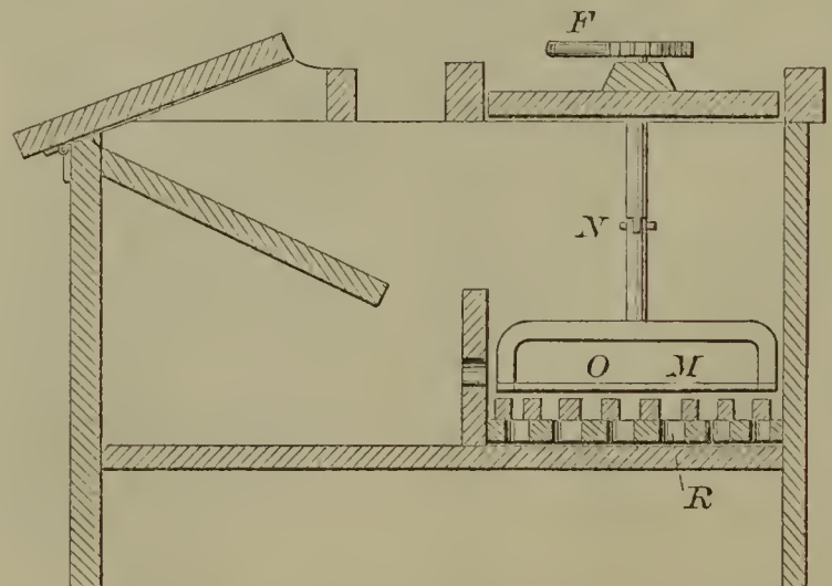
52265—C. G. Campbell— Washing Machine.
