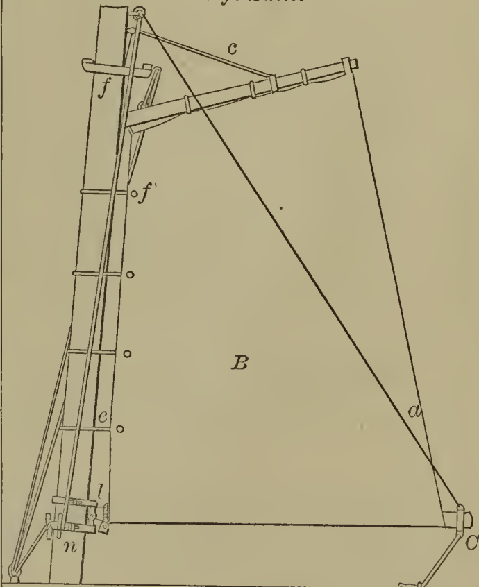
52517—G. A. Bigelow— For Reefing Fore and Aft Sails.
