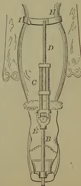
53276—R. Cunningham—Ankle Supporter.
