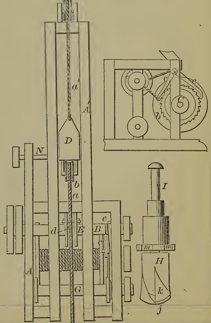
53189—I. M. Rose— Drilling and Driving Machine.
