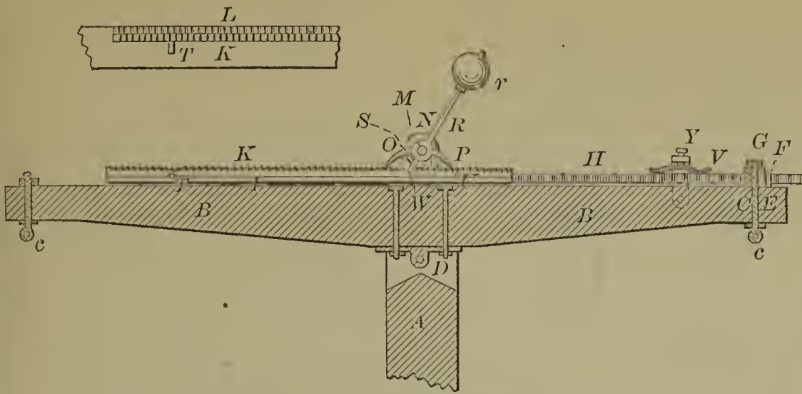
59482—W. B. Trunick— Boring Tool for Wells.
