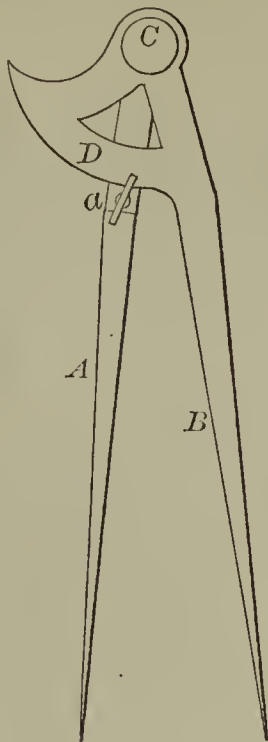
51967—Pfeghar & Schollhorn—Compass and Culipers.
