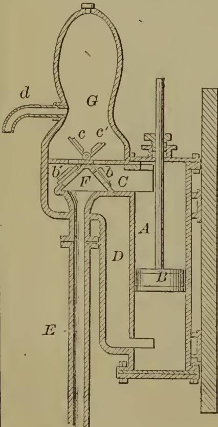
54719—T. Hansbrow— Pump.
