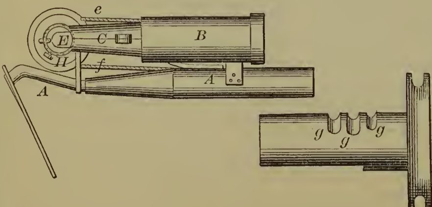
53752—Tyler & Tattershall—Hand Corn Planter.
