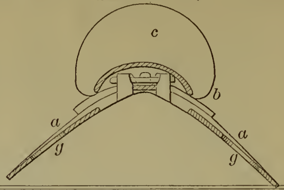
52924—J. C. Young—Crupper Loop for Saddle Trees.
