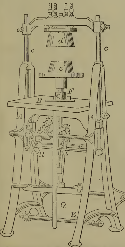
55658—G. C. Howard— For Pressing and Moulding Materials.
