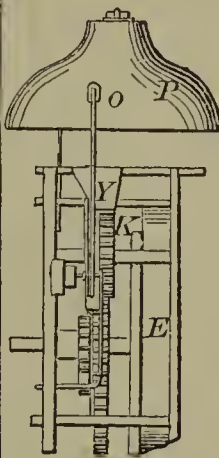
58662—E. Middleton—Fire and Burglar Alarm.
