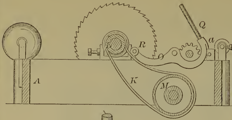
59846—D. Lane—Saw Mill.
