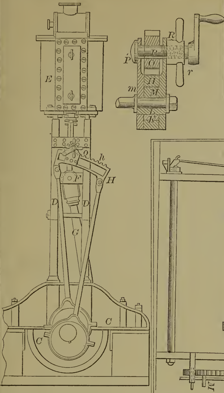
58479—S. H. Rhoades— Driving Pump.
