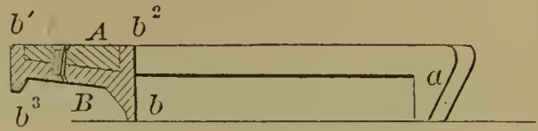
56310—A. S. Wilkinson— Horse Shoe.
