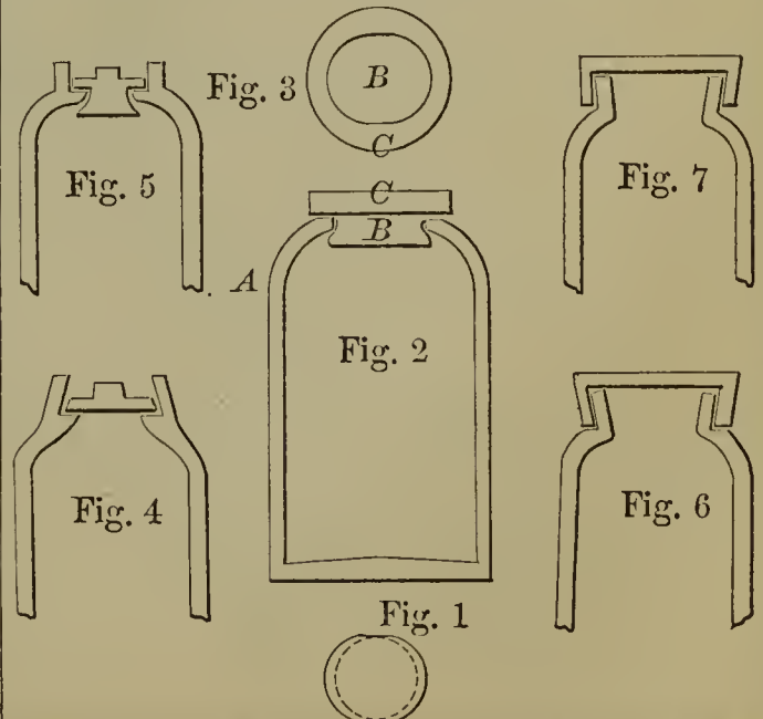
54015—G. M. Ramsy— Constructing Fruit Jars.
