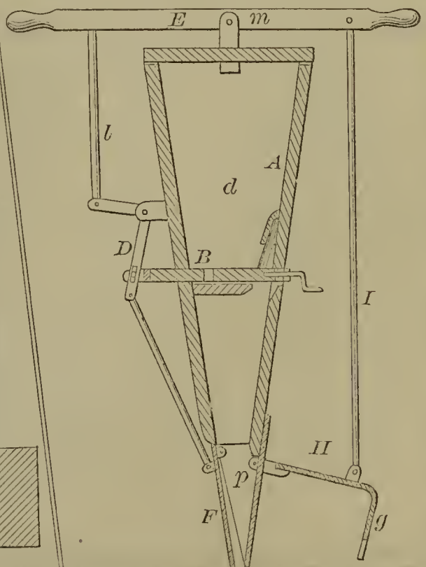
52563—S. Guild—Seeder and Fertilizer Combined.
