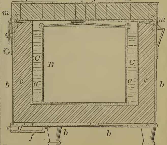
59441—J. & I. Neuburg— Cooking Apparatus and Refrigerator.
