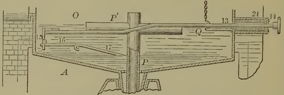
54358—W. G. W. Jaeger—For Continuous Distillation.
