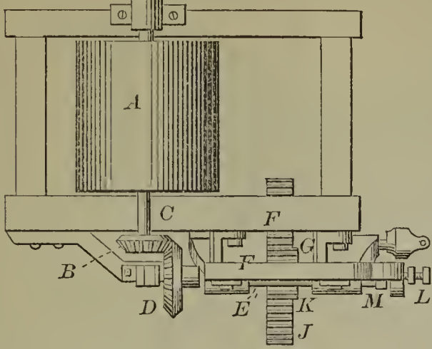
52048—L. B. Hubbell— Threshing Machine.
