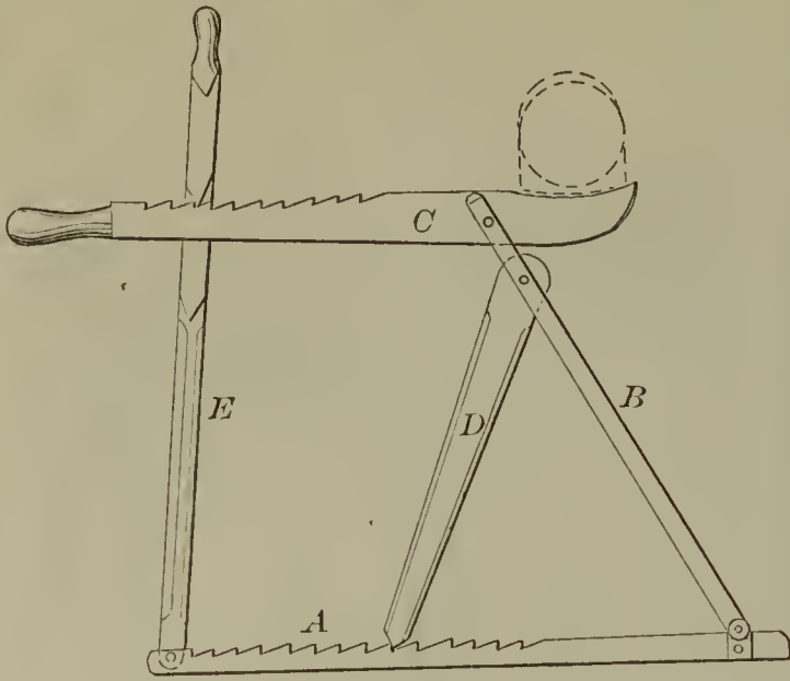
51807—H. Culver— Lifting Jack.
