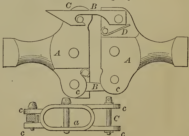
54237—C. O. Wheeler— Car Coupling.
