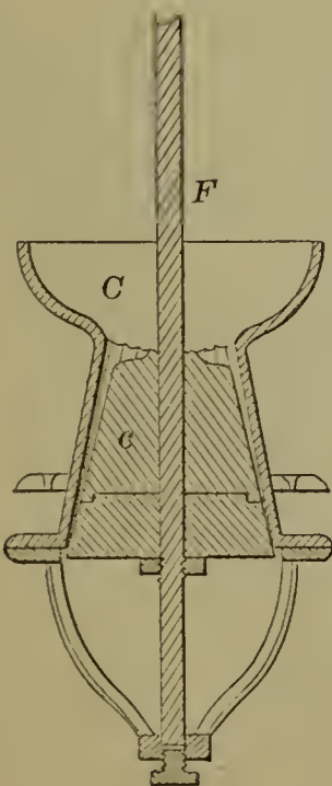
52953—M. Bishop— Paint and Drug Mill.
