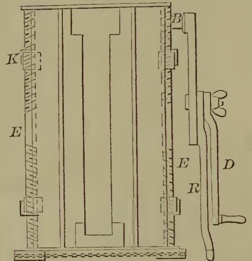
55734—A. B. Stillings— Knitting Machine.
