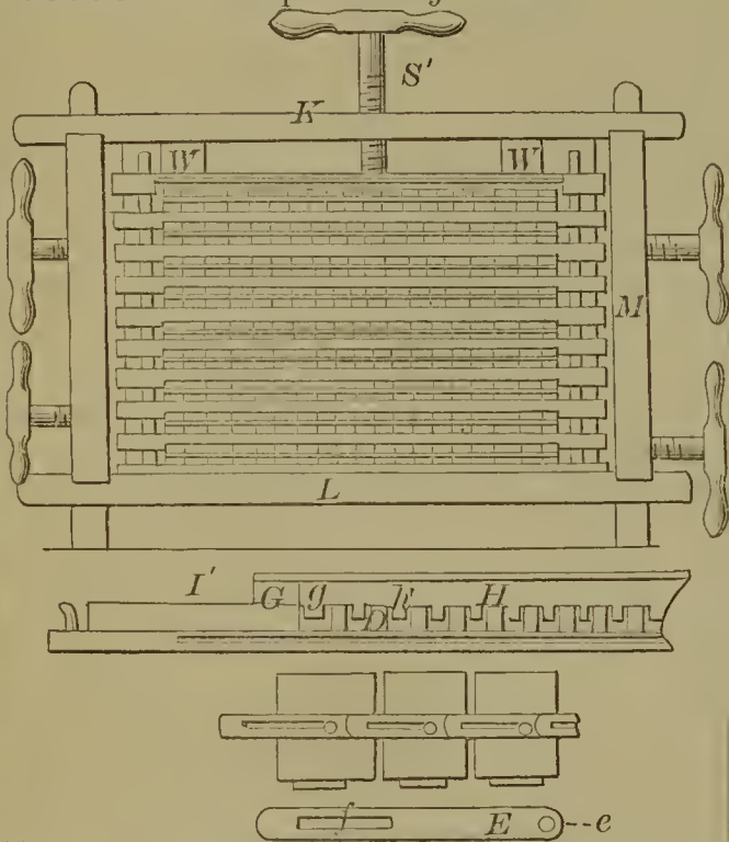
58541—P. C. Ellsworth— Hay Elevator.
