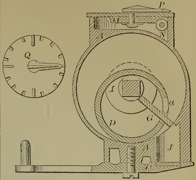
56342—J. G. Baker— Measuring Faucet.
