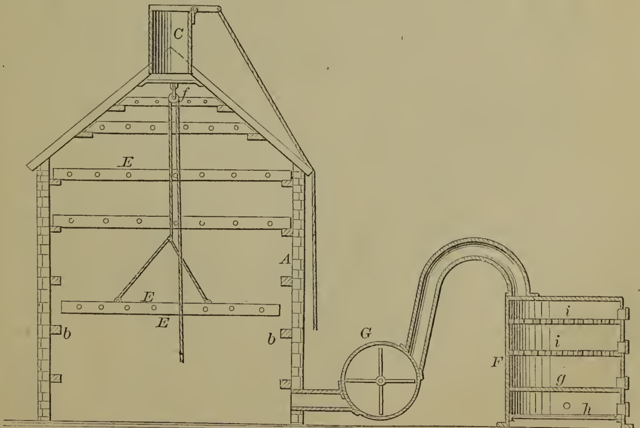
56690—H. A. Amelung—Smoke House.
