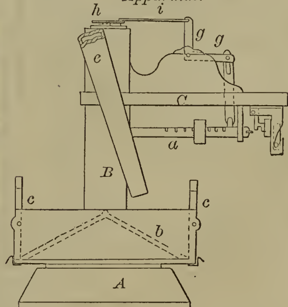
55691—R. S. Morrison—Grain Weighing Apparatus.
