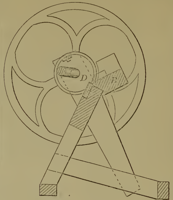
58507—J. A. Taplin—For Cutting Wood.
