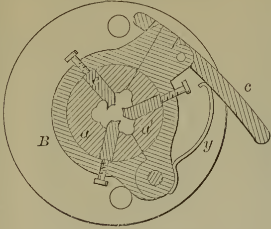
52247—F. H. Higgins—Screw Cutting Chuck.
