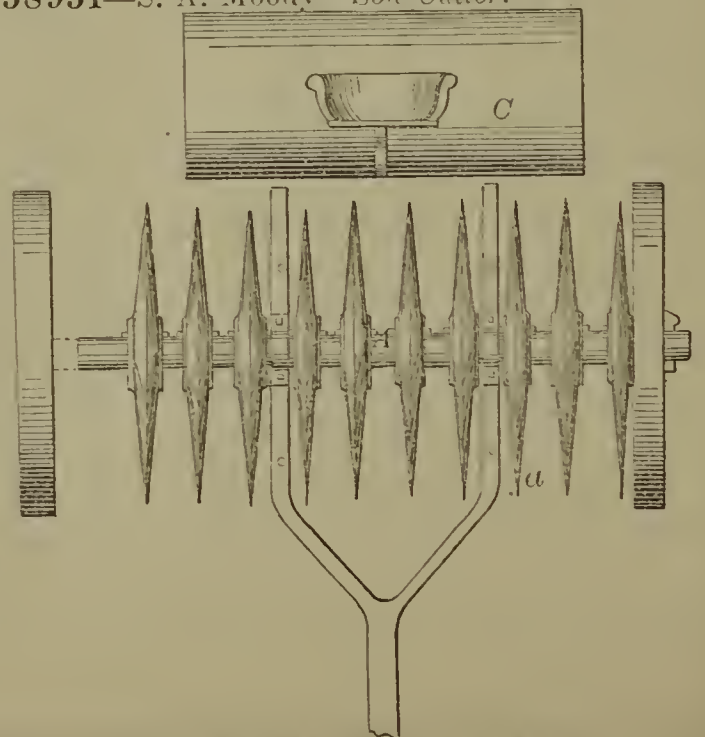
58951—S. A. Moody—Soil Cutter.
