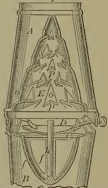
53026—J. B. Moody— Breech-Loading Ordnance.
