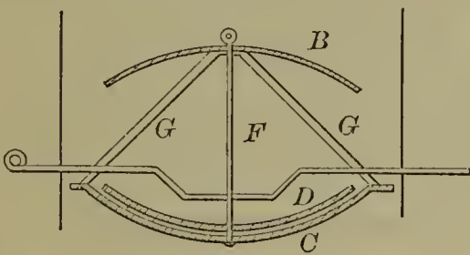
53605—D. L. Grover—Stove Pipe Damper.
