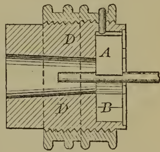
53368—Wells & Mayott— Drill Chuck.
