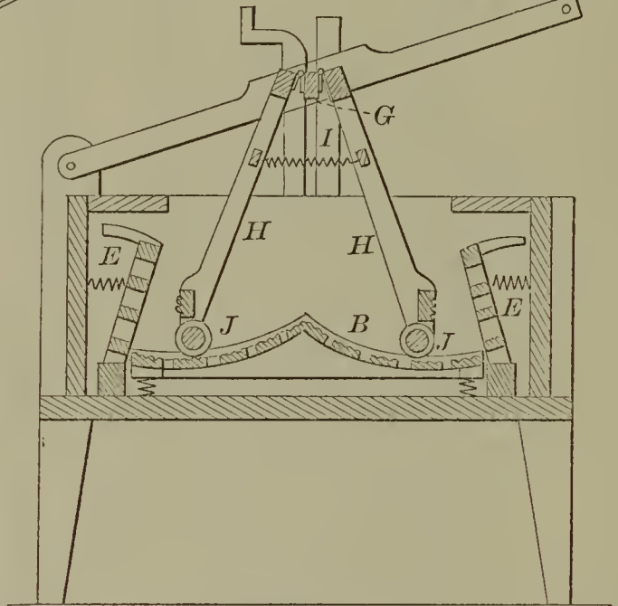
52108—J. Adams— Washing Machine.
