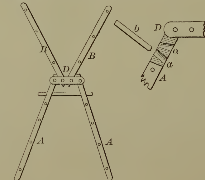
59935—L. C. Wright—Clothes Dryer.
