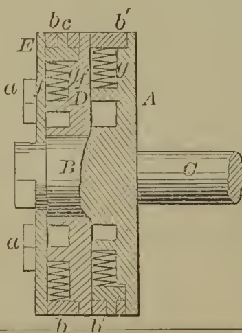
58766—J. Broughton— Piston Packing.
