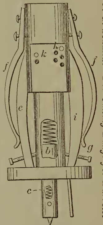
60430—J. G. Schmidt—For Cutting Bungs for Barrels.
