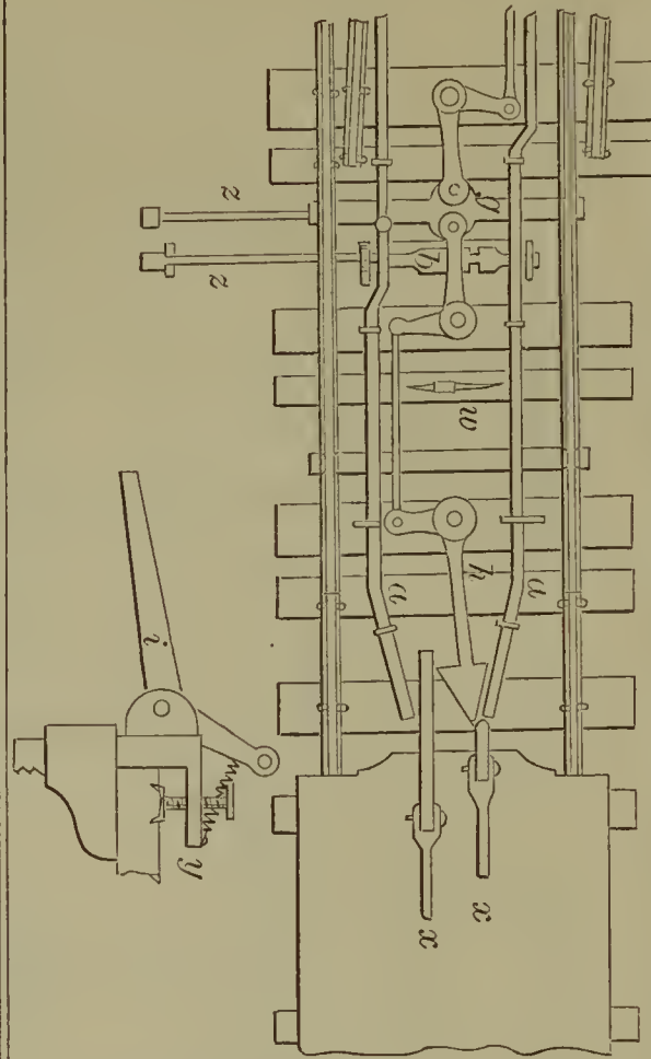
55913—C. H. Sawyer—Railway Switch.
