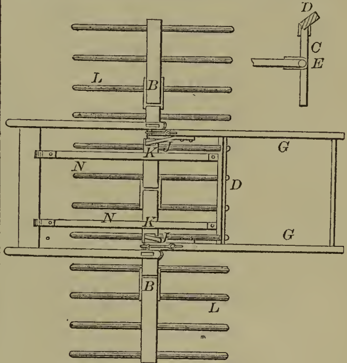
60270—Smith & Brumfield—Horse Rake.
