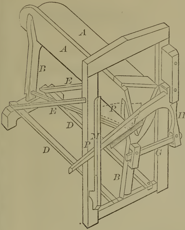
52543—J. W. Dixon— For Making Paper Pulp.
