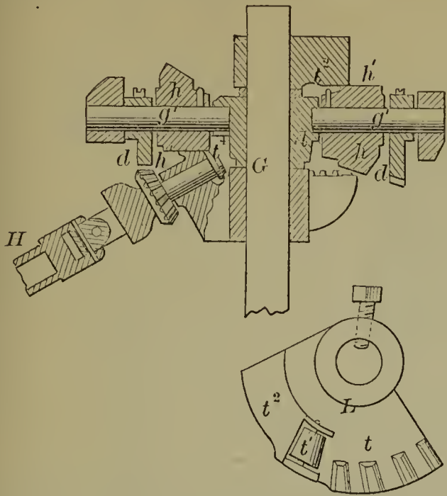
53653—C. Moul—Harvester Rake.
