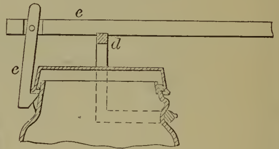
54929—W. W. Lyman— For Opening Fruit Cans.
