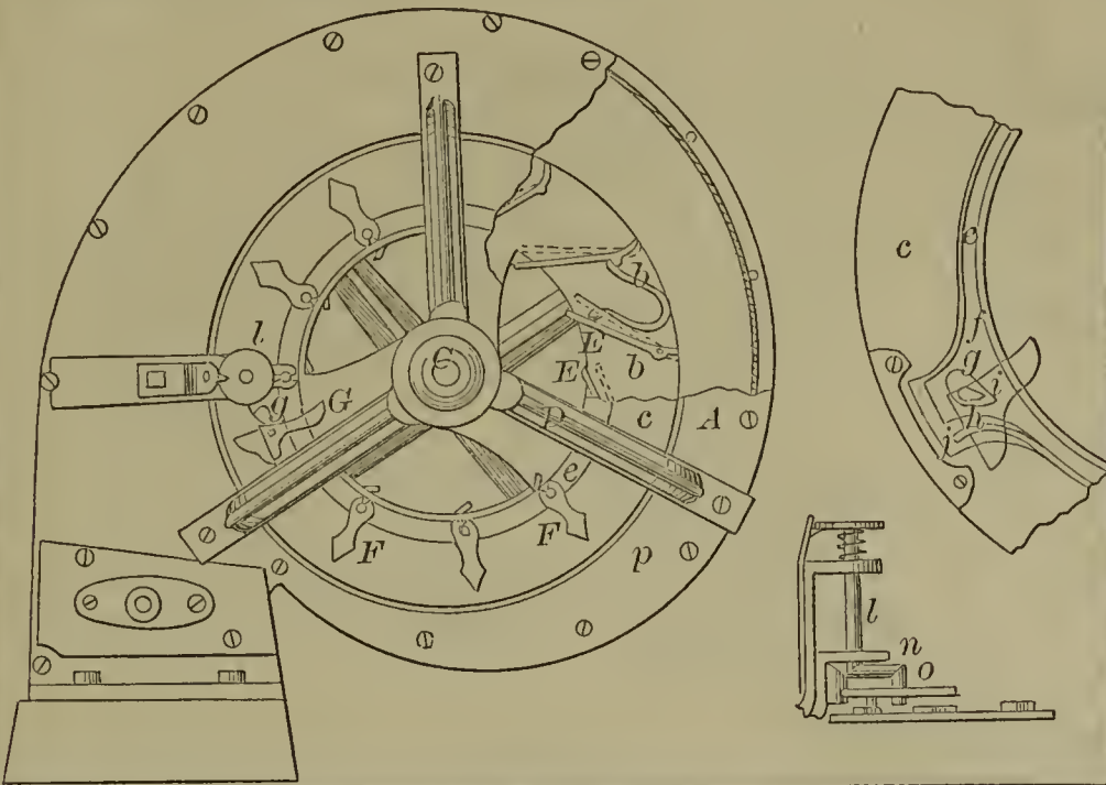
55688—J. McCloskey—Button Hole Sewing Machine.
