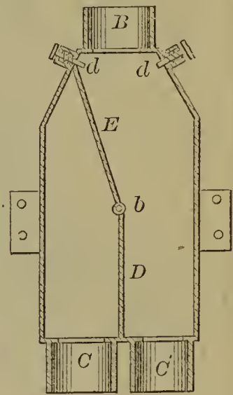
55072—L. W. Doty—Rain Water Cut-off.
