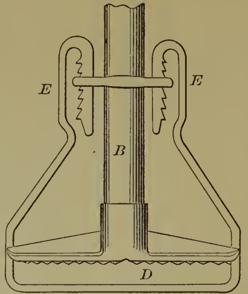
53704—L. H. Thomas— Mop Head.
