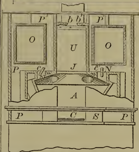
56045—R. F. Hatfield—Steam Engine, Valve, &c
