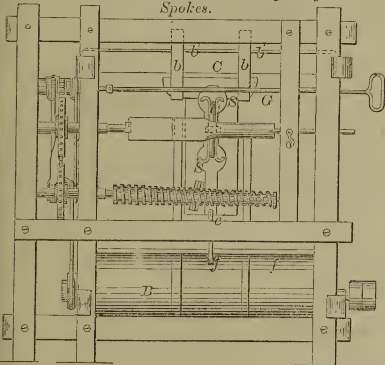
57099—T. Derington—For Turning Wagon Spokes.
