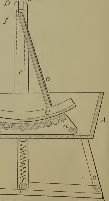
56761—W. & A. G. Kelsey—Washing Machine.
