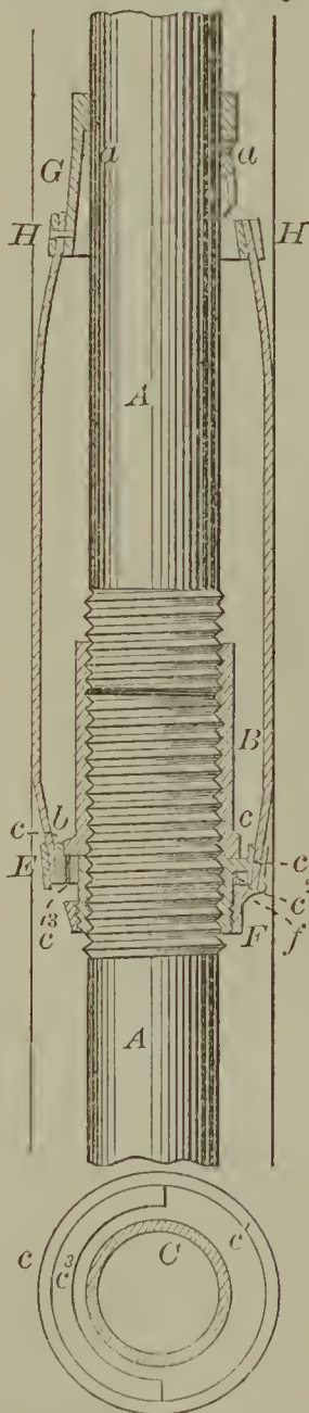
51945—S. E. Hewes— Well Tube Packing.
