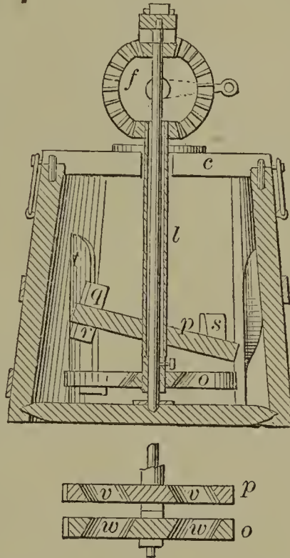
57942—W. R. McCutcheon— Churn.
