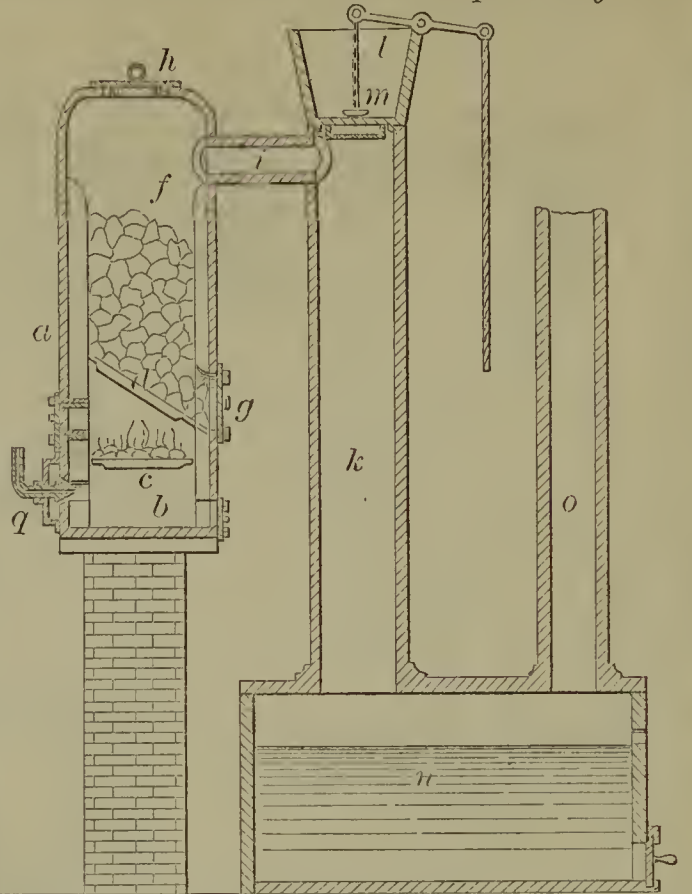
52191—B. G. Noble—For Desulphurizing Ore.
