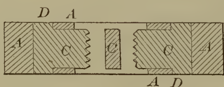
52783—C. G. Cross—Screw Cutting Die.
