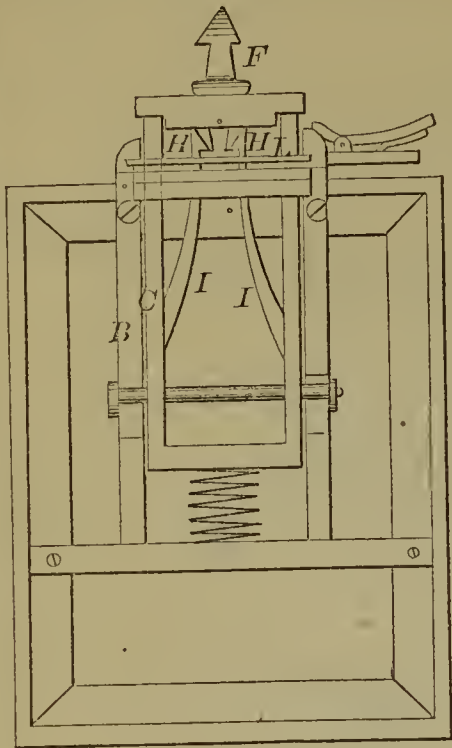
55104—Hinman & Nevill— Car Coupling.
