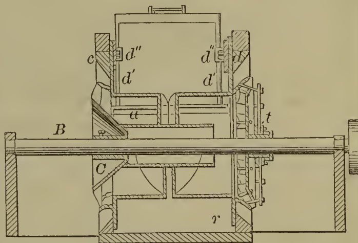
56572—F. J. Kindleberger— Water Wheel.
