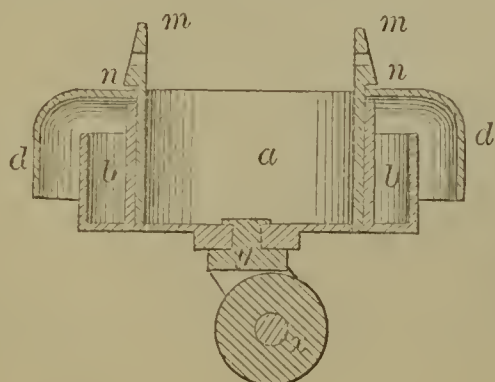
57036—T. Beach—Caster.
