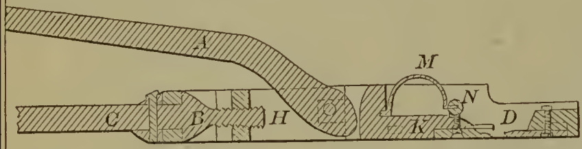
59673—A. J. Smith—Bolt Cutter.
