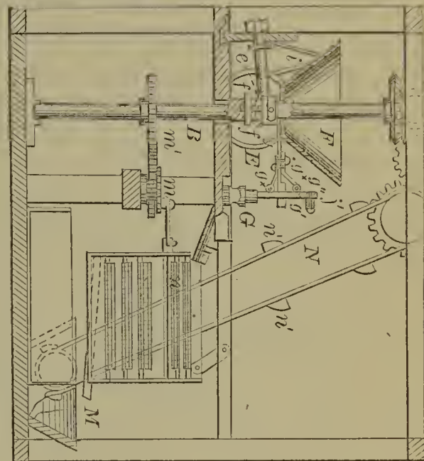
56768—A. Lindsay— Quartz Crusher.
