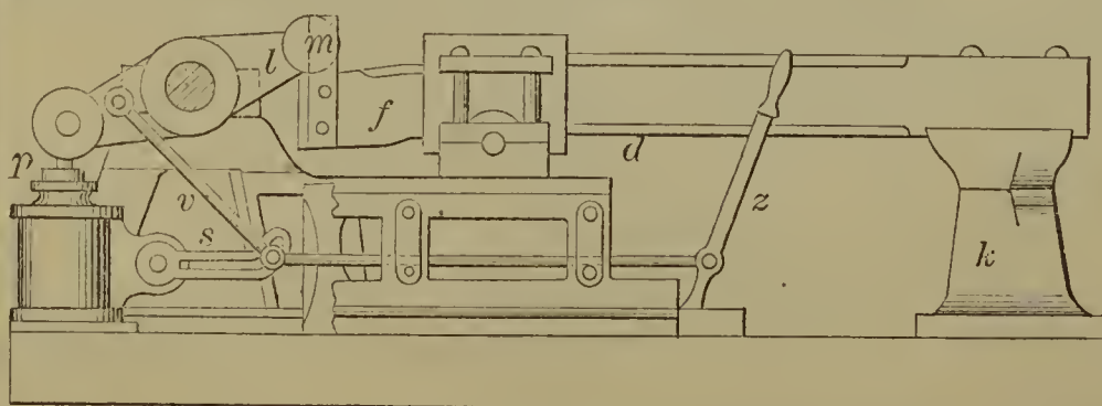
54560—E. L. Kinsley— Steam Hammer.
