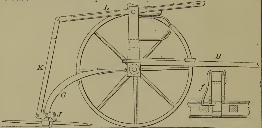
54225—H. M. Smith— Water Elevator.
