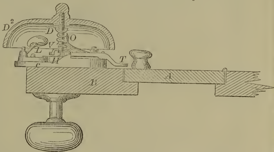
55823—E. H. Crane—Door Bell and Burglar Alarm.
