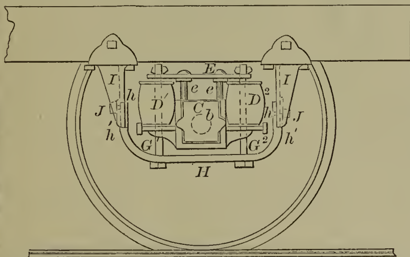
55457—A. Bridges—Suspending Cars upon Springs.
