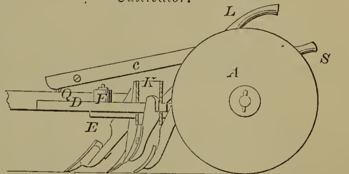
54139—J. L. Fountain—Combined Seeder and Cultivator.
