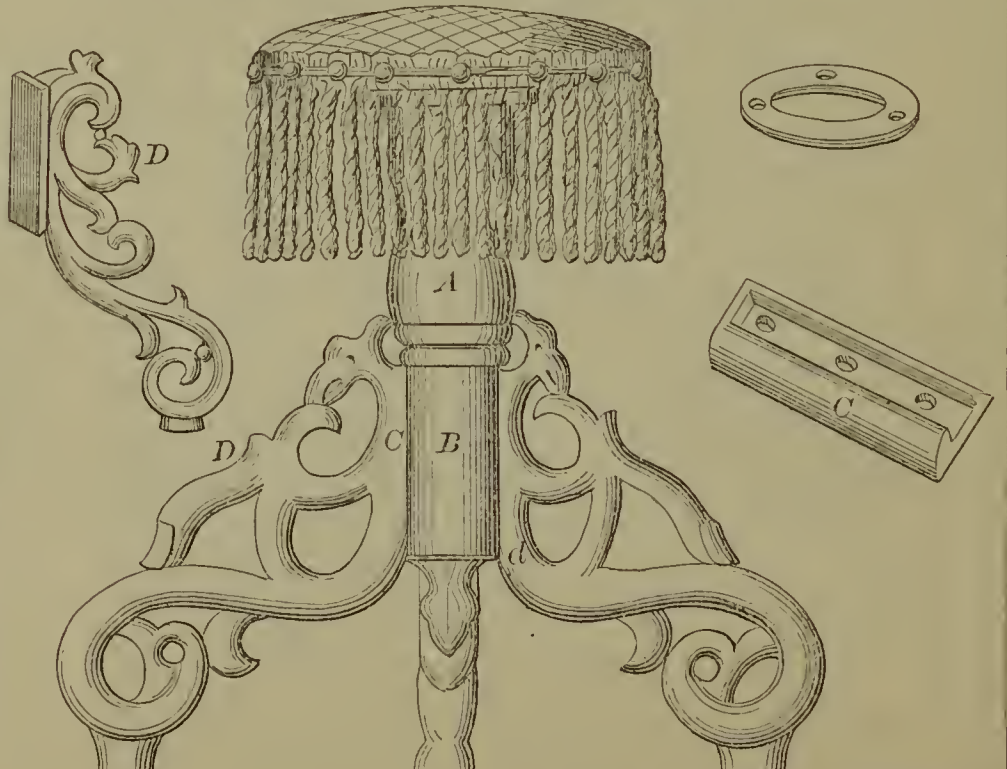
53571—E. D. Castelow— Means of Attaching Legs to Music Stools.
