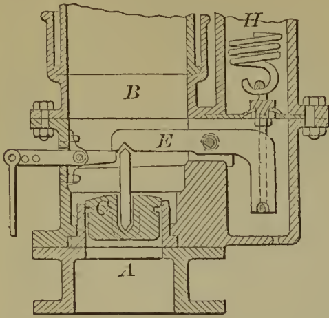
58962—W. Naylor— Steam Safety Valve.
