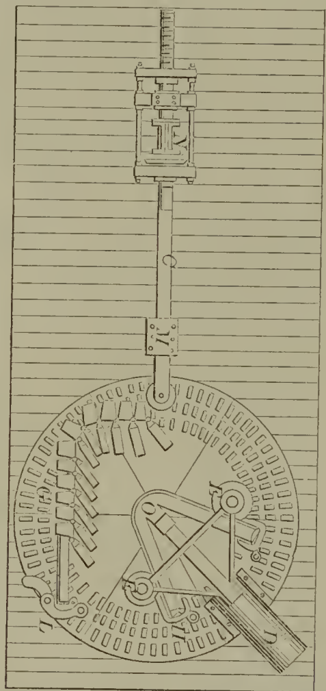
51826—J. W. Griffiths—Wood Bending Machine.
