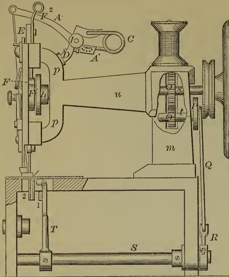
52847—J. Hanlon—Sewing Machine.
