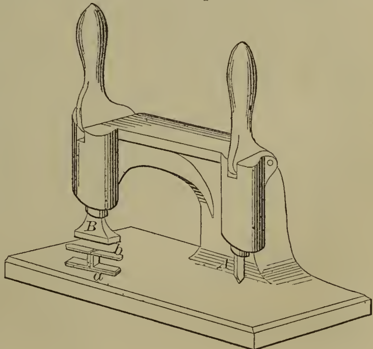
56587—G. W. McGill— Paper Fastener.
