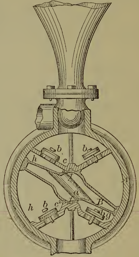
53373—J. E. Hallet—Oscillating Pump.
