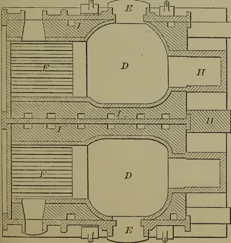
52813—C. D. Baker—Puddling Furnace.
