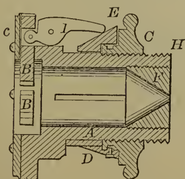
56330—I. Smith—Chuck.
