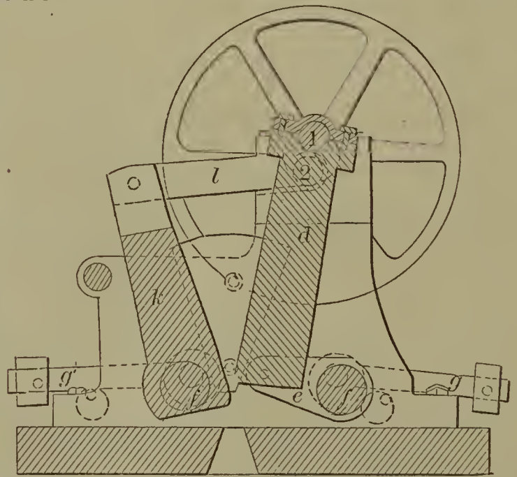
58090—R. G. Fowler— Car Coupling.
