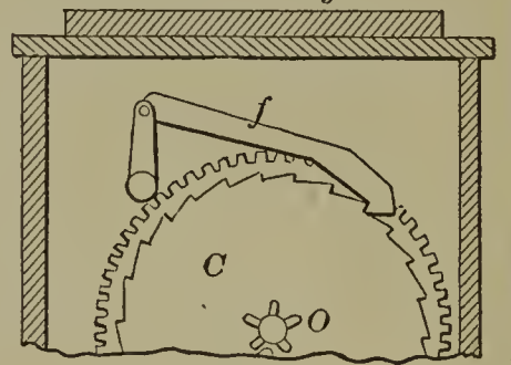
58593—A. J. Burke—Tally Box for Measuring Grain.
