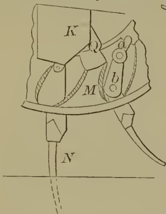
57053—G. M. White— Curtain Ficture.
