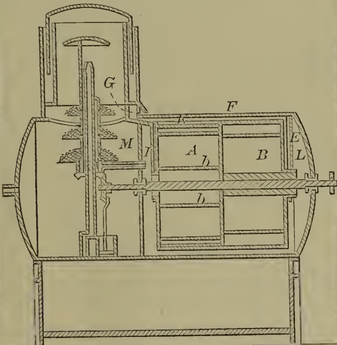
55741—J. B. Terry—Apparatus for Carburetting Air.
