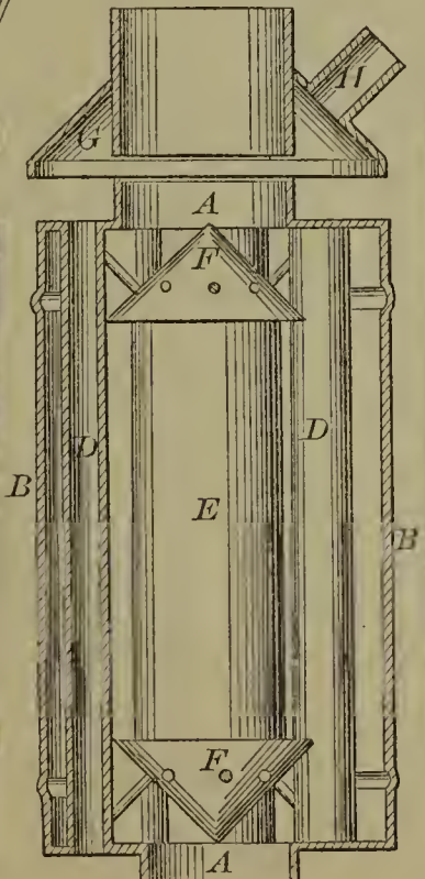
53029—E. P. Morse—Stove Pipe Drum.
