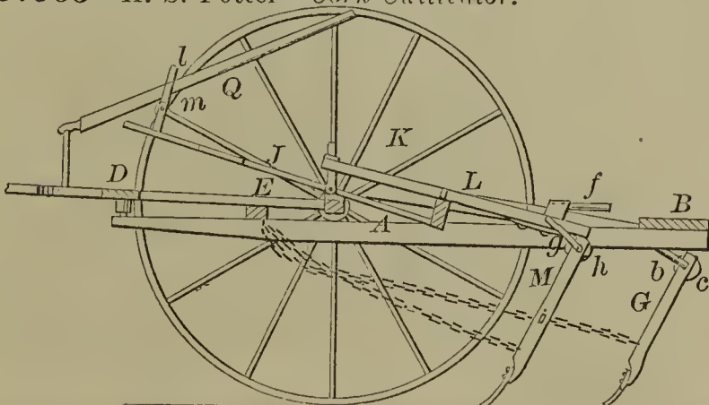
57563—H. S. Potter—Corn Cultivator.
