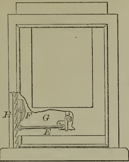
51983—G. W. Wareham—Sash Fastener.
