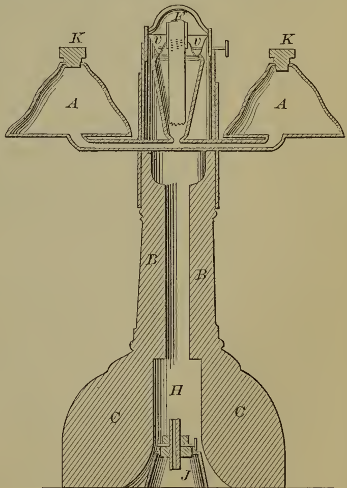
53103—Beidler & Crihfield—Kerosene Lamp.
