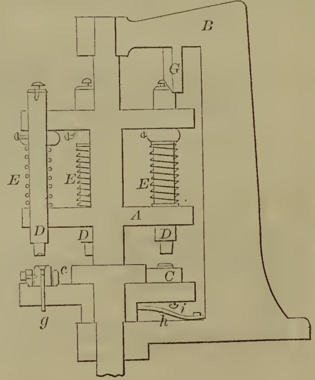
56268—J. C. Rhodes— Tack Capping Machine.
