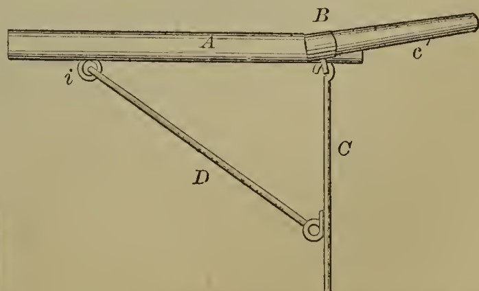
56328—M. C. Remington—Grain Fork.
