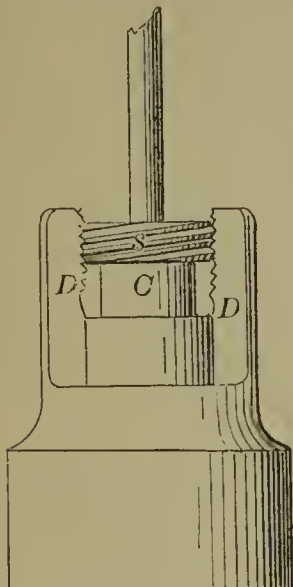
59837—W. Harsen—Stuffing Box.
