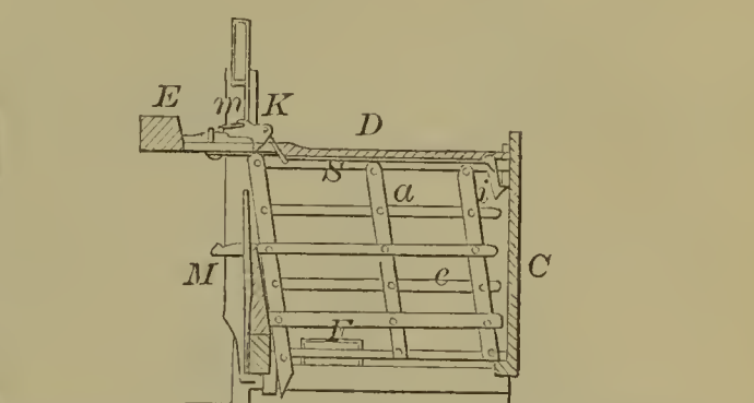
59407—J. Keith— Lathe for Turning Pen Handles.
