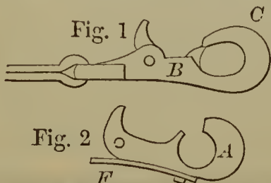
53255—W. Armstrong— Snap Hook.
