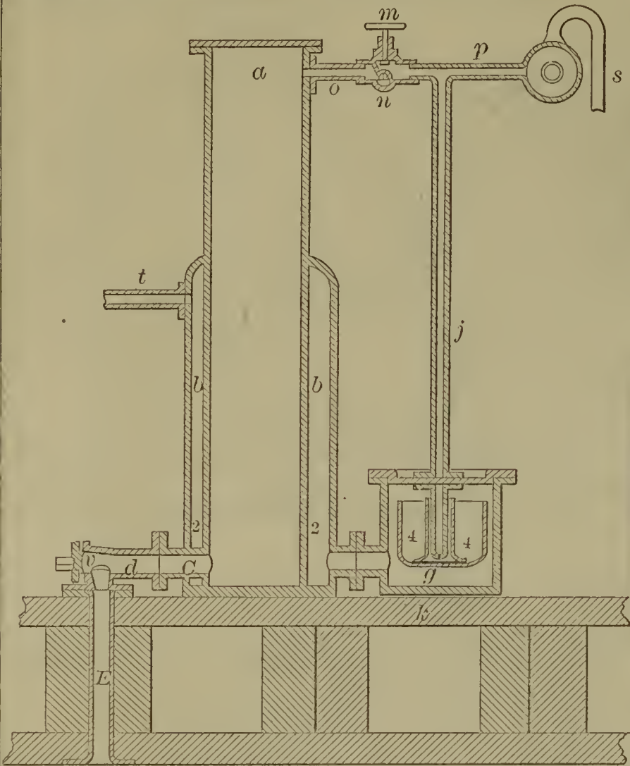
52477—N. W. Wheeler—Relieving Liquids of Gases.
