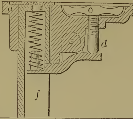
58521—A. Whittemore—For Making Split Spikes.
