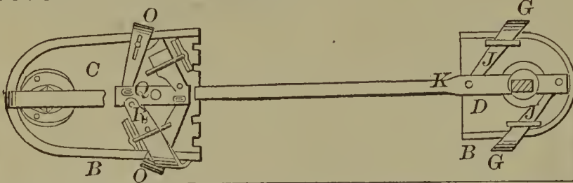
58088—Foreman & Mathowson— Amalgamating Gold with Mercury.
