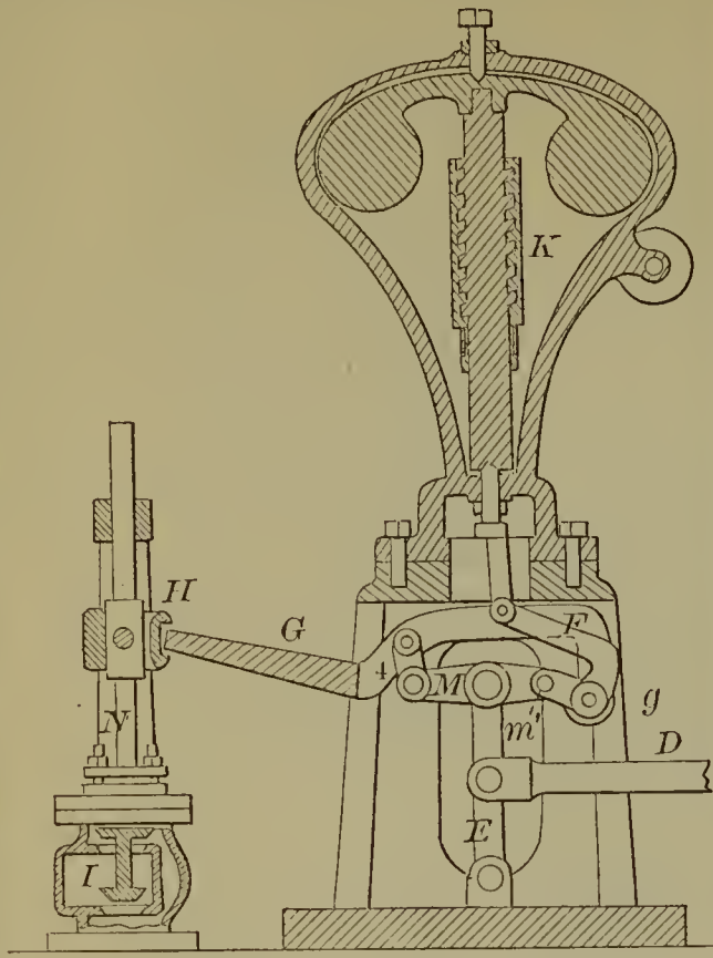
53680—J. T. Rich—Cut-off Valve Gear.
