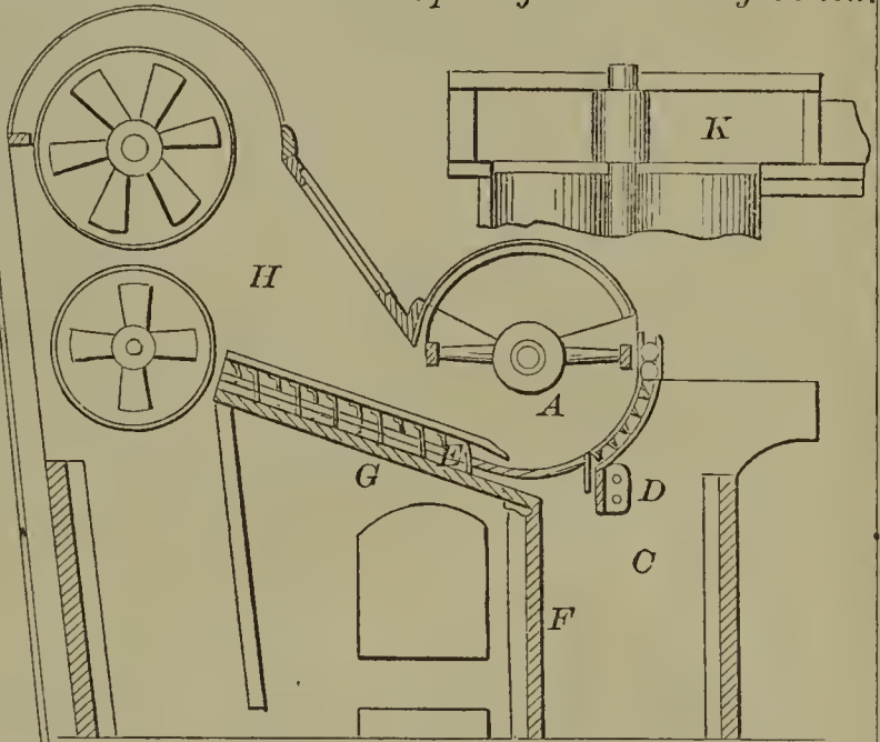
60387—R. Kitson—For Opening and Cleaning Cotton.
