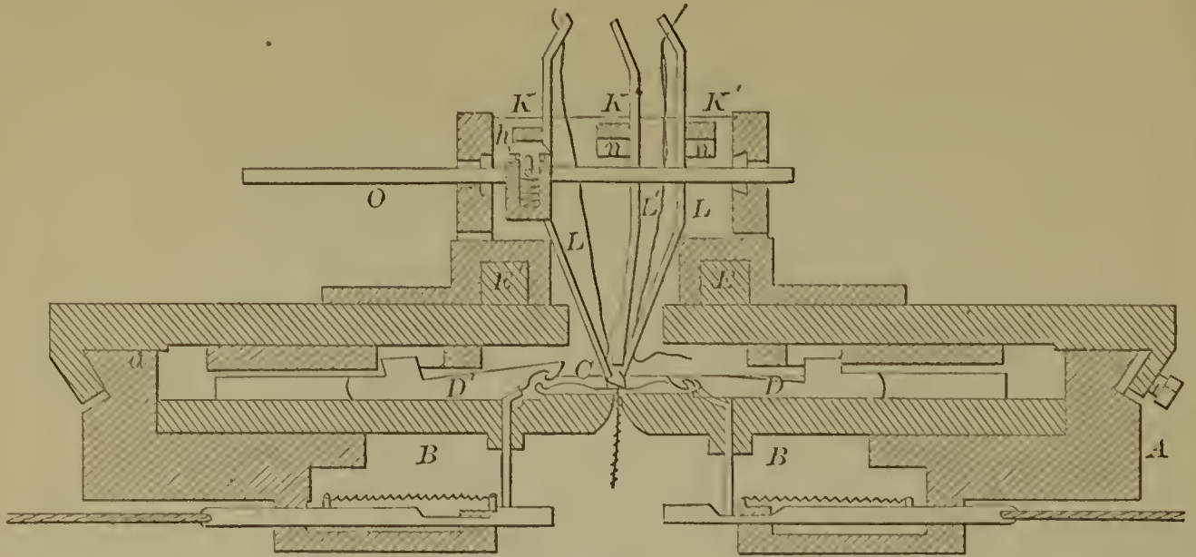
55244—Corbett & Burns— Lock.
