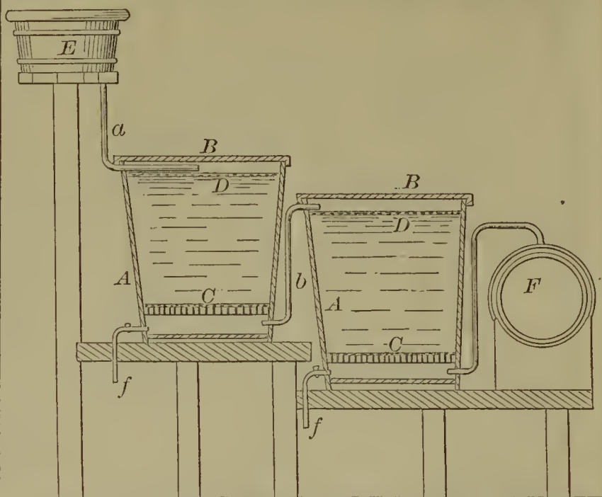
56197—G. W. Ferris— Refining Spirituous Liquors.
