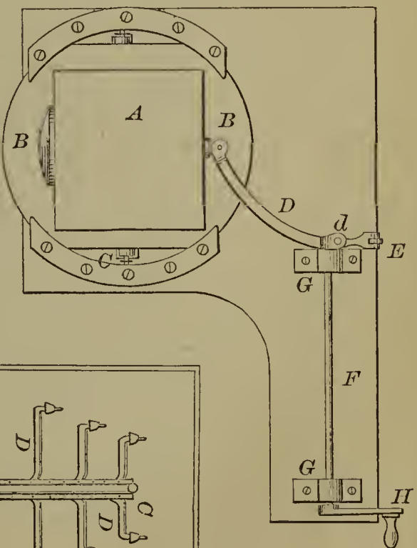
54714—C. D. Gibson—Adjustment of Headlights.
