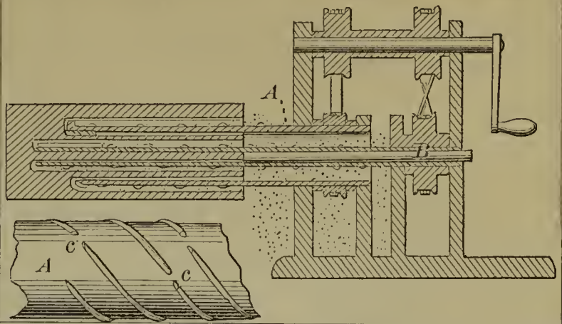
53900—T. P. Thorpe—Exercising Machine.
