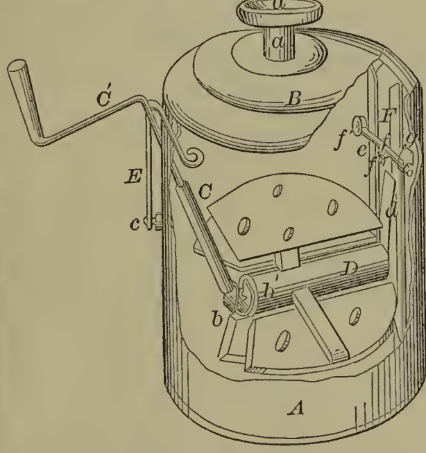
55996—J. Boyers—Churn.
