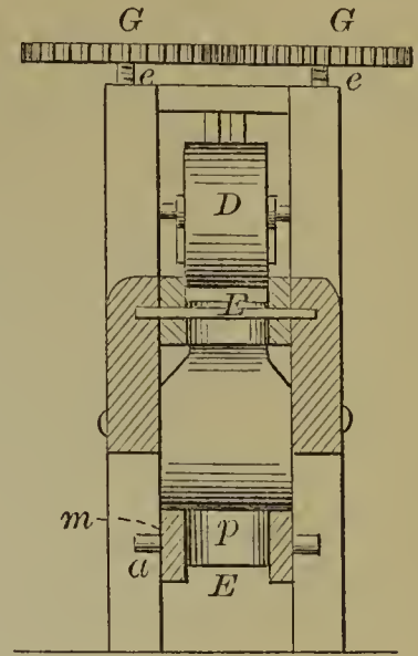
53105—J. Blackie—For Making Plug Tobacco.
