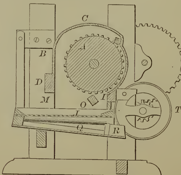
55485—W. Gilman—Corn Sheller.
