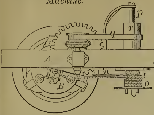
56372—C. Cobb—Cordage Machine.
