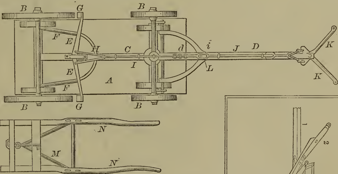
52595—L. C. Percival—Wagon Brake.
