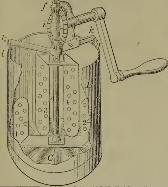
57573—G. H. Sanborn—Churn.
