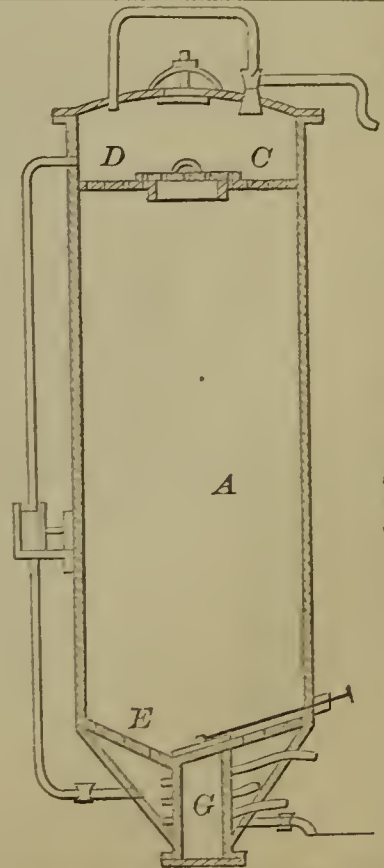
55253—J. W. Dixon—For Pulping Wood.
