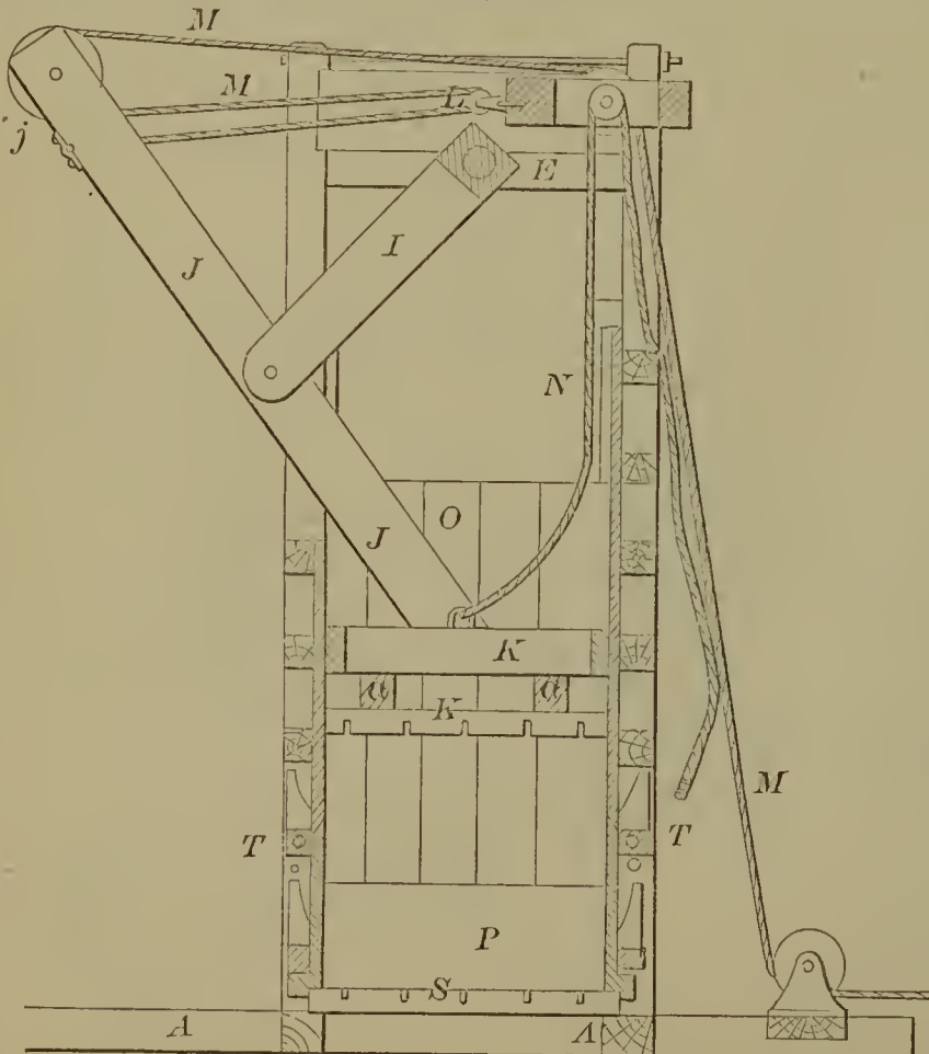
59309—H. A. Ashley—Baling Press.
