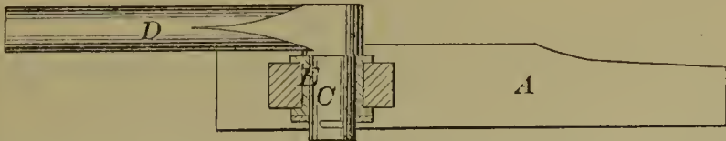
52811—J. Anderson—For Driving Fence Posts.
