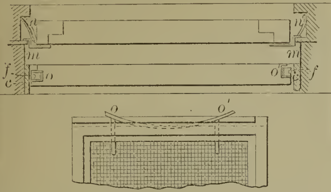
56994—E. A. G. Roulstone— Mosquito Bar.
