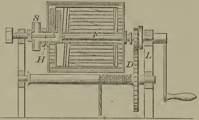
51946—Hutchinson & McAvoy— For Carburetting Air.
