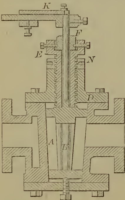
59565—J. L. Dickinson— Valve Device for Steam Engines.
