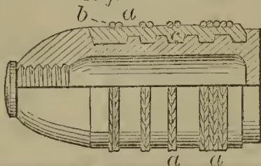
55761—L. W. Broadwell—Packing Projectiles for Rifled Ordnance.
