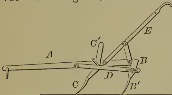
57719—J. Hollinger—Cultivator.
