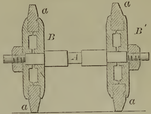
51895—H. Hall—Drawing Rollers for Spinning.
