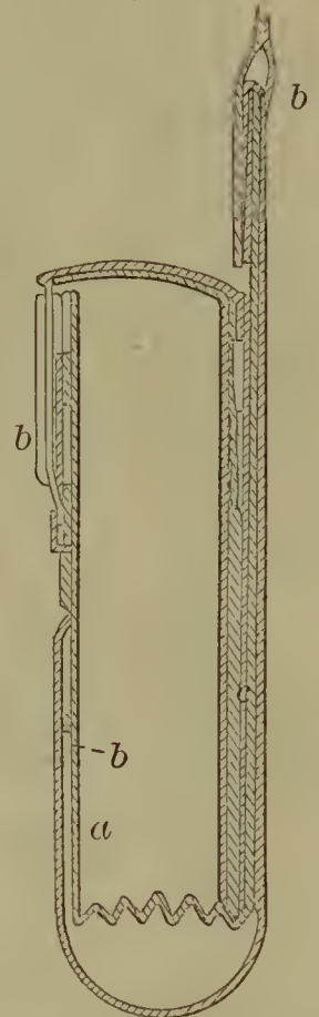
56248—G. A. Mitchell—Safety Pocket.
