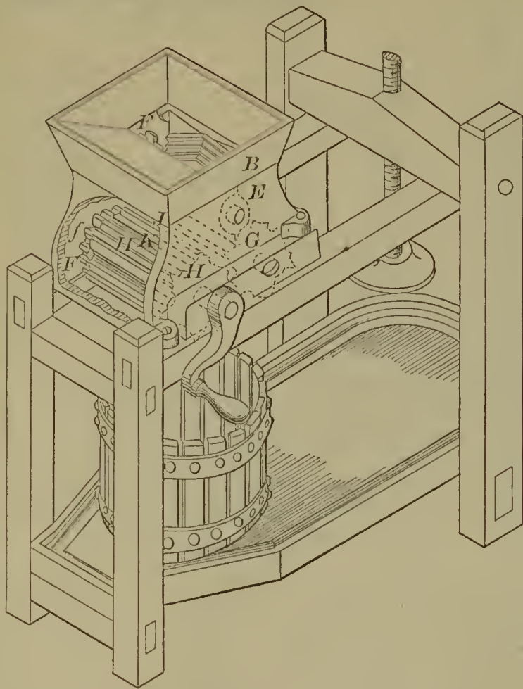
52583—S. Males—Cider Mill.
