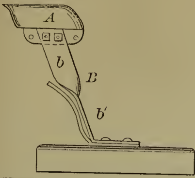
54246—N. B. Brown— Device For Lubricating Axles.
