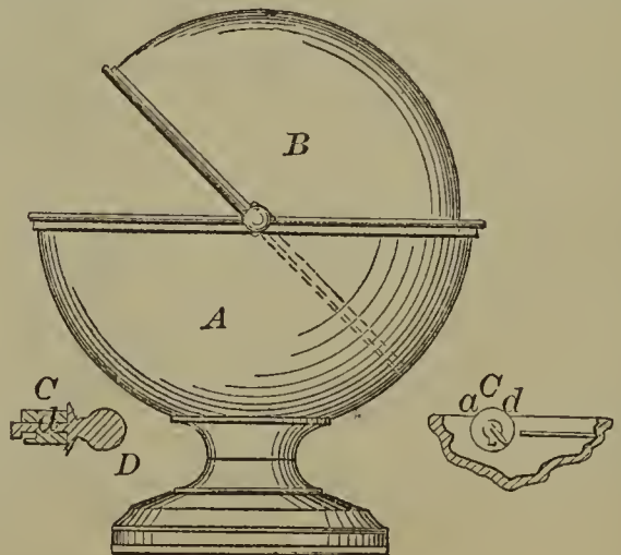
60308—W. M. Whittaker—Butter Dish.
