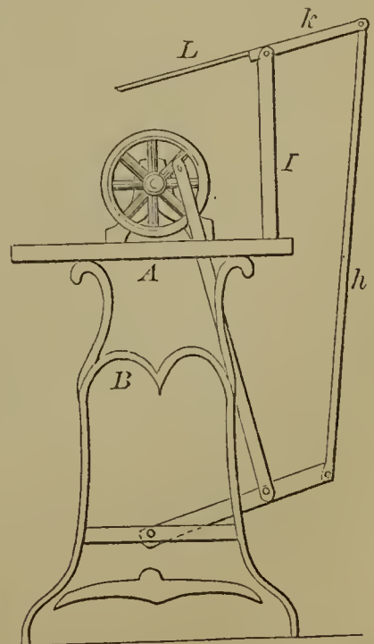
58333--S. Burr--Sewing Machine Foot Attachment.
