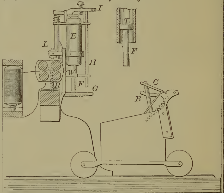
56829—J Sutherland—Self-Acting Mule.
