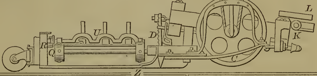
56519—J. Briggs—Clamp for Holding Saws.
