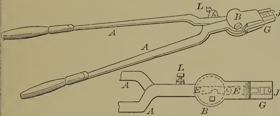
57705—J. Guthrie—Bolt Cutting Shears.
