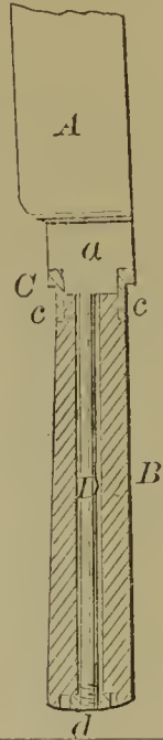
57677—W. Clayton— Attaching Knives to Handles.
