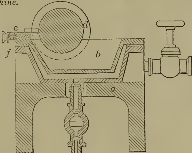
55335—Merriam & Norton—Glueing and Cementing Machine.
