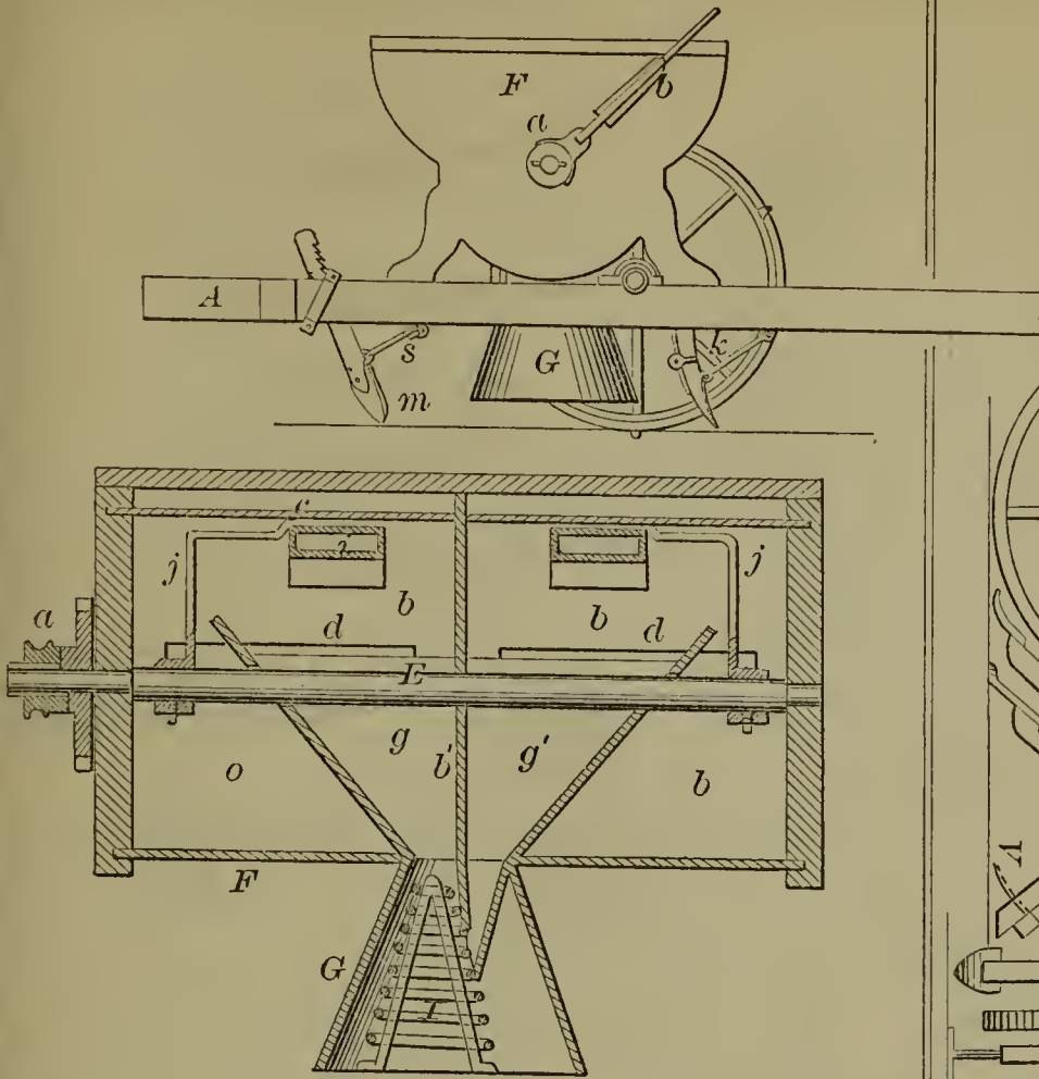
53910—J. Watrous, Jr.—Cotton Gin.
