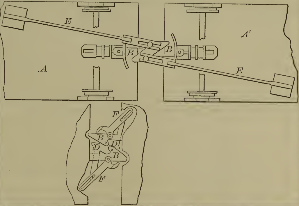
52736—Newell & Simmerman— Car Coupling.
