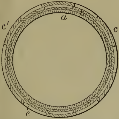
56620—T. P. Shaffner— Packing Nitro-Glycerine.
