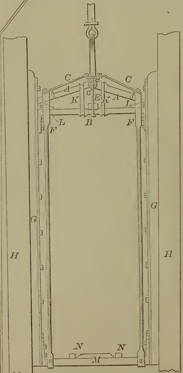
54490—Berry, Hochholzer & Denver—Cage for Hoisting.
