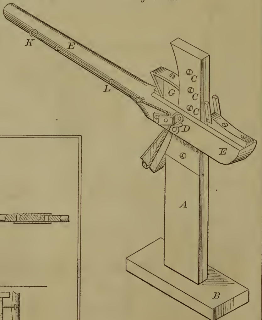
56510—M. Andriot—Carriage Jack.
