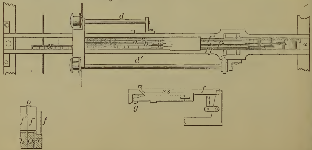
59675—Soule & Sholes—Numbering Machine.
