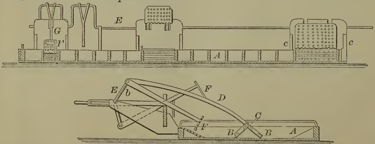
57954—R. C. Nourse—Evaporator.
