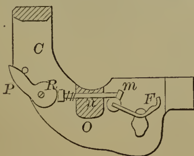
54926—W. M. Leavens— Sewing Machine.
