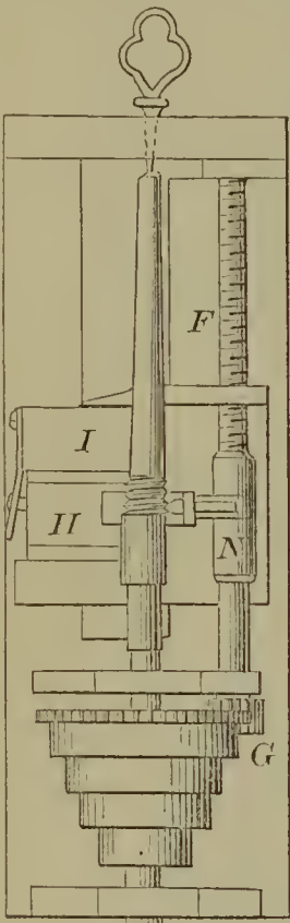
55493—B. Hotchkiss— Screw Tap.
