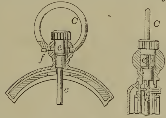
57495—E. A. Giles— Stem Winding Watch.
