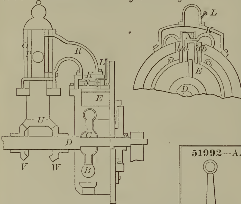
51996—W. Goodwin—Rotary Steam Engine.
