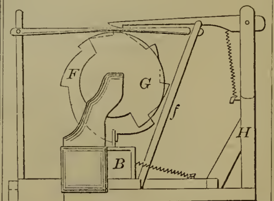
53858—I. Orndorff—Loom.
