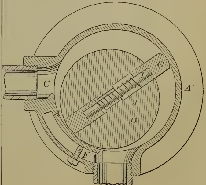
54581—J. J. Morris— Rotary Pump.
