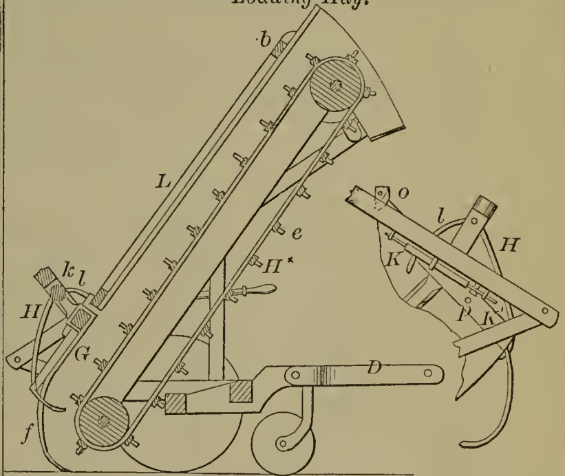
53464—W. D. Mayfield— Machine for Raking and Loading Hay.
