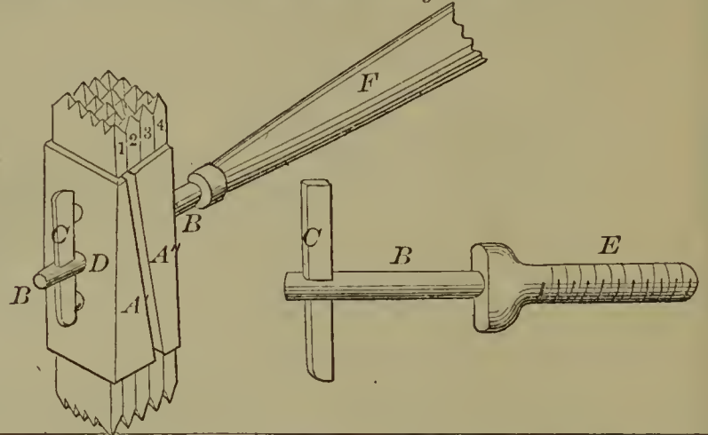
54256—Putnam & Dwelley— Horse Shoe Nail Machine.
