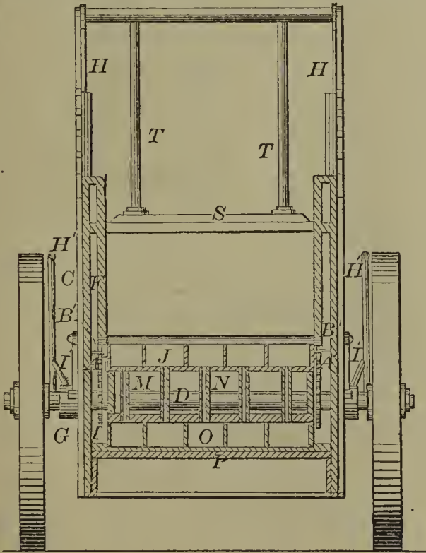
60323—W. C. Bartol—Brick Machine.
