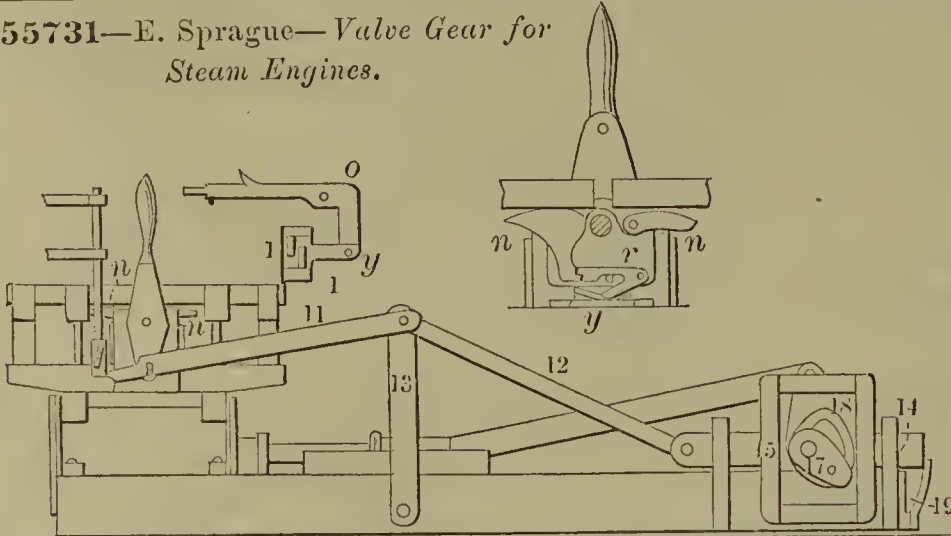
55732—Springer & Bartram— Indicator for Steam Generators.
