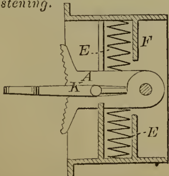
56347—B. Beach— Sash Fastening.
