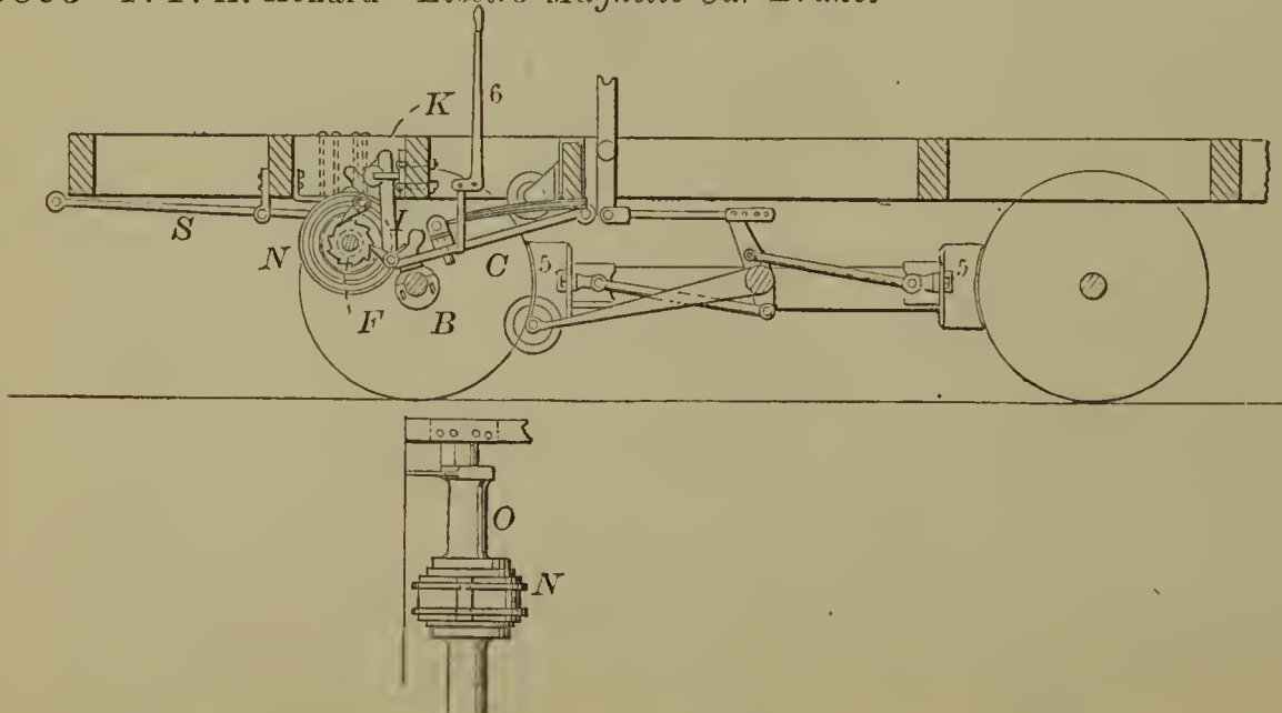
59805—F. F. A. Achard— Electro-Magnetic Car Brake.
