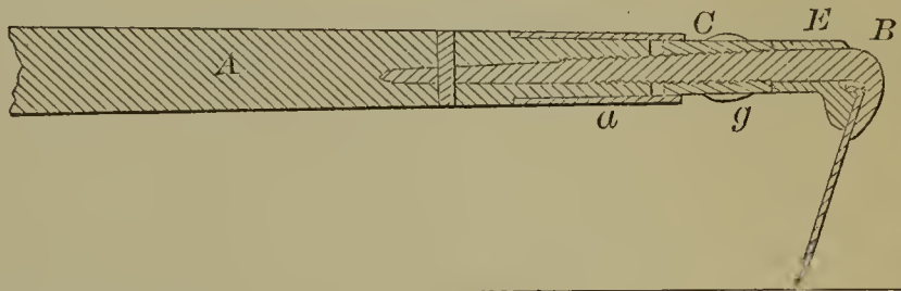
55000—A. Boyden— For Attaching Handles to Rakes, &c.
