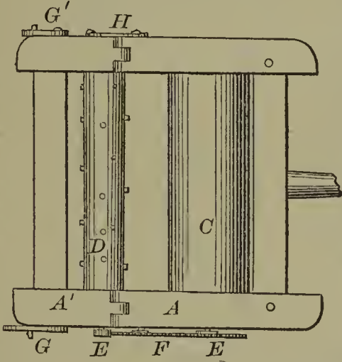
57961—A. Pierce—Combined Harrow and Marker.
