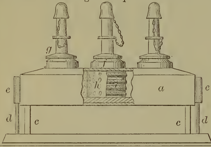
55261—J. H. Elward— For Separating Metals from Ores.
