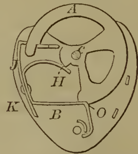
56451—Saladee & Armstrong—Padlock.
