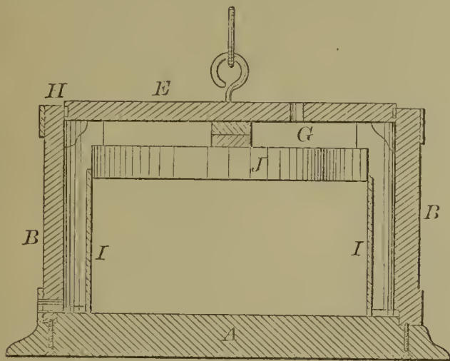
59475—W. H. Stevens—Cheese Press.
