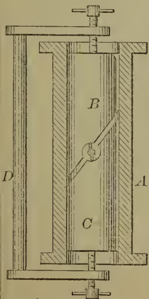
57062—R. B. Angus— Throttle Valve Mould.
