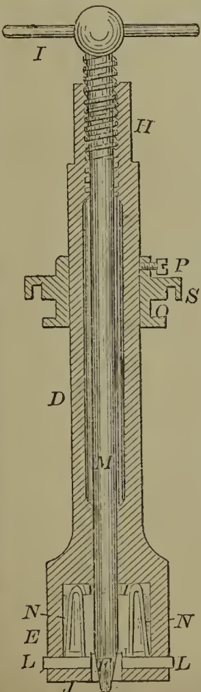
58886—Ransey & Miller— Tool for Cutting Boiler Tubes.
