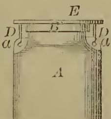
56755—W. Hunt—Fruit Jar.
