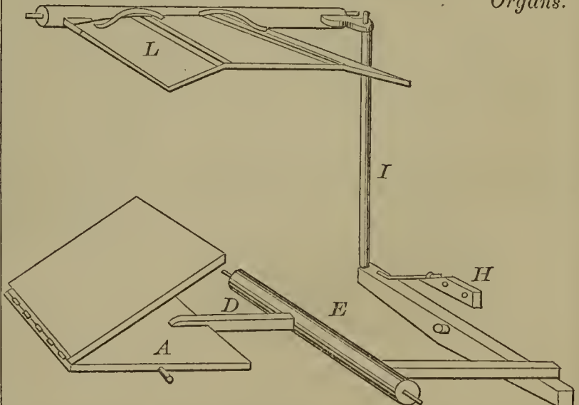
52771—A. E. Thompson—Operating the Swell of Organs.
