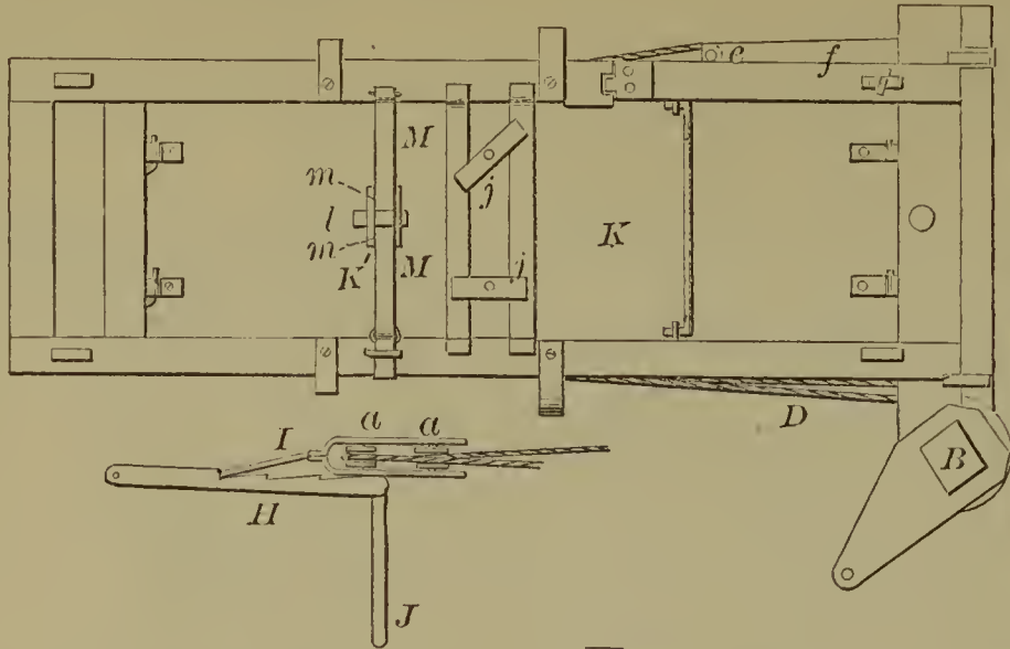
59832—C. W. Gillis— Baling Press.
