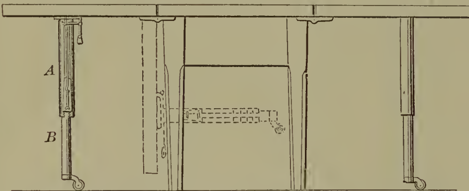
59974—A. Cutler—Table Leaf Support.
