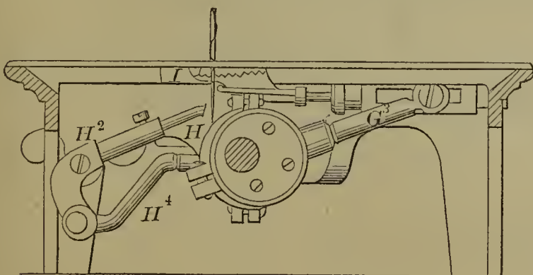
55029—J. Hayes— Sewing Machine.
