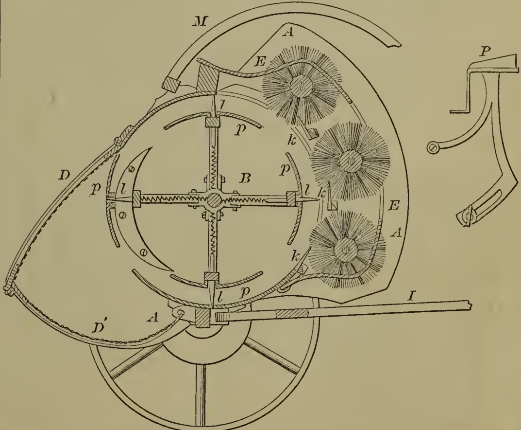
53901—A. Tiensch—Cotton Picking Machine.
