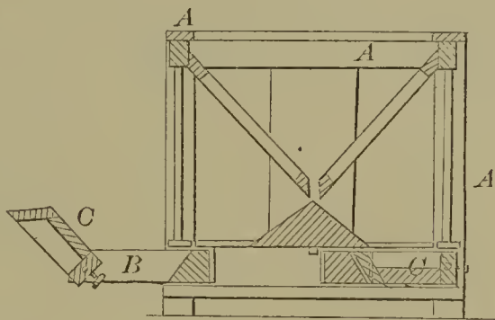
59240—M. T. Lincoln—Bookbinder's Sewing Table.
