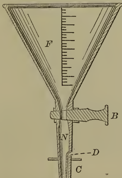
55941—A. H. Whitney—Measuring Funnel.
