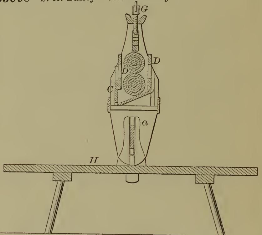
53098 —S. A. Bailey— Clothes Wringer.
