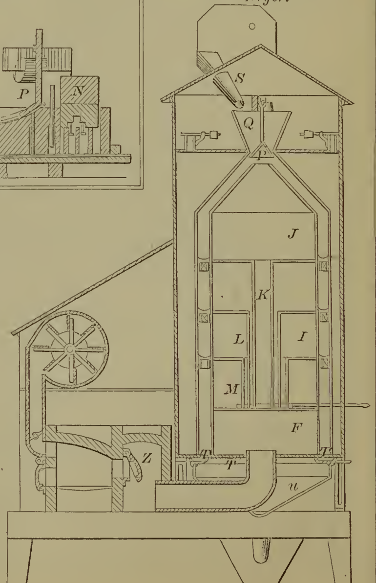
56708—G. Clark— Grain Dryer.
