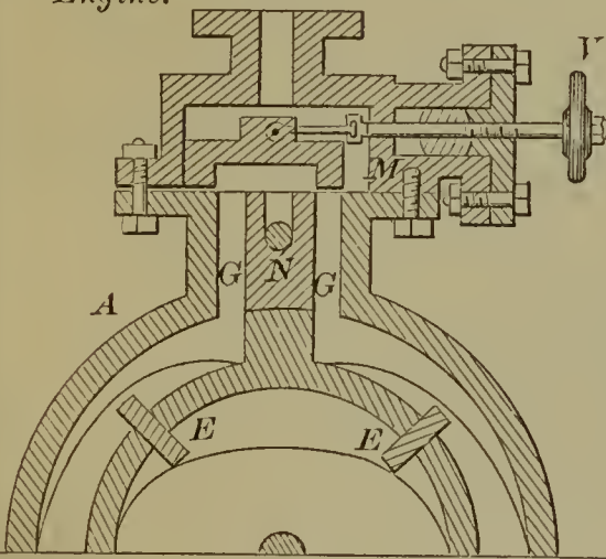
54079—F. Chatelain—Rotary Engine.
