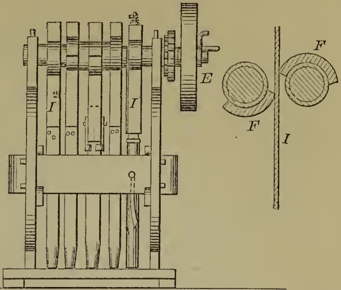
53319—J. M. May— Quartz Crusher.
