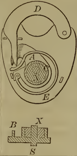
56450—C. W. Saladee—Padlock.
