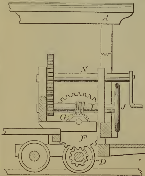
57623—J. W. Conway—Propelling Street Car.
