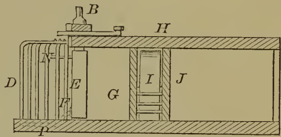
54890—D. Garrison—For Jointing Oval Frames.
