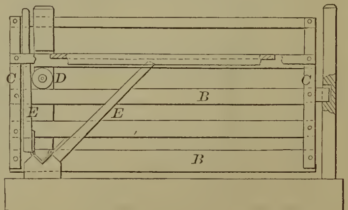
54641—D. B. Baker—Gate.
