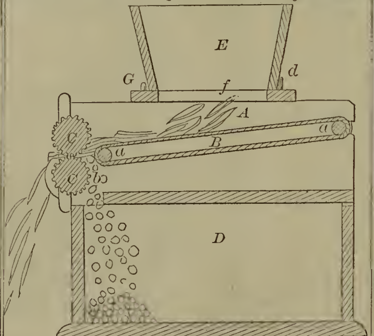
52356—Bray & Talpey—Pea Shelling Machine.
