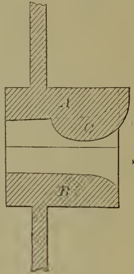
54643—J. Fieldhouse—Die for Forming Gas Pipes.
