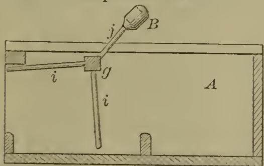
52678—Clark & Jenks— For Mixing Dough.
