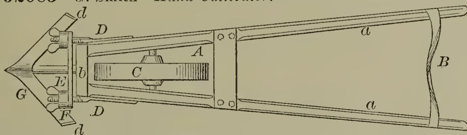
52082—W. H. Sears—Tide Wheel.
