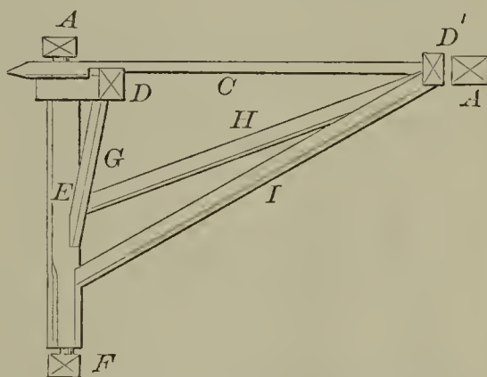
51939—S. Godfrey—Bolt for Flouring Mills.
