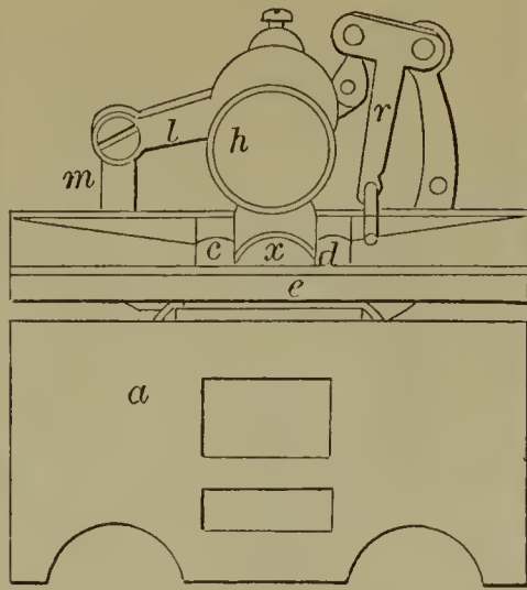
54195—P. H. Niles—For Soldering Tin Cans.
