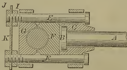
57140—B. J. Hunter— Harvester Pitman.
