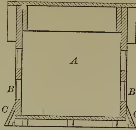
59931—L. S. Stevens—Metallic Smoke House.
