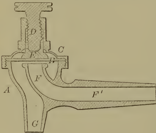
59346—W. Blake— Diaphragm Faucet.
