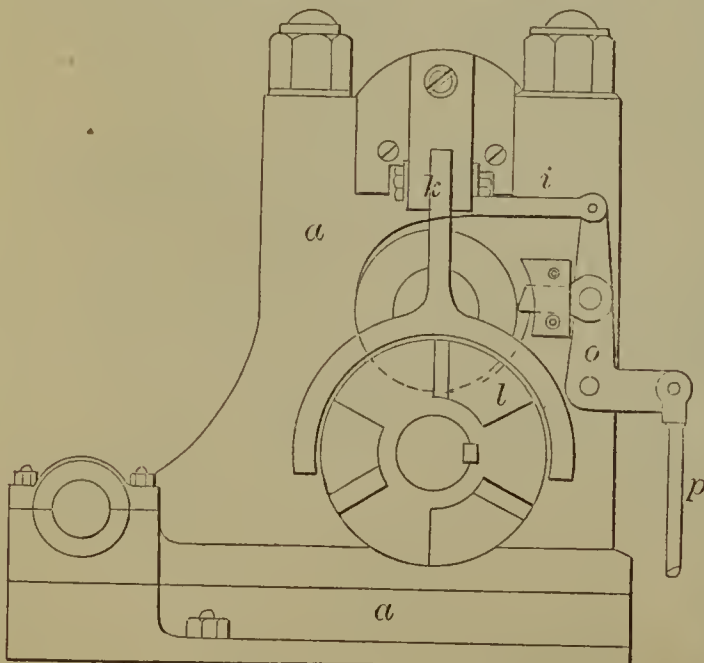
54310—J. Dodge— Shaping File Blanks, &c.
