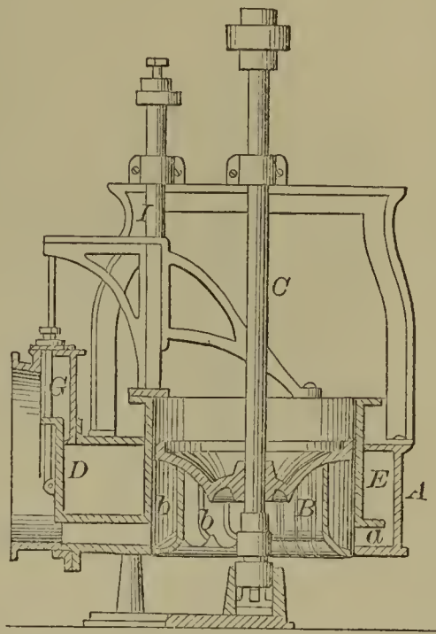
52625—J. Tyler— Turbine Water Wheel.
