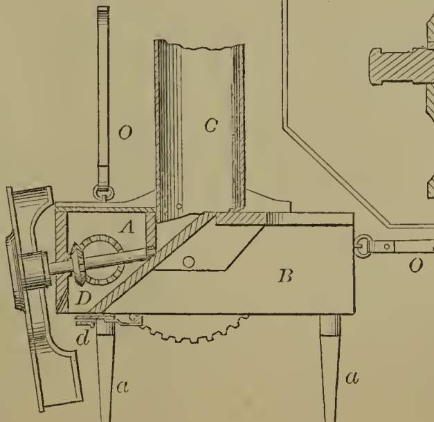
58217—Clark & Splitdorf— Insulating Wires of Helices.
