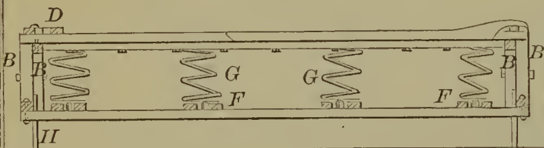
56844—Wilsey & Forbes—Bed Bottom.
