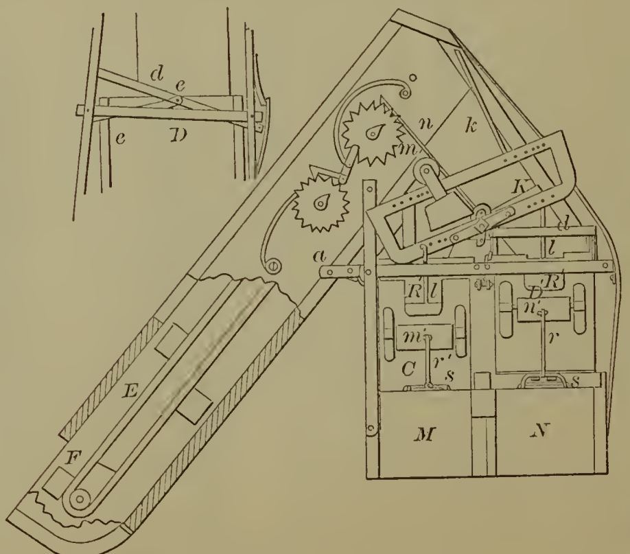
53553—D. D. Armes— Weighing and Measuring Grain.
