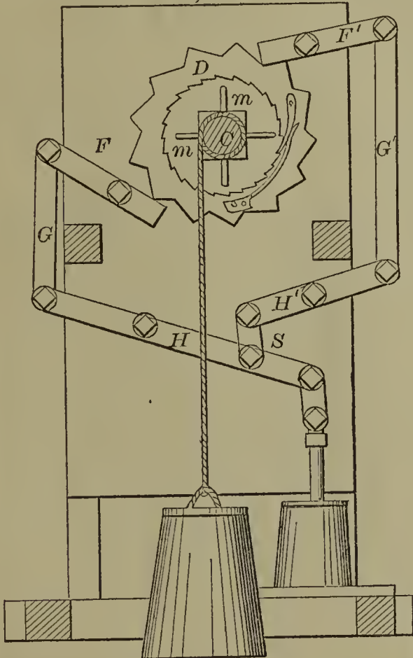
60232—J. P. Nichols—For Operating Churns, &c.
