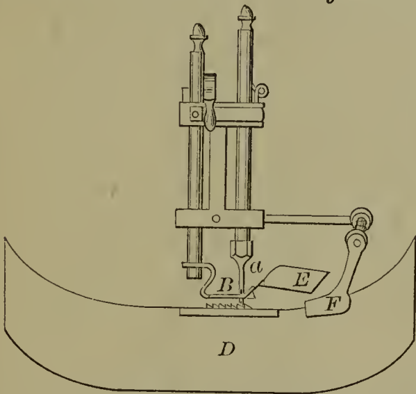
53928—Sheffield & Palmer— Device for Detaching Bolts from Davits .
