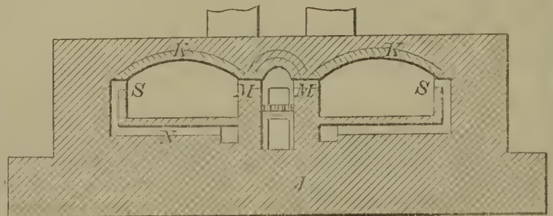
52605—S. Reynolds— Oven for Annealing Iron.
