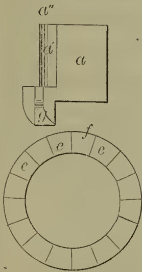
52224—F. Swatzel— Water Wheel.
