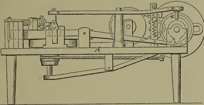
57873—C. O. Crosby—Wire Pointer.
