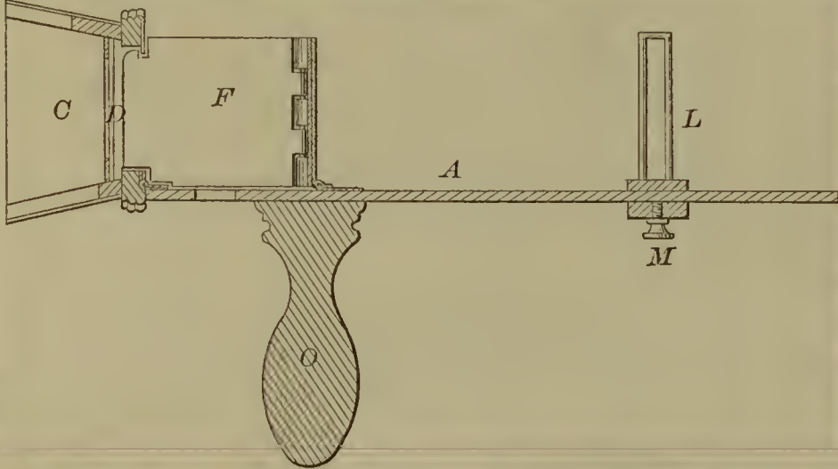
52744—A. Quirolo—Stereoscope.
