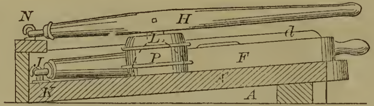
56113—W. G. Smith— Car Spittoon.
