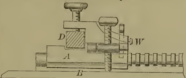
57191—J. J. Russ—Planing Machine.
