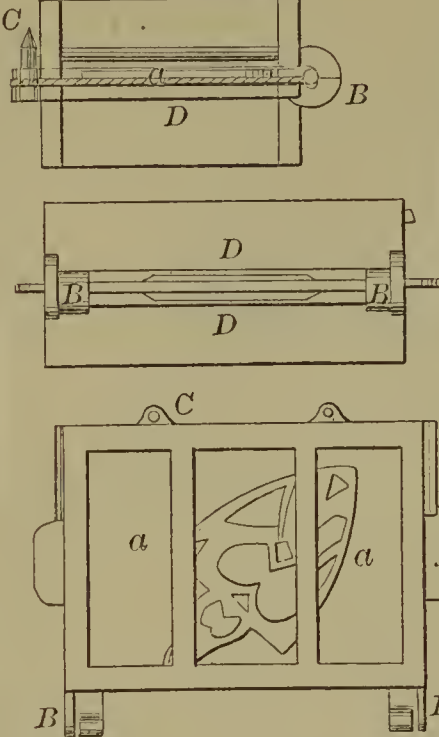
58173—E. C. Little—Moulders' Flask.
