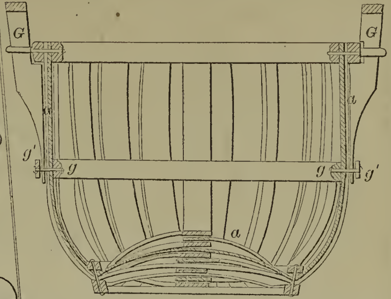
60387—R. Kitson—For Opening and Cleaning Cotton.
