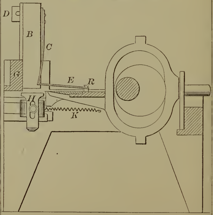
54180—C. Learned— Cutting Lath.
