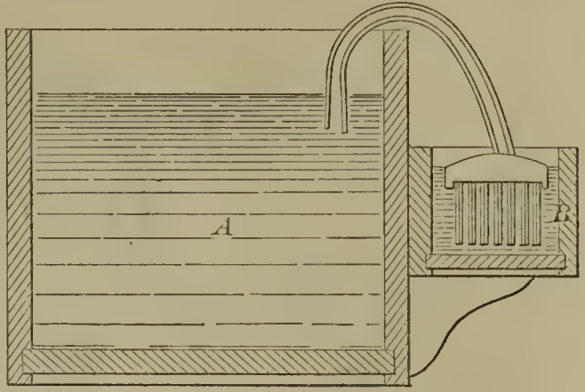
52450—J. Russell—For Hardening Files.
