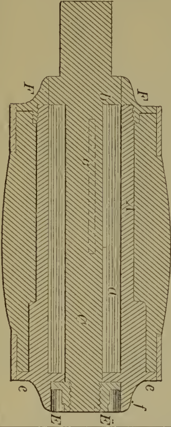
59781—J. T. Rittenhouse— Churn Dasher.
