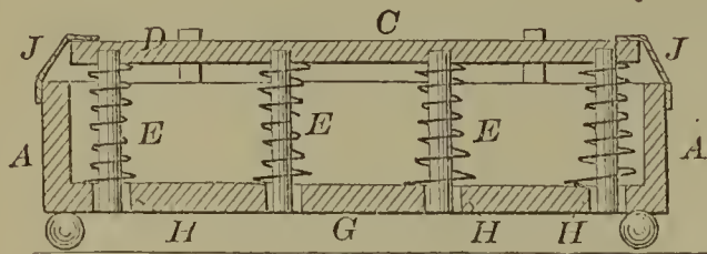
58915—F. J. Tinker—Lamp Chimney Attachment.
