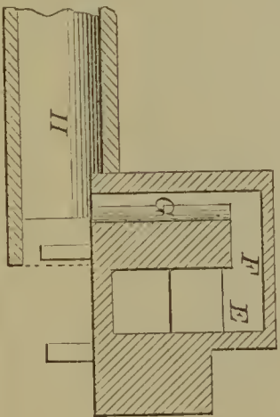
56725—J. Davies—Copper Smelting Furnace.
