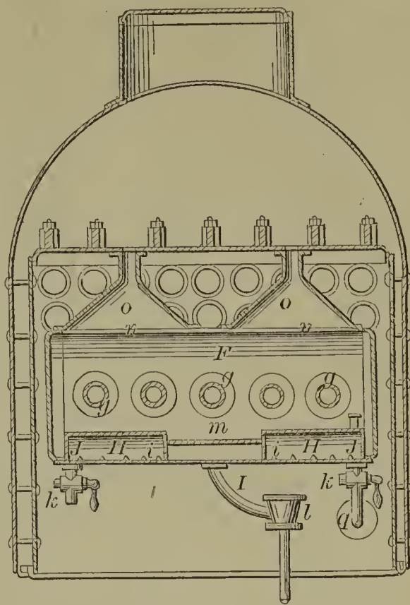
60124—T. E. Belton—Steam Heater.
