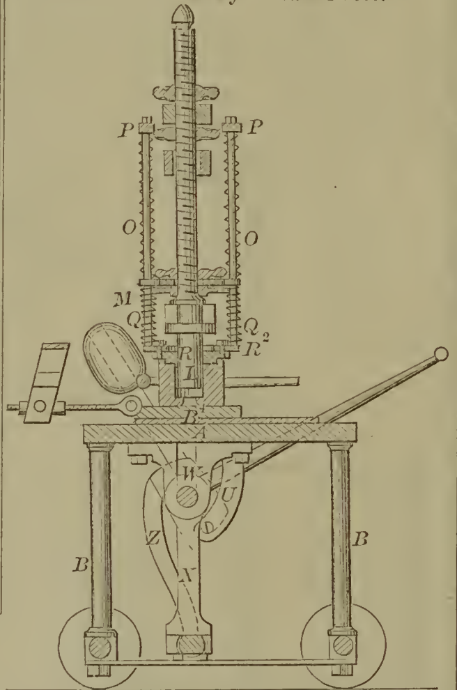
57296—H. Dillaway— Glass Press.
