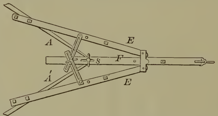
57953—W. Nichols—Steam Engine Governor.
