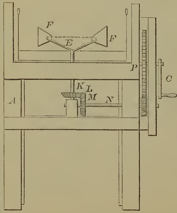
59598—Hasket & Cox—Centrifugal Machine for Draining Sugar.
