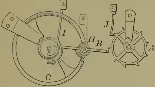
59660—C. Rogers—For Hitching Horses.
