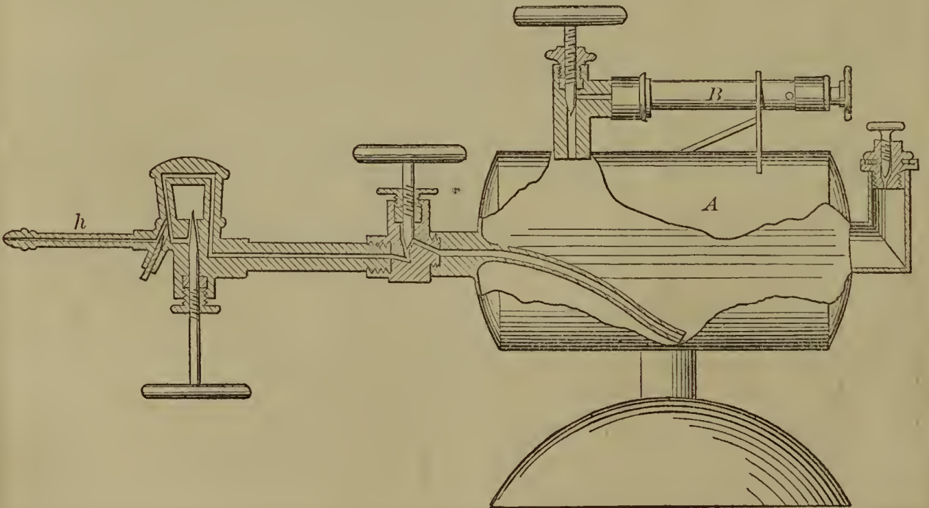
56051—J. S. Hull—Soldering Lamp and Blow Pipe.
