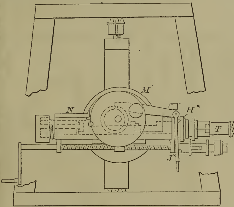
55308—E. Kay— Stop Motion for Knitting Machines.
