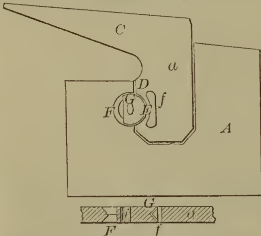
57092—E. Coleman—Wheel Tire.
