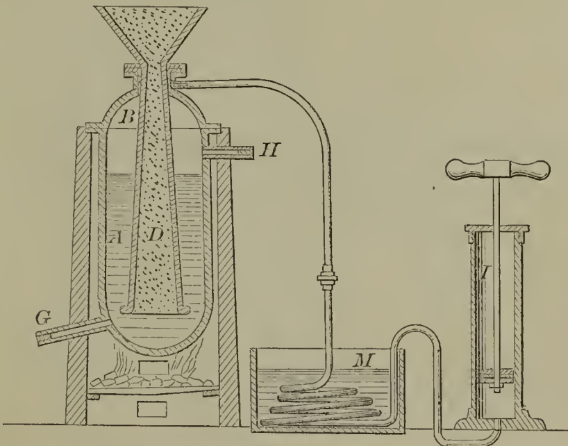
51822—W. M. Fuller— For Extracting Gold from Quartz, &c.
