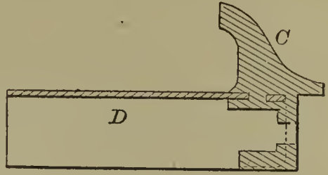
57957—C. Parker—Vise.
