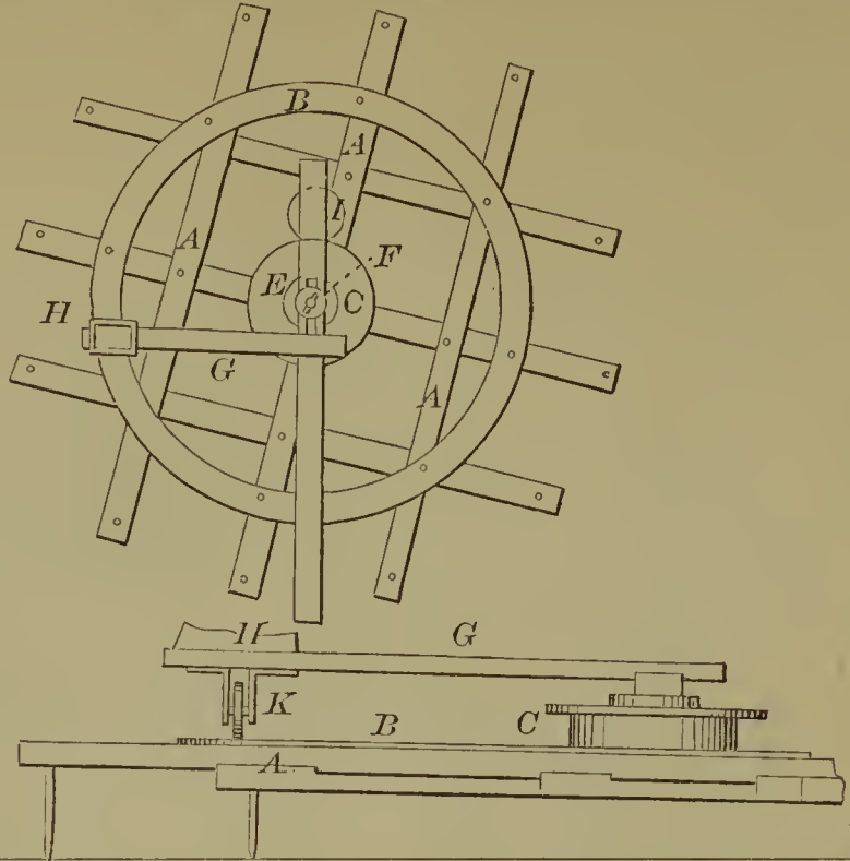
58191—S. Grenell—Rotating Harrow.
