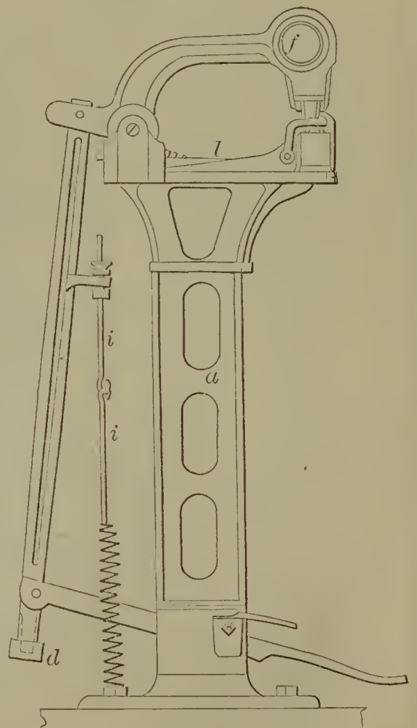
55813—J. T. Bruen—Hammer for Bending Couplings.
