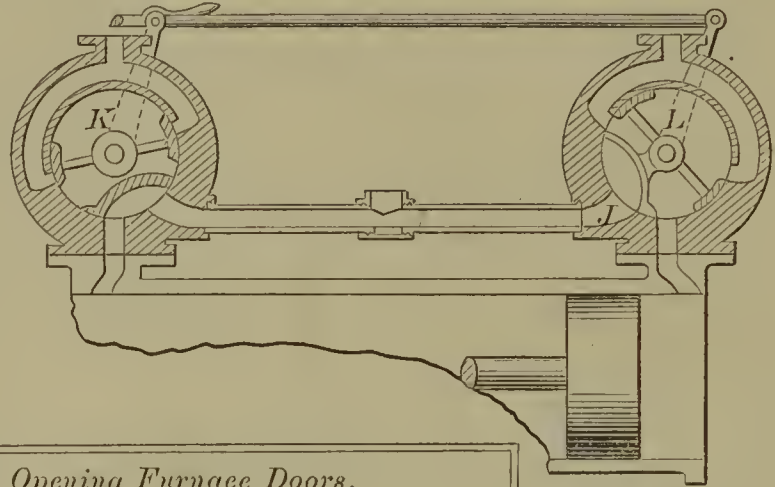
58799—Fessler & Maxell—For Opening Furnace Doors.
