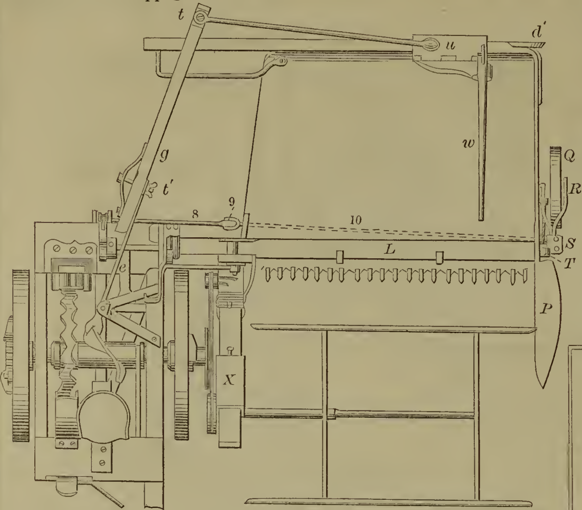
55767—J. Gardner—Capping Wood Screws.
