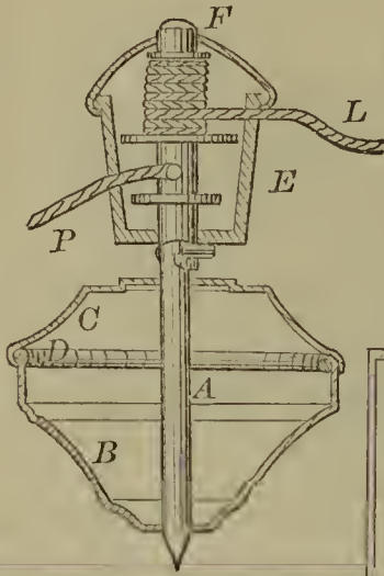
55593—P. Dinzey— Anchor.
