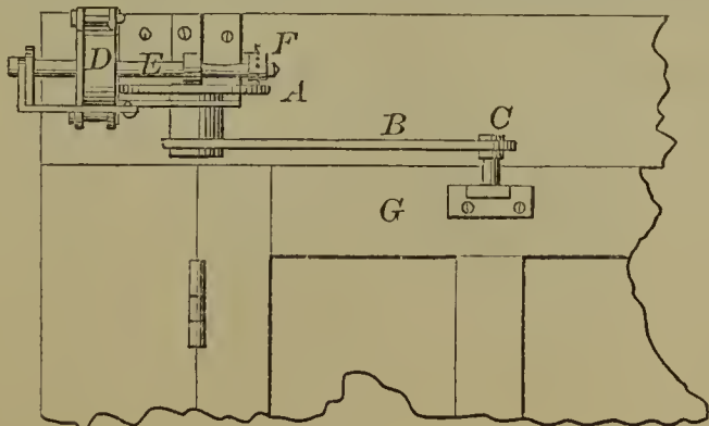
59667—G. K. Coates—Mechanism for Closing Doors.
