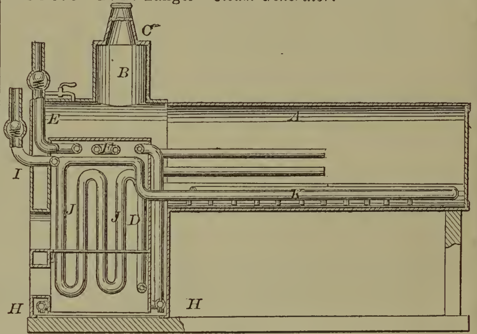
60279—D. B. Tanger— Steam Generator.
