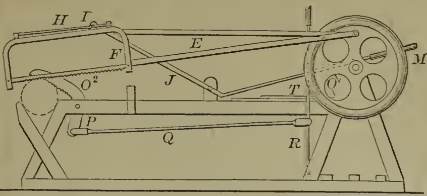
58933—I. Allard—Wood Sawing Machine.
