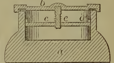
59111—L. J. Wicks—Fruit Can.
