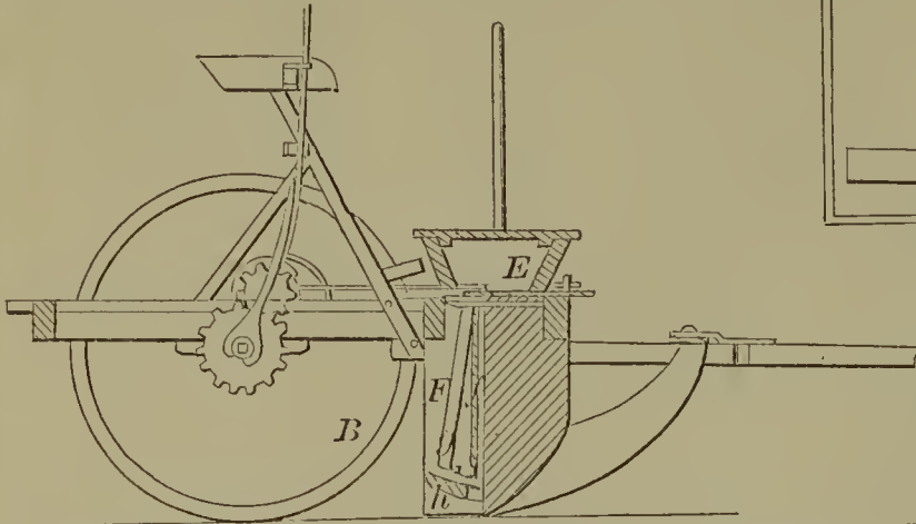
58876—C. C. Myers—Corn Planter.
