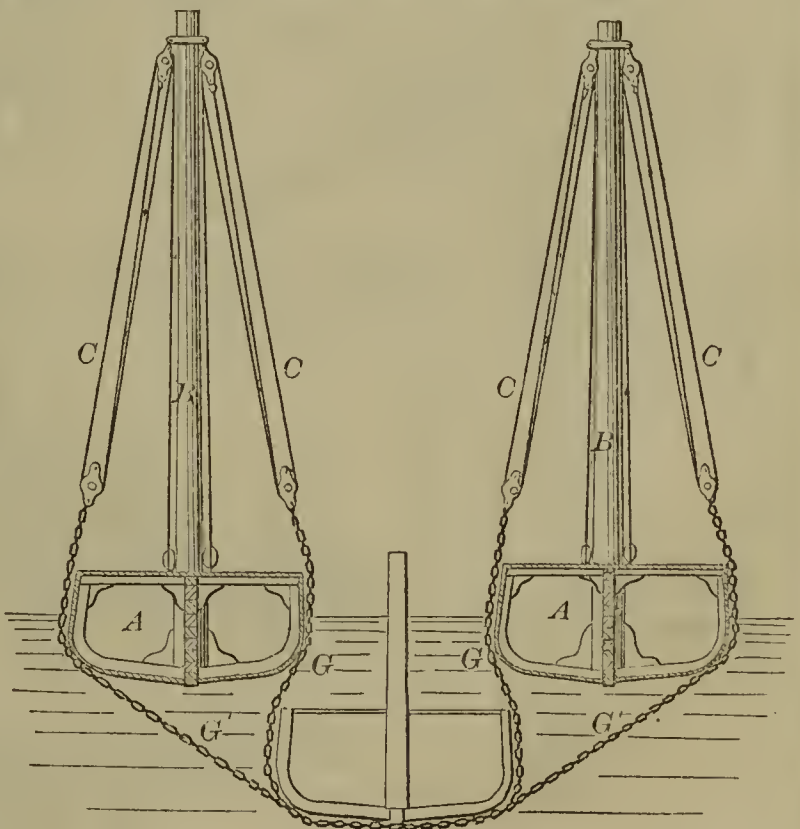
57183—S. Petre—Derrick for Raising Sunken Vessels.
