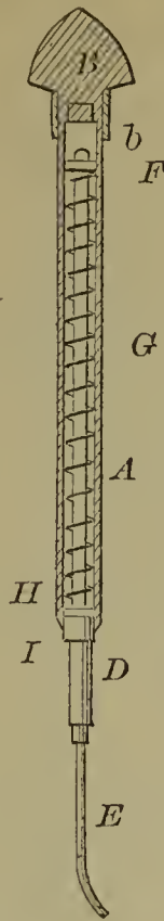
58257—C. M. Hooker— Dentists' Tooth Plugger.
