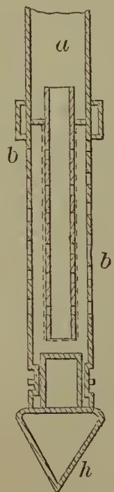
57974—T. Rose—Separating Sand from Water in Wells.
