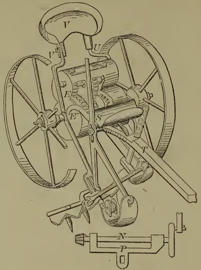
60427—N. Rowe—Harvester.
