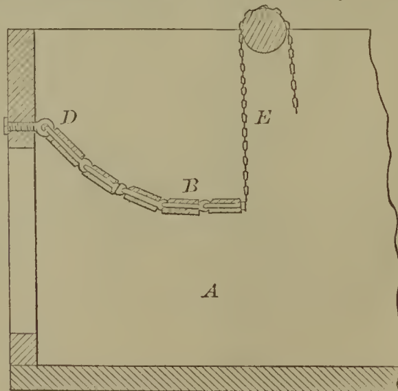
55882—Mecker & Cortright—Gate for Forebay.
