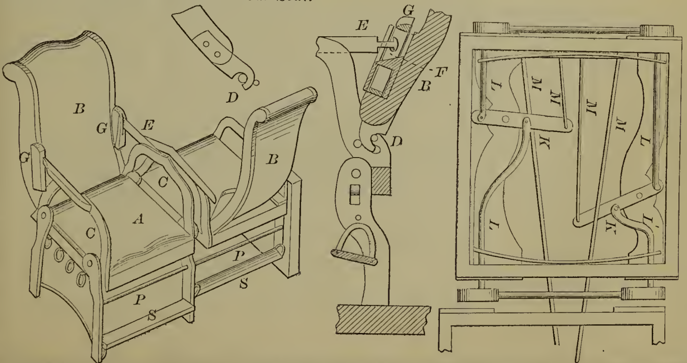
53842—Lockwood & Pitman—Car Seat.
