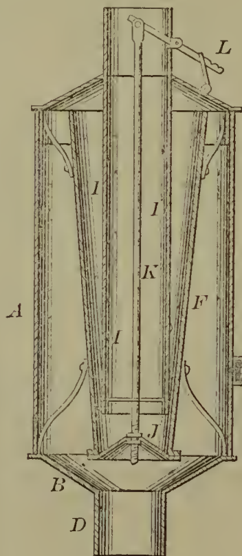
57572—Ruth & De Long—Store Pipe Drum.
