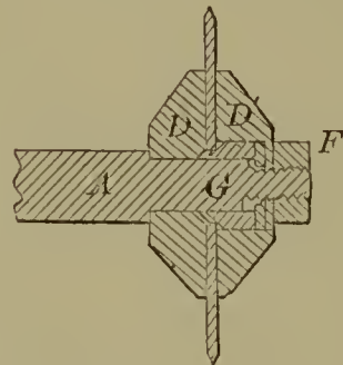
54774—A. L. Rice— Attaching Circular Saws to Arbors.
