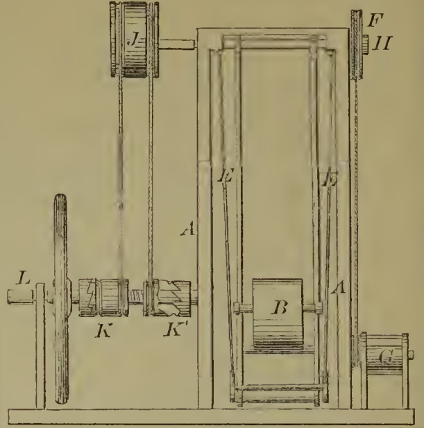
59878—Valentine & Longton—Swing Power.
