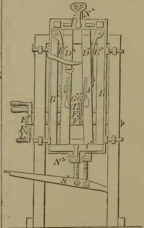
54748—W. C. Marshall—Extinguishing Fires.
