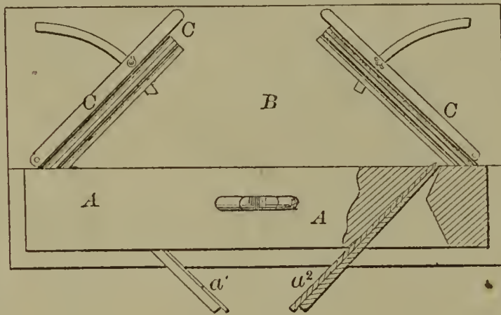
60265—J. Sawyer—Mitre Plane.
