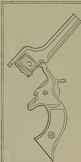
52165—H. Hammond—Cartridge Retractor.
