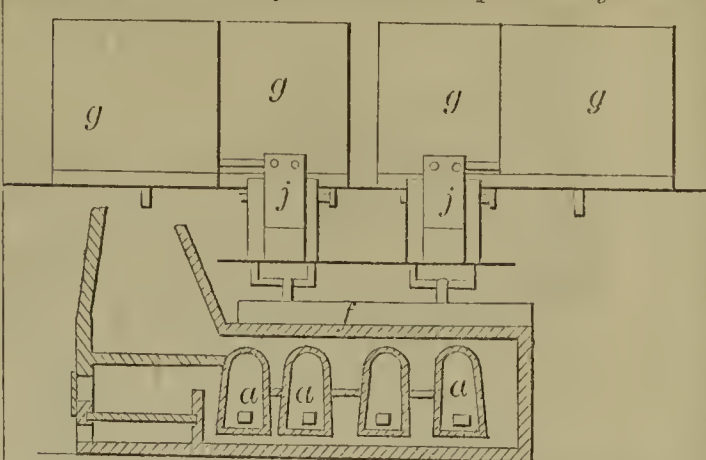
57194—V. B. Ryerson—Desulphurizing Ores.
