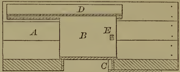
56113—W. G. Smith— Car Spittoon.
