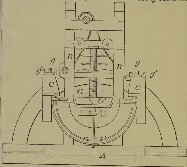
54316—J. Fishbaugh— Wood Bending Machine.
