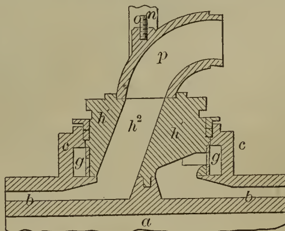
56657—W. E. Worthen—Rotary Valve.
