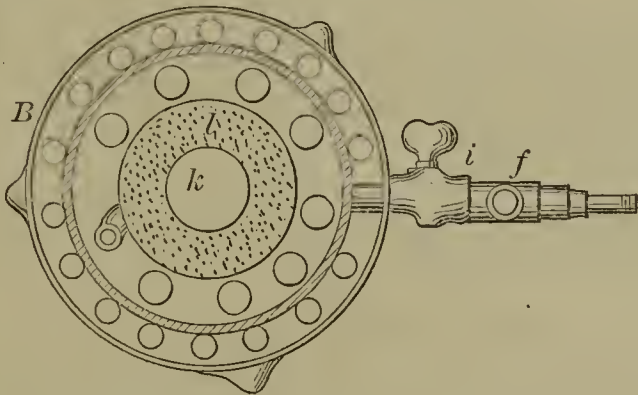
52300—Lesley & Craig— Gas Stove.
