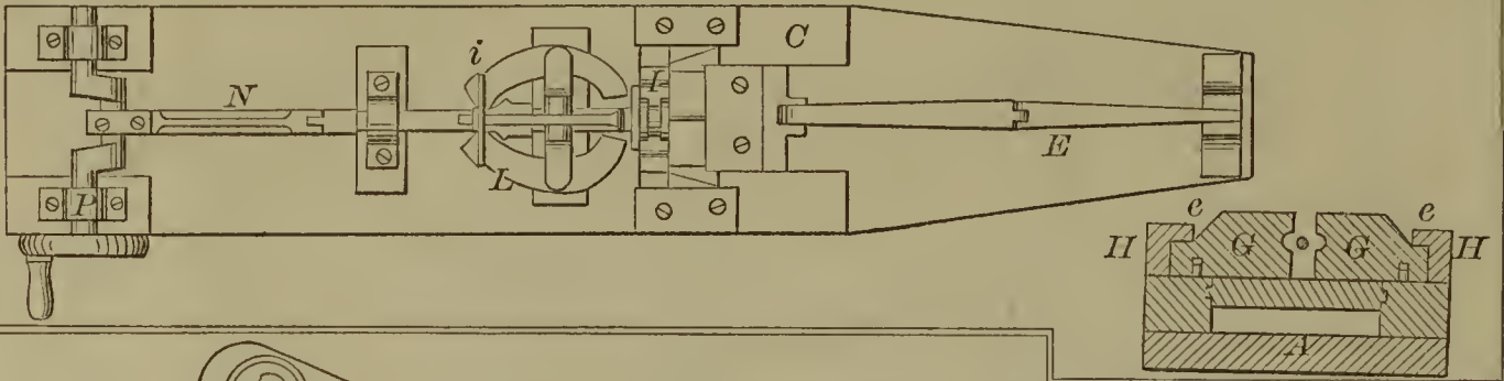
52728—W. P. Martin—For Rolling Leather.
