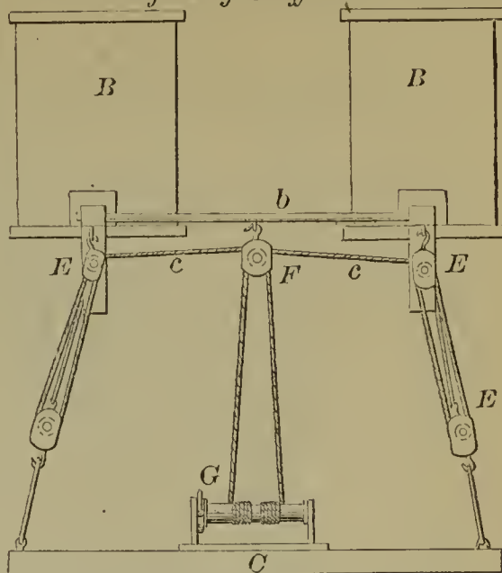
59824—W. A. Devon—For Holding and Adjusting Scaffolds.
