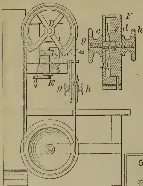
57565—P. Pryibril—Saw Mill.
