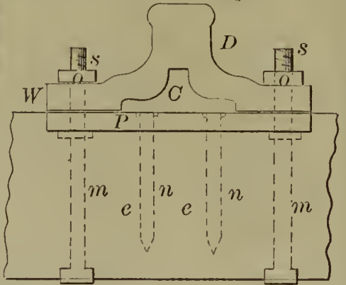
57501—F. Hanson—Turn Table.
