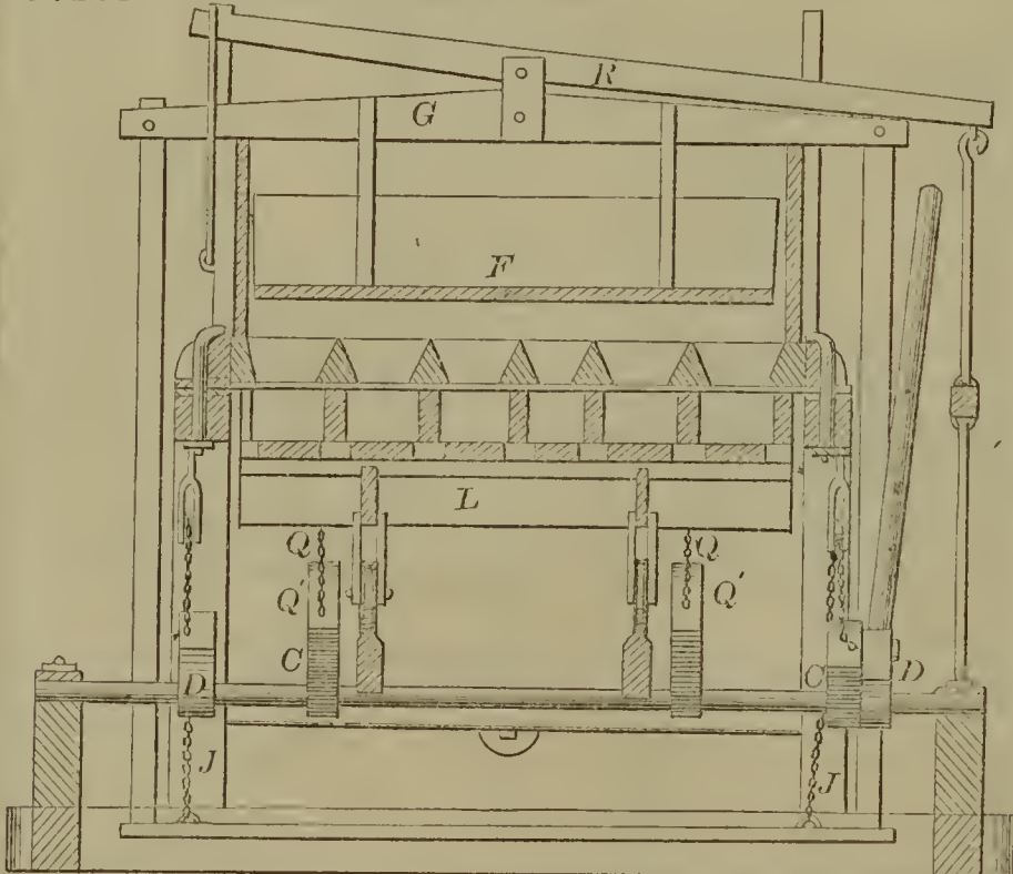
57128—E. Hallett—Brick Machine.
