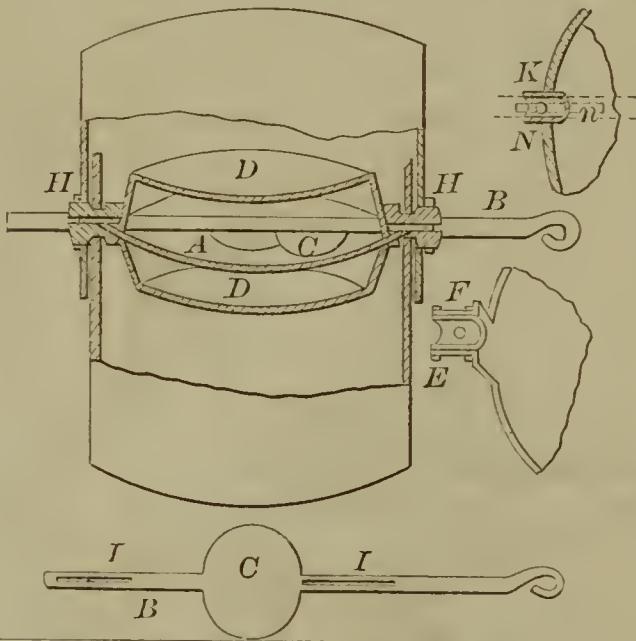
57369—M. W. Owens— Broom Head and Clamp.
