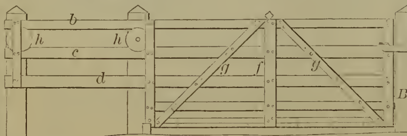
59060—M. Packard—Gate.
