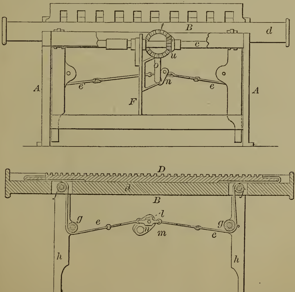
54742—L. J. Knowles—Loom for Weaving Tapes, &c.
