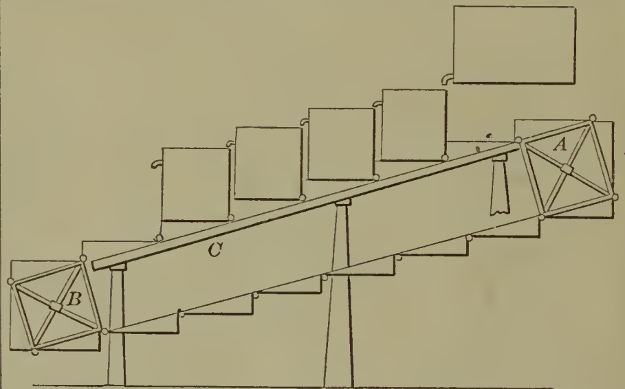
60445—P. H. V. Weyde—Percolator and Filtering Machine.
