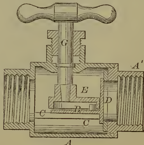
52895—Shedlock, Shedlock & Marshall Stop Valve.
