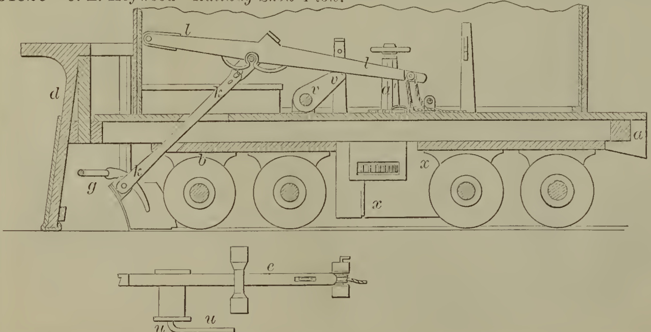
51829—C. L. Heywood—Railway Snow Plow.
