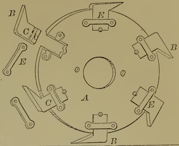
54827—J. Woodrough—Saw.
