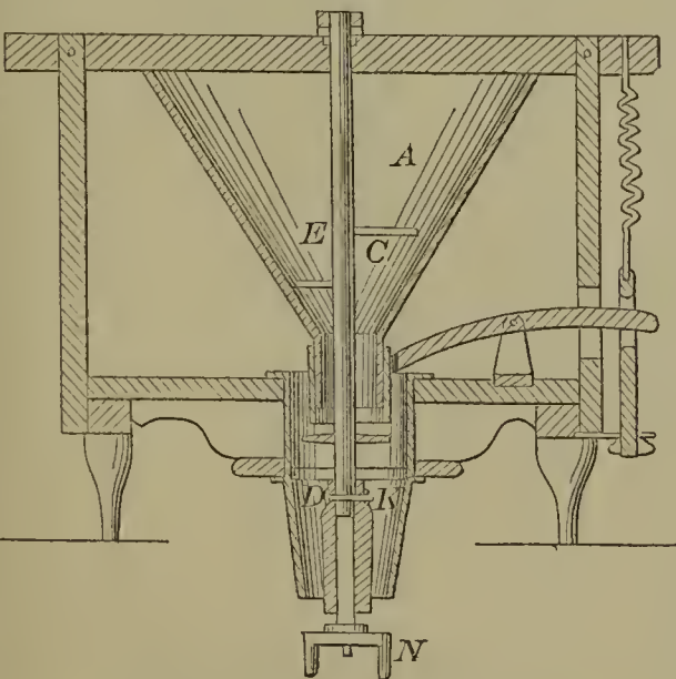
55872—J. Hutchison—Grinding Mill.
