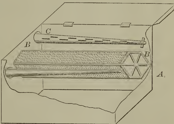
51939—S. Godfrey—Bolt for Flouring Mills.
