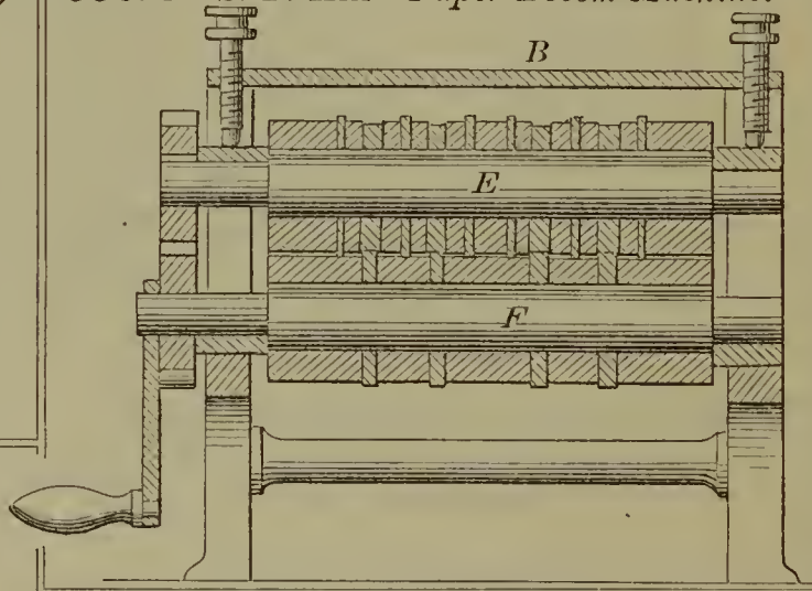
53615—S. B. Hill—Paper Bosom Machine.
