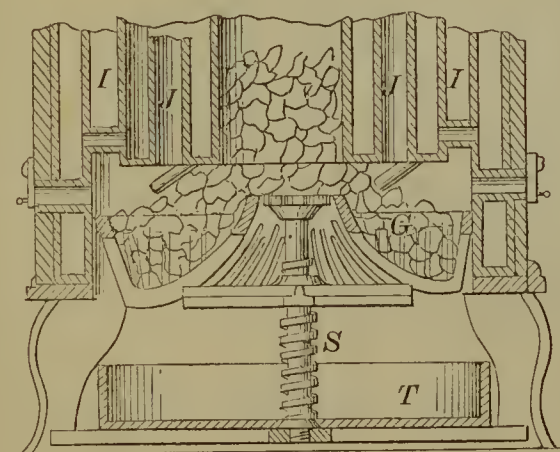
54064—R. W. & D. Davis— Grate for Furnaces, &c.
