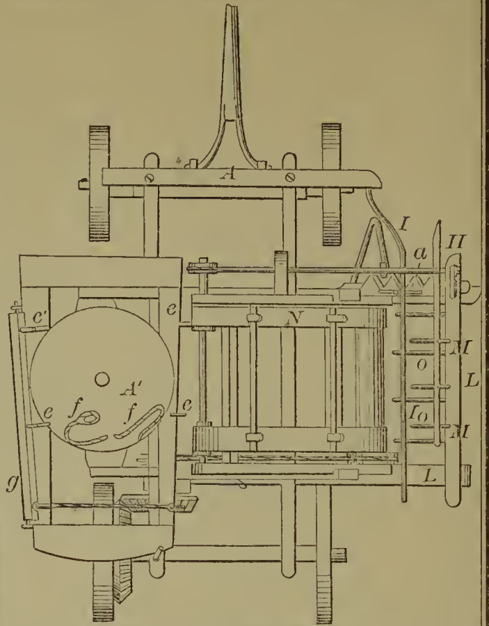
58349—Manlove & Green—Corn Harvester.
