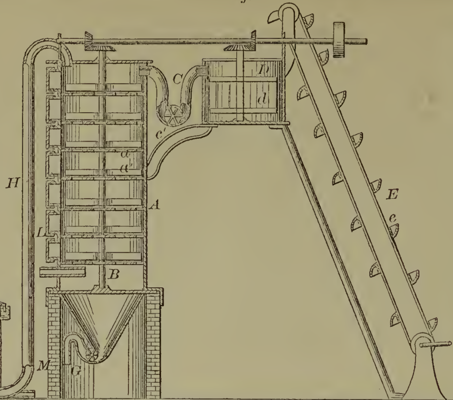
58005—P. H. V. Weyde— Distilling Petroleum and other Liquids.
