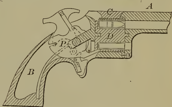
53959—W. B. Dodds— Lock.
