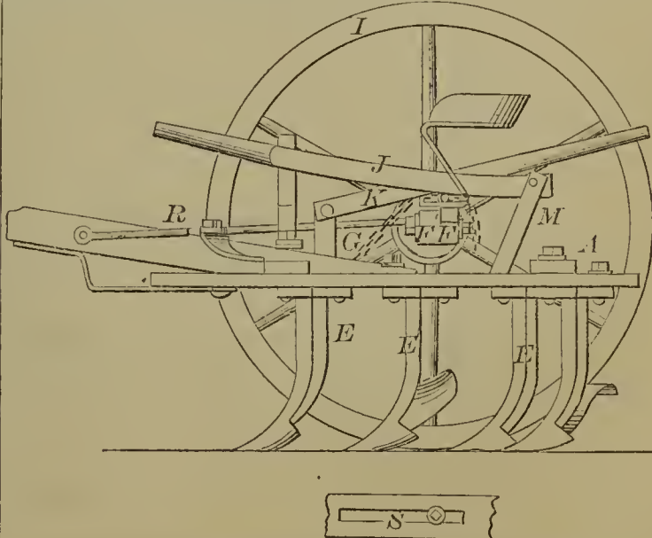
58188—A. Anderson— Cultivator.
