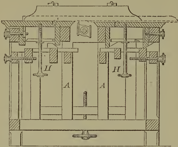
59964—P. Ceredo—Ash Sifter.
