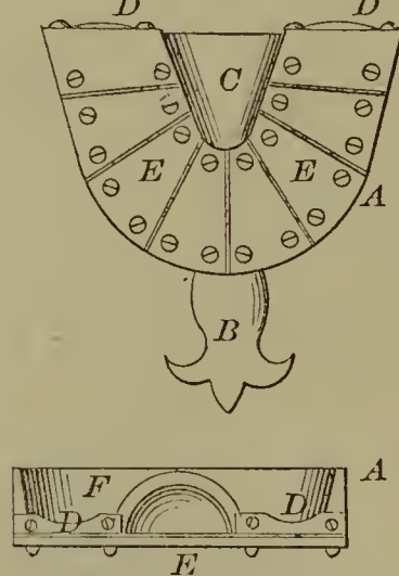
53346—J. Romans— Sheep Rack.
