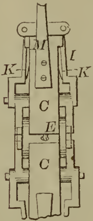
57535—J. McCalvey—Hoisting Machine.
