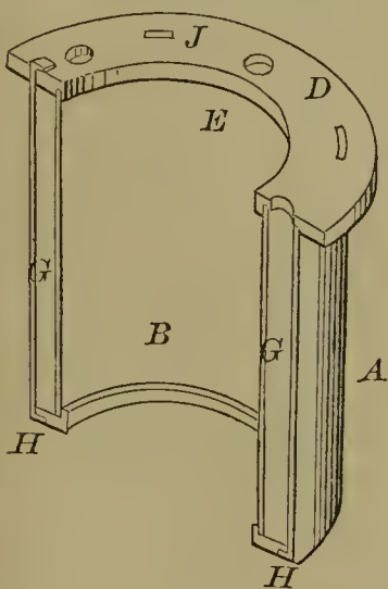
55268—C. H. Fitch—Stove Pipe Thimble.
