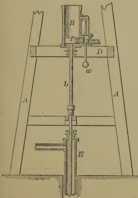
58299—J. B. Root— Boring and Pumping Apparatus for Oil Wells.
