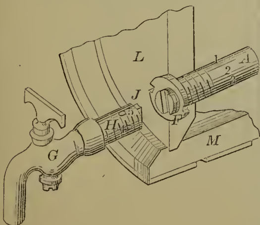
56889—W. Boynton—Tapping Barrels.
