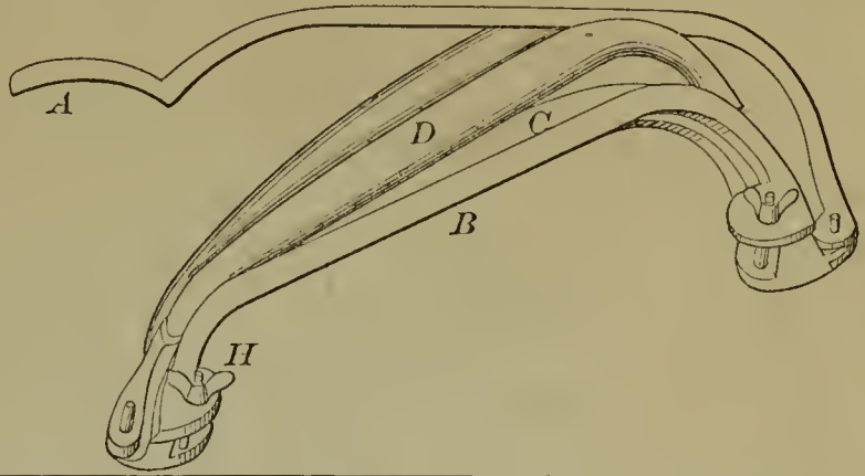
52831—E. C. Dow—Boring Tool for Oil Wells.
