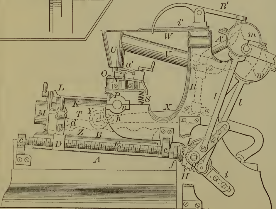
52926—E. Bueklin Jr—For Cutting Files.
