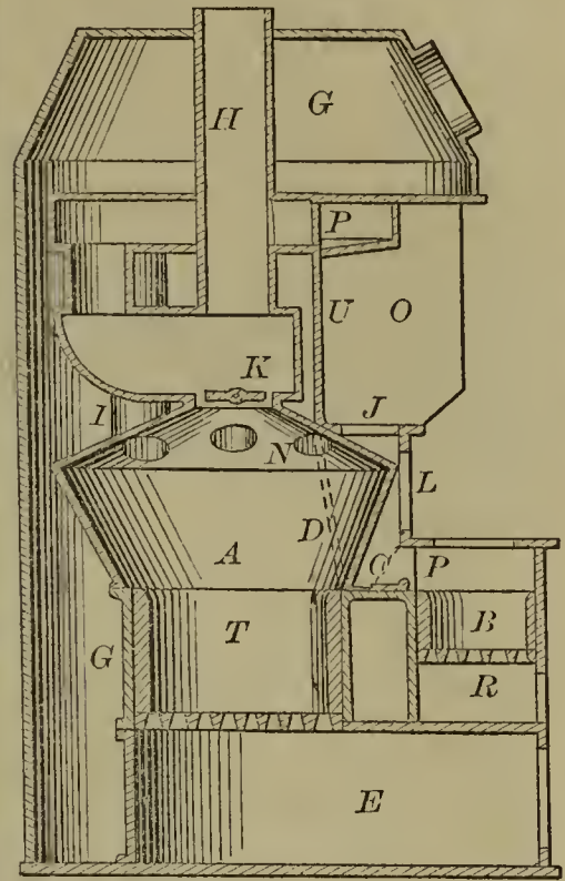
56041—W. A. Greene—Combined Range and Furnace.
