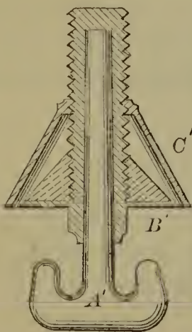
53426—A. B. Ely—Telegraph Insulator.
