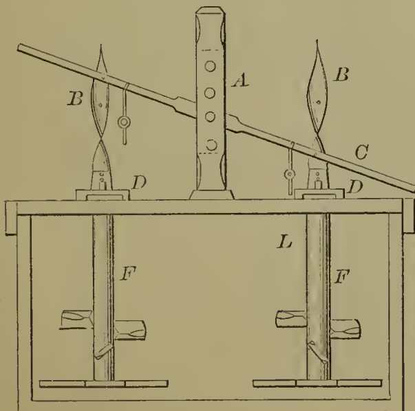
57794—H. C. Stoll—Churn.
