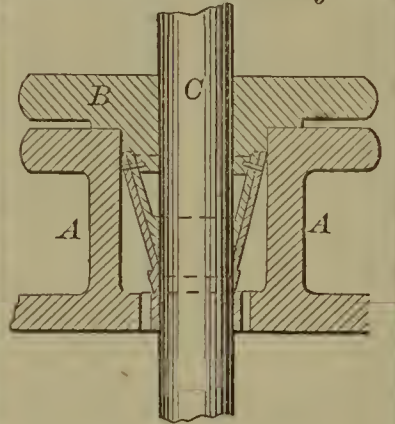
52742—G. S. Prindle—Piston Rod Packing.
