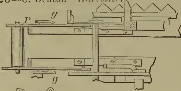
58720—C. Denton—Harvester.
