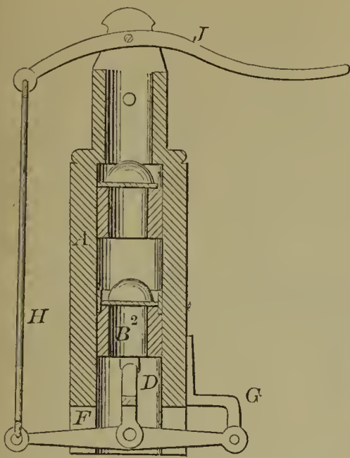
59869—W. P. Squire—Pump.
