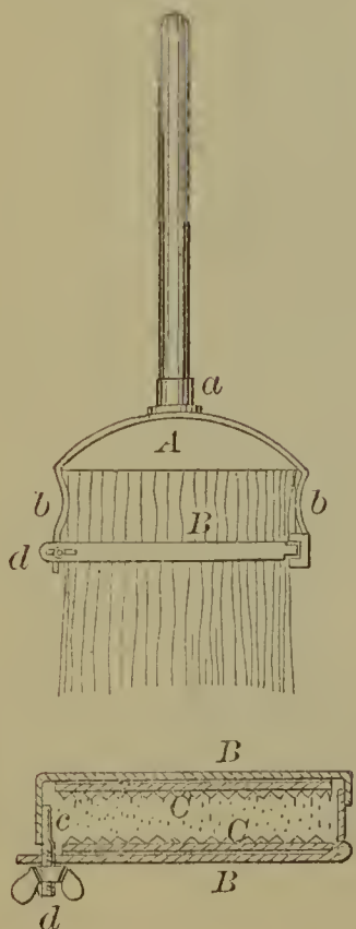
54338—J. Harris— Broom Head.
