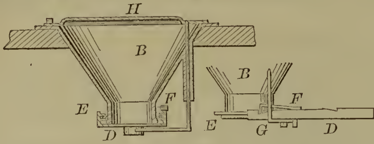
55729—W. G. Smith— Spittoon for Cars.
