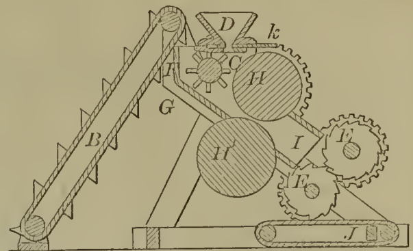
52470—S. D. Tripp—Heel Polishing Machine.
