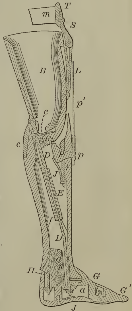
51953—J. Madden—Artificial Leg.
