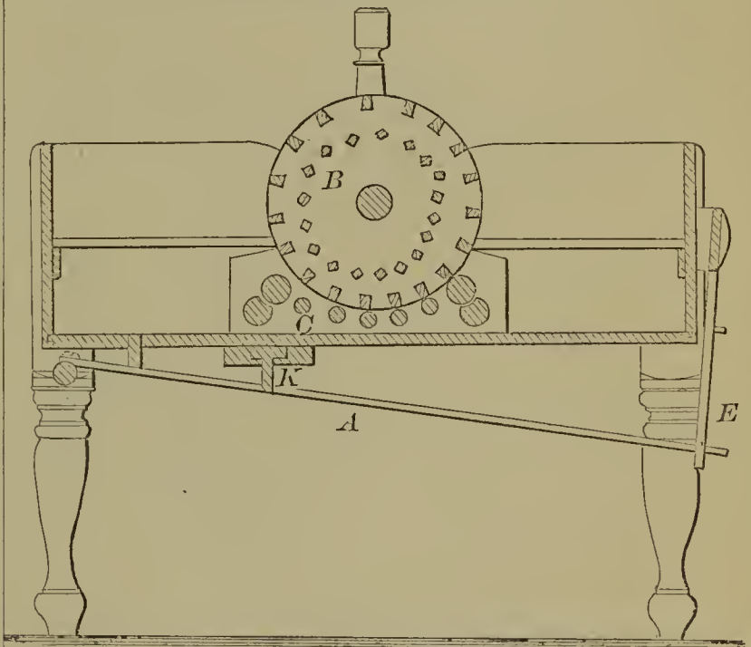
57679—T. Cole— Washing Machine.
