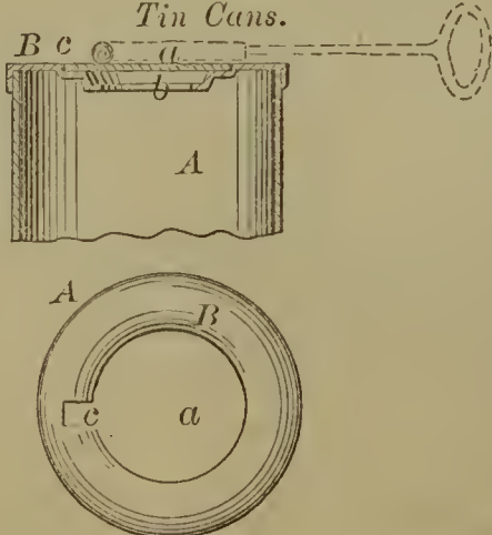
58554—J. Osterhondt—Opening Tin Cans.
