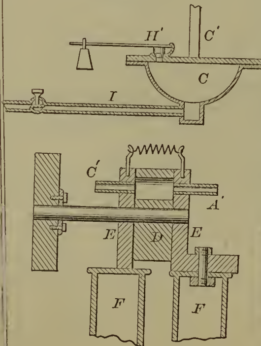
53097 —J. B. Atwater— Air Engine.
