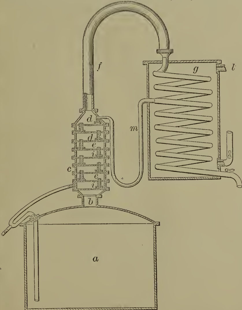
60166—A. Foubert—Distilling and Refining Oils, &c.
