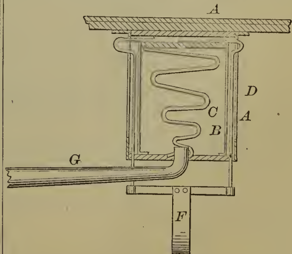
54922—P. Killin— Alarm Whistle.
