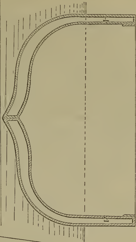
58743—W. L. & T. Winans— Application of Rudders to Spindle Shaped Hulls.
