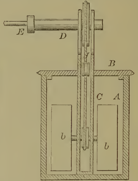
59428—W. D. Matthews— Churn.
