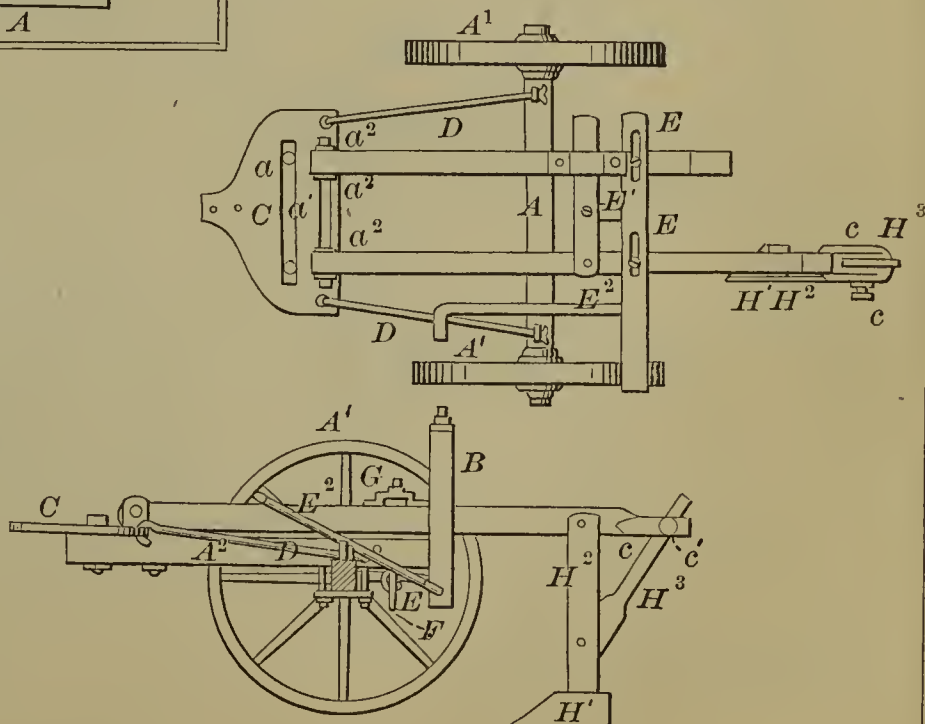
54089—C. Atwood— Gang Plow.
