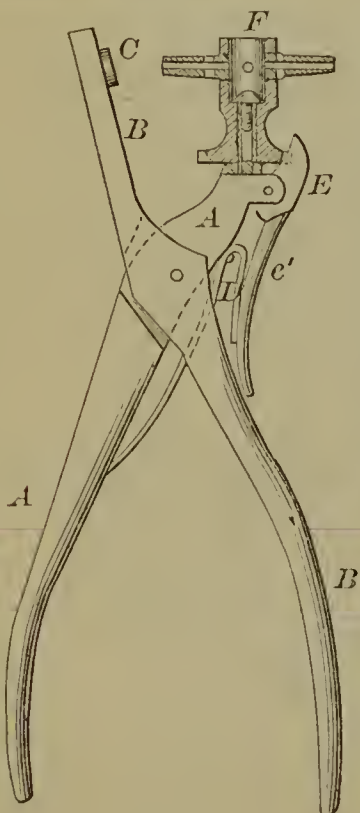
53537—J. Lyle—Spring Punch.
