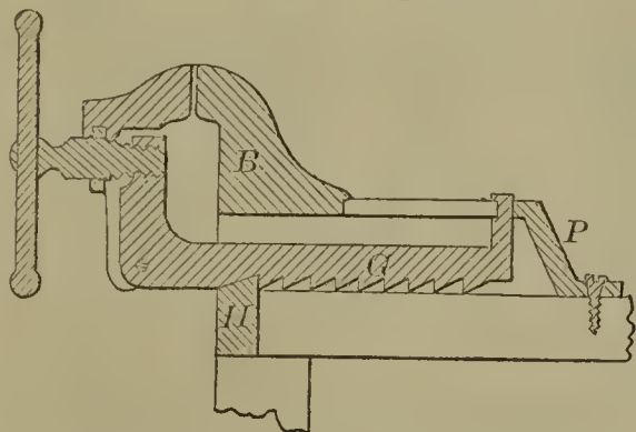
57250—O. V. Flora— Carpenter's Vise.
