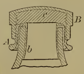
58281—M. V. Olry—Bottle Cap.
