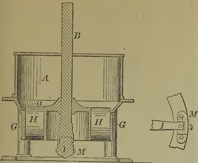
56852—M. P. Euring—For Distilling Petroleum.
