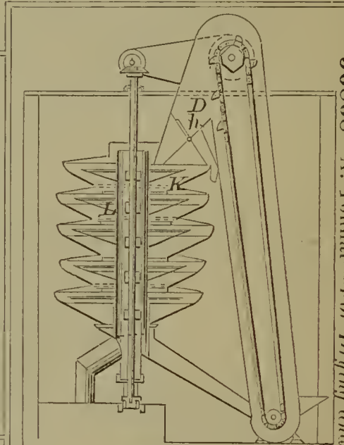
56868—A. Tommar—For Drying and Cleaning Grain.
