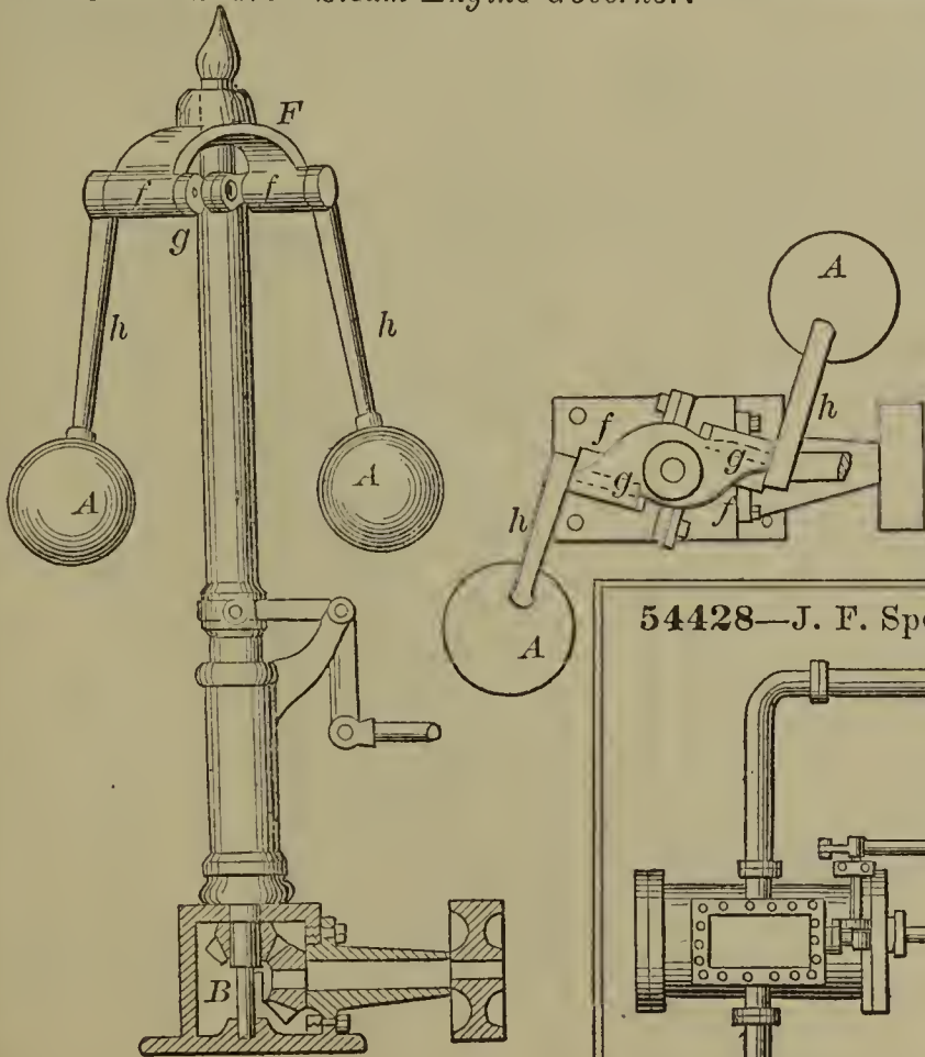
54423—D. Shive— Steam Engine Governor.
