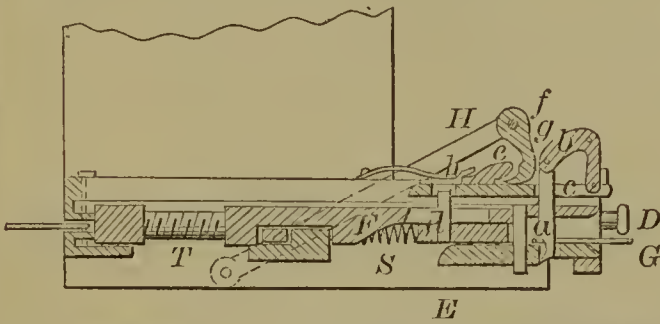
58418—C. Holtz—Car Coupling.
