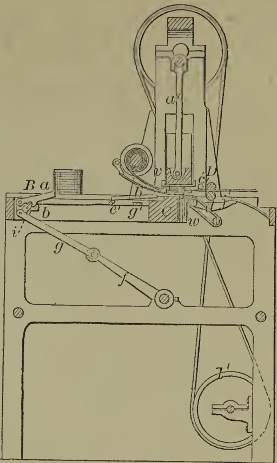
59957—J. T. Bruen—For Cutting and Reenforcing Button Holes.
