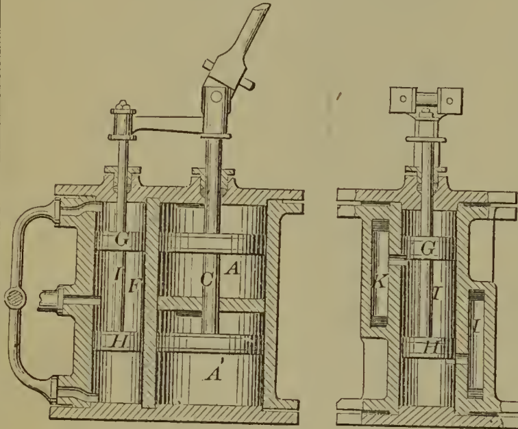
57799—G. I. Washburn— Steam Engine.
