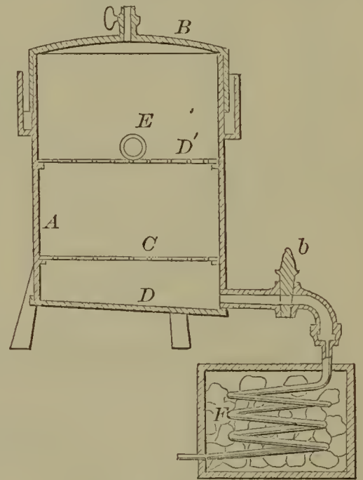
55915—J. Schneider—For Producing Extract of Hops.
