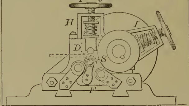
58156—Vose & Toshach—Coiling Springs.
