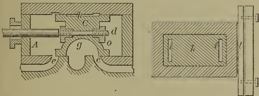
54334—C. Gullmann—Well Curb.
