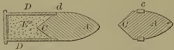
55796—S. H. Haycock—Projectile.
