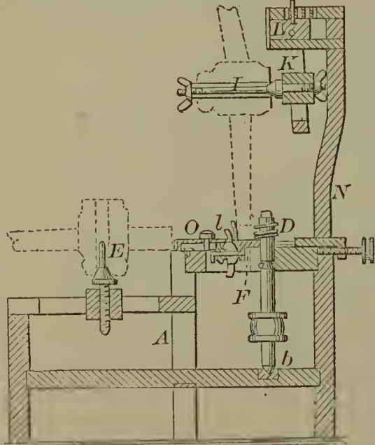
60040—A. P. Odholm—Machine for Dressing Felles.
