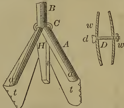
56462—W. Peabody—Harness.
