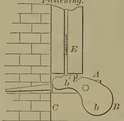
57239—J. D. Winslow—Shutter Fastening.
