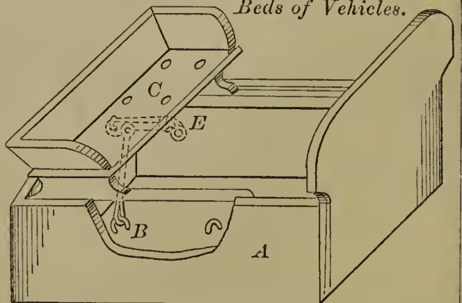
53371—W. Bench— Attaching Seats to the Beds of Vehicles.
