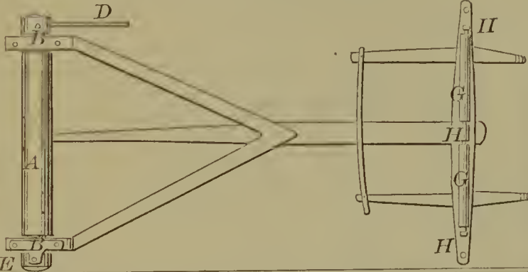
57652—Fowler, Worby & Greig— Steam Plow.
