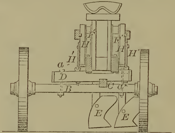
52651—J. E. Travis— Gang Plow.
