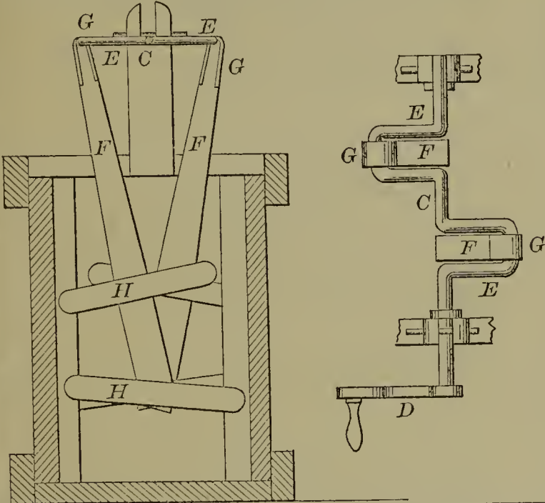
53382—H. C. Sisco—Lathe for Turning Wagon Hubs.
