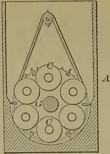
54045—O. G. Warren—Quartz Comminutor.
