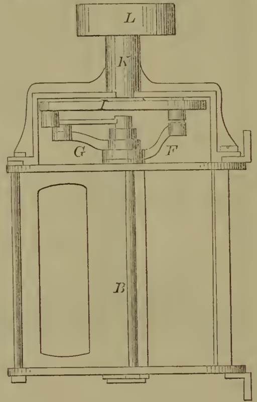
56165—Bigelow & Murray—Blower.
