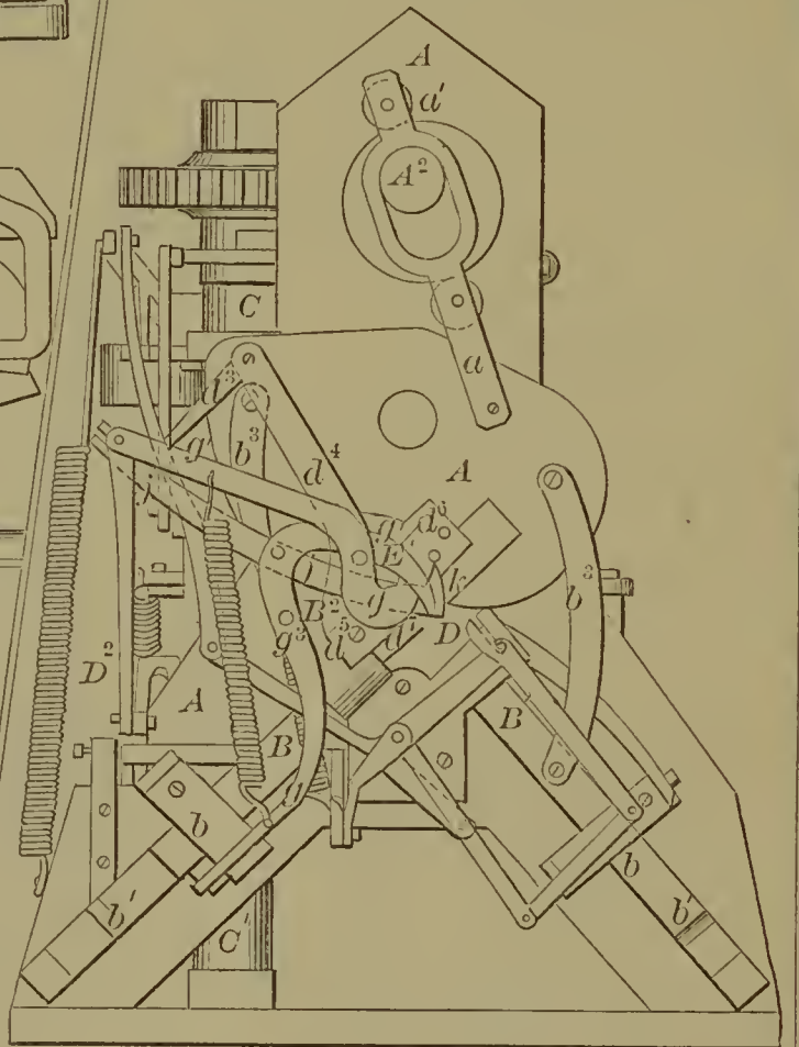
58520—A. Whittemore—For Making Horse Shoe Nails.
