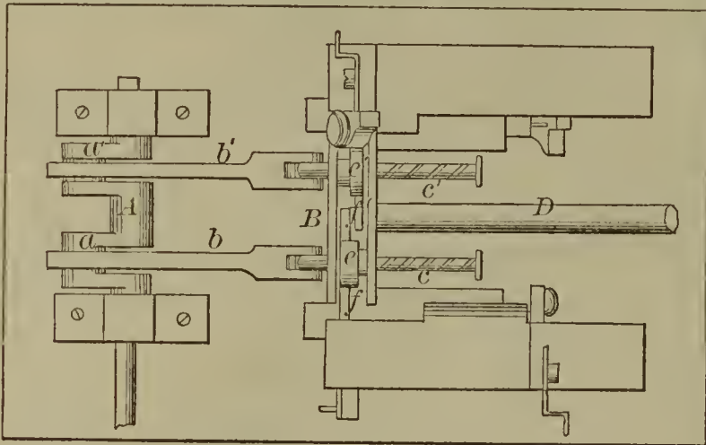
52354—F. Yeiser—Transmitting Motion.
