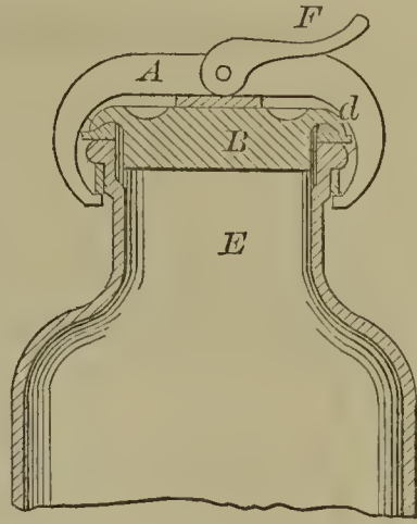
52525—F. A. Bunnell—Fruit Jar Cover.
