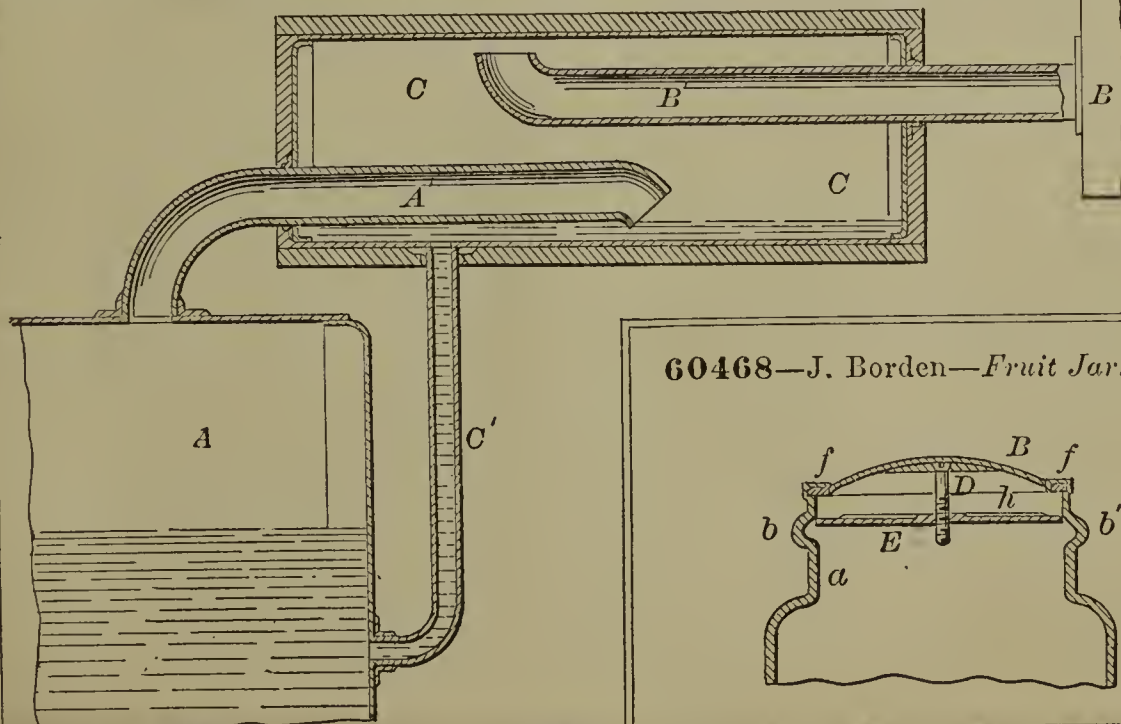
60470—R. C. Bristol— Water and Steam Separator for Steam Generators.
