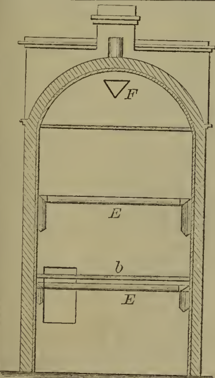
57117—Gallup & Wood—Drying House.
