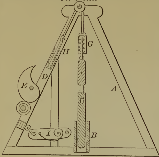
52816—Bateman & Cumming—Drill for Oil Wells.
