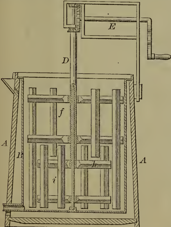
53912—E. P. Whitecomb—Churn.
