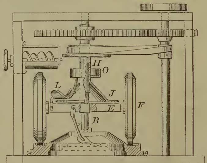
56581—J. Mabbs—Quartz Crusher.
