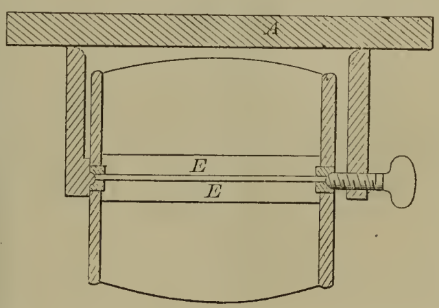
57496—G. P. Goodwin— Twine Spool Stand.
