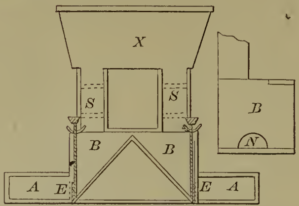
56560—R. S. Holton—Water Wheel.
