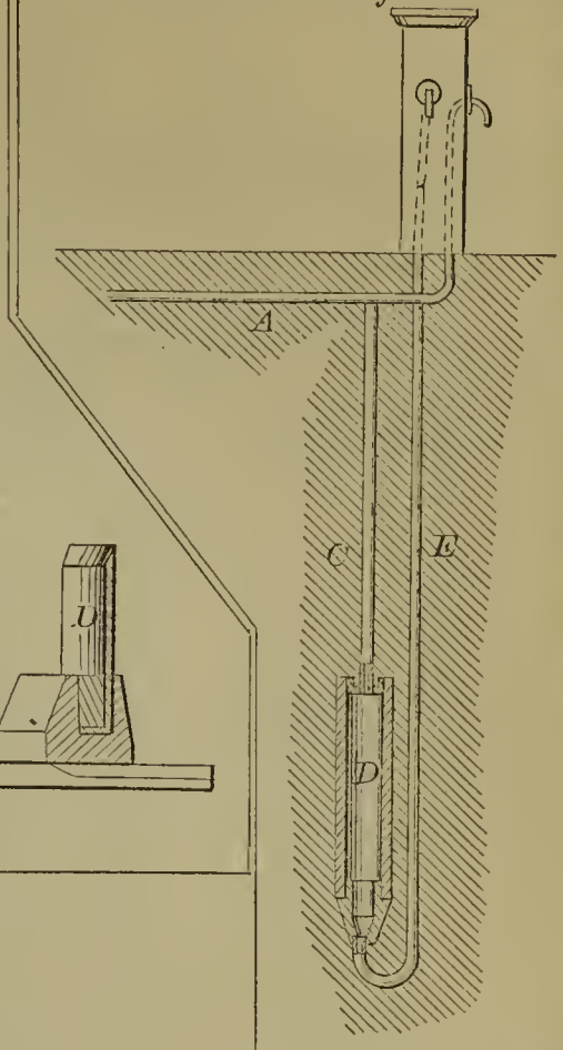
55040—J. S. Baldwin—Charging Water with Carbonic Acid.
