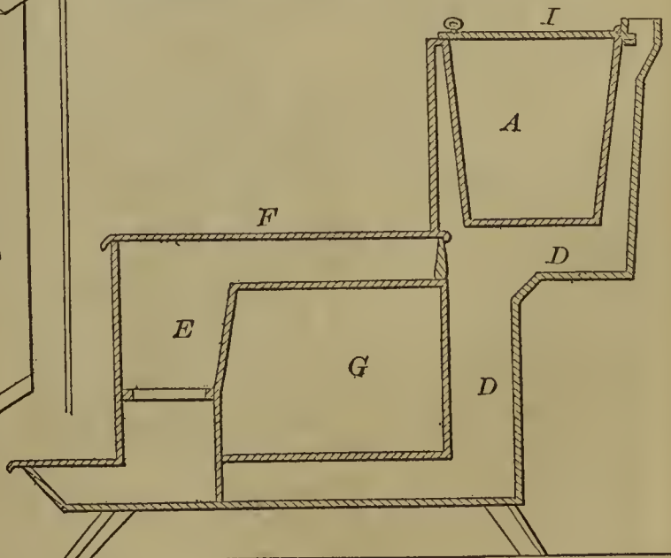
56488—E. Bussey—Cooking Stove.
