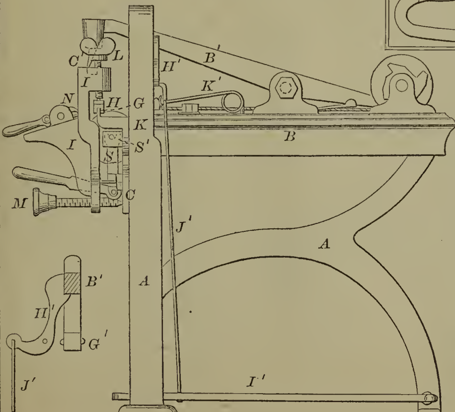
60180—S. C. Hall—For Cutting Sickle Sections.
