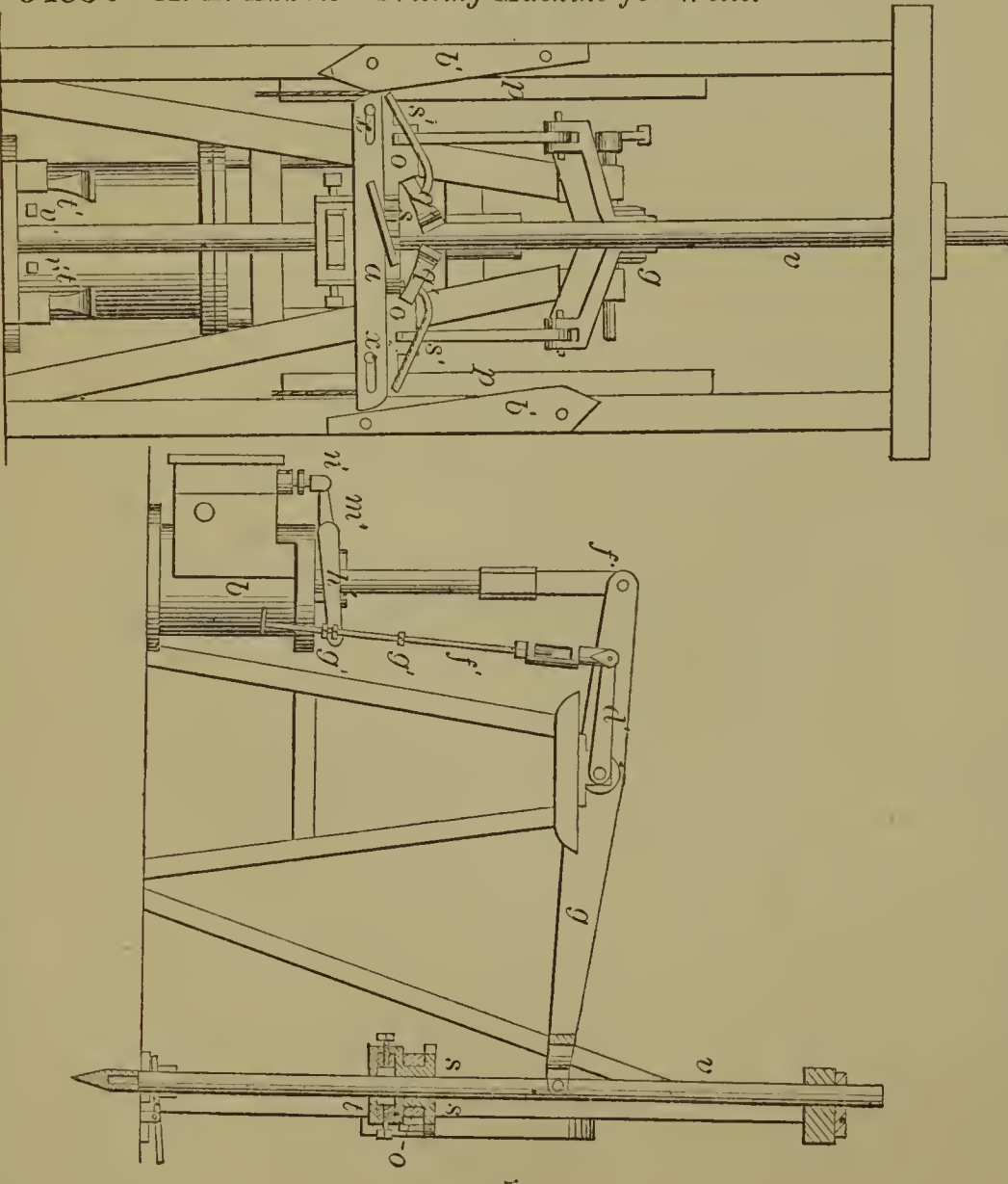
54836—M. E. Abbott—Drilling Machine for Wells.
