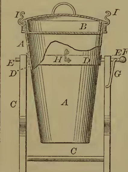
60652—S. J. Talbott—Dough Mixer.
