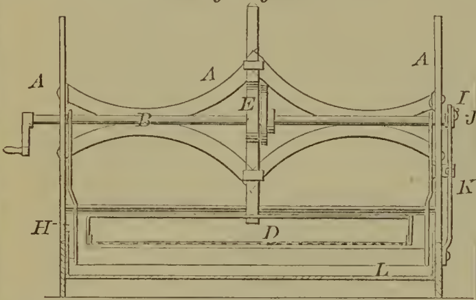
59308—J. H. Aiken—For Oiling Wool for Carding Engines.
