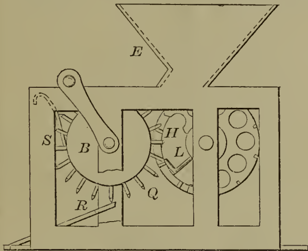
53855—S. C. Moore—For Seeding Raisins.
