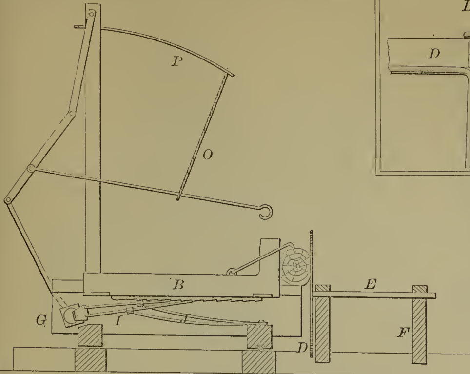
56929—J. A. Griggs—Head Block for Saw Mills.
