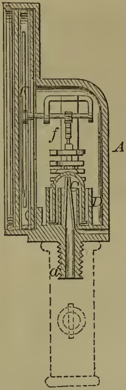
56070—J. Lowe— Steam Gauge.
