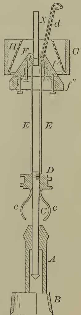
51806—L. J. Crans— Well Boring Machine.
