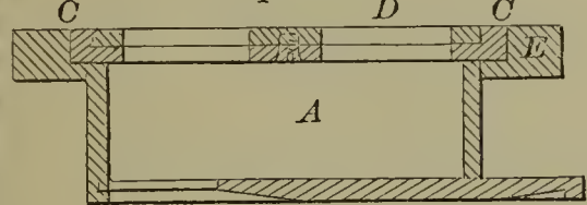
55458—A. Brigham—Dust Receptacle.
