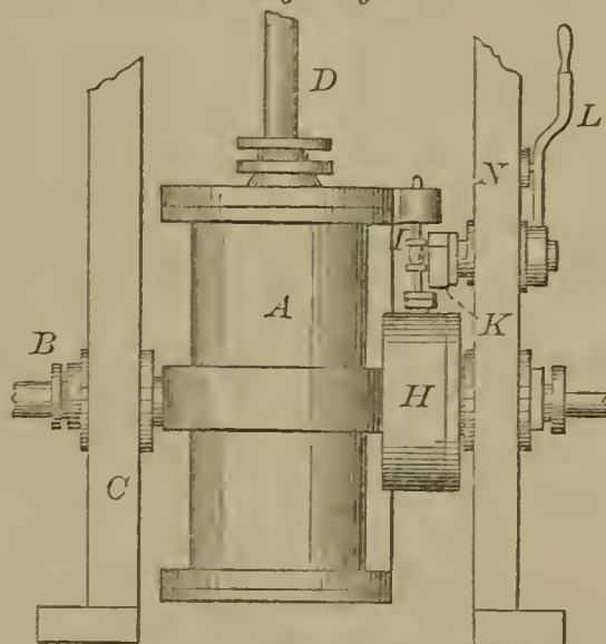
52677—H. T. Carter— Valve Gear for Oscillating Engines.
