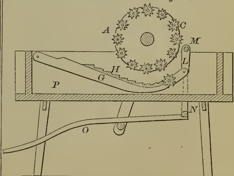
53626—W. Kenderline— Washing Machine.
