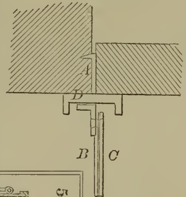
52469—G. E. Thompson—Door Fastener.
