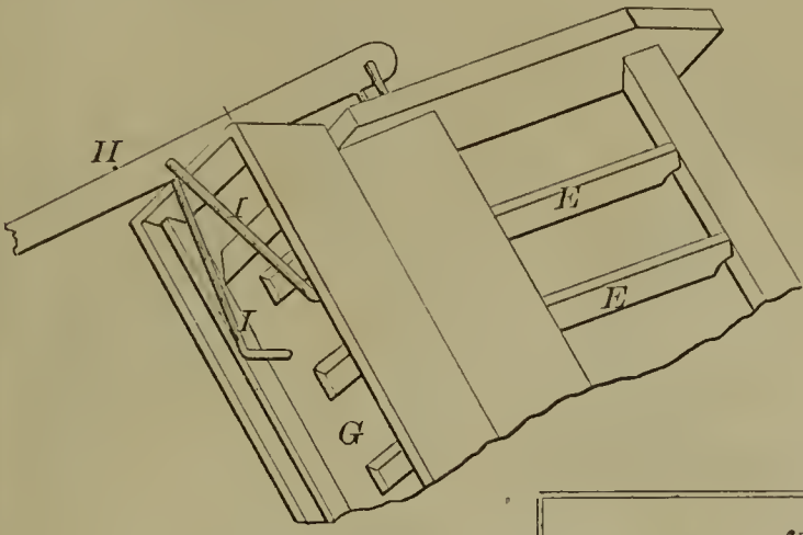
M. C. C. Church—Petroleum Tank. 57479—
