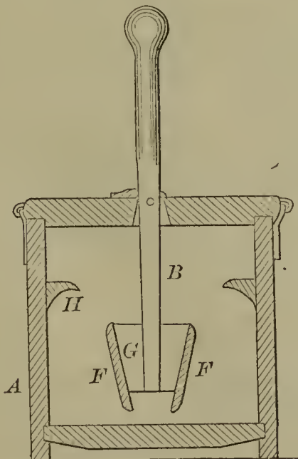
52313—M. Neal—Churn.
