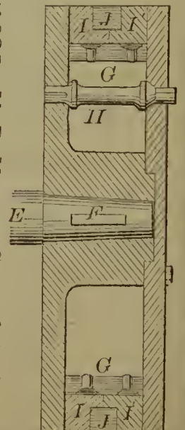
57823—M. B. Mason— Steam Cylinder Piston.
