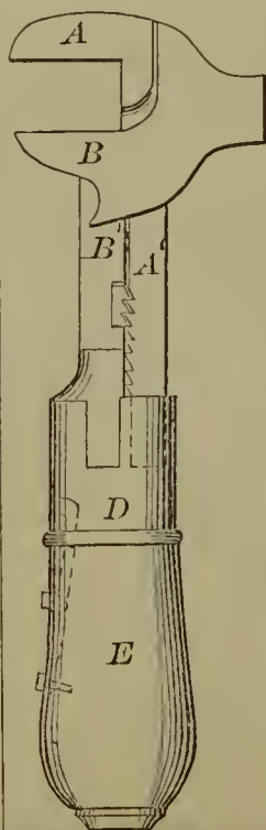
55066—J. L. Crist—Screw Wrench.
