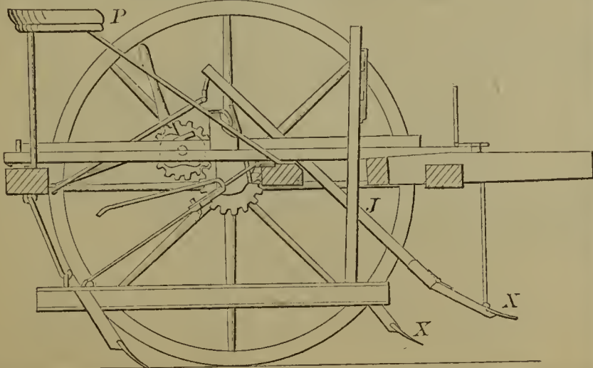
57752—L. B. Moore—Corn Cultivator.
