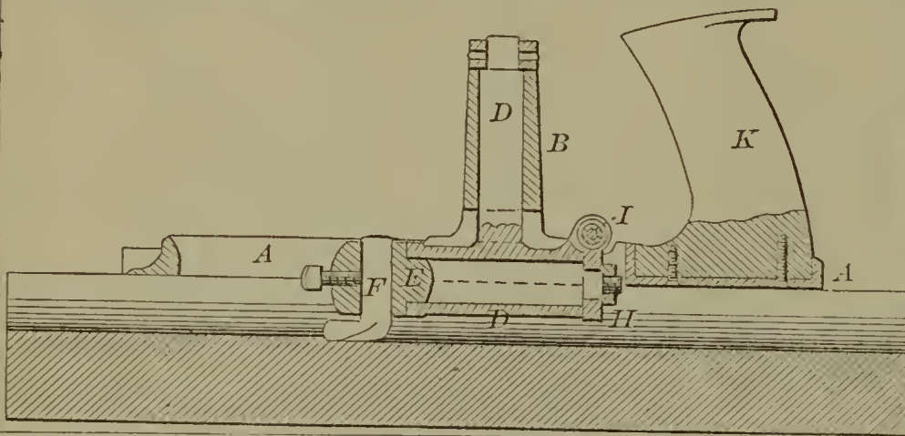
60209—J. J. Look—Wagon Brake.
