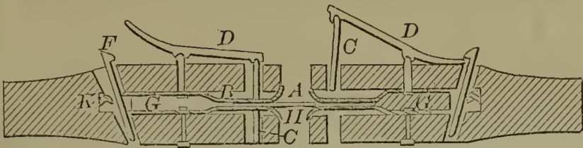
58887—J. O. Reilley— Spike Making Machine.
