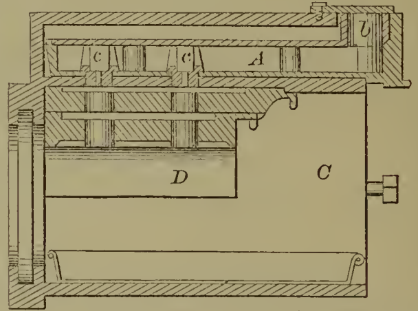
54771—T. H. Quick— Purifying Bone Black.
