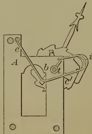
53146—H. J. Holden— Time Piece.
