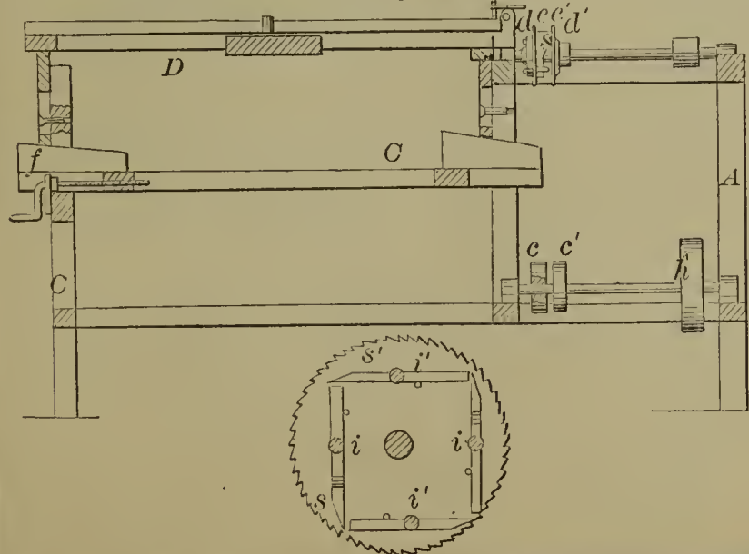
59826—D. Evers—Tenoning Machine.
