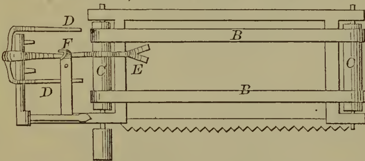
53409—Canfield, Still & Wheeler—Harvester.
