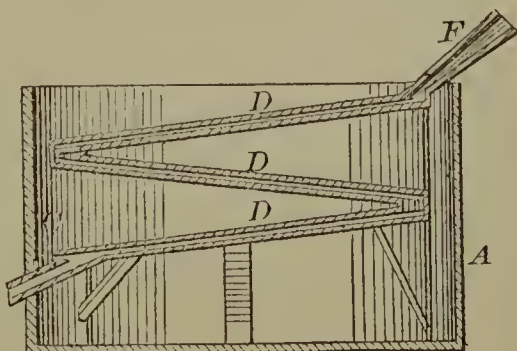
58009—J. C. Wharton— Condenser.
