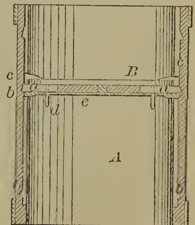
59186—L. Coates— Variable Measure.
