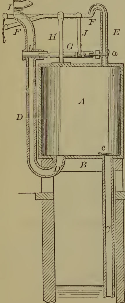
53469—Myers & Noble— Steam Water Elevator.
