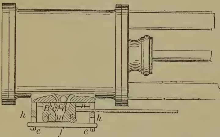
56388—Z. S. Durfee—Flask for Casting.
