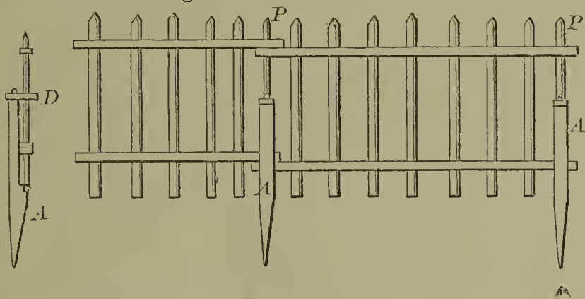
60127—B. Billings—Fence.
