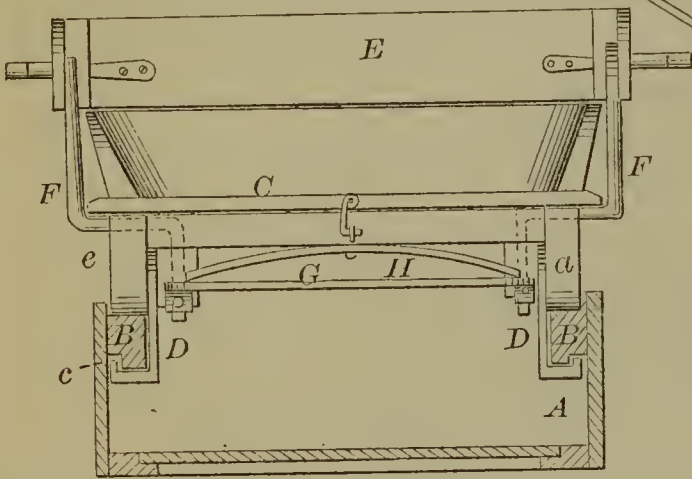
53330—J. Pelsor—Hand Loom.
