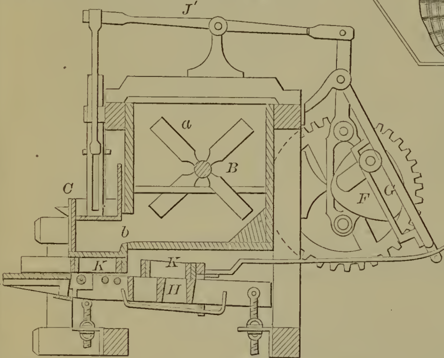
54610—Seeley & Jacobie— Brick Machine.
