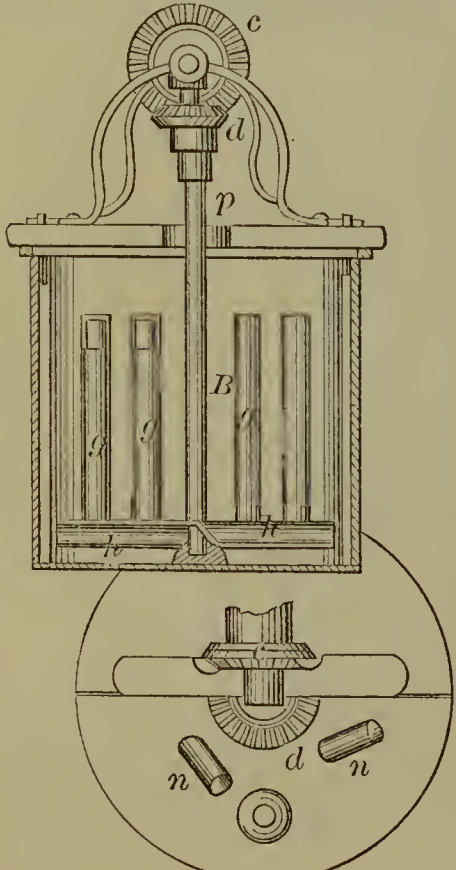
53876—F. J. Robinson—Churn.
