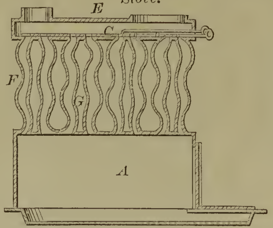
58782—E. N. Cummings—Heating Stove.
