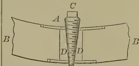
54485—H. Austin— Coupling for Carriage Felloes.
