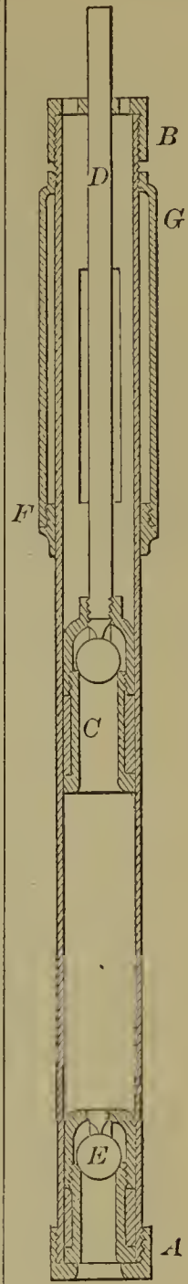
53118—I. E. Craig— Steam Generator for Heating Purposes.
