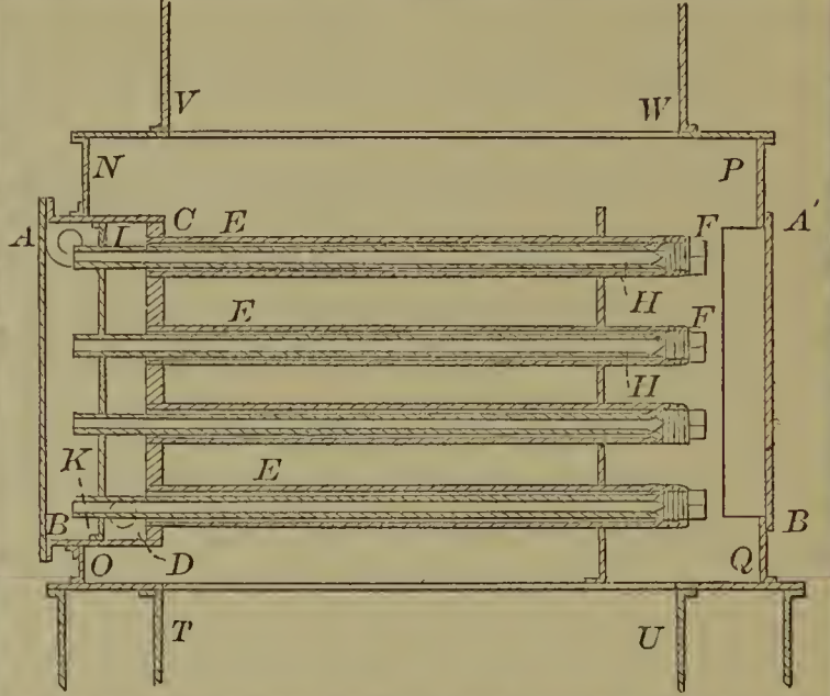
54759—E. Oldham—Pantographic Machine.
