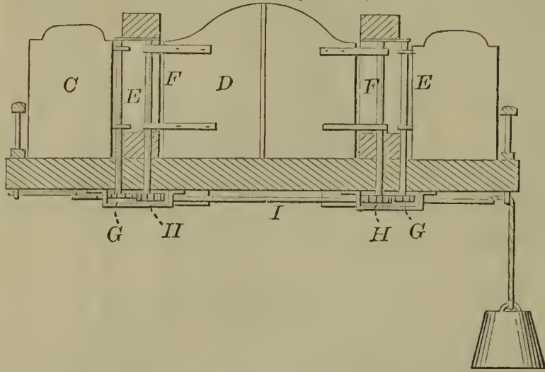
55628—L. P. Decker— Ferry Bridge Gate.
