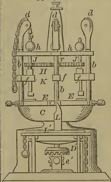
56095—D. Reese—For Tapping Nuts.
