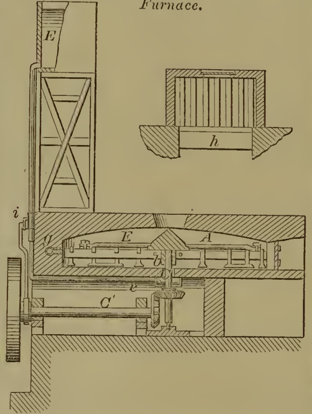
60654—J. M. Whiteside—Reverberatory Furnace.
