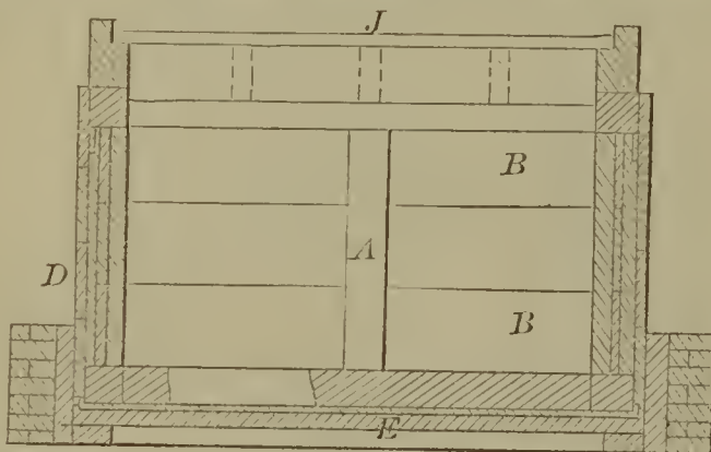
55812—D. Bruce—Constructing Vacuum Vessels.
