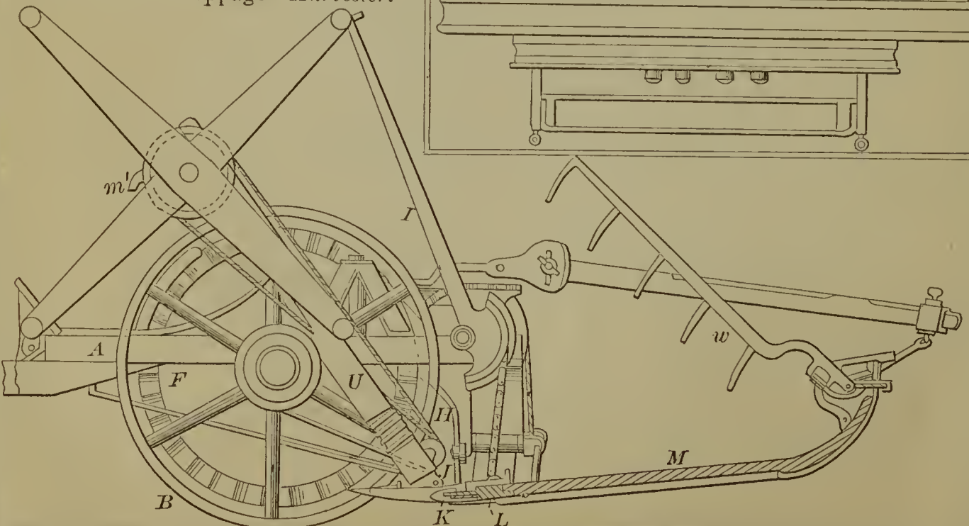
56320—F. C. Coppage—Harvester.
