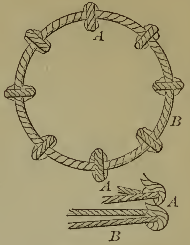
53161—McAuley & Cheney— Covering for Hose.
