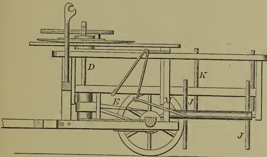
53710—Wallis & Miller— Corn Harvester.
