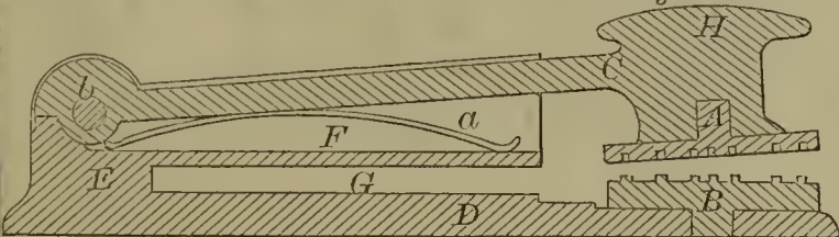
56244—Merriam & Weeden—Embossing Press.
