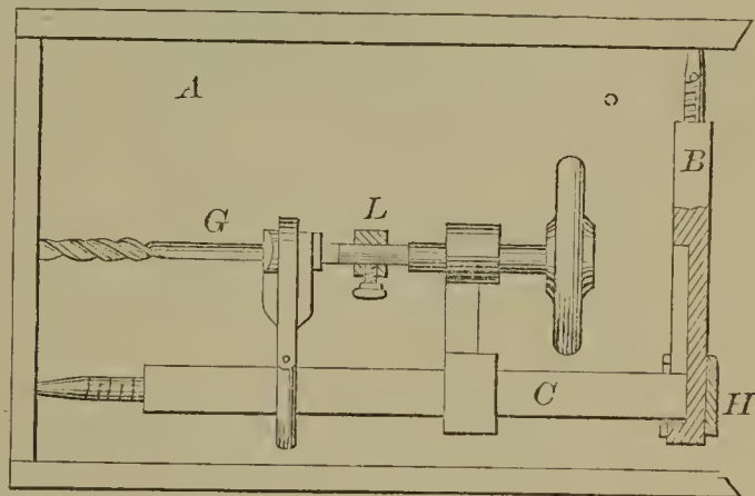
57011—R. A. Thomas— Drilling Machine.
