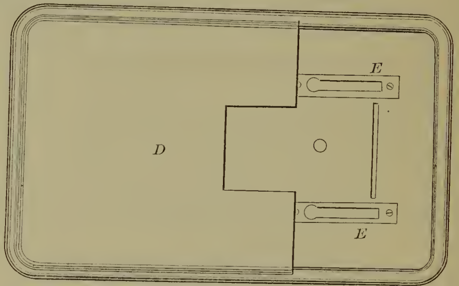
55023—A. J. Thompson— Cover for Sewing Machines.
