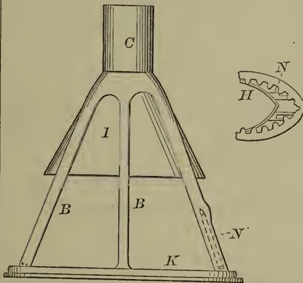
55519—C. Messenger— Broom Head.
