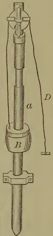
52799—W. W. Winter— For Driving Wood into the Ground.
