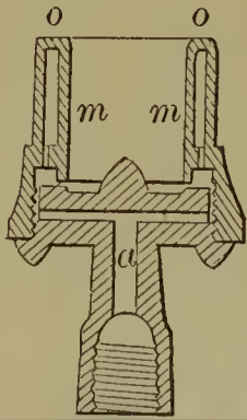
54193—Murray & Oakes—Argand Gas Burner.
