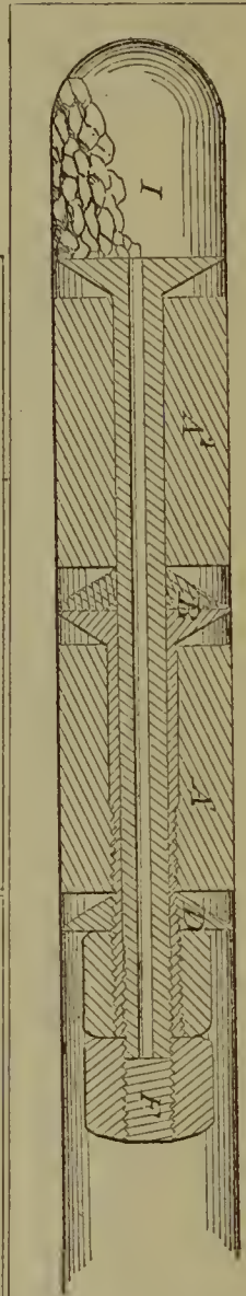
52836—G. H. Felt—Plug for Blasting.
