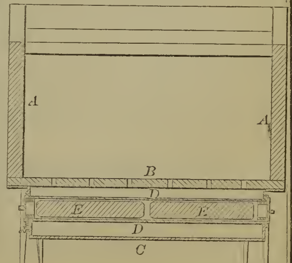
59068—W. H. Pratt— Washing Machine Heater.
