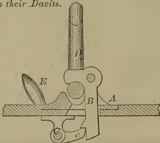
55303—T. Huntington— For Detaching Boats from their Davits.
