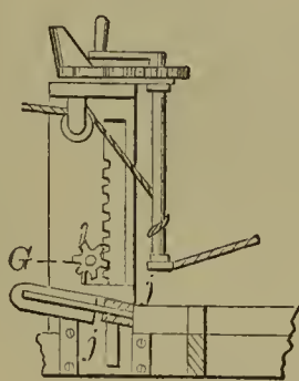
59860—H. L. Ogden—Car Coupling.
