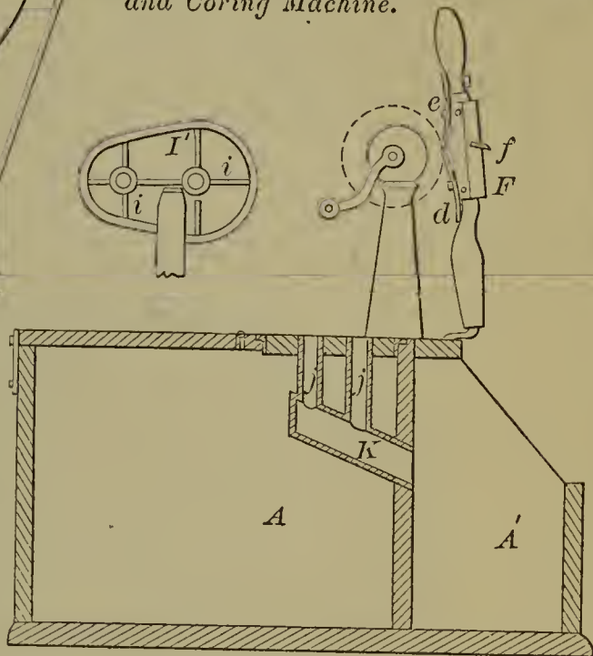
53754—W. Weaver—Paring, Cutting and Coring Machine.
