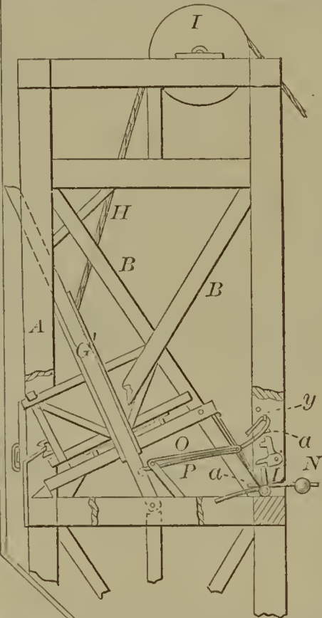
58740—W. Goodman— Ship's Windlass.
