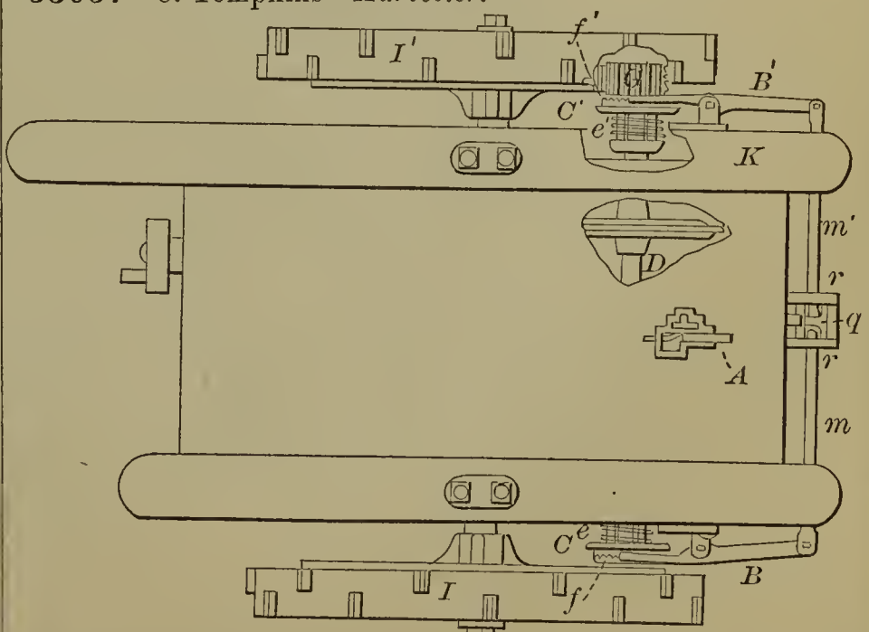
53057—C. Tompkins—Harvester.
