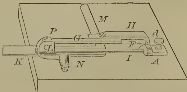
52646—G. C. Overhiser—Sewing Machine Hemmer.
