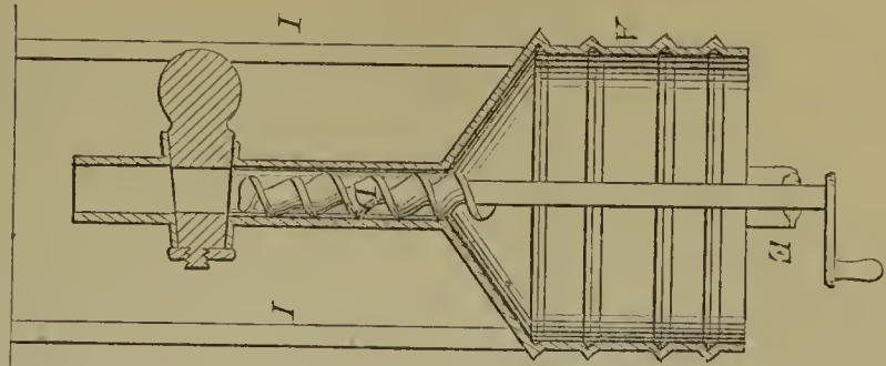
56713—E. T. Colburn—Paddle Wheel.
