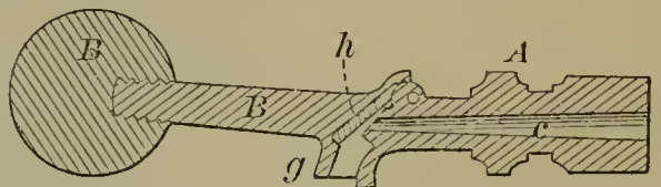
53337—J. Register—Try Cock for Steam Generators.
