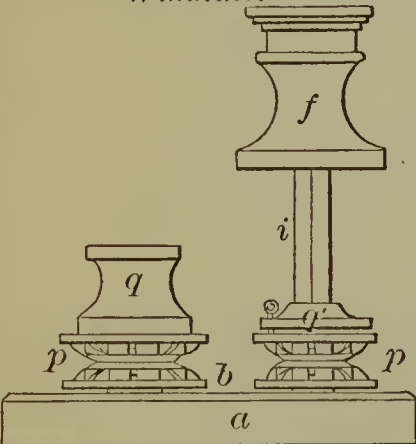
53182—Price & Wilson—Sand Box for Locomotive Engines.
