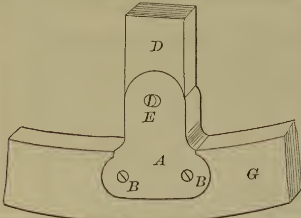
52744—A. Quirolo—Stereoscope.
