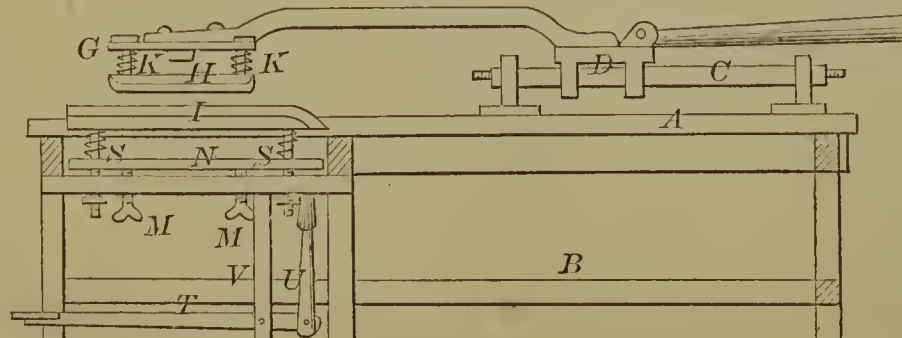
54821—J. Parker—For Boarding and Graining Leather.
