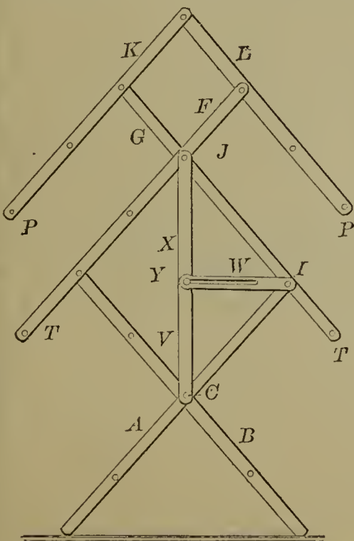
57681—I. C. Connor— Clothes Dryer.
