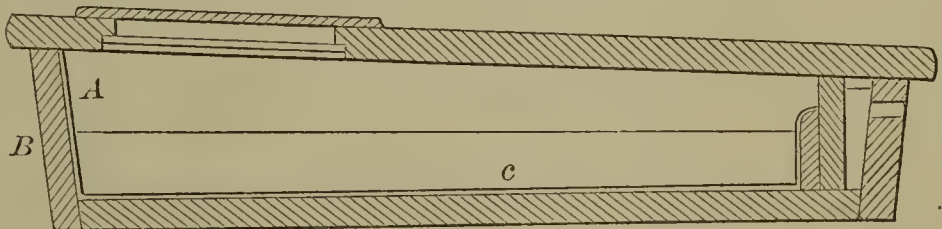
52756—G. W. Scollay—Burial Case.
