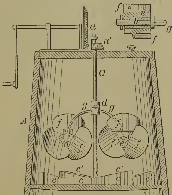
59811—E. H. Beckwith—Churn.
