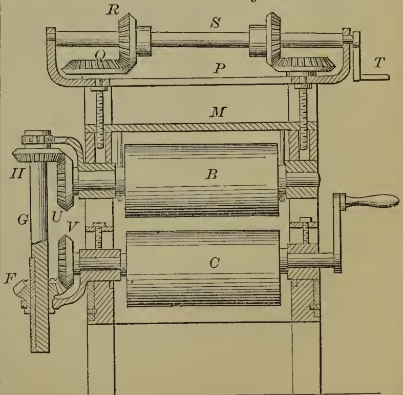
53466—W. B. McIver— Planing Machine.
