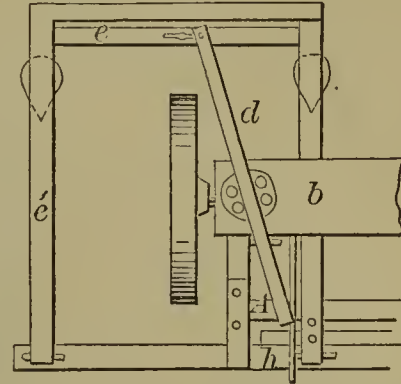
54844—H. E. Bodwell, Jr.— Sewing Machine Guide for Stitching Hats.
