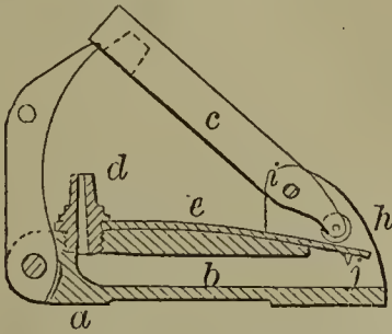
58645—C. Huie—Horse Shoe Punch.
