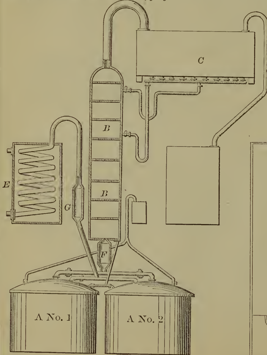
59149 H Lamotte—For Rectifying Alcohol.
