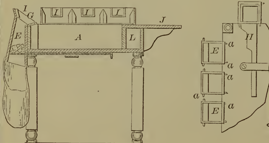
59883—G. Whitaker—Distributing Table.
