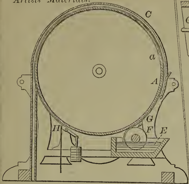
60386—Kirk & Pendergast—Wool Oiling Apparatus.
