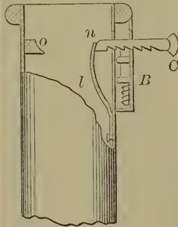
59278—H. Saylor— Whip Soeket.
