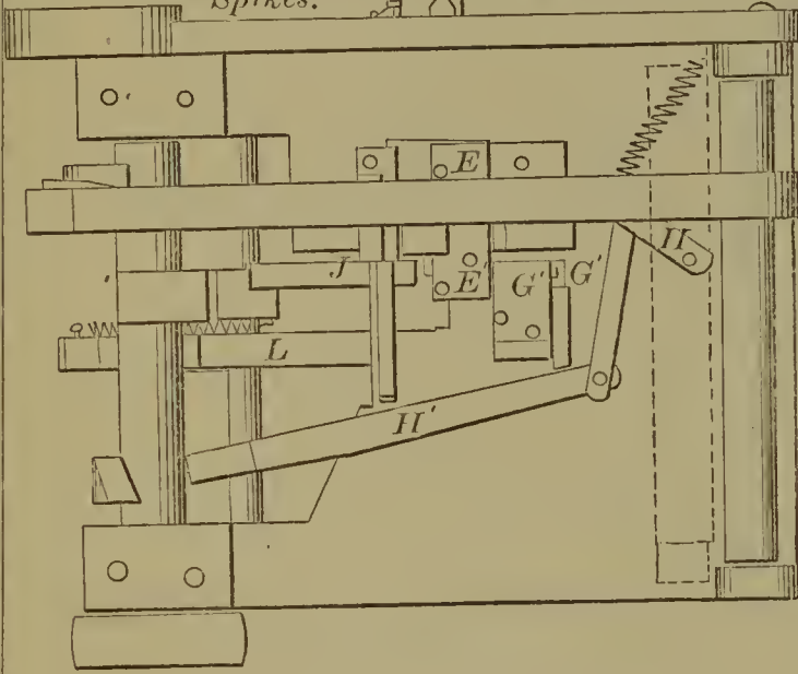
58521—A. Whittemore—For Making Split Spikes.
