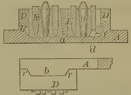
56161—H. H. Baker—Horse Shoe.
