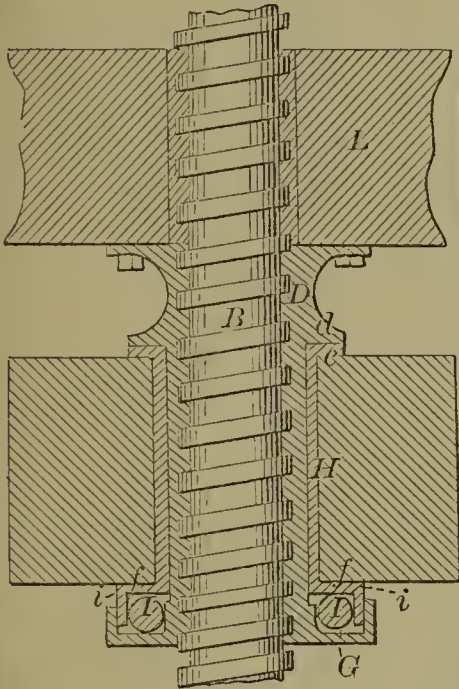
58342—R. H. Gray— Lifting and Pressing Screw.
