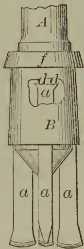
51925—A. G. Coles— Well Drill.
