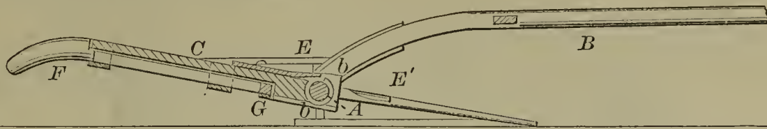
52098—A. Wells—Horse Rake.
