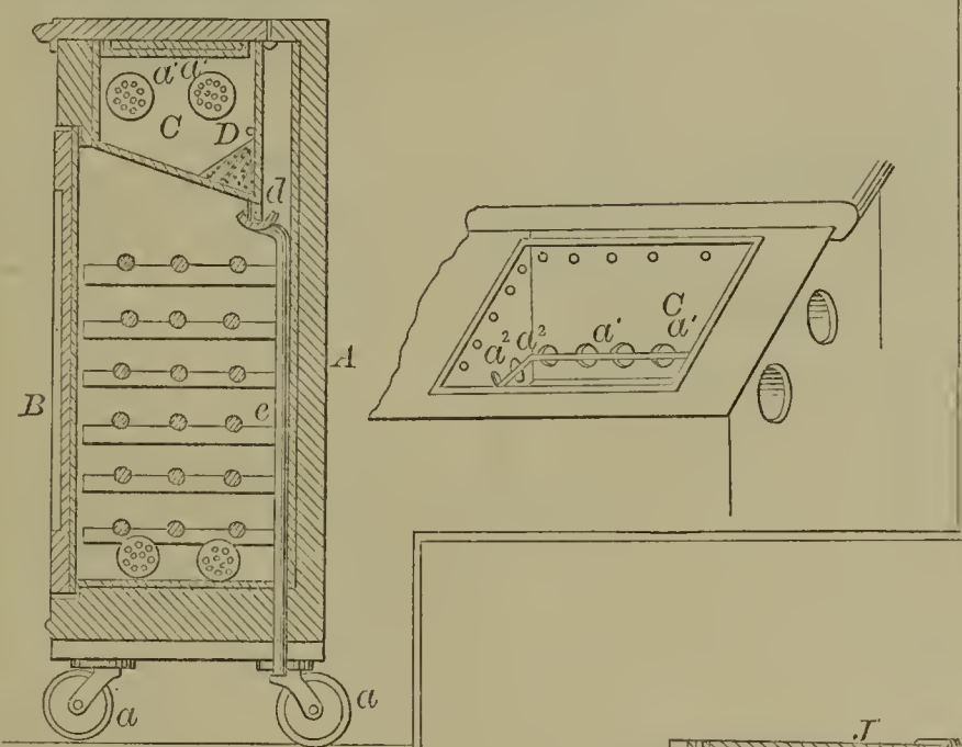
52436—J. McKelvey—Refrigerator.
