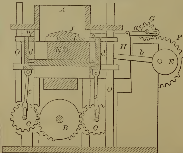
55146—I. Morley—Brick Machine.
