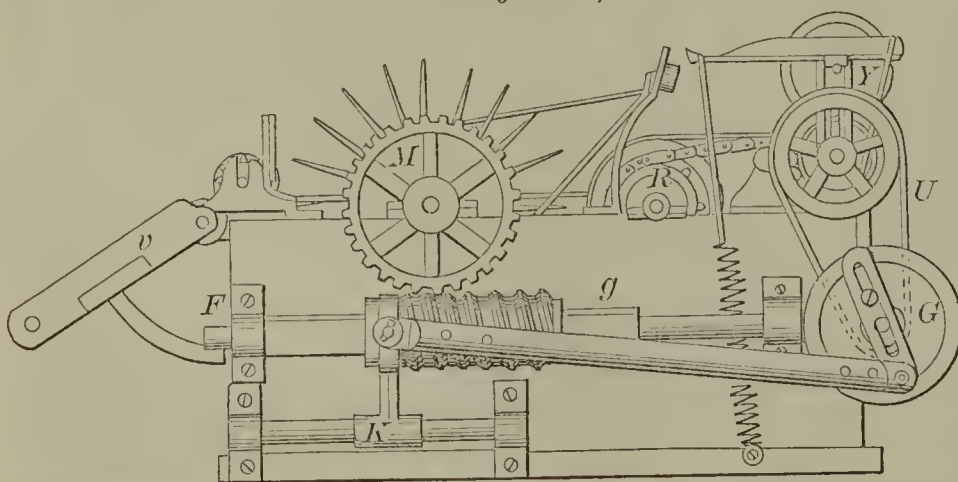
51900—W. Murkland—For Washing Wool, &c.
