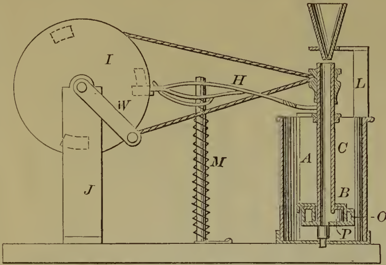
54081—J. A. Pastorelli—Extracting Turpentine from Wood.
