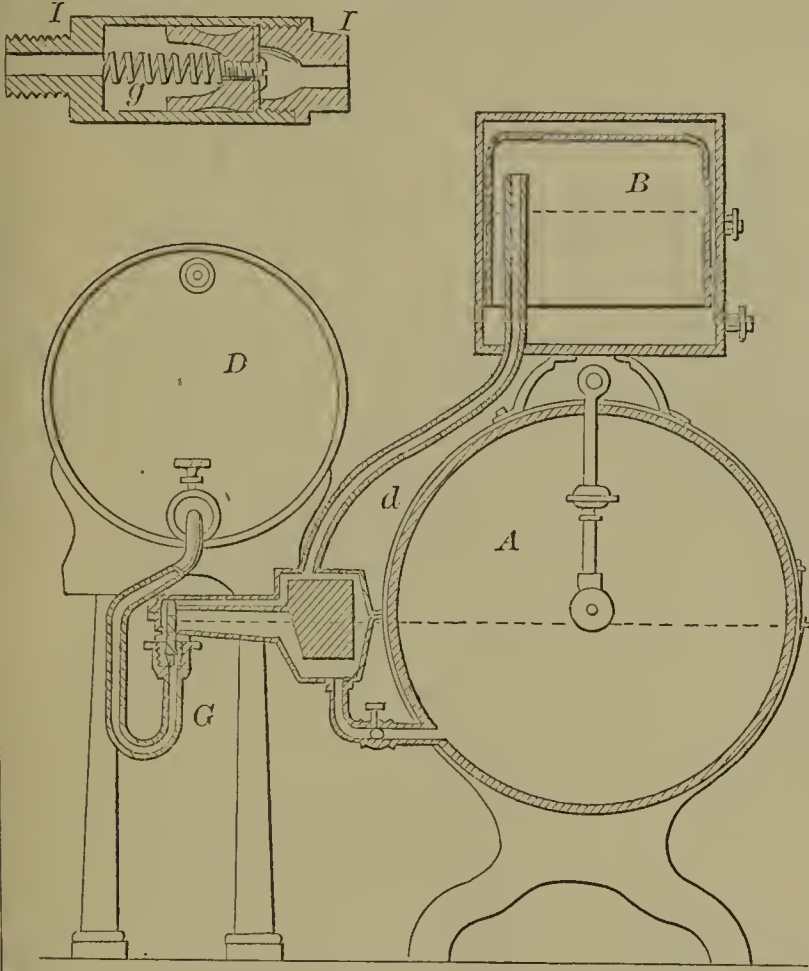
59146—Woodford & Bancroft—Steam Generator.
