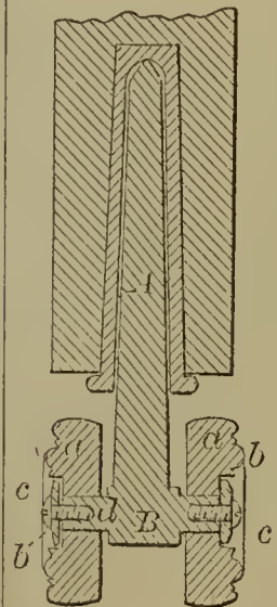
59163—J. T. Barnes—Furniture Caster.
