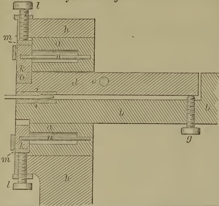
52494—L. Kirkup—Bolt-Heading Machine.
