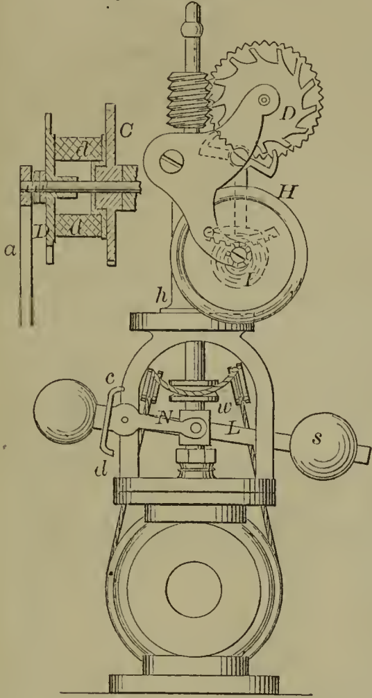
57490—R. Eickemeyer— Steam Engine Governor.
