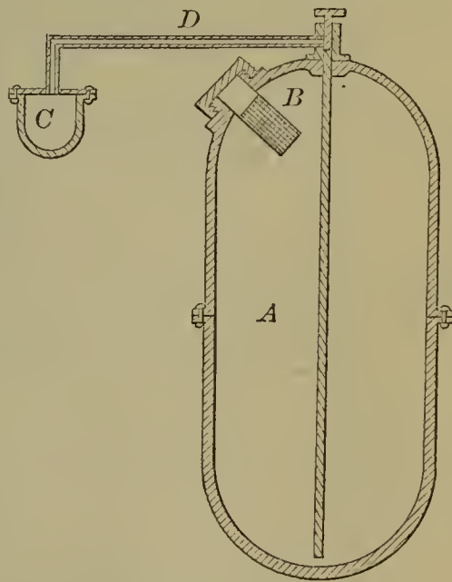
55040—J. S. Baldwin—Charging Water with Carbonic Acid.
