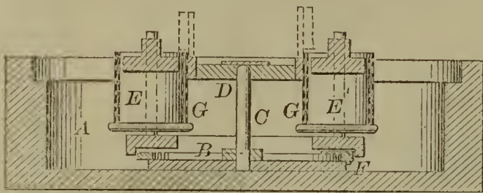
57353—G. B. Massey—Railroad Turn Table.
