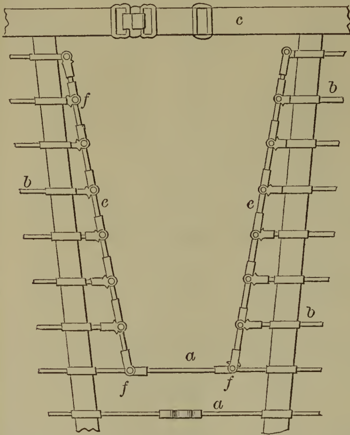
56019—Dixon & Close—Gate.
