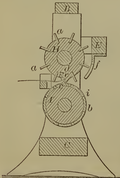
53228—A. Leland— Perforating Metal Bands.
