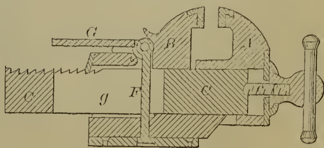
54352—H. P. Hood—Bench Vise.
