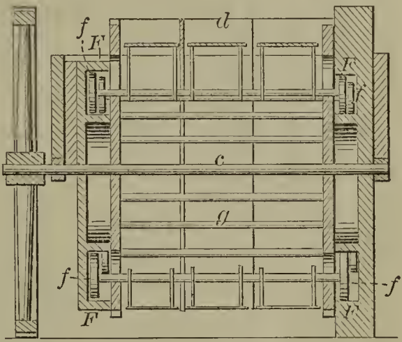
52245—J. Grant—Brick Machine.
