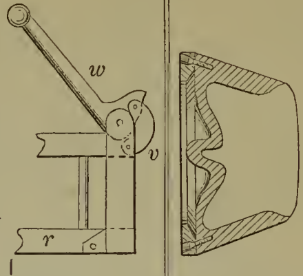
55210—J. F. Severance—Stove Pipe Thimble.
