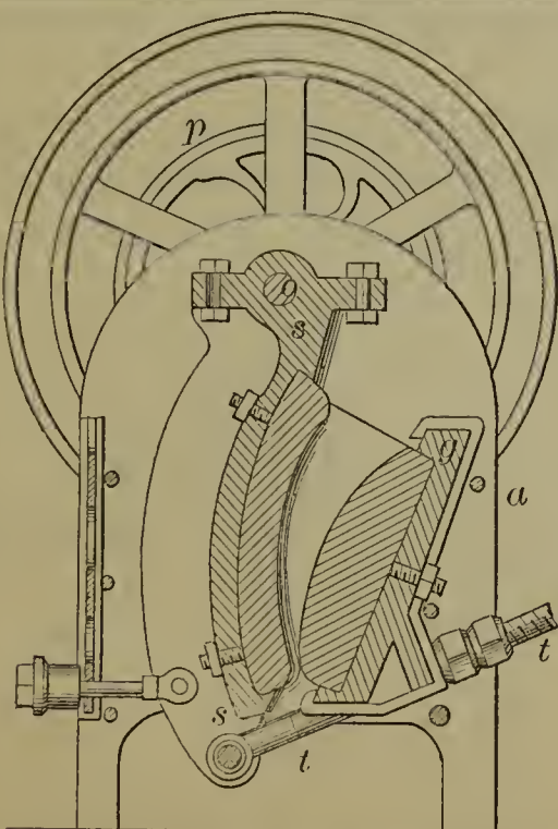
53066—Z. Wheeler—Ore Crusher.
