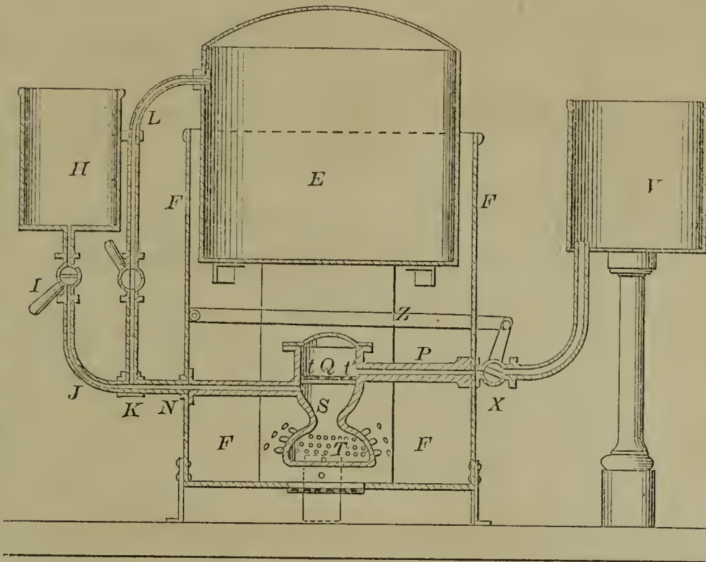
57430—T. D. Worrall— For Desulphurizing Quartz.
