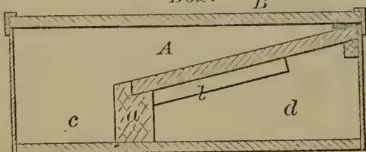
53275—C. D. Copeland—Knife Cleaning Box.
