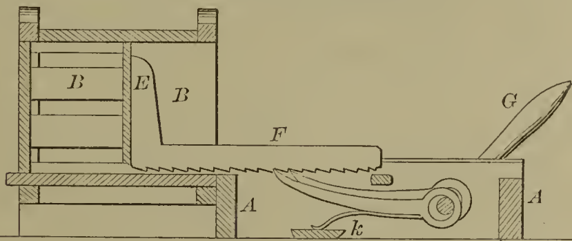
52786—Day & Noel—Hay and Cotton Press.
