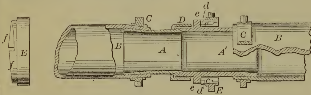
52839—J. E. Ford—Car Coupling.
