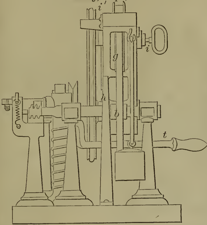
55336—Merriam & Norton—Cutting Machine.
