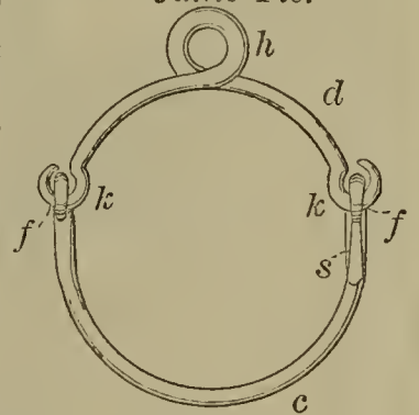
55727—H. C. Small— Cattle Tie.
