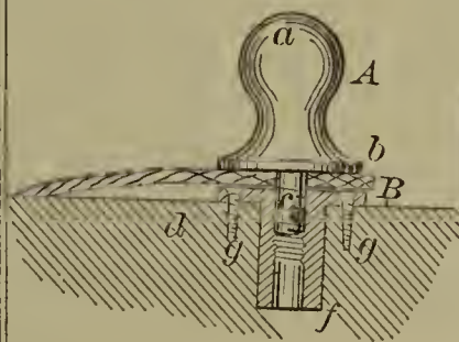
52985—J. H. Friederich—Carpet Fastener.
