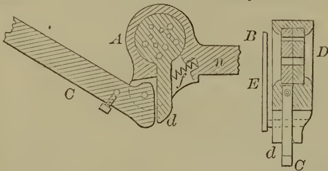
54520—W. H. Flinn— For Cutting Wire.
