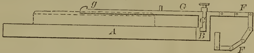
56123—J. W. Thyng— Printing Press.
