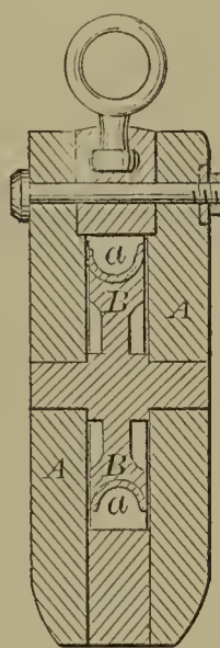
57610—Wicks & Fowler—Tackle Block for Hay Elevators.
