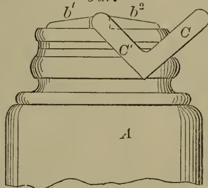
56226—J. Johnson— Fruit Jar.
