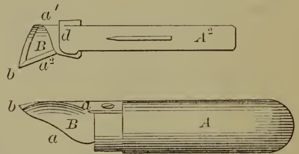
56368—S. P. Chapin—For Opening Cans.
