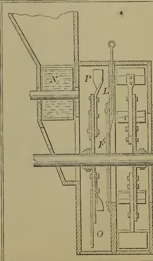
59685—Whepley & Storer—For Feeding Fuel to Furnaces.
