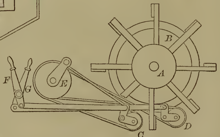
56118—J. M. Story— For Driving Paddle Wheels.
