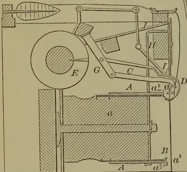
53001—R. B. Hugunin—Roller for Clothes Wringers.
