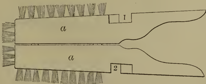
52787—S. Gissinger—Blacking Brush and Boot Jack.
