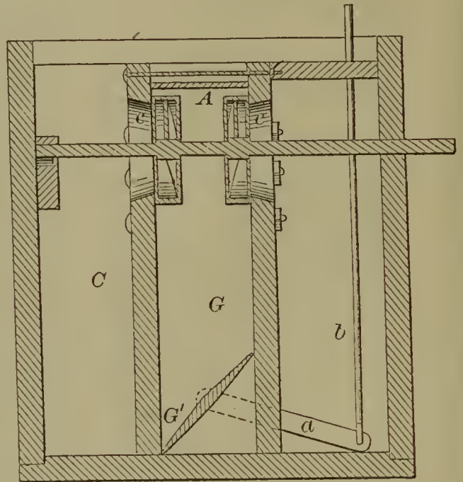
56560—R. S. Holton—Water Wheel.
