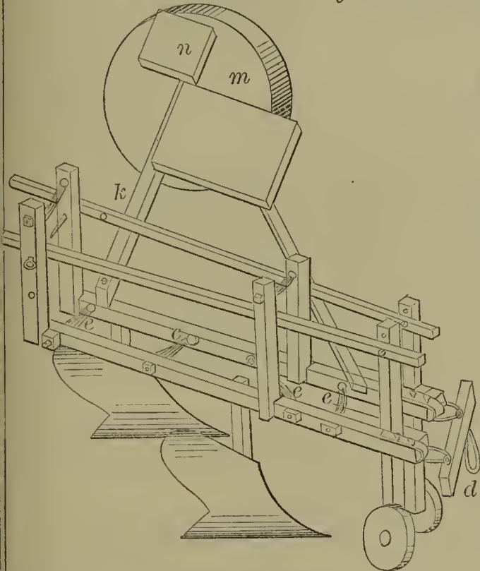
54453—W. M. Watson— Gang Plow.
