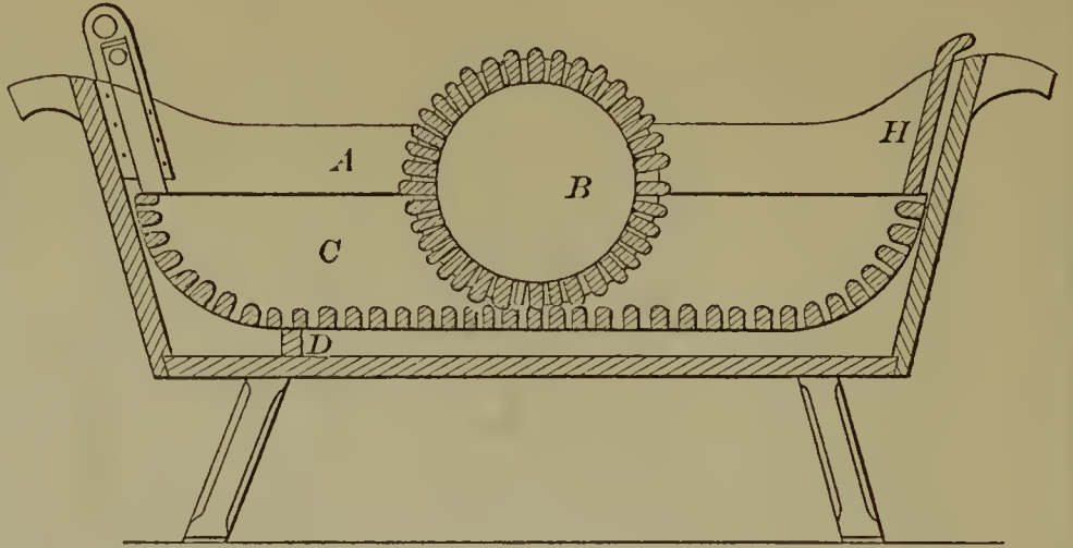
53177—J. Peacock—Barrel Washing Machine.
