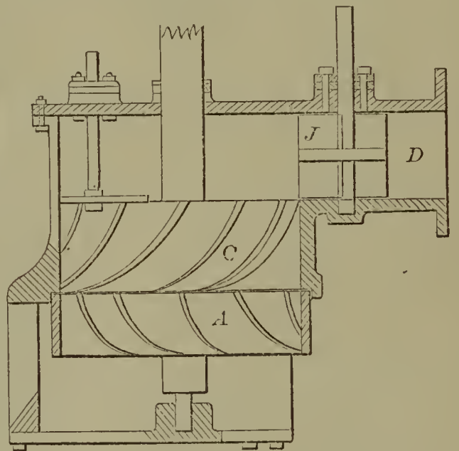
58846—A. Lind— Water Wheel.
