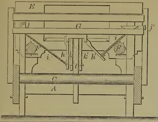
57719—J. Hollinger—Cultivator.
