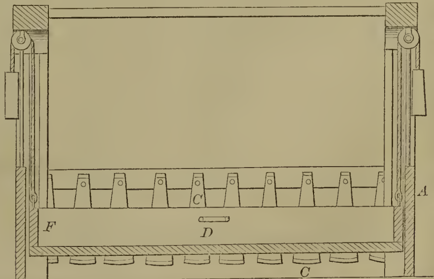
55370—D. F. Sexton—Sheep Rack.
