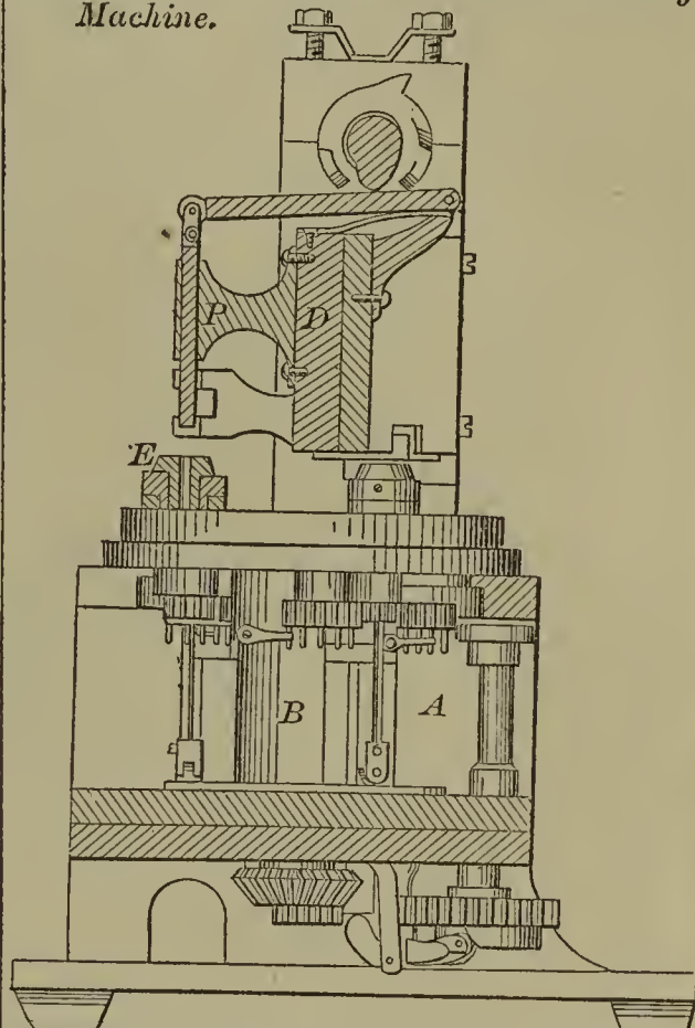
58092—J. French—Inserting Fusible Plugs in Steam Generators.
