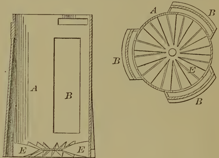
54850—P. Budenbach— Headlight for Engines.
