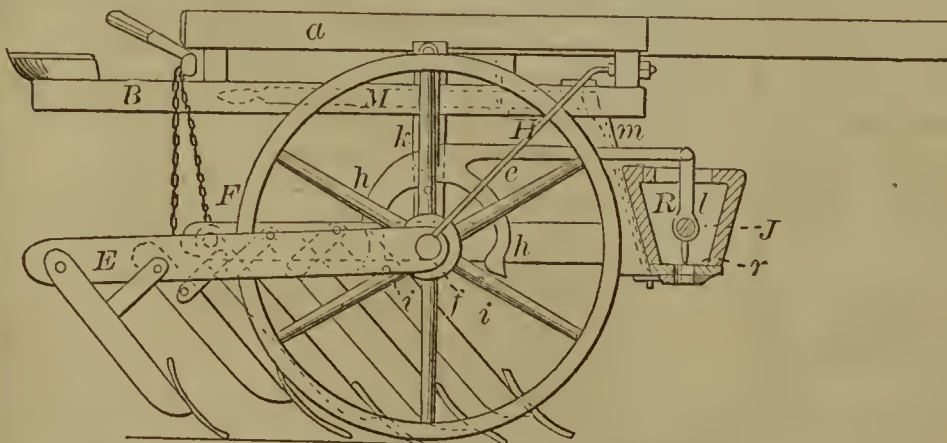
56454—S. C. Schofield—Seeder and Cultivator.
