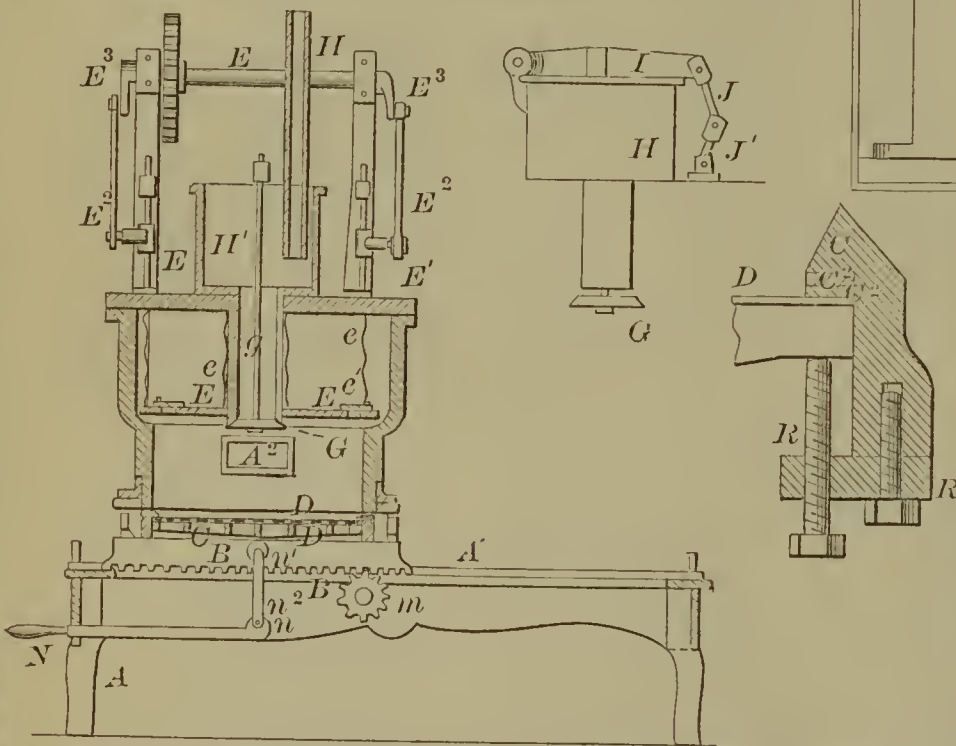
59509—S. R. Krom— For Separating Metals from Ores.
