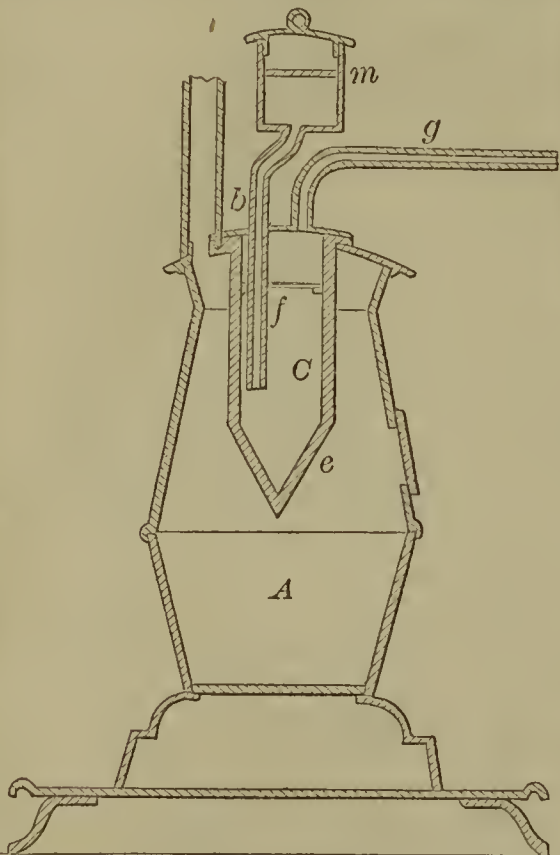
55328—J. McWilliams—Gas Generator.
