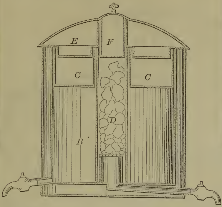
57284—W. Bryant—For Suppressing Effluvia from Drains.
