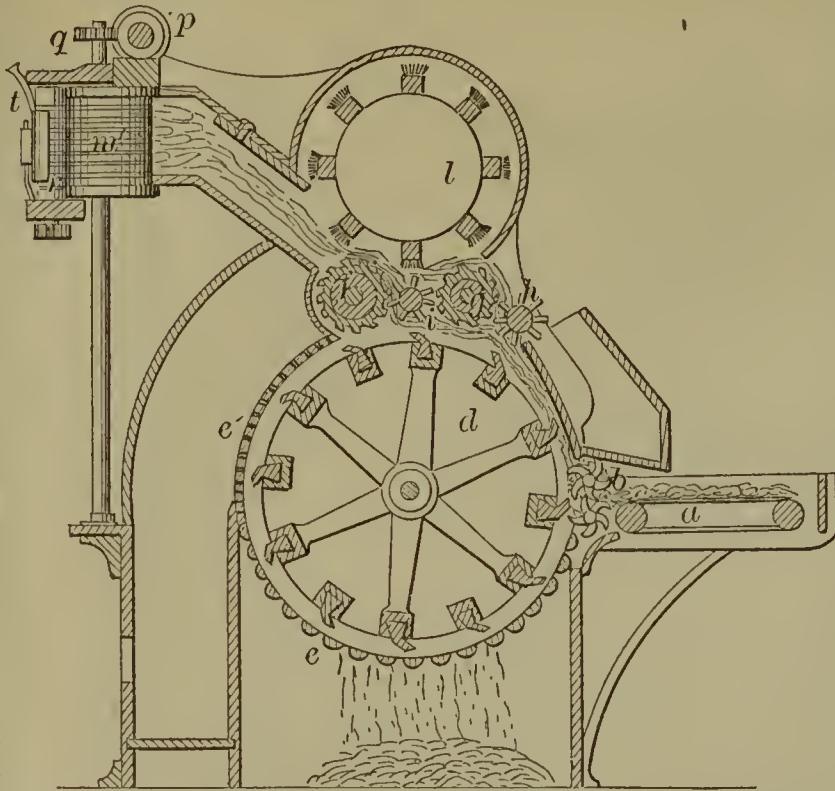
56675—S. R. Parkhurst— Picking and Cleaning Cotton, &c.
