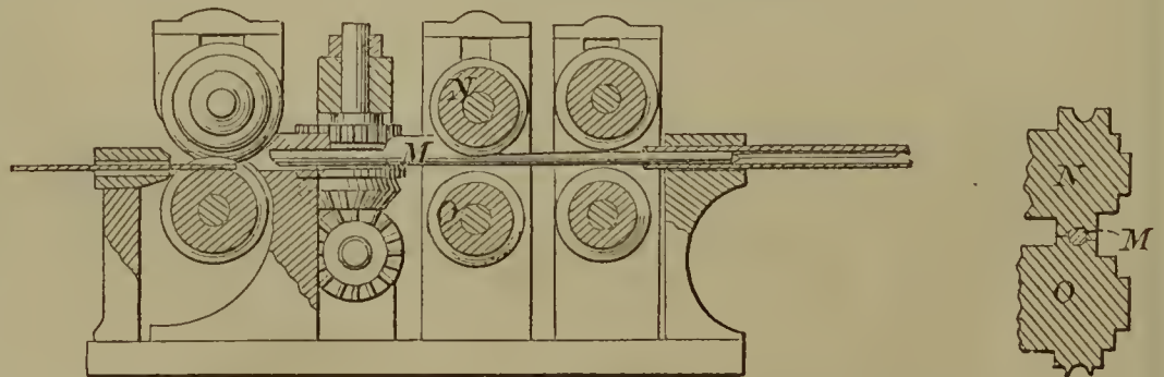
56561—H. Hotchkiss—For Making Metal Tubes.
