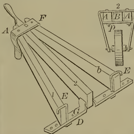
58805—J. Fridy—Cultivator.
