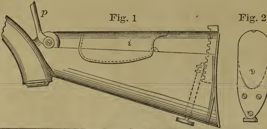
56506—C. W. Jones—Fire Arm.
