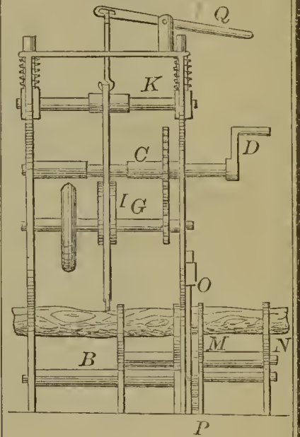
59368—H. A. Daniels— Sawing Machine.
