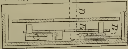
55549—Stachelin & Young—Lock.
