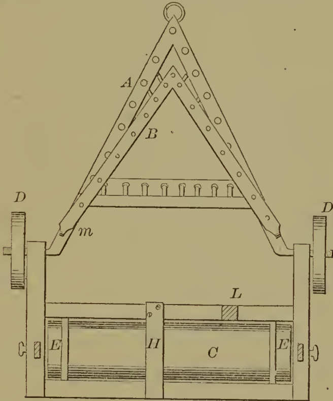
54790—Steiner & Miller—Harrow and Roller.
