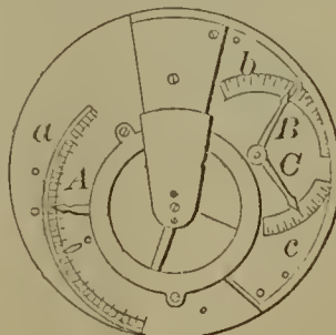
57848—W. M. Beeman—Register for Regulating Time Keepers.
