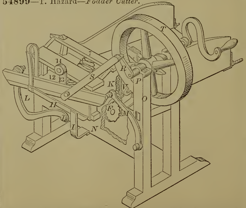
54899—T. Hazard— Folder Cutter.
