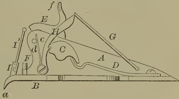
60162—W. Farnham—Burglar Alarm.
