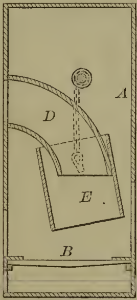
52738—S. W. Norton— Hot Air Furnace.
