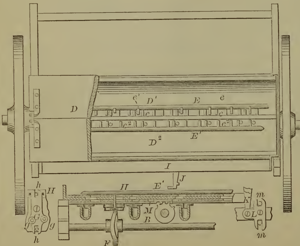
55243—G. E. Cooper— Drill and Fertilizer.
