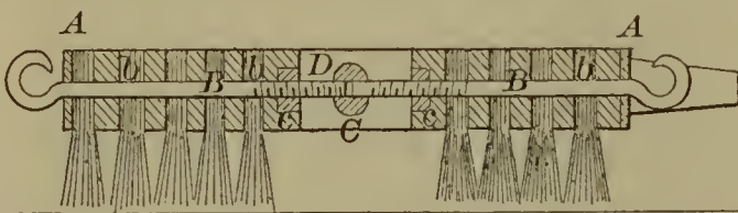
56038—C. L. Goddard— Wool Burring and Carding Machine.
