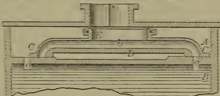
60252—W. B. Robinson—Slide Valve.
