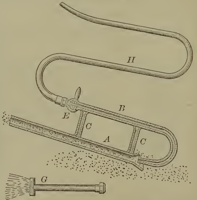
52309—W. Moses—Grain Mover.
