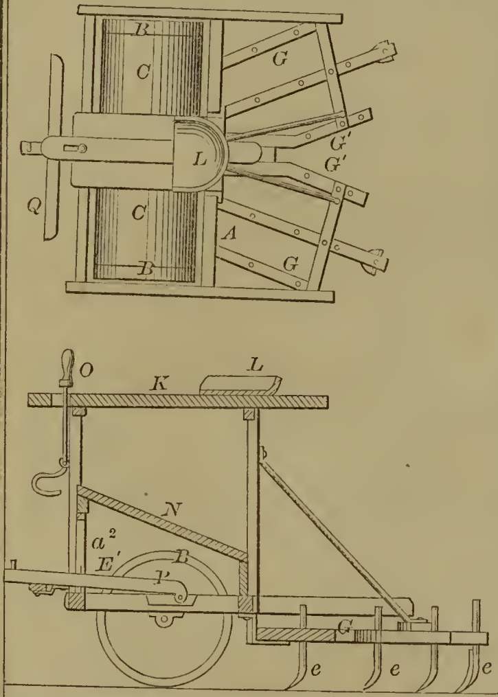
60655—G. H. Woodruff—Roller and Harrow.
