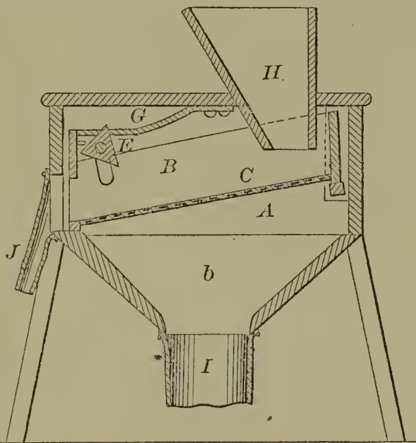
59964—P. Ceredo—Ash Sifter.
