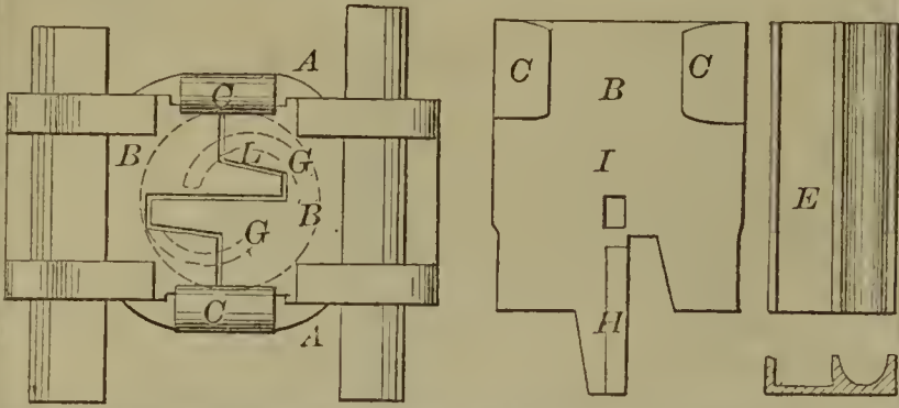
57142—E. F. Hurd— For Making Axes.
