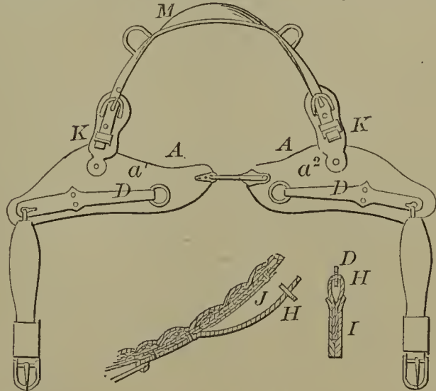
60031—A. McMullen—Hame Tug and Breast Collar.
