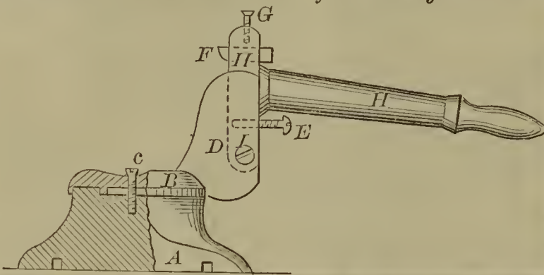
55749—W. T. Vose—Lathe Rest for Turning Balls.
