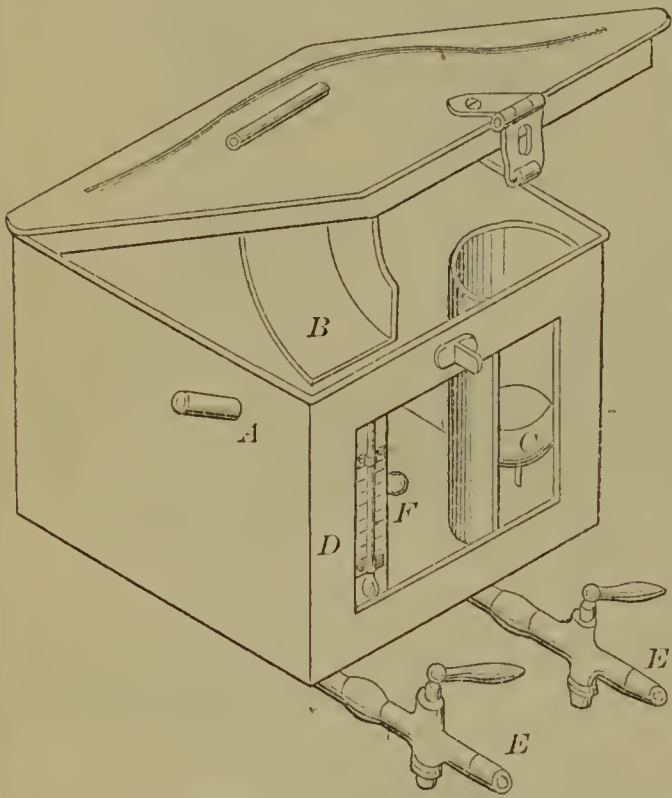
59688—W. J. Walker—Apparatus to be attached to Stills to prevent frauds on the Revenue.
