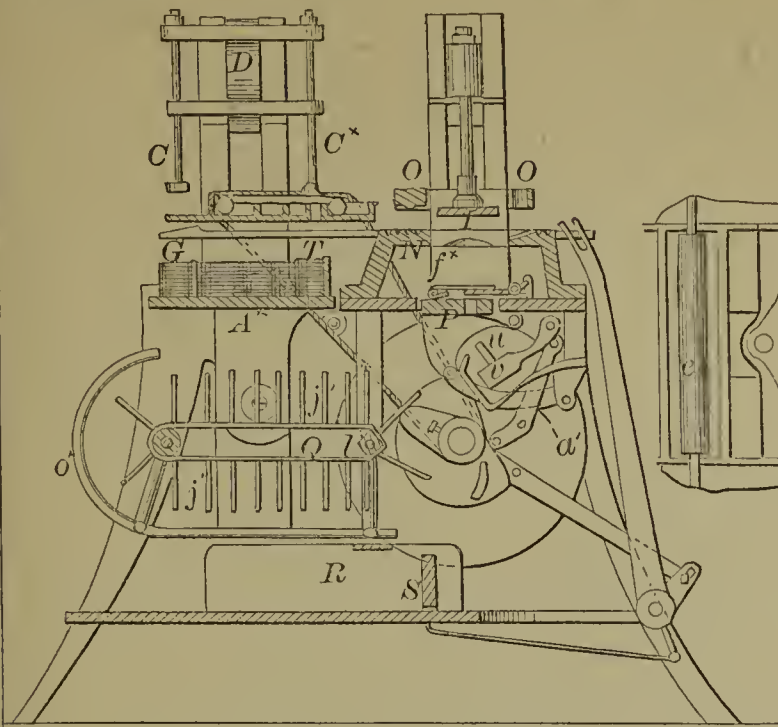
58327--T. V. Waymoth--Envelope Machine.
