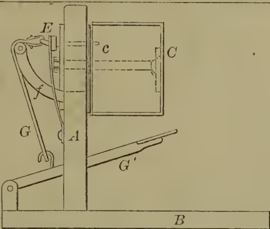
60617—W. D. Burnett— Anvil to Rivet Trunks .
