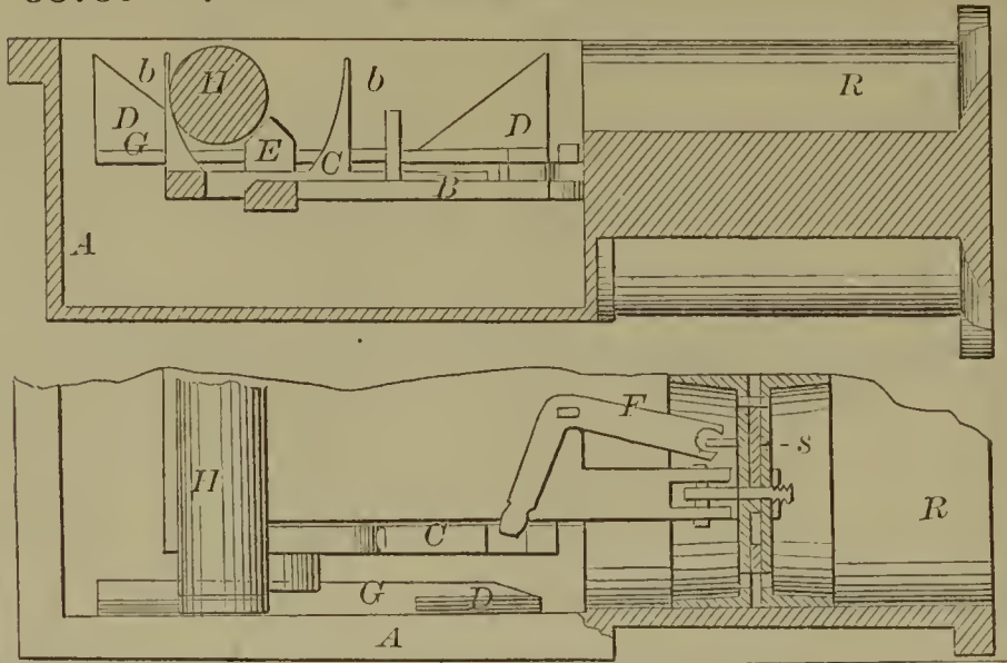
58739—Bailly, Durand, Mesnard & Poirier— Anti-Friction Device for Axles.
