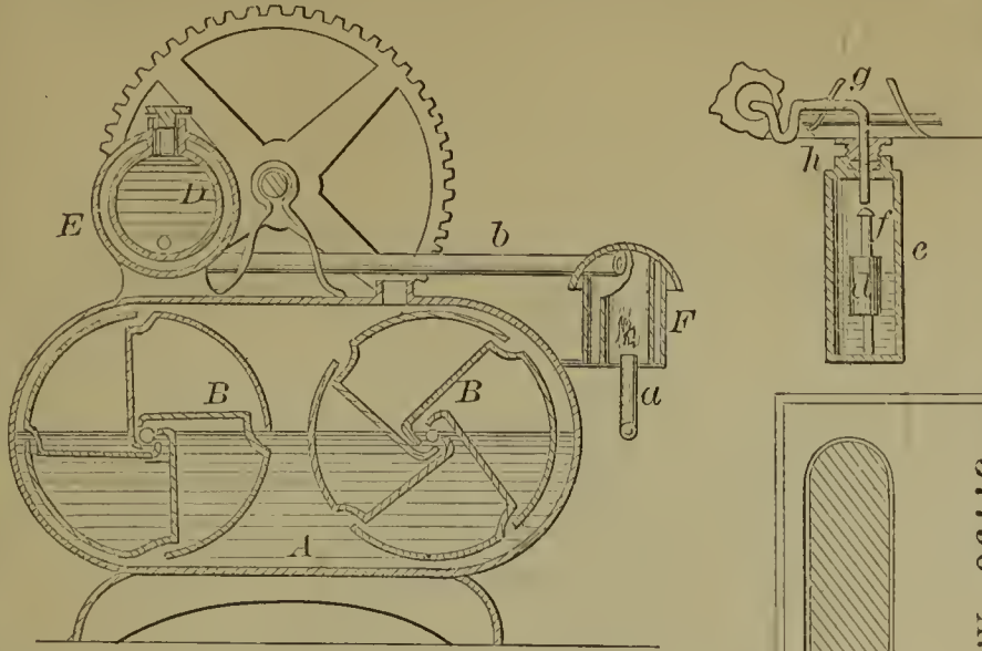
57788—J. F. Spence—For Carburetting Air.
