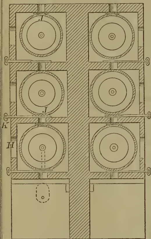
56549—E. Gaussoin—Treating Ores with Chlorine.
