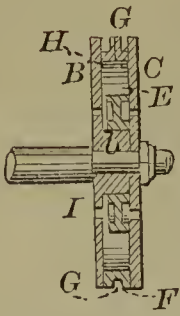
57916—A. W. Jackson—Piston Packing.
