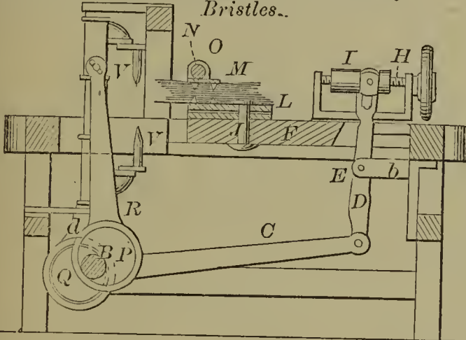
54564—Lannay & Parks—For Combing Bristles.
