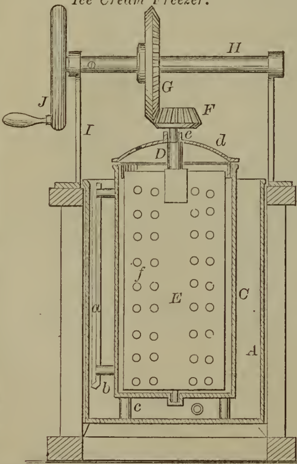
55960—T. W. Pomeroy— Churn and Ice Cream Freezer.
