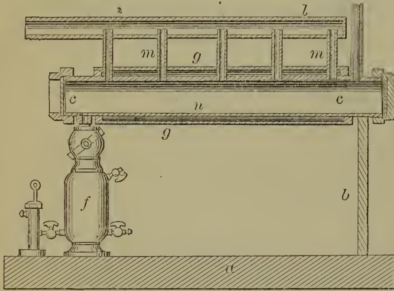
54629—C. Wahl—Vacuum Pan.
