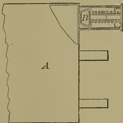
58496—T. S. Speakman— Safety Valve in Water Backs for Ranges.
