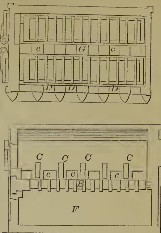
56919—J. Fieldhouse—Furnace.
