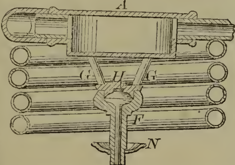
57576—H. S. Saroni—Steam Generator Feed Water Heater.
