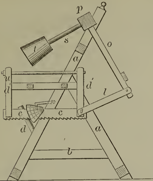
51851—W. Melville—Sawing Machine.
