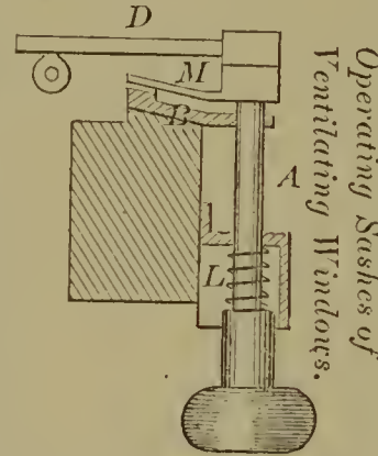
54818—E. Lockwood—Operating Sashes of Ventilating Windows.
