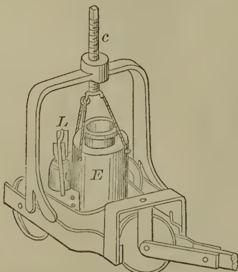
52324—J. Ryan—Hydraulic Jack.
