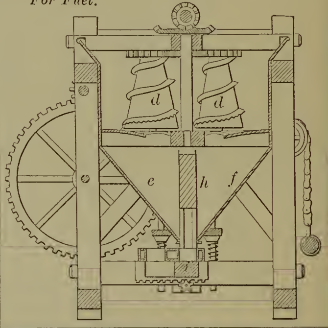
53538—S. Marden—For Preparing Peat For Fuel.
