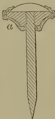
52781—H. P. Brooks—Picture Nail.
