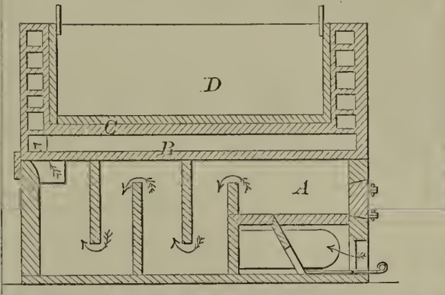
51921—J. Chilcott—Hot Air Furnace.
