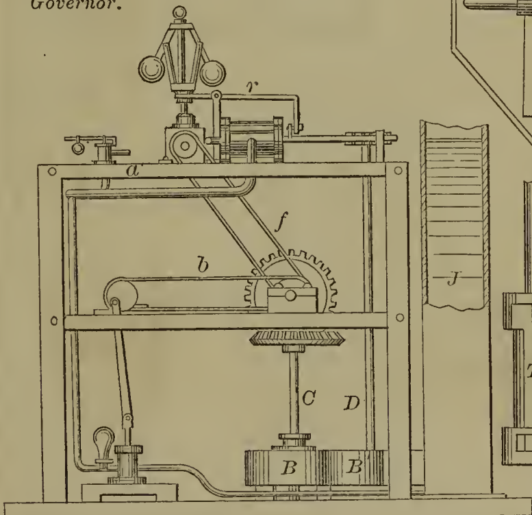
60632—S. M. Hunter— Hydraulic Governor.
