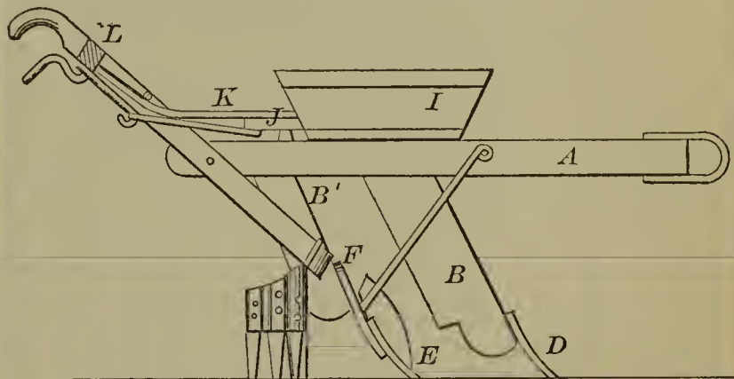
53156—M. H. Lineback— Corn Planter Cultivator.
