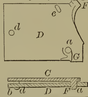
59144—C. Swett—Cotton Bale Tie.
