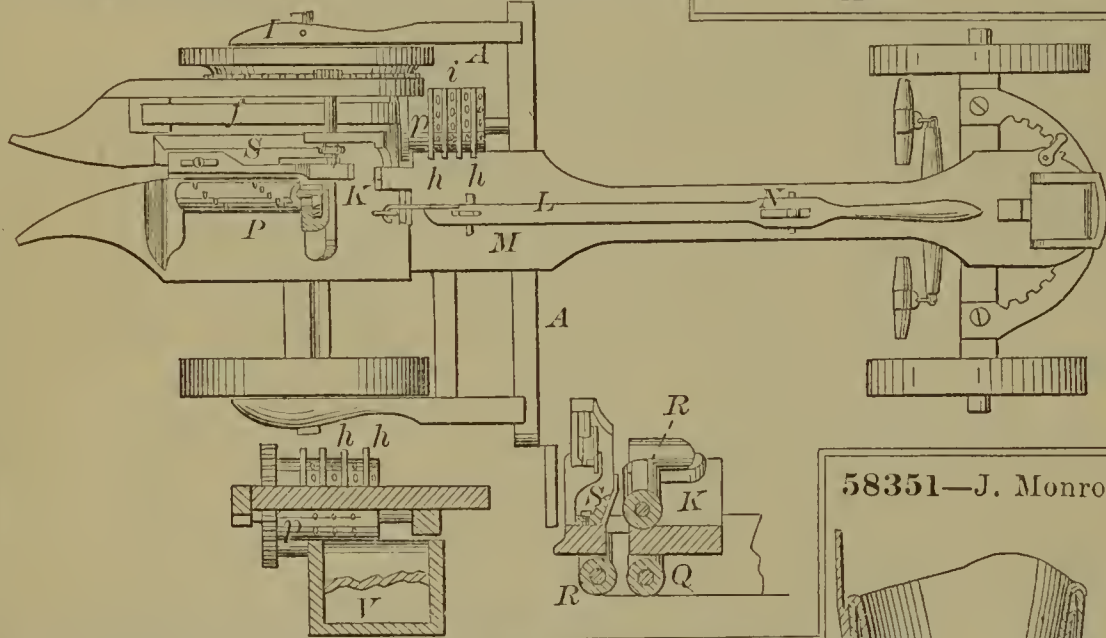
58347—S. J. Kelso—Cyphering Machine.
