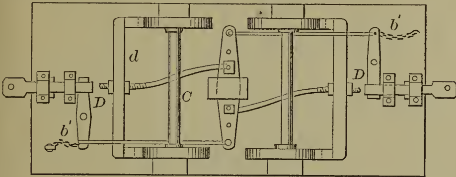
53544—D. T. Robinson— Car Brake.
