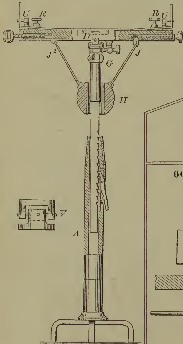
60346—S. L. Donnell—Grading Instrument.
