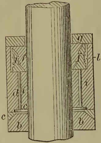
56658—F. Wright— Piston Rod Packing.
