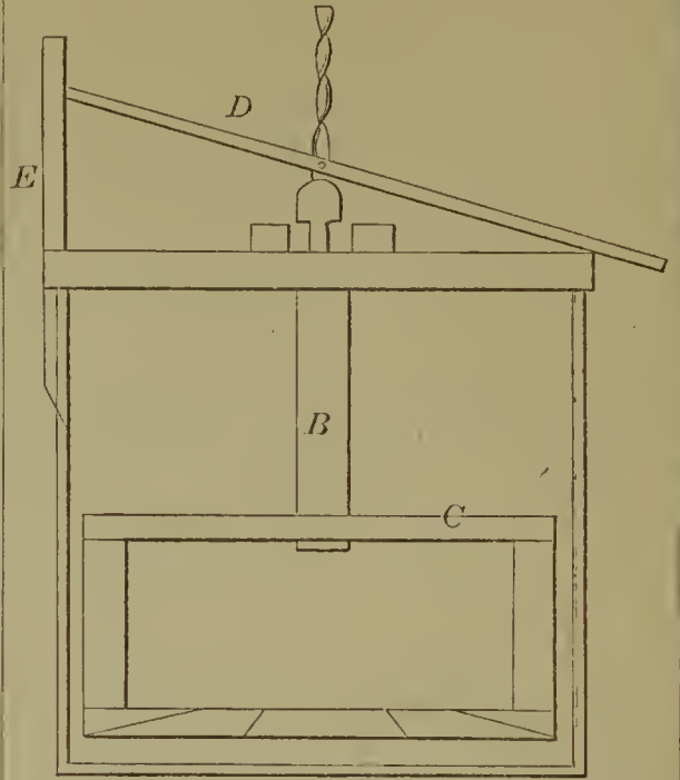
59444—W. Oreutt—Washing Machine and Churn.
