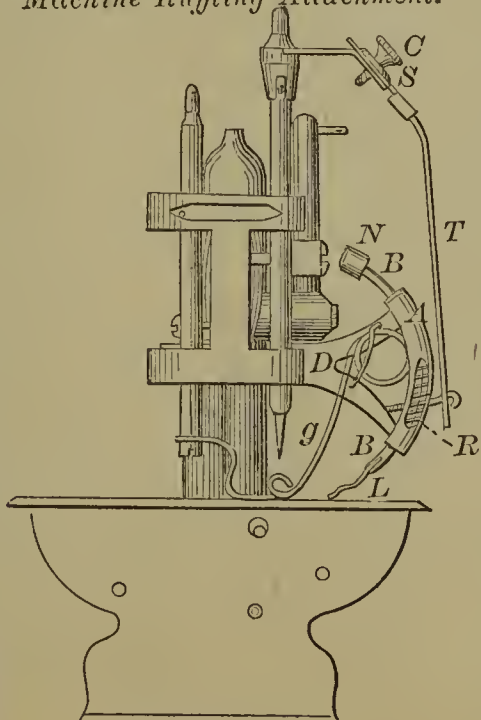
58376—D. C. Cary—Sewing Machine Ruffling Attachment.
