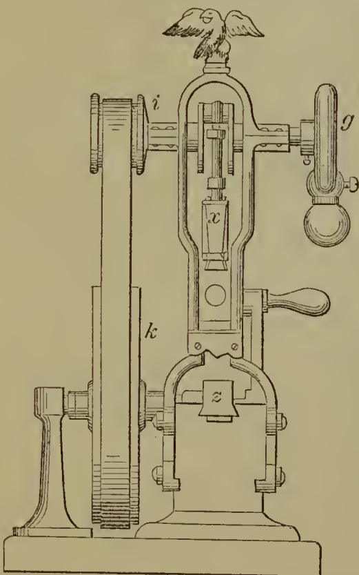
52894—T. Shaw— Power Hammer.
