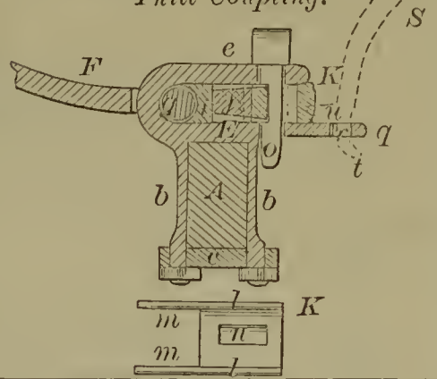
52619—J. L. Sesserott—Attaching Shafts to Vehicles.
