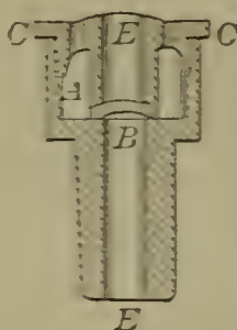
60252—W. B. Robinson—Slide Valve.
