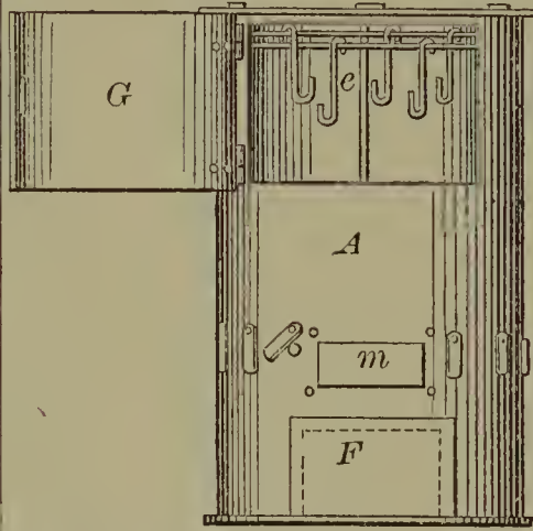
59931—L. S. Stevens—Metallic Smoke House.
