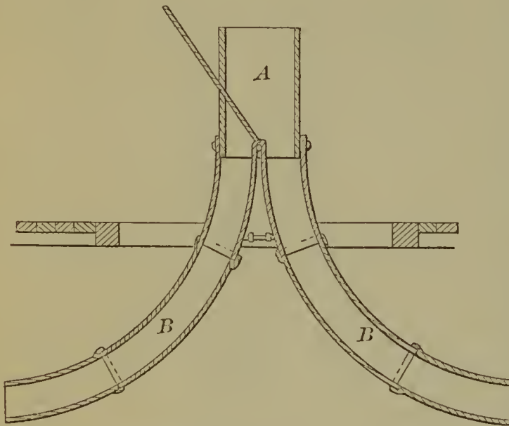
54322—A. D. Foote—Grain Spout.
