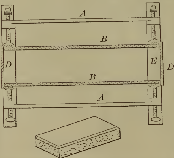
55667—F. Jones—Manufacture of Bricks.
