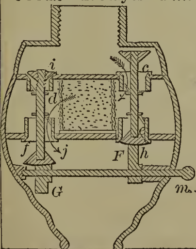
60512—T. Hayes—Filter.
