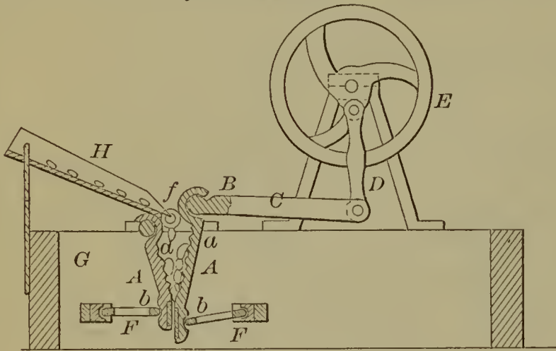
52837—J. Fleck—Quartz Crusher.
