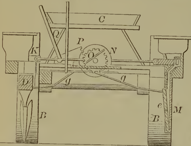
56970—P. McQuaid—For Marking Ground for Planting.
