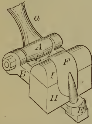
54574—F. McRoy—Attaching Thills to Vehicles.
