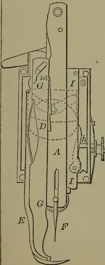
58614—J. A. Davis—Needle Feed of Sewing Machines.
