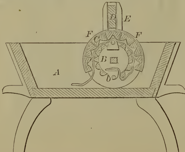
59005—J. J. Green— Washing Machine.
