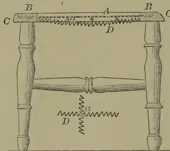
58917—J. Ungerer—Chair.
