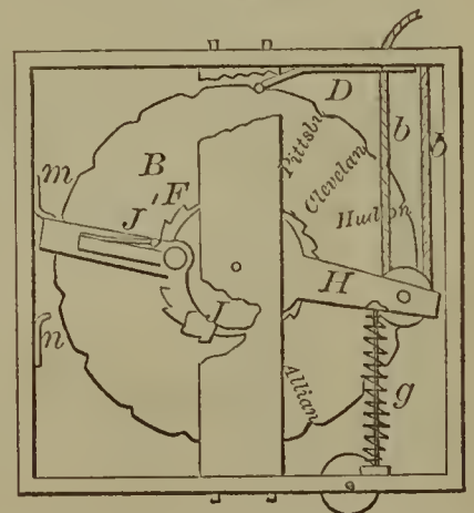
52704—C. C. Gale—Railroad Station Indicator.
