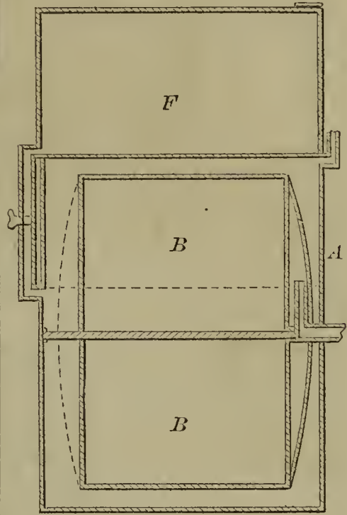
57442—D. McDonald— For Carburetting Air.
