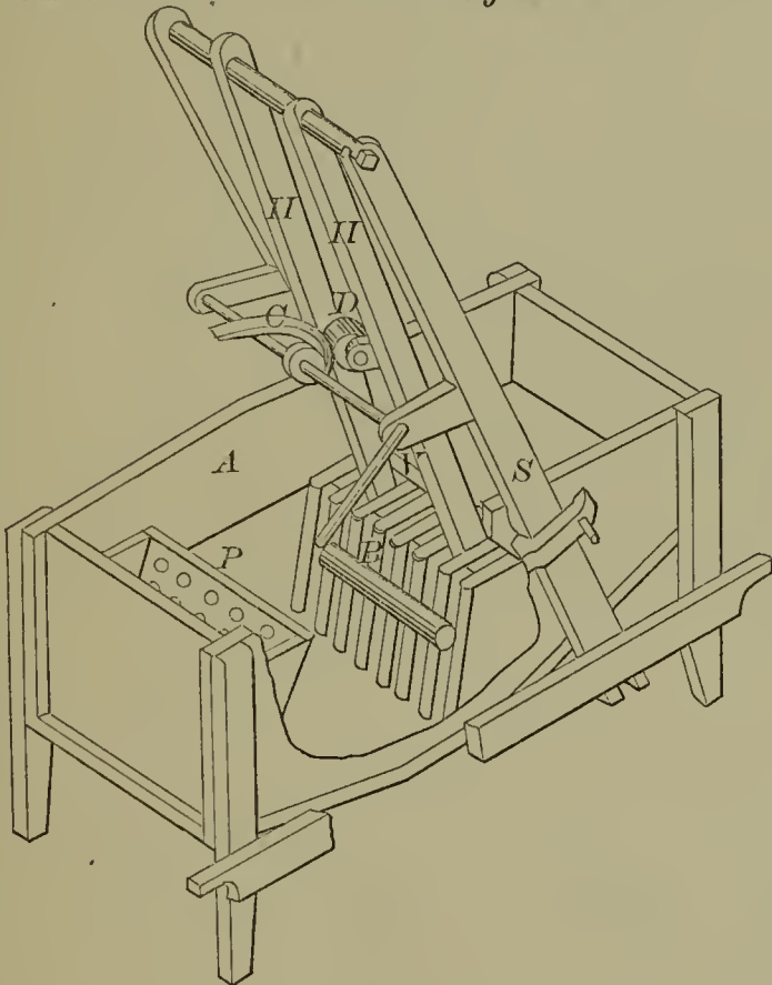
55471—E. H. Cook— Washing Machine.
