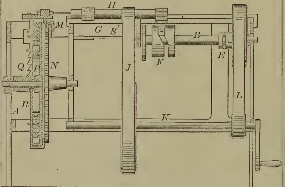
52409—J. H. Gibbs— For Boring Blinds.
