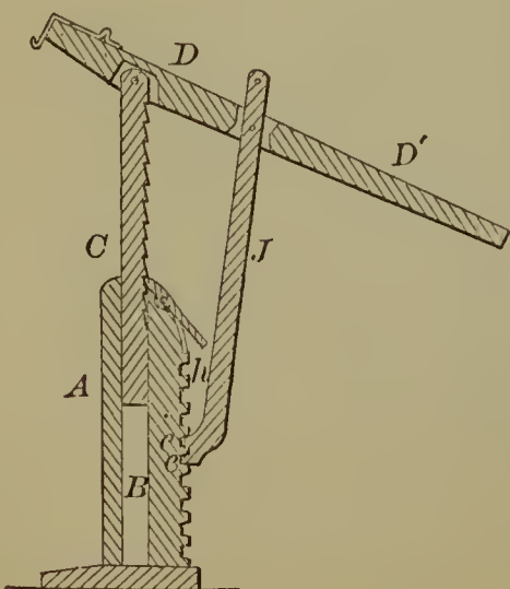
54706—D. Fasig— Lifting Jack.
