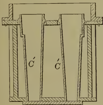
59840—J. G. Holt—Making Sand Cores for Axle Skeins and Hub Boxes.
