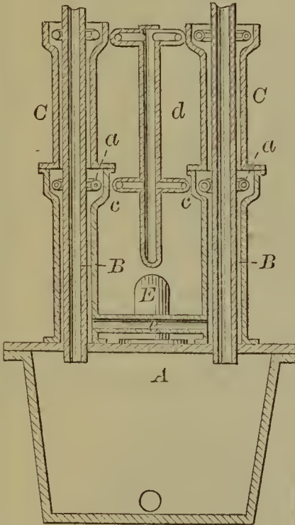
53967—A. C. Fletcher—Surface Condenser.
