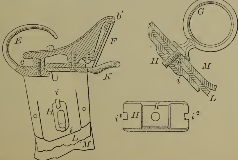
53578—E. A. Cooper—Gig Tree
