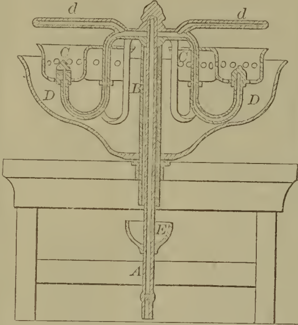
52565—A. Hallowell—For Washing Tumblers.
