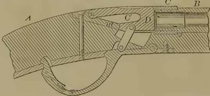
60607—T. Yates— Breech-Loading Fire Arm.
