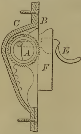
60633 —B. S. Hyers— Sash Fastener.
