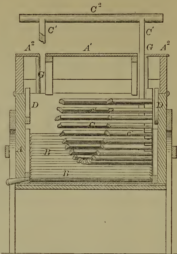
53844—P. Lutes—Washing Machine.
