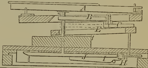
54397—A. Palmer— Harvester Crank Motion.
