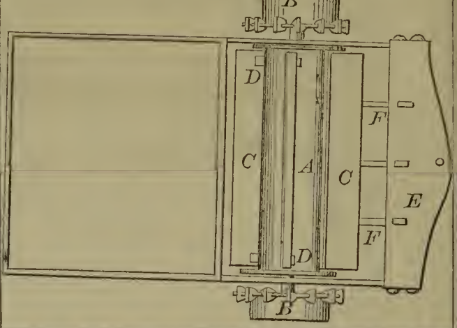
57105—R. H. Emerson—Turf Cutting Machine.
