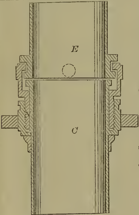
56223—R. Henrage— Hose Coupling.
