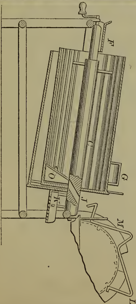
53221—G. B. Hamilton—Ore Washer.
