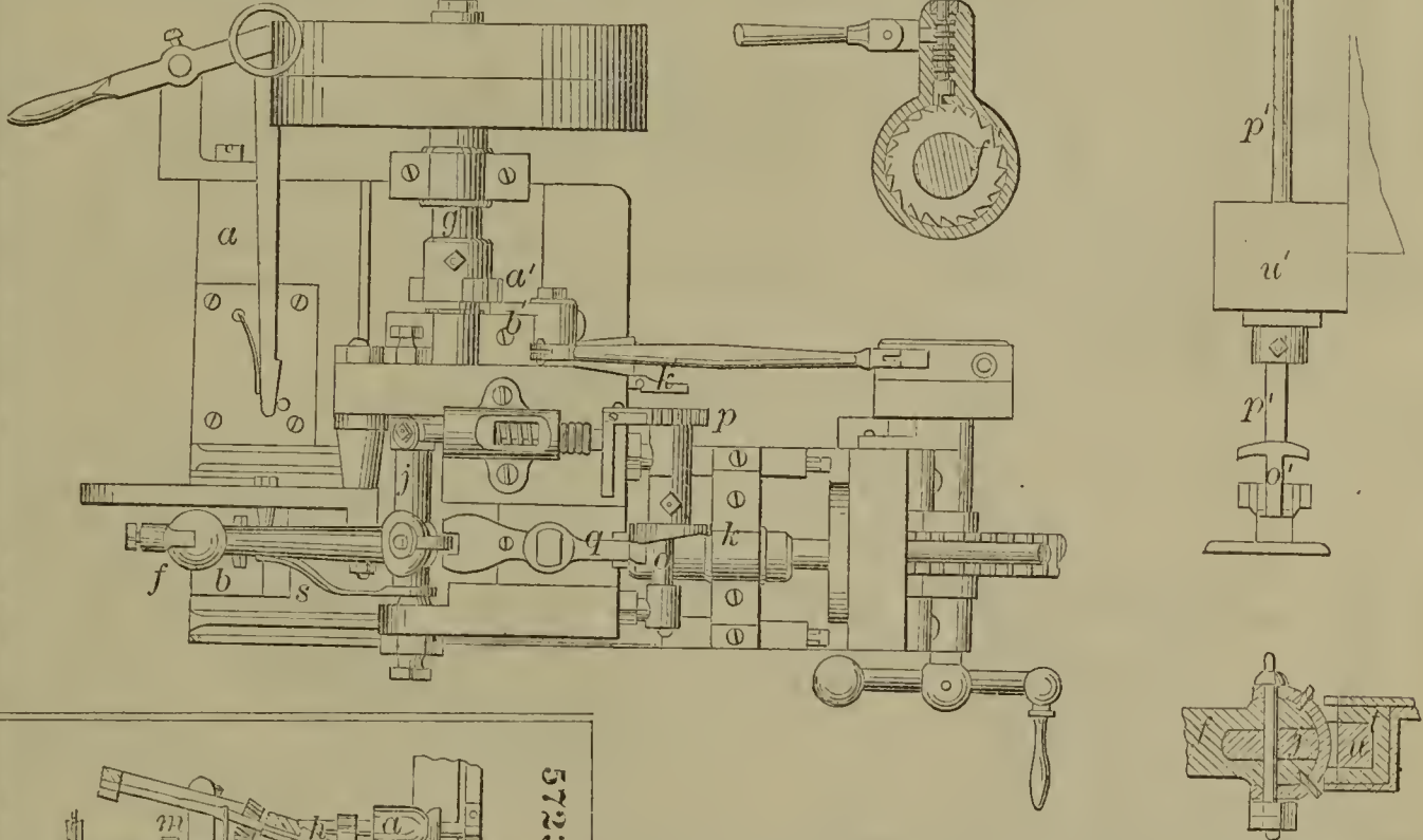
57231—G. E. West—Driving Fence Posts.
