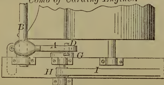
55046—A. A. Bennett— For Operating the Doffer Comb of Carding Engines.
