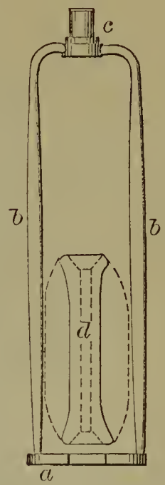
53874—G. Richardson—Flyer for Spinning.
