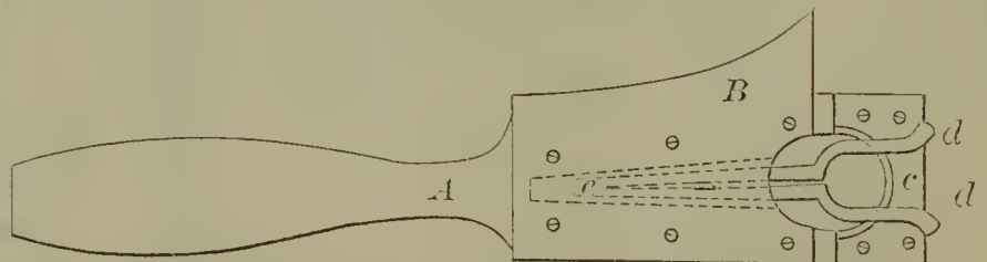
52282—N. Gabel—Corn Stalk Cutter and Stripper.
