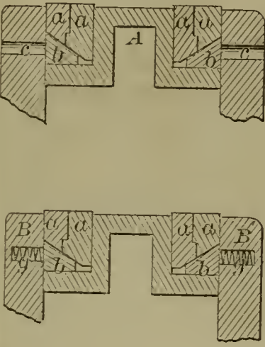
57375—E. T. Prindle—Piston Packing.
