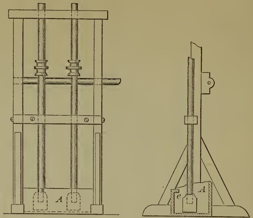
53552—S. F. Ambler— Quartz Crusher.
