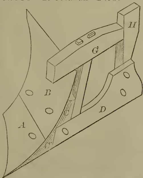
52539—T. Cottman— Plow.
