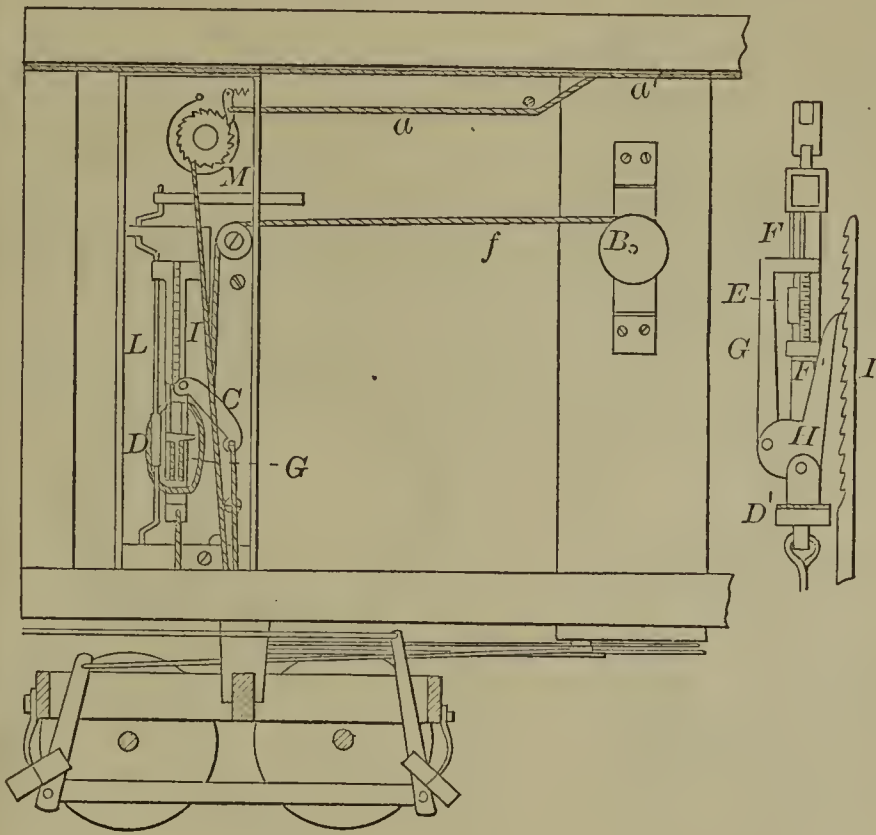
52310—D. Myers—Car Brake.
