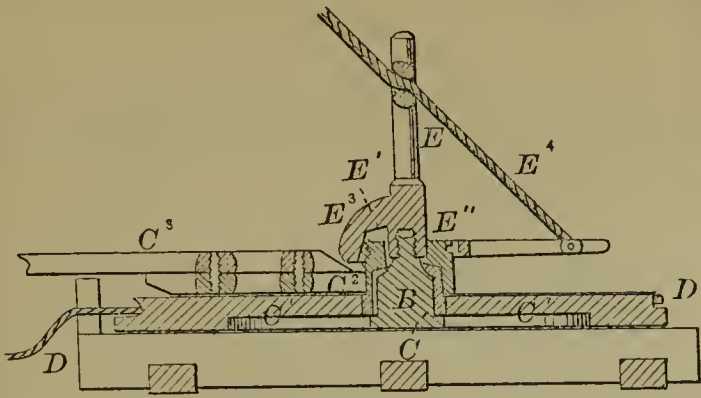
53380—J. W. Sefton—Churn.
