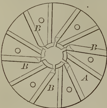
52015—F. J. Belknap—Shoe and Die for Amalgamating Machines.
