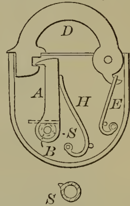
55167—C. W. Saladee—Padlock.
