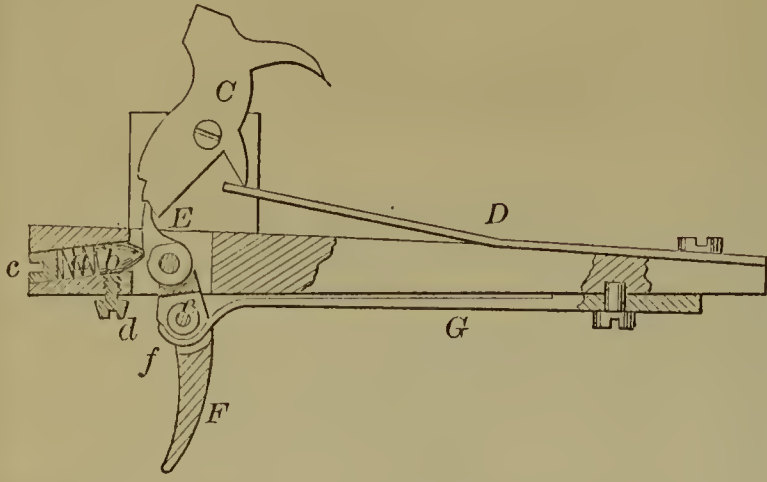
53306—E. C. Kirk— Gun Lock.
