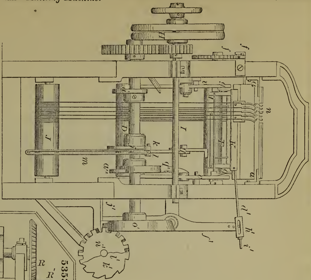
53530—J. Goodman—Knitting Machine.
