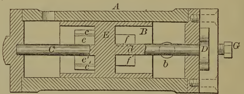
58307—D. Sexton—Rotary Valve.
