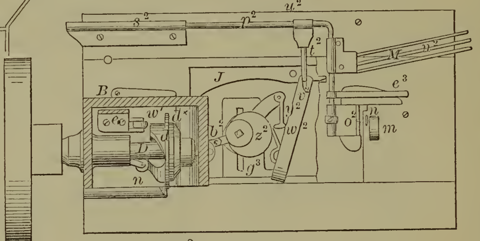
55182—A. Warth— Sewing Machine.
