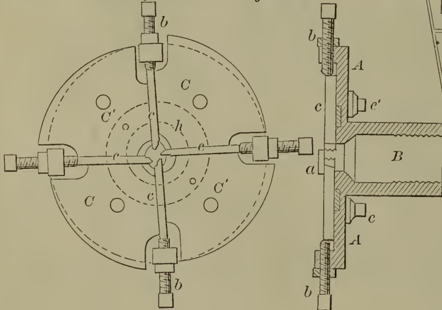
52294—T. Kennedy— Screw Cutting Chuck.
