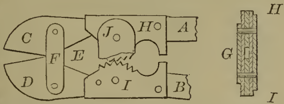
55366—D. D. Robinson—Rivet or Bolt Cutter.
