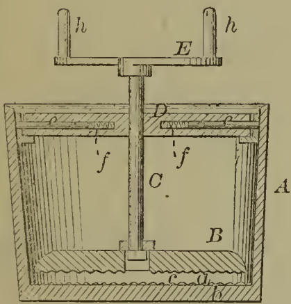
56748—D. G. Haskins—Steam Generator.
