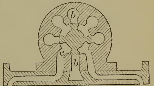
54959—T. Richards— Balanced Valve for Steam Engines.
