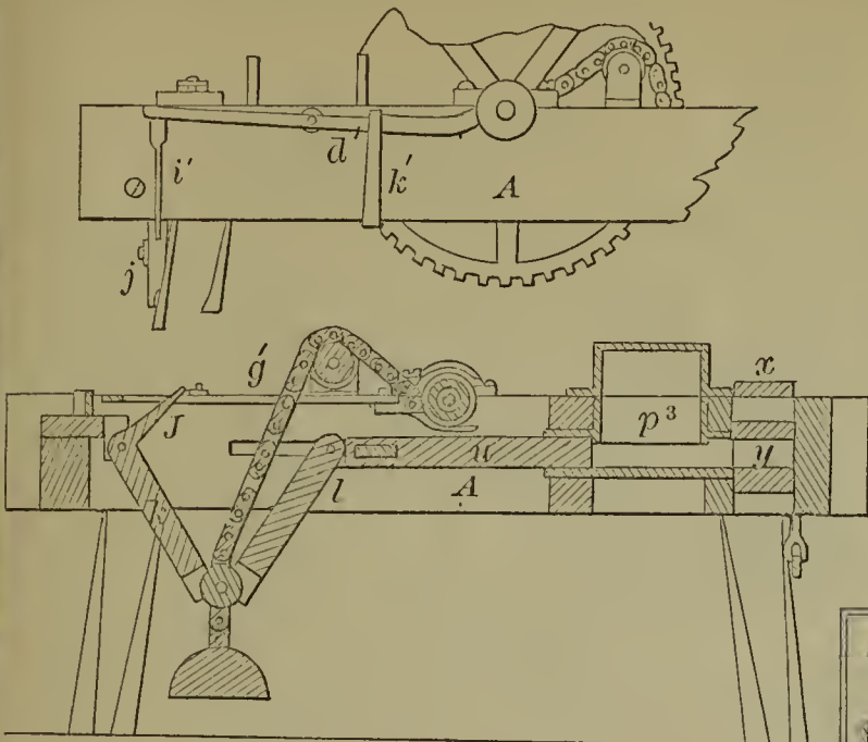
55205—S. Marden—For Preparing Peat.
