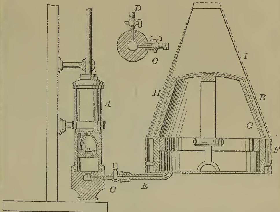
54528—E. Gilliam— For Exterminating Insects.
