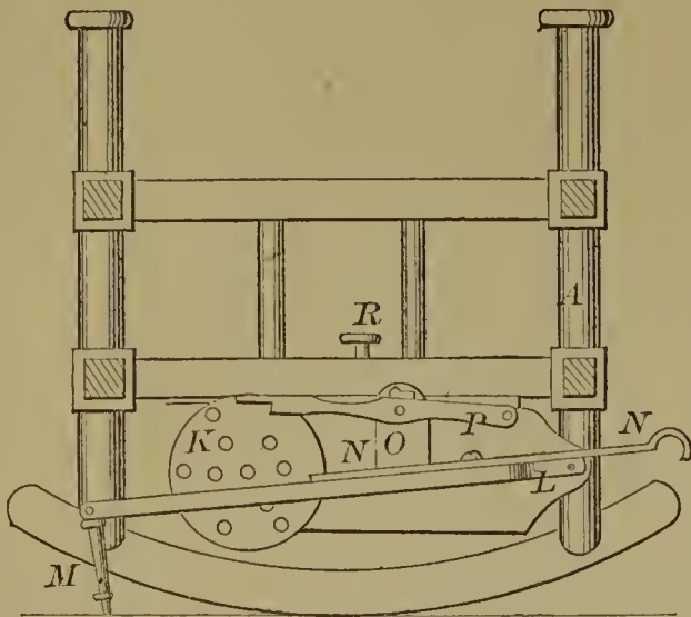
54816—G. N. Goodspeed—Feeding Mechanism for Sewing Machines.
