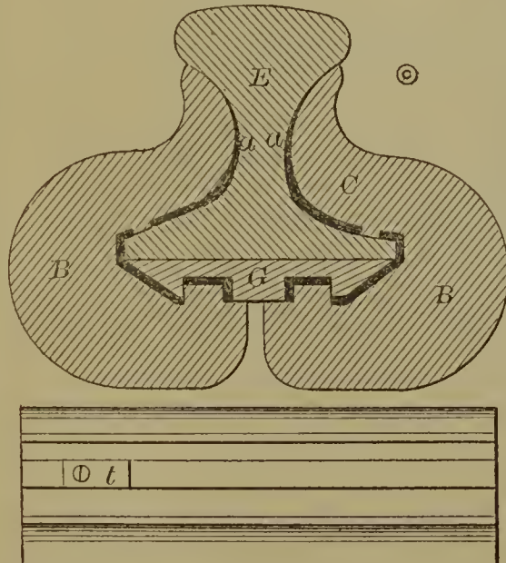
54868—D. W. Crocker—Railway Chair.
