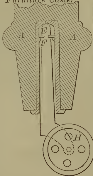
55358—J. C. Plumer—Furniture Caster.
