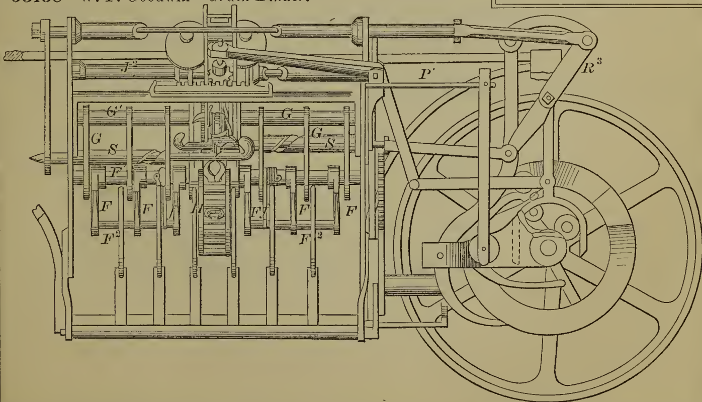
53138—W. F. Goodwin—Grain Binder.
