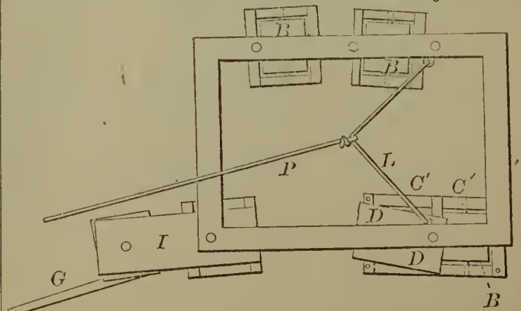
58970—E. H. Avery— For Moving Buildings.
