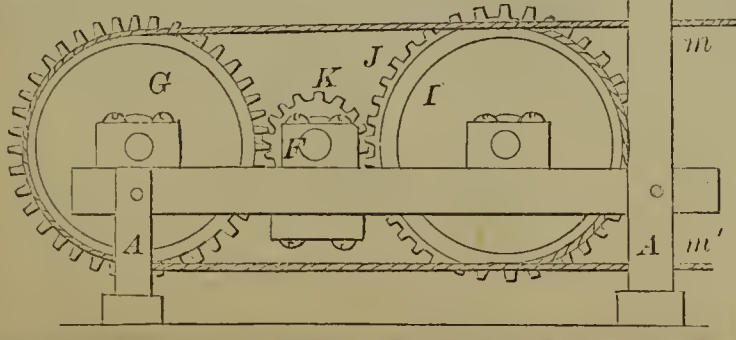
59687—S. B. Whiting— Rope Driving Machine.
