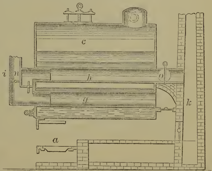
59317—A. Lapham—Petroleum Still.
