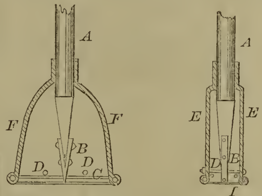
60610—P. Badore— Anvil for Swaging Culks for Horse Shoes .
