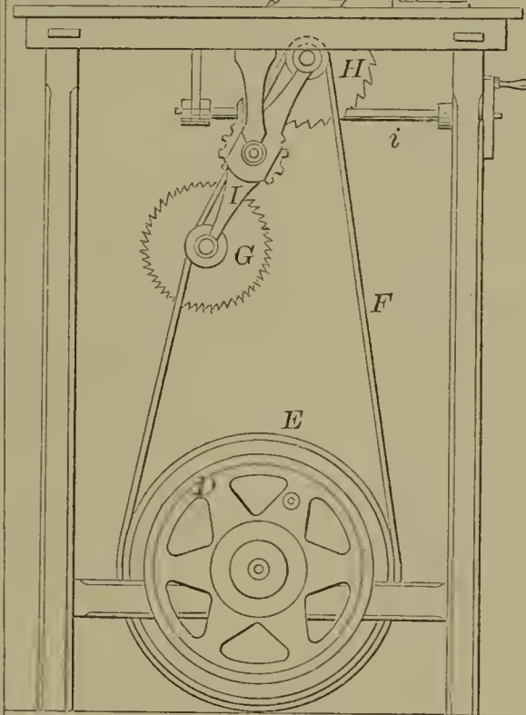
57046—S. W. Putnam— Sawing Machine. B
