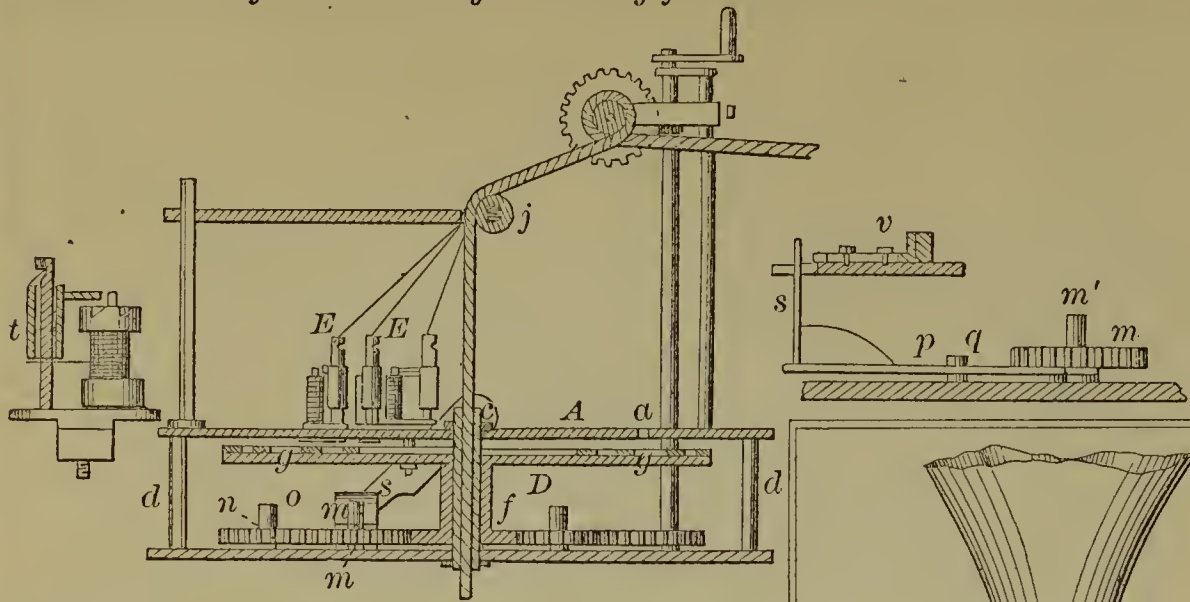
53372—J. Danby—For Weaving a Covering for Cords.
