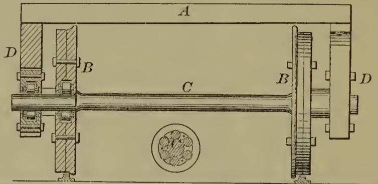
52949—D. Babson, 2d— Wheels and Axles of Railway Cars.
