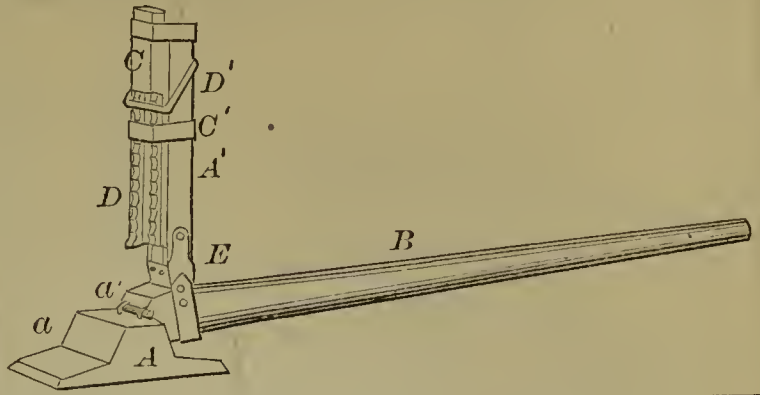
55102—A. Higley— Lifting Jack.
