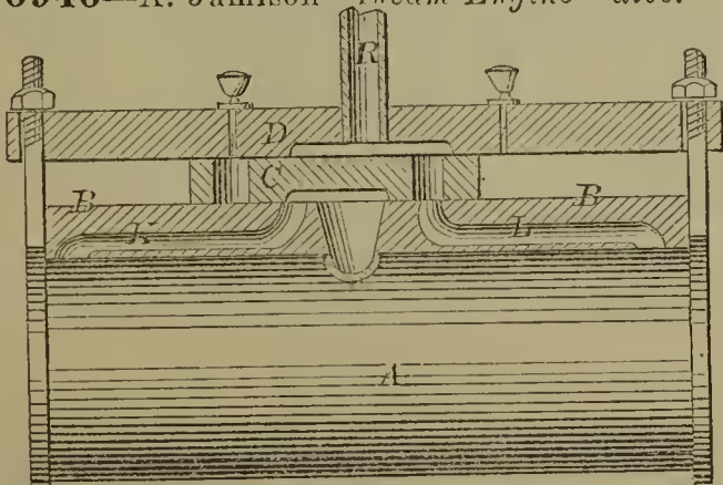
56946—A. Jamison—Steam Engine Valve.
