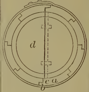
58450—J. Merrill—Cask, Barrel, &c.
