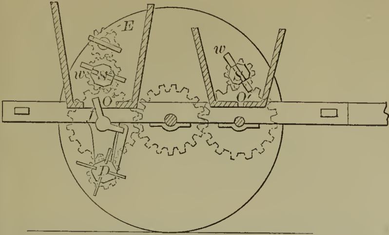
55471—E. H. Cook— Washing Machine.
