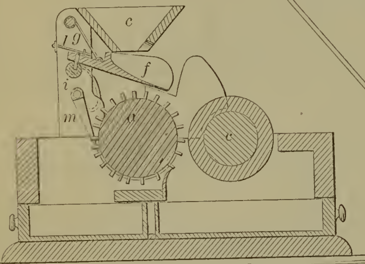
56721—J. B. Crosby—Raisin Seeder.
