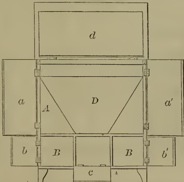
57317—R. Hagen— Ice and Coal Box.
