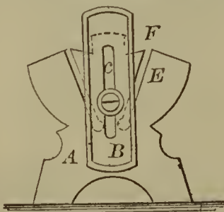
56615—J. J. Russ—Knife and Scissors Sharpener.
