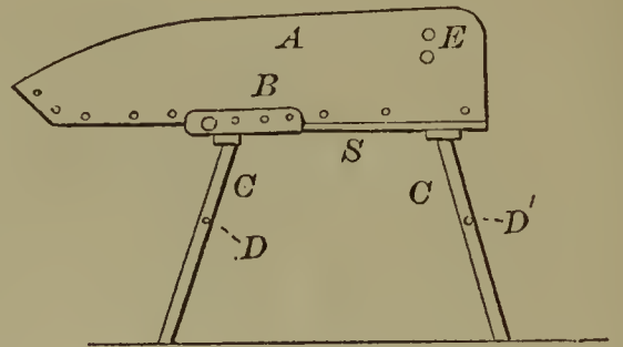
60266—J. Service—Tool Rest for Lathes.
