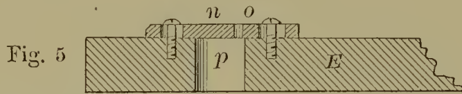
54091—J. C. Baer— Beer Faucet.
