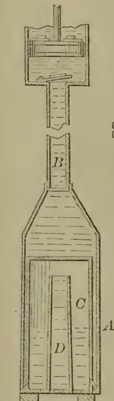
57306—D. Flagg—Water Elevator.
