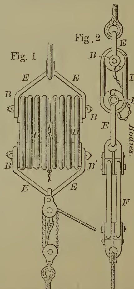
53684—T. W. Roys—For Raising Sunken Whales and other Bodies.
