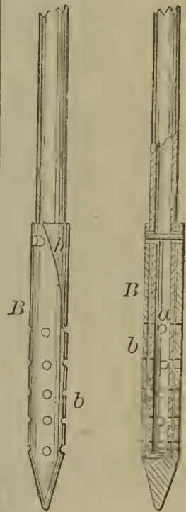
58953—R. T. Osgood—For Sinking Well Tubing.
