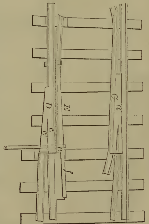
55736—W. J. Stowell— Railroad Switch.
