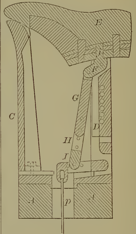
54369—G. A. Knowlton—Pegging Jack.
