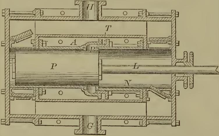
56218—R. Hartley—Pump.
