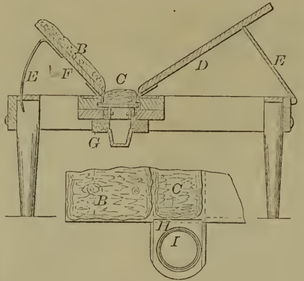
57340—M. M. Latta— Fracture Bed.
