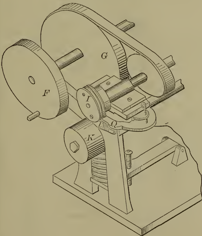
58761—J. M. Bent— Creasing or Ornamenting Leather.
