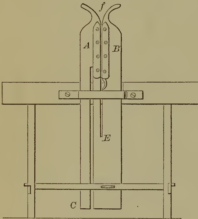
53126—K. W. Doudna—Broom Corn and Sorghum Stripper.
