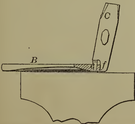
58645—C. Huie—Horse Shoe Punch.
