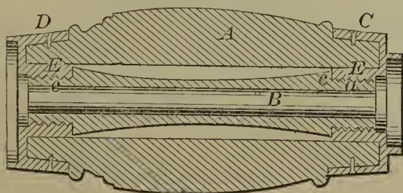
54529—W. Greenleaf— Securing Boxes in Hubs.
