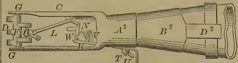
56427—J. F. Maguire—Artificial Hand.
