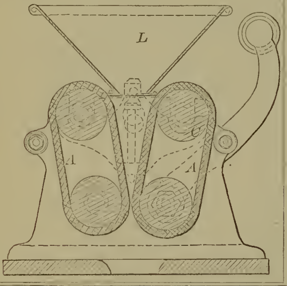
59320—J. Starkey—Curtain Eyelet.
