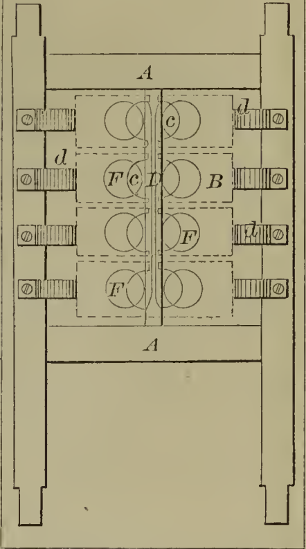
57557—D. H. Nichols—Sorghum Stripper.
