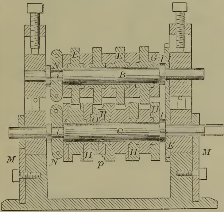
55602—H. J. Batchelder—Horse Shoe Machine.
