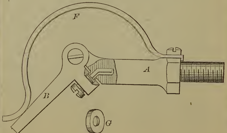
53079—J. Holderaft— Gauge Cock for Steam Boilers.
