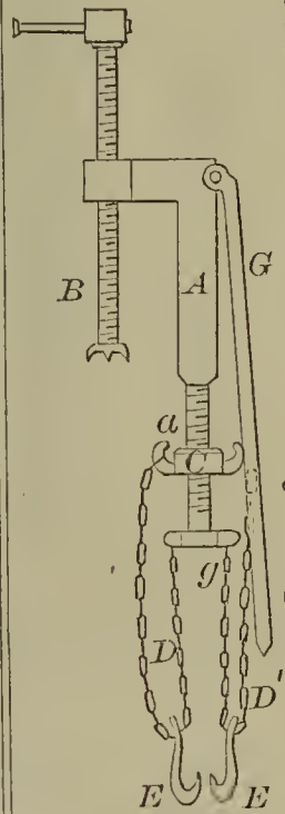
55554—J. C. Thomas—Planking Clamp.
