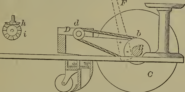
58989—Crockett & Mills— For Stripping Top Flats of Carding Engines.
