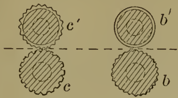
54067—J. B. Fuller—Roller for Spinning Machines.
