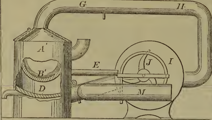
57104—Eckel & Schuyler—For Rendering Tallow, Lard, &c
