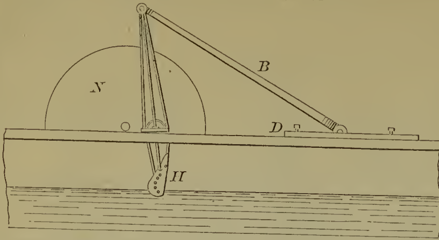
57798—M. Vergnes— Boat Propelling Apparatus.
