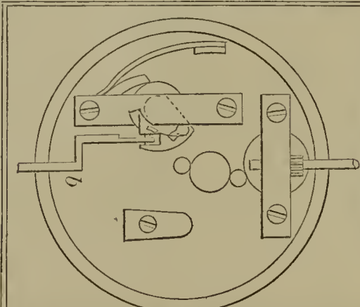
52505—F. R. Theurer— Self-Winding Watch.
