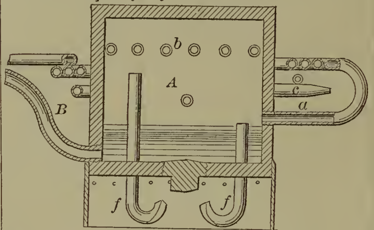
58087—H. R. Foote— Generating and Burning Vapor of Hydro Carbon Oil.
