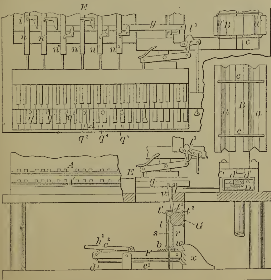
54603—W. Robjohn— Organ.
