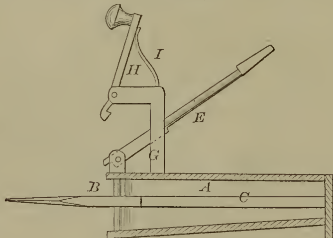
52410—J. Harris— Car Coupling.
