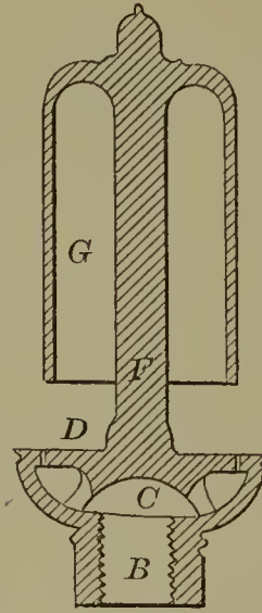
60541—J. Murray—Steam Whistle.
