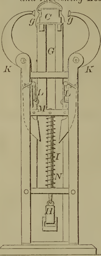
57392—E. Shaw—For Clamping and Stretching Leather.
