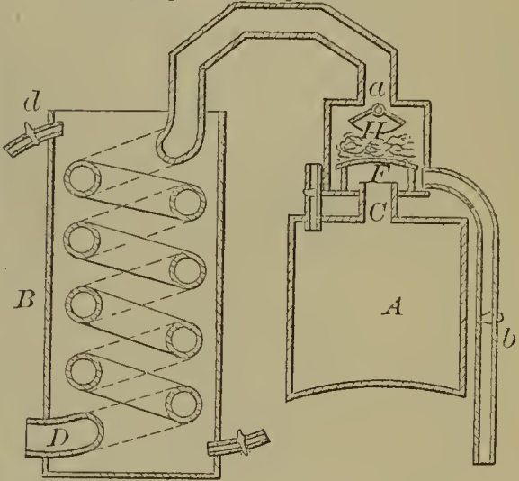
56797—Prentiss & Parsons—For Purifying Whiskey &c.
