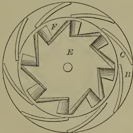
58906—F. Speck— Water Wheel.
