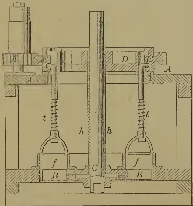
54792—C. C. Stillman—Water Wheel.
