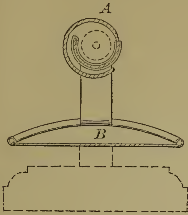
54841—J. R. Batey— Hand Protector for Sad Irons.
