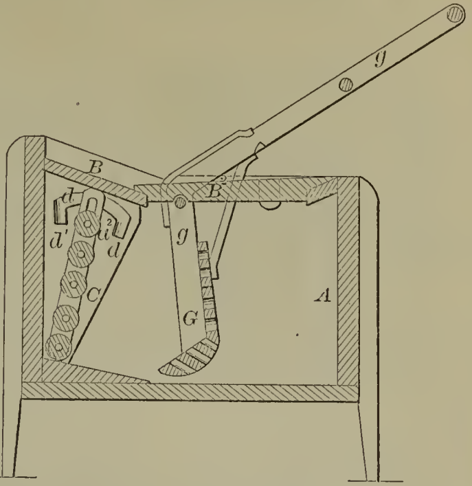
52052—H. P. Jones— Washing Machine.
