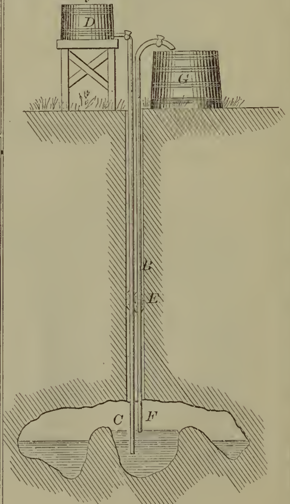
52209—O. Rotton—Obtaining Oil from Wells.
