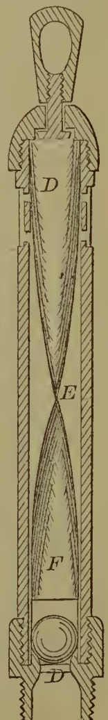
54867—R. Cornelius—Sand Pump.
