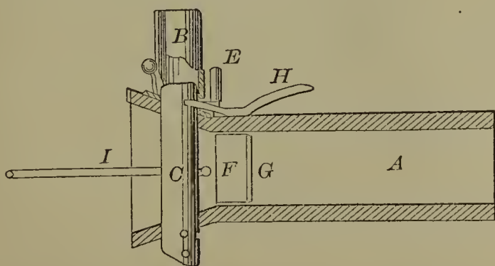
60012—J. H. Kavanagh—Car Coupling.
