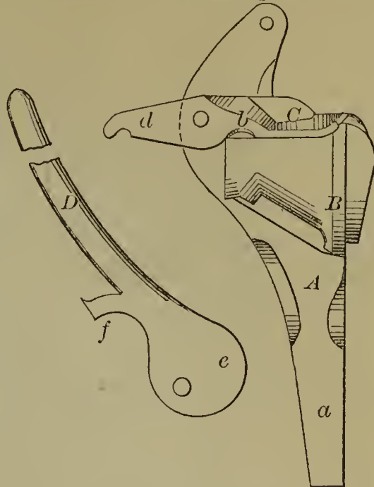
53515—S. F. Woodworth—For Swaging Sheet Metal Spouts.
