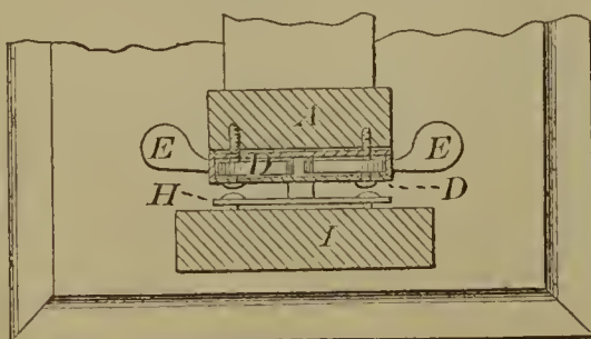
58268—R. A. Leeds— Gate Fastening.
