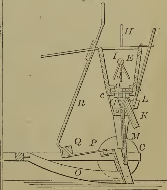
57862—C. C. Carter—Wheat Sowing Machine.
