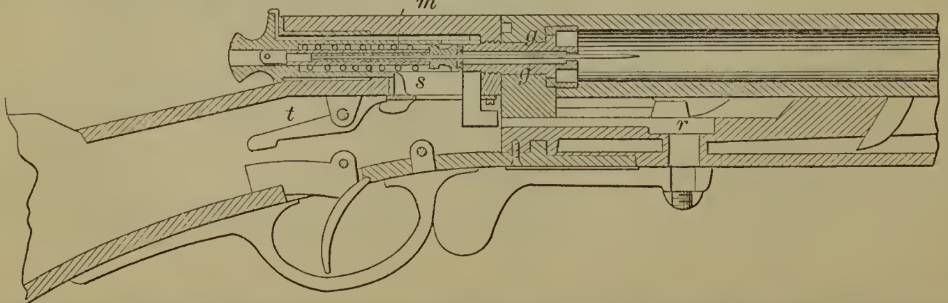
52938—J. F. C. Carle—Breech-Loading Fire Arm.
