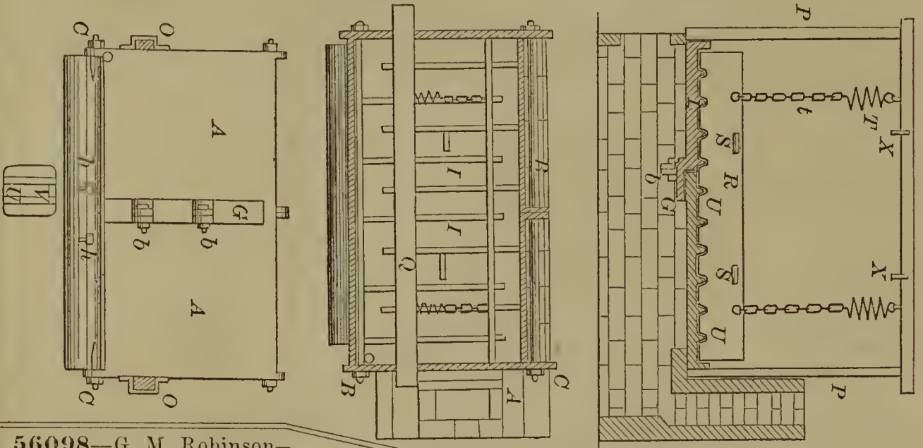
56098—G. M. Robinson—Water Box for Tuyeres.
