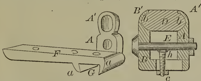
52170—J. Howarth—Coupling for Carriage Thills.
