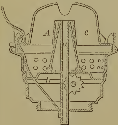
58524—S. W. Wilcox—Lamp Burner.
