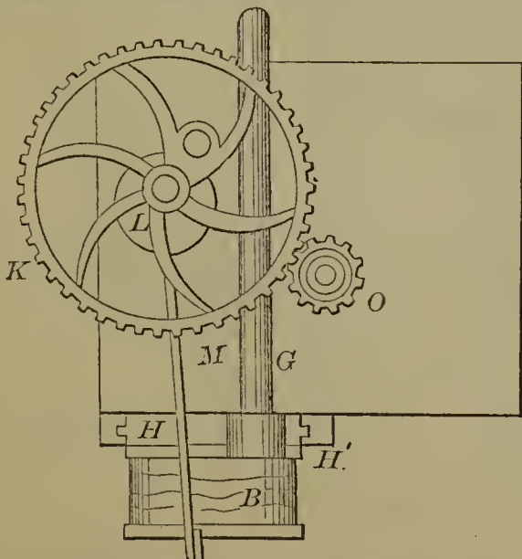
52919—A. Westcott—Churn.
