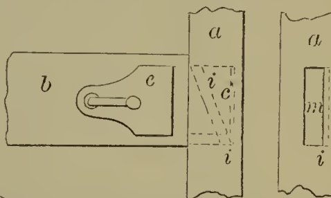
59825—W. H. Elliot—Bedstead Fastening.
