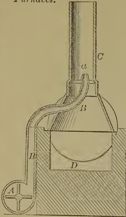
58239—C. Fisher—For Promoting Combustion in Furnaces.
