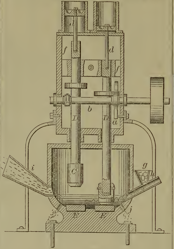
52716—D. Hughes—Quartz Crushing.
