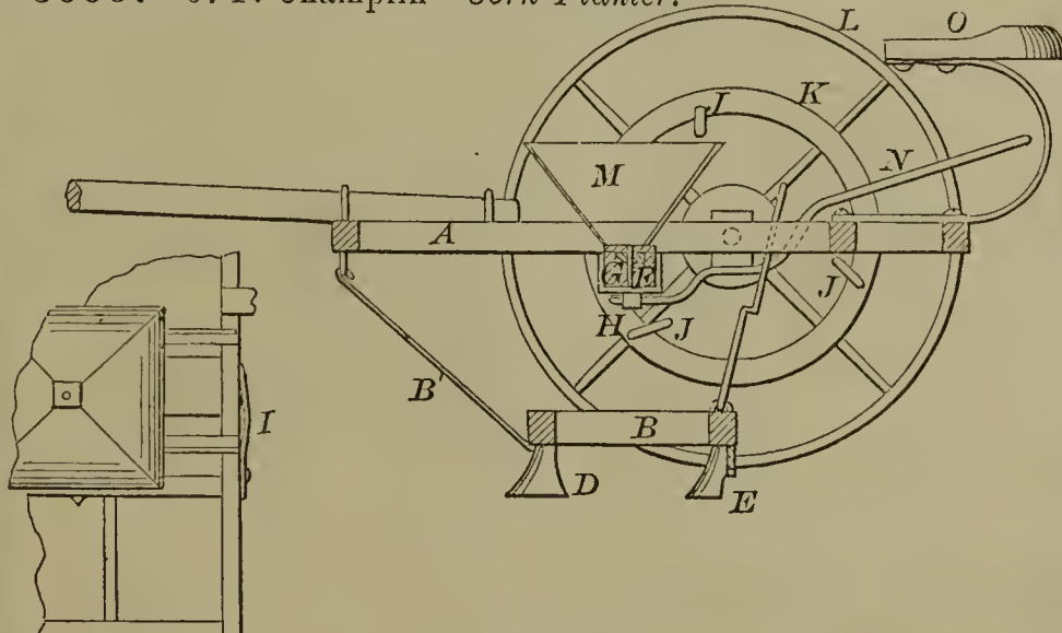
56667—J. F. Champlin—Corn Planter.
