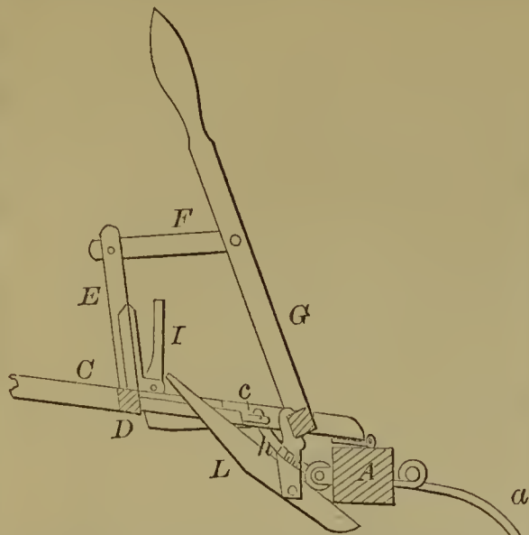
54864—S. Colahan—For Preparing Hay for Market.
