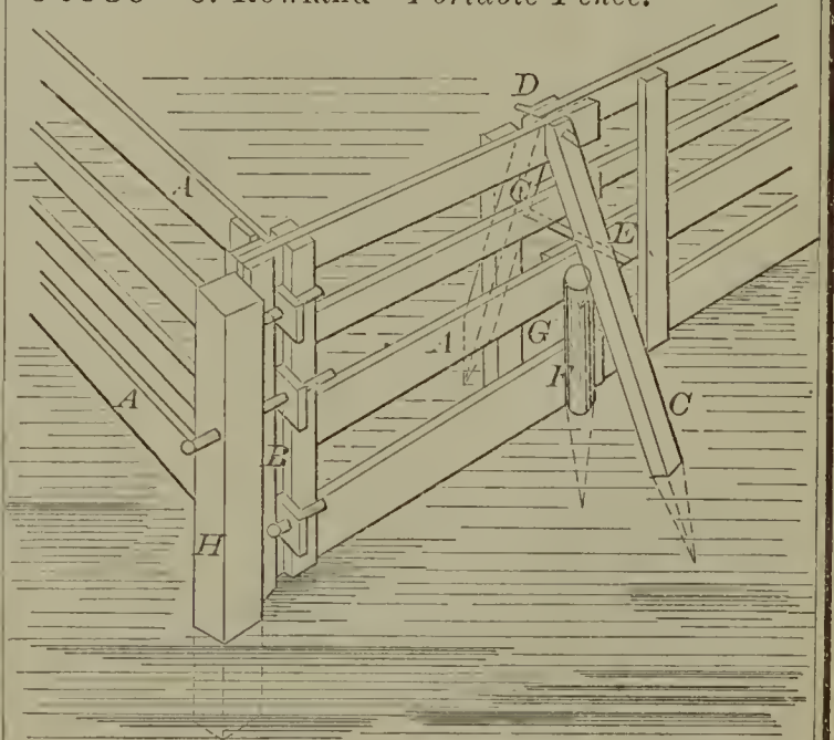
52080—C. Rowland— Portable Fence.
