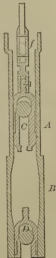
55626—J. H. Davis— Deep Well Pump.
