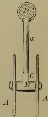
54223—J. Shepard— Meat and Vegetable Cutter.
