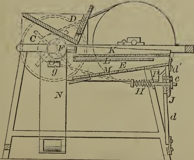
58048—B. Barney— Grain Cleaner.
