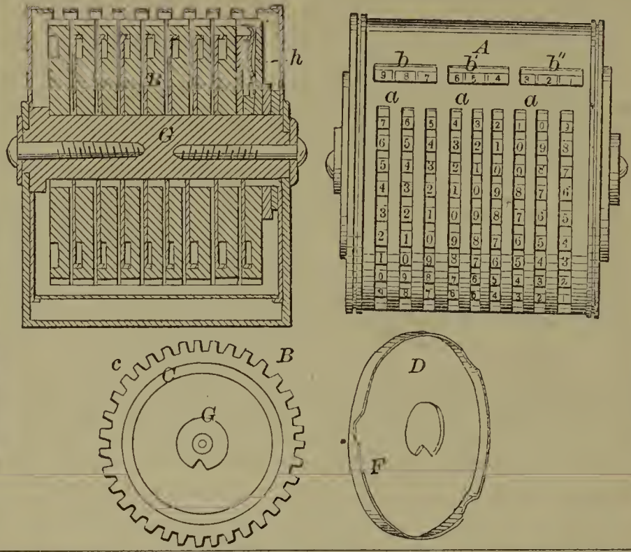
60475—J. H. Chidester—Computing Machine.
