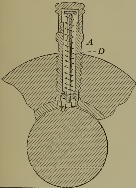
54248—N. P. Eddy— Machine Drill.
