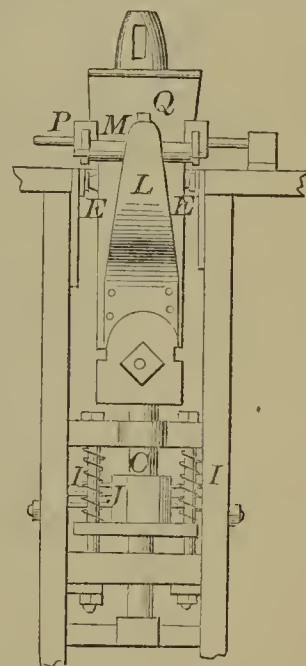
56838—W. G. Ward—Nail Hammer.
