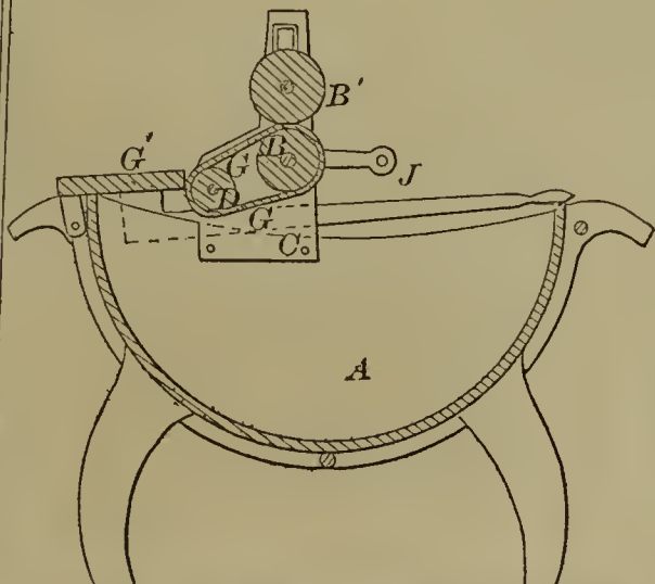
56110—W. S. Shoemaker— Washing and Wringing Machine.
