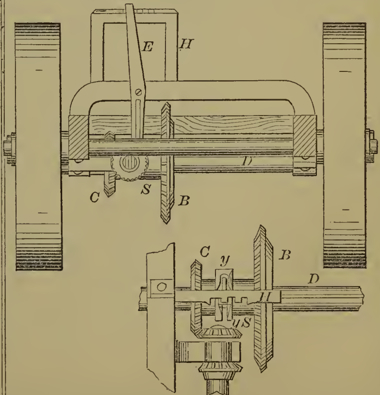
54875—M. Easterbrook—Reaping and Mowing Machine.
