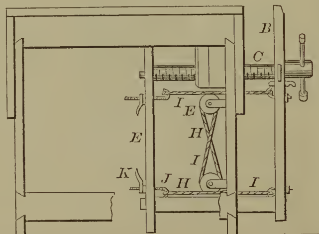
52689—W. H. Cutter—Vise for Carpenter's Bench.
