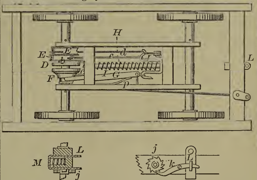
60515—A. Higley—Car Brake.
