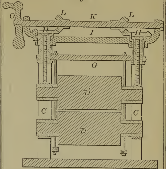
59514—F. J. Plummer—Feed Roller for Planing Machines.
