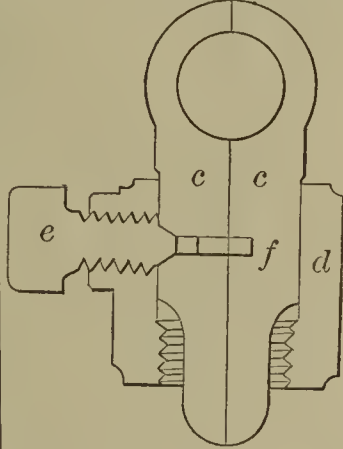
52455—T. Shaw—Connecting Rod Joint.
