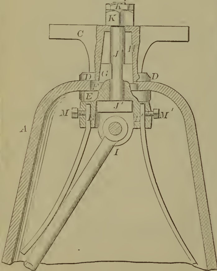
59099—E. W. Vanduzen— Mode of Hanging Bells.
