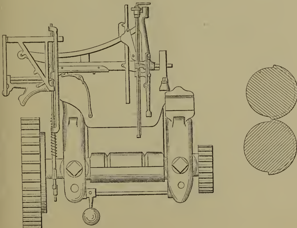
59488—H. Waters— Rolling-Die Apparatus.
