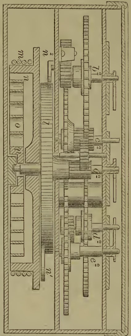
55330—Merriam & Norton—Slitting Machine.
