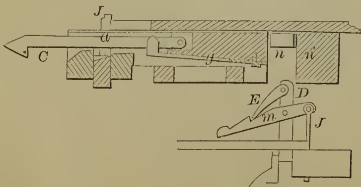
54913—M. Ingersoll—Car Coupling.
