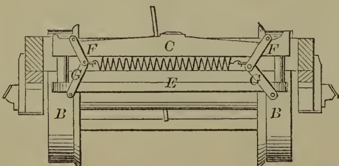
60227—D. Myers—Car Spring.
