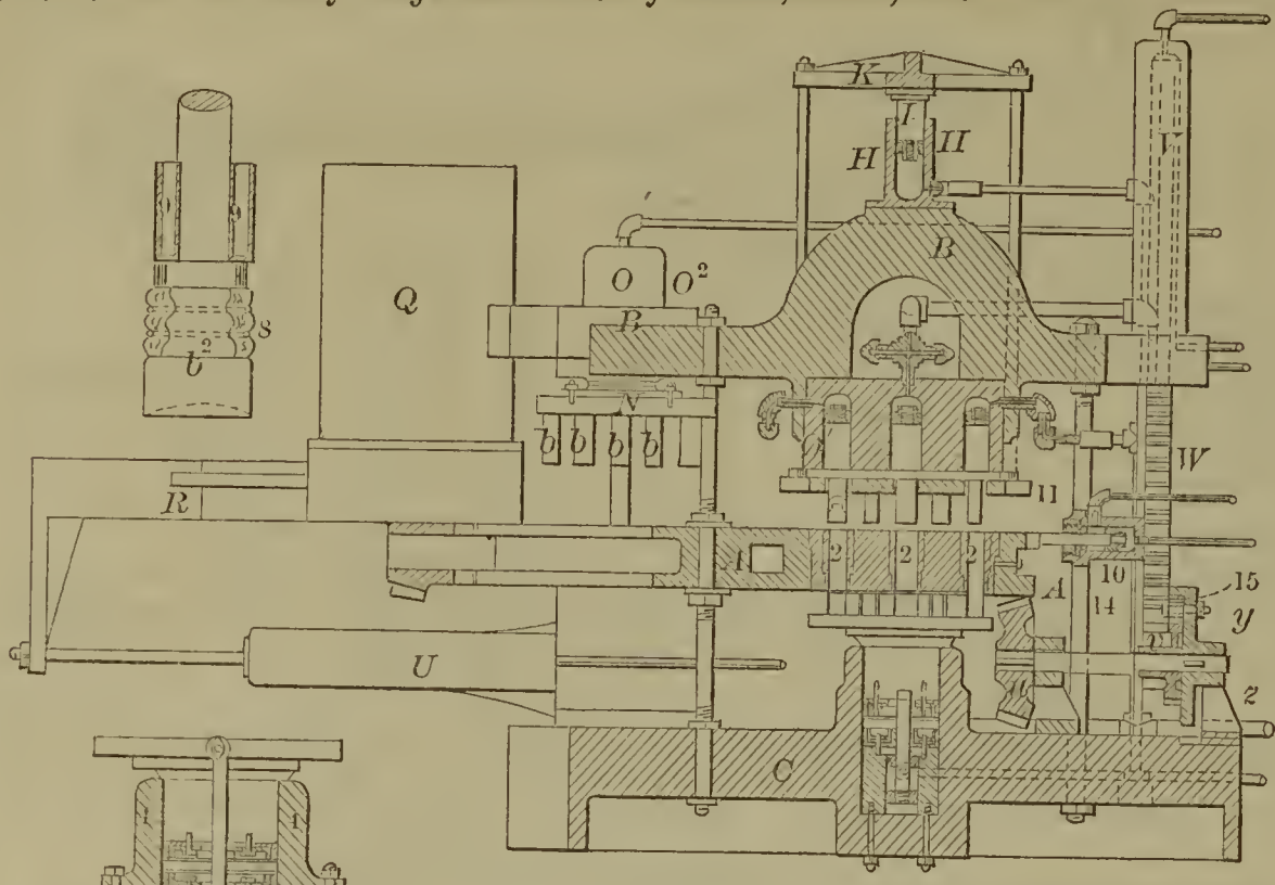
57303—A. H. Emery—Hydraulic Press for Peat, Brick, &c.
