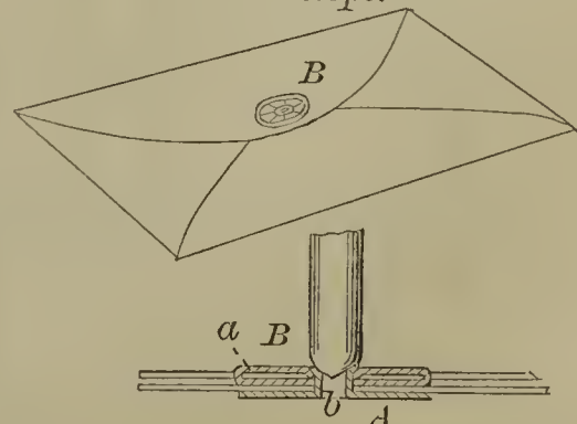
55955—R. S. Jennings— Metallic Seal Envelope.
