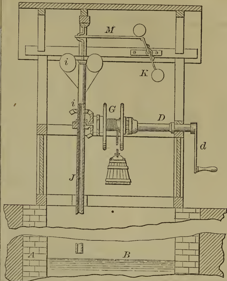
56553—G. Gullmann— Elevator for Wells.
