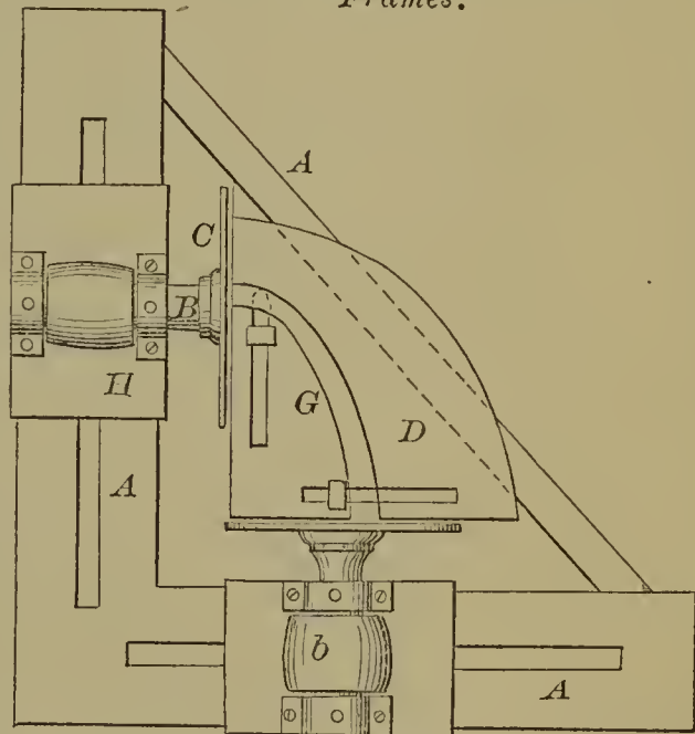
54891—J. Gelston—Churn Dasher.
