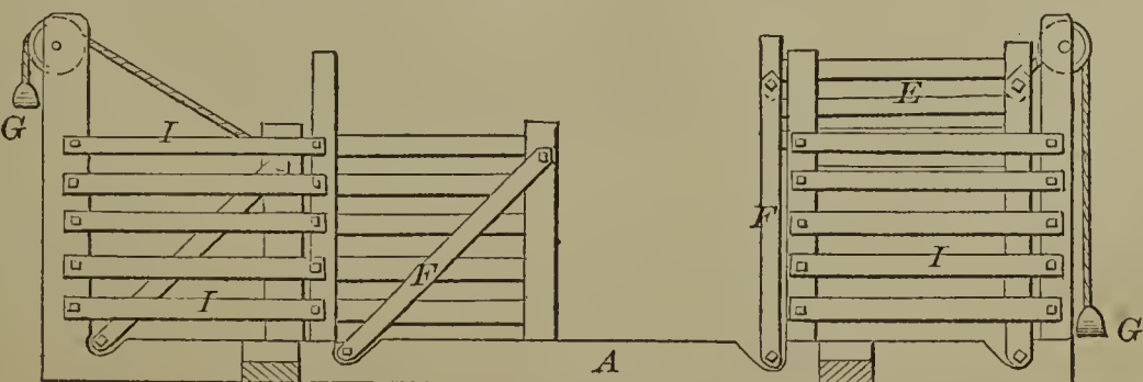
57946—H. D. Mead— Farm Gate.
