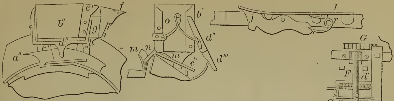
59142—E. M. Smith—Feeder for Carburetors.
