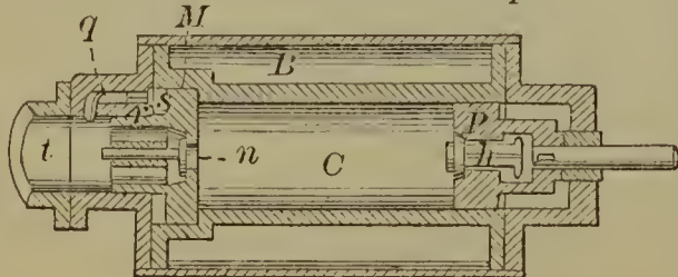
54328—H. Gottfried—Pneumatic Pump.
