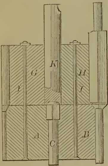
57781—J. W. Sibbet—Die for Bolt Heading Machines.
