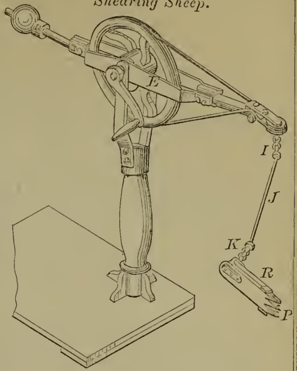
59103—Washburn & Brintnall— For Shearing Sheep.
