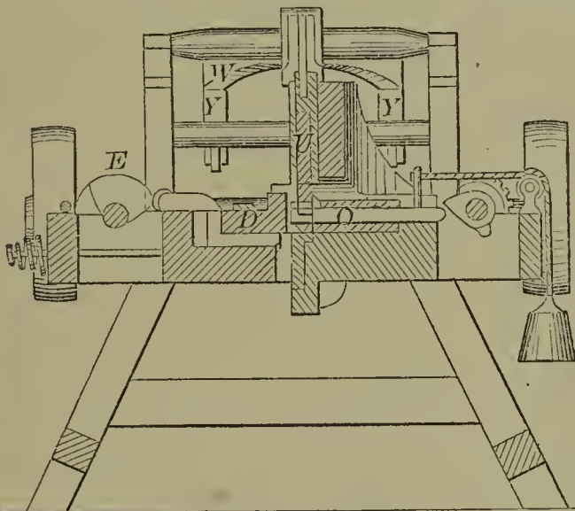
58889—C. Rosenberry— Cork Extractor.
