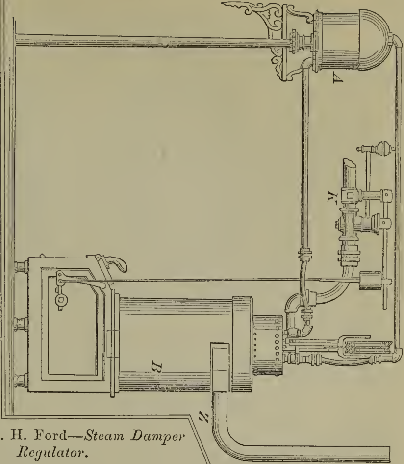
52115—C. H. Ford—Steam Generator.
