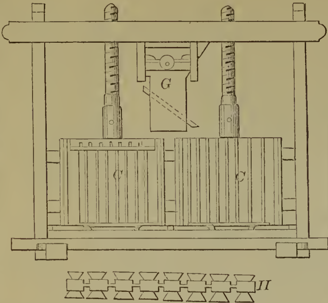
56824—M. Stevens—Cider Mill Press.
