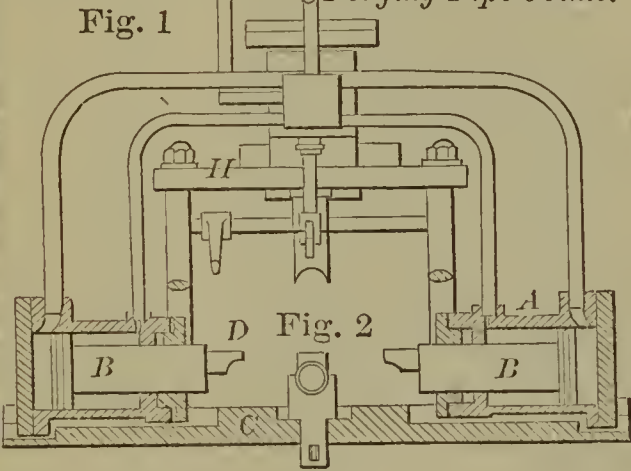
58963—Shipton & Mitchell— For Forging Pipe Joints.
