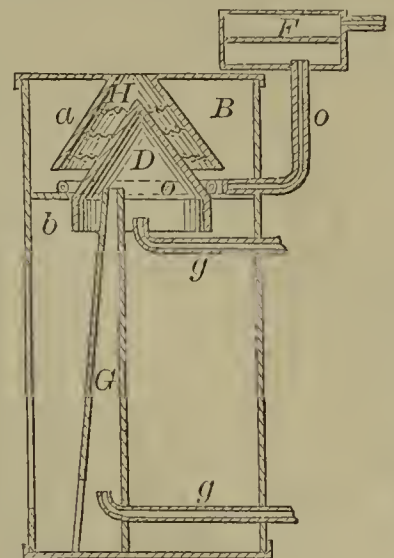
55652—D. G. Haskins— Gas Stove.
