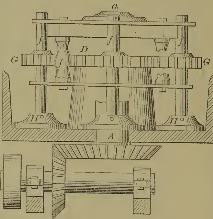
58539—I. S. Croll— Quartz Crusher.
