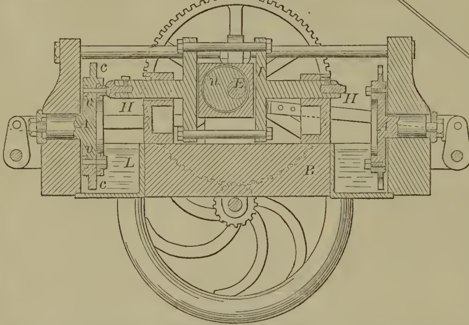
52494—L. Kirkup—Bolt-Heading Machine.
