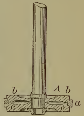
53949—C. H. Clarke—Piston Packing.
