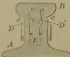
56760—R. V. Jones—Railroad Rail.
