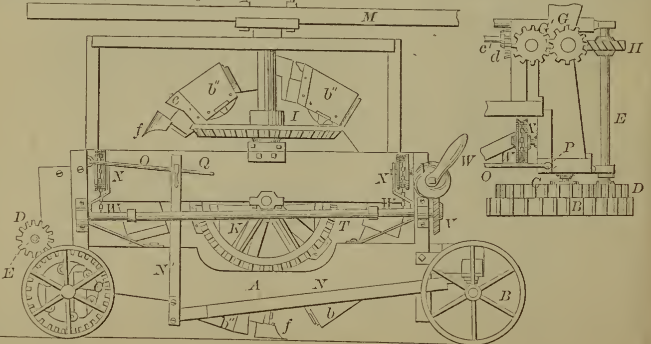
59140—D. Sawyer—Ditching Machine.
