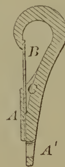
59506—Forbush & Letchworth— Snap Hook.
