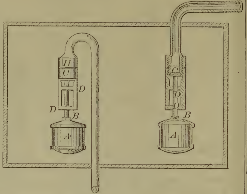
57321—E. Heald—Float Valve.
