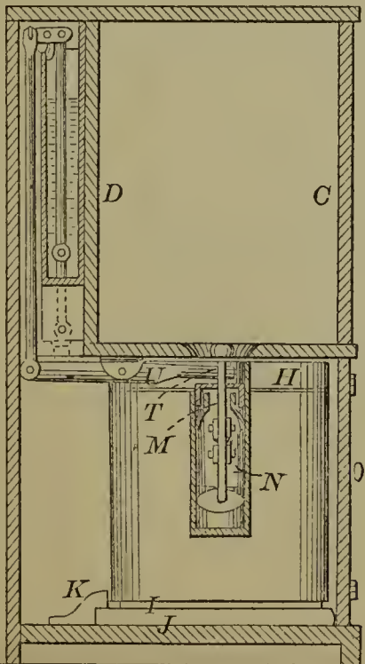
53343—E. Robinson—Portable Water Closet.
