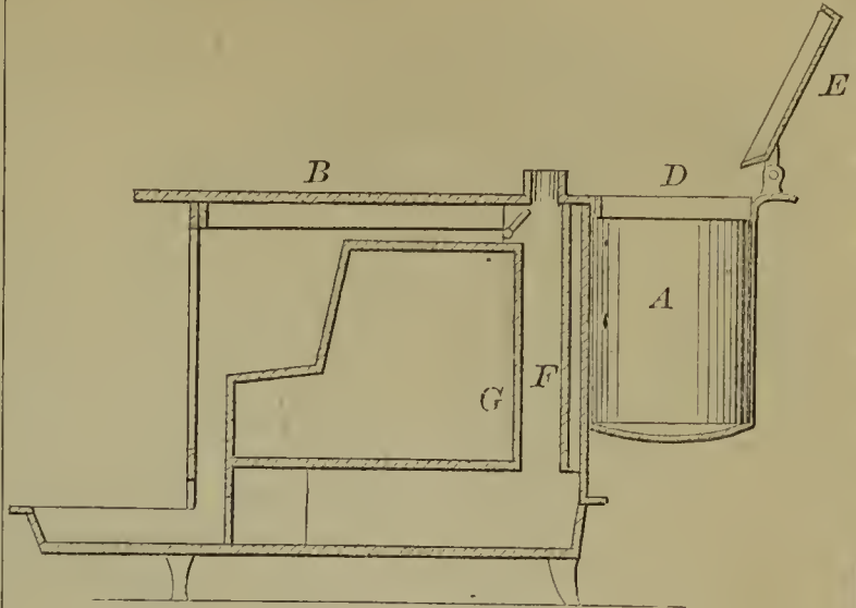
56686—E. Bussey—Cooking Stove.
