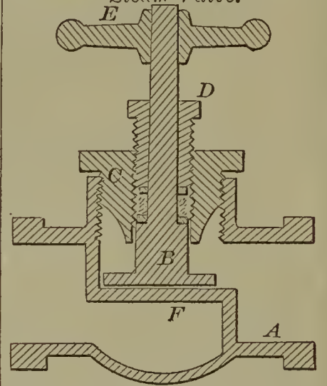
58042—J. O. Altie—Globe Steam Valve.
