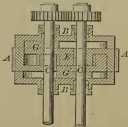
53915—H. I. Behrens—Rotary Engine.
