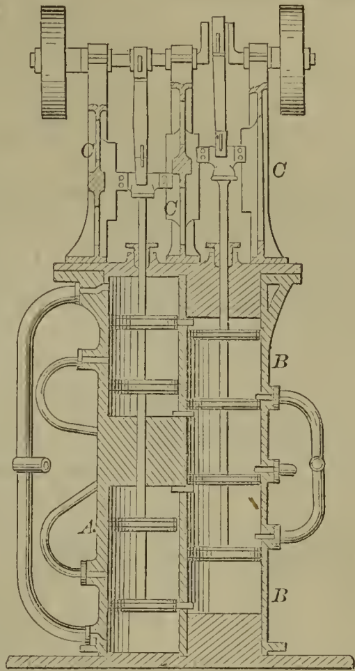
57228—G. I. Washburn—Steam Engine.
