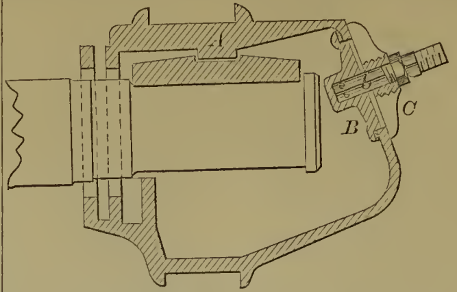
54667—D. W. Baker— Meat Chopper.
