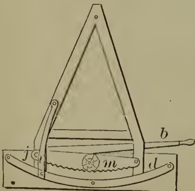
58586—N. Brockway—Sawing Machine.
