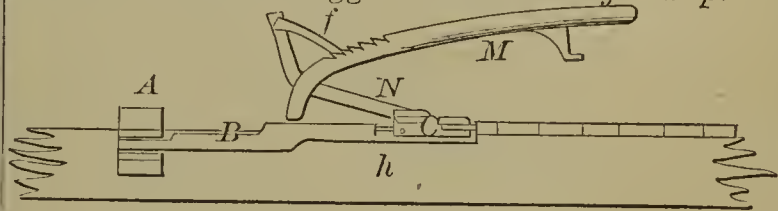
58167—H. B. Gregg—Floor Planking Clamp.
