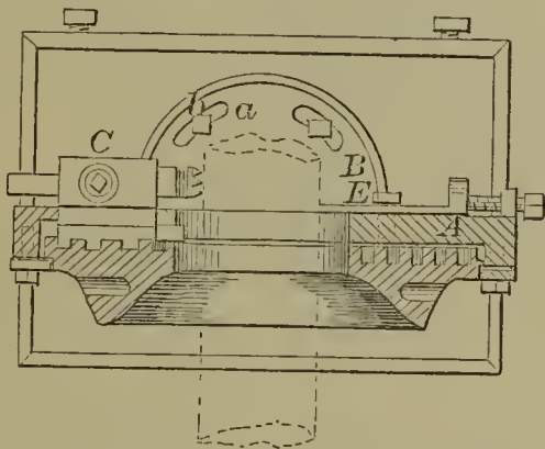
56841—A. H. Woodruff—Slide Valve.
