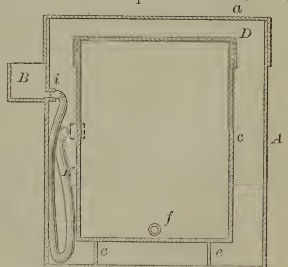
52047—E. E. Hopkins—Water Cooler.
