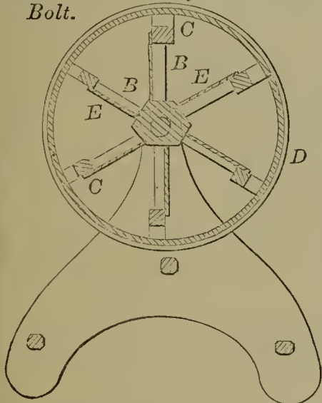
56889—W. Boynton—Tapping Barrels.
