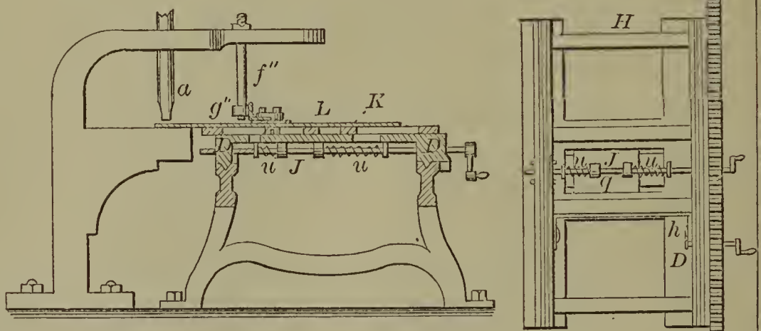
58676—Riter & Farquhar—For Punching Sheets of Metal.
