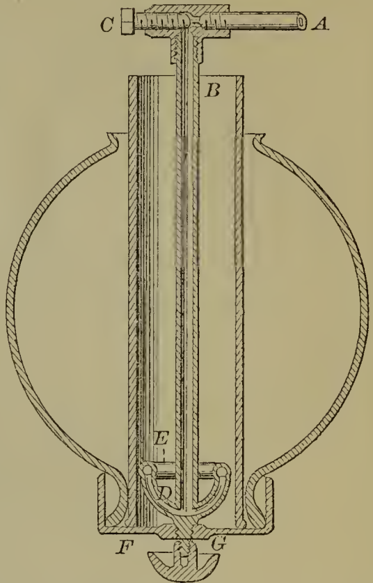
53383—J. Stratton—Hydro-Carbon Burner.
