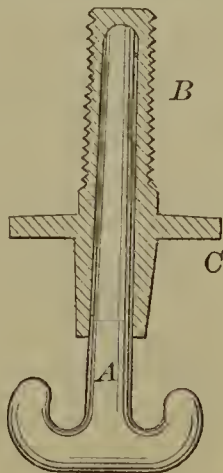
53427—A. B. Ely—Telegraph Insulator.
