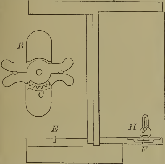
58442—Maltby & Brown— Stove Cover Lifter, &c.
