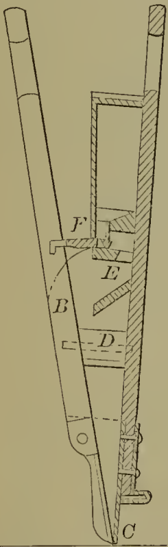
55004—C. B. Cottrell— For Tempering Steel.
