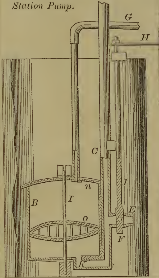
56468—Tully & Reece— Pump.
