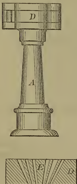
55285—W. Gurley— Water Spreading Nozzle for Fire Engines
