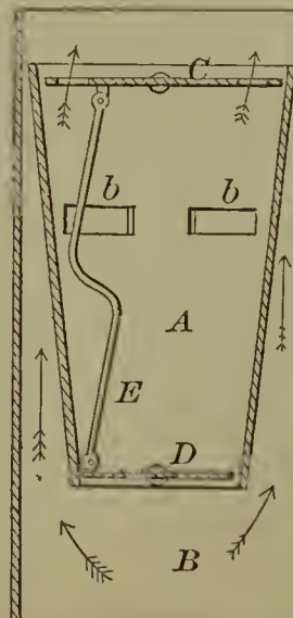
53925—S. Marvin—Stove Pipe Damper.
