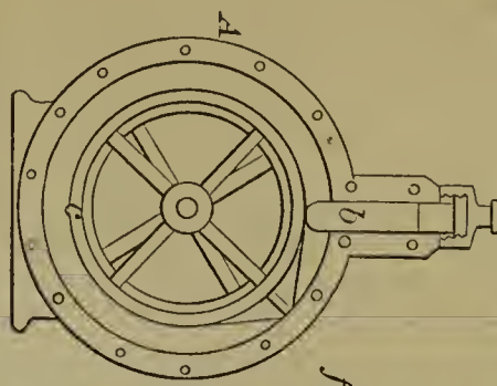
53755—R. D. Wright—Rotary Engine.
