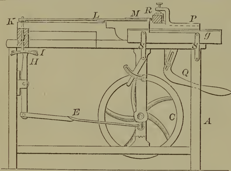
58878—W. Nangel—Morising Machine.
