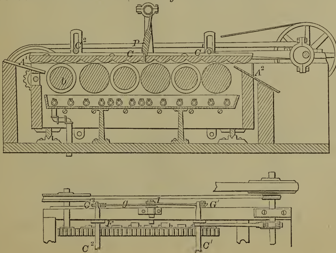
59758—J. W. Blackham—For Felting Hat Bodies.
