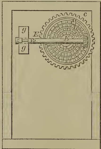
52334—H. Smith—Mechanical Movement.
