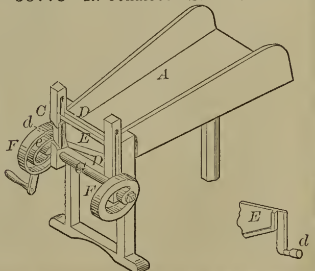
58778—R. Conarroe—Straw Cutter.
