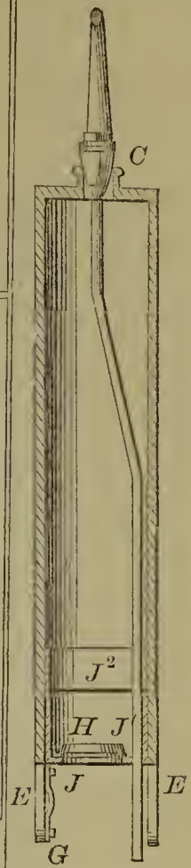
54738—C. Kane—Die for Heading Bolts.
