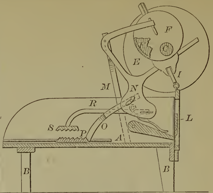
58968—W. R. Andrews— For Operating the Harness of Looms.
