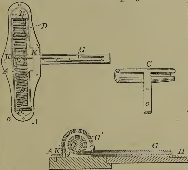
60484—Currier & Wells—For Finishing and Boxing Paper Collars.
