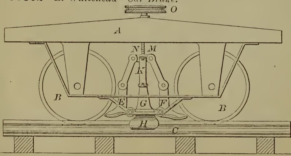
56302—E. Whitehead—Car Brake.
