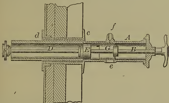
54282—E. Bigelow—Measuring Faucet.
