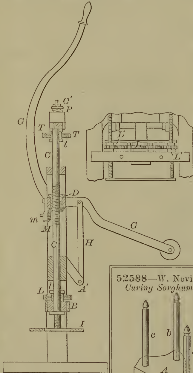
52584—G. Matthewman—Press.
