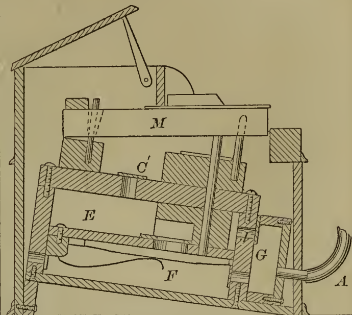
56106—G. E. Shaw— Carbon Oil Fire Tester.
