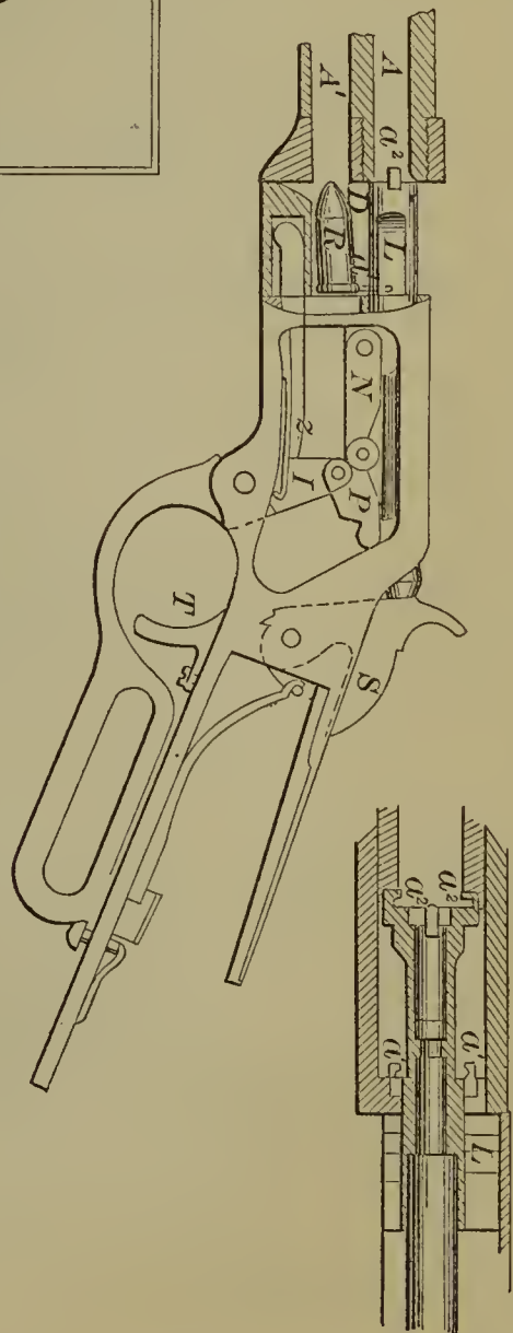
52933—J. D. Smith—Magazine Fire Arm.
