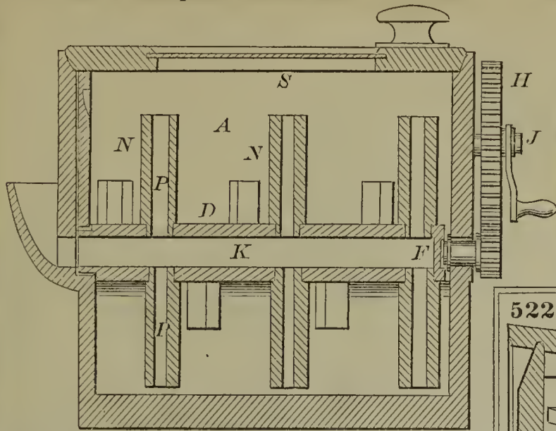
52270—J. E. Crane—Screen for Wool Dryer.
