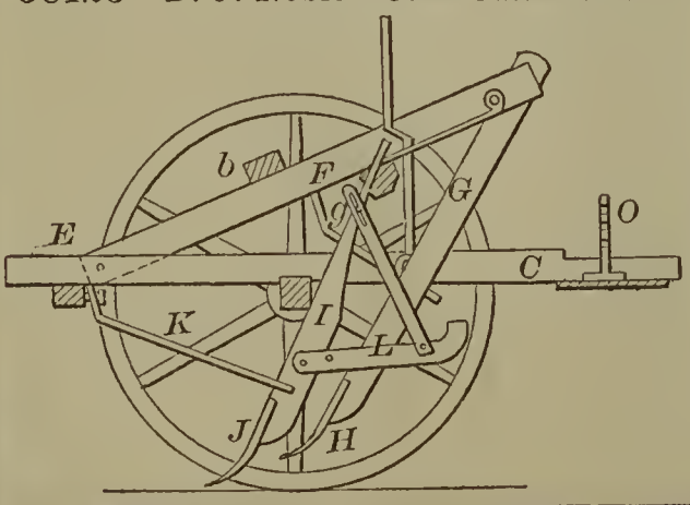
58125—D. J. Noble—Corn Cultivator.
