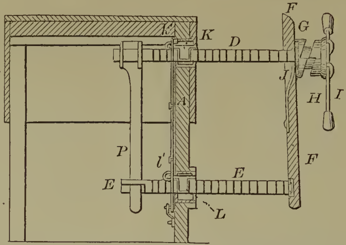
58858—R. McConnell— Carpenters' Bench.
