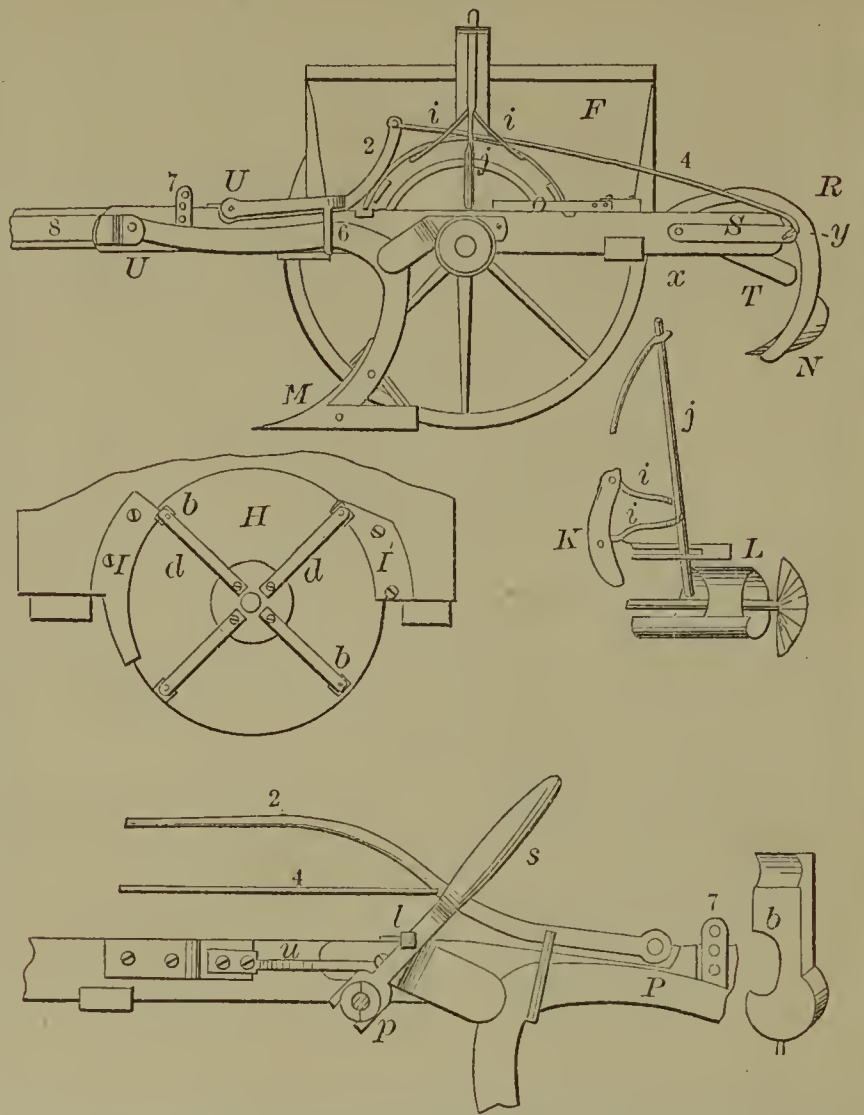
60172—C. Glidden—Plow.
