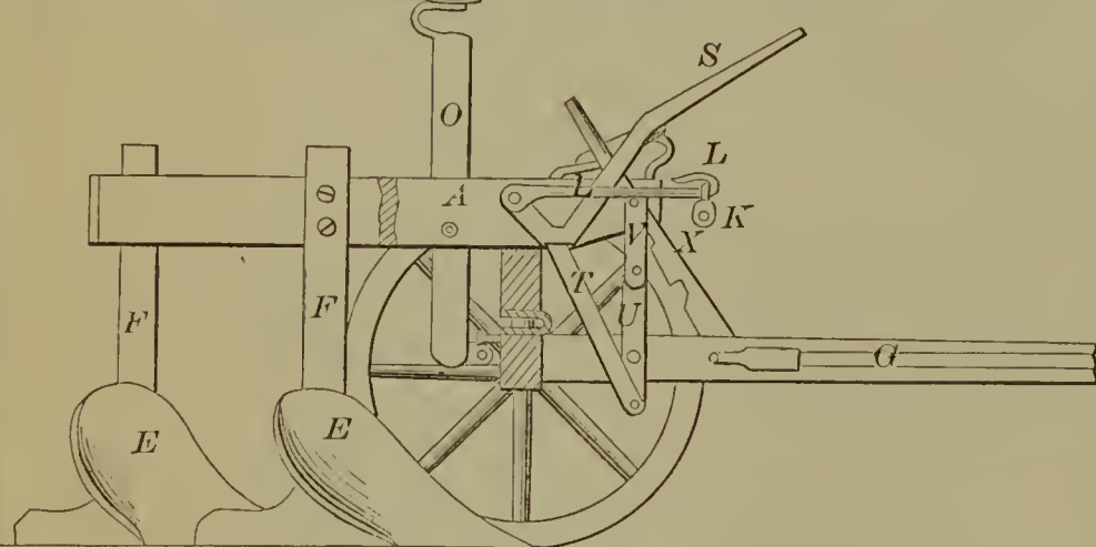
54963—Runk, Brown & Morgan—Gang Plow.
