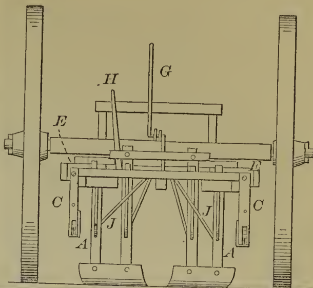
54316—J. Fishbaugh— Wood Bending Machine.
