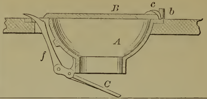
59282—Z. B. Shannon— Churn.
