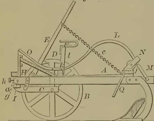
56878—W. Battell—Gang Plow.
