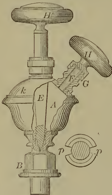
58767—J. Broughton— Steam Engine Lubricator.
