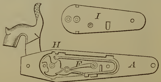
54021—Rudolph & Braun—Gun Lock.
