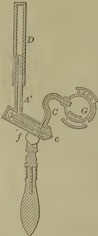
52459—H. B. Stiles— Water Motor.
