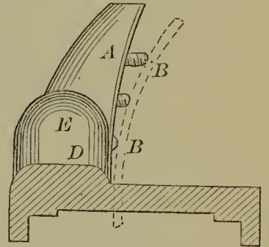
55238—A. Casebeer—For Jointing Staves.
