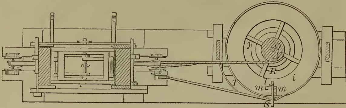
56589—J. McKnight— Harvester Cutter Sharpener.
