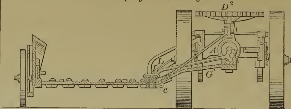
56893—R. Brown—Reaping and Mowing Machine.
