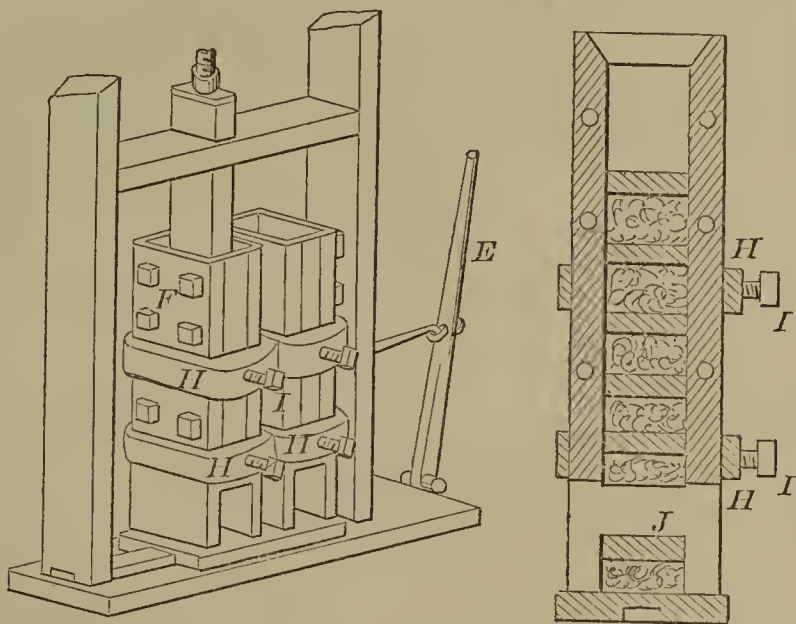
55759—J. W. Barber—Tobacco Press.
