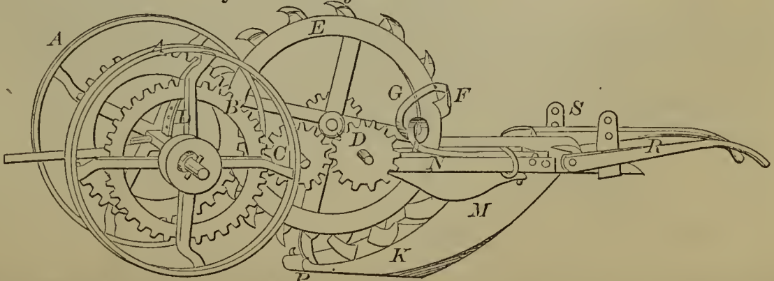
53264—J. C. Boyd—Ditching Machine.
