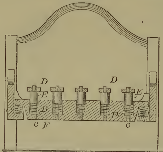
52585—J. B. McClanathan—Spring Bedstead.
