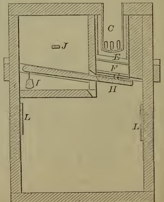
53164—C. Melone—Animal Trap.
