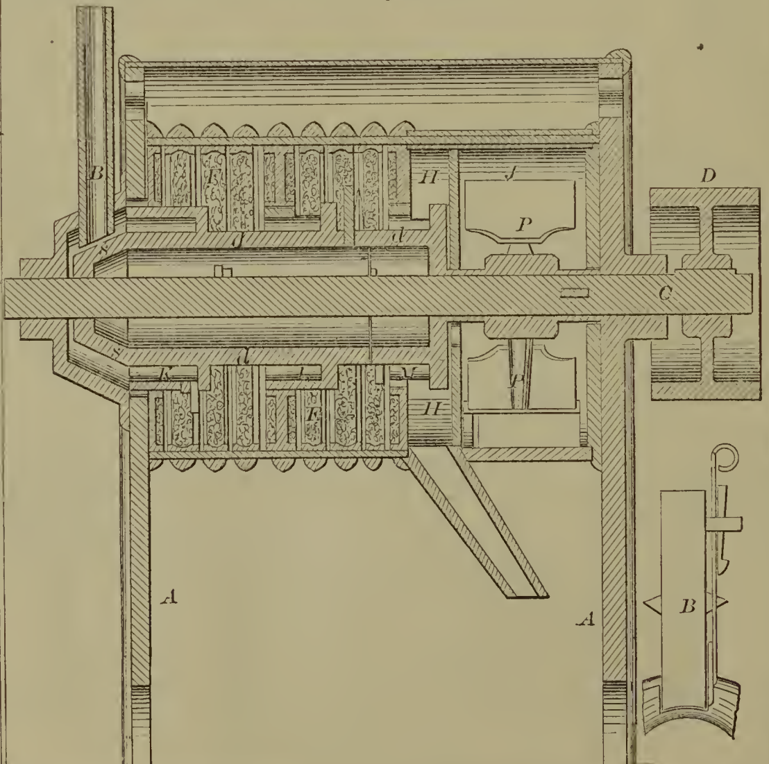
57605—J. A. Welsh—Grain Hulling Machine.
