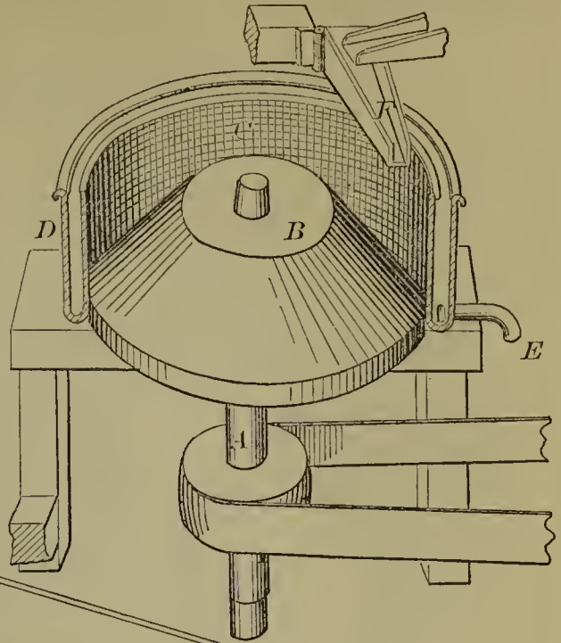
53448—H. Hunt—Centrifugal Machine.
