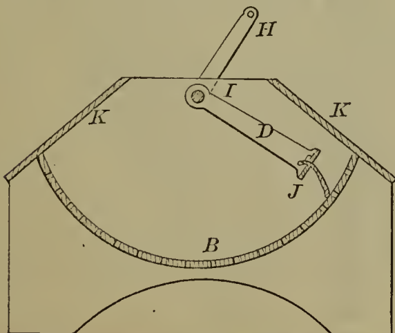
53644—W. C. McGill—Flour Sifter.
