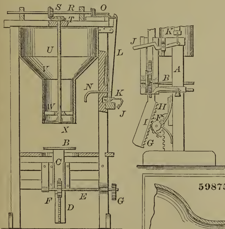
59872—L. W. Feeter—Flour Packer.
