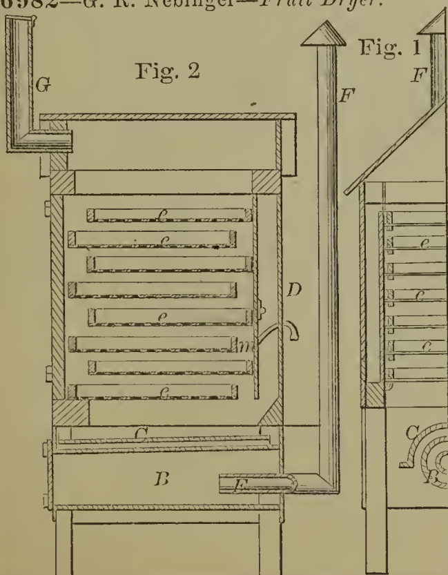
56982—G. R. Nebinger— Fruit Dryer.
