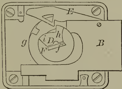
51973—Sargent & Covert—Lock.
