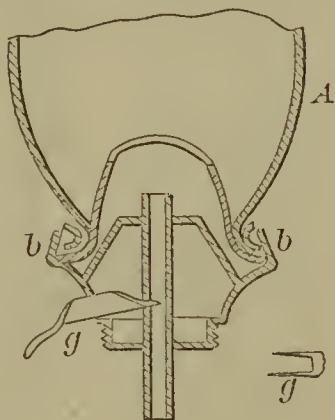
56250—Mund & Hoffman—Lamp Wick Regulator.
