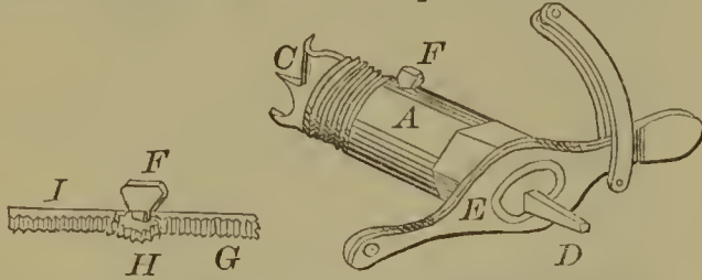
59427—C. C. Mather— Fence.
