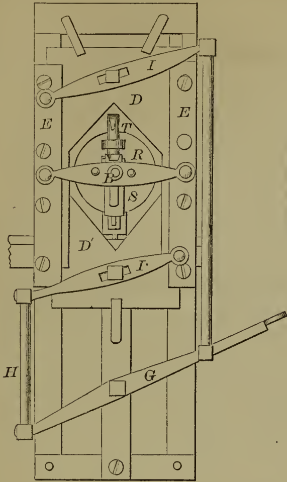
54750—L. Mason—For Boring Wagon Hubs.
