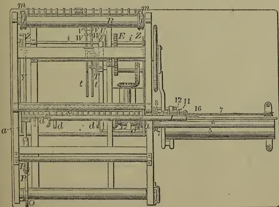
57898—G. Hasecoeter—Loom for Weaving Slatted Window Shades.
