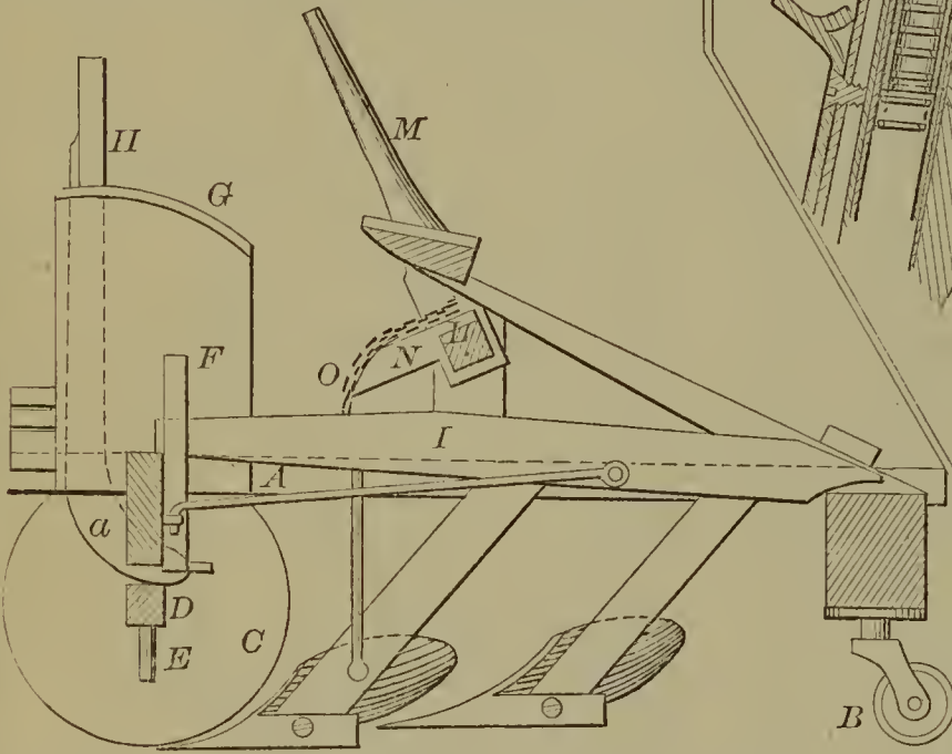
56942—S. Hutchinson—Gang Plow.
