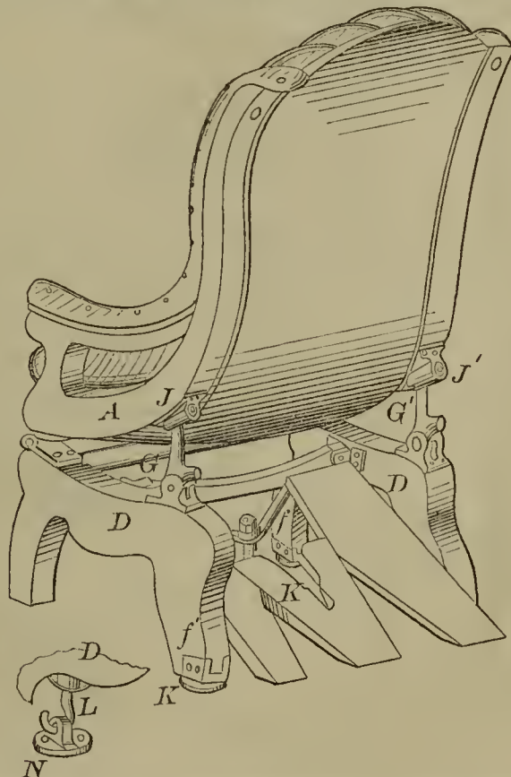
57351—M. M. & F. Martin— Railroad Car Seat.
