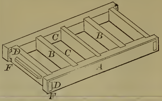
53192—C. F. Smith— Butter Worker.
