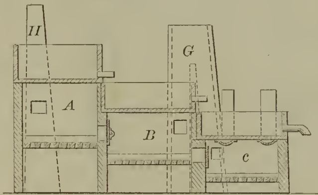
51828—F. M. Harris—Evaporator.
