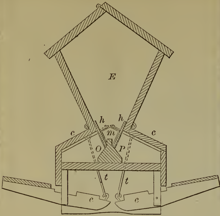
54285—G. W. Boynton— Sheep Rack.
