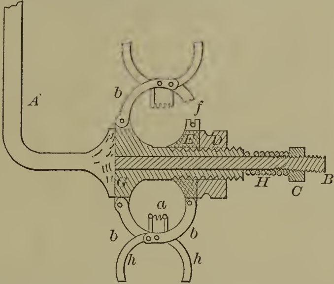
52720—E. F. Light—Journal Box.
