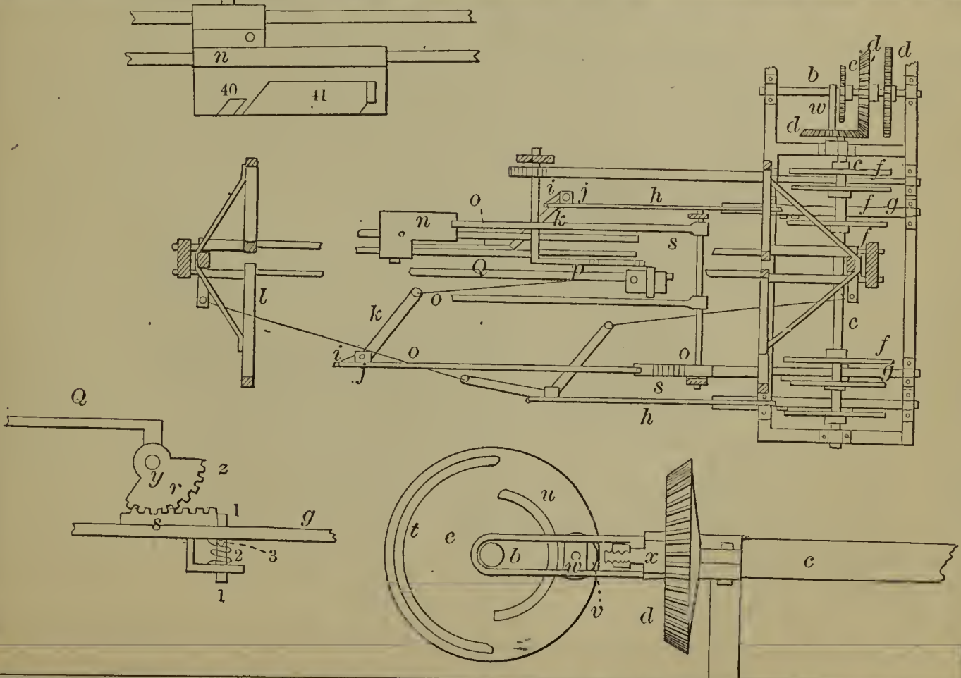
54177—I. Lancaster—Grain Binder.
