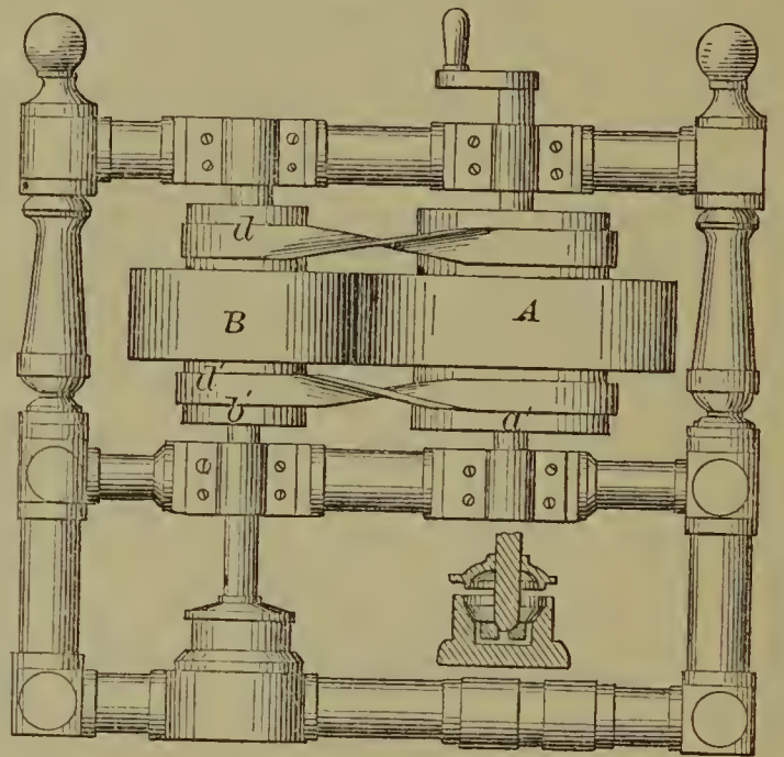
53717—J. D. Whelpley— Friction Gearing.
