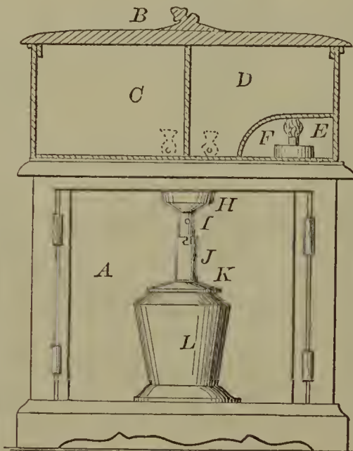
60362—S. B. Guernsey—Wash Stand.
