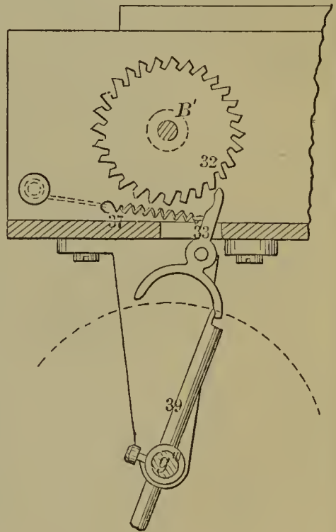
55056—E. A. Calahan— For Punching Paper for Telegraph.
