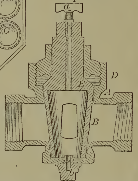
58845—B. E. Lehman— Stop Cock.
