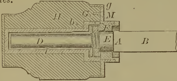
59445—I. Osgood—For Securing Wheel Hubs to Axles.
