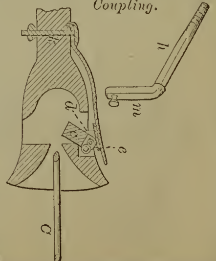
57767—J. H. Reed— Car Coupling.
