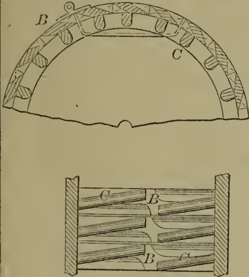
570775—B. Bisbee— Washing Machine.
