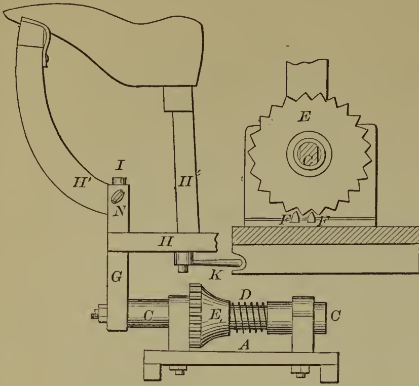
54691—L. L. Coon— Shoemaker's Jack.
