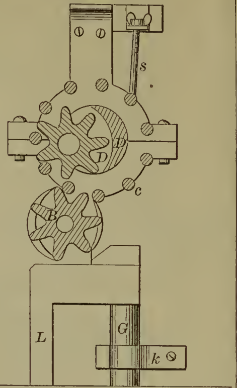
56676—Pease & Lewis— Clothes Wringer.
