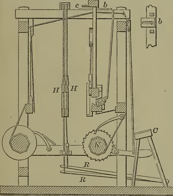
60305—J. Whitehead—Hand Loom.
