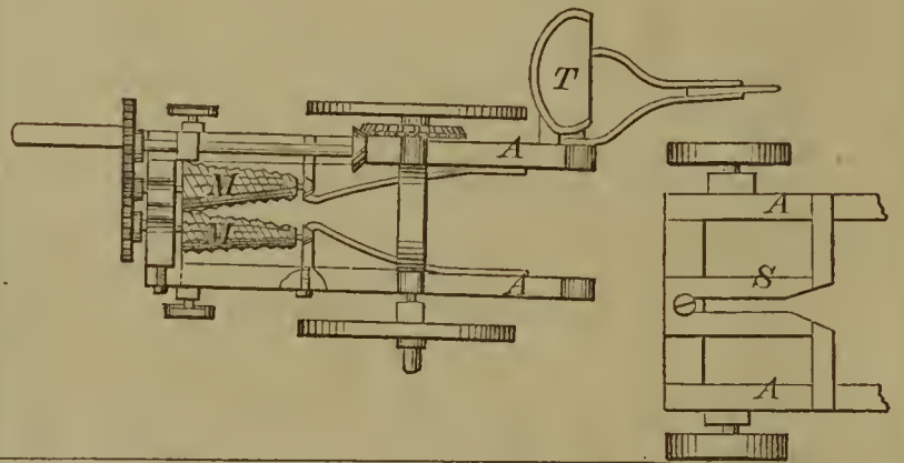
56510—M. Andriot—Carriage Jack.
