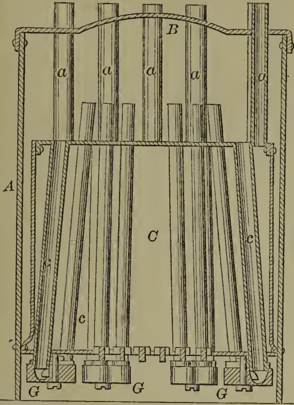
60500—J. Frot— Engine for the Utilization of Ammonical Gas.
