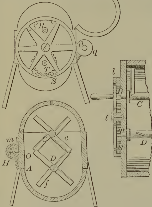
52075—J. Rankin— Churn.
