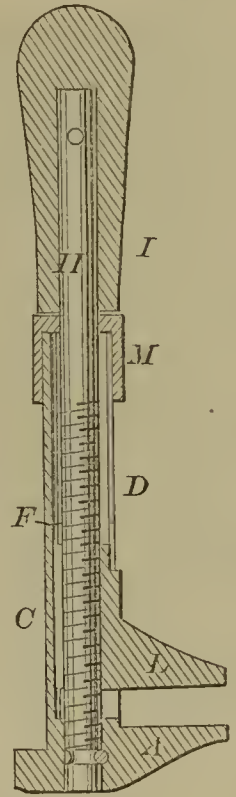
52487—J. C. Conner— Wrench.
