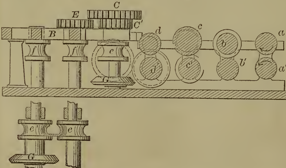
56152—P. L. Weimer—Metal Tube Machine.
