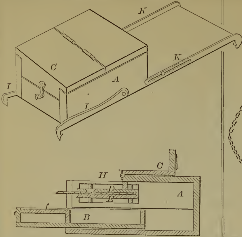
57866—Church & Knight— Petroleum Tank.
