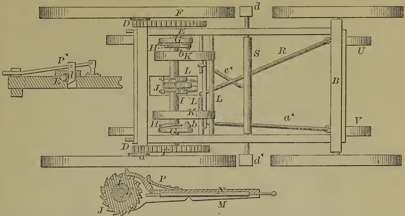
53575—G. Clarke—Grain Dryer.
