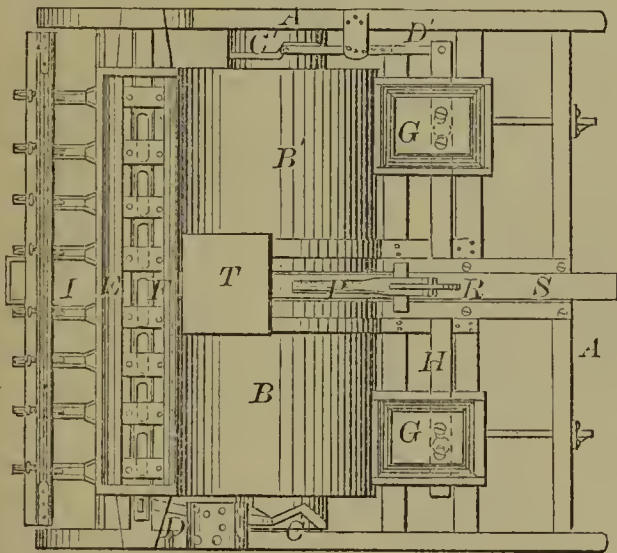
57842—A. Armstrong—Wheat Drill.
