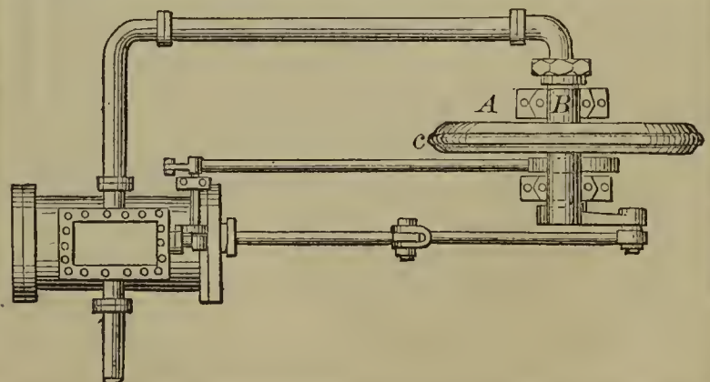
54428—J. F. Spence— Revolving Condenser.
