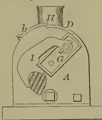
57197—J. Segondy—Sausage Meat Cutter.
