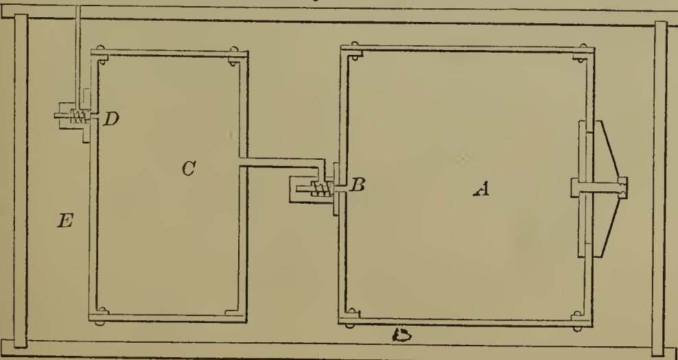
55039—J. S. Baldwin—Storing Carbonic Acid Gas.
