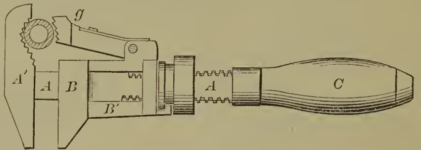
59852—J. McLaren—Wrench.
