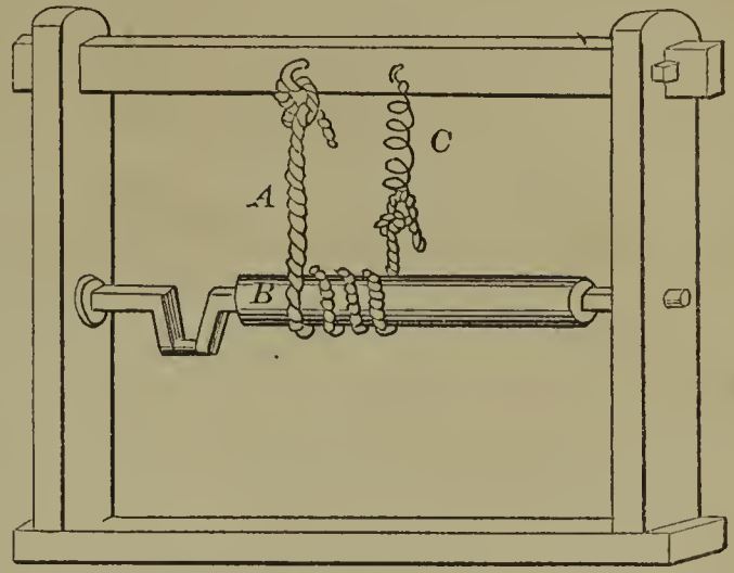
60509—J. Hanley—Spiral Friction Clutch.
