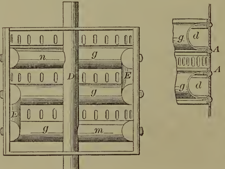
60490—E. Detwiler—Radiator for Stove Pipes.
