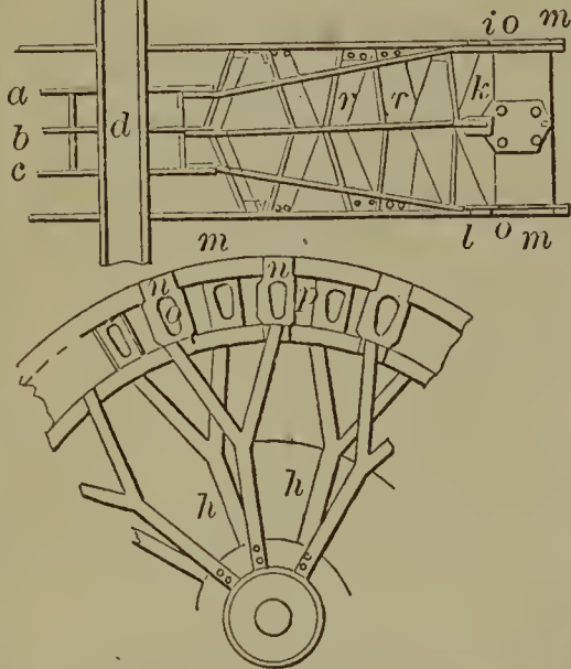
58603—Collins & Holland—Paddle Wheel.
