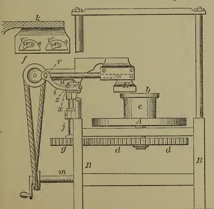
53518—Best & Drake—Machine for Ironing Hats.
