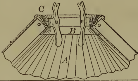
60580—A. M. Shurtleff—Atomizing Tube.
