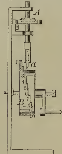
51821—A. W. Foster, Jr.— Cut-off Valve Gear.
