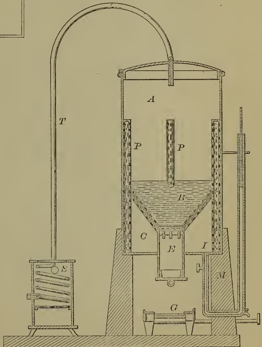
53547—H. Y. Hind— For Preparing Peat.
