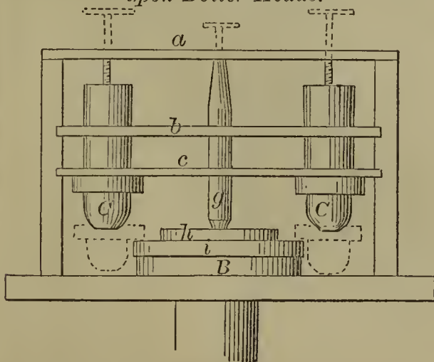
55687—W. W. Martin—Bending Flanges upon Boiler Heads.
