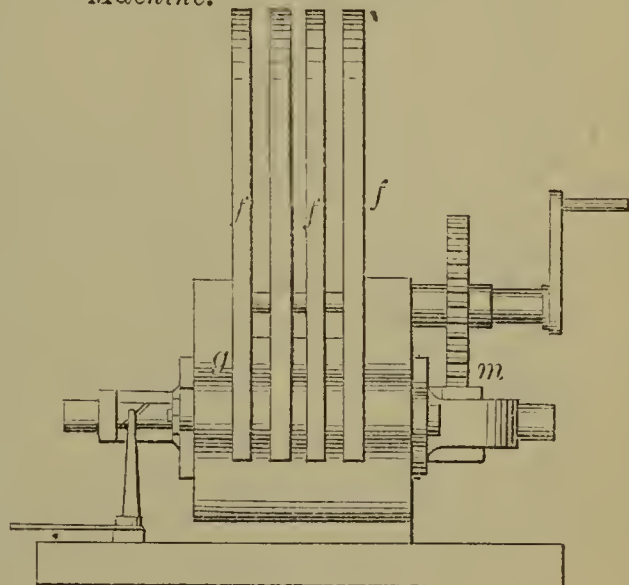
59738—H. Wilde— Magneto-Electric Machine.
