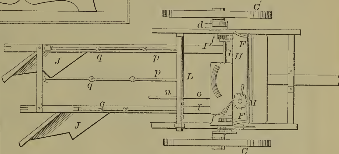
59855—P. Merkel—Gang Plow.
