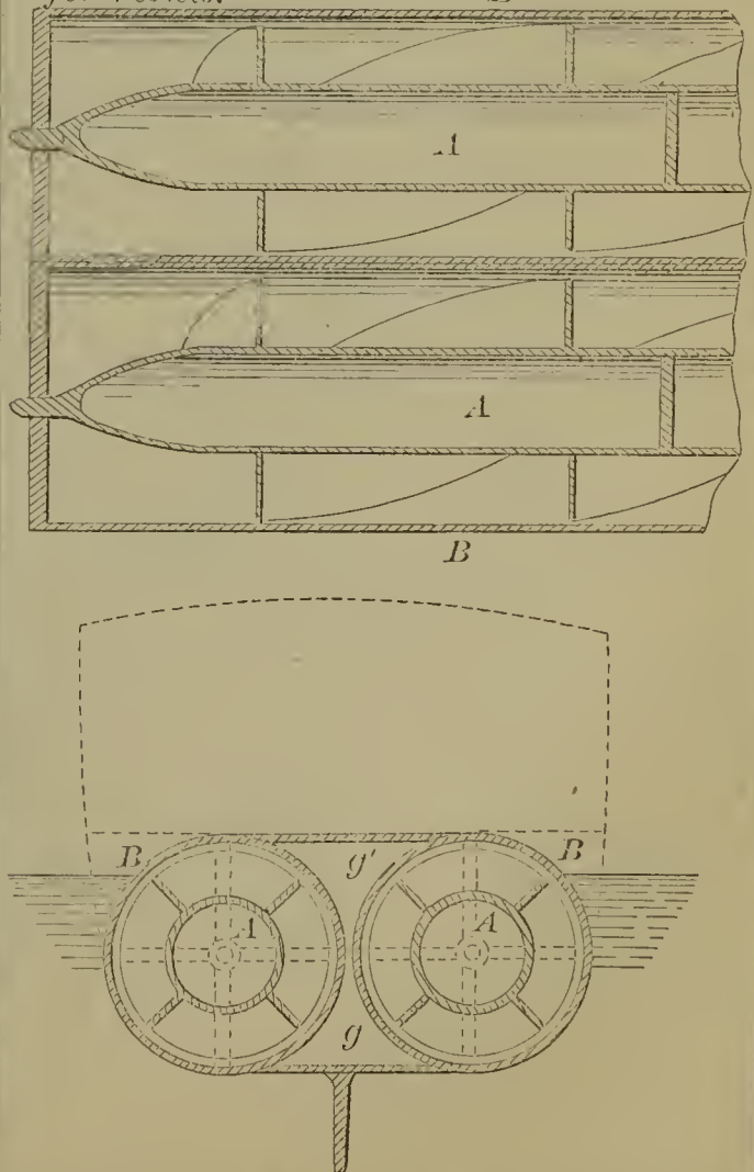
57033—D. Winer—Propelling Apparatus for Vessels.
