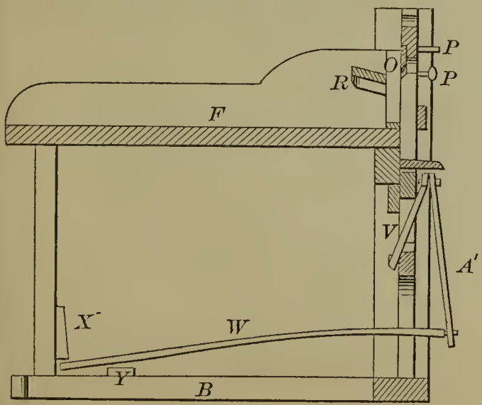
52992—W. Green—Cutting Box.
