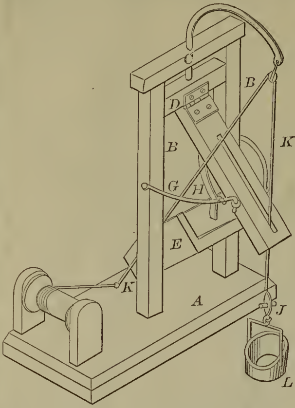
55557—J. P. Tucker— Coal Elevator.
