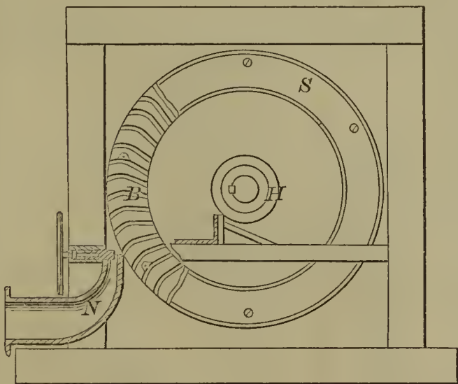
55323—T. McAuley—Water Wheel.
