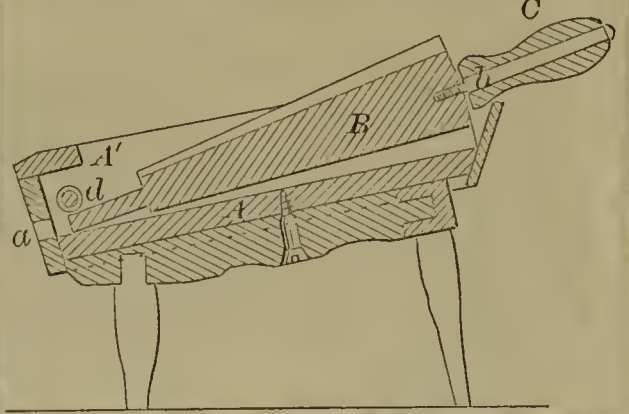
55714—J. Robinson—Butter Worker.
