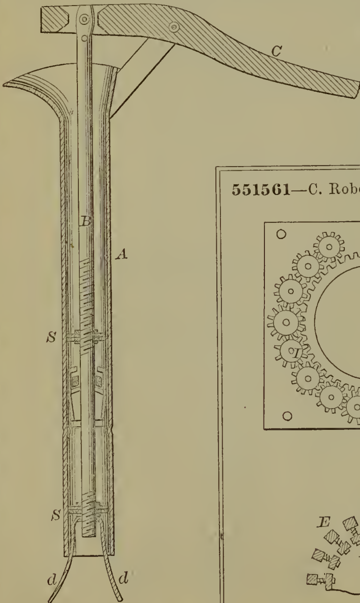
55155—Palmer & Bean—Reservoir for Wells.
