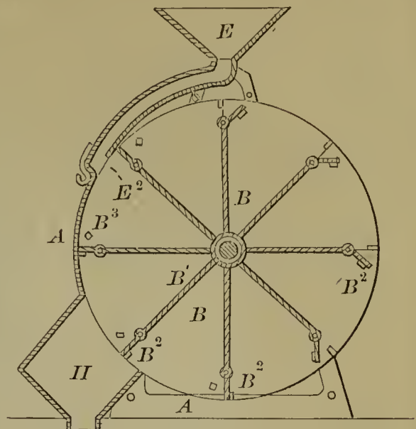
54072—W. S. Sampson—Grain Meter.
