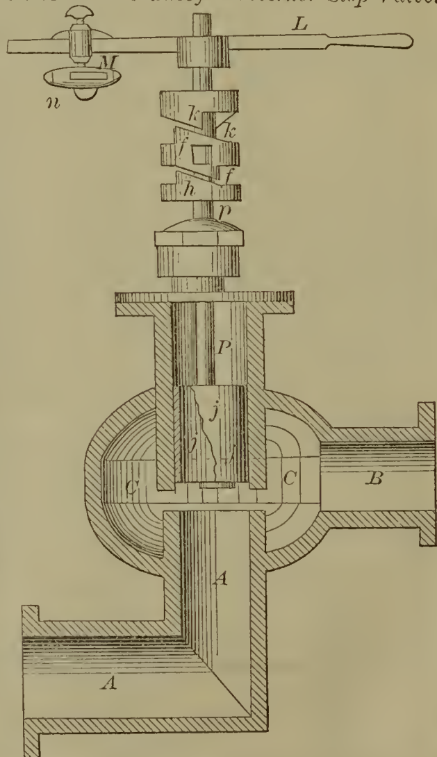
56186—J. Crawley—Governor Stop Valve.
