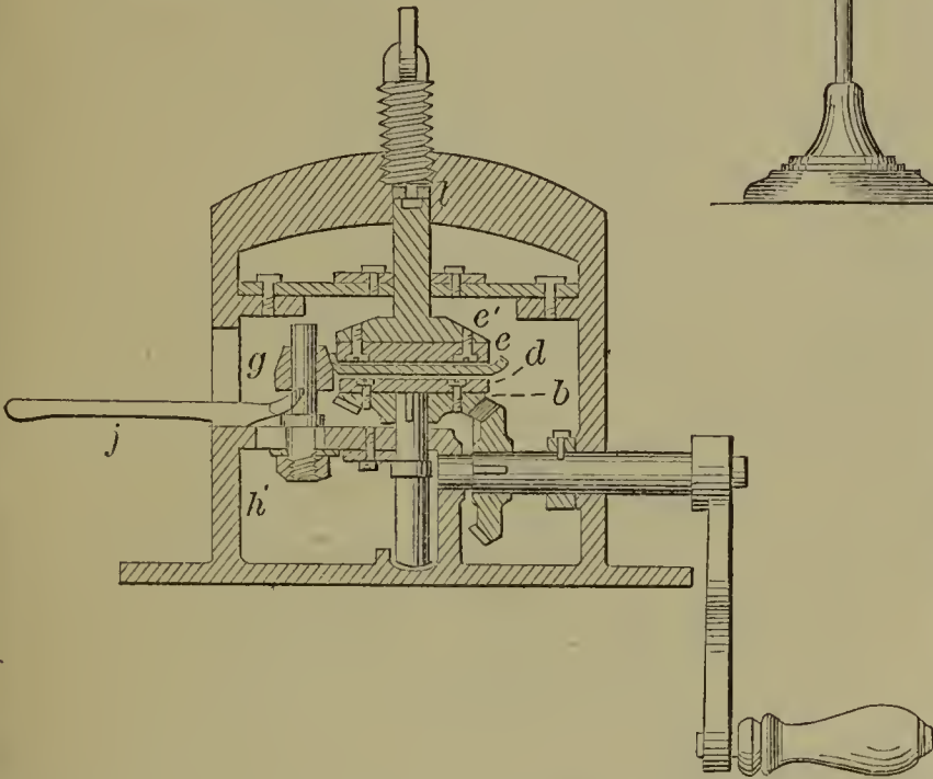
54923—A. Kollenberg— For Making Tin Fruit Cans.
