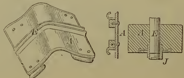
59651—H. A. Rains— Cart Harness Saddle.
