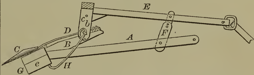
58578—T. Beale— Cultivator.
