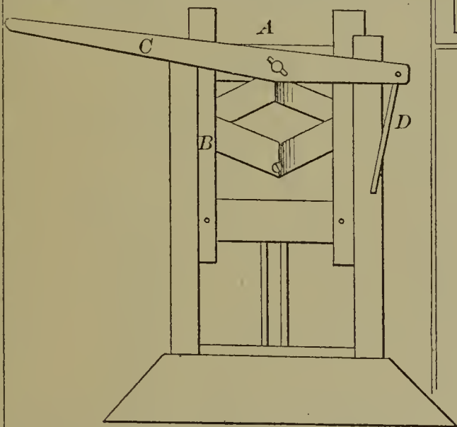
53416—M. Cole—Straw Cutter.
