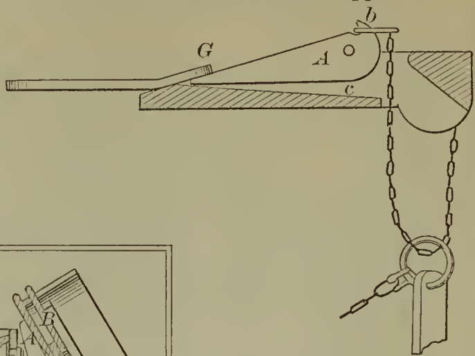
52143—E. Davidson—Anchor Tripper.
