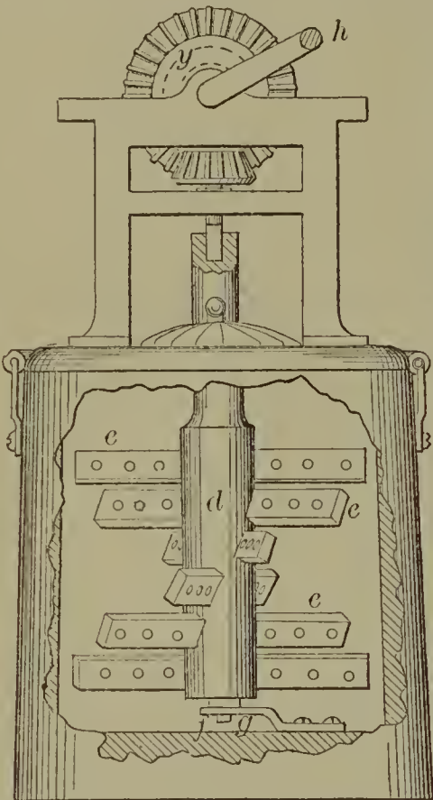
60040—A. P. Odholm—Machine for Dressing Felles.
