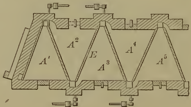
52801—T. M. Gisborne— Brick Machine.
