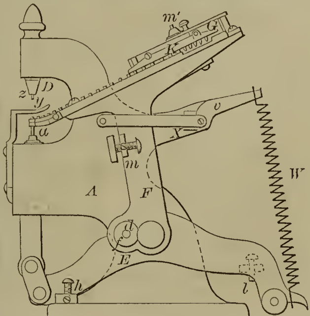
57446—G. Shipman— Eyeletting Machine.
