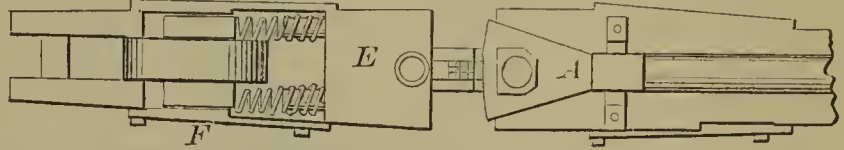
57658—J. Bailor— Car Coupling.
