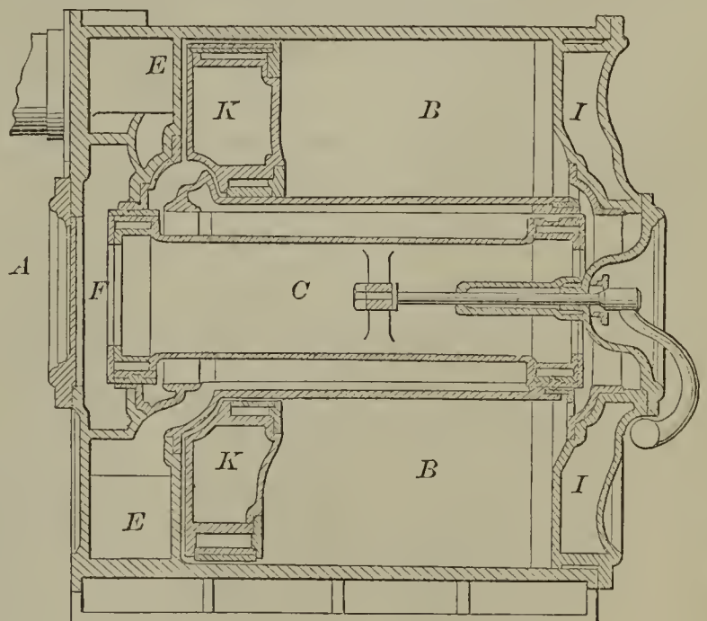
51885—G. B. Whiting— Steam Engine.
