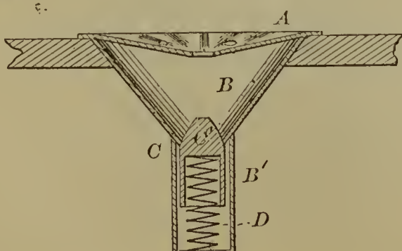
56400—F. H. Furniss—Car Spittoon.
