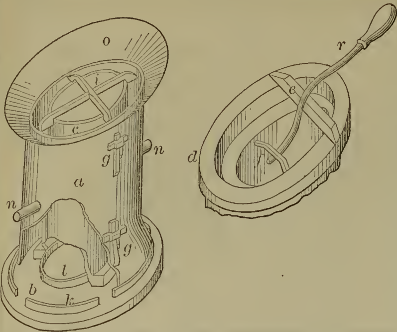
54520—W. H. Flinn— For Cutting Wire.
