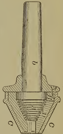
56329—I. Smith—Chuck.
