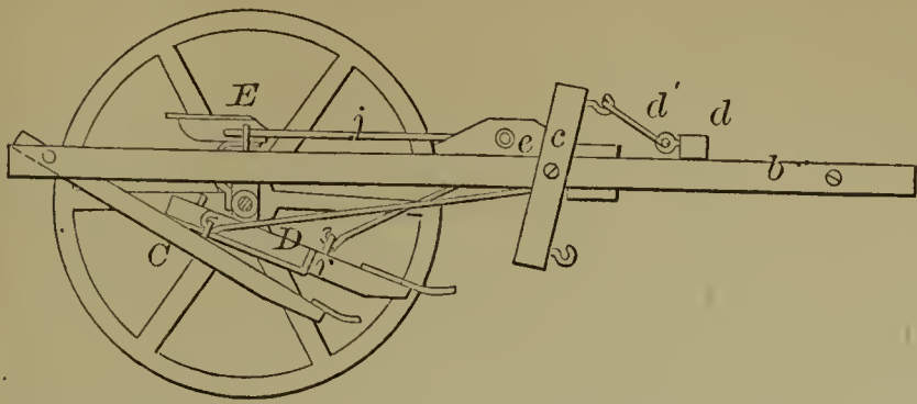
54763—Parmele & Patterson—Cultivator.
