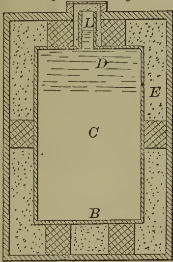
56620—T. P. Shaffner— Packing Nitro-Glycerine.
