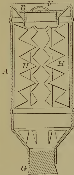
54776—A. M. Robinson— Egg Beater.
