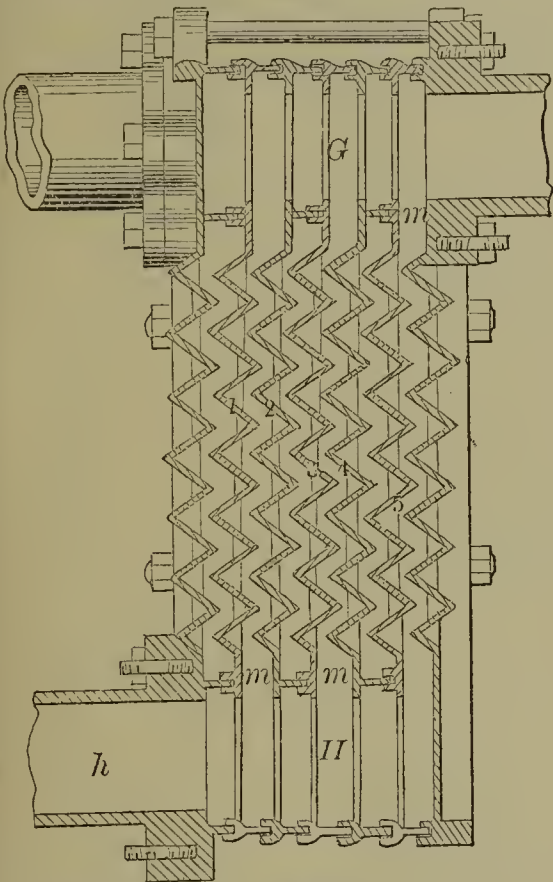
55149—J. Nason— Surface Condenser.
