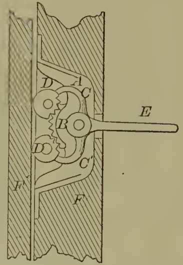
52388—C. B. Clark— Sash Fastening.
