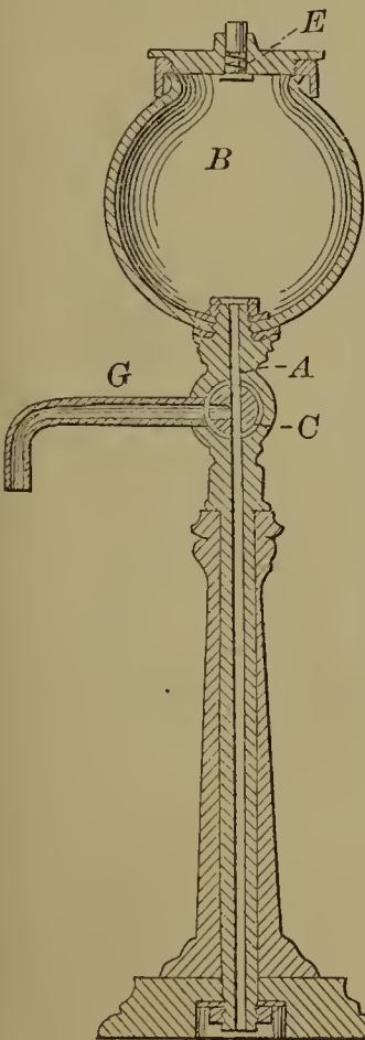
54548—F. H. Houghton— For Measuring Liquids.
