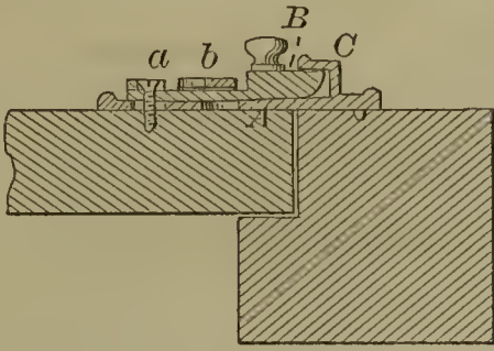
52750—A. H. Rowe—Door Latch.
