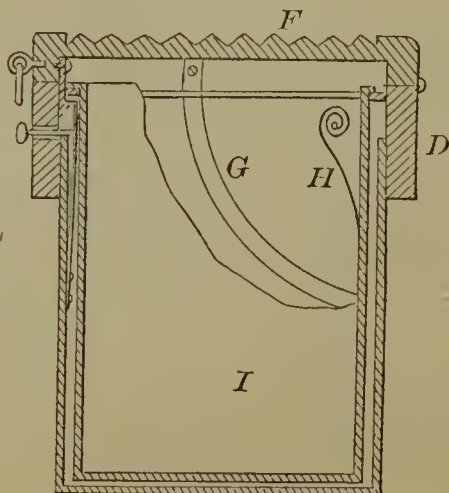
54172—Kee & Sloan— Ash Box.
