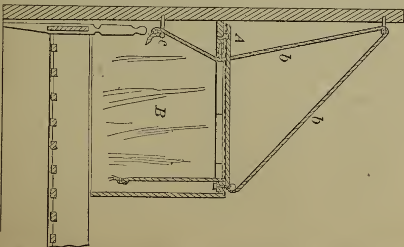
54674—M. Bliss— Musquito Canopy.
