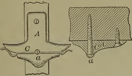
60210—Luther & Marsh—Blind Fastening.
