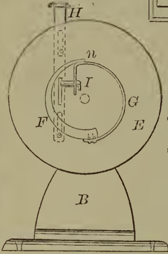
60278—Stoner & Sigwalt— For Boxing Paper Collars.
