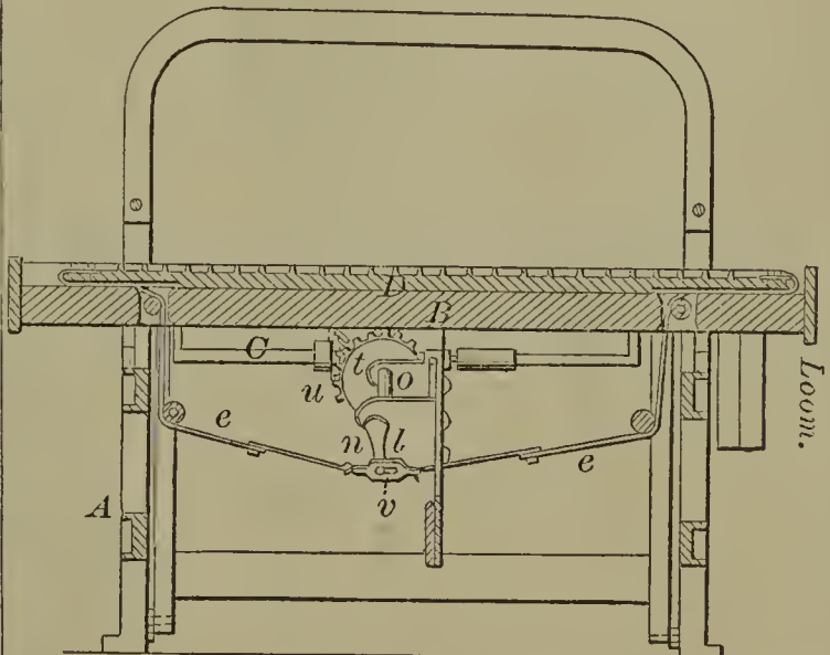
60388—L. J. Knowles—Narrow Ware Loom.
