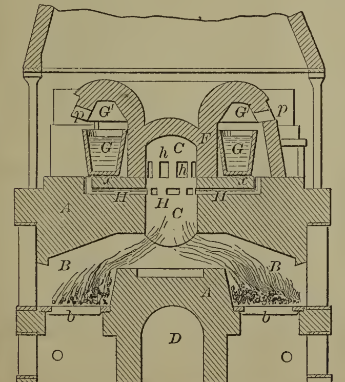
60307—S. A. Whitney—Melting Furnace.
