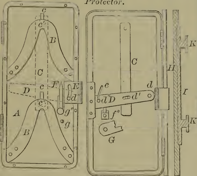
55838—A. Drummond— Pocket Book Protector.
