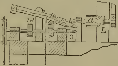
57232—Wheeler & Manley—Hat Pomering Machine.
