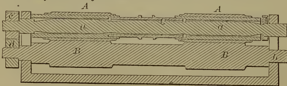
54732—D. Hussey—Drawing Rollers.
