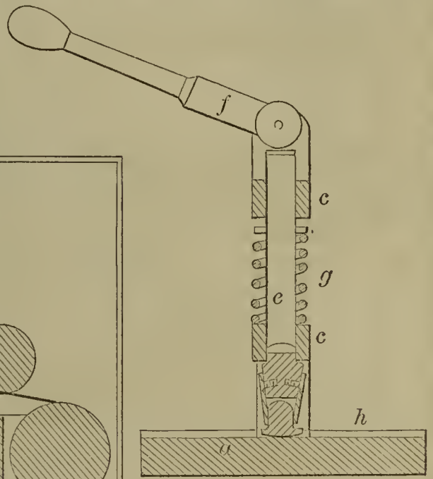
55334—Merriam & Norton—Glueing Press.
