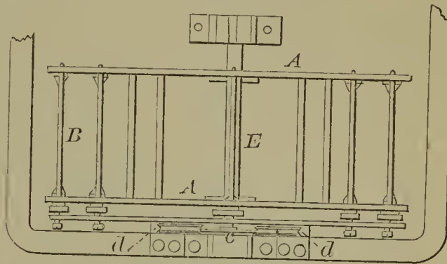
56712—J. W. Cochran—Packing Projectiles.
