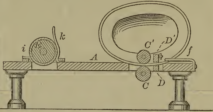
52739—E. Nougaret— For Pouncing Hats.
