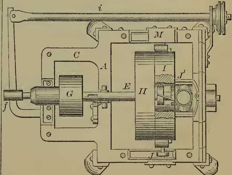
53989—C. & A. Kaestner—Grinding Mill.
