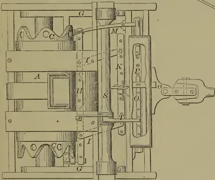
59826—D. Evers—Tenoning Machine.
