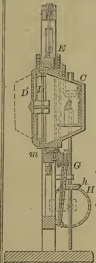
60594—E. H. Tobey—Railroad Signal Light.
