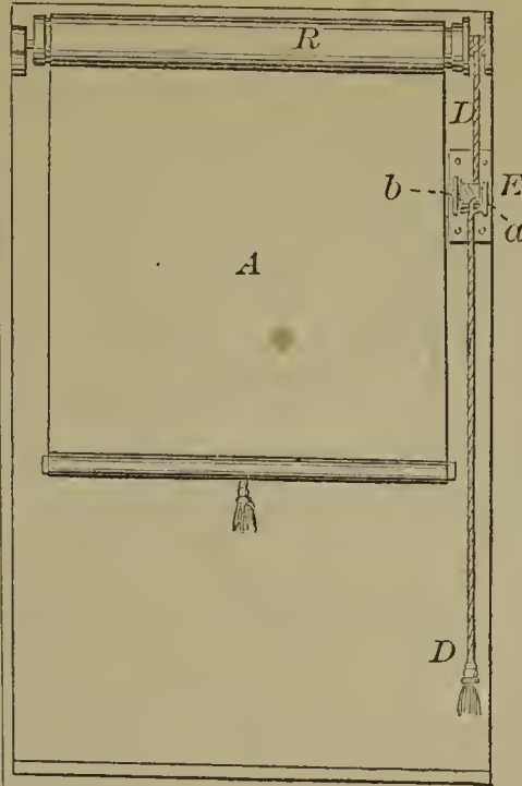
59009—B. Handforth— Curtain Fixture.
