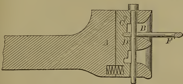
55271—E. J. Frazier—Car Coupling.
