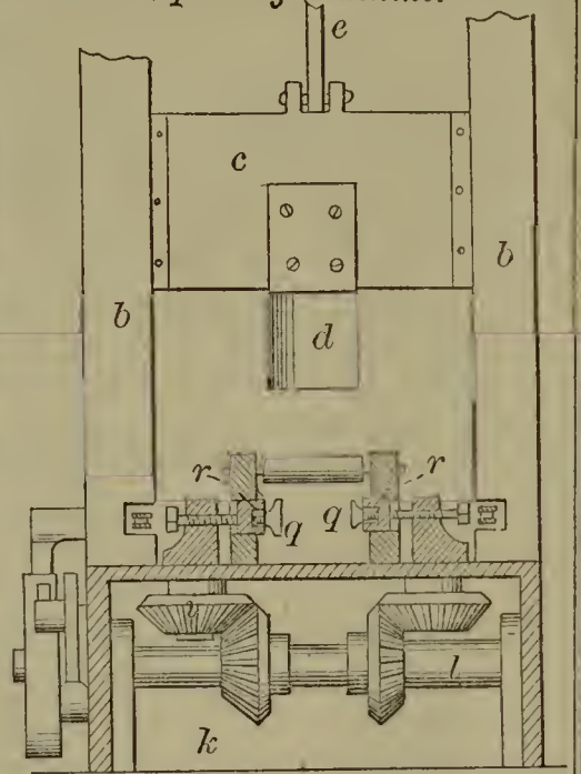
52352—W. L. Williams—Wood Splitting Machine.
