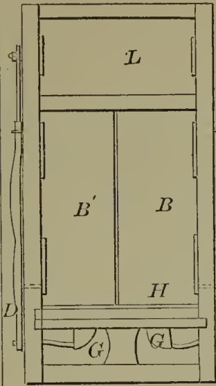
60022—H. L. Lowman—Die for Forming the Eyes of Pick Axes.
