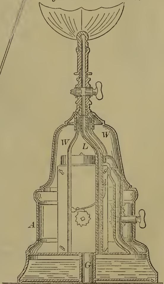
56155—Herzog & Cohn— Hydro-Carbon Burner.
