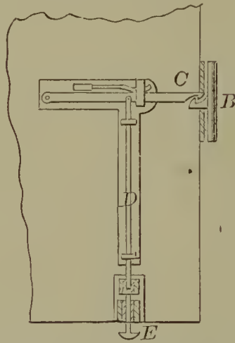
60021—G. H. Lenher—Sewing Machine Shuttle.
