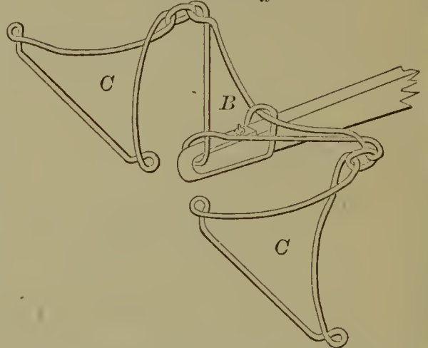
57804—T. H. White— Knife Sharpener.
