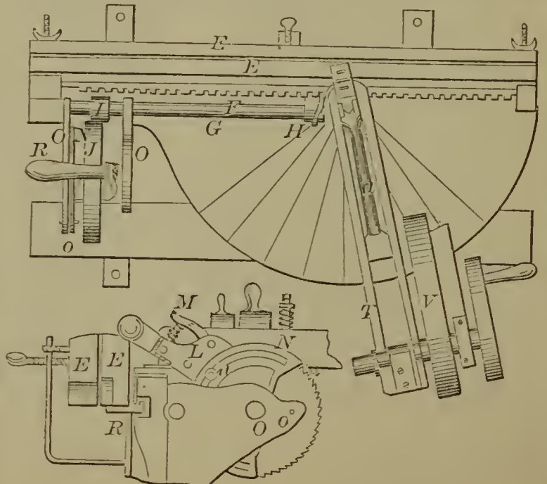
59193—J. W. H. Doubler—Saw Filing Machine.
