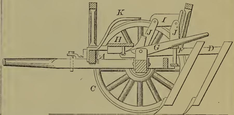
54159—G. Hillegrass— For Tightening Wagon Tires.
