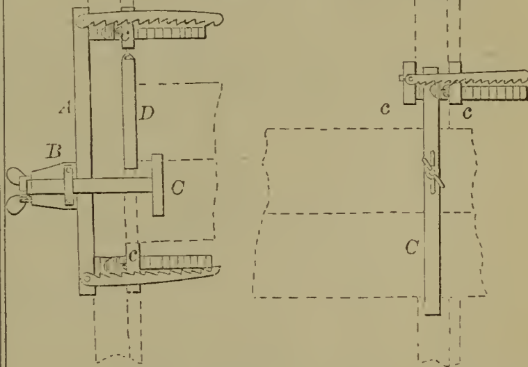
59626—D. M. Mourland—Clamp and Gauge for Weather Boarding.
