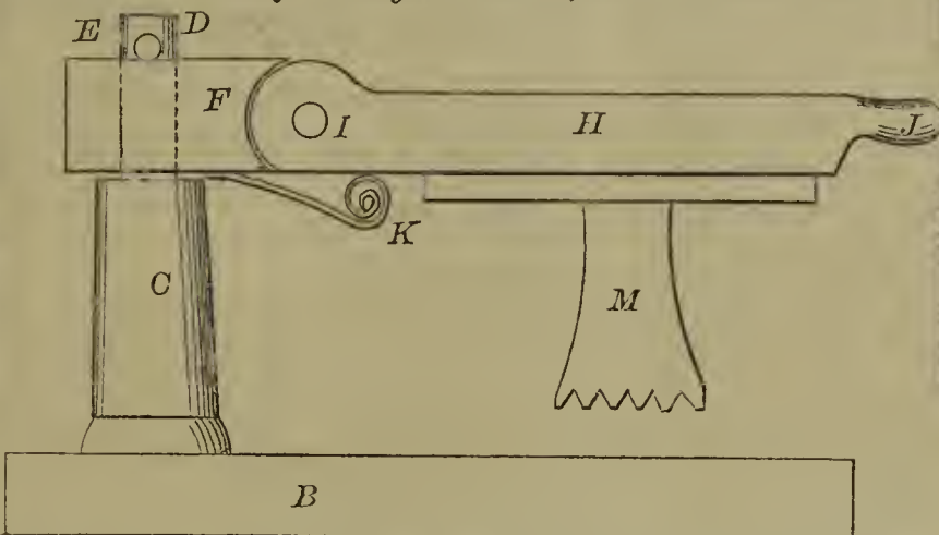
56092—C. N. Pond—Lamp Chimney Cleaner.
