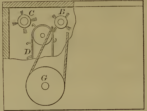
55373—N. B. Sherwood—Cotton Seed Planter.
