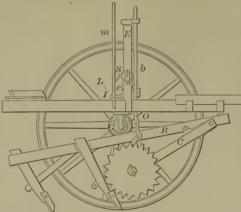
52093—Thomas & Mast—Cultivator.
