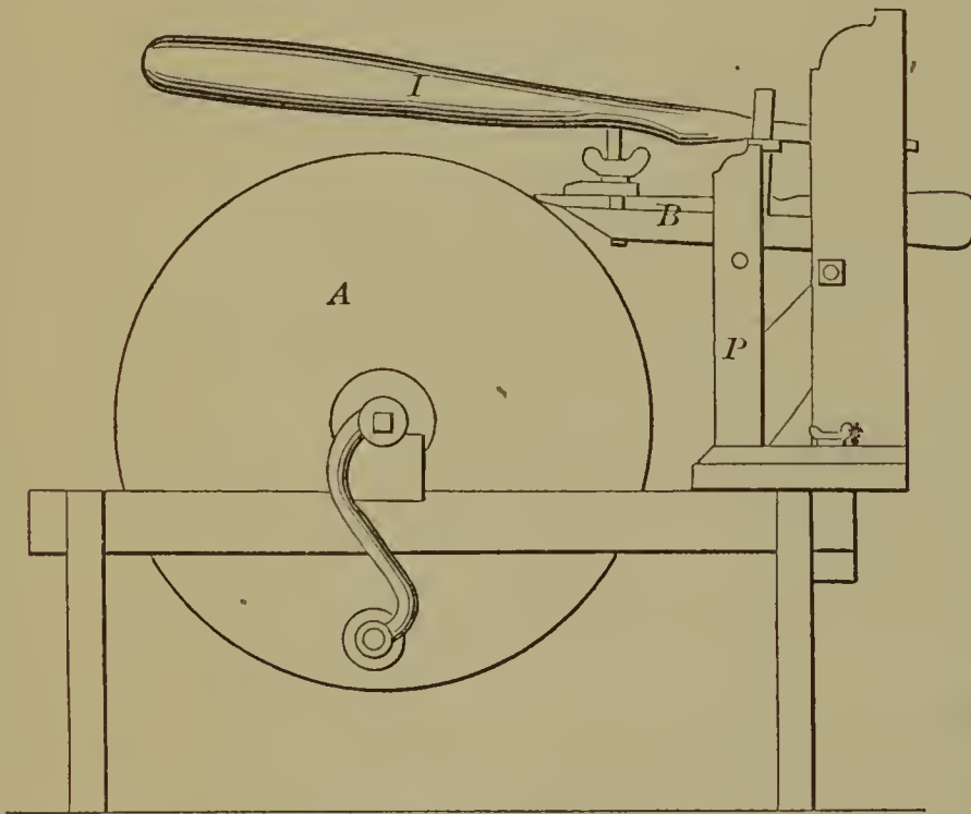
53747—J. Richardson—Machine for Holding and Grinding Edge Tools.
