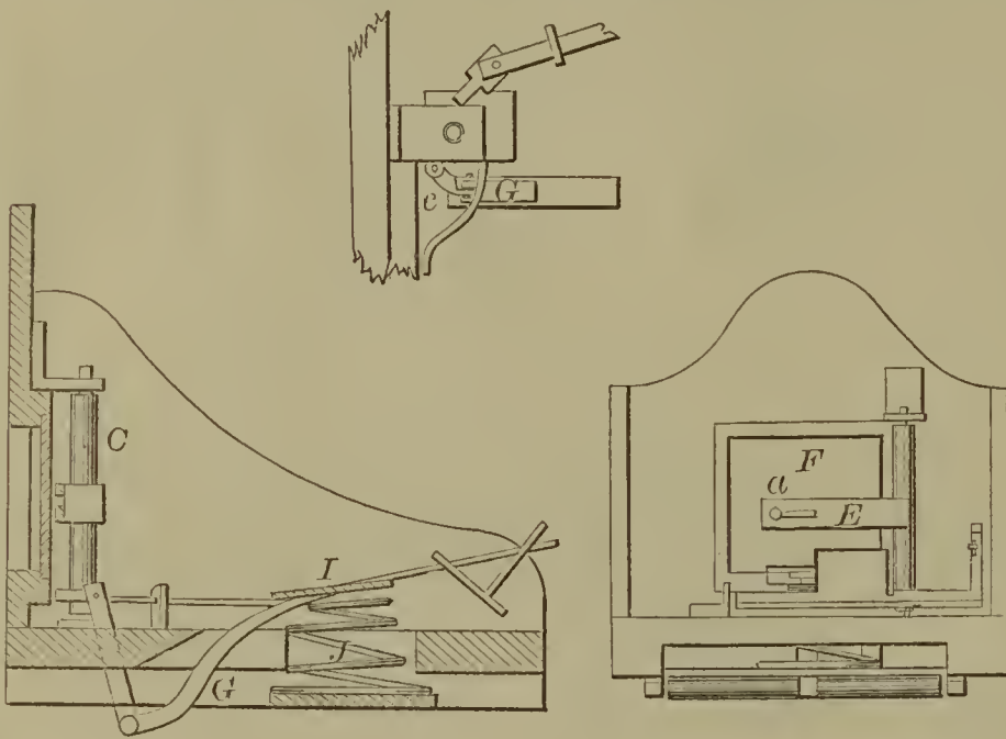
58799—Fessler & Maxell—For Opening Furnace Doors.
