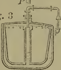
59312—C. J. Everett—Rendering Apparatus.
