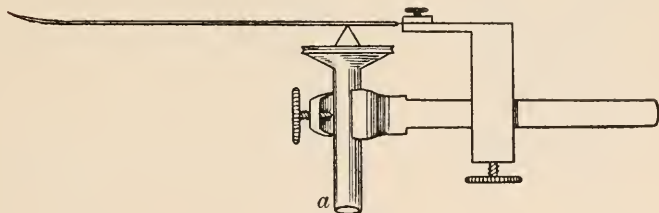
FIG. 66.—DIAGRAM (AFTER SCHENCK) TO SHOW THE PRINCIPLE OF THE HÜRTHLE KYMOGRAPH. a , TUBE TERMINATING ABOVE IN A TAMBOUR-LIKE ENLARGEMENT COVERED BY A STOUT RUBBER MEMBRANE UPON WHICH IS A METAL DISK AND A WEDGE ACTUATING A VERY LIGHT LEVER. THE TUBE IS CONNECTED BY RUBBER PRESSURE TUBING WITH AN ARTERY CANNULA LIKE THAT SHOWN IN FIG. 64, AND THE WHOLE IS FILLED WITH SODIUM BICARBONATE SOLUTION.
