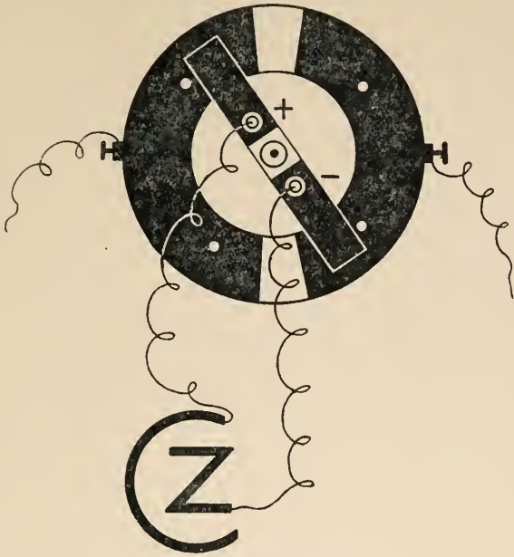
FIG. 17.—WALLER'S COMMUTATOR.
