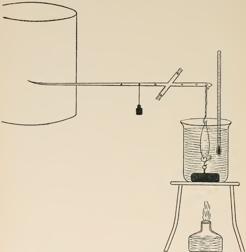
FIG. 38.—EXPERIMENT FOR INVESTIGATING THE EFFECT OF HEAT ON THE EXTENSIBILITY OF MUSCLE.
