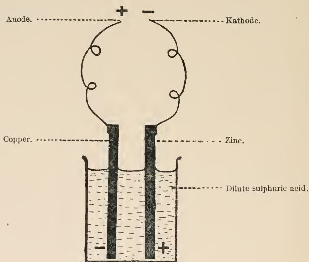
FIG. 1.—VOLTAIC COUPLE.
