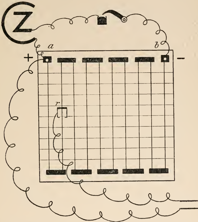
FIG. 20.—DIAGRAM OF THE OXFORD FORM OF RHEOCHORD. a , b , RHEOCHORD WIRE ZIG-ZAGGED UPON A MAHOGANY BOARD, MARKED BY CROSS LINES INTO HUNDREDETHS; r , RIDER.
