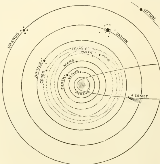
FIG. 2.--The Planets of our Solar System.
