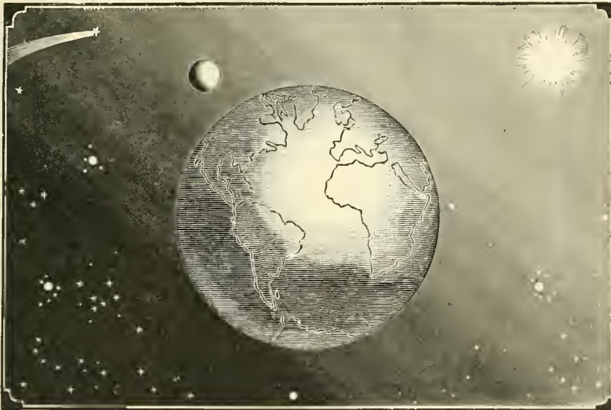
Fig. 5--The Earth as it Appears in Space.
