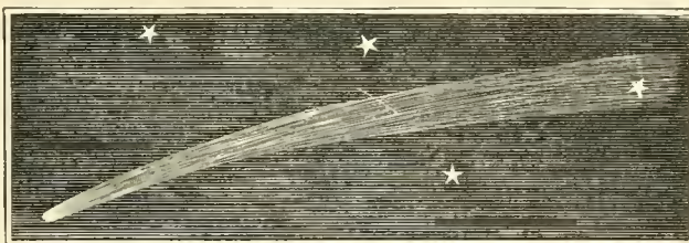
Fig. 7--The Great Comet of 1843, The tail of which was 130,000,000 miles in length.
