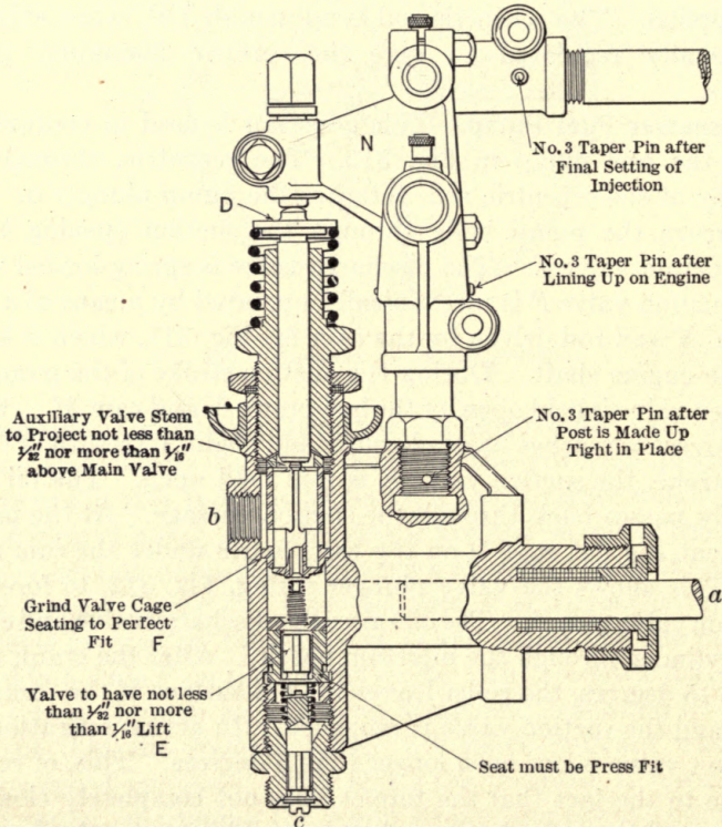
FIG. 312.—Bessemer oil engine fuel pump.
