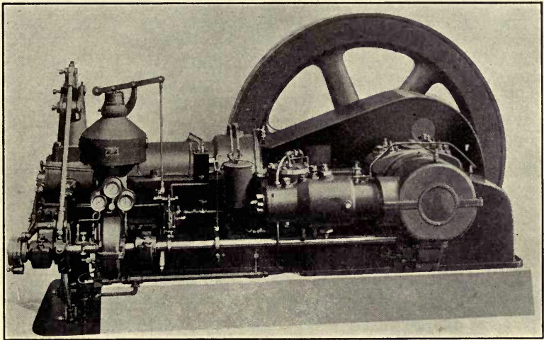
FIG. 12.—Allis-Chalmers Diesel, single cylinder.
