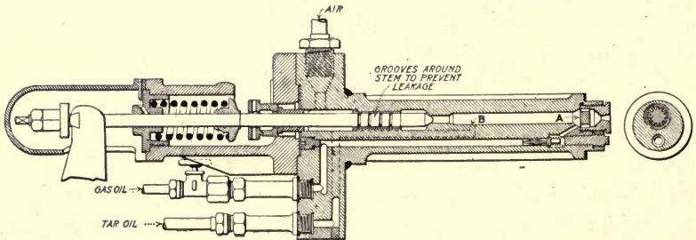
FIG. 133.—Körting tar oil fuel valve.
