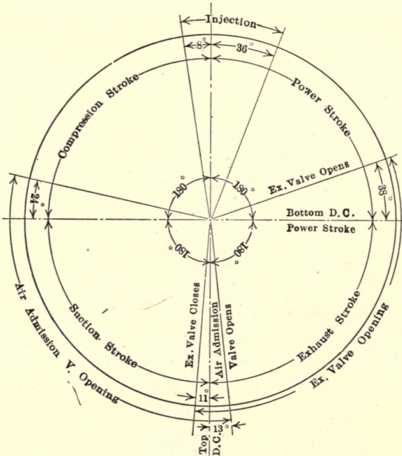
FIG. 96.—National Transit Diesel. Valve timing.
