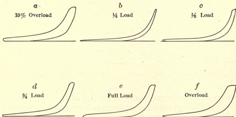
FIG. 201.—Indicator cards, National Transit Diesel.
