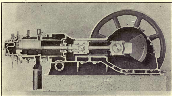
FIG. 255.—Bessemer oil engine.
