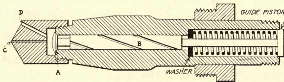
FIG. 321.—Fairbanks-Morse oil engine fuel atomizer nozzle.
