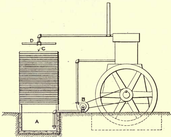
FIG. 165.—“Closed” cooling water system.
