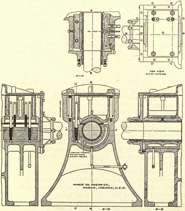
FIG. 285.—Muncie oil engine main bearing, quarter-box type.
