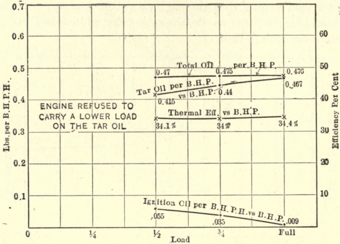
FIG. 188.—100 H.P. Körting Diesel using tar oil and an ignition oil.
