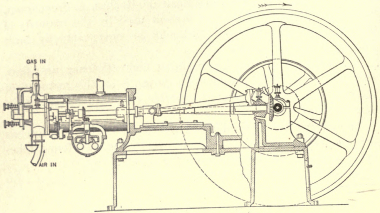
FIG. 2.—Otto's silent engine.
