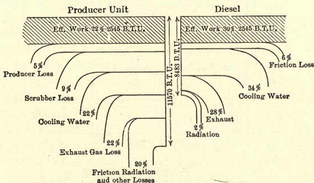
FIG. 194.—Heat balances.
