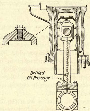
FIG. 47.—Busch-Sulzer Diesel connecting-rod.
