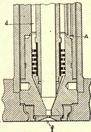
Fig. 115.—Bush-Sulzer type B fuel valve.
