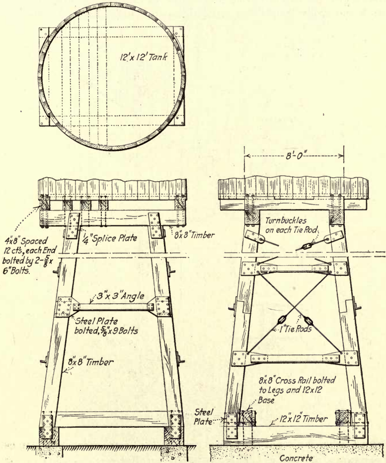
FIG. 167.—Wooden tank and tower.
