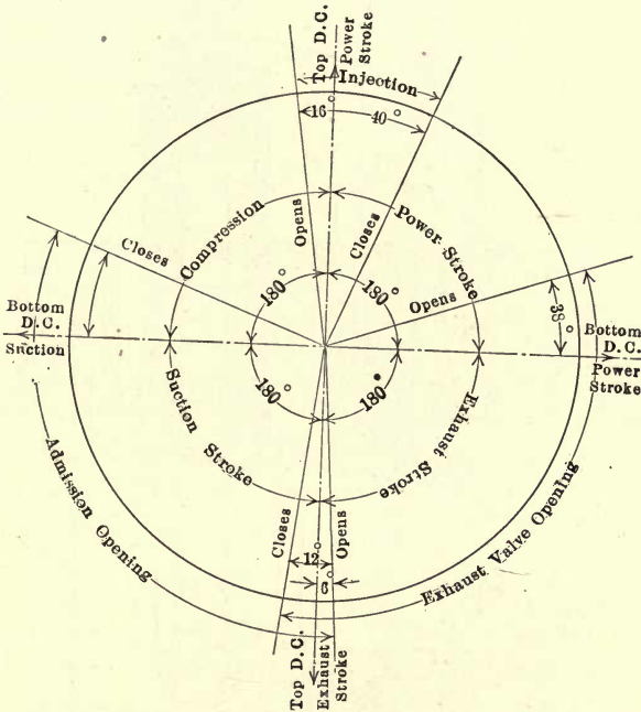
FIG. 88.—Valve timing McIntosh & Seymour 500 H.P. Diesel engine 164 R.P.M. 4 cylinders 18 \frac{7}{8} dia. \times 28 \frac{3}{4} stroke.
