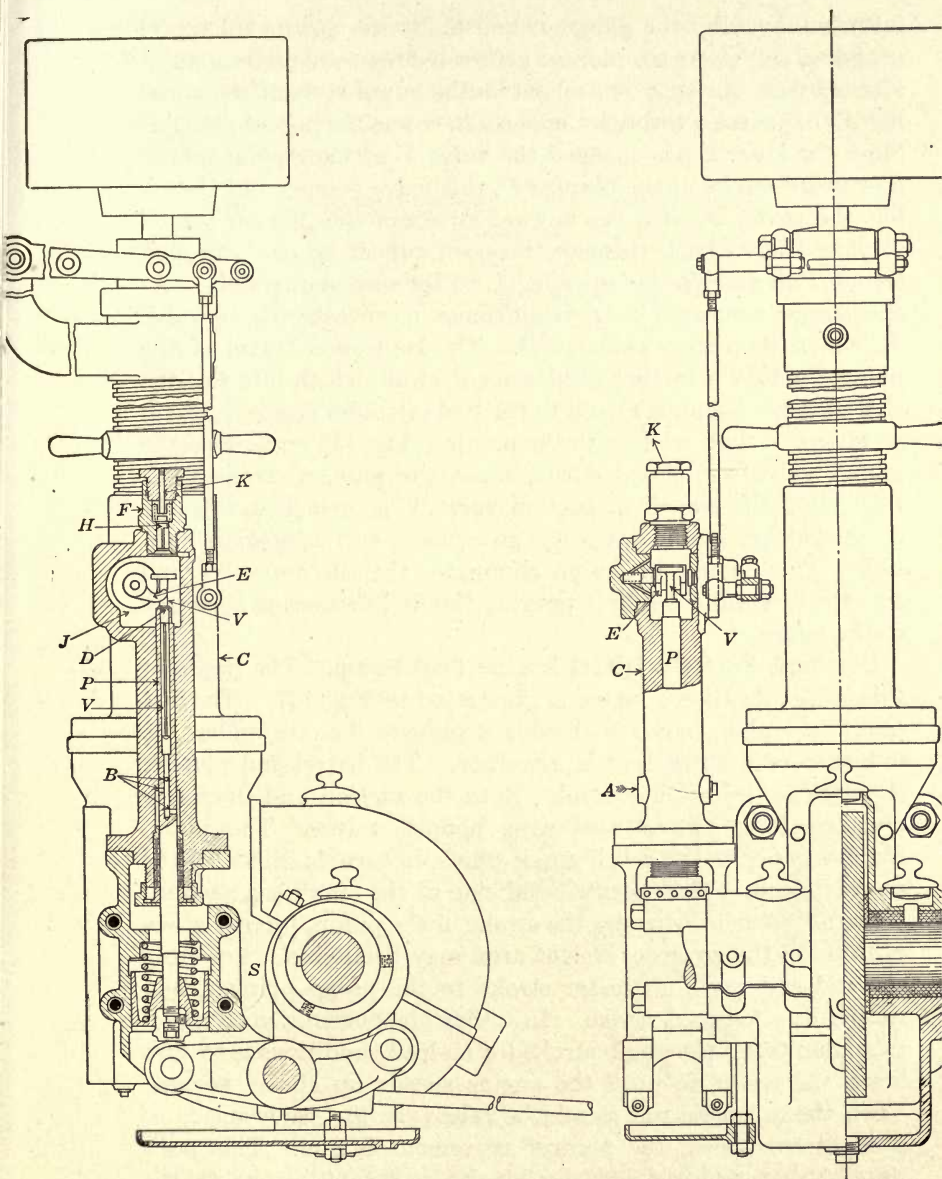
FIG. 146.—Fuel pump and governor, type D-3. National Transit Diesel.
