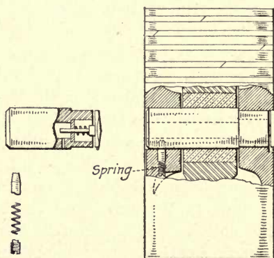
FIG. 271.—Piston pin oiling. (Fairbanks Morse Co.)
