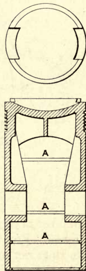
FIG. 53.—McIntosh and Seymour Diesel piston.
