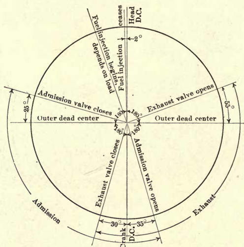
FIG. 317.—De La Vergne type D.H. engine valve timing.
