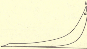
FIG. 203.—Two cycle engine delayed ignition.
