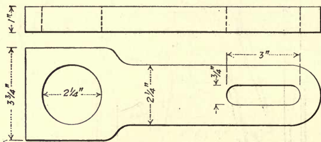
FIG. 25.—Centering strip.
