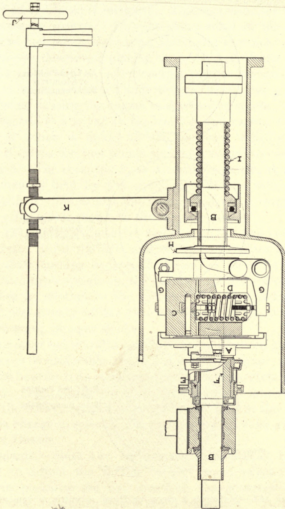
Fig. 152. — McIntosh & Seymour Diesel governor.
