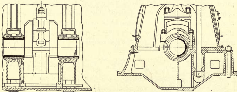
FIG. 32.—Busch-Sulzer Bros. Diesel main bearing.
