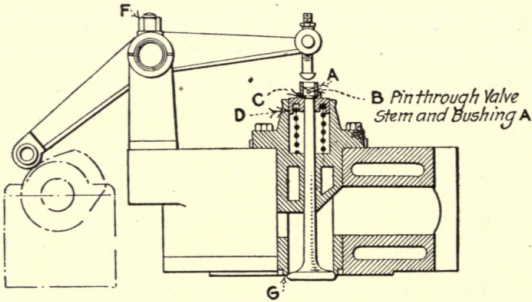
FIG. 86.—McIntosh and Seymour valve layout.
