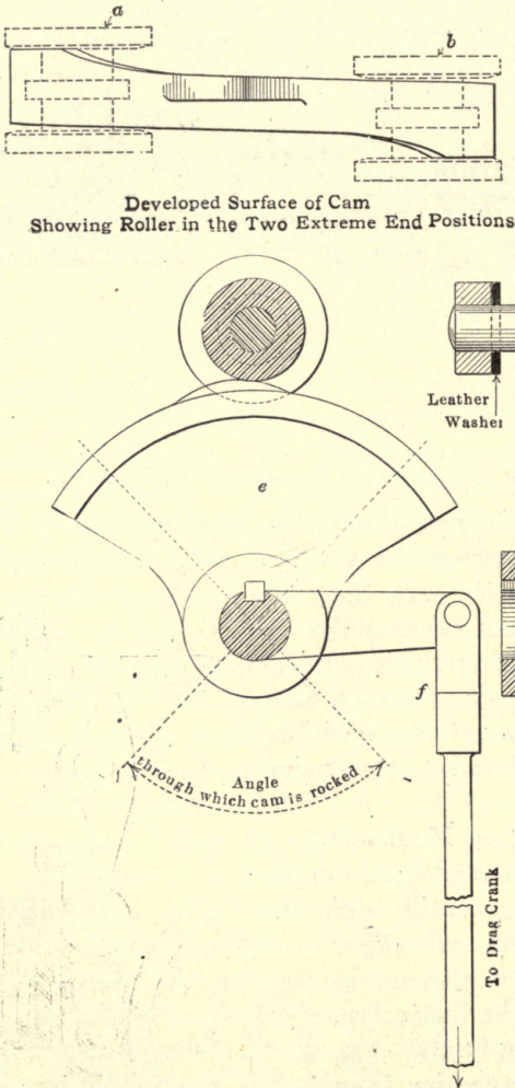
FIG. 131.—Standard Fuel Oil engine fuel cam.
