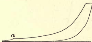
FIG. 209.—Four stroke cycle Diesel early exhaust opening.
