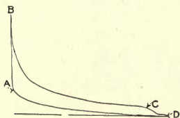
FIG. 215.—Card from two-stroke low compression engine.
