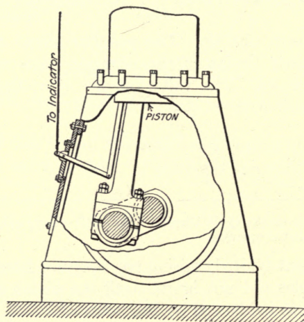
FIG. 213.—Indicator rigging.
