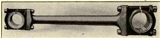
FIG. 45.—McEwen Diesel connecting rod.
