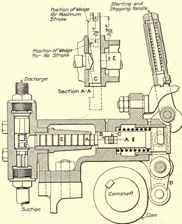
FIG. 140.—McEwen Bros. Diesel fuel pump.
