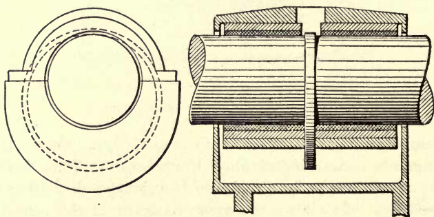
FIG. 284.—Main bearing.
