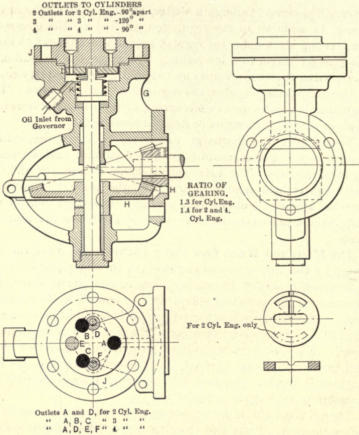
FIG. 305.—Fuel distributor M. & W. vertical engines.
