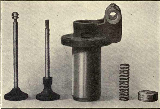
FIG. 93.—McEwen Diesel admission valve and cage.
