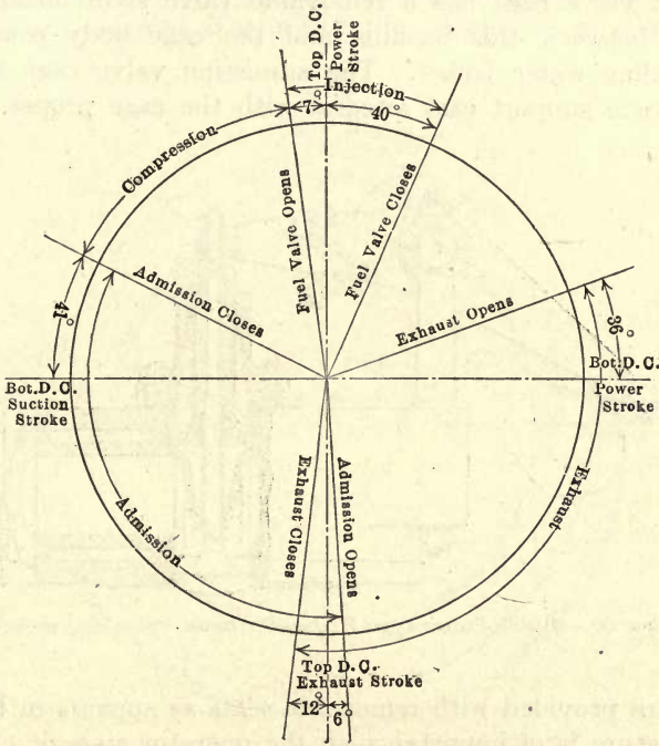
FIG. 79.—Valve timing of American Diesel engines.
