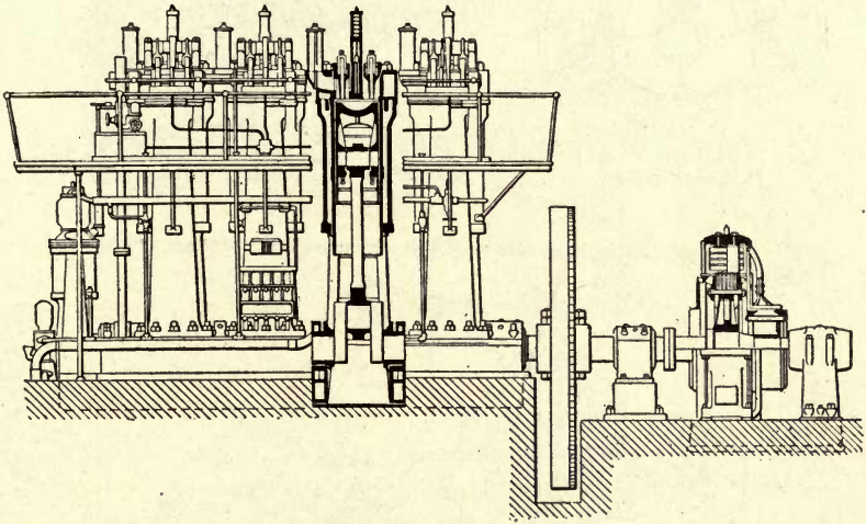
FIG. 68.—McIntosh & Seymour A frame Diesel.
