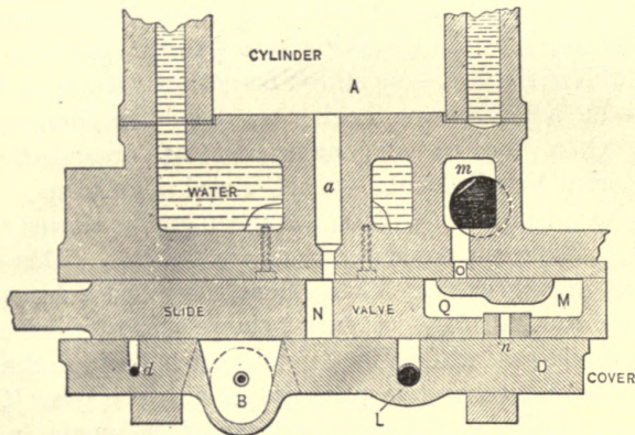
FIG. 3.—Cross-section of Otto's silent engine valve.
