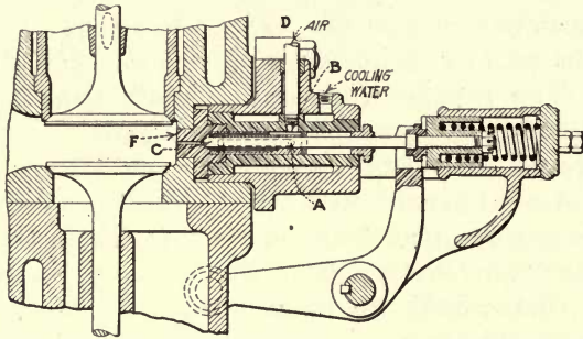
FIG. 112.—American Diesel fuel valve assembly.
