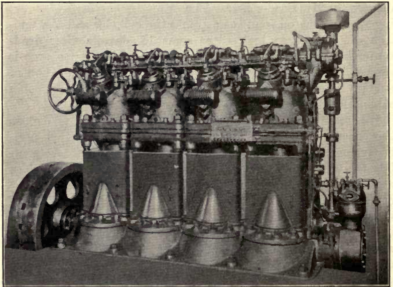
FIG. 223.—Midwest type V.D.H. vertical semi-Diesel oil engine.
