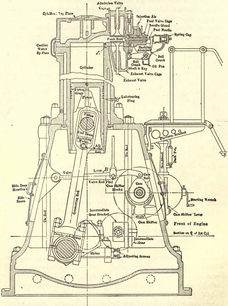
FIG. 7.—Cross section of American Diesel engine.
