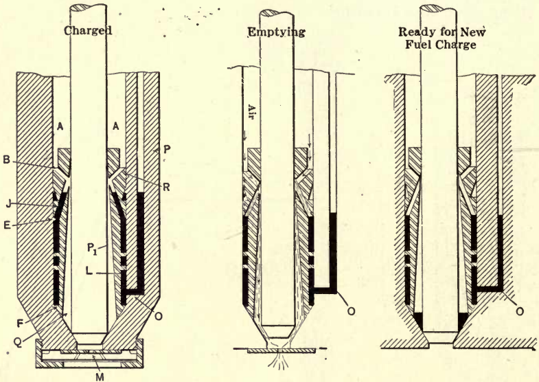
FIG. 119.—McIntosh & Seymour Diesel Hesselmann fuel valve action.
