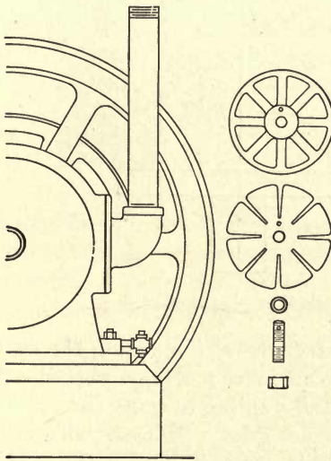
FIG. 276.—Air suction valve, F. M. & Co. horizontal oil engine.
