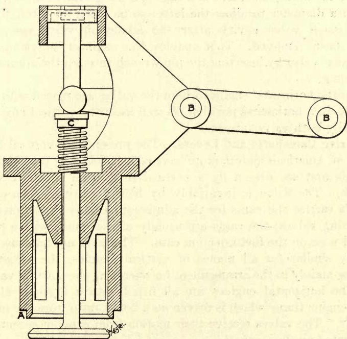
FIG. 77.—Admission valve cage. American Diesel.
