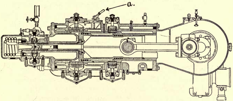
FIG. 159.—Snow Diesel three-stage air-compressor.
