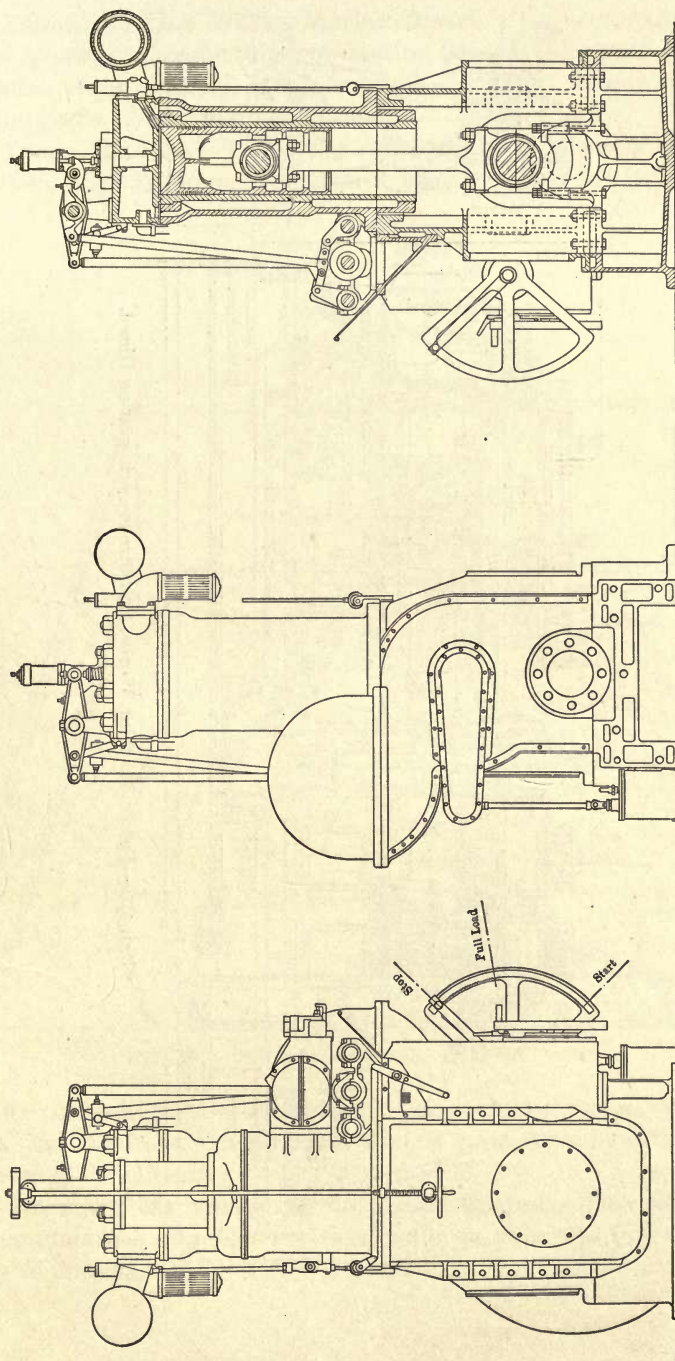
Fig. 21.—McIntosh and Seymour marine Diesel.
