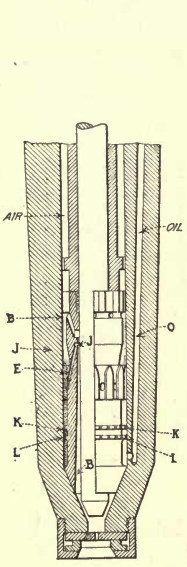
FIG. 117.—McIntosh & Seymour fuel valve.
