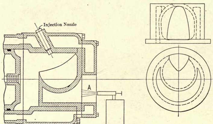
FIG. 254.—Buckeye Barrett oil engine combustion chamber.
