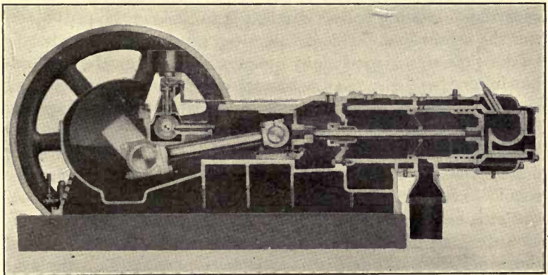
FIG. 275.—Buckeye-Barrett oil engine.
