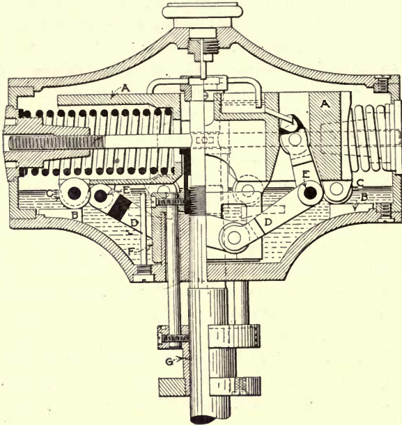
FIG. 148.—System Jahns governor.
