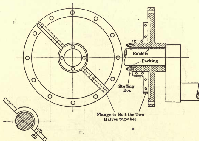
FIG. 280.—Stuffing box air seal.
