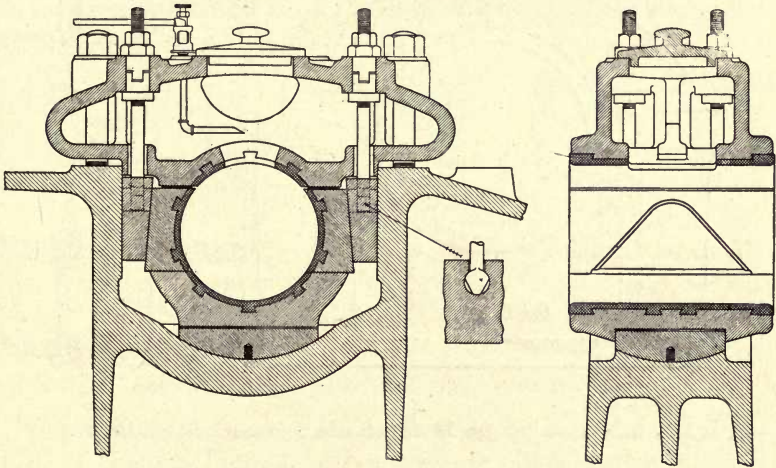
FIG. 30.—Allis-Chalmers Diesel main bearing.
