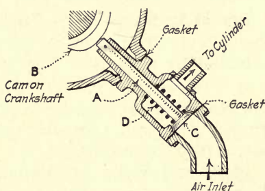
FIG. 340.—Fairbanks-Morse Co. vertical air starting valve.
