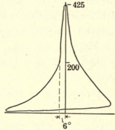
FIG. 241.—Distorted card Price engine.
