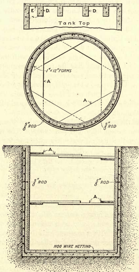
FIG. 183.—Concrete oil storage tank.
