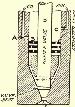
FIG. 110.—Fuel valve, closed type.
