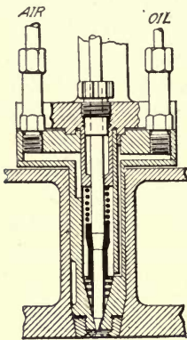
FIG. 132.—Fulton Machine Co. Diesel fuel valve.
