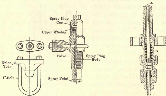
FIG. 323.—Fuel nozzle, Primm oil engine.
