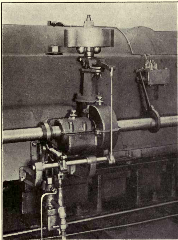
FIG. 143.—De La Vergne type FD Diesel fuel pump.
