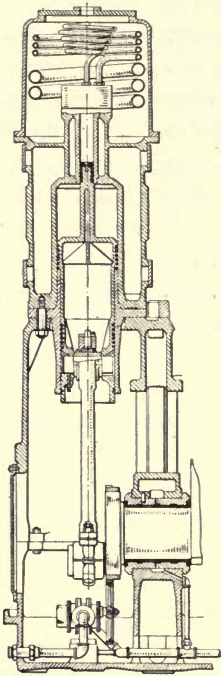
FIG. 156.—Three-stage compressor.
