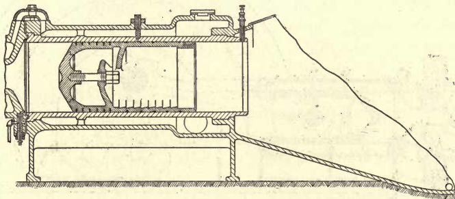
FIG. 71.—Allis-Chalmers Diesel cylinder.
