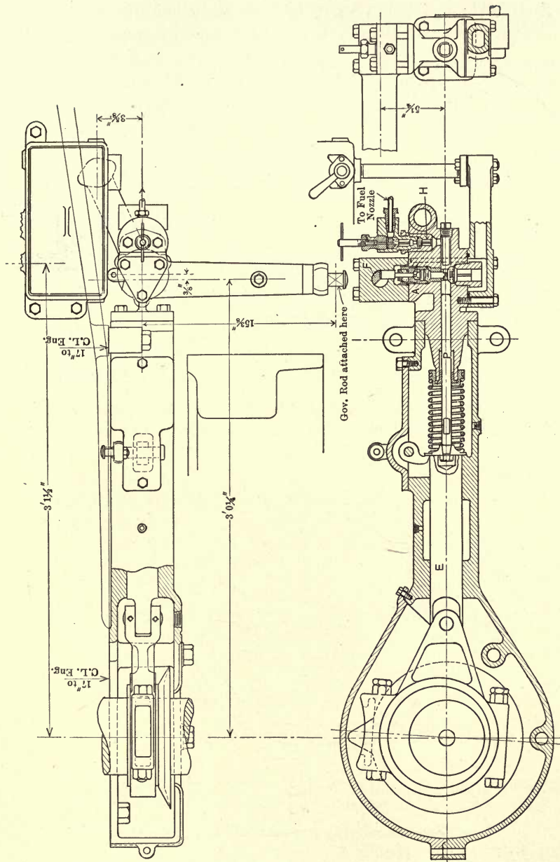
FIG. 227.—Nordberg semi-Diesel engine fuel pump.
