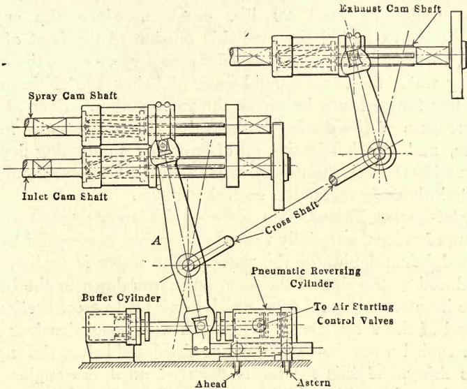
FIG. 104.—Nelseco four-cycle-engine reversing mechanism.
