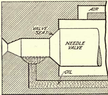
FIG. 111.—Open nozzle fuel valve, elementary form.
