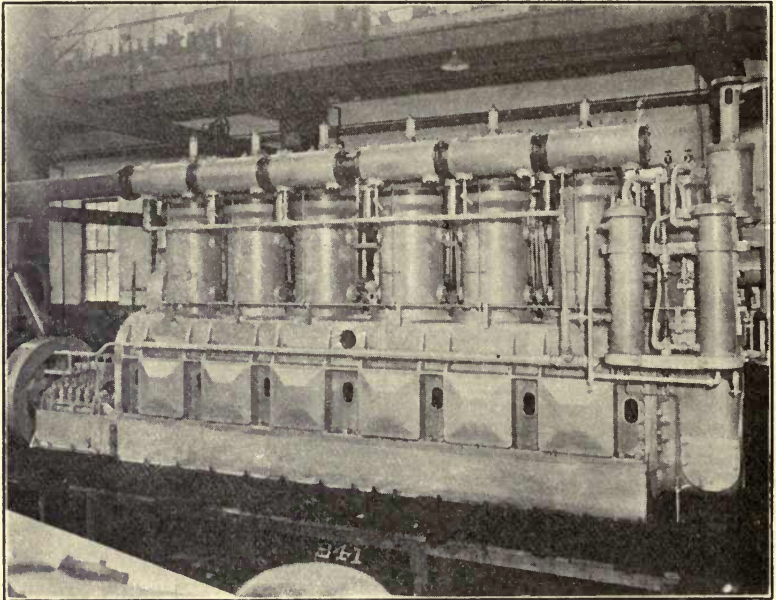
FIG. 20.—600 H.P. McIntosh and Seymour marine Diesel four-stroke-cycle reversible type.
