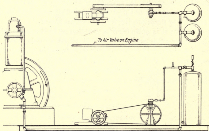
FIG. 339.—Air piping arrangement.
