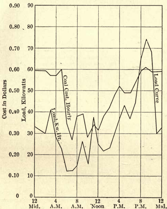
FIG. 356.—Hourly load and fuel cost, steam power.
