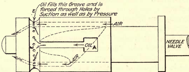
FIG. 113.—American Diesel atomizer.
