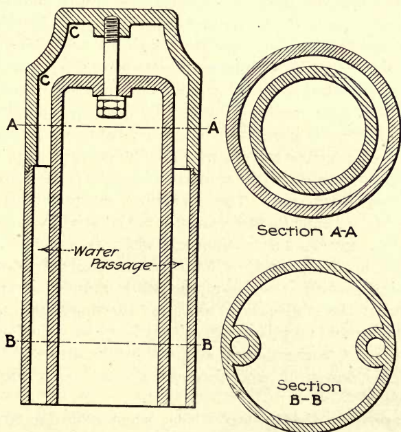
FIG. 57.—Standard Fuel Oil Diesel. Power piston.
