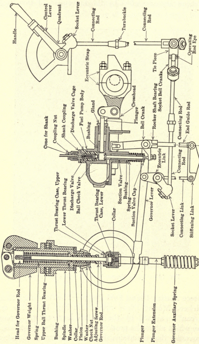
FIG. 144.—Nelseco marine Diesel fuel pump.
