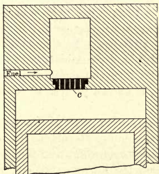
FIG. 232.—Muller modified ignition device.
