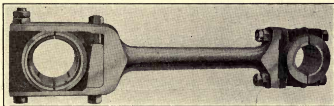
FIG. 44.—Snow Diesel connecting-rod.
