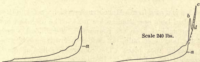
FIG. 344.—Fairbanks-Morse type Y indicator card. FIG. 345.—Fairbanks-Morse oil engine kerosene fuel.
