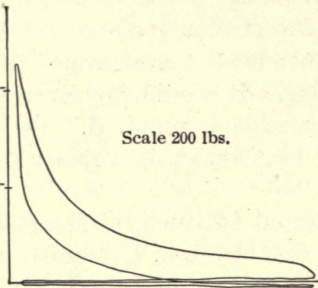
FIG. 240.—Full load indicator card Price engine.
