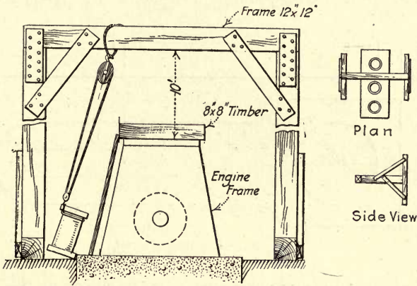
FIG. 24A.—Scaffolding.
