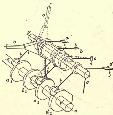
FIG. 82.—Busch-Sulzer Diesel rocker layout.
