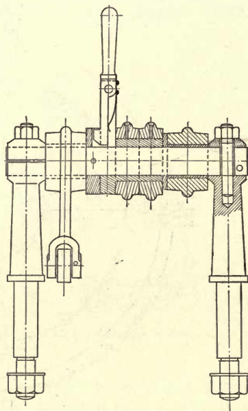
FIG. 83.—Lever shaft.
