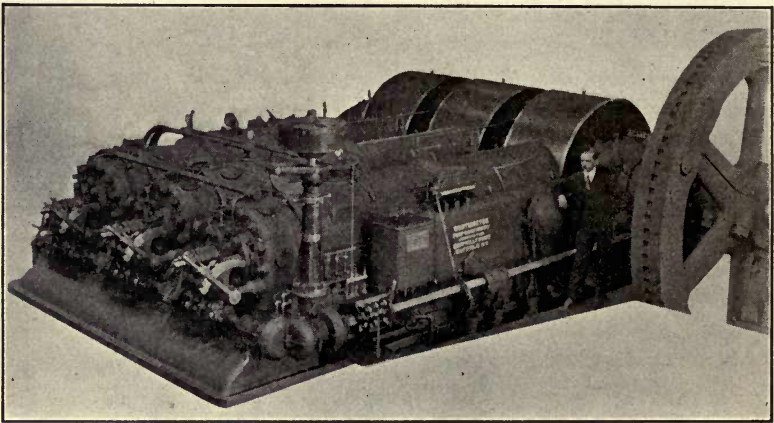
FIG. 11.—Snow four-stroke-cycle Diesel.
