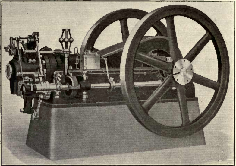
FIG. 222.—Midwest-type V.D.H. horizontal four-stroke-cycle semi-Diesel engine.
