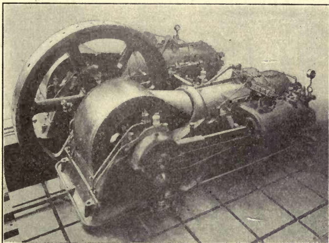
FIG. 16A.—Standard Fuel Oil twin cylinder two-stroke-cycle Diesel.
