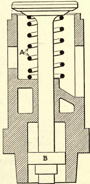
FIG. 105.—Regrinding valves.
