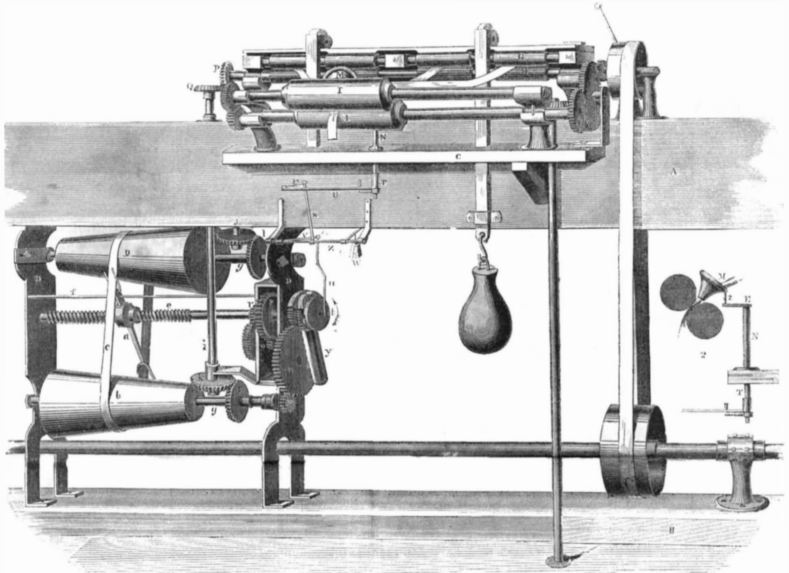
IMPROVED DRAWING REGULATOR.---Fig. 1.
