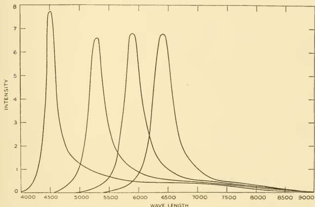
FIG. 1.—Energy transmission curves for 6-inch Christiansen filters.
