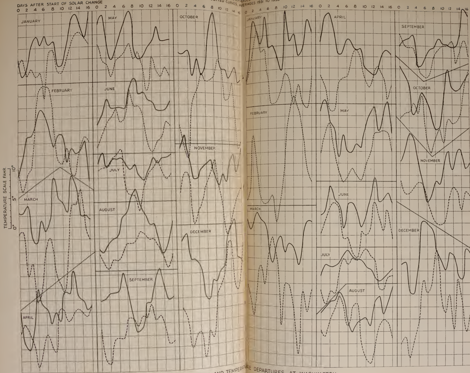
FIG. 4.—Temperature effects following solar changes 1924 to 1930 compared to those 1931 to 1935.
