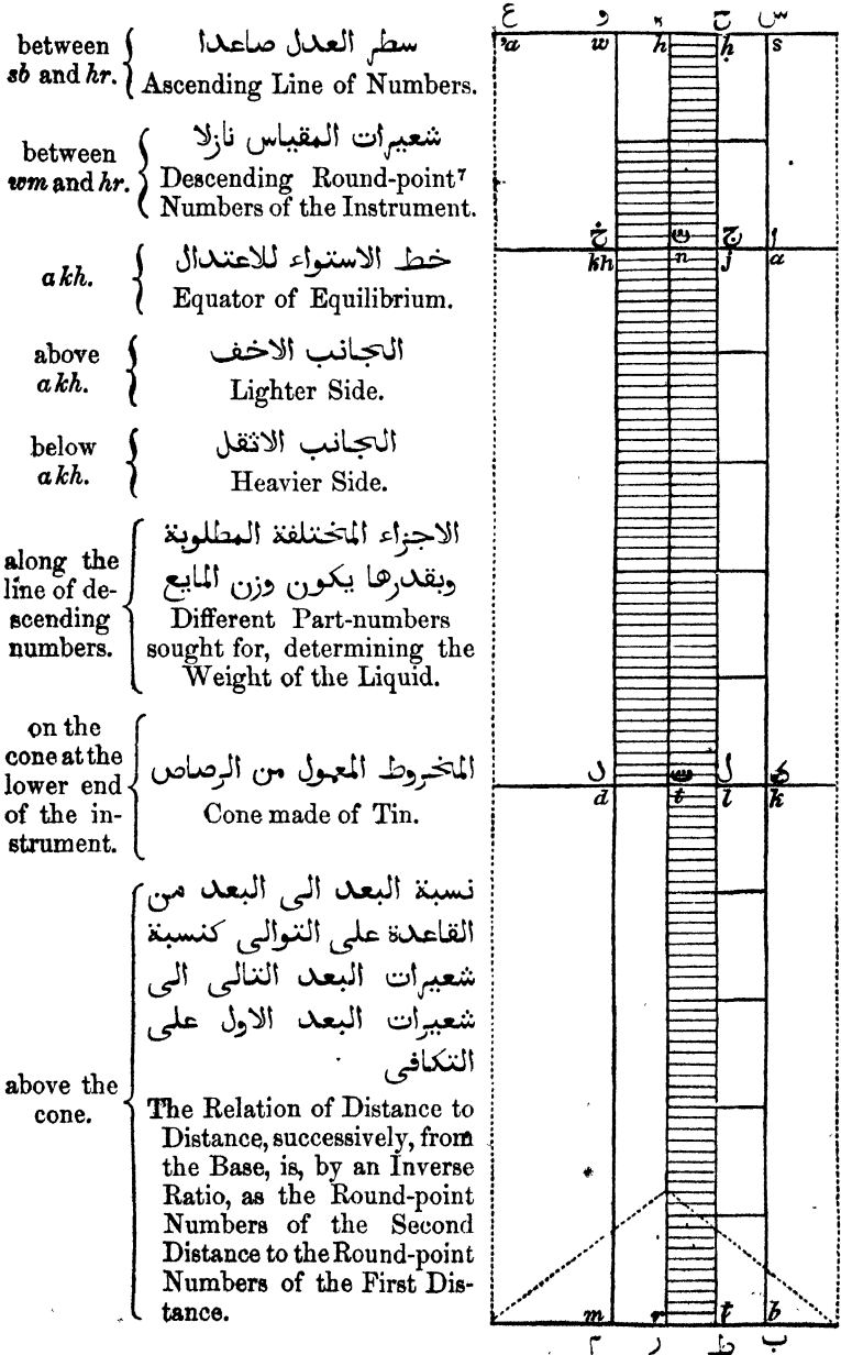
Form of Pappus the Greek's Instrument for Measuring Liquids. 6
