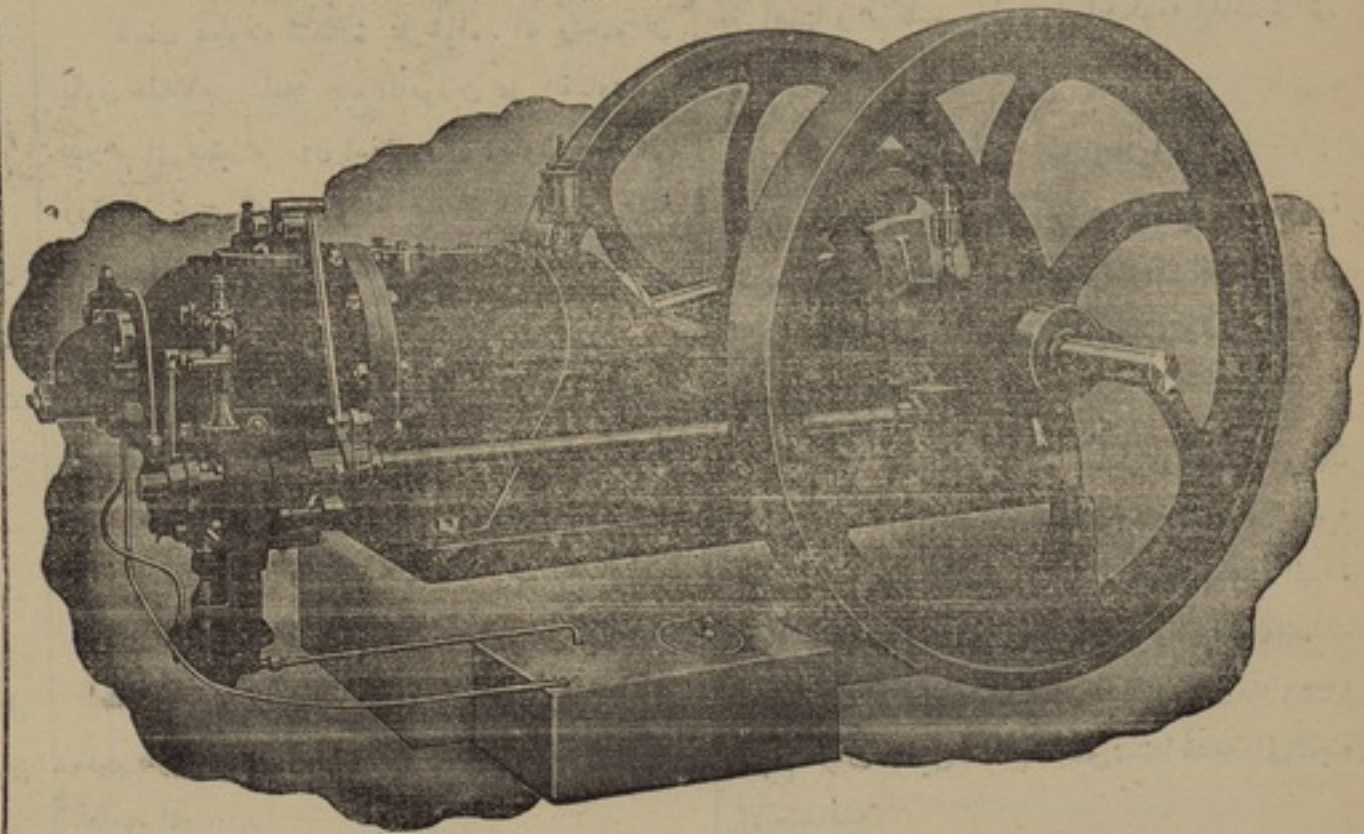
THE VICTORY CRUDE OIL ENGINE
