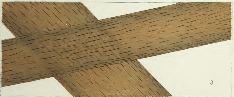
3. Human Hair.
