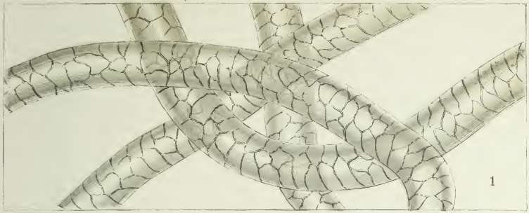
1. Wool.
