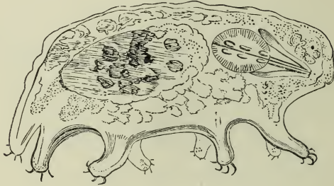
No. 23.—Water-Bear.
