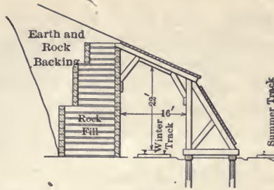
TYPICAL SHED Fig.94
