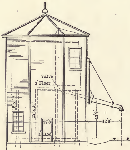
Fig. 208c. Water Tanks.
