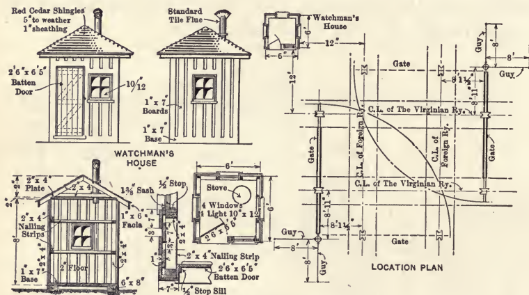
Fig. 109. Watchman's Cabin.
