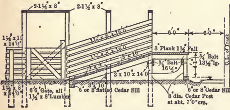
SECTION THRO' LOADING CHUTES
