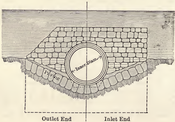
PIPE CULVERTS
