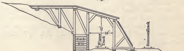
TOE CRIB AND GALLERY Fig.98
