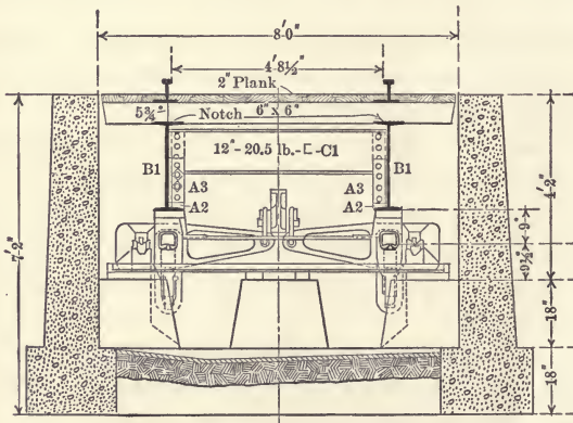
Fig. 195. Cross Section, C. P. R. Track Scale.
