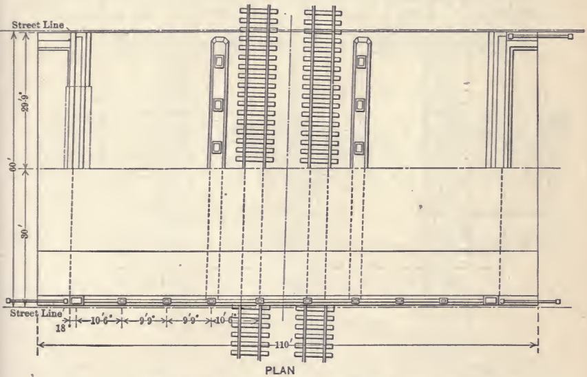
Fig. 28. Arsenal St. Bridge at St. Louis.
