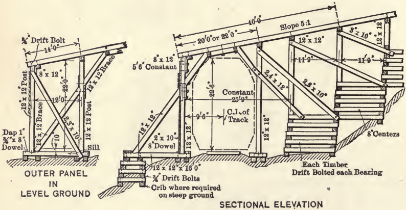
Fig. 99. Great Northern Snow Shed.
