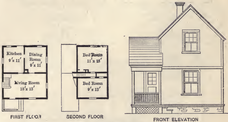
Fig. 167. Single Section House.
