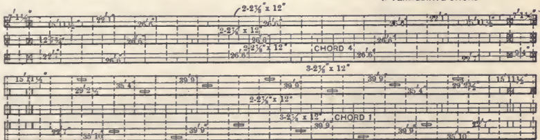
BOTTOM AND TOP CHORD FRAMING PLANS
