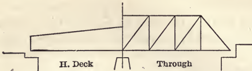
FIG. 27. Half Deck and Through Drawbridges.
