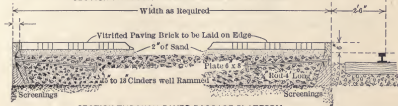
Fig. 189. P. R. R. Station Platforms.
