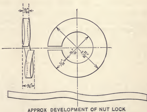
APPROX DEVELOPMENT OF NUT LOCK
