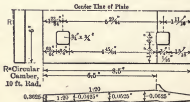
Fig. 62. Lundie Tie Plate.
