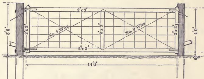
Fig. 84. Swing Wire Gate (Wood Frame).
