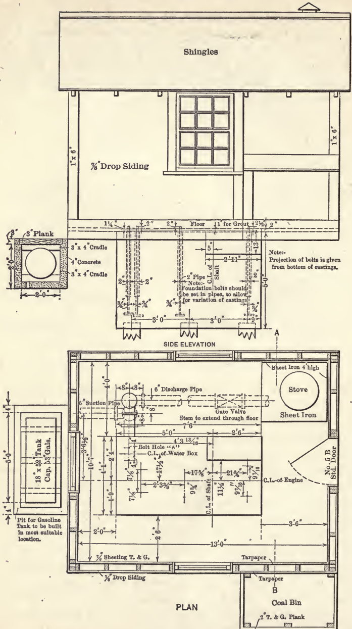
Fig. 217. C. L. O. & W. Ry. Pump House.
