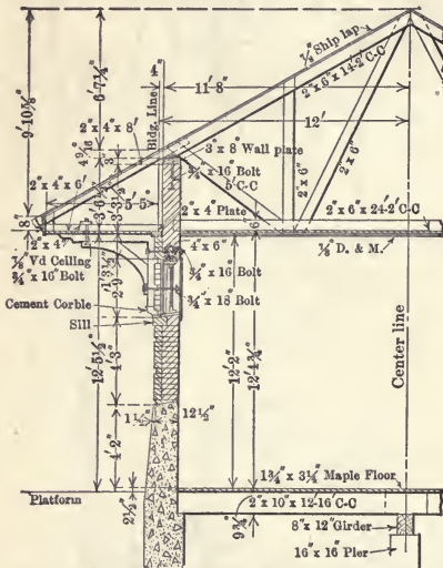
SECTION THRU BAGGAGE & EXPRESS ROOMS Fig. 132.
