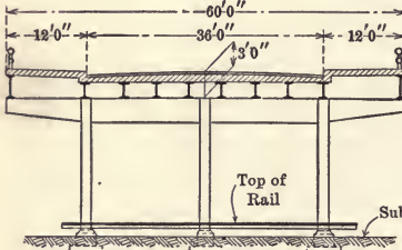
CROSS-SECTION, 60'-0" STREET, 36'-0" ROADWAY TYPES F2 - F4
