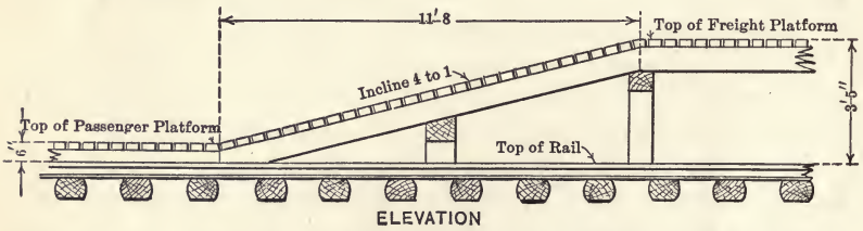
Fig. 191. P. R. R. Standard Section through Freight and Transfer Platform.
