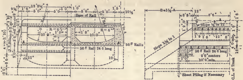
10 FT. DOUBLE CULVERT
