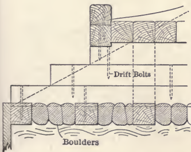
Fig. 41. Wood Box Culverts.
