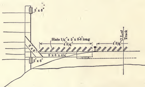
Fig. 87. Wood Cattle Guard.
