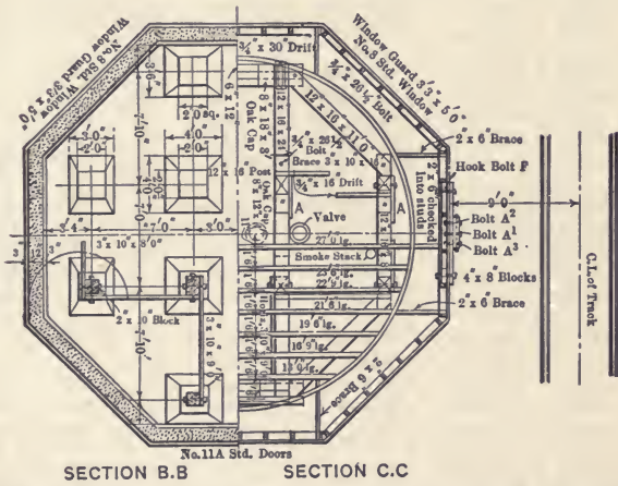
Fig. 209 (Continued). C. P. R. Standard Water Tank. Capacity 50,000 U. S. Gallons.
