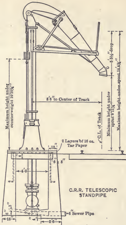
C. P. R. Telescopic Standpipe.
