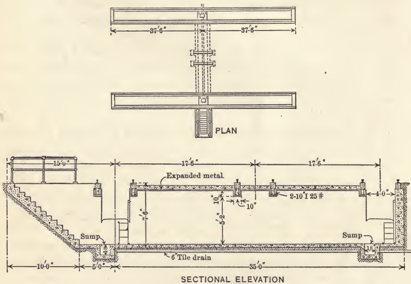
Fig. 245. Plan and Section of Inspection Pits, C. & A.
