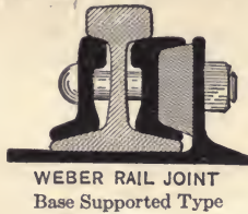
ELEMENTS OF SOME RAIL JOINTS. A. S. C. E. and other Rail
