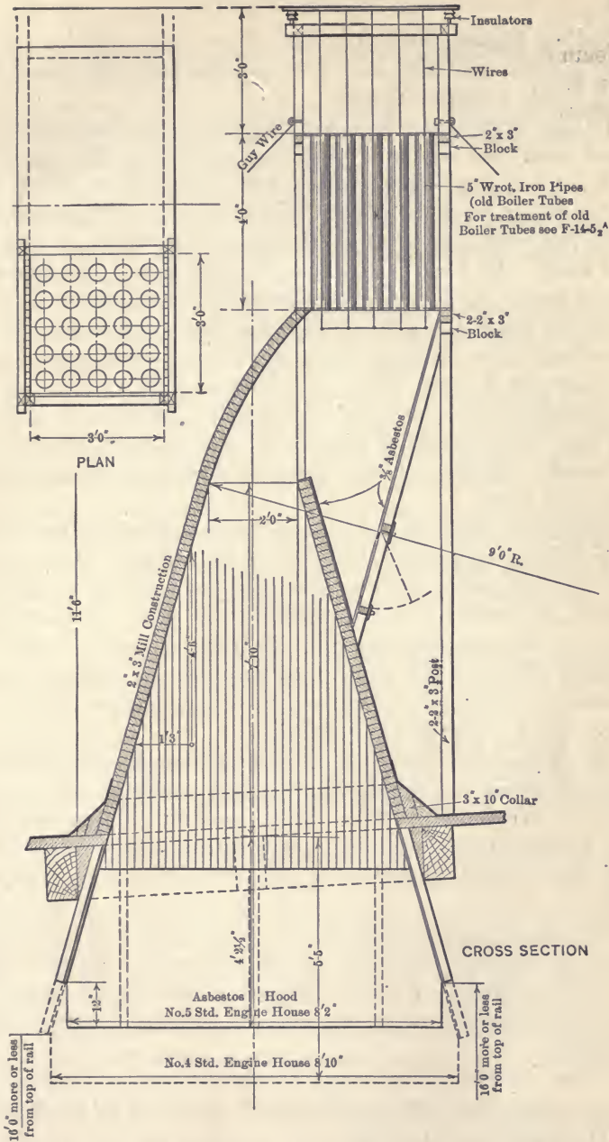
Fig. 243d. Electric Precipitation Mill Type Smoke Jack, Cross Section.
