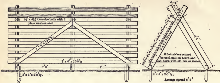
Fig. 92. Portable Snow Fence.
