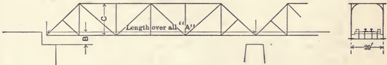
Fig. 26. Through Lattice Riveted Trusses.
