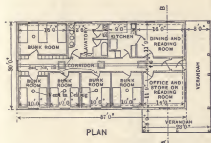
Fig. 173. C. P. R. No. 1 Bunk House.
