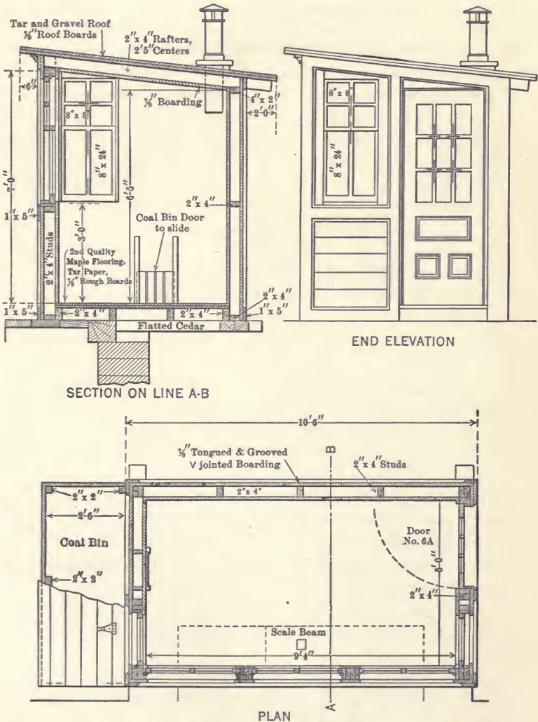
Fig. 197. Scale Shelter
