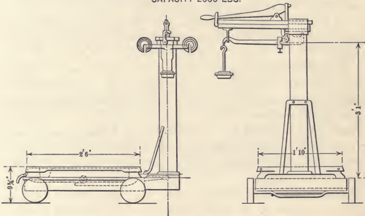
Fig. 192a. Portable Platform Scale with Drop Lever.
