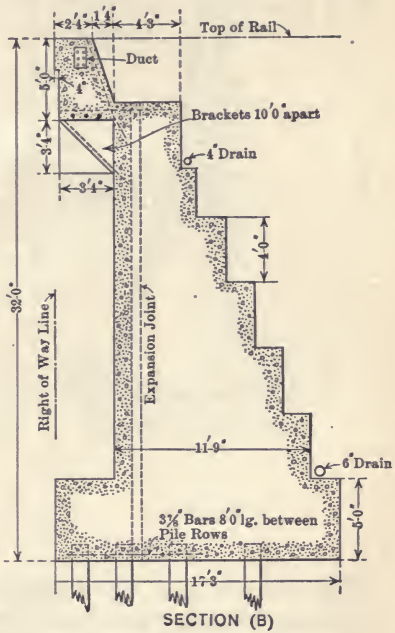
SECTION (B)
