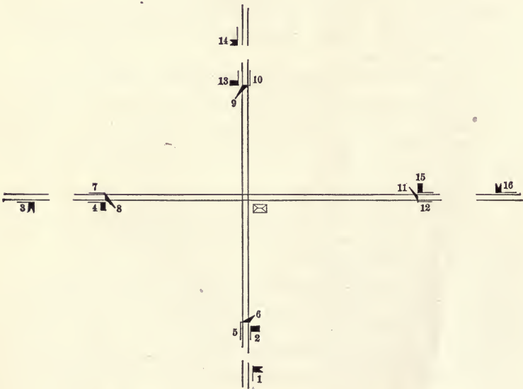
Fig. 80. Interlocked Single-track Lay-out.
