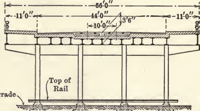
CROSS-SECTION, 66'-0" STREET, 44'-0" ROADWAY TYPES F6
