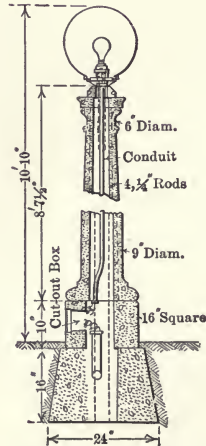
Fig. 152b. Reinforced Concrete, E. L. Standard.
