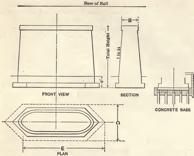
Fig. 19. Bridge Piers.
