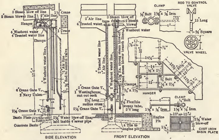
Fig. 242. Details, 35-stall Engine House, A. T. & S. F. Ry.
