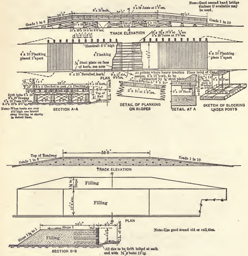
Fig. 192. C. P. R. Grain Loading Platforms.
