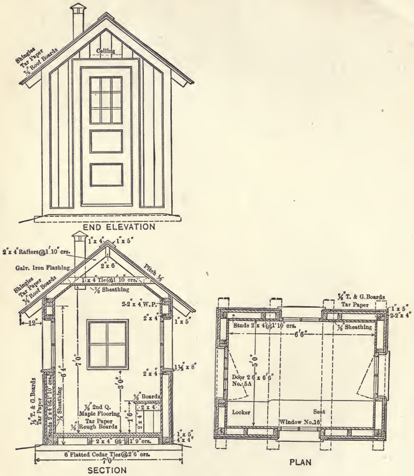
Fig. 178. Watchman's Cabin.
