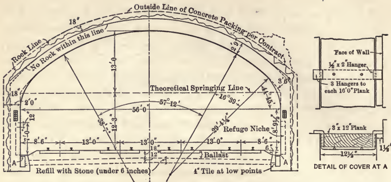
Fig. 2. Cross Section Four-track Tunnel Bergen Hill Tunnels, Erie Ry.
