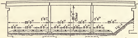
HALF ELEVATION, 6 TRACK SCHEME TYPES F6
