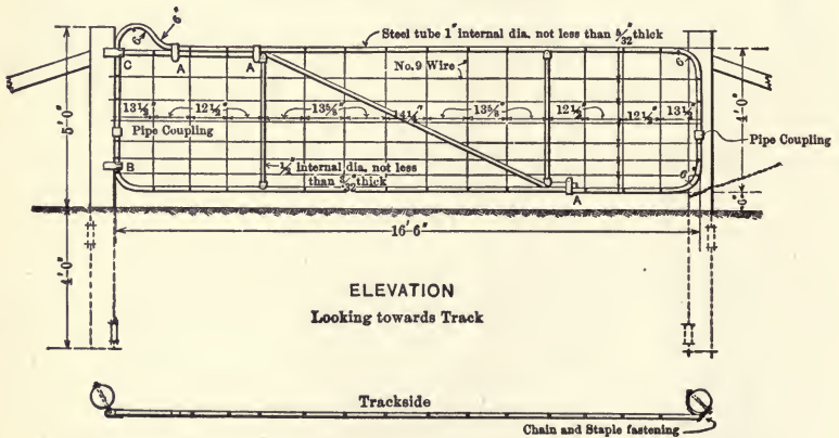
Fig. 85. Steel Gate.
