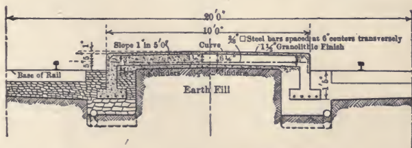
Fig. 159. C. P. R. Baggage Platform.
