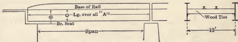
Fig. 24. Half Deck Plate Girders, 13 ft. centers.
