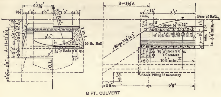
8 FT. CULVERT Fig. 45.
