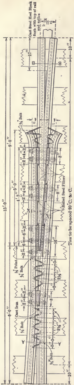
No. 15 FROG
