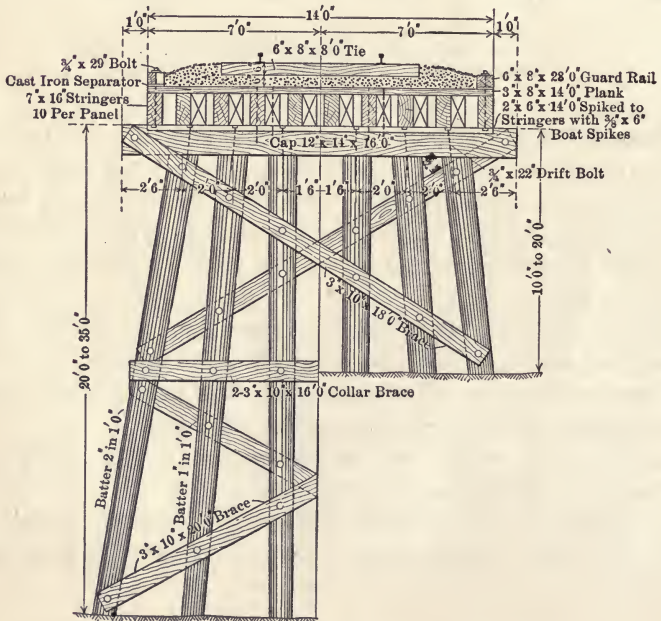
Fig. 35. Ballast Floor Trestle, Ill. Cent. R.R.
