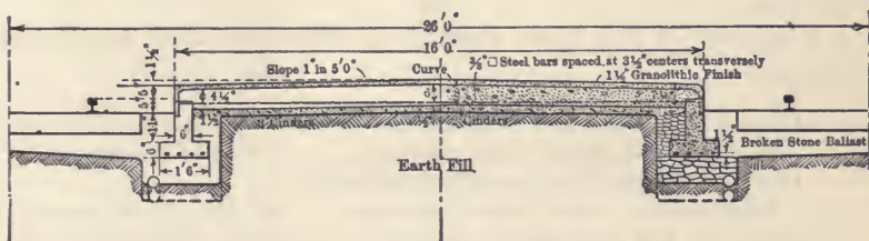
Fig. 158. C. P. R. Passenger Platform.
