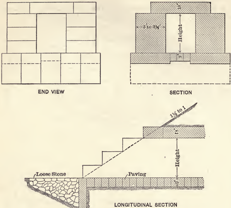
Fig. 42. Stone Box Culverts.
