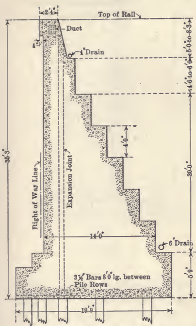
SECTION (A)
