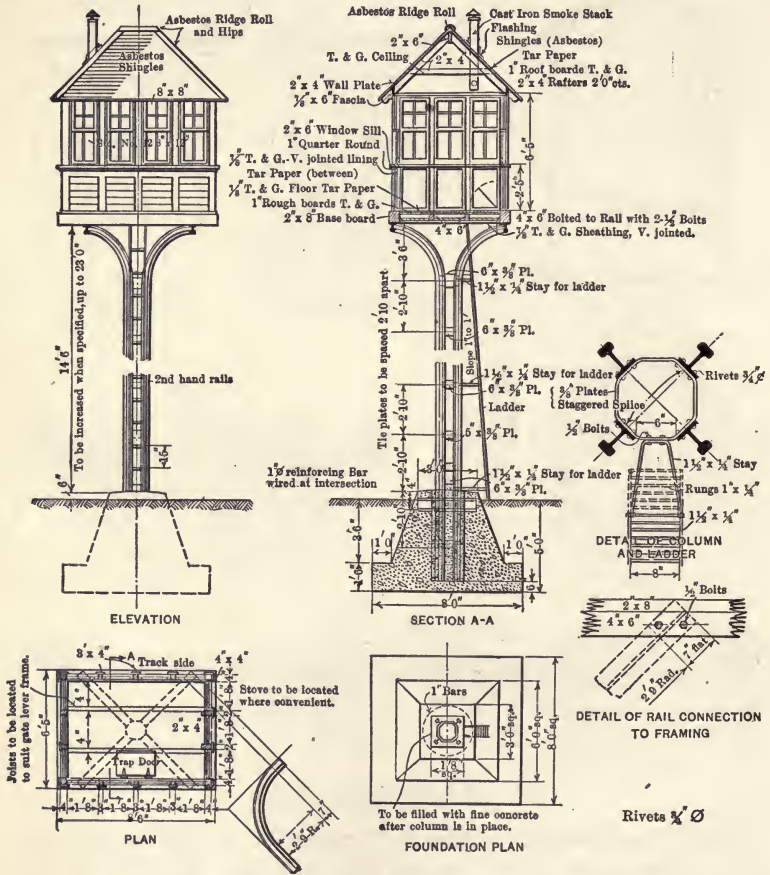
Fig. 111. C. P. R. Tower for Crossing Gates.
