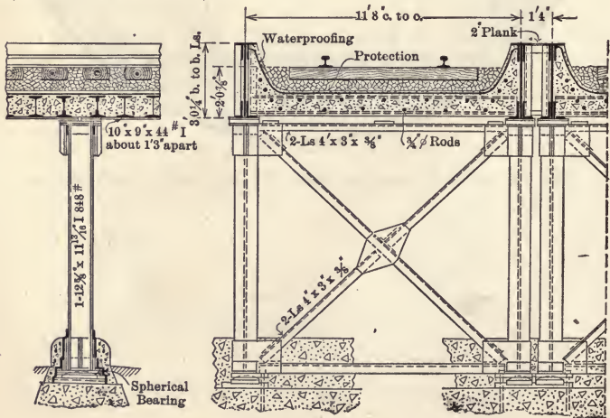
Fig. 15. Shallow Floor.
