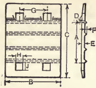
Typical 4 Hole.
