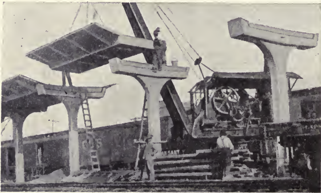
Fig. 161a. Placing Roof Slabs.
