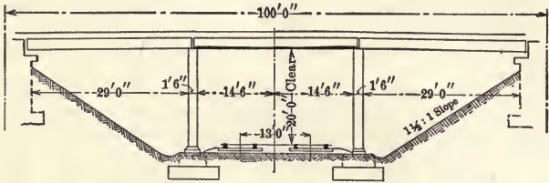
TYPES F2, ELEVATION, 2 TRACK SCHEME
