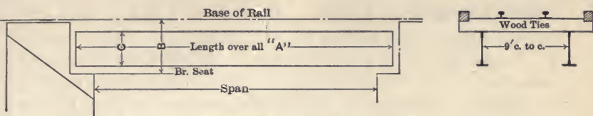
Fig. 23. Deck Plate Girders, 9' 0" centers.
