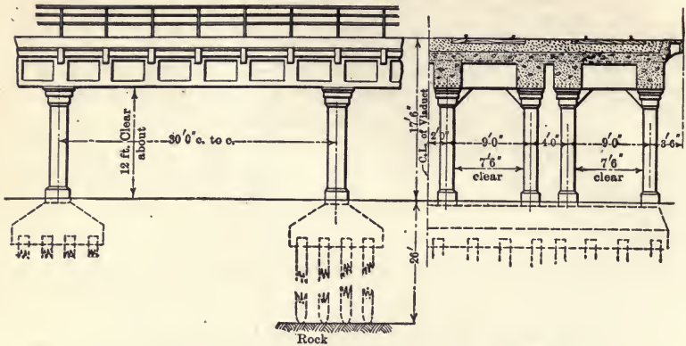
"A" — Typical Section, Reinforced Concrete (30-Ft. Spans).
