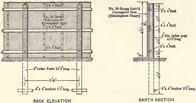
Fig. 93. Picket Fence.
