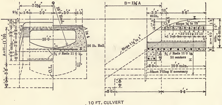
10 FT. CULVERT Fig. 46.
