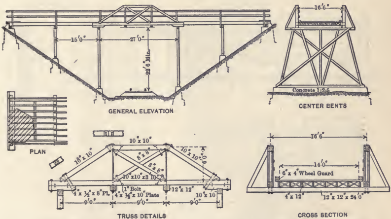
Fig. 104. Overhead Farm Crossing.
