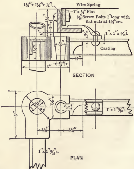
Fig. 174. Two Tier Iron Bunks.
