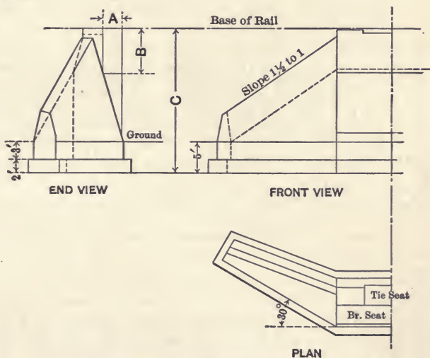
Fig. 18. Bridge Abutments.
