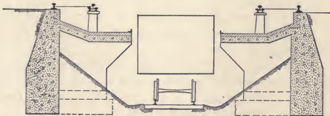
Fig. 253. Depressed Ash Car Track.
