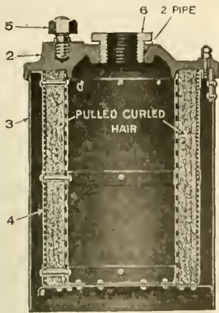
SECTION VIEW OF STRAINER.
