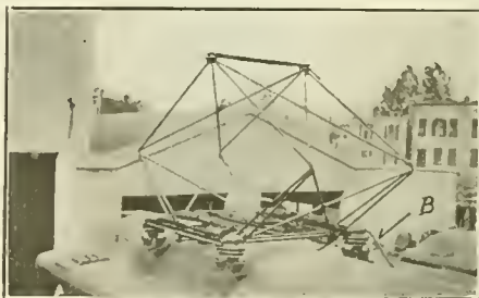
FIG. 6. PANTOGRAPH RAISED.
