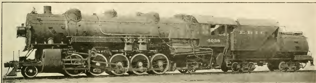
2-10-2 TYPE LOCOMOTIVE FOR THE ERIE RAILROAD.
