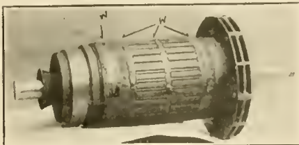
FIG. 30. COMPLETE ARMATURE.
