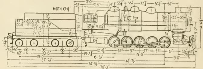
FIG. 4. HUMP YARD ENGINE.
