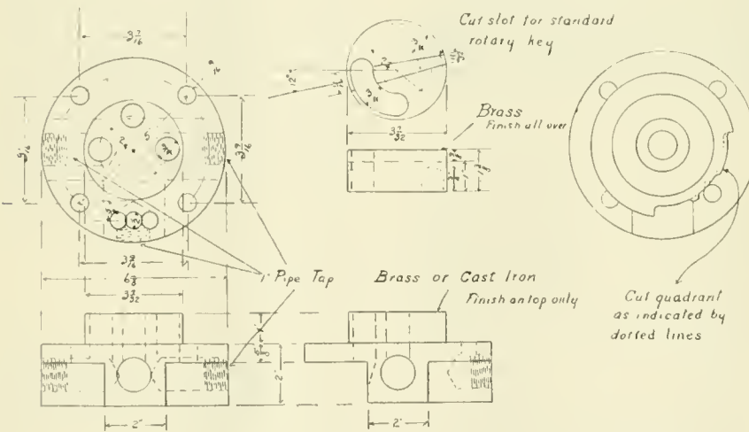
DETAILS OF THREE WAY COCK FOR OPERATING AIR PASSES.
