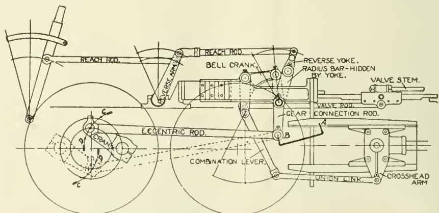
BAKER VALVE GEAR.
