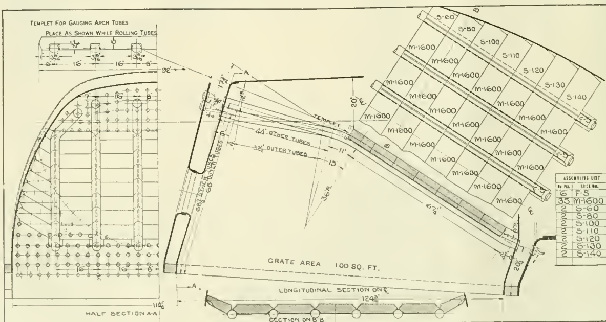
TYPICAL ARCH FOR LARGE MIKADOS, SANTA FE TYPES AND MALLET.
