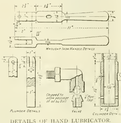
DETAILS OF HAND LUBRICATOR.
