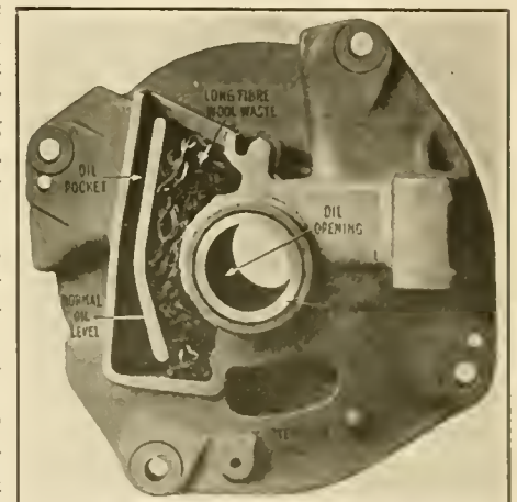
FIG. 26. HOUSINGS WITH SECTIONAL ARMATURE BEARING AND OIL WELL.
