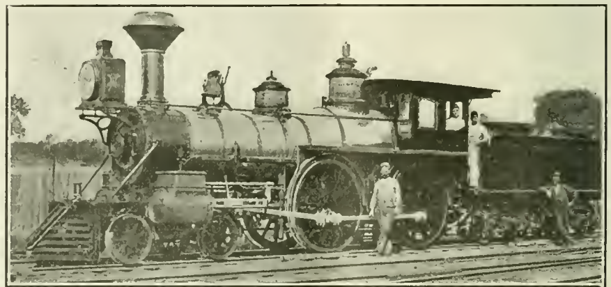
LOCOMOTIVE NO. 58, BOSTON & MAINE RAILROAD.
