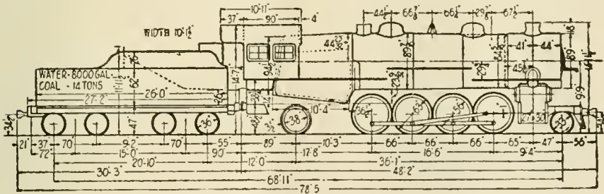
FIG. 5. OUTLINE OF MIKADO OR 2-8-2 ROAD ENGINE.
