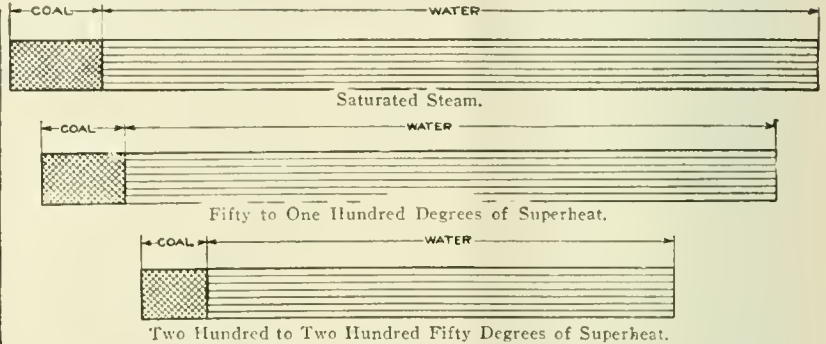
FIG. 2.—COMPARISON OF COAL AND WATER CONSUMPTION OF SATURATED AND SUPERHEATED STEAM LOCOMOTIVES OF THE SAME TRACTIVE POWER.
