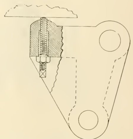
REPAIRS ON DOUBLE LEAF BASCULE BRIDGE.
