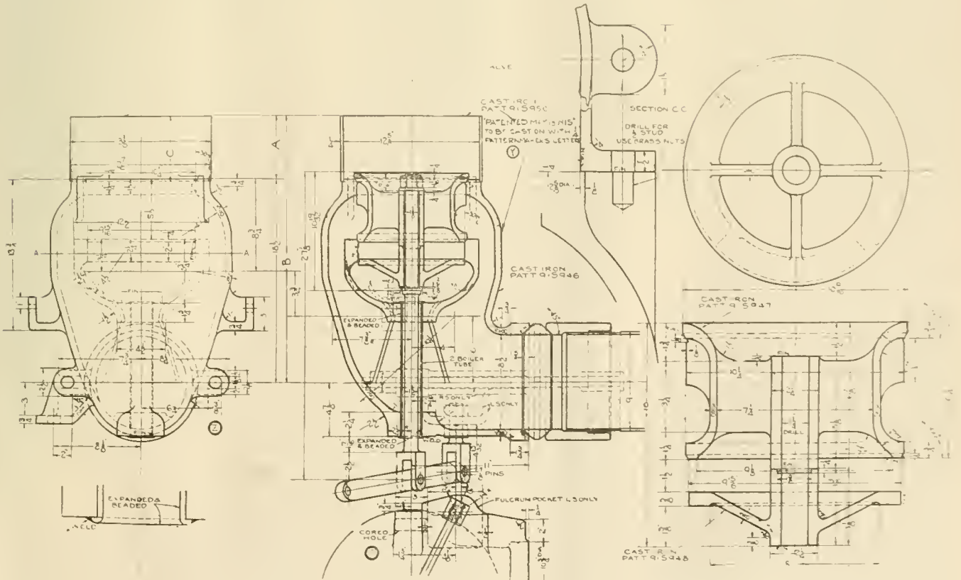
DETAILS OF THE WOODARD THROTTLE VALVE.
