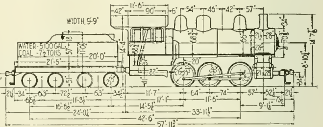
FIG. 2. SIX-WHEEL SWITCHER, STRAIGHT TENDER.
