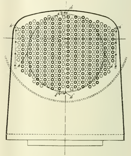
LOCATION OF FLUES. LOCO. CLASS N-2.
