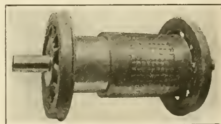
NEW YORK CENTRAL GEARLESS MOTOR.
