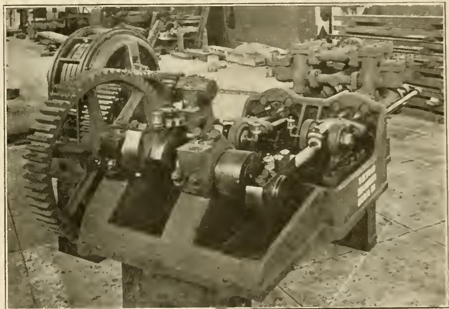
TYPE OF HYDRAULIC PUMPS FOR THE PUGET SOUND NAVY YARD.
