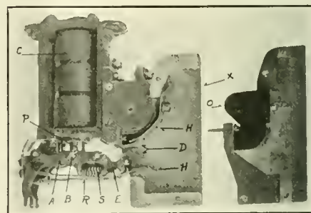
FIG. 19. VIEW OF CONTACTOR WITH ARC SIDE REMOVED.
