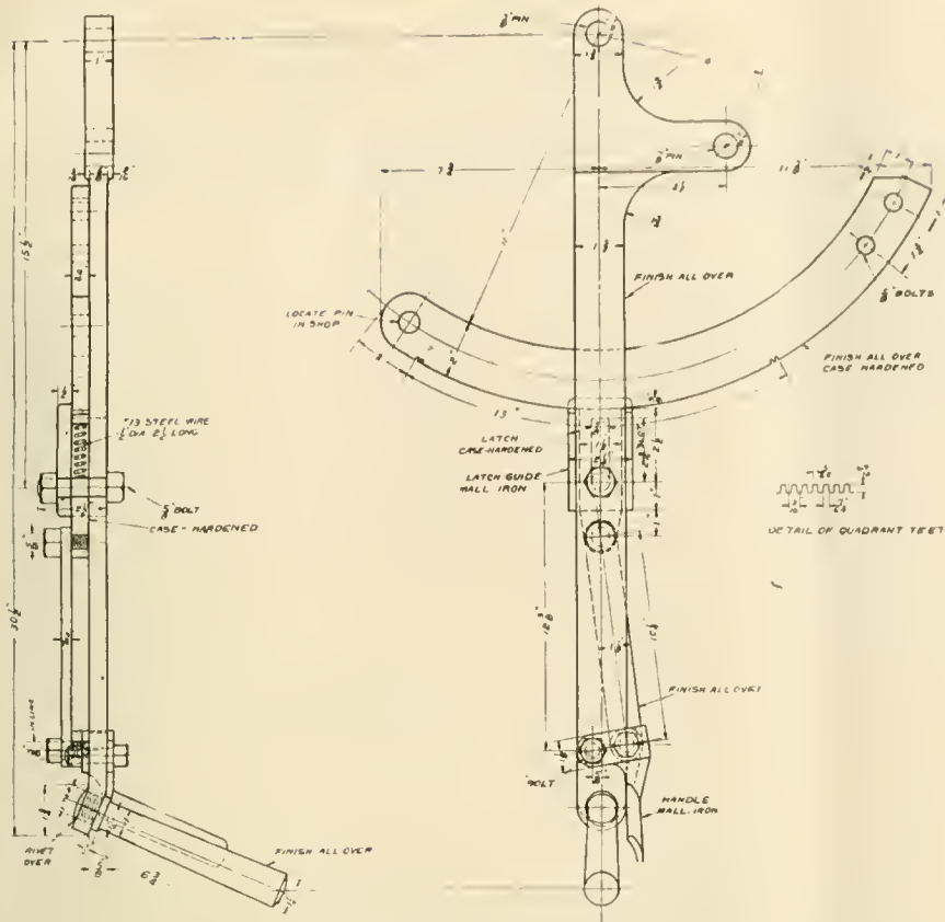
DETAILS OF WOODARD THROTTLE LEVER.
