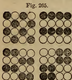
Illustration of Isomerism.
