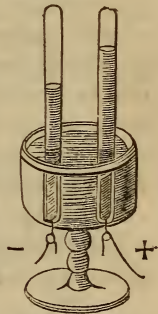
Electro-Decomposition.
