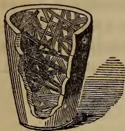
Sulphur crystals.
