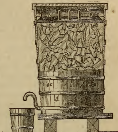
The Quick Vinegar Process.
