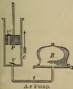
Air Pump.
