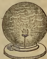
Combustion of Phosphorus.
