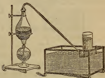
Making Oxygen.
