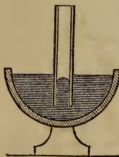
Convex liquid surface.
