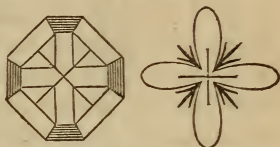
Four-membered symmetry.
