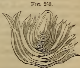
Starch Grains Ruptured by Boiling.
