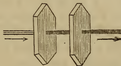
Polarization by Tourmalines.
