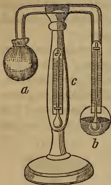
Daniell's Hygrometer.
