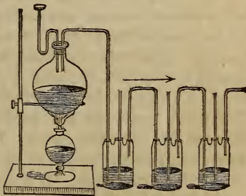
Woulfe's Bottles.
