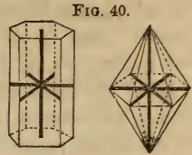
Rhombohedral system.
