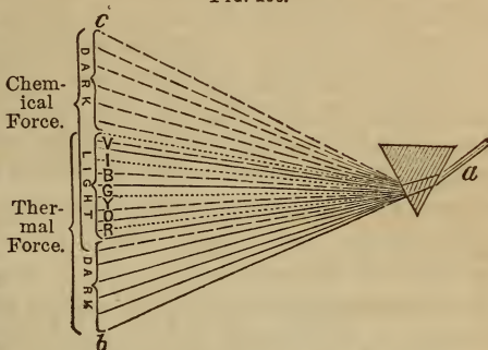
Distribution of the Forces of the Spectrum.
