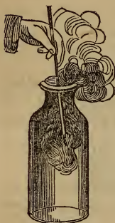
Combustion in Chlorine.
