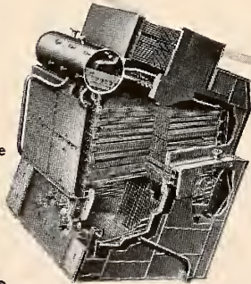
B & W Single-Uptake, Controlled- Superheat Boiler
