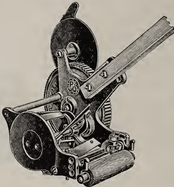
Pennsylvania Combined Trimmer
