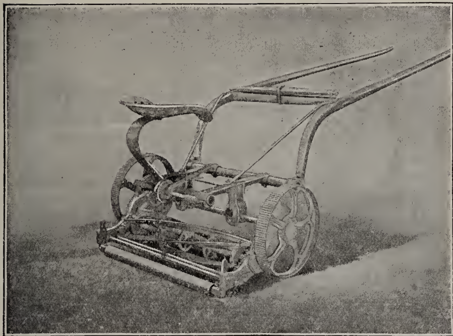
Pennsylvania Fairway Pony Mower
