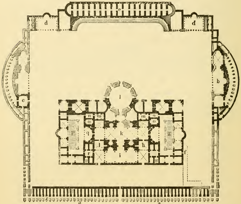
Ground-Plan of the Thermae of Caracalla.
