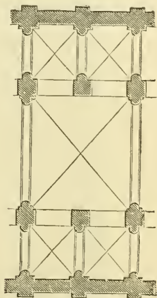
Part of the Ground-Plan of the Cathedral at Worms.
