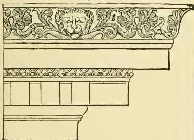
Ionic Cornice from the Temple of Minerva Polias at Priene.
