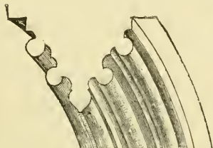
Profile of Rib-vaulting in Notre Dame at Paris.
