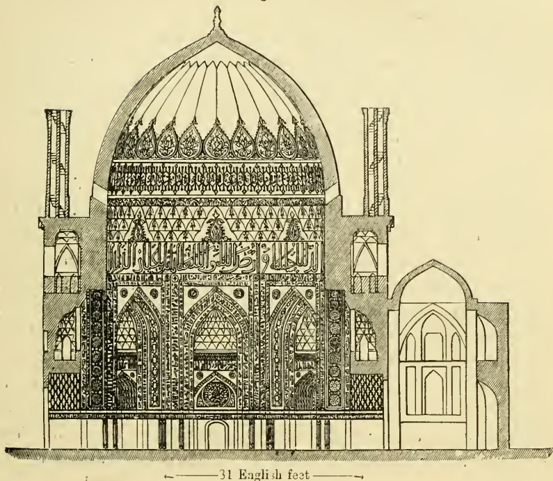
Section of the Tomb of Sultan Khodabendah (A. D. 1303--1316) at Sultanich.
