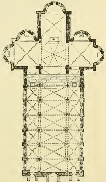
Ground-Plan of the Cathedral at Parma.
