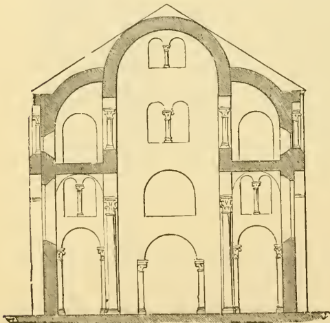
Gross Section of the Church of Notre-Dame du Port at Clermont.
