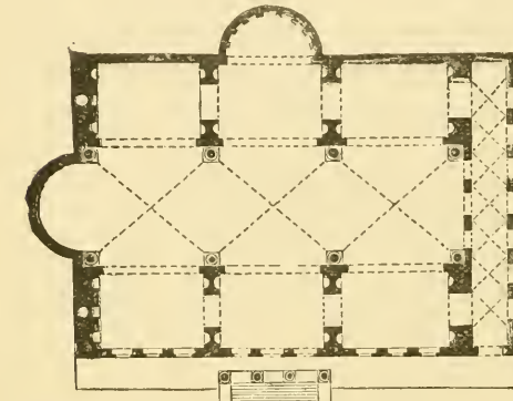
Basilica of Constantine at Rome.
