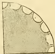
Plan of the Flutings of the Ionic and Corinthian Column. \frac{1}{4} scale.
