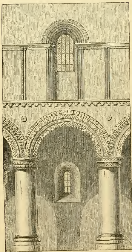
Part of the Nave of Steyning Church.
