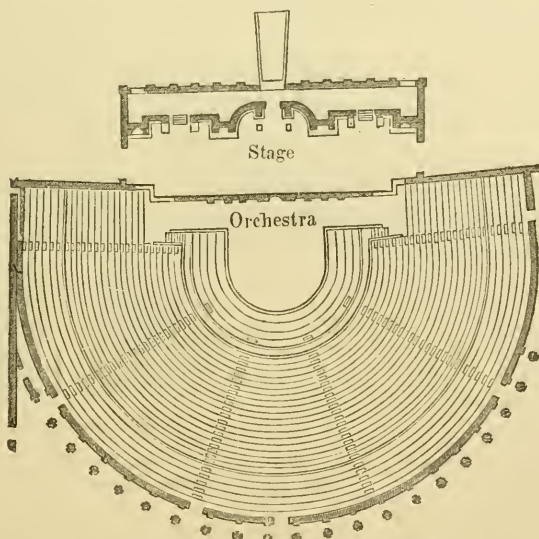
Ground-Plan of the Theatre at Pompeii.
