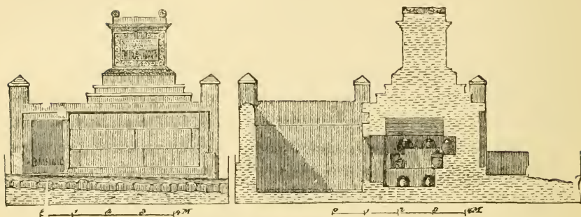
Tomb of Naevoleia Tyche at Pompeii.
