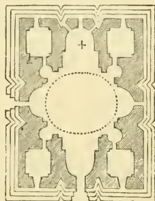
Ground-Plan of a Church at Vagharschabad.
