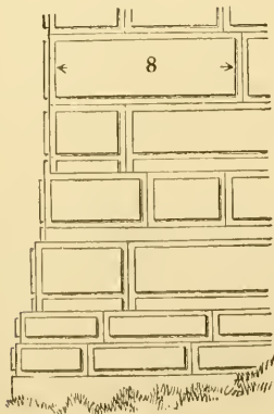
Elevation of Platform at Pasargadae.
