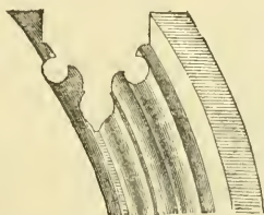
Profile of Rib-vaulting in Notre Dame at Paris.
