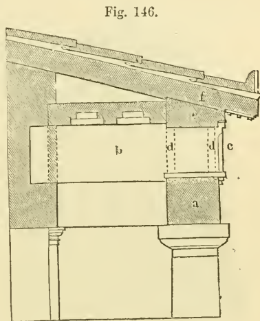
Construction of the Doric Entablature.
