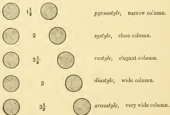
Diagram of Intercolumniation.
