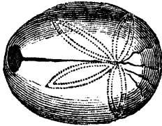
The Sea-egg (Spatangus ovum-marinum, BRISS.).
