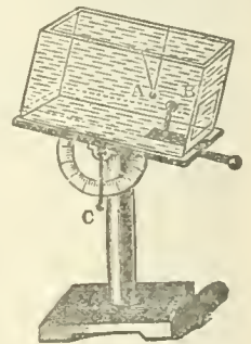
FIG. 6.—Sine Electrometer.
