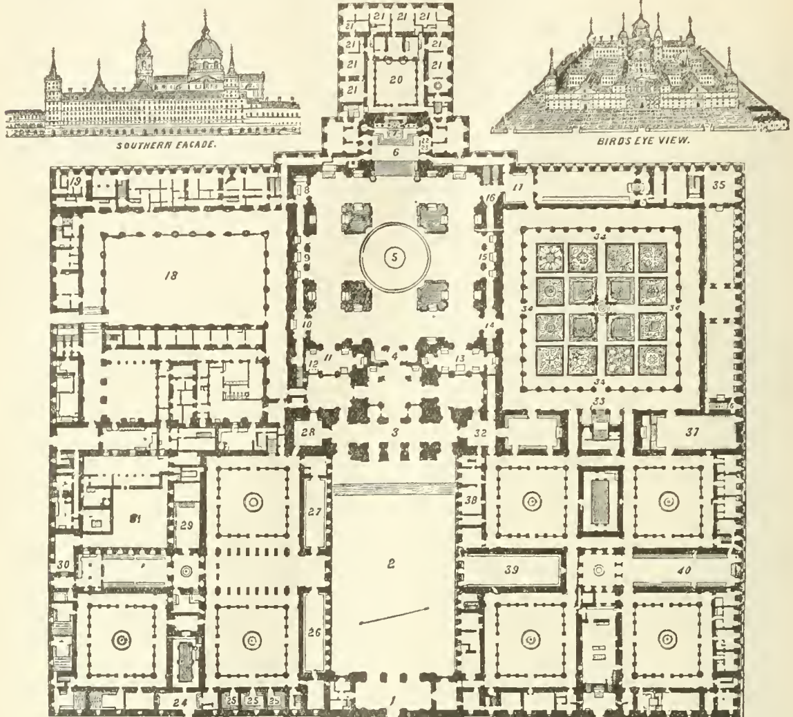
Views and Plan of the Escorial. 1
