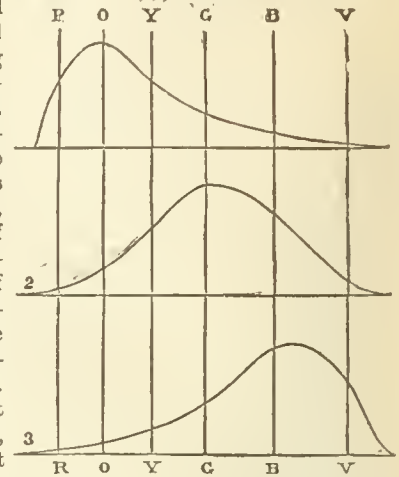
FIG. 22.—Diagram showing the irritability of the three kinds of retinal elements. 1. Red; 2. Green; 3. Violet. R, O, Y, G, B, V, initial letters of colours.
