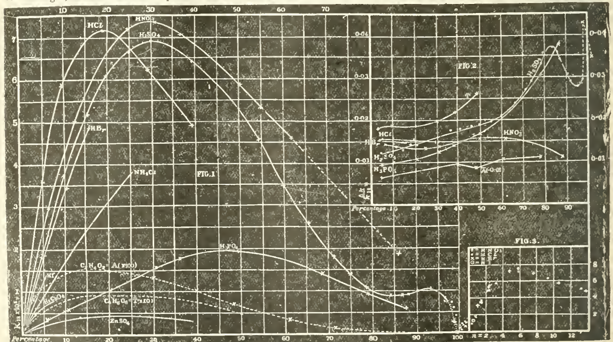
Diagram illustrating Electrical Conductivity.
