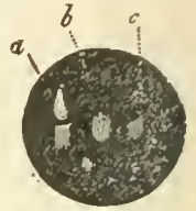
Fig. 12.—Reflected images in the Eye.
