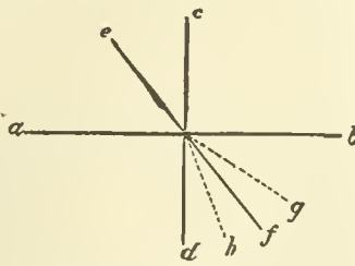
FIG. 1.—Refraction of Light.
