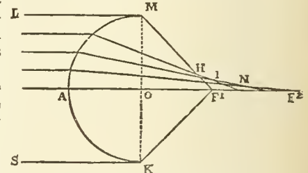
FIG. 7.—Spherical Aberration.
