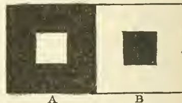
FIG. 16.—Illustrating the effect of irradiation.
