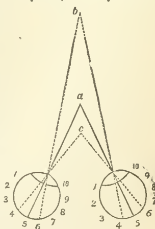
FIG. 25.—Diagram to illustrate phenomena of double vision. (Müller.)
