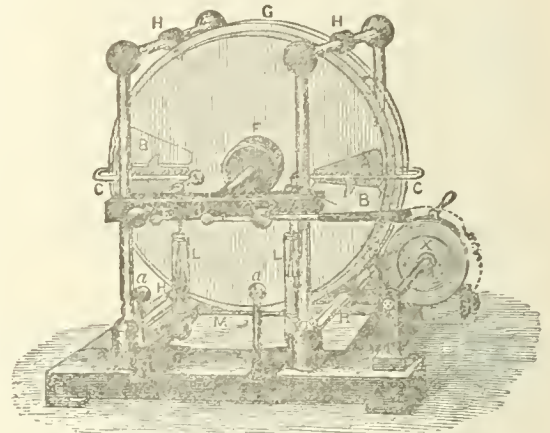
FIG. 58.—Holtz's machine.
