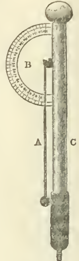
FIG. 5.—Henley's Electrometer.
