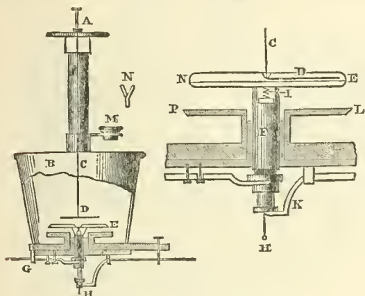
Fig. 7.—Dellman's Electrometer.
