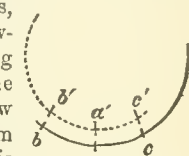
FIG. 24.—Diagram to illustrate the physiological relations of the two retinæ.
