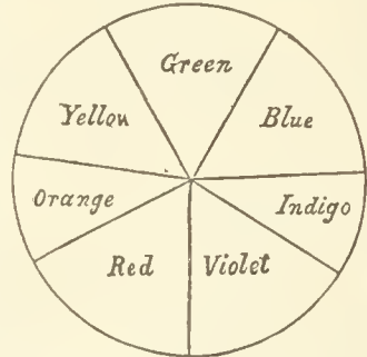
FIG. 20.—Diagram of the Colour Disc of Sir Isaac Newton.
