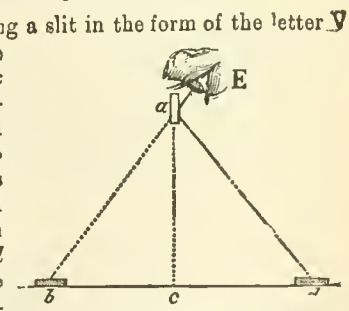
FIG. 19.—Diagram showing Lambert's method of mixing sensations of colour.
