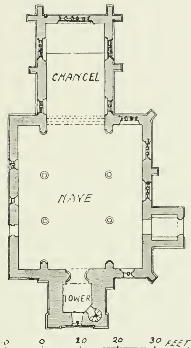
68. AYTON, RUTLAND
