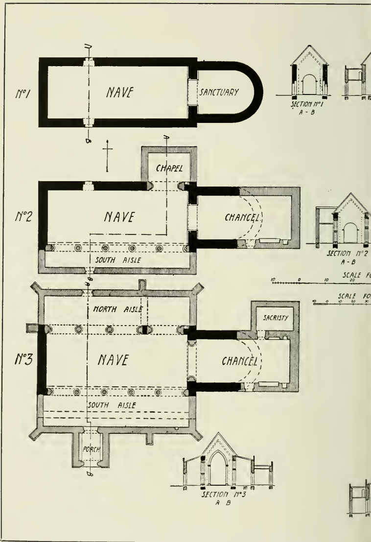
43. SERIES OF PLANS SHOWING TYPICAL CHANGES IN A NORMAL PARIS
