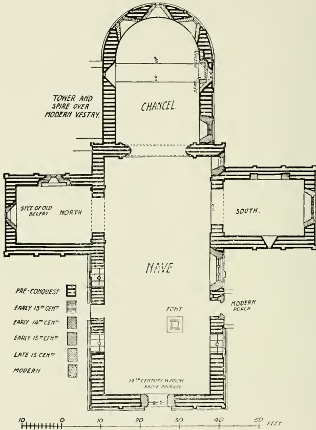
47. WORTH, SUSSEX
