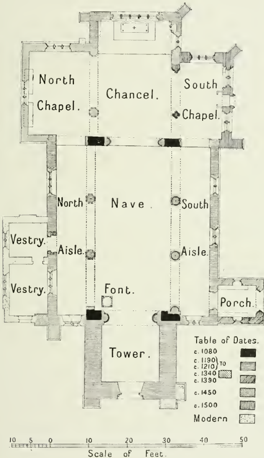
70. MERSTHAM, SURREY
