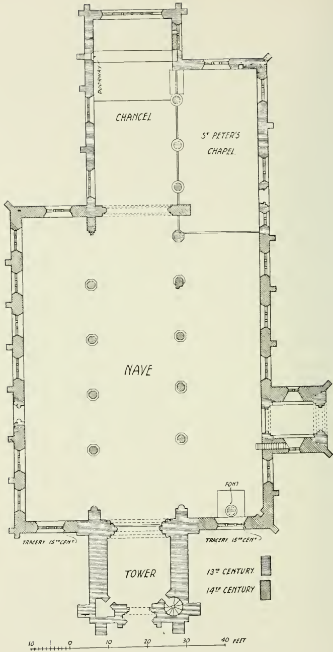
69. RAUNDS, NORTHANTS
