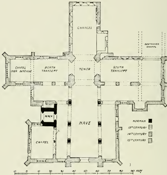
42. WITNEY, OXFORDSHIRE
